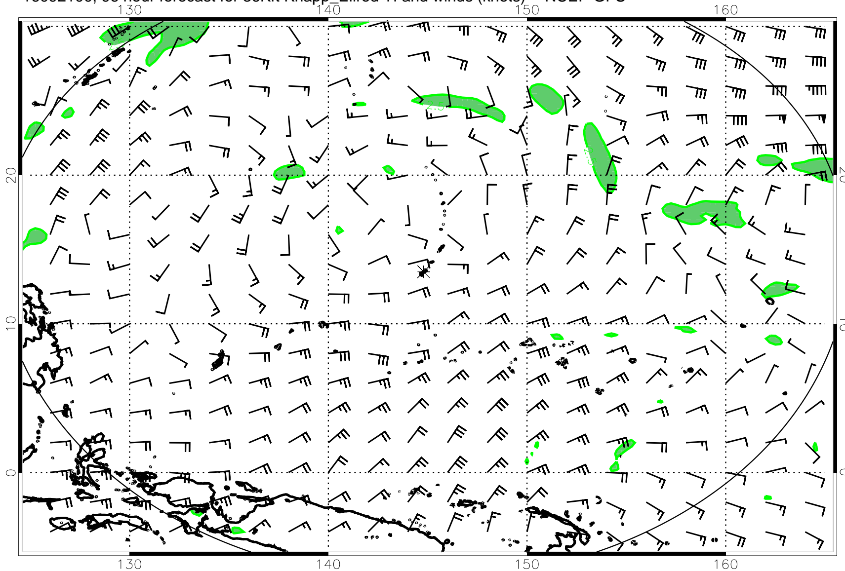
16092100, 96 hour forecast for 36Kft Knapp_Ellrod TI and winds (knots) -- NCEP GFS
