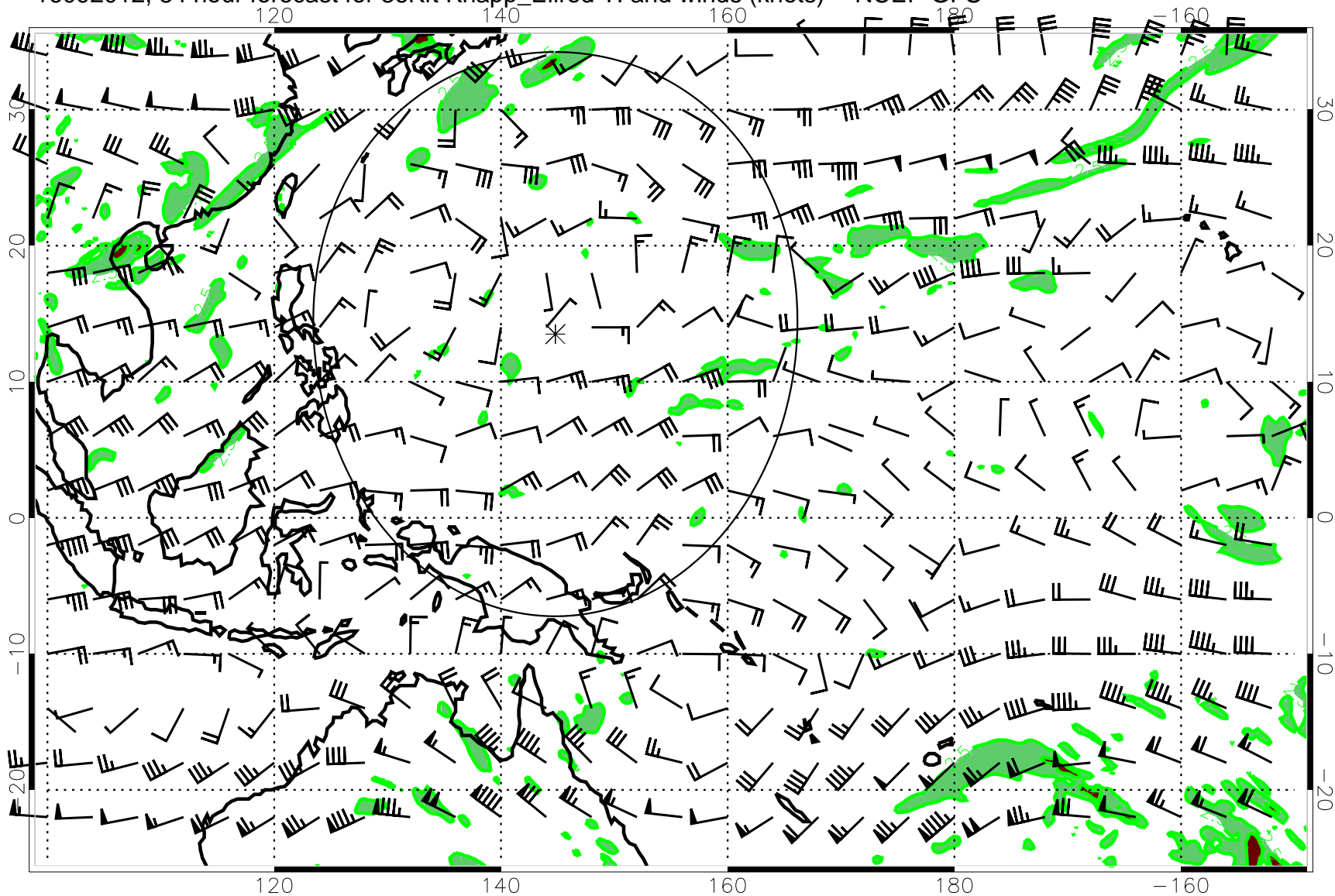
16092012, 84 hour forecast for 36Kft Knapp_Ellrod TI and winds (knots) -- NCEP GFS
