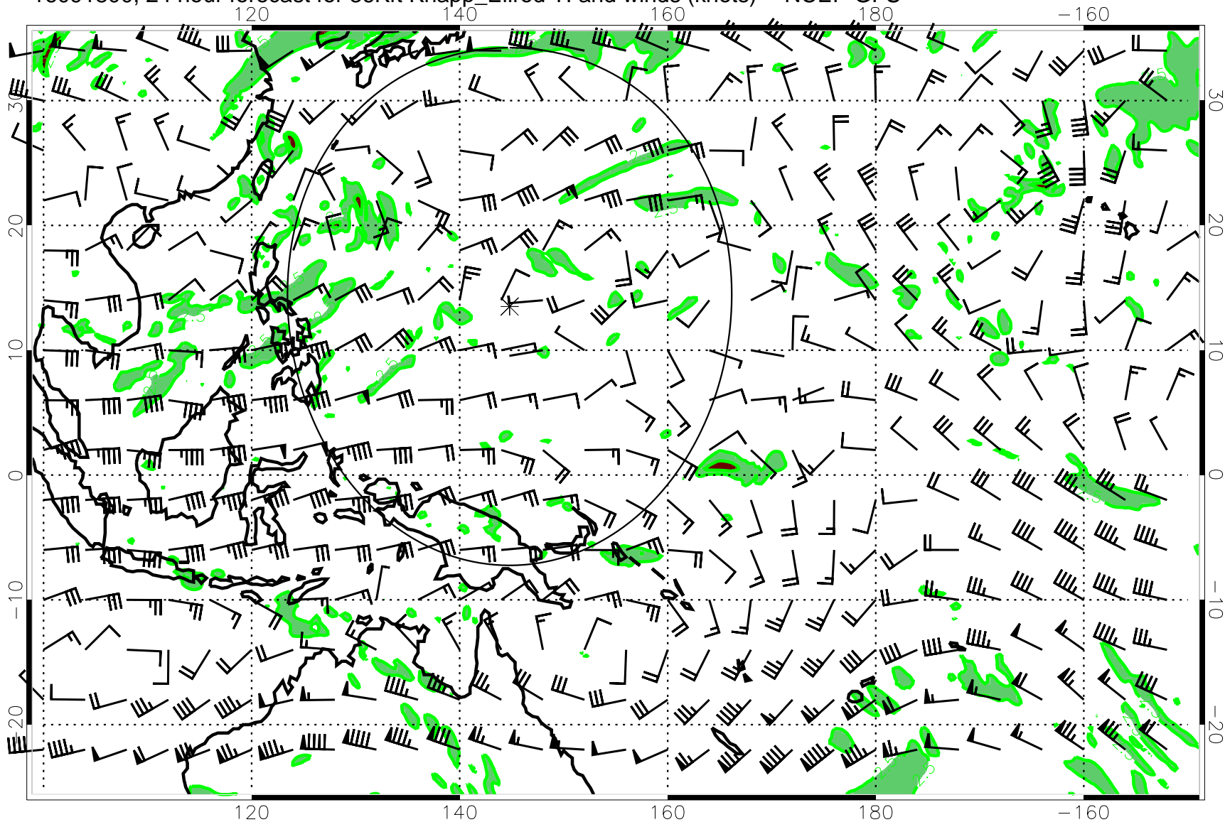
16091800, 24 hour forecast for 36Kft Knapp_Ellrod TI and winds (knots) -- NCEP GFS
