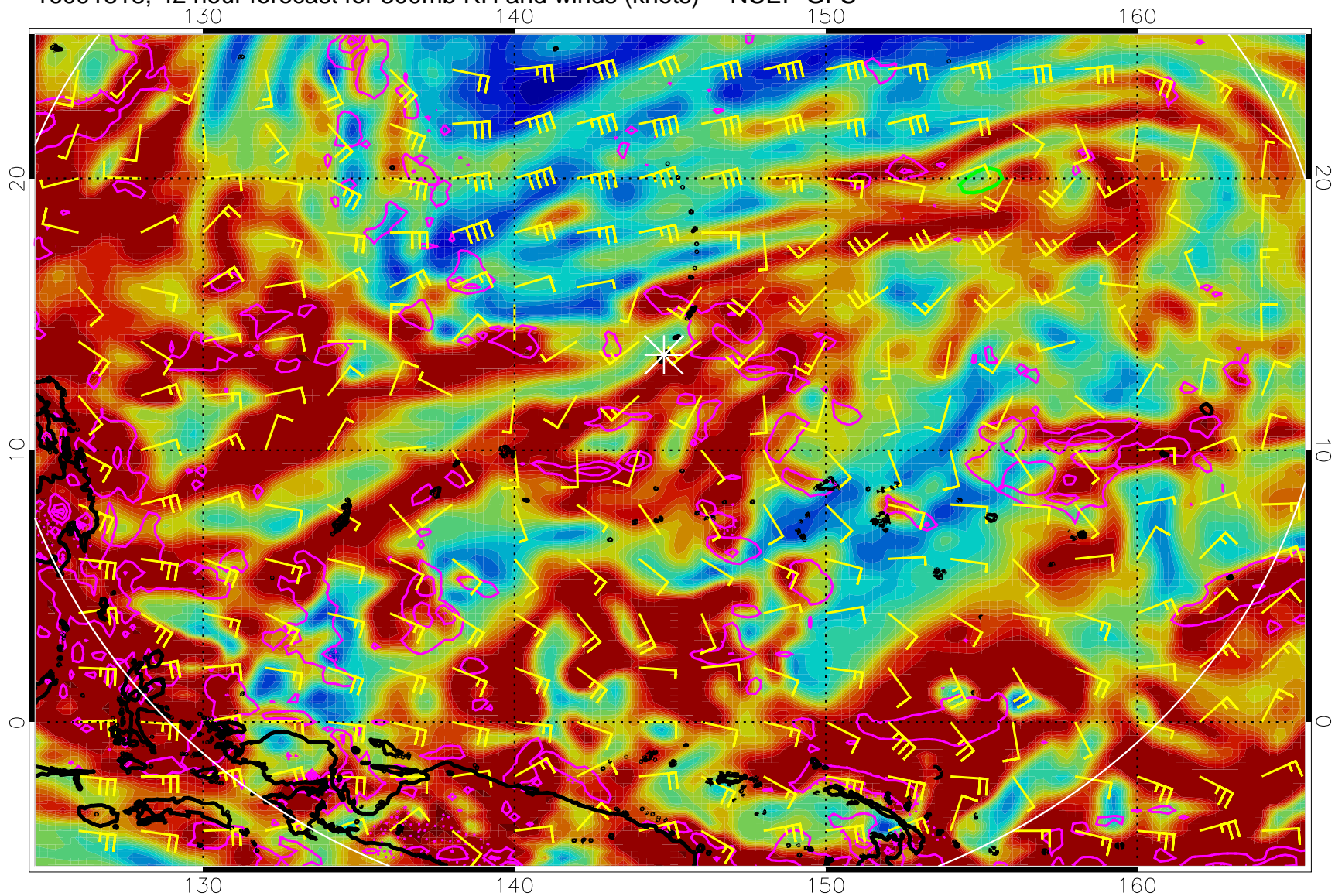
16091818, 42 hour forecast for 300mb RH and winds (knots) -- NCEP GFS
