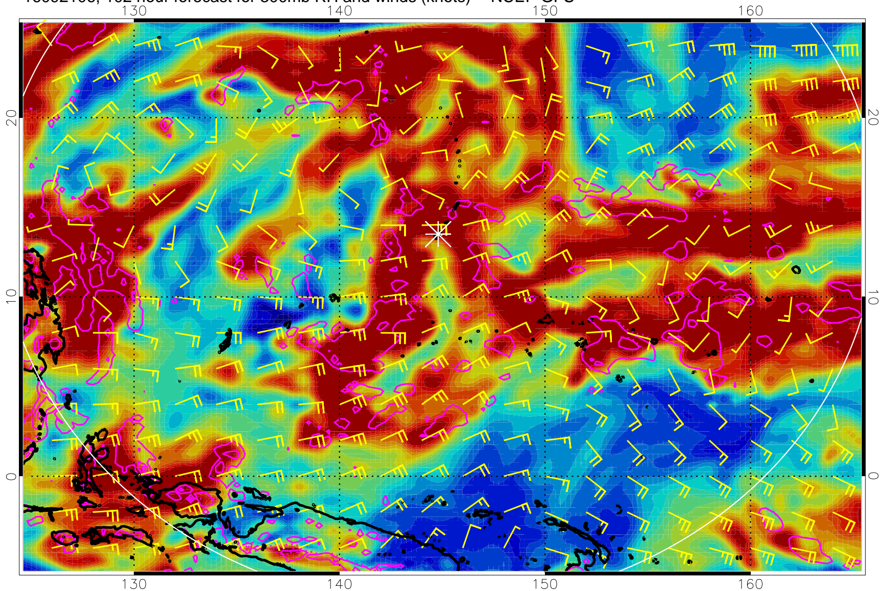
16092106, 102 hour forecast for 300mb RH and winds (knots) -- NCEP GFS
