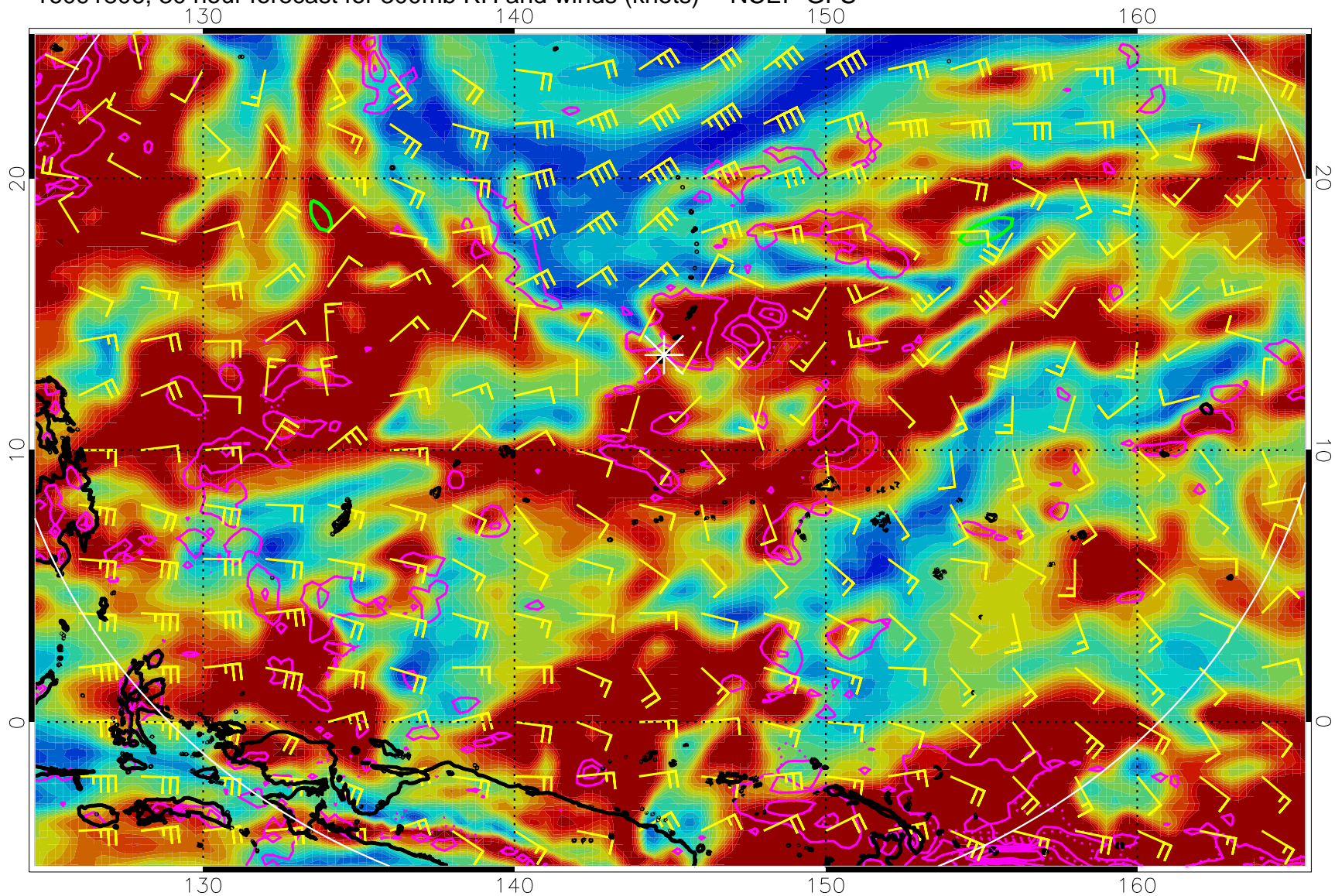
16091806, 30 hour forecast for 300mb RH and winds (knots) -- NCEP GFS
