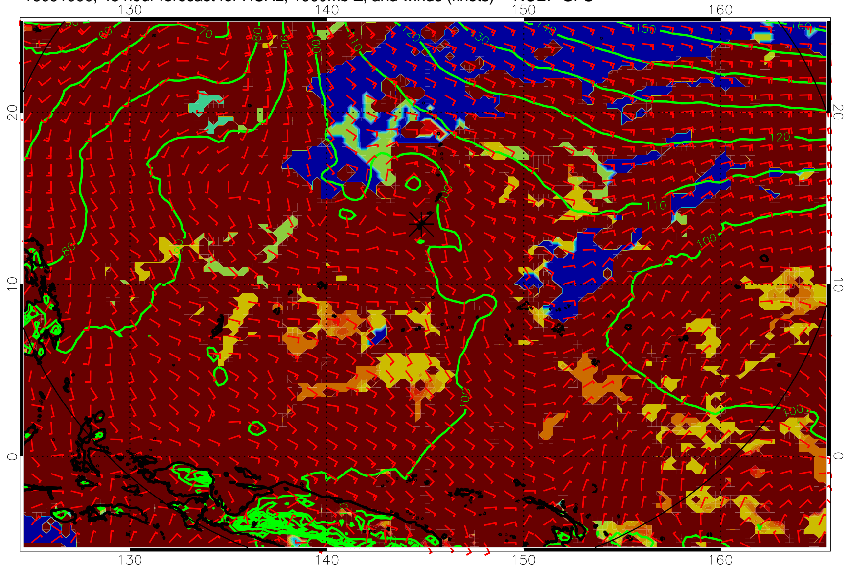
16091900, 48 hour forecast for HCAL, 1000mb Z, and winds (knots) -- NCEP GFS
