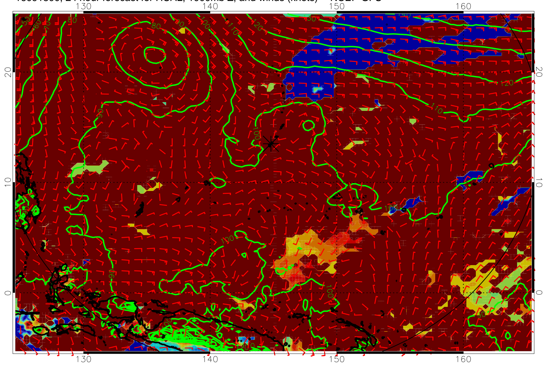
16091800, 24 hour forecast for HCAL, 1000mb Z, and winds (knots) -- NCEP GFS
