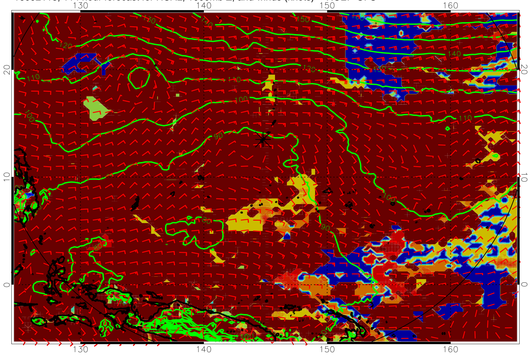
16092118, 114 hour forecast for HCAL, 1000mb Z, and winds (knots) -- NCEP GFS
