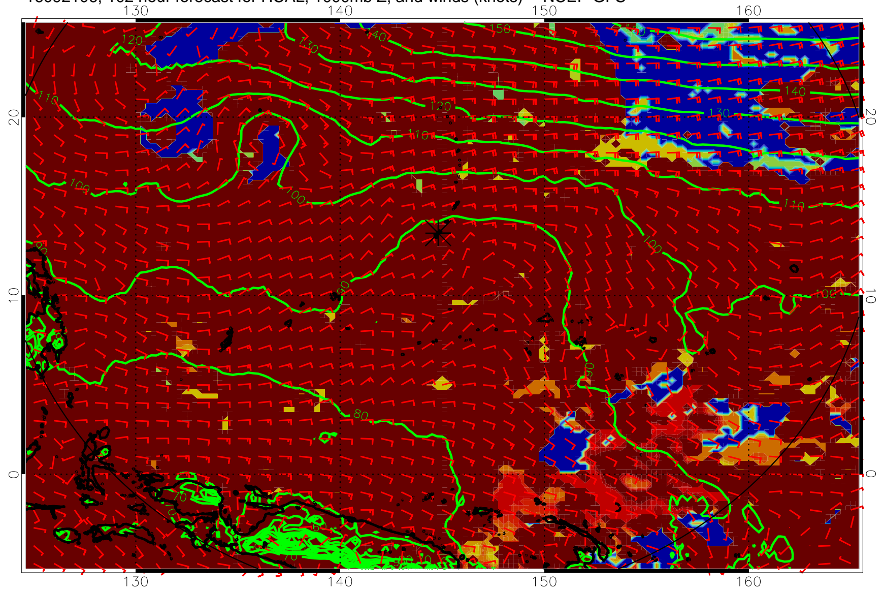
16092106, 102 hour forecast for HCAL, 1000mb Z, and winds (knots) -- NCEP GFS
