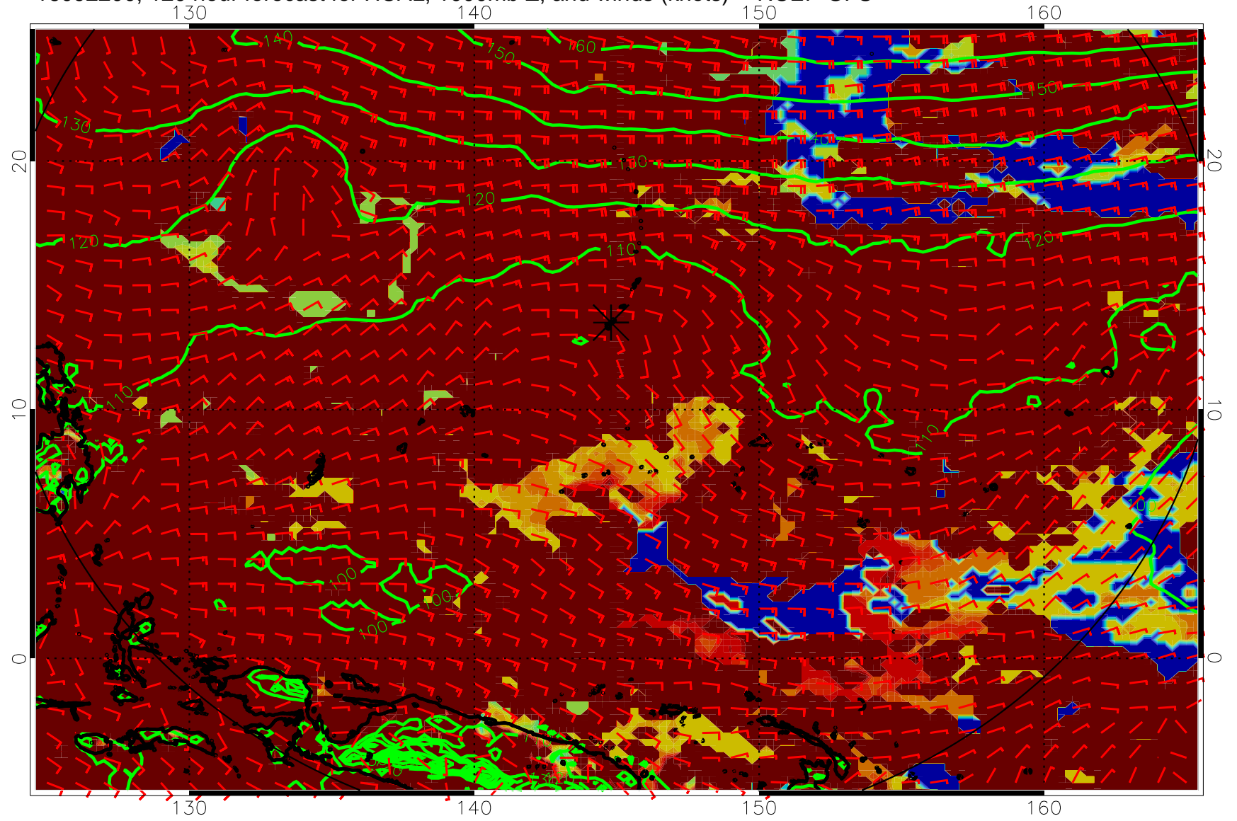
16092200, 120 hour forecast for HCAL, 1000mb Z, and winds (knots) -- NCEP GFS
