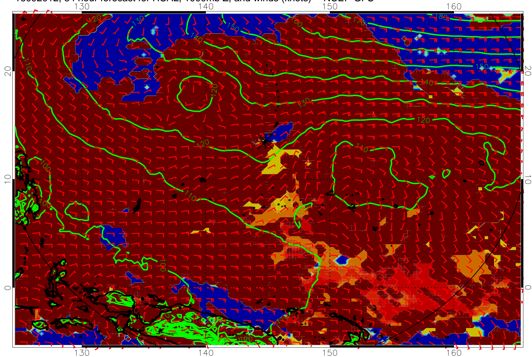
16092012, 84 hour forecast for HCAL, 1000mb Z, and winds (knots) -- NCEP GFS
