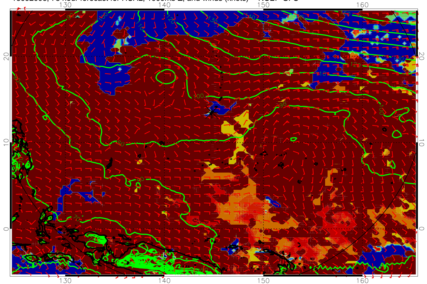
16092006, 78 hour forecast for HCAL, 1000mb Z, and winds (knots) -- NCEP GFS
