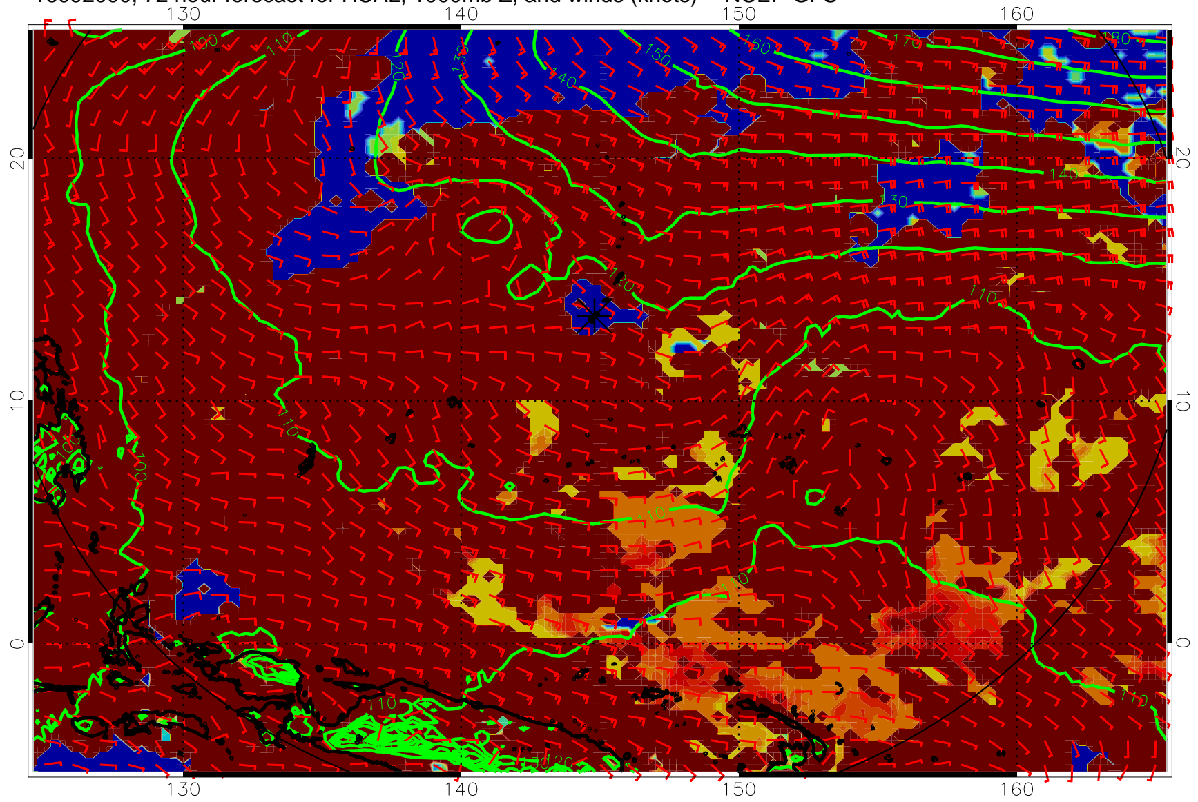
16092000, 72 hour forecast for HCAL, 1000mb Z, and winds (knots) -- NCEP GFS
