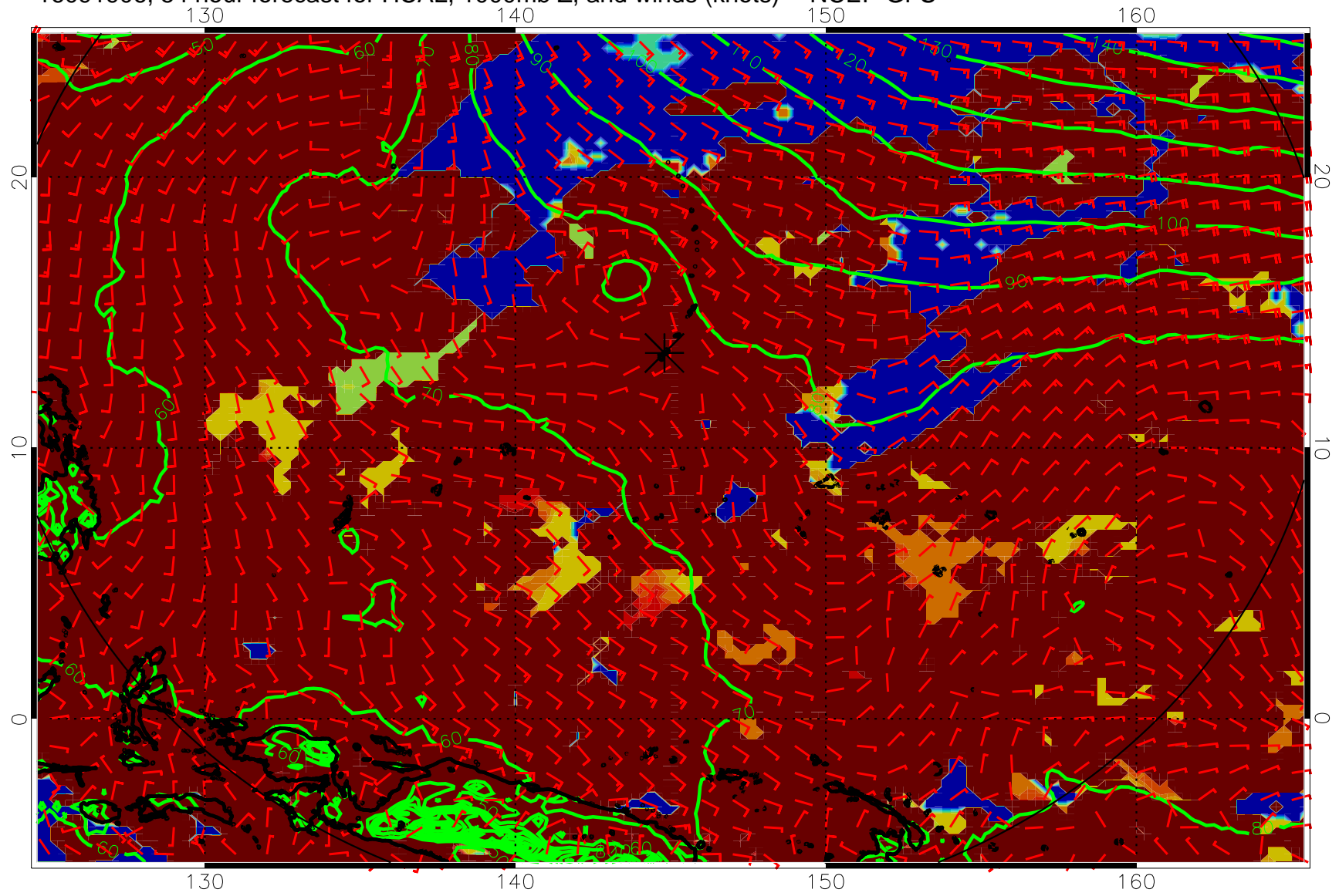
16091906, 54 hour forecast for HCAL, 1000mb Z, and winds (knots) -- NCEP GFS
