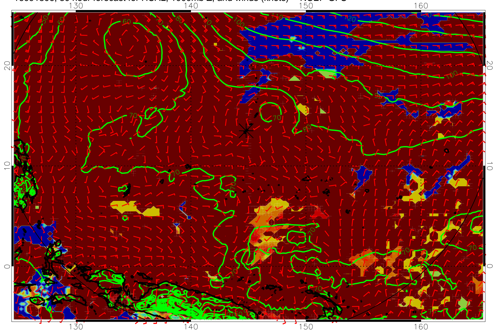
16091806, 30 hour forecast for HCAL, 1000mb Z, and winds (knots) -- NCEP GFS
