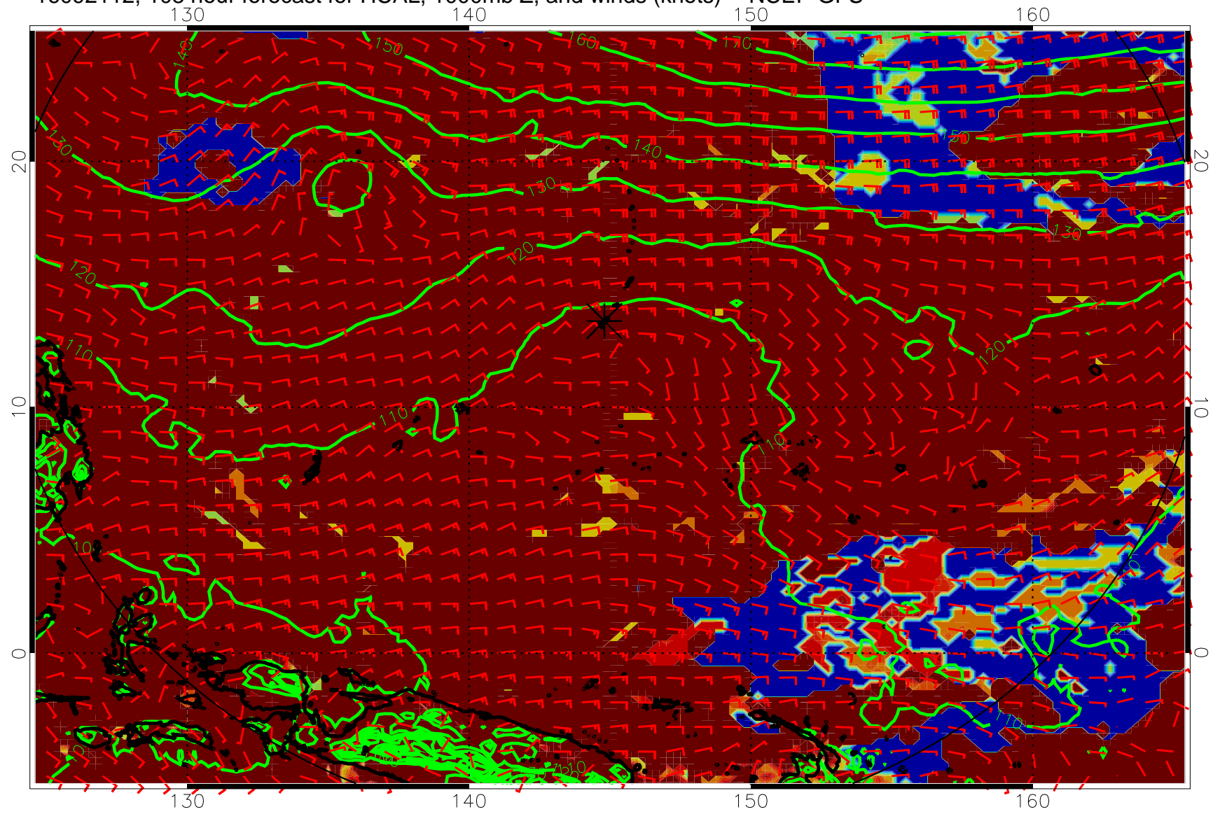
16092112, 108 hour forecast for HCAL, 1000mb Z, and winds (knots) -- NCEP GFS
