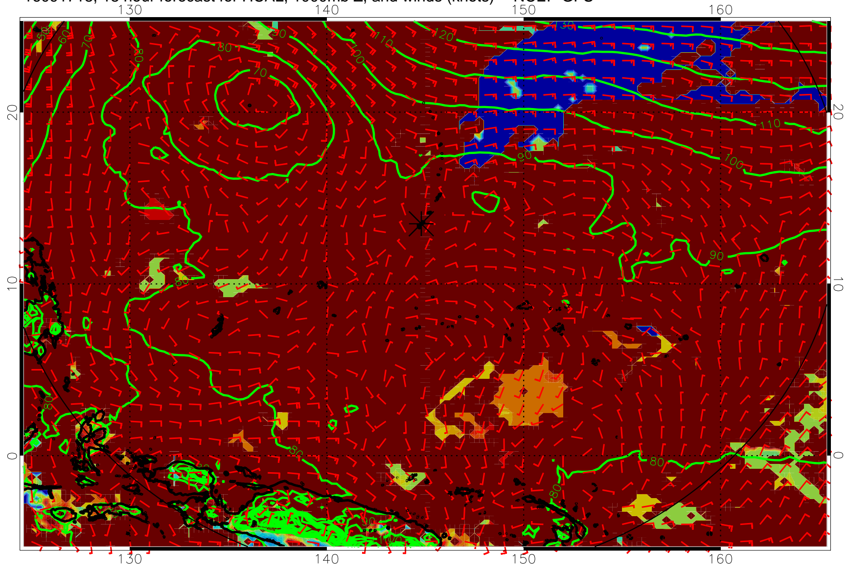
16091718, 18 hour forecast for HCAL, 1000mb Z, and winds (knots) -- NCEP GFS
