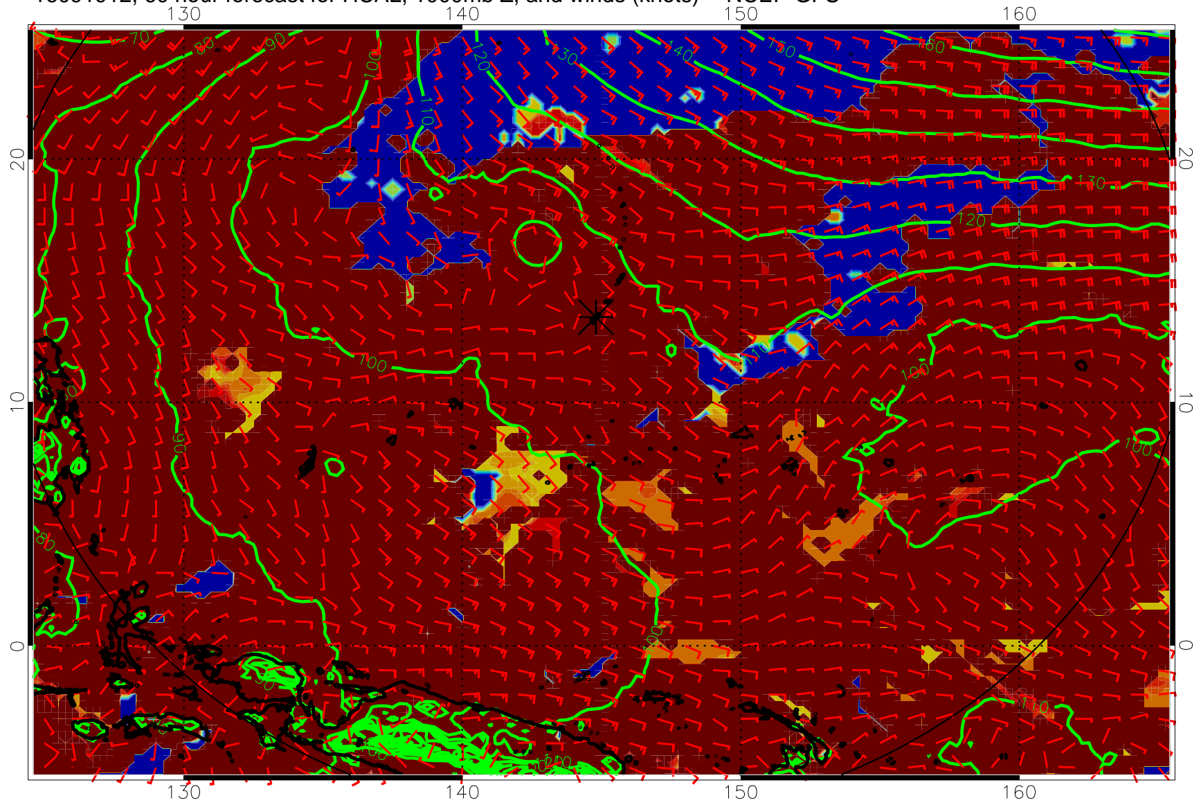
16091912, 60 hour forecast for HCAL, 1000mb Z, and winds (knots) -- NCEP GFS
