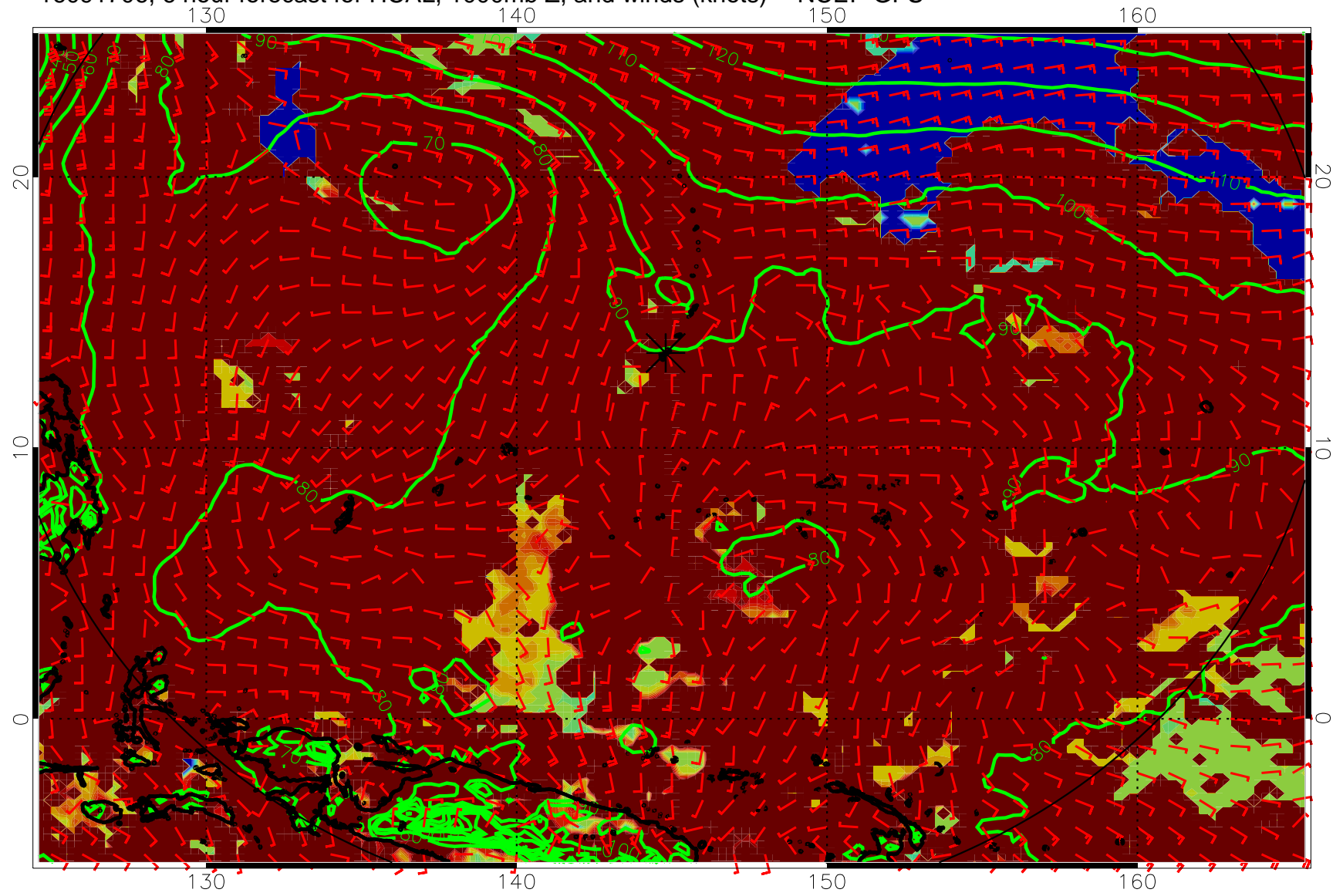
16091706, 6 hour forecast for HCAL, 1000mb Z, and winds (knots) -- NCEP GFS
