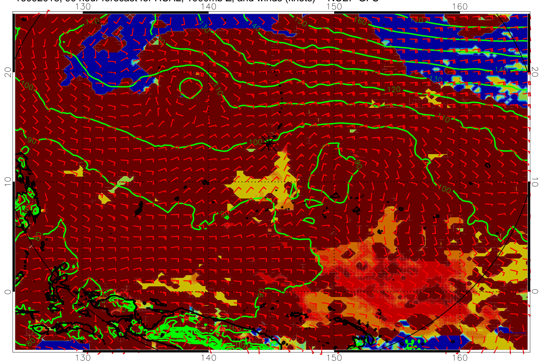
16092018, 90 hour forecast for HCAL, 1000mb Z, and winds (knots) -- NCEP GFS
