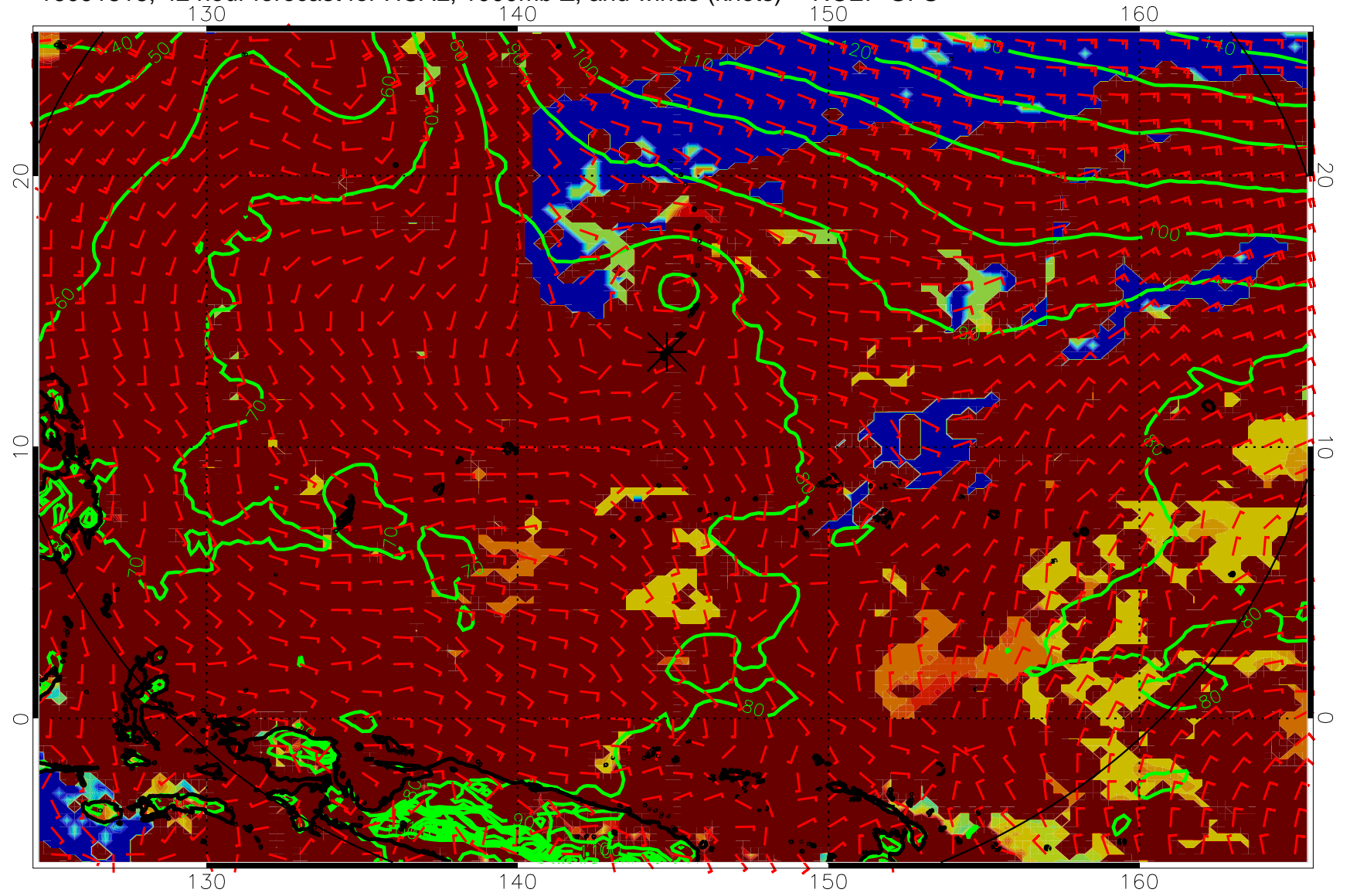
16091818, 42 hour forecast for HCAL, 1000mb Z, and winds (knots) -- NCEP GFS
