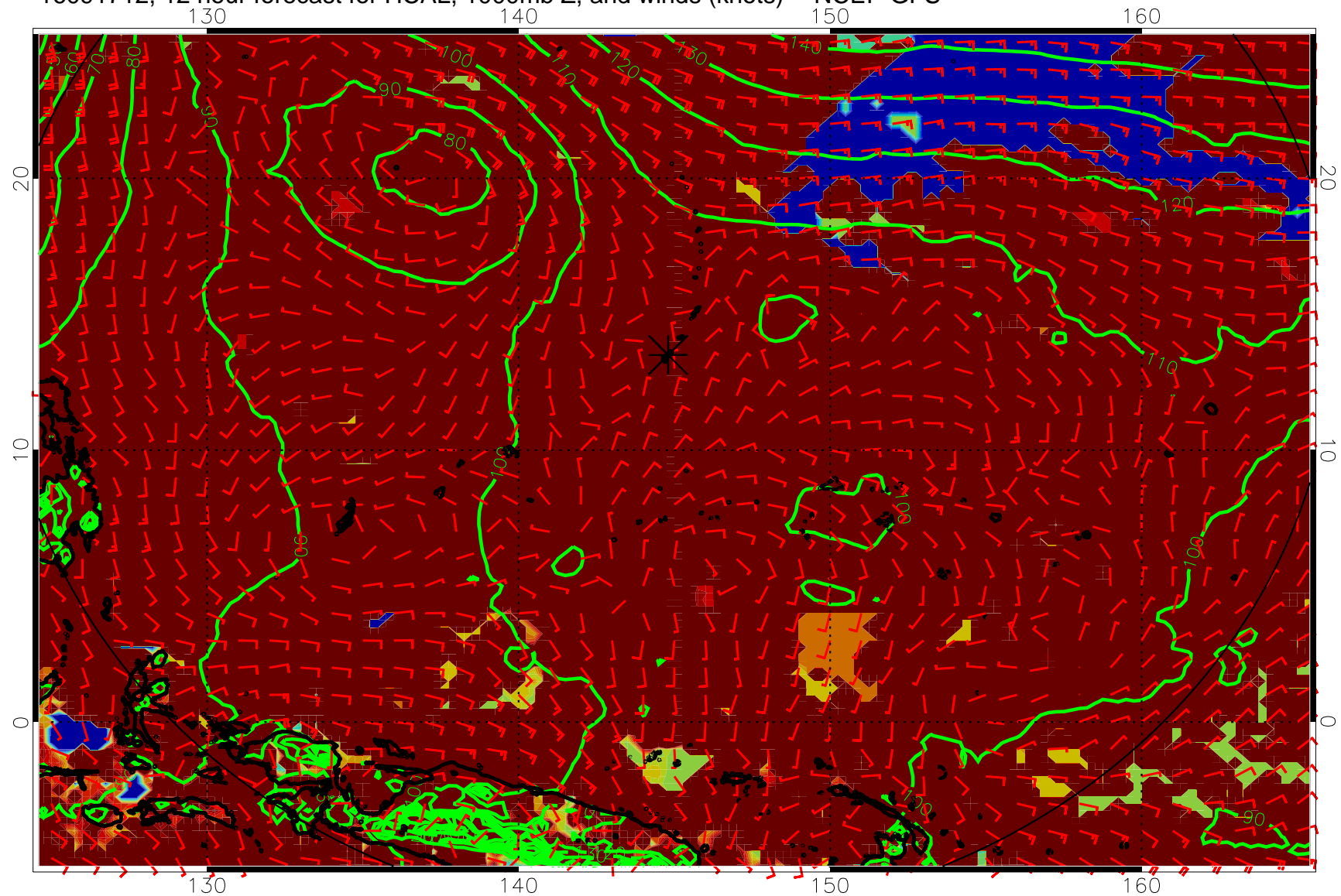
16091712, 12 hour forecast for HCAL, 1000mb Z, and winds (knots) -- NCEP GFS
