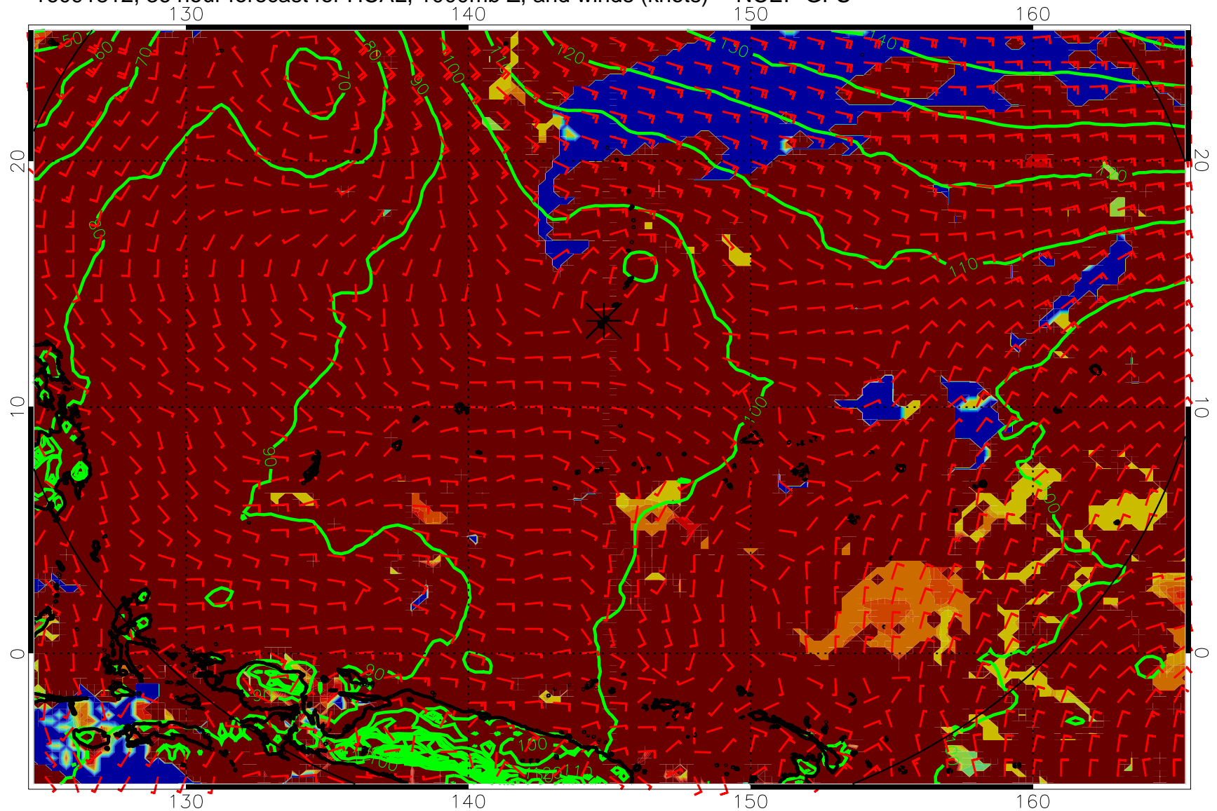
16091812, 36 hour forecast for HCAL, 1000mb Z, and winds (knots) -- NCEP GFS
