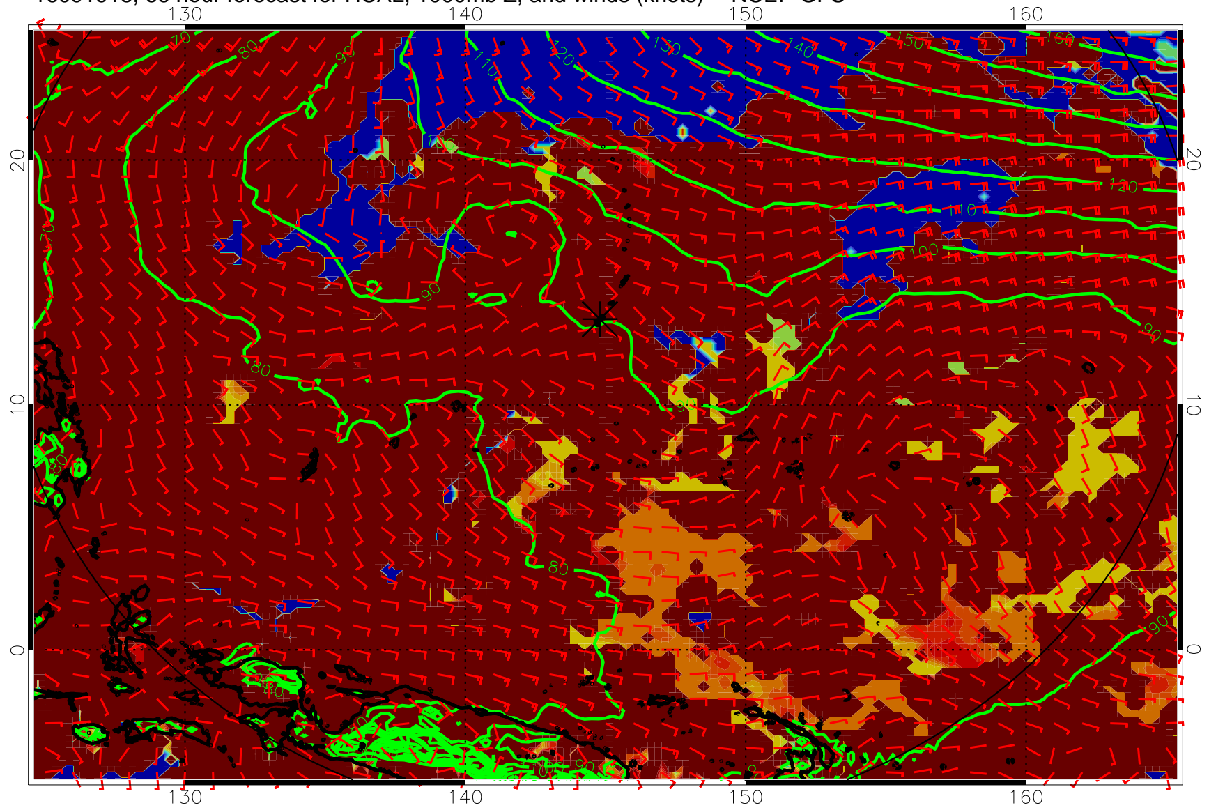
16091918, 66 hour forecast for HCAL, 1000mb Z, and winds (knots) -- NCEP GFS
