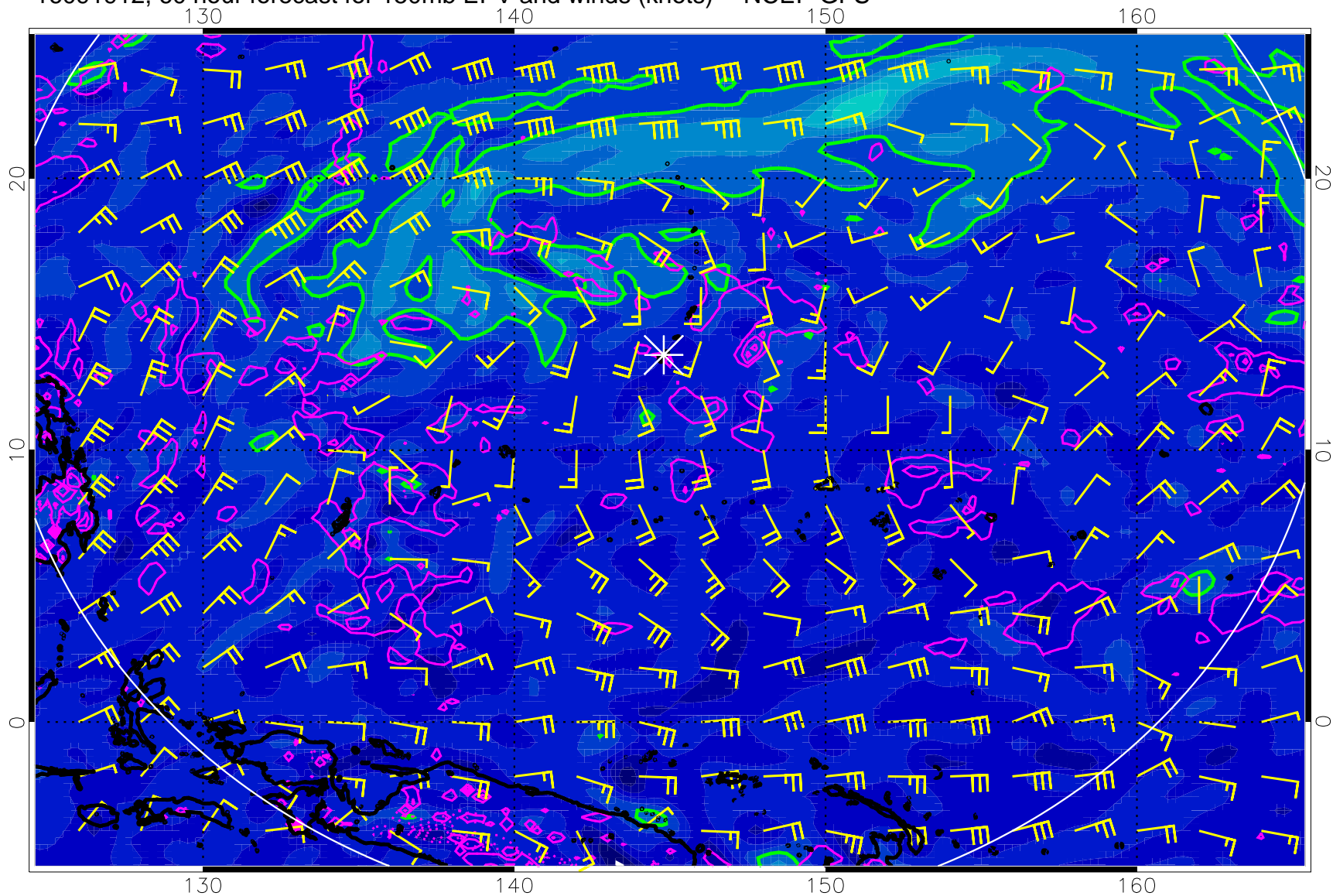
16091912, 60 hour forecast for 150mb EPV and winds (knots) -- NCEP GFS
