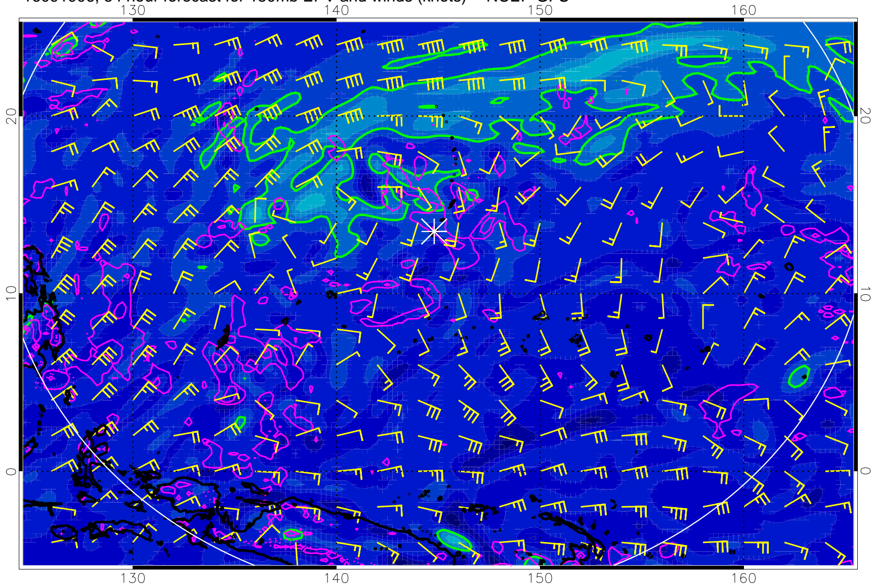
16091906, 54 hour forecast for 150mb EPV and winds (knots) -- NCEP GFS
