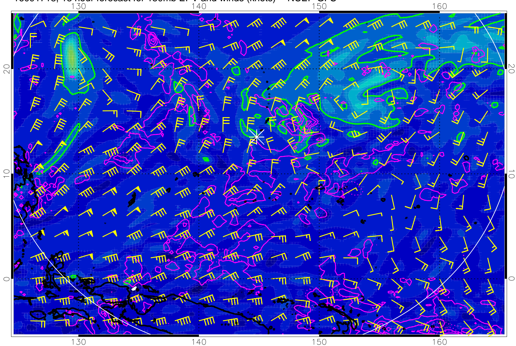
16091718, 18 hour forecast for 150mb EPV and winds (knots) -- NCEP GFS
