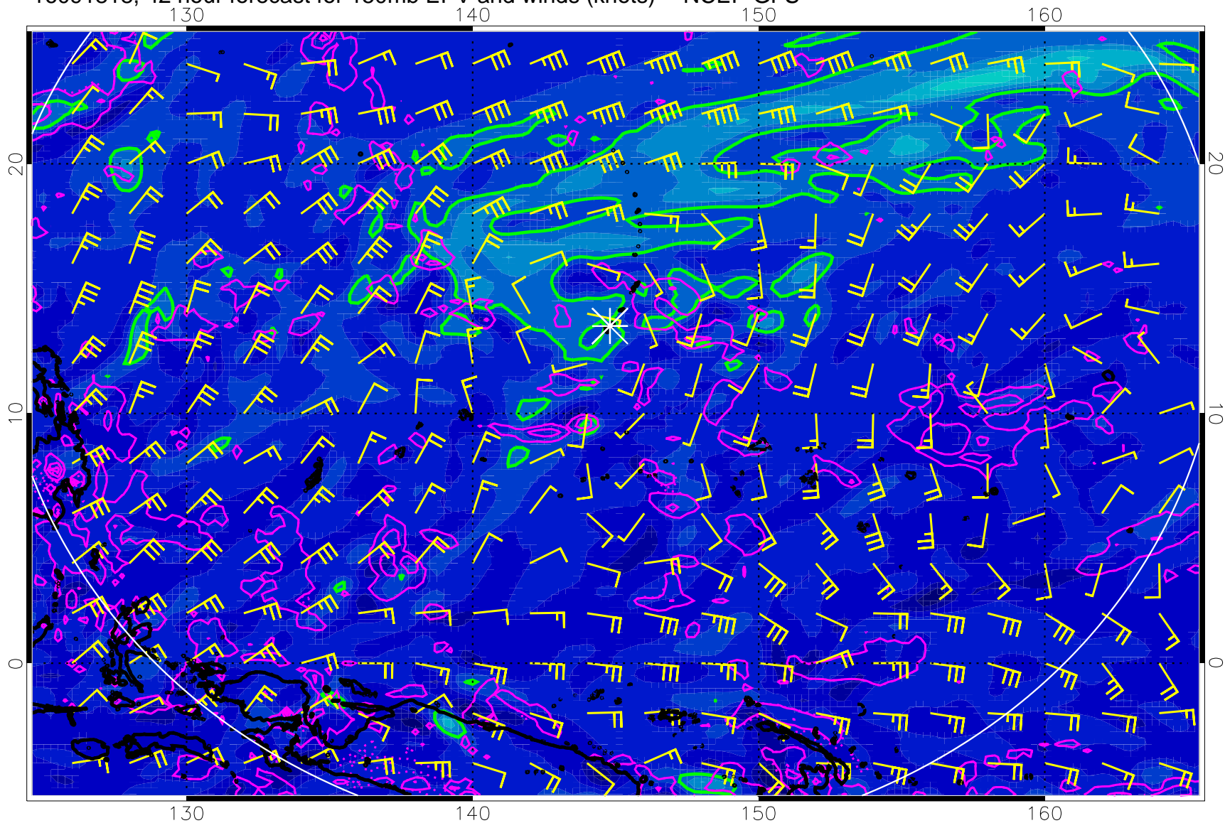
16091818, 42 hour forecast for 150mb EPV and winds (knots) -- NCEP GFS
