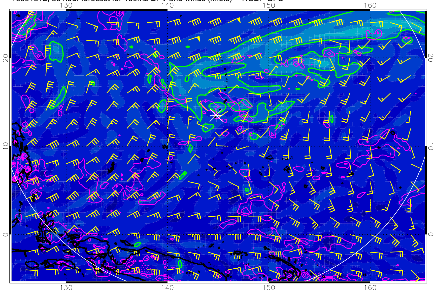
16091812, 36 hour forecast for 150mb EPV and winds (knots) -- NCEP GFS
