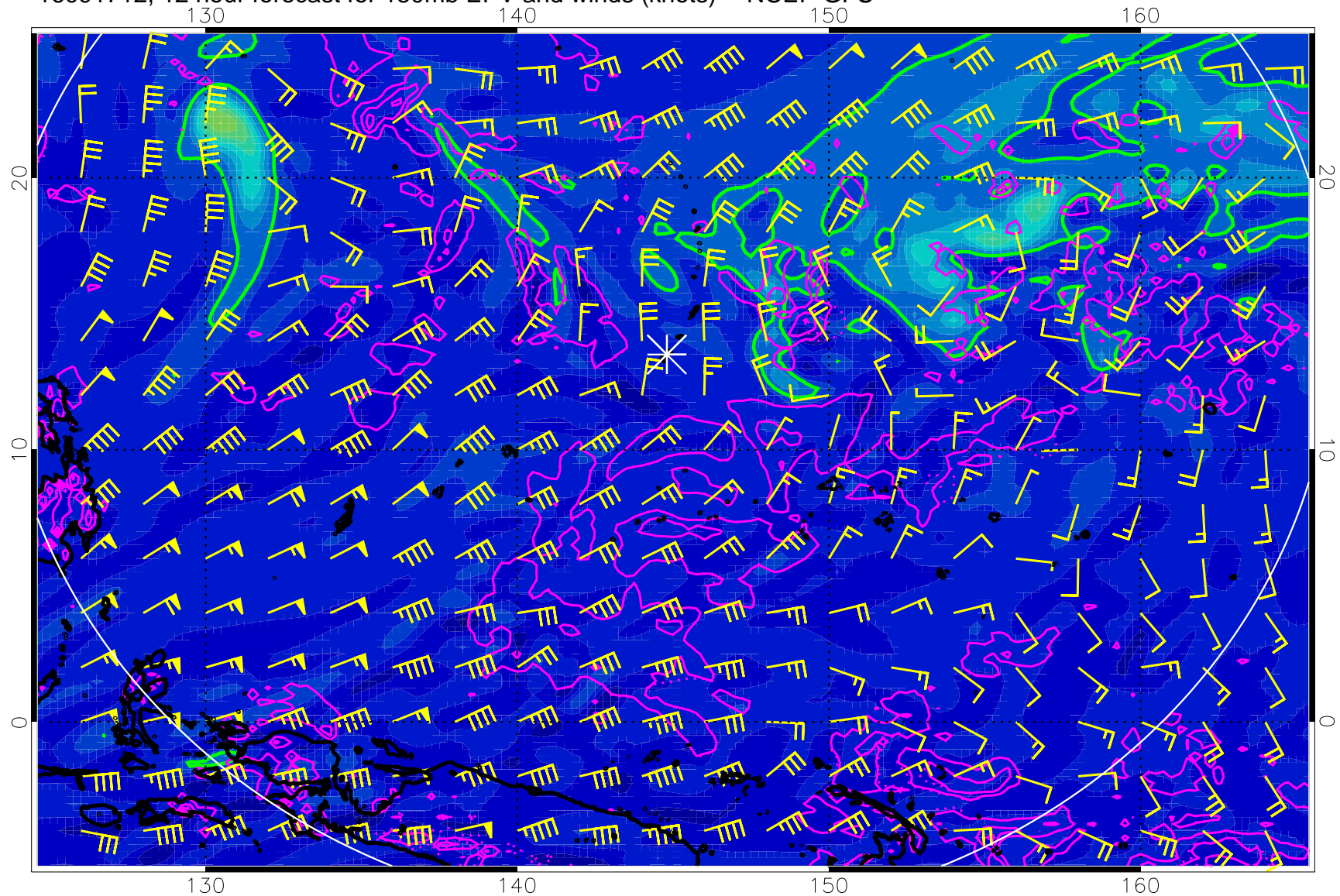
16091712, 12 hour forecast for 150mb EPV and winds (knots) -- NCEP GFS
