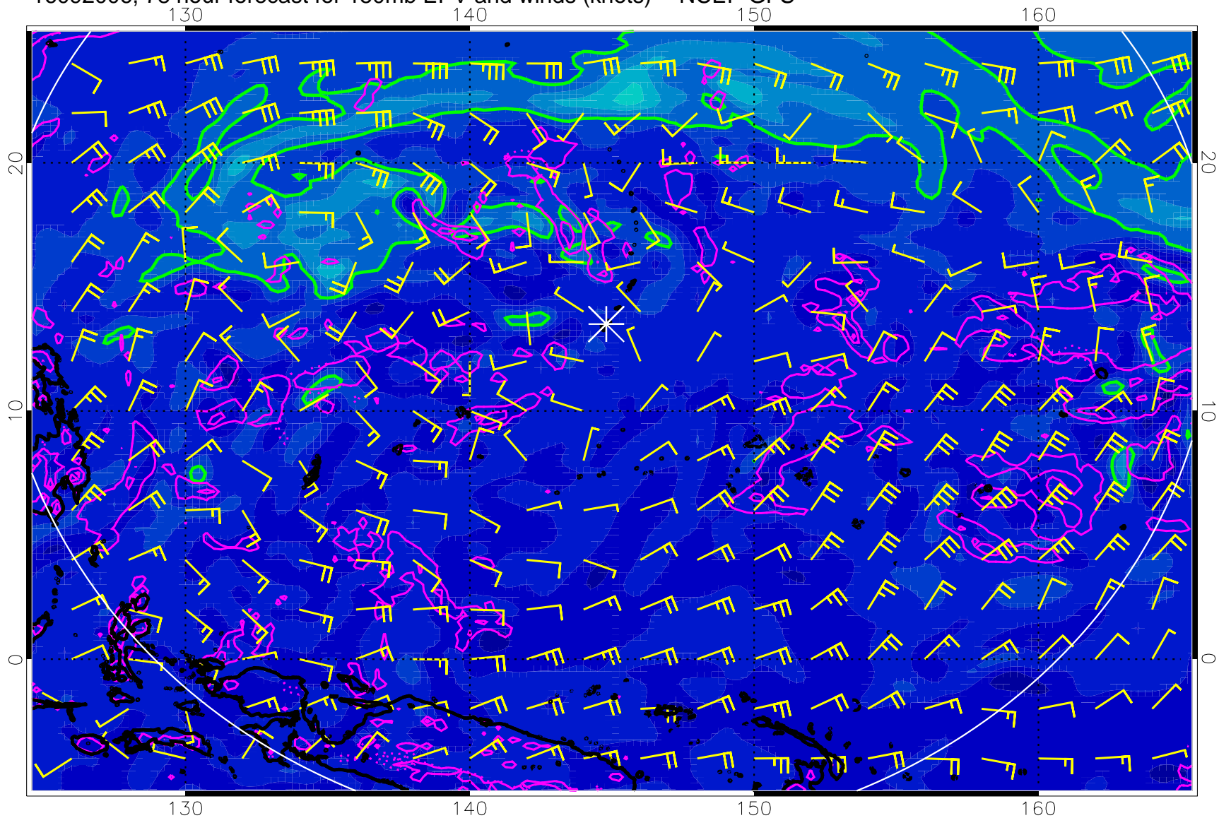
16092006, 78 hour forecast for 150mb EPV and winds (knots) -- NCEP GFS
