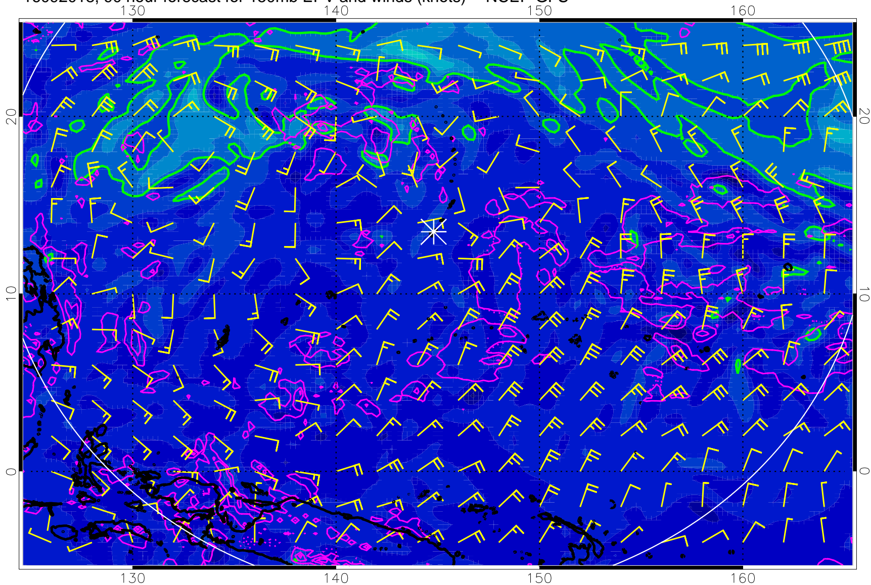
16092018, 90 hour forecast for 150mb EPV and winds (knots) -- NCEP GFS
