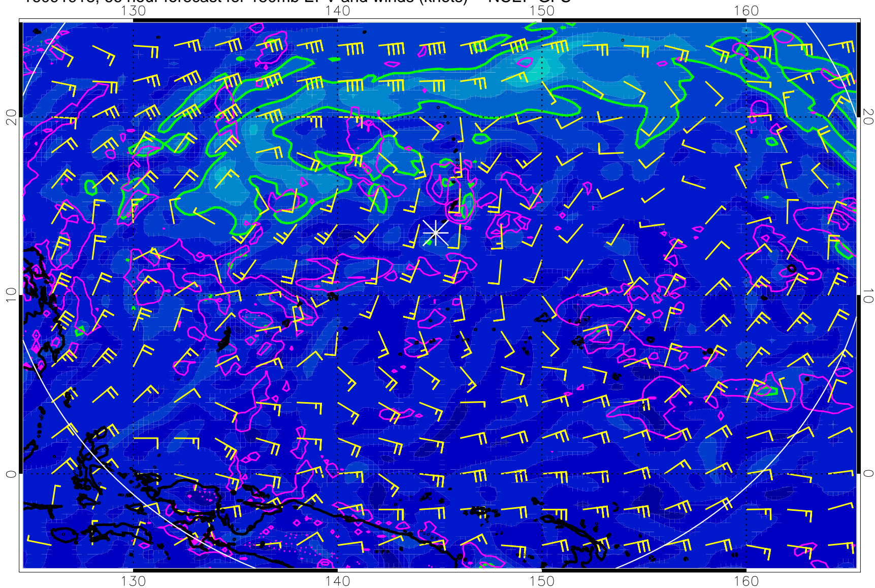
16091918, 66 hour forecast for 150mb EPV and winds (knots) -- NCEP GFS
