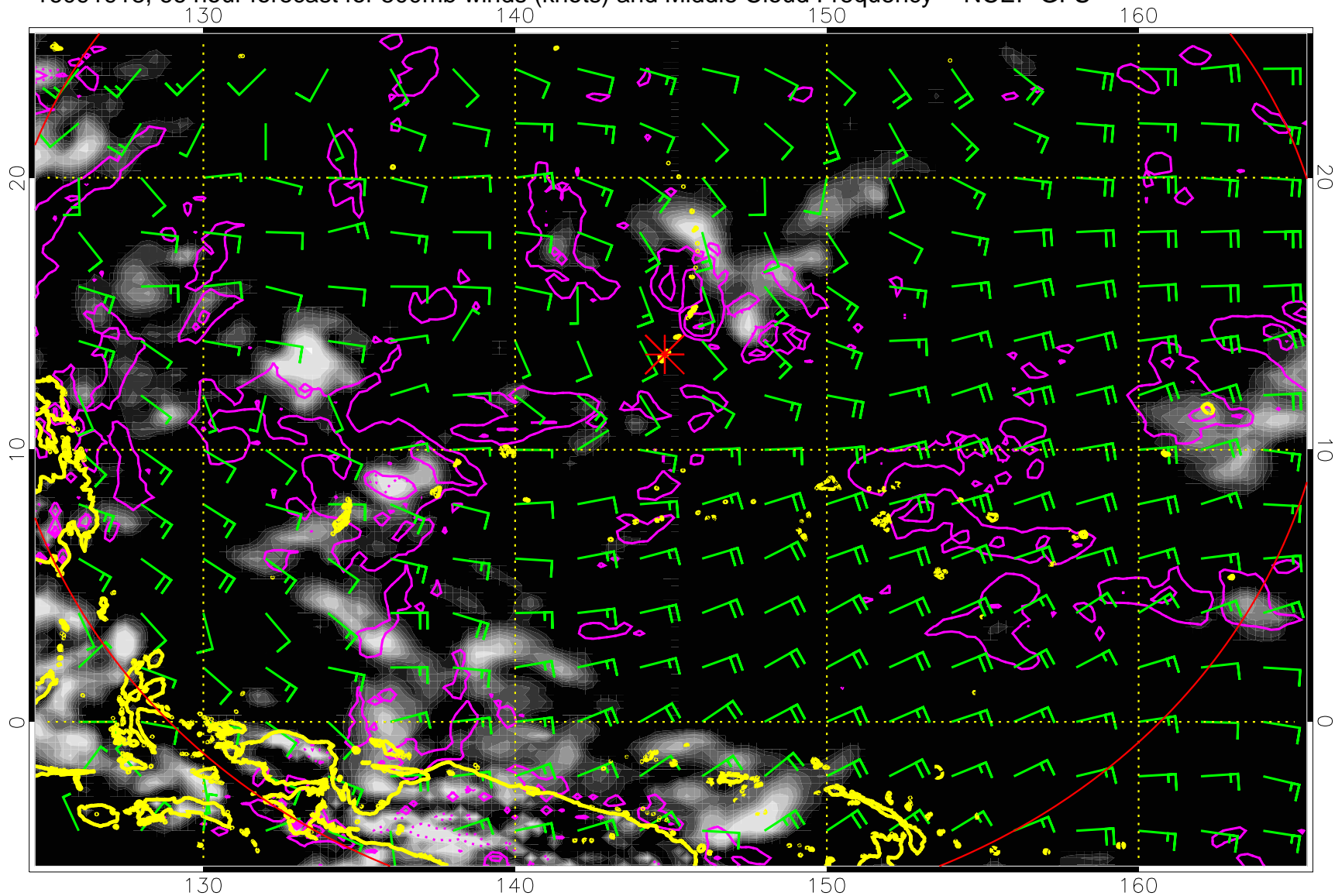
16091918, 66 hour forecast for 500mb winds (knots) and Middle Cloud Frequency -- NCEP GFS
