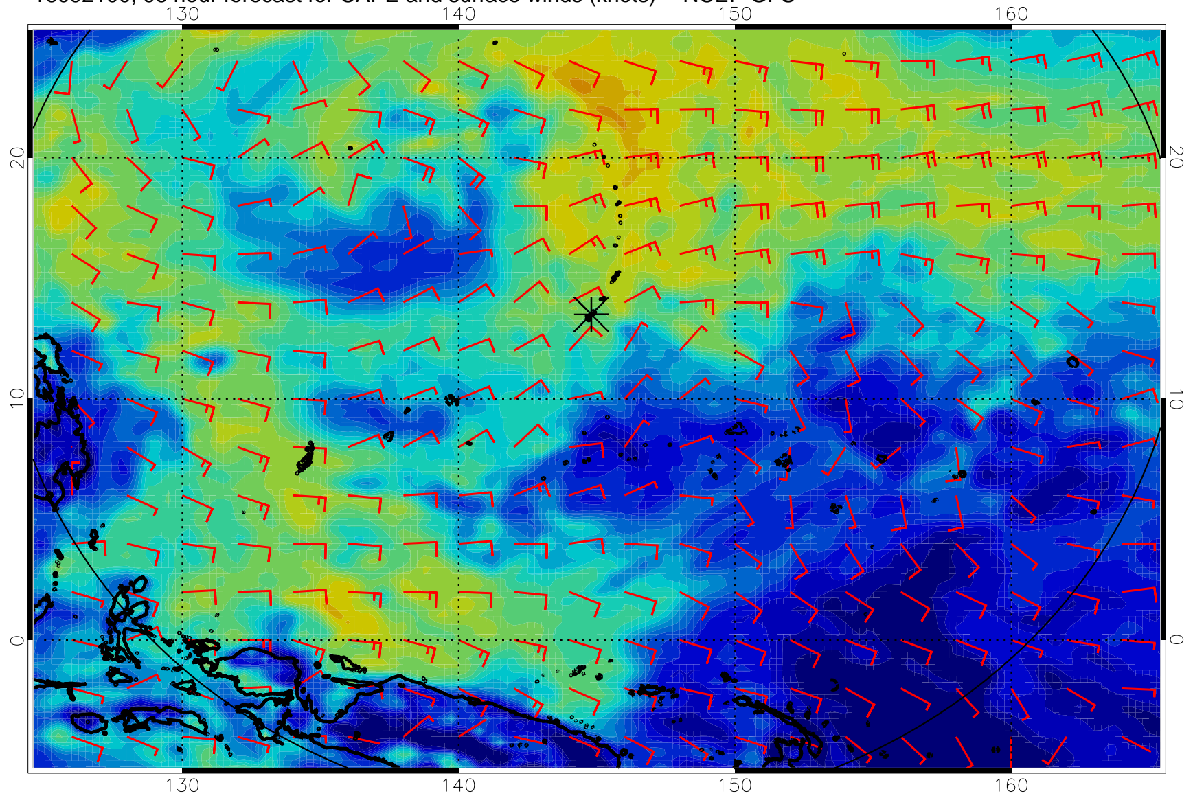
16092100, 96 hour forecast for CAPE and surface winds (knots) -- NCEP GFS
