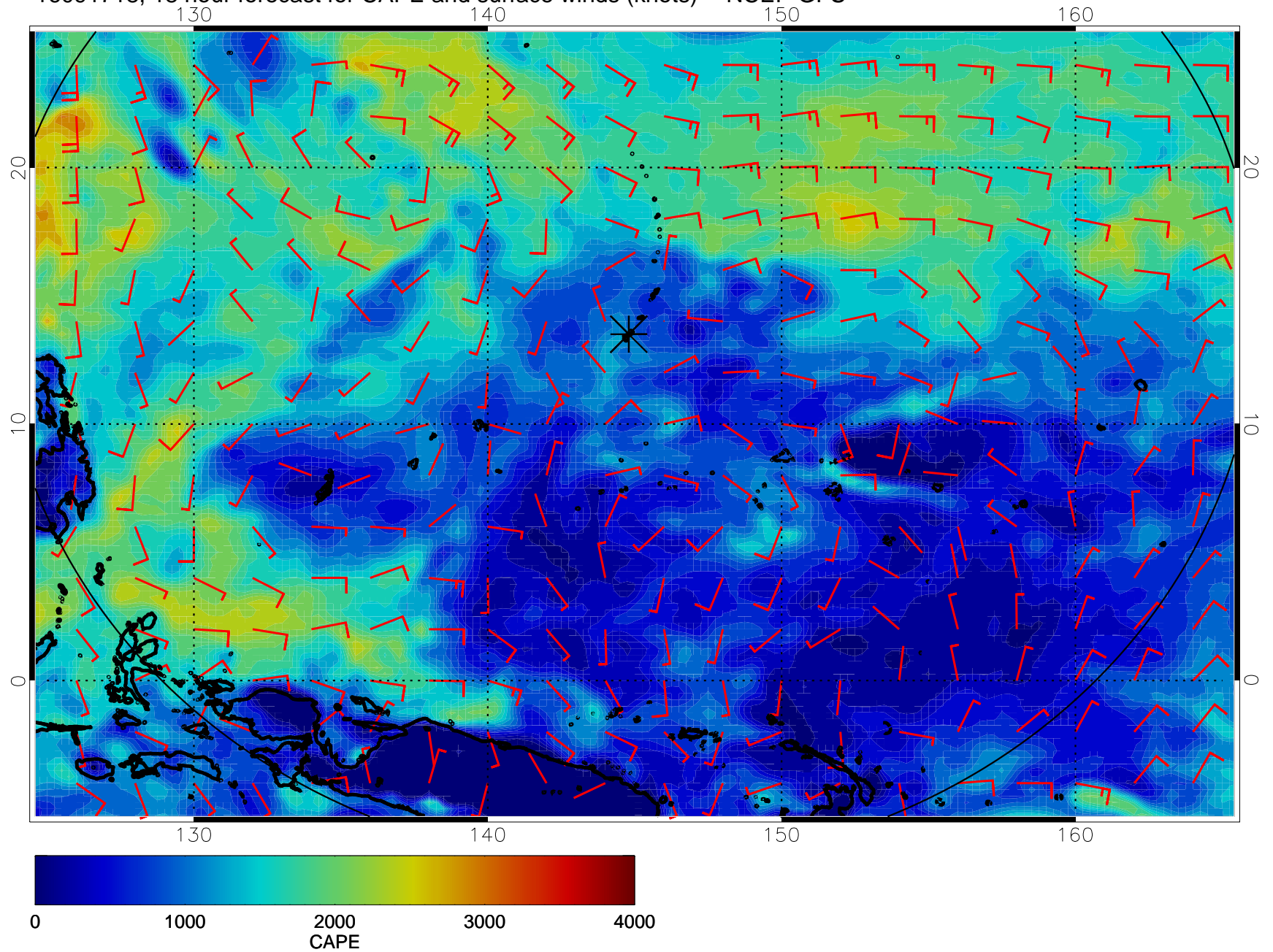
16091718, 18 hour forecast for CAPE and surface winds (knots) -- NCEP GFS
