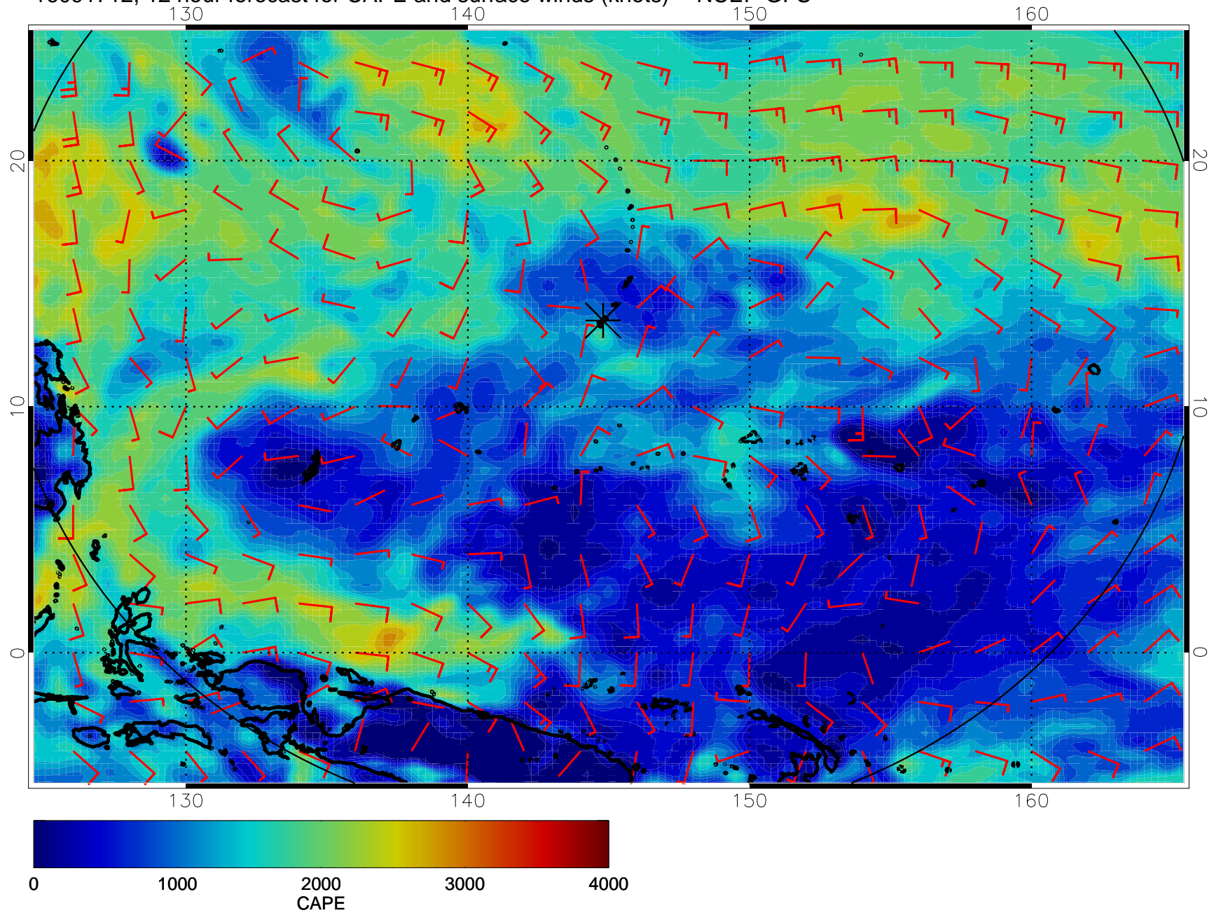
16091712, 12 hour forecast for CAPE and surface winds (knots) -- NCEP GFS
