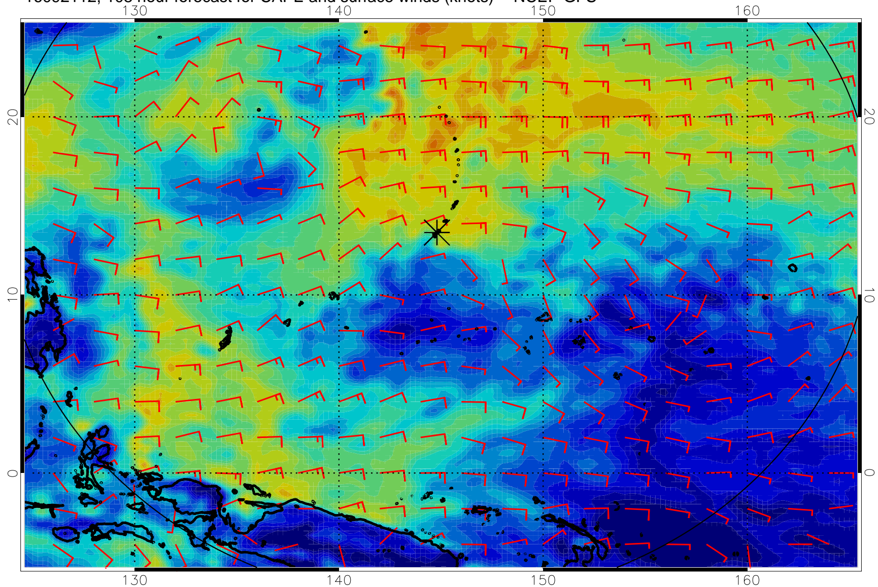
16092112, 108 hour forecast for CAPE and surface winds (knots) -- NCEP GFS
