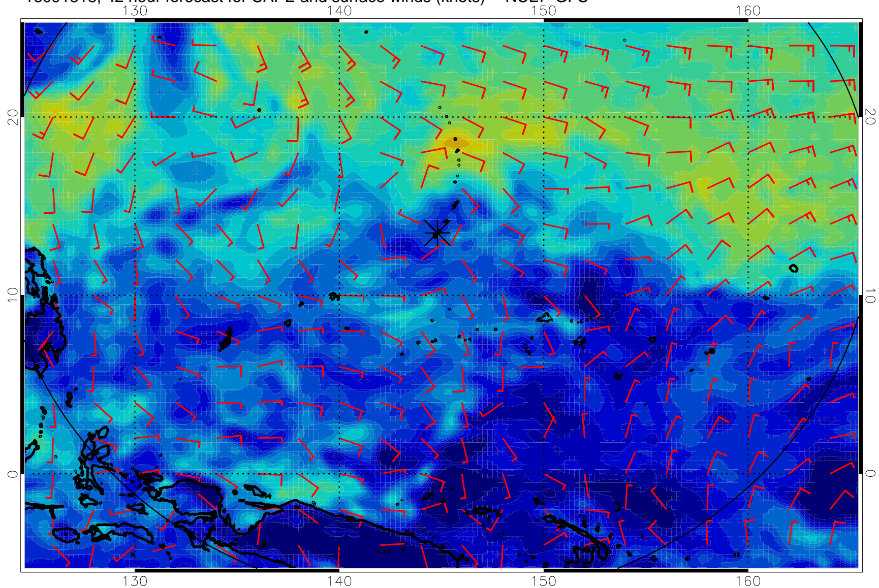
16091818, 42 hour forecast for CAPE and surface winds (knots) -- NCEP GFS
