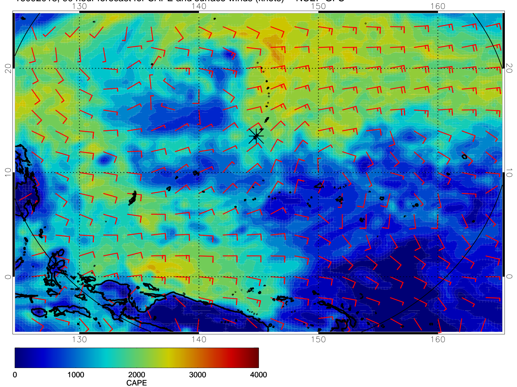
16092018, 90 hour forecast for CAPE and surface winds (knots) -- NCEP GFS
