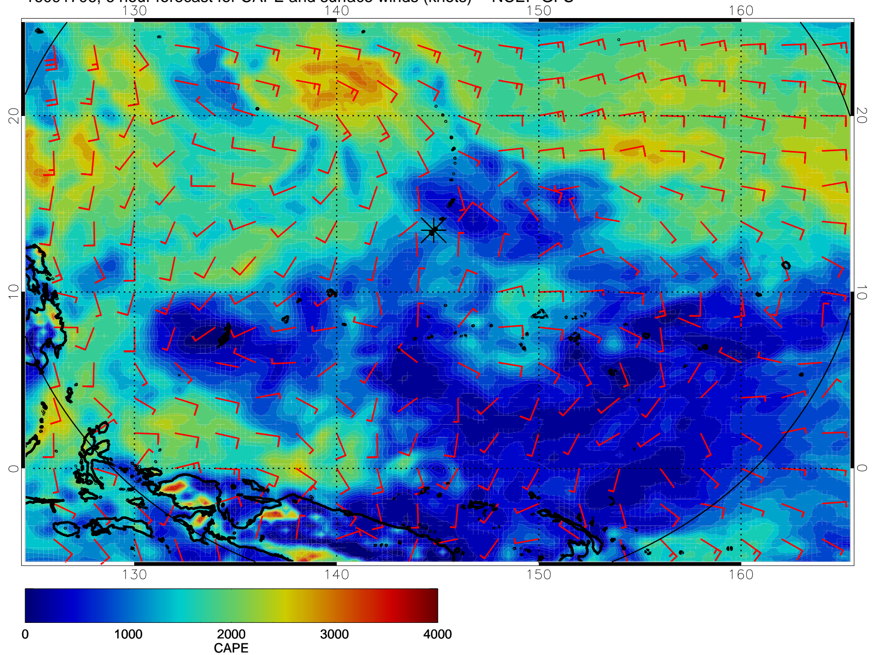
16091706, 6 hour forecast for CAPE and surface winds (knots) -- NCEP GFS
