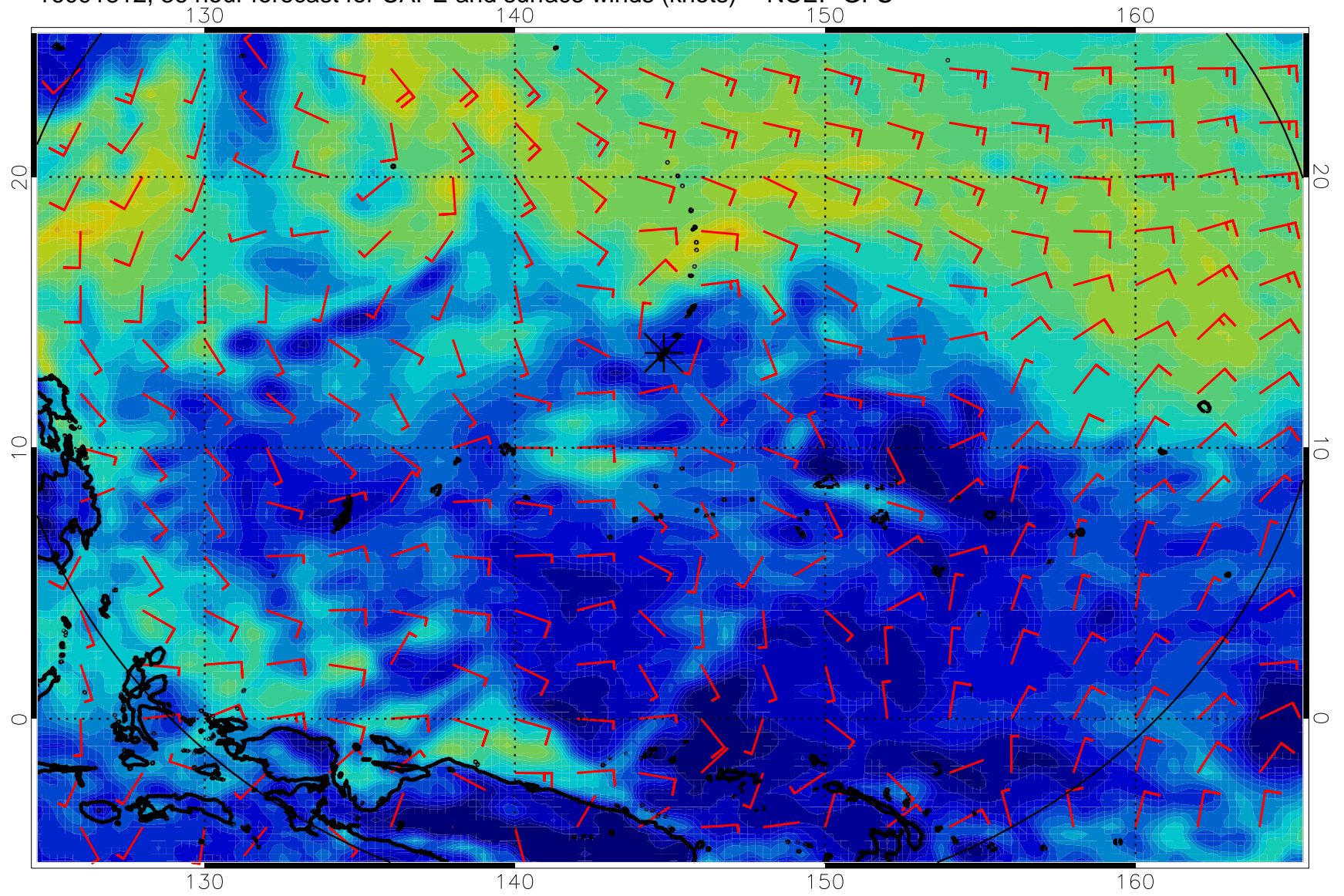
16091812, 36 hour forecast for CAPE and surface winds (knots) -- NCEP GFS
