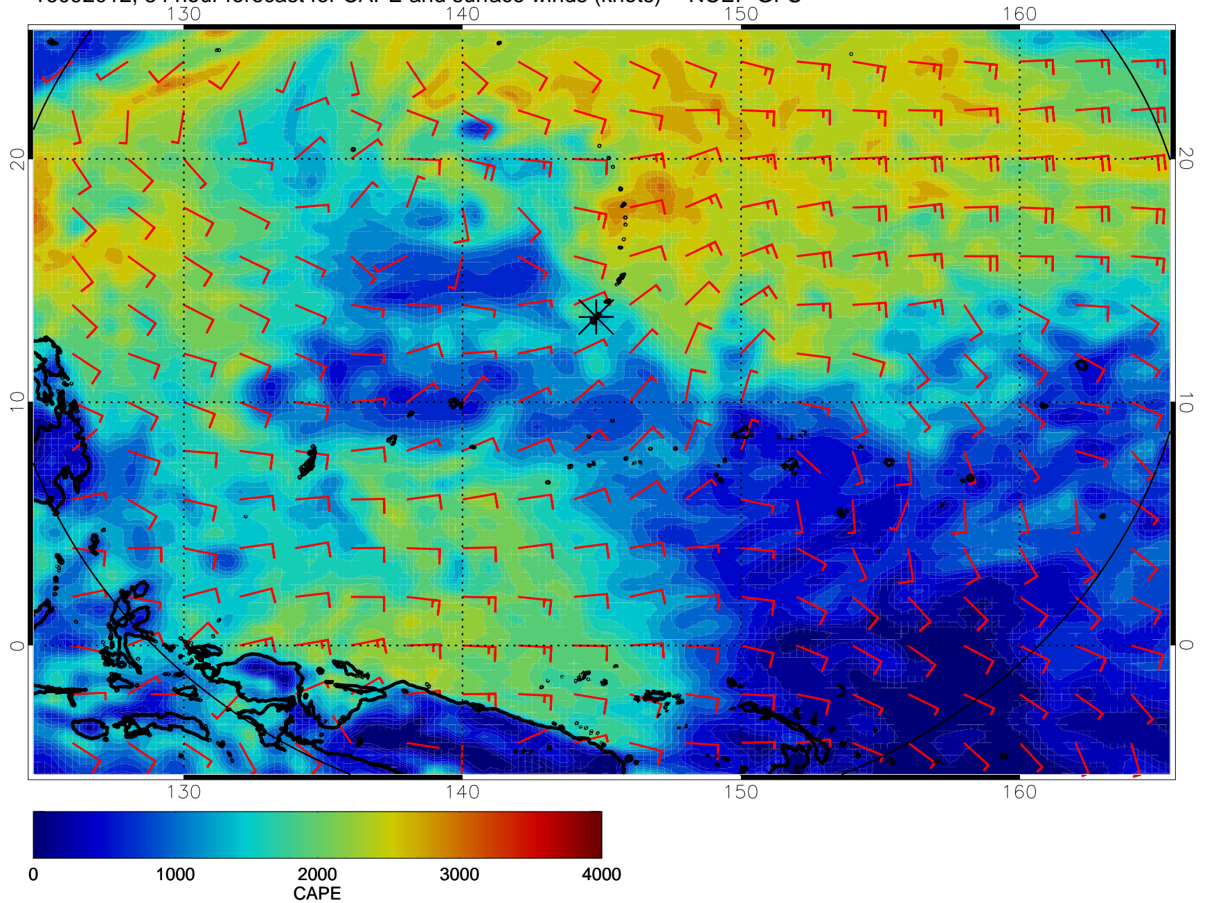
16092012, 84 hour forecast for CAPE and surface winds (knots) -- NCEP GFS
