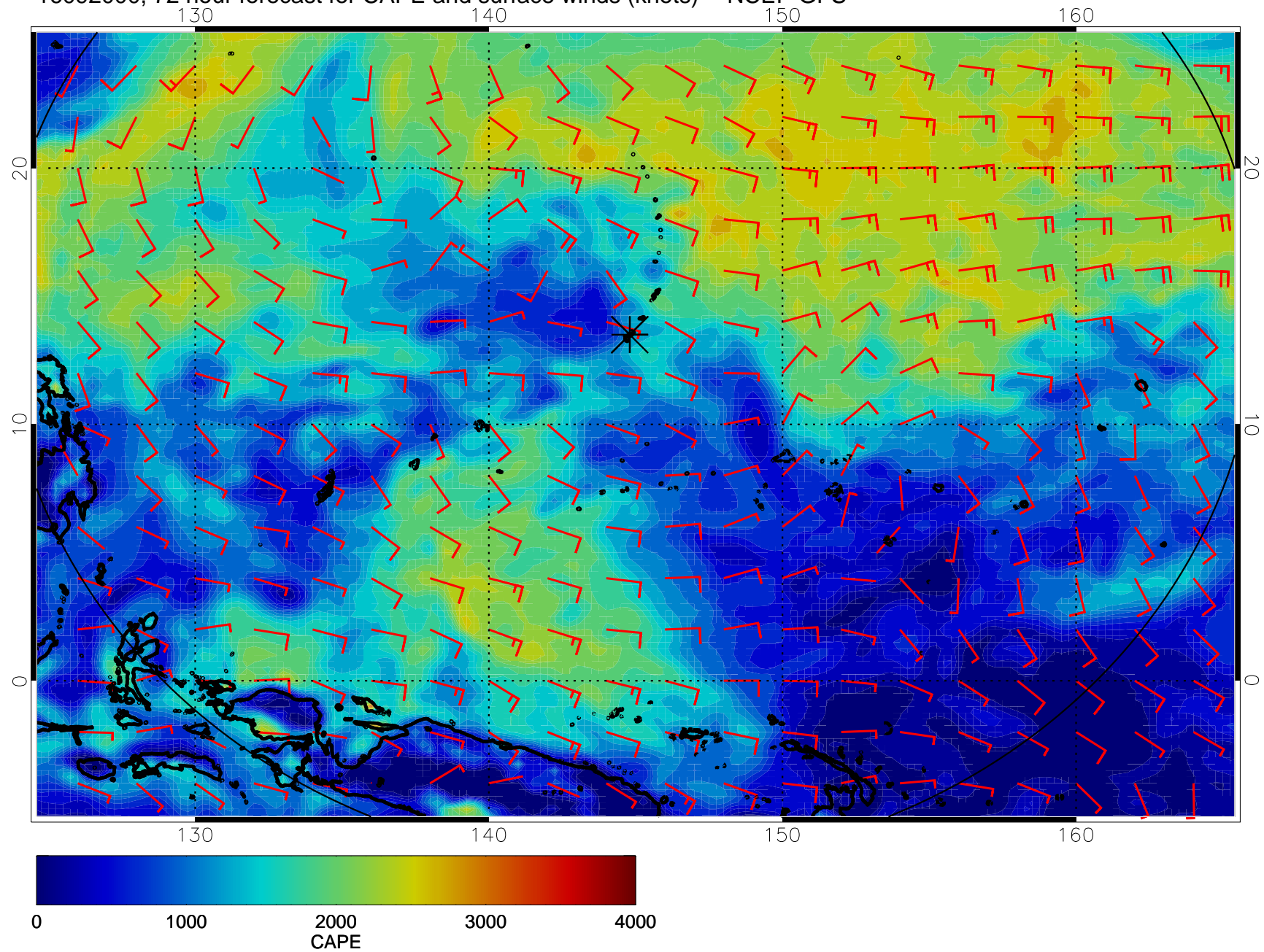
16092000, 72 hour forecast for CAPE and surface winds (knots) -- NCEP GFS
