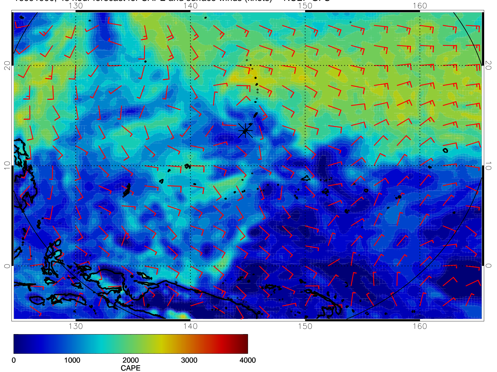
16091900, 48 hour forecast for CAPE and surface winds (knots) -- NCEP GFS
