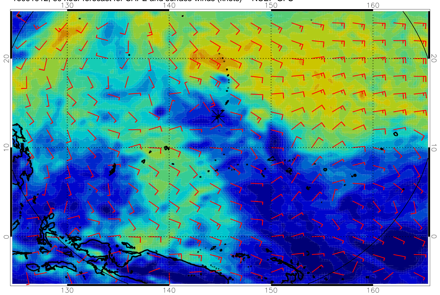
16091912, 60 hour forecast for CAPE and surface winds (knots) -- NCEP GFS
