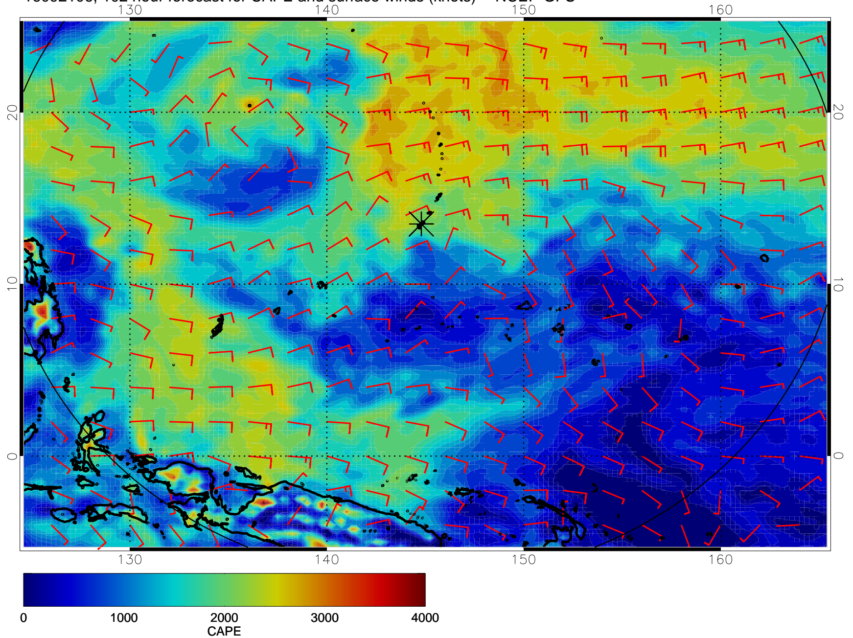
16092106, 102 hour forecast for CAPE and surface winds (knots) -- NCEP GFS
