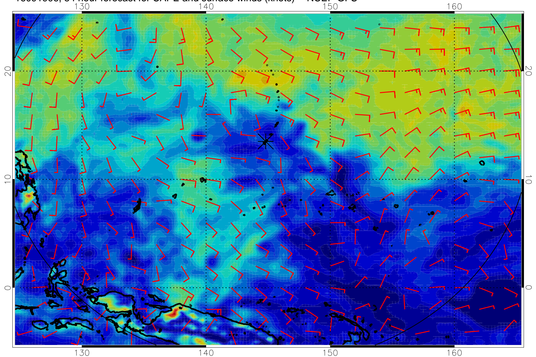
16091906, 54 hour forecast for CAPE and surface winds (knots) -- NCEP GFS
