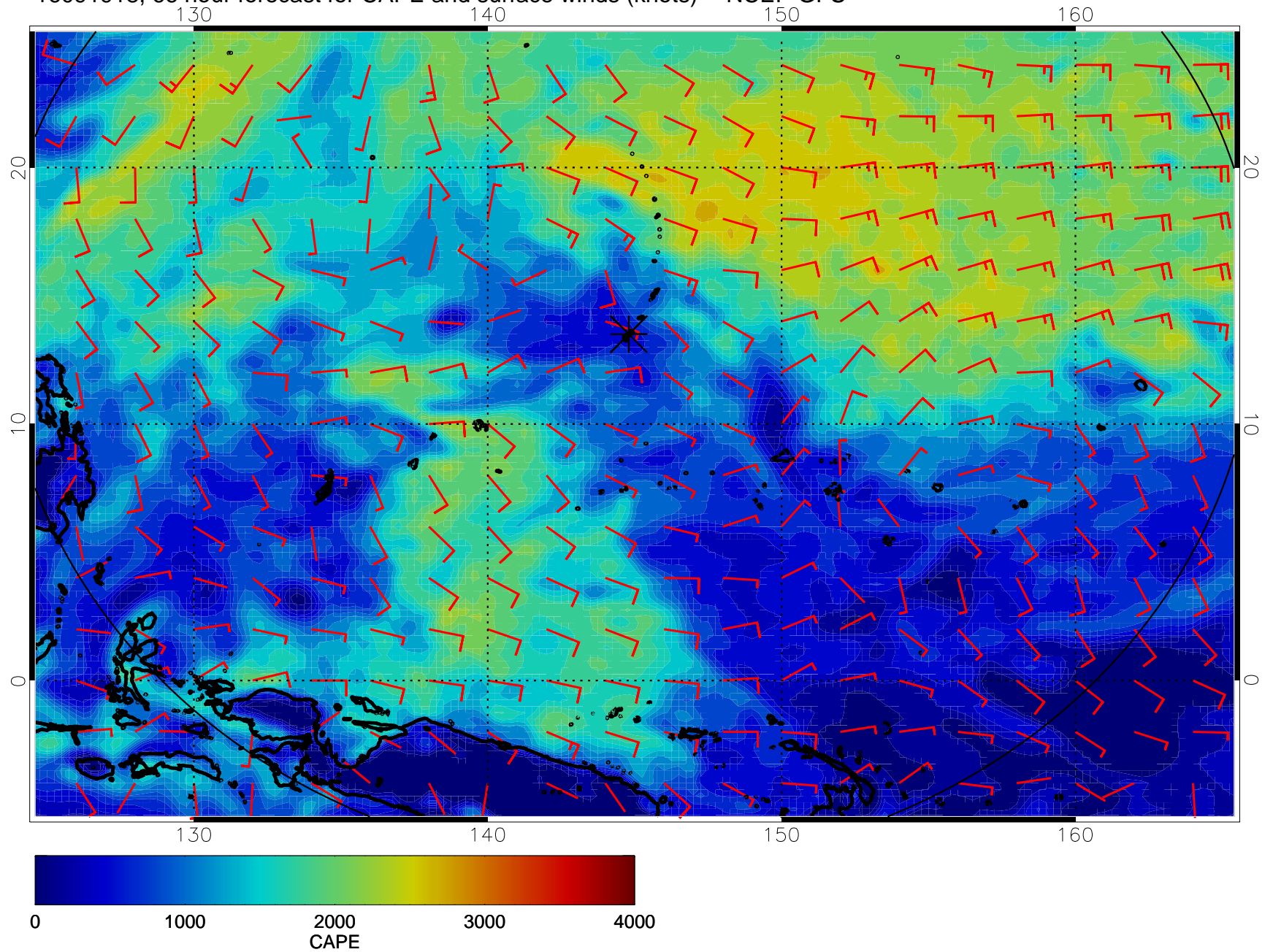
16091918, 66 hour forecast for CAPE and surface winds (knots) -- NCEP GFS
