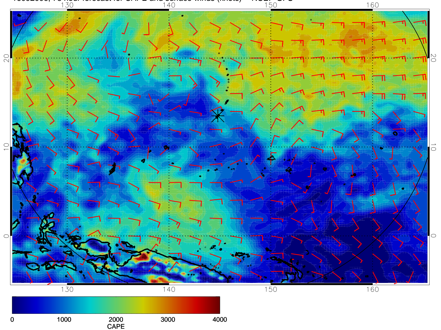
16092006, 78 hour forecast for CAPE and surface winds (knots) -- NCEP GFS
