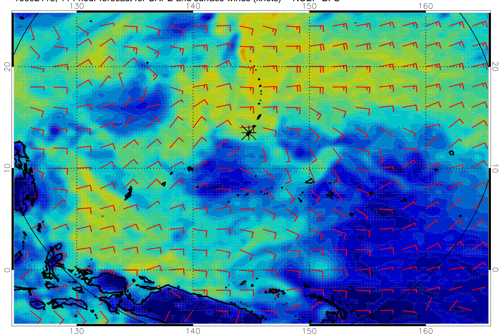
16092118, 114 hour forecast for CAPE and surface winds (knots) -- NCEP GFS
