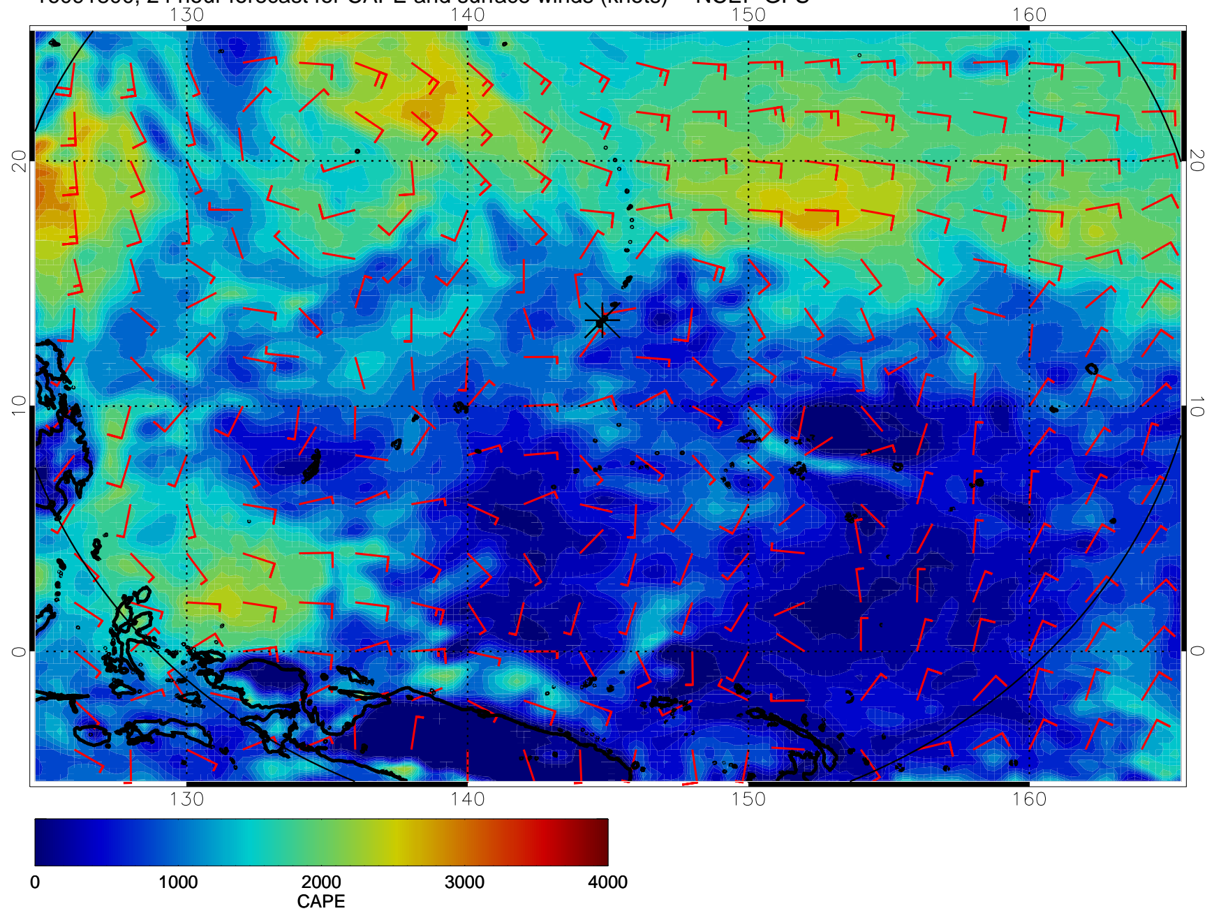
16091800, 24 hour forecast for CAPE and surface winds (knots) -- NCEP GFS
