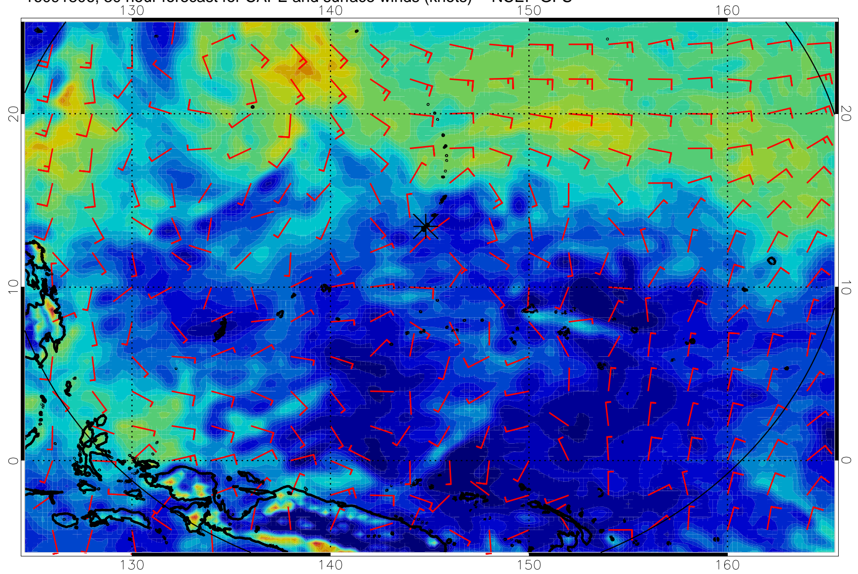
16091806, 30 hour forecast for CAPE and surface winds (knots) -- NCEP GFS
