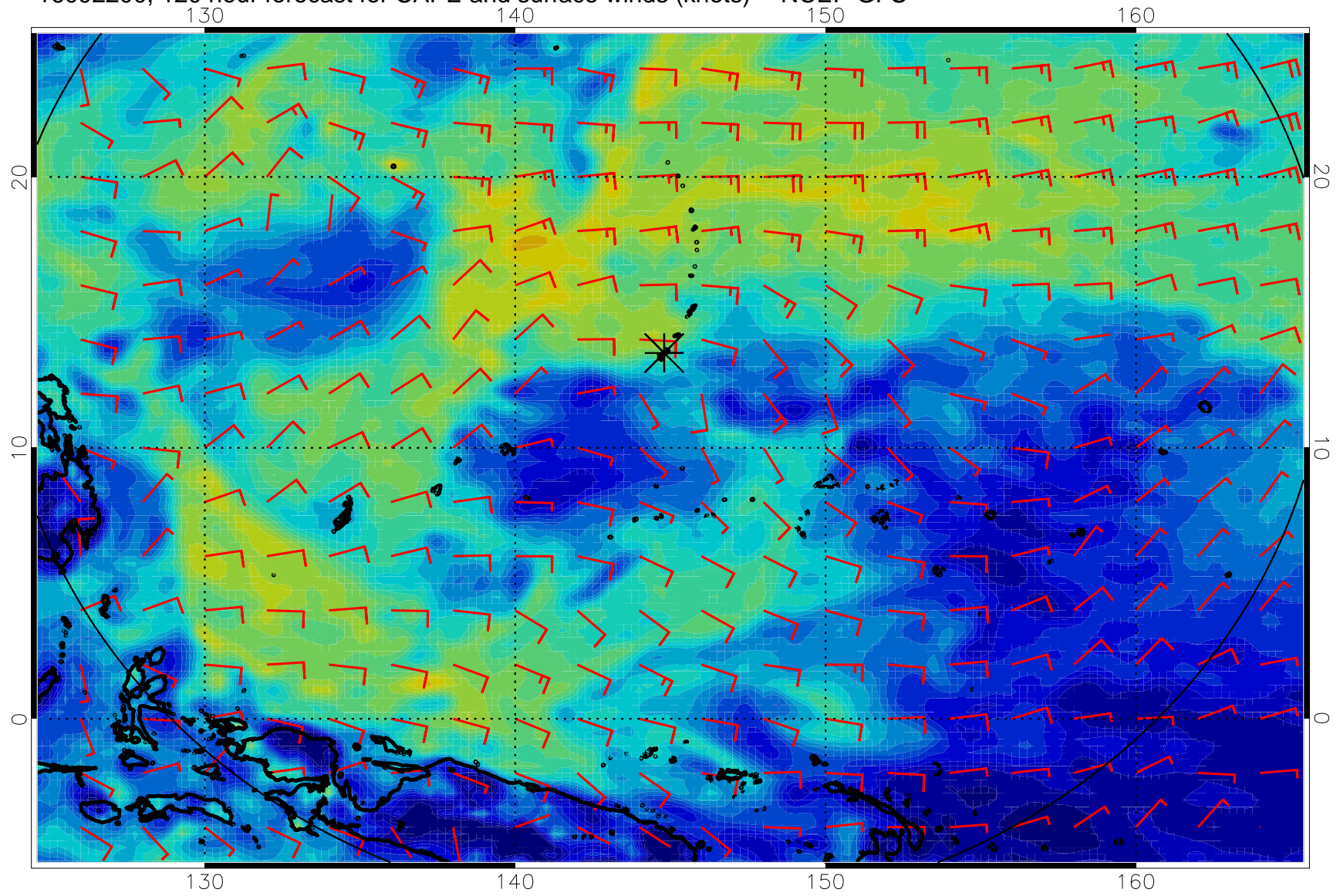
16092200, 120 hour forecast for CAPE and surface winds (knots) -- NCEP GFS
