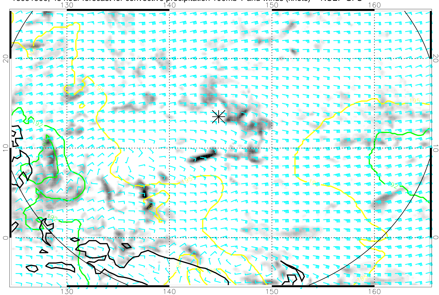
16091900, 48 hour forecast for convective precipitation 100mb T and winds (knots) -- NCEP GFS
