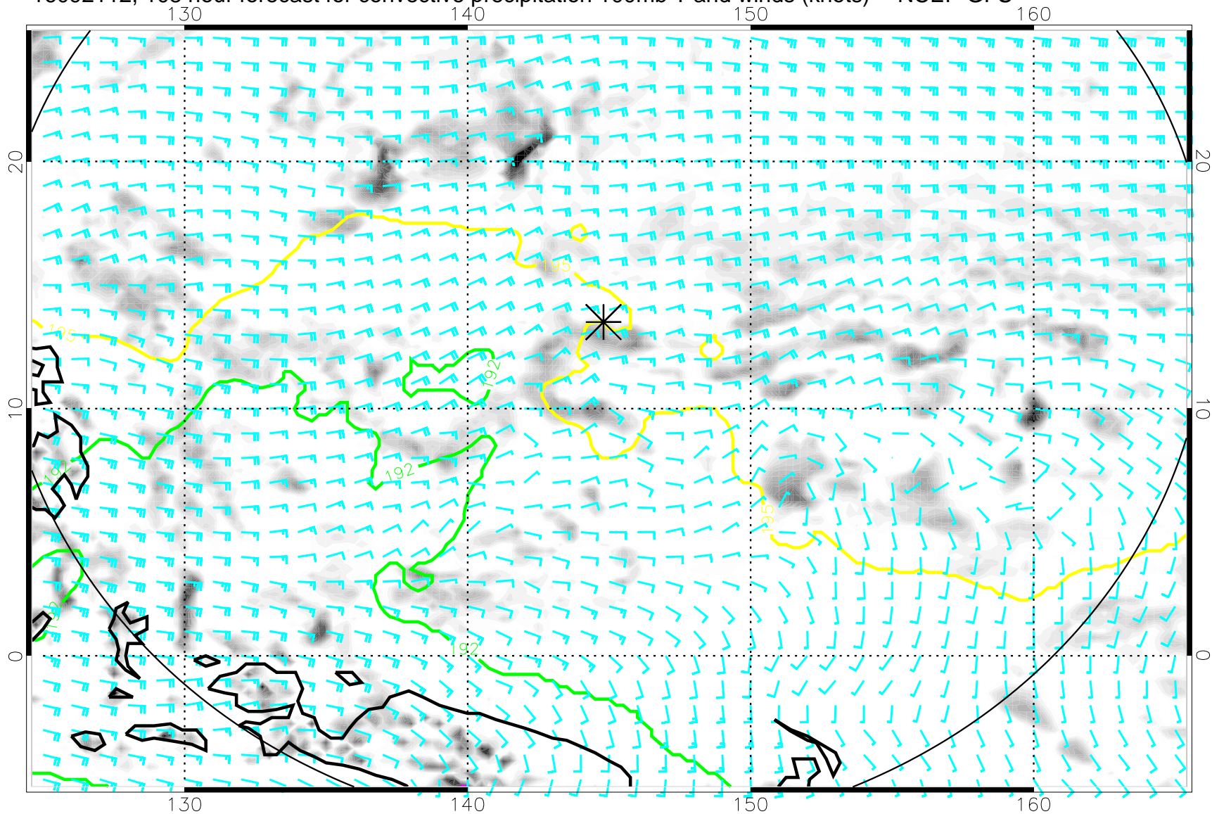
16092112, 108 hour forecast for convective precipitation 100mb T and winds (knots) -- NCEP GFS
