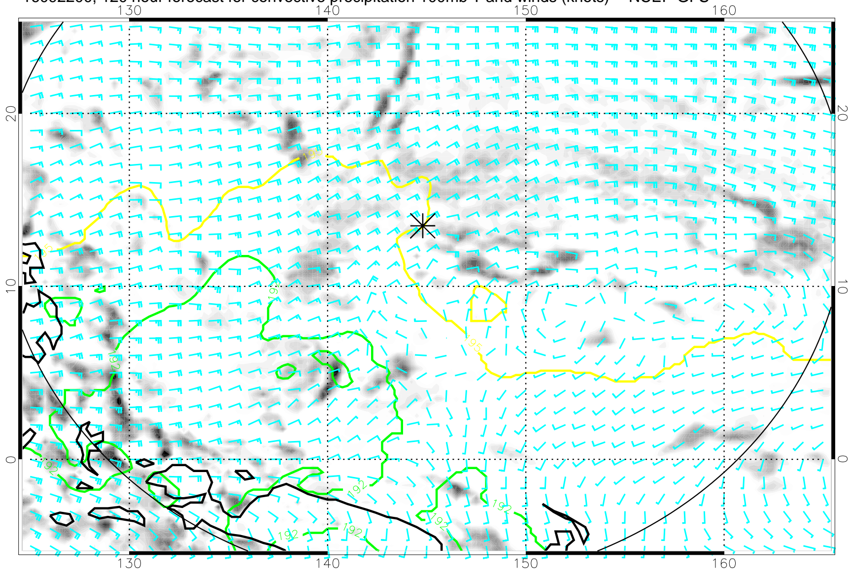
16092200, 120 hour forecast for convective precipitation 100mb T and winds (knots) -- NCEP GFS
