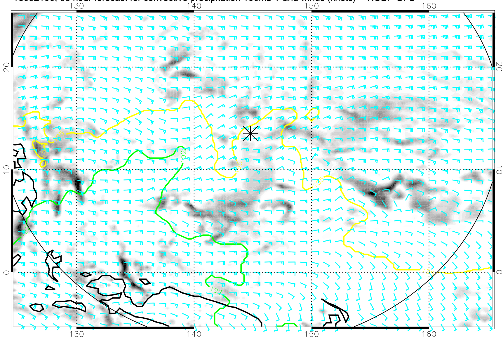
16092100, 96 hour forecast for convective precipitation 100mb T and winds (knots) -- NCEP GFS
