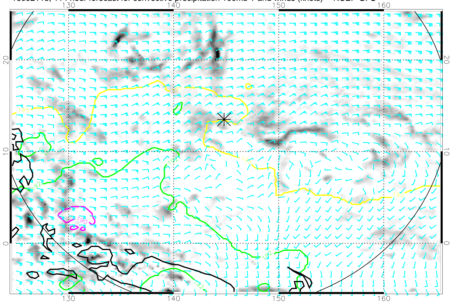
16092118, 114 hour forecast for convective precipitation 100mb T and winds (knots) -- NCEP GFS
