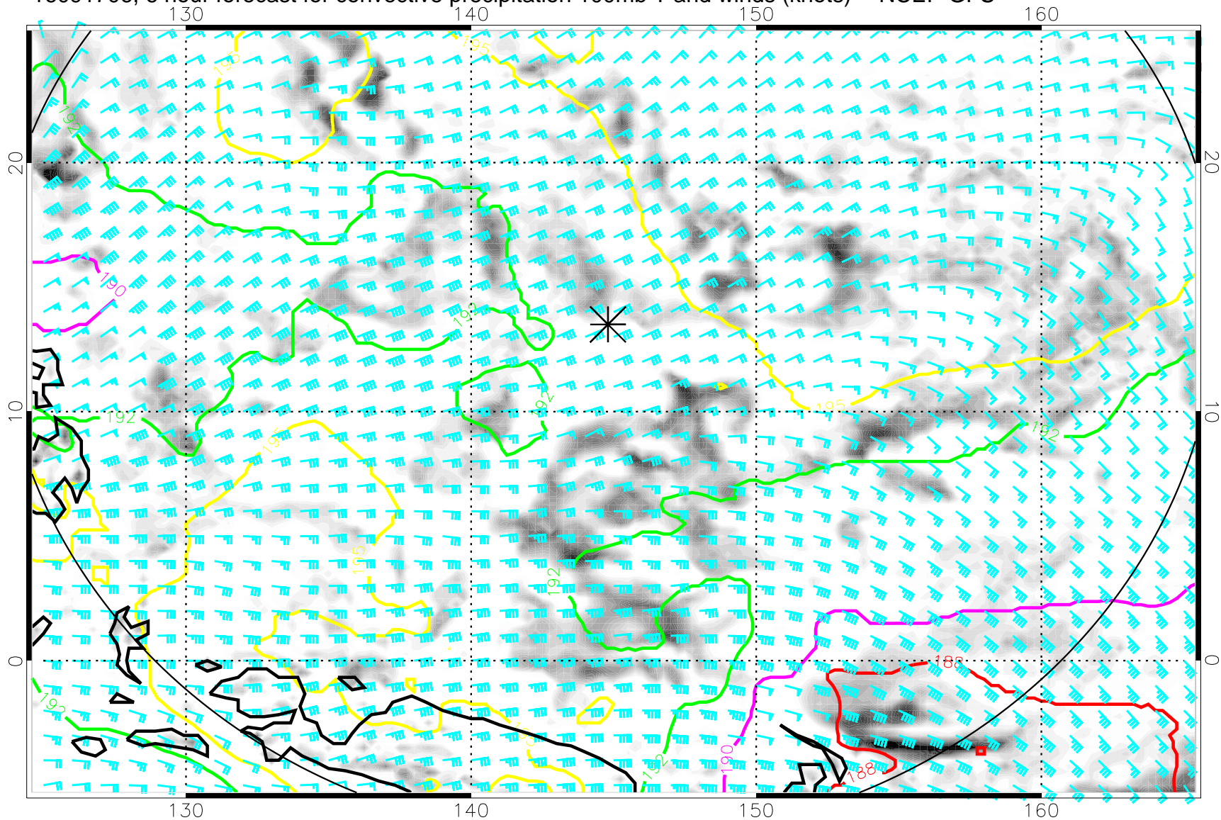
16091706, 6 hour forecast for convective precipitation 100mb T and winds (knots) -- NCEP GFS
