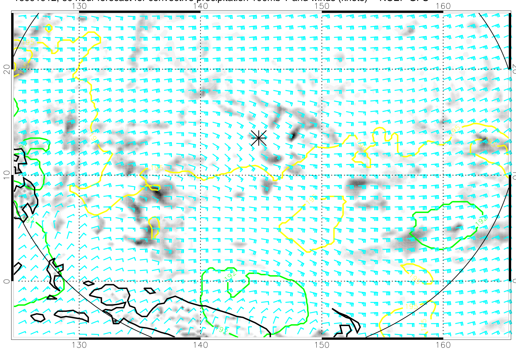
16091912, 60 hour forecast for convective precipitation 100mb T and winds (knots) -- NCEP GFS
