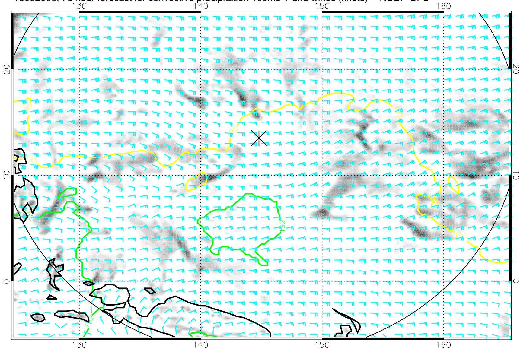
16092006, 78 hour forecast for convective precipitation 100mb T and winds (knots) -- NCEP GFS
