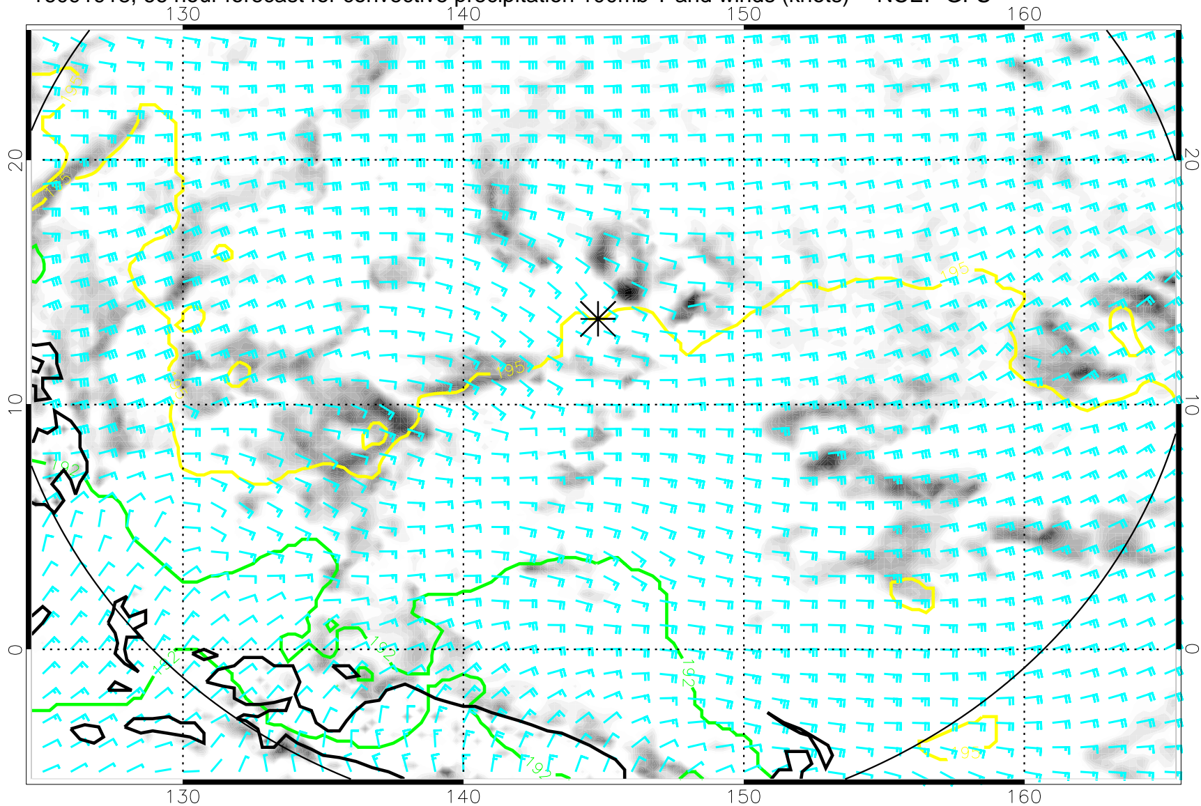
16091918, 66 hour forecast for convective precipitation 100mb T and winds (knots) -- NCEP GFS
