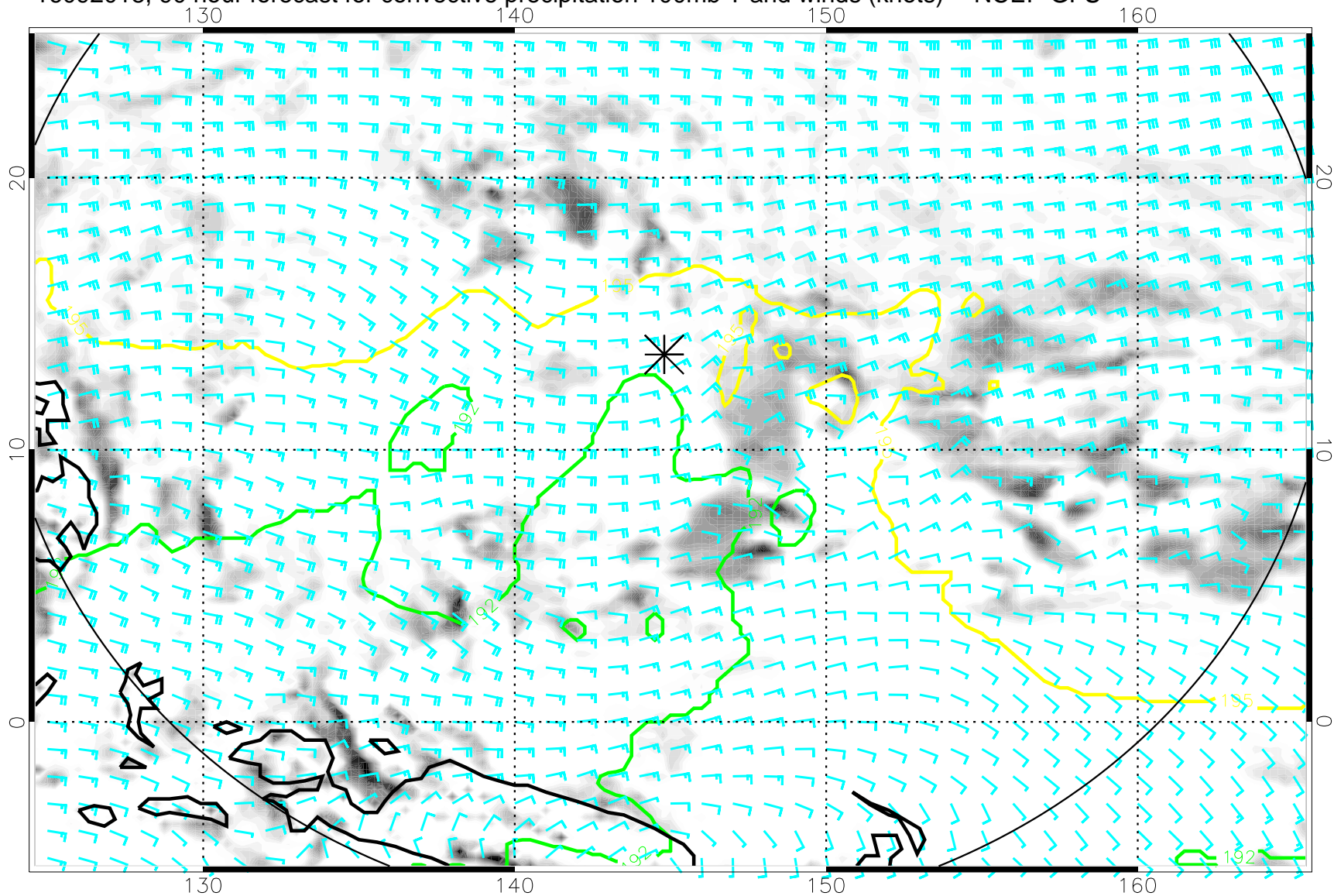
16092018, 90 hour forecast for convective precipitation 100mb T and winds (knots) -- NCEP GFS
