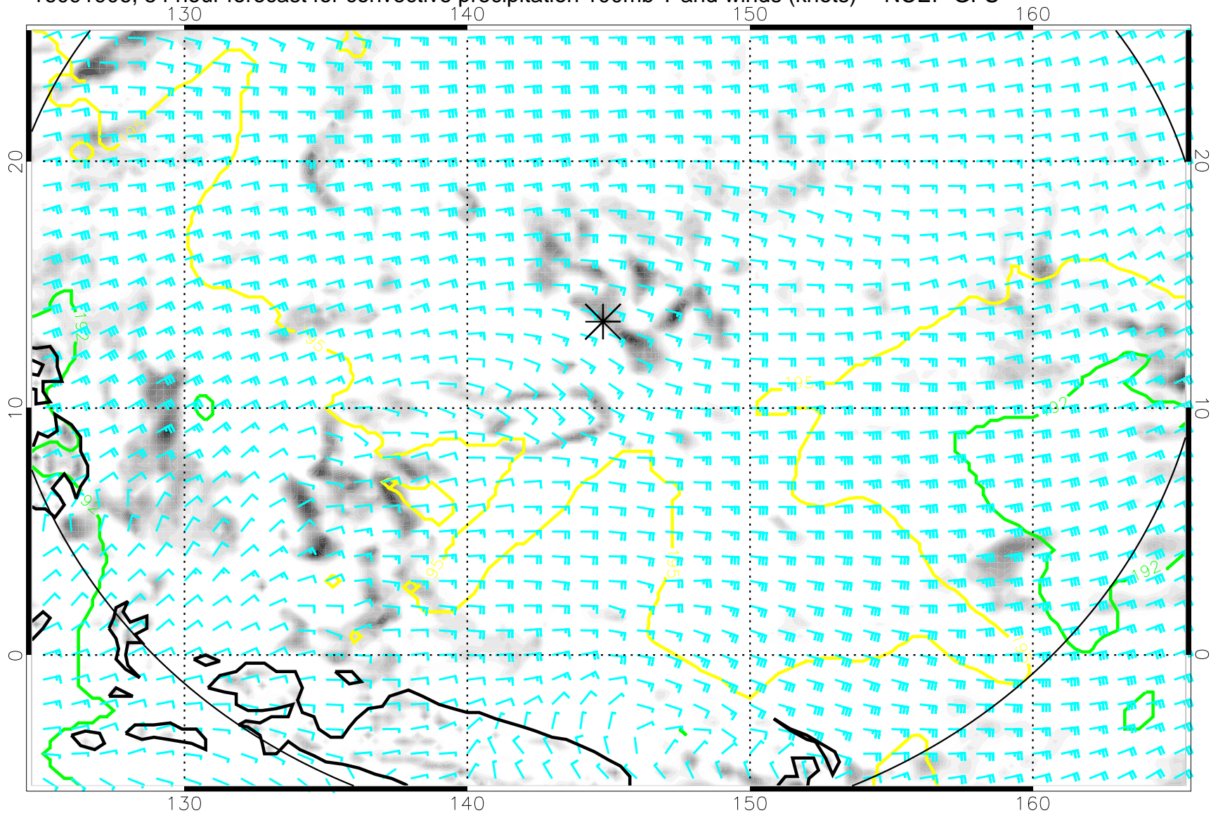
16091906, 54 hour forecast for convective precipitation 100mb T and winds (knots) -- NCEP GFS
