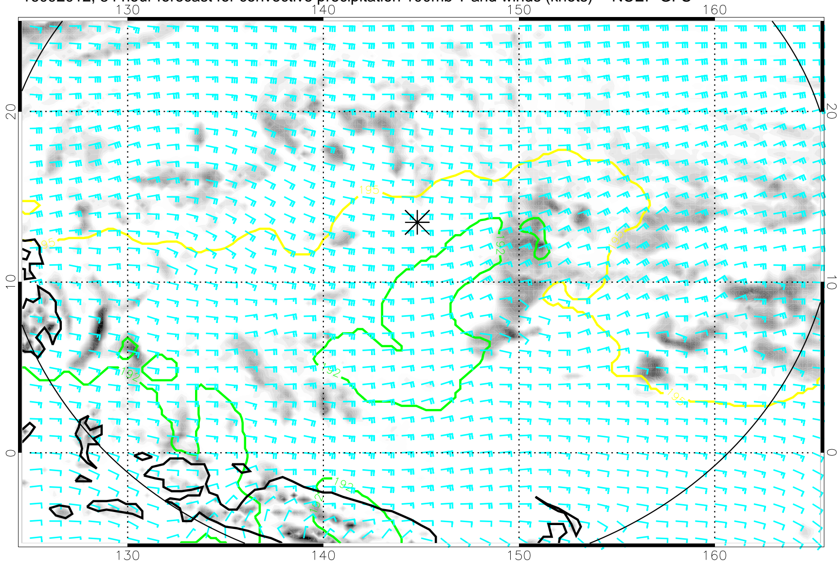
16092012, 84 hour forecast for convective precipitation 100mb T and winds (knots) -- NCEP GFS
