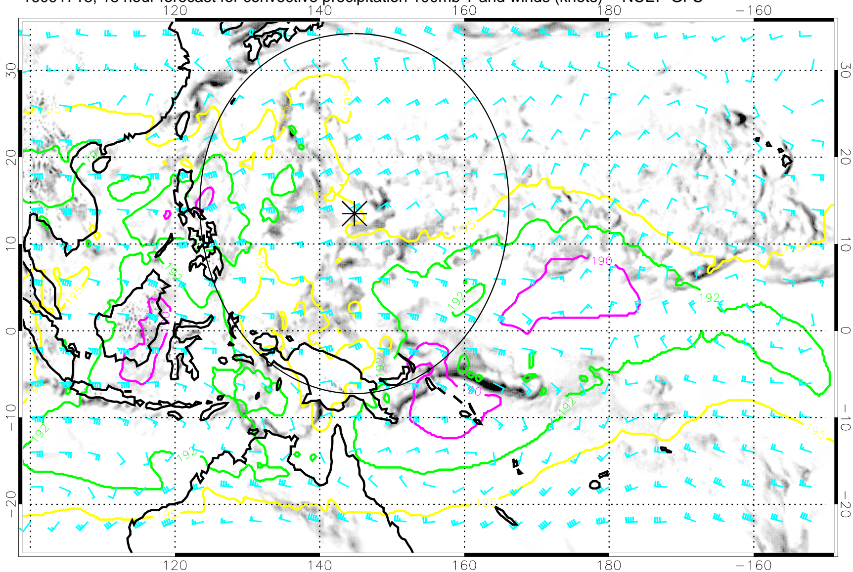
16091718, 18 hour forecast for convective precipitation 100mb T and winds (knots) -- NCEP GFS
