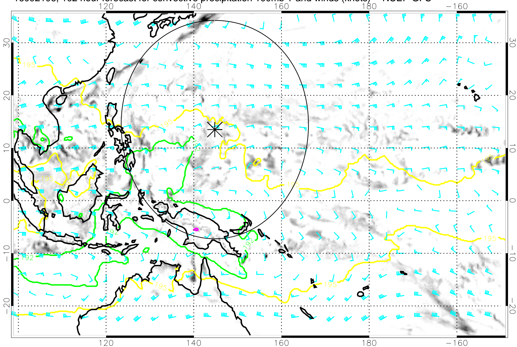
16092106, 102 hour forecast for convective precipitation 100mb T and winds (knots) -- NCEP GFS
