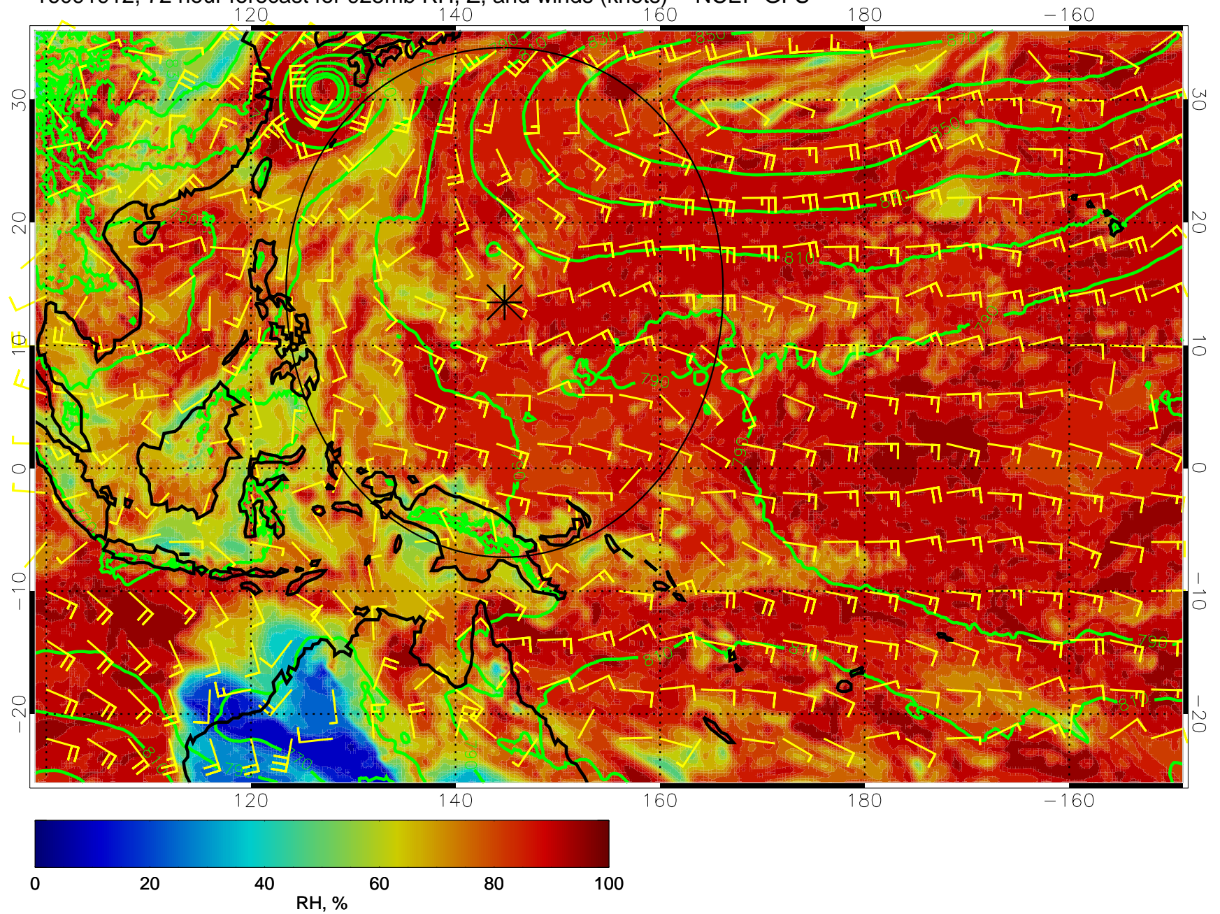
16091912, 72 hour forecast for 925mb RH, Z, and winds (knots) -- NCEP GFS
