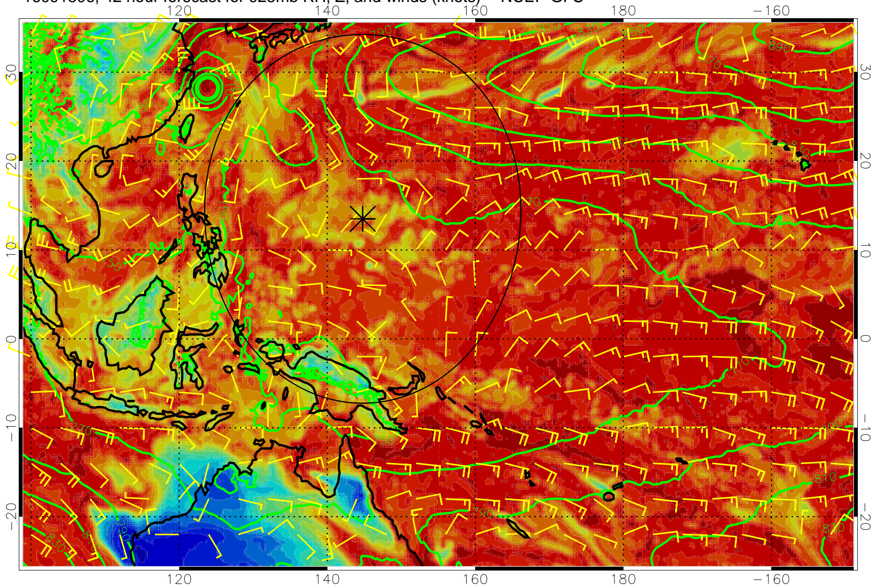
16091806, 42 hour forecast for 925mb RH, Z, and winds (knots) -- NCEP GFS
