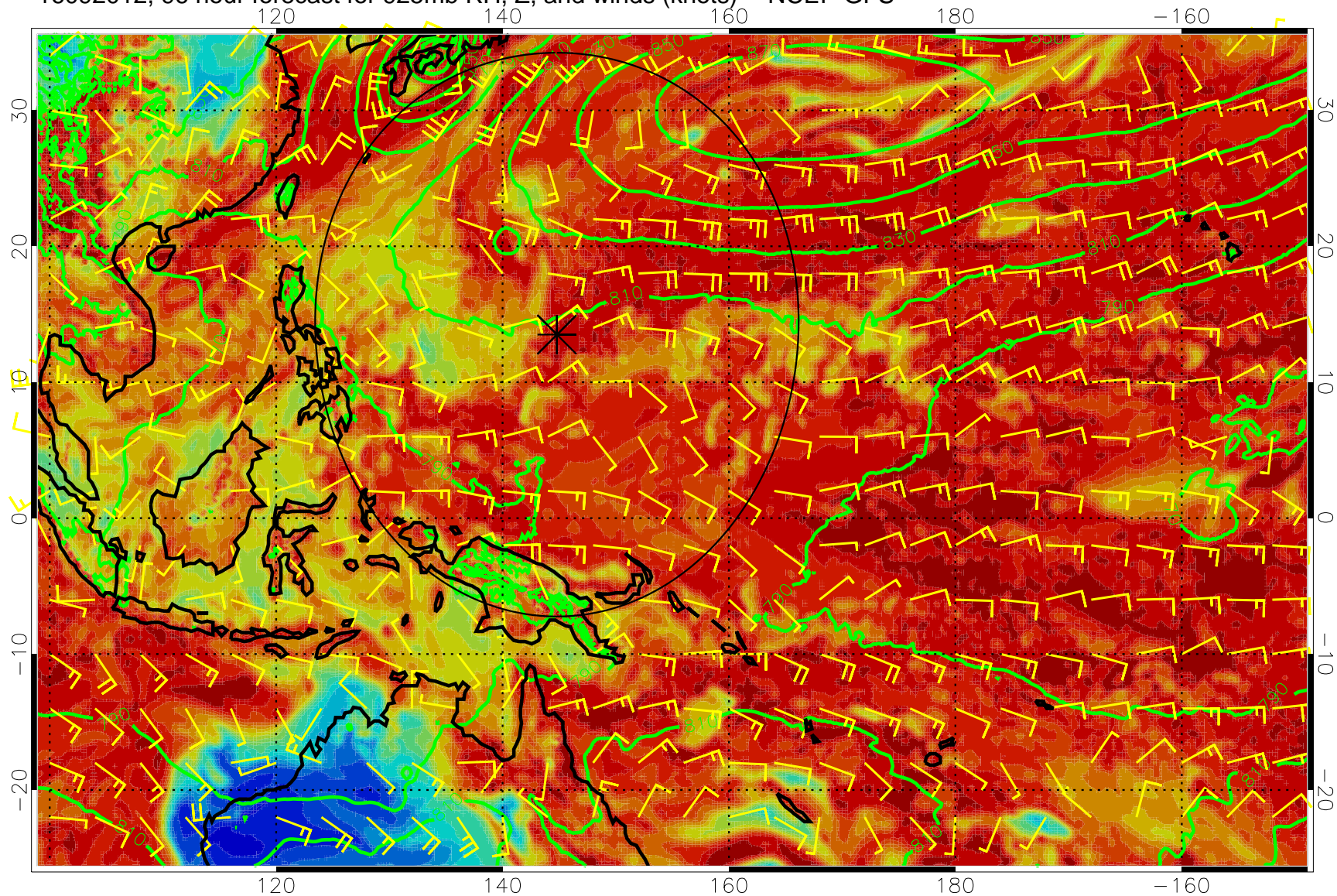
16092012, 96 hour forecast for 925mb RH, Z, and winds (knots) -- NCEP GFS
