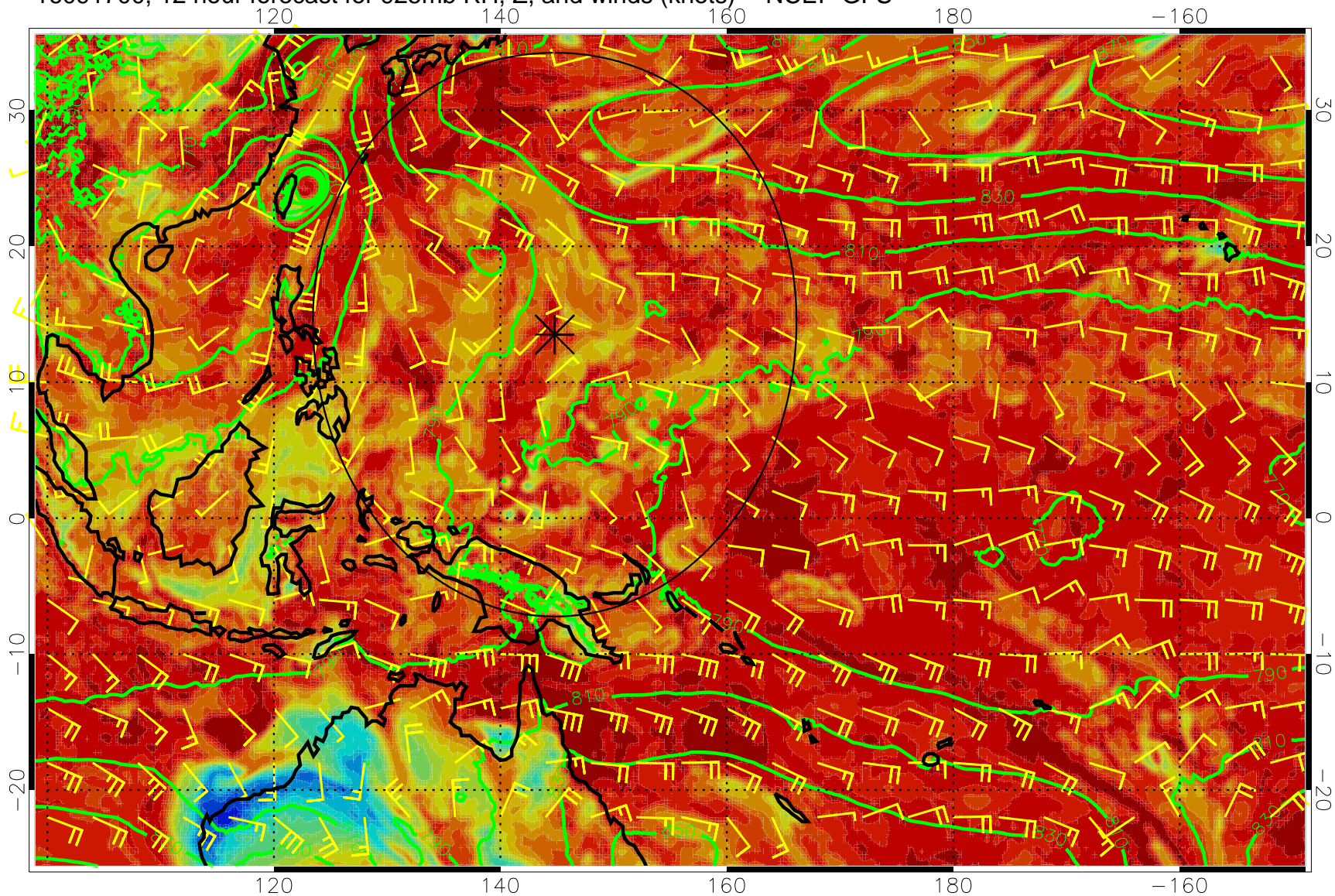
16091700, 12 hour forecast for 925mb RH, Z, and winds (knots) -- NCEP GFS
