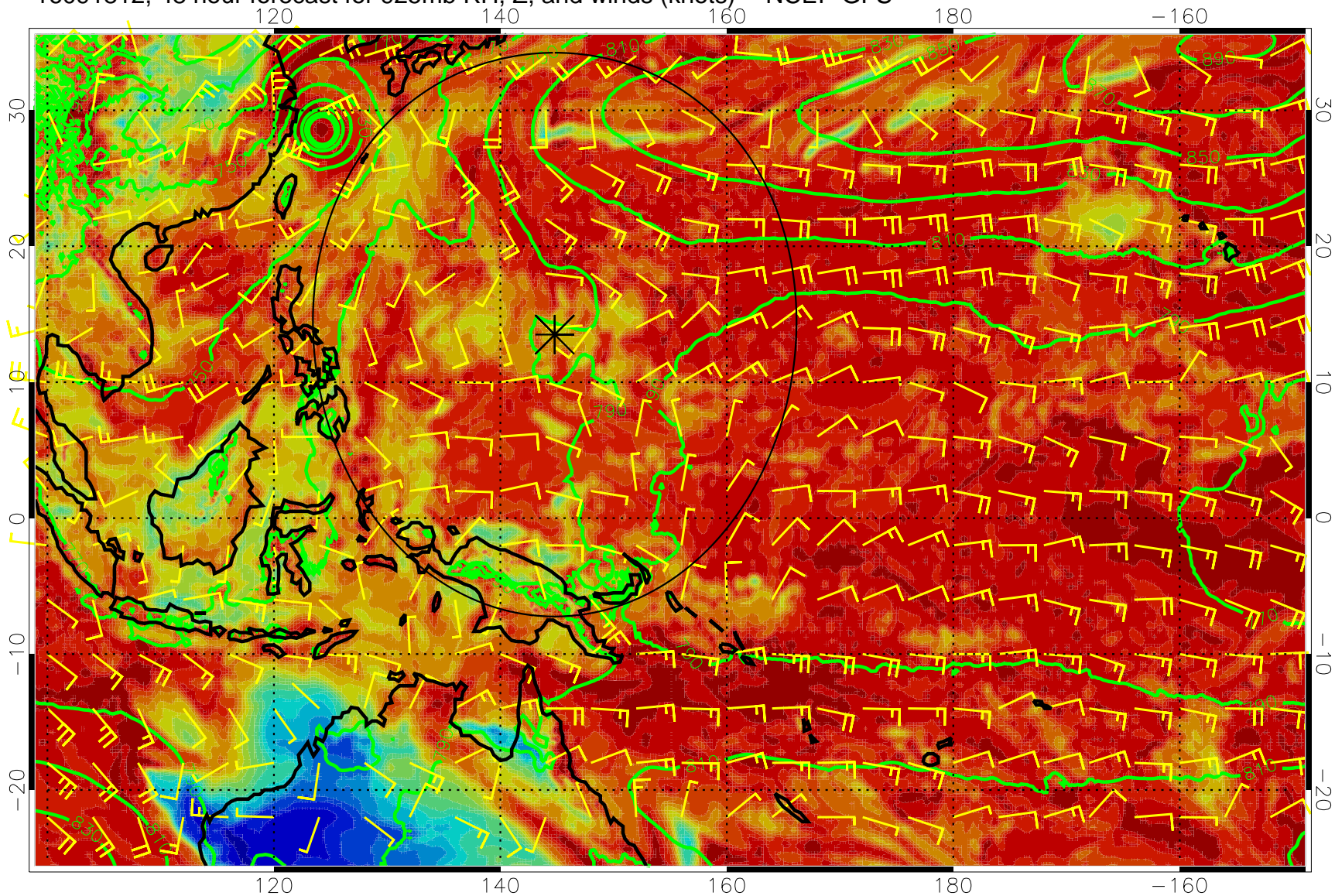
16091812, 48 hour forecast for 925mb RH, Z, and winds (knots) -- NCEP GFS
