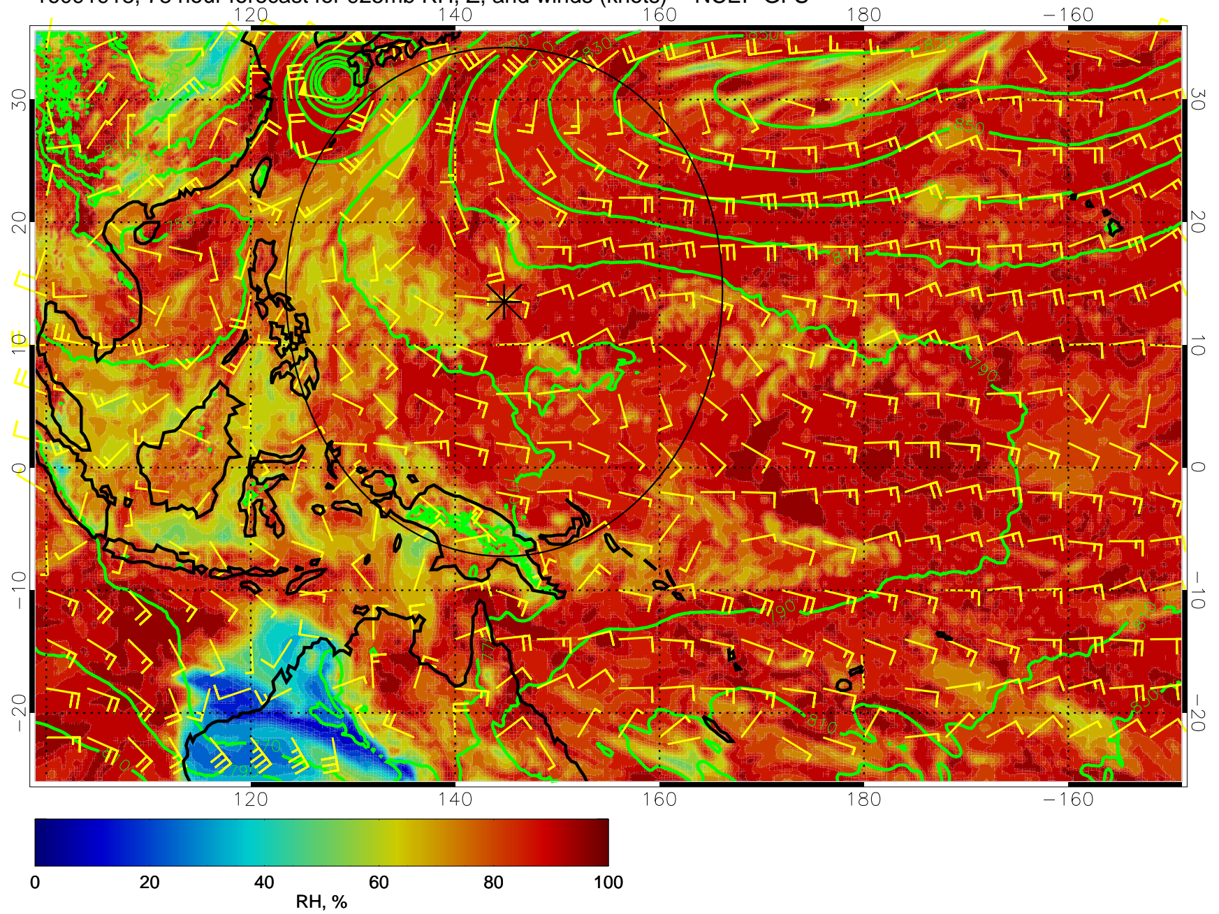
16091918, 78 hour forecast for 925mb RH, Z, and winds (knots) -- NCEP GFS
