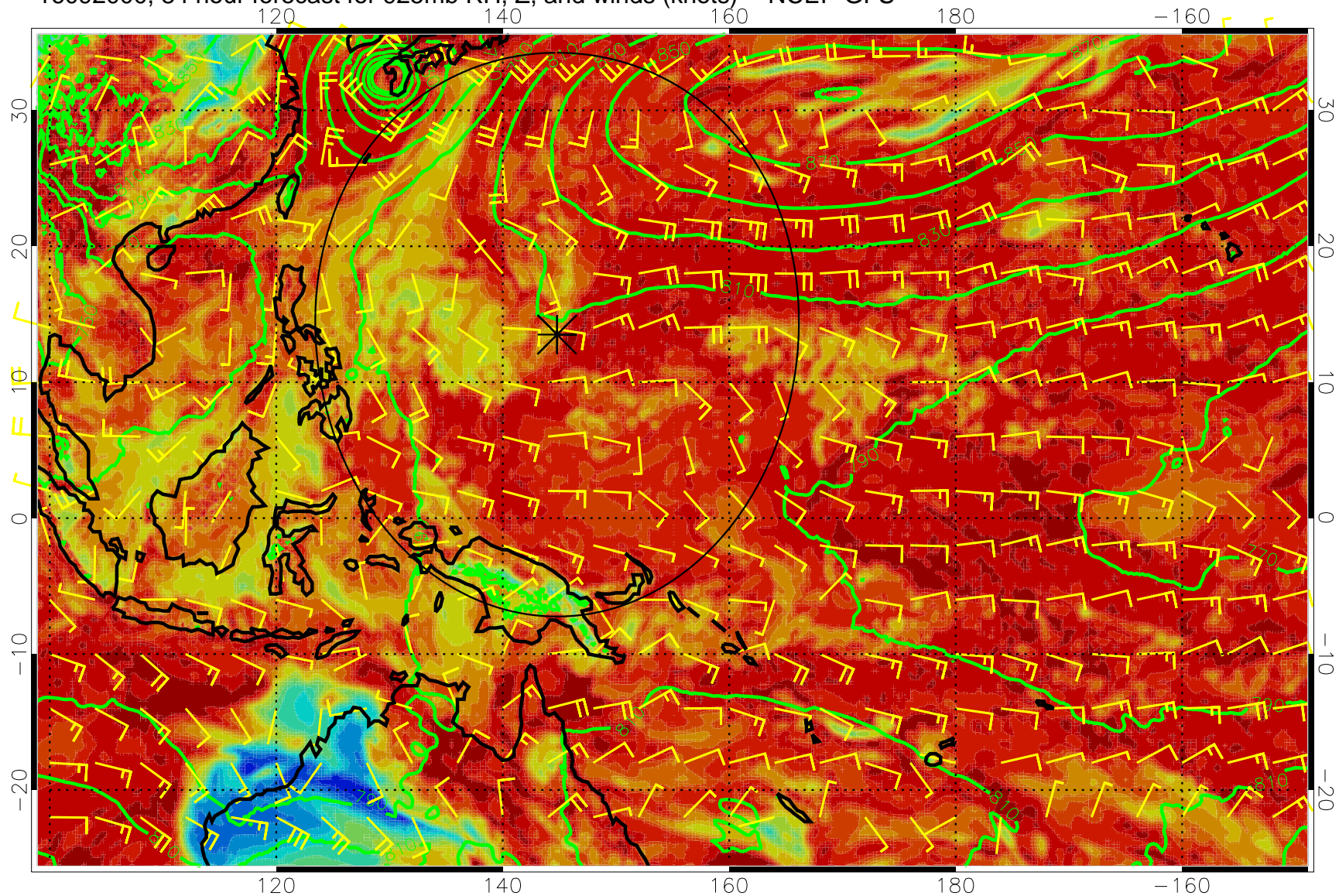
16092000, 84 hour forecast for 925mb RH, Z, and winds (knots) -- NCEP GFS
