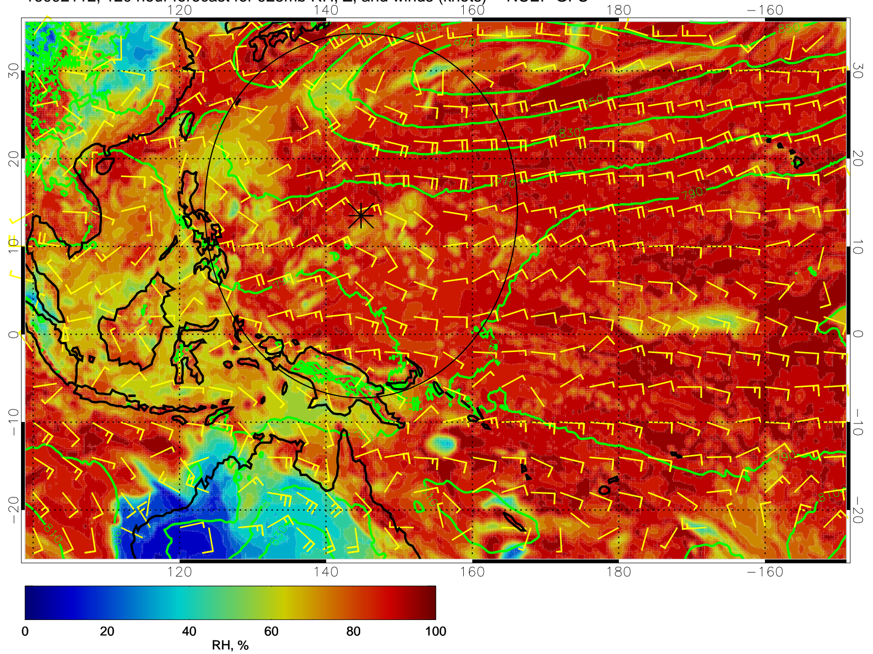
16092112, 120 hour forecast for 925mb RH, Z, and winds (knots) -- NCEP GFS
