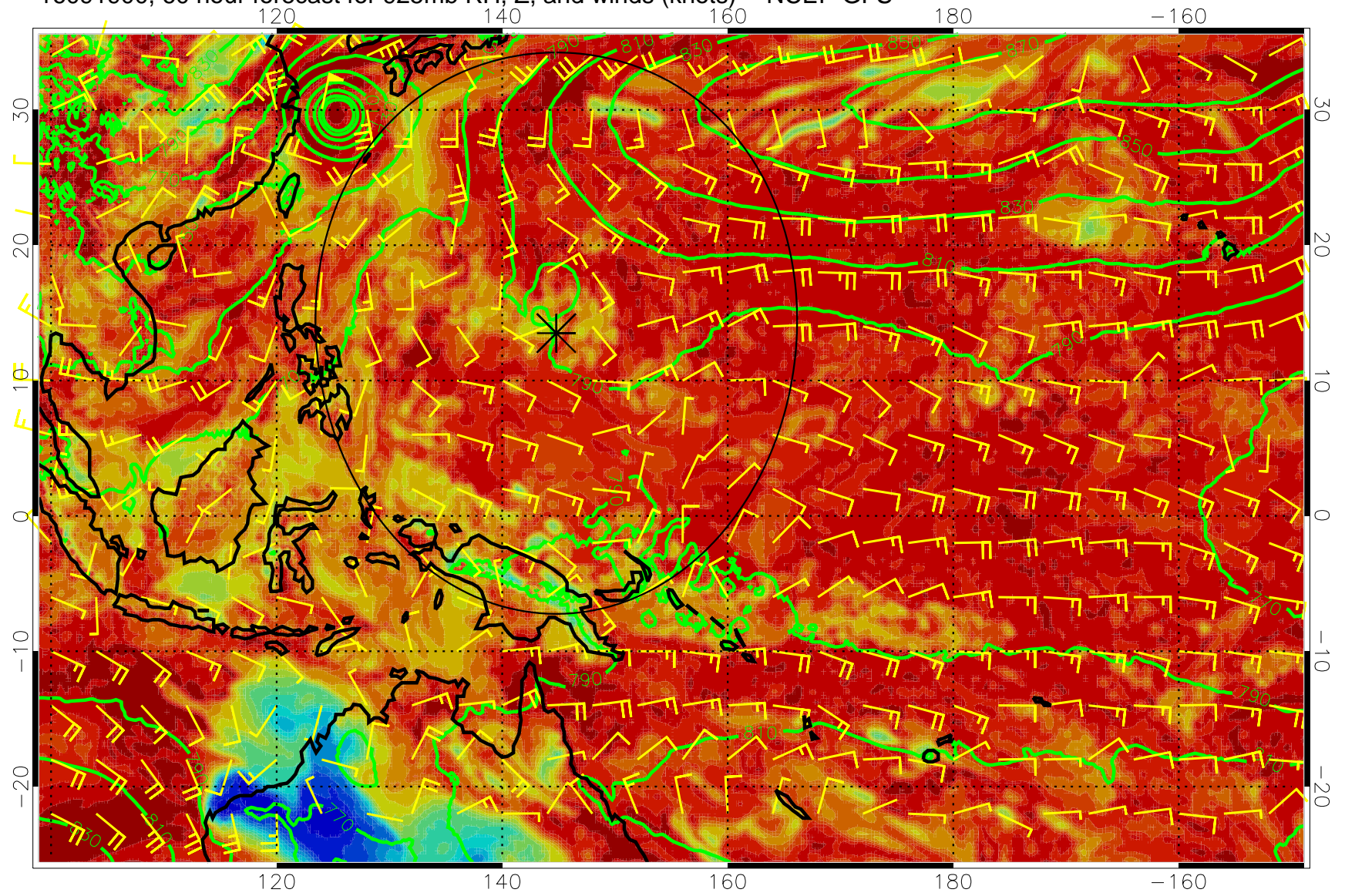
16091900, 60 hour forecast for 925mb RH, Z, and winds (knots) -- NCEP GFS
