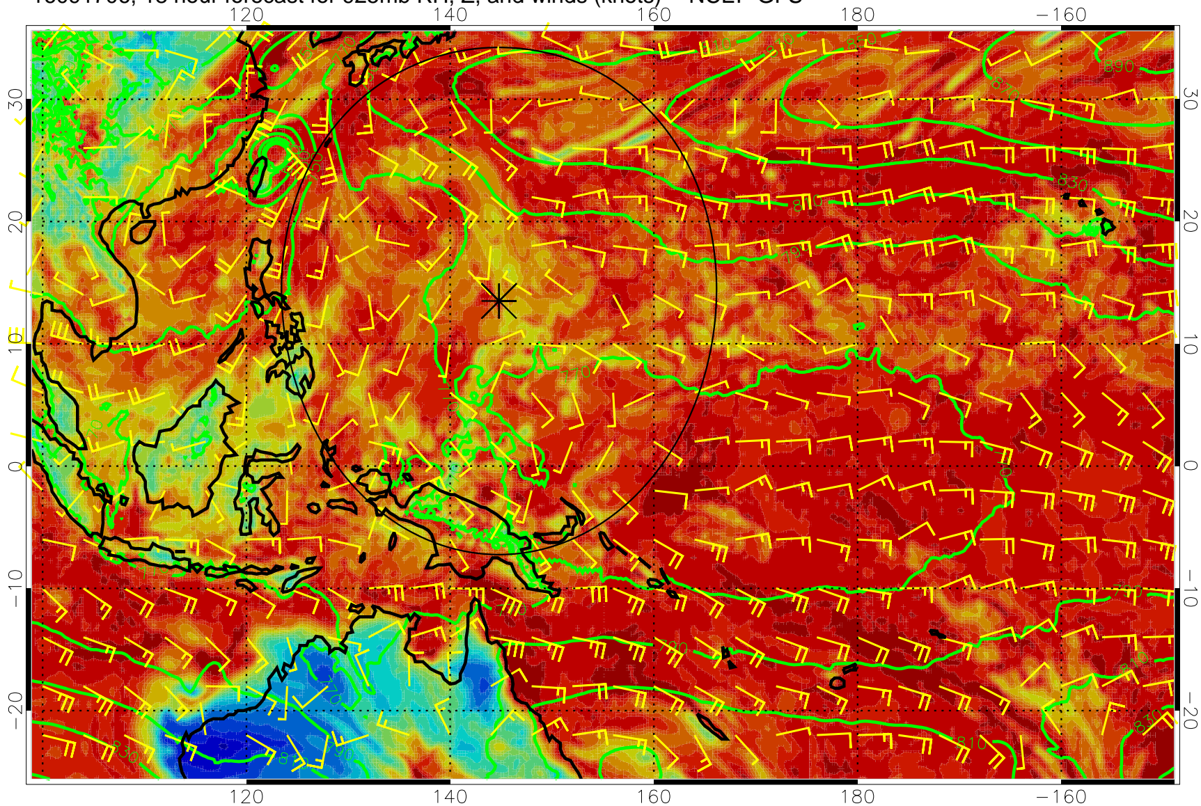
16091706, 18 hour forecast for 925mb RH, Z, and winds (knots) -- NCEP GFS
