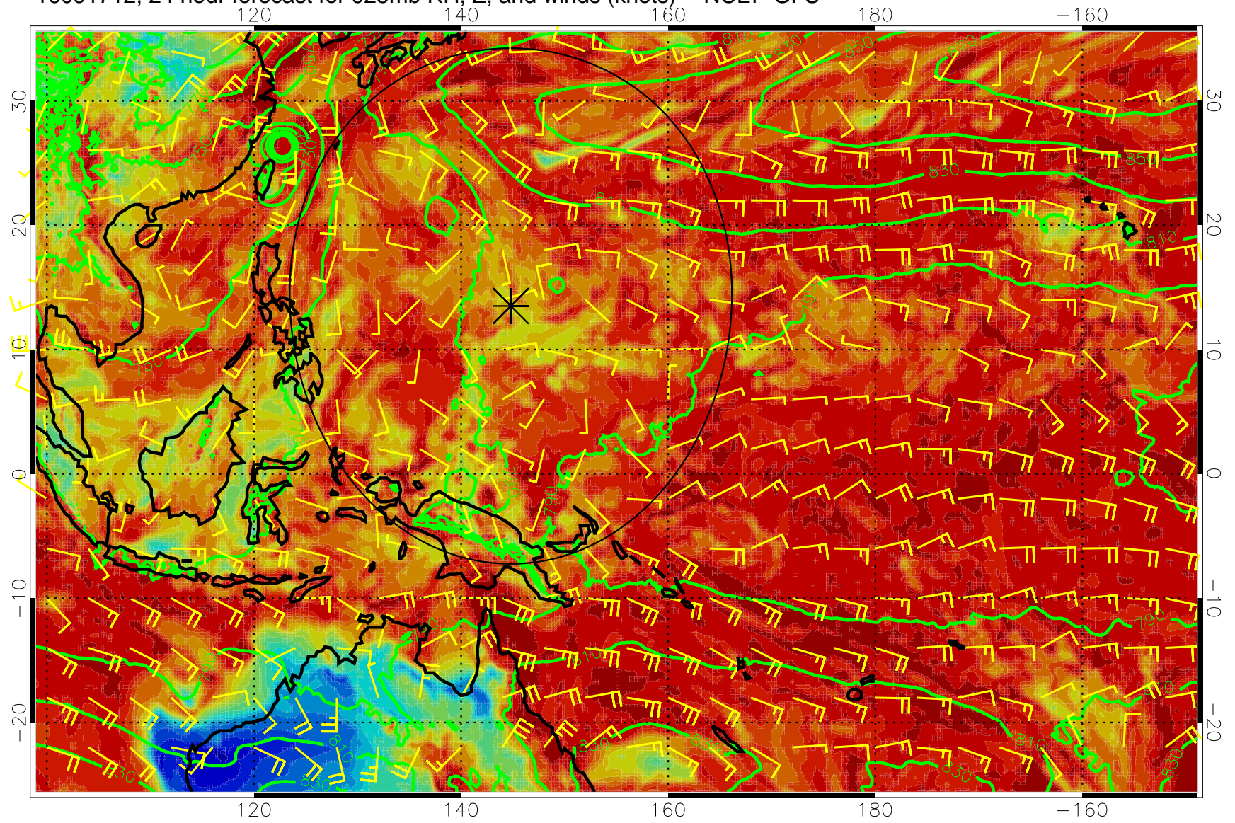
16091712, 24 hour forecast for 925mb RH, Z, and winds (knots) -- NCEP GFS
