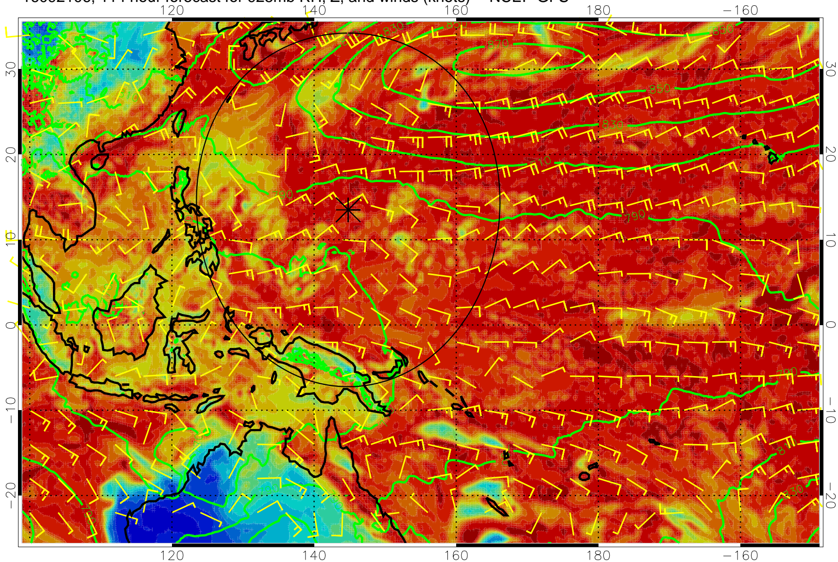
16092106, 114 hour forecast for 925mb RH, Z, and winds (knots) -- NCEP GFS
