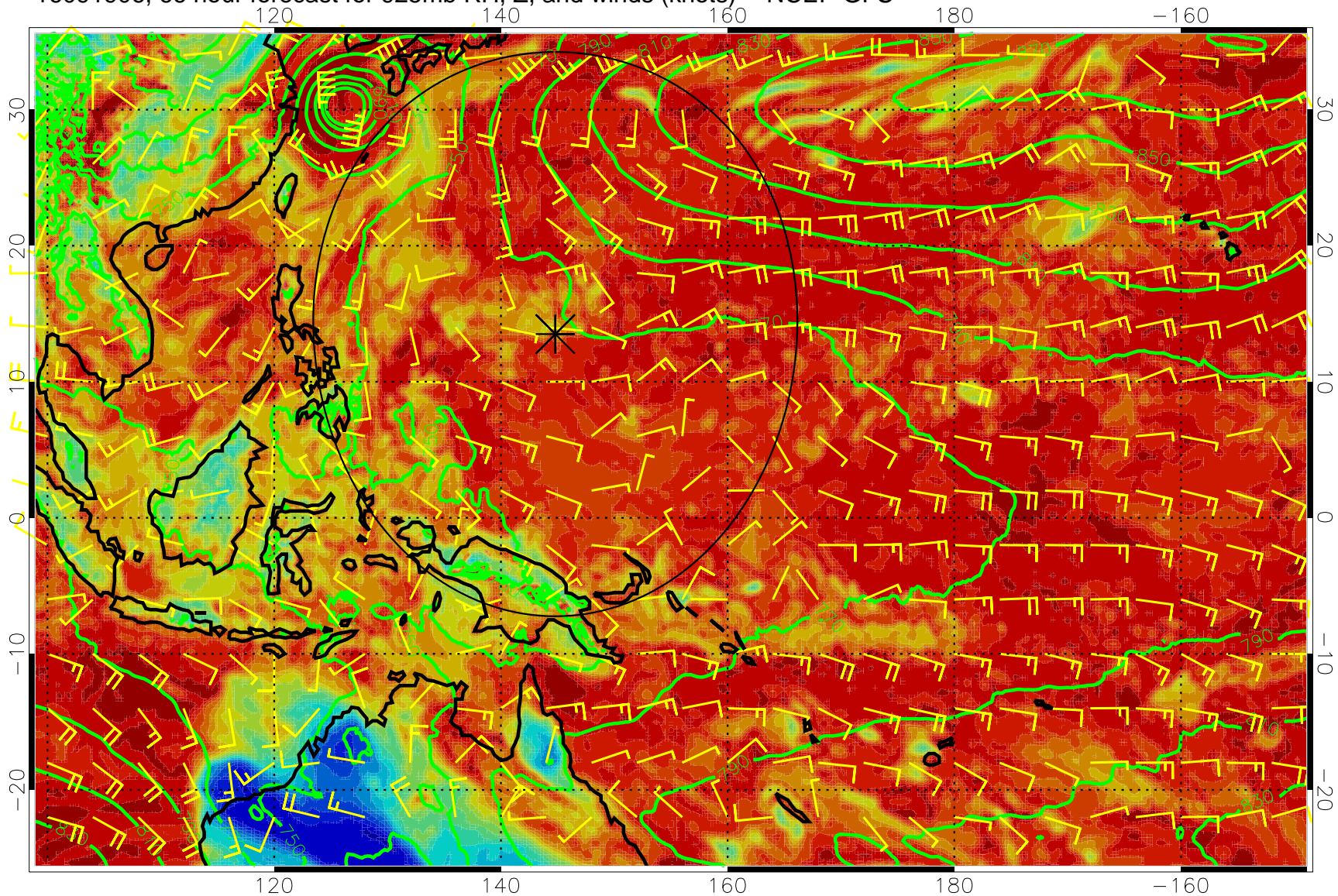
16091906, 66 hour forecast for 925mb RH, Z, and winds (knots) -- NCEP GFS
