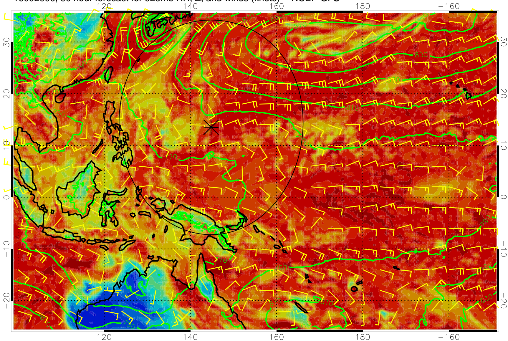
16092006, 90 hour forecast for 925mb RH, Z, and winds (knots) -- NCEP GFS
