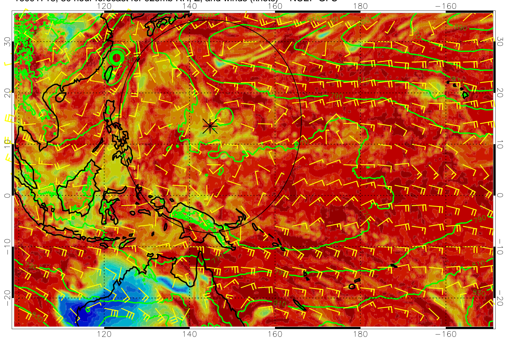
16091718, 30 hour forecast for 925mb RH, Z, and winds (knots) -- NCEP GFS
