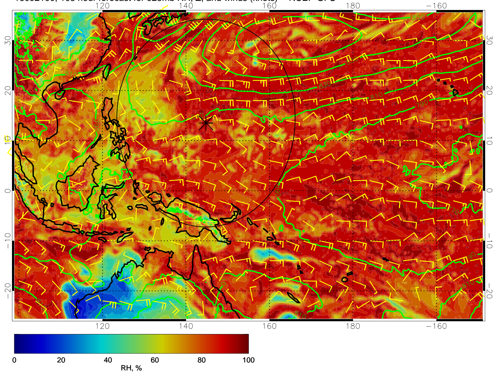
16092100, 108 hour forecast for 925mb RH, Z, and winds (knots) -- NCEP GFS
