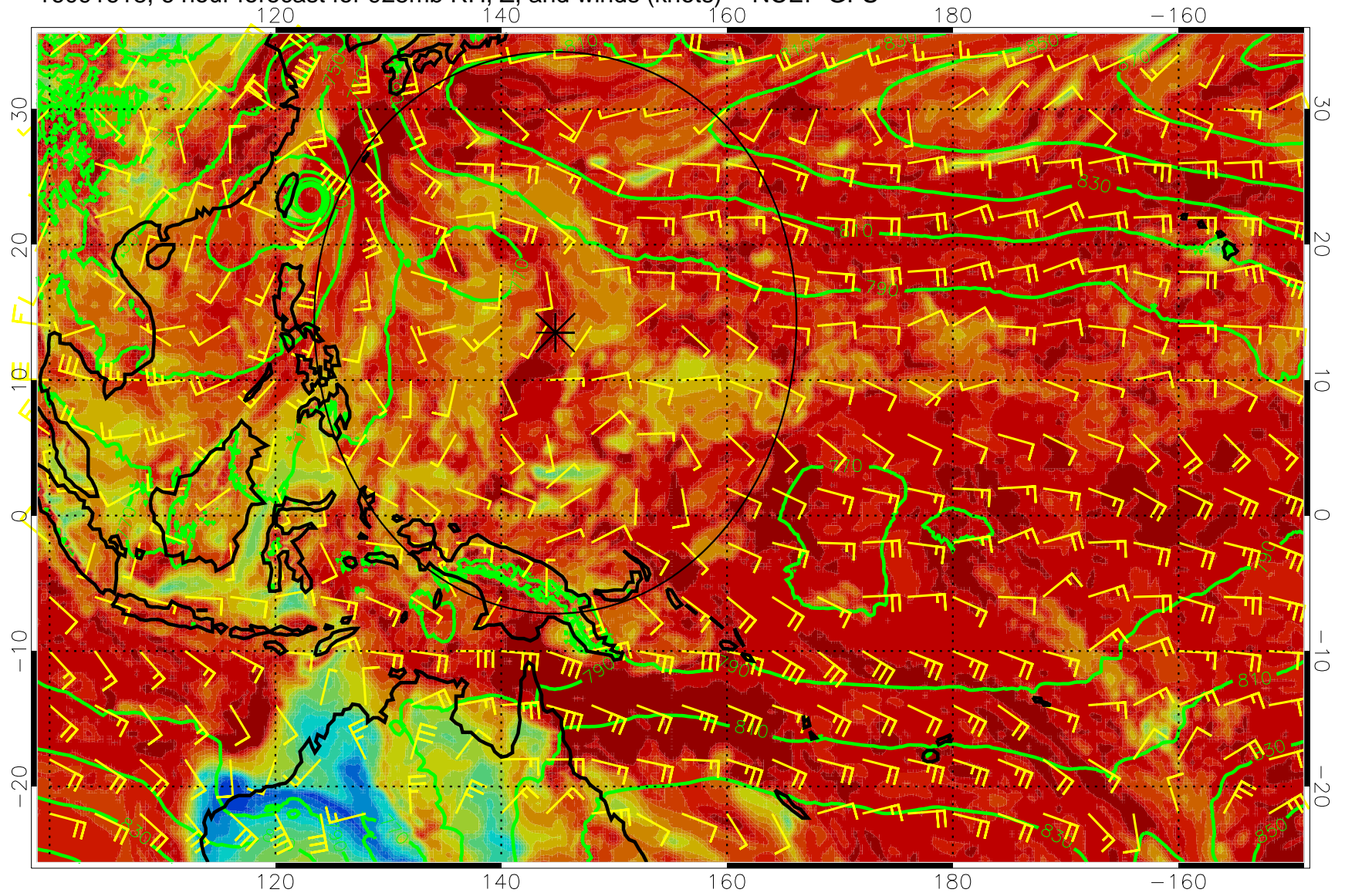
16091618, 6 hour forecast for 925mb RH, Z, and winds (knots) -- NCEP GFS
