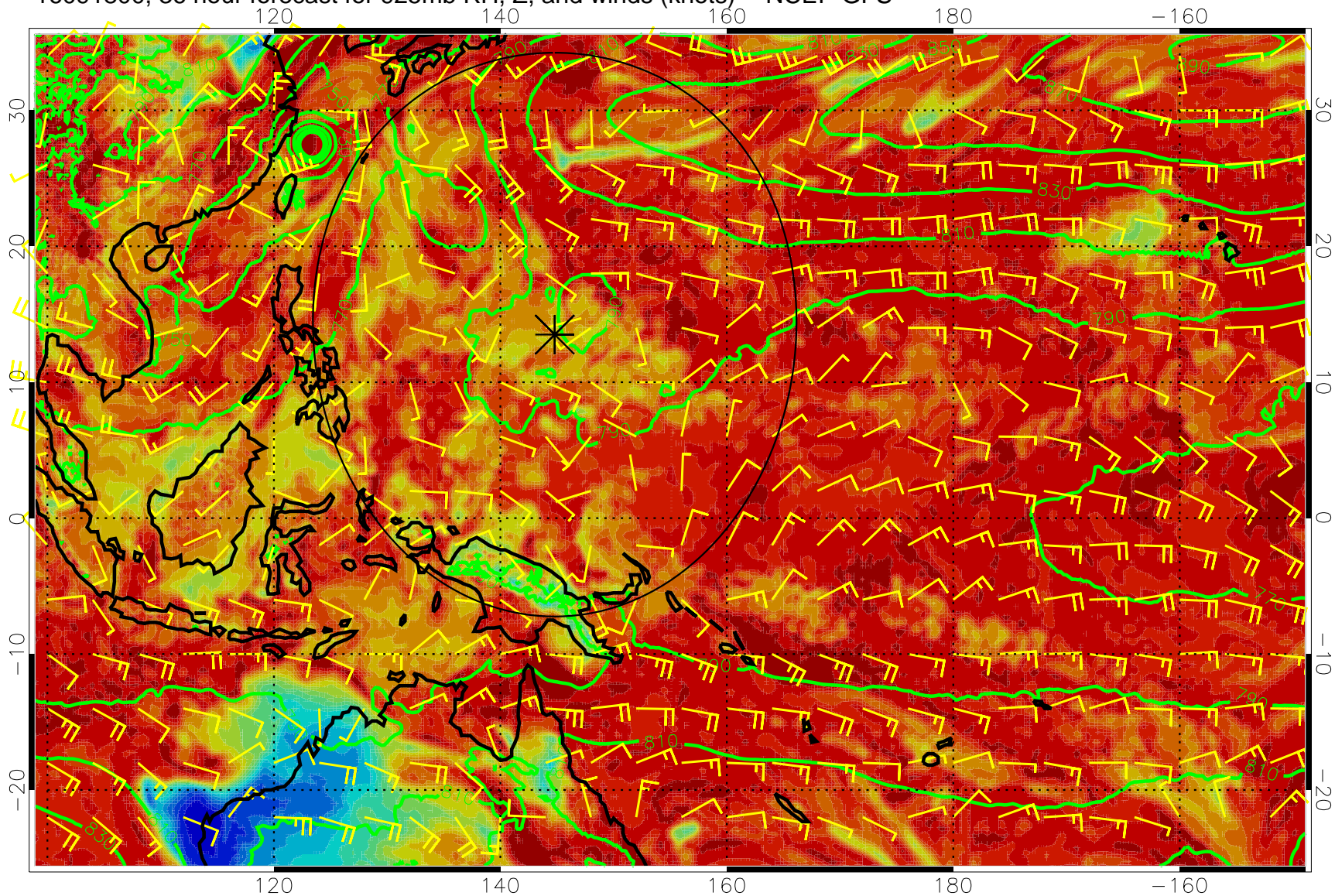
16091800, 36 hour forecast for 925mb RH, Z, and winds (knots) -- NCEP GFS
