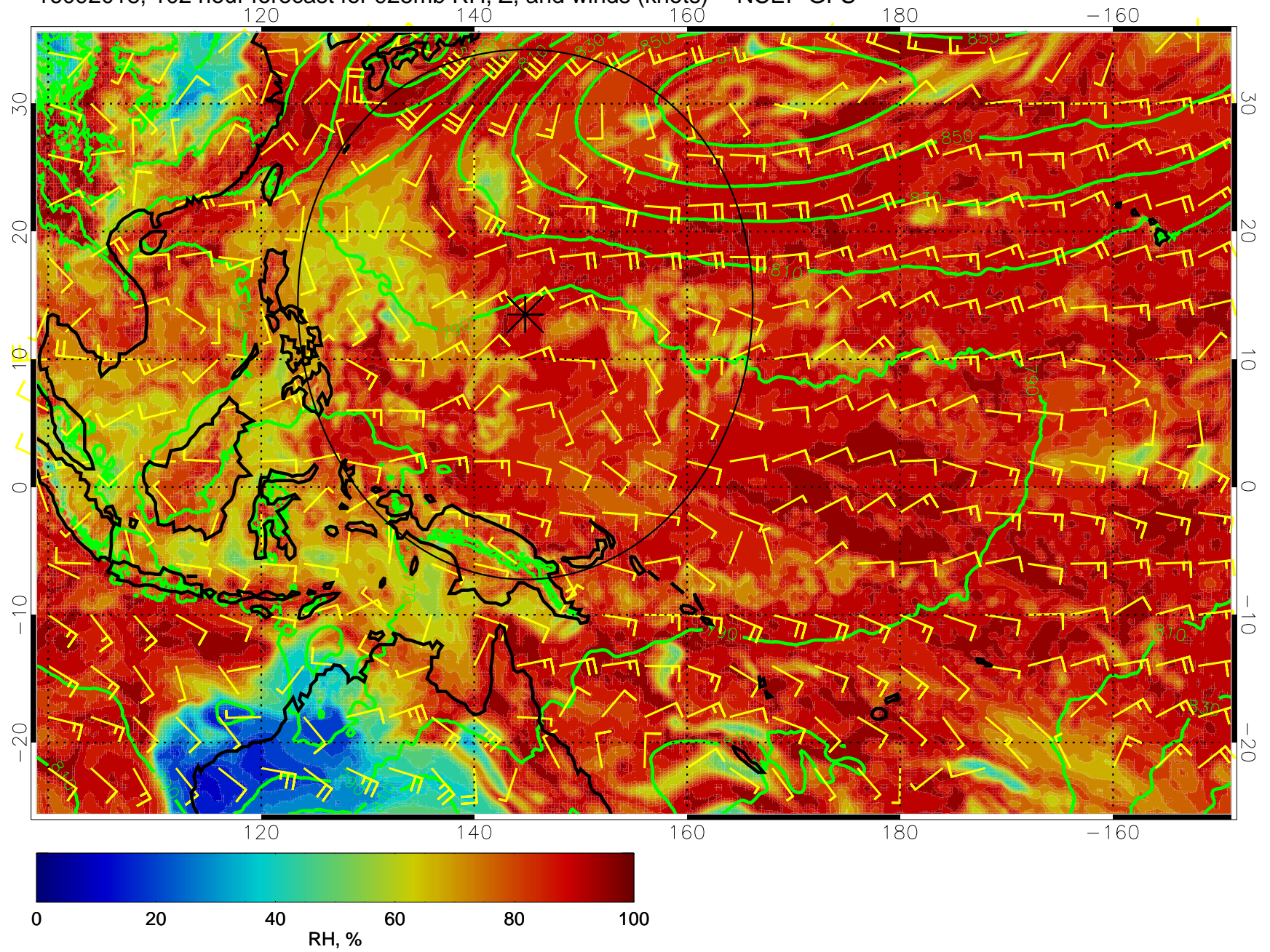
16092018, 102 hour forecast for 925mb RH, Z, and winds (knots) -- NCEP GFS
