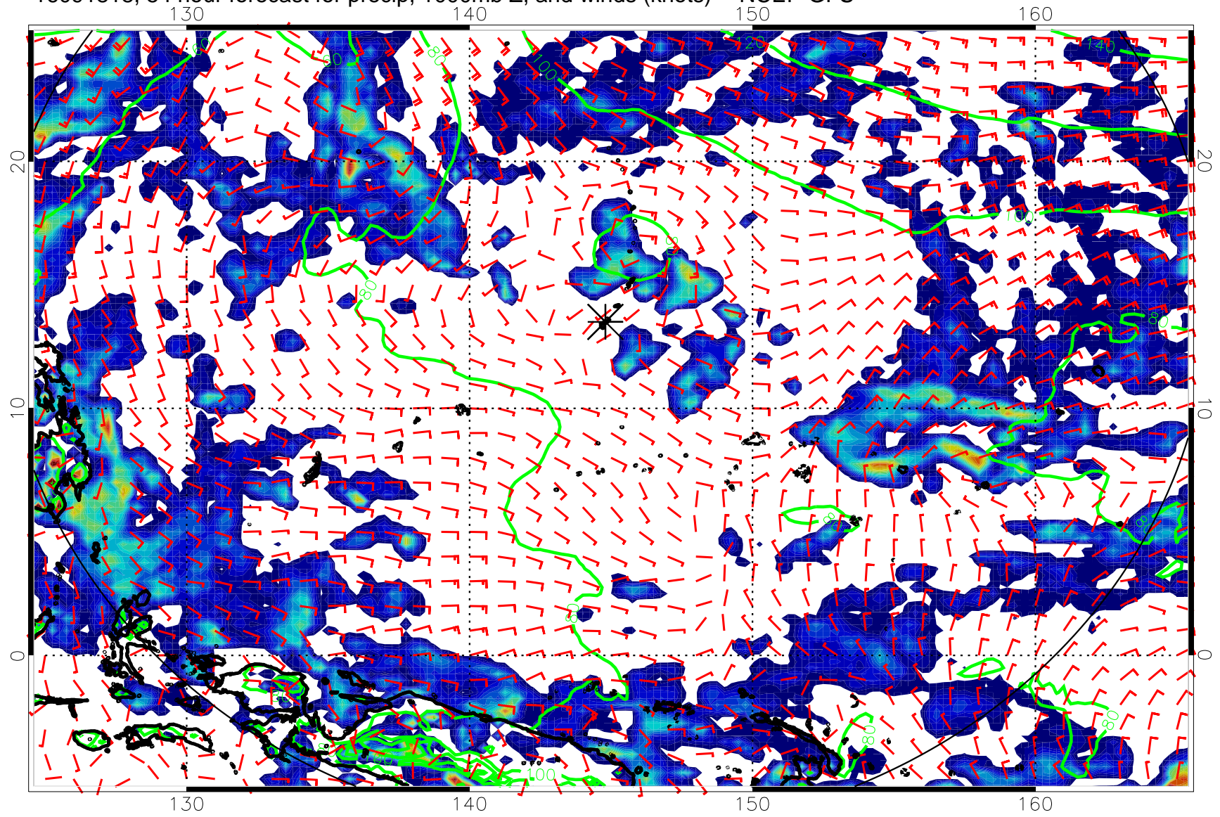
16091818, 54 hour forecast for precip, 1000mb Z, and winds (knots) -- NCEP GFS
