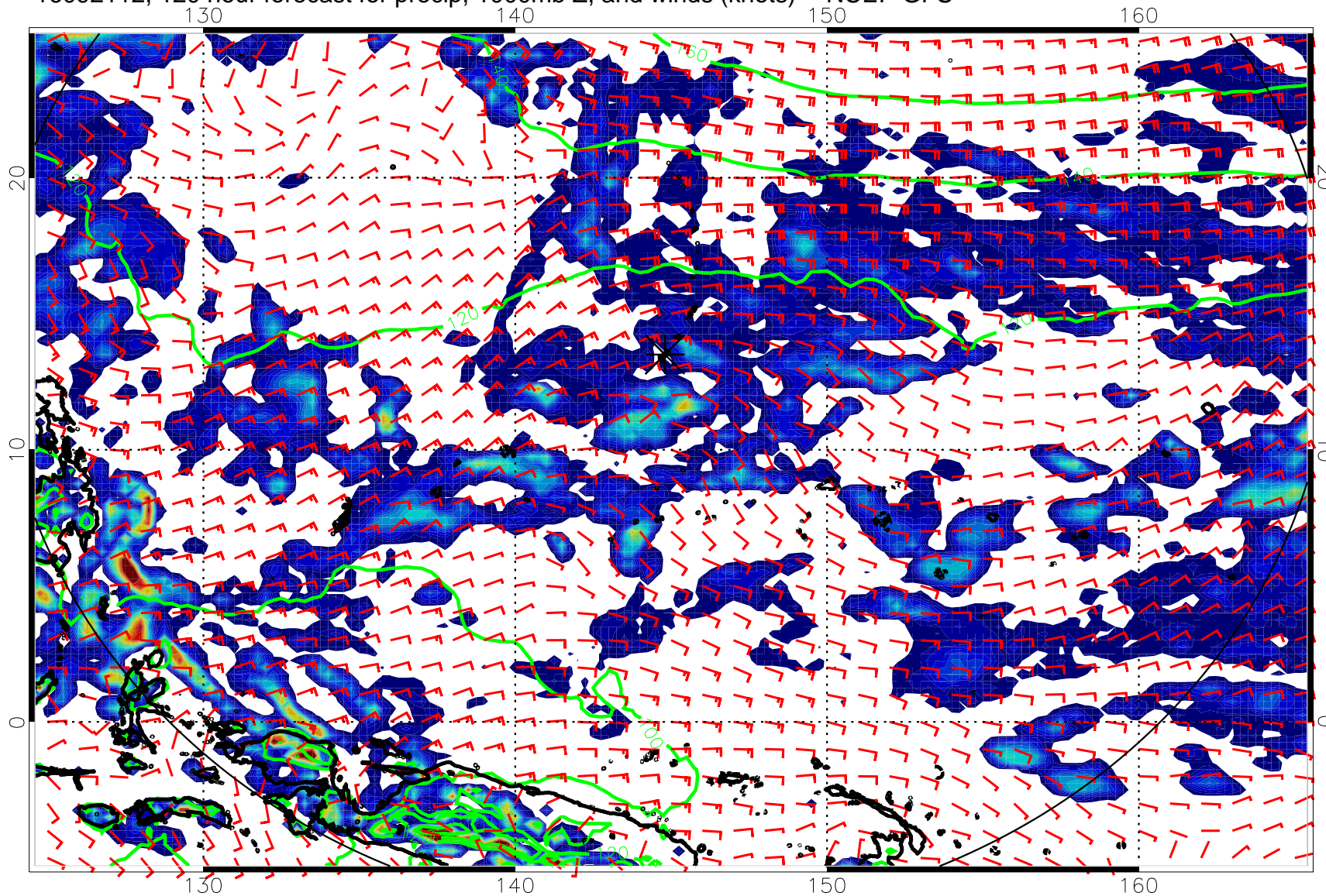
16092112, 120 hour forecast for precip, 1000mb Z, and winds (knots) -- NCEP GFS
