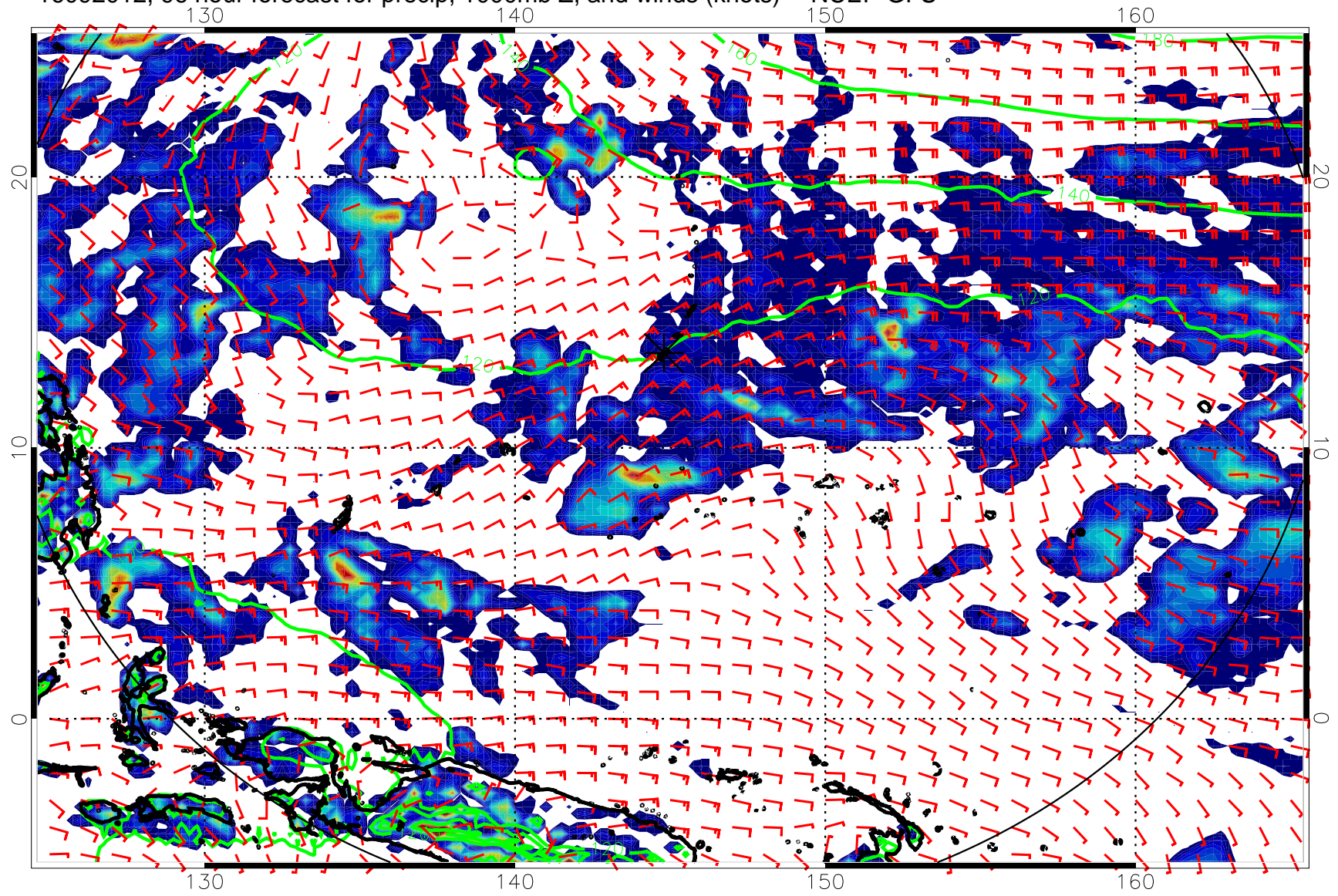
16092012, 96 hour forecast for precip, 1000mb Z, and winds (knots) -- NCEP GFS
