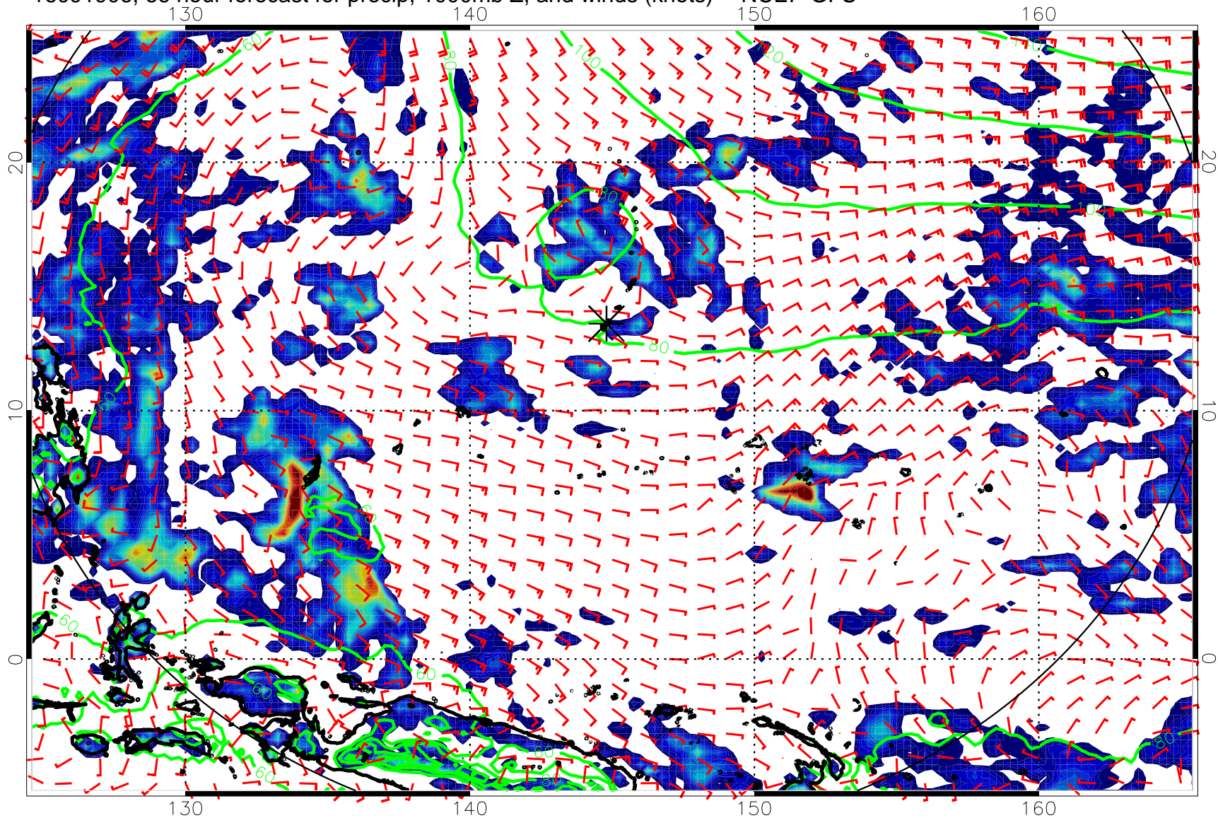
16091906, 66 hour forecast for precip, 1000mb Z, and winds (knots) -- NCEP GFS
