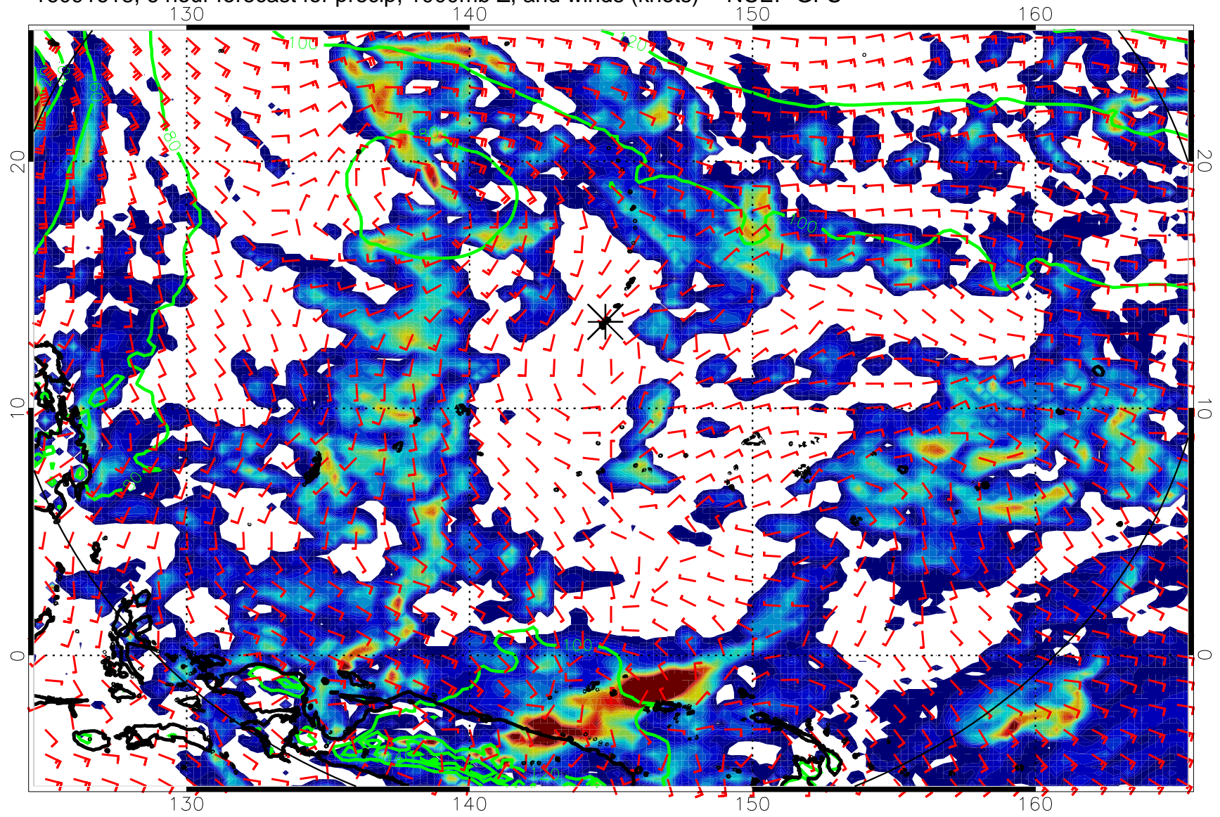
16091618, 6 hour forecast for precip, 1000mb Z, and winds (knots) -- NCEP GFS
