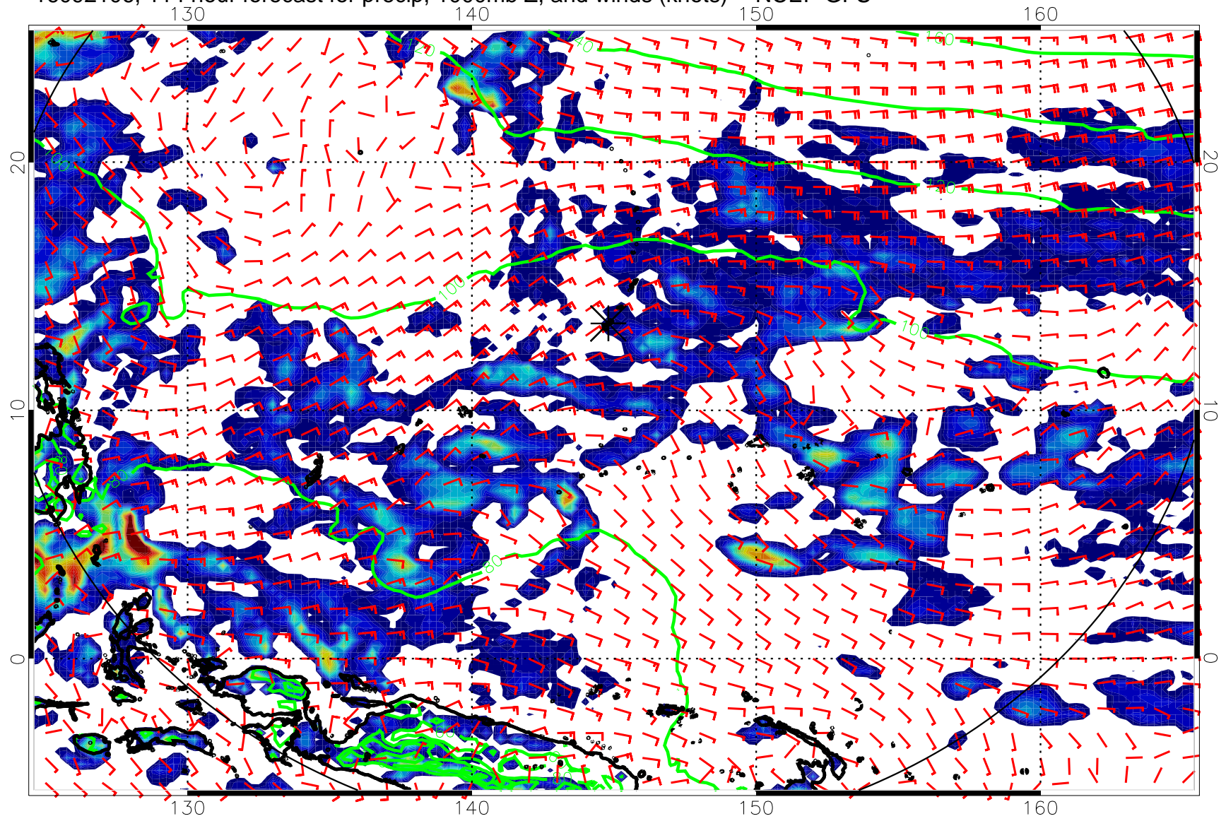
16092106, 114 hour forecast for precip, 1000mb Z, and winds (knots) -- NCEP GFS
