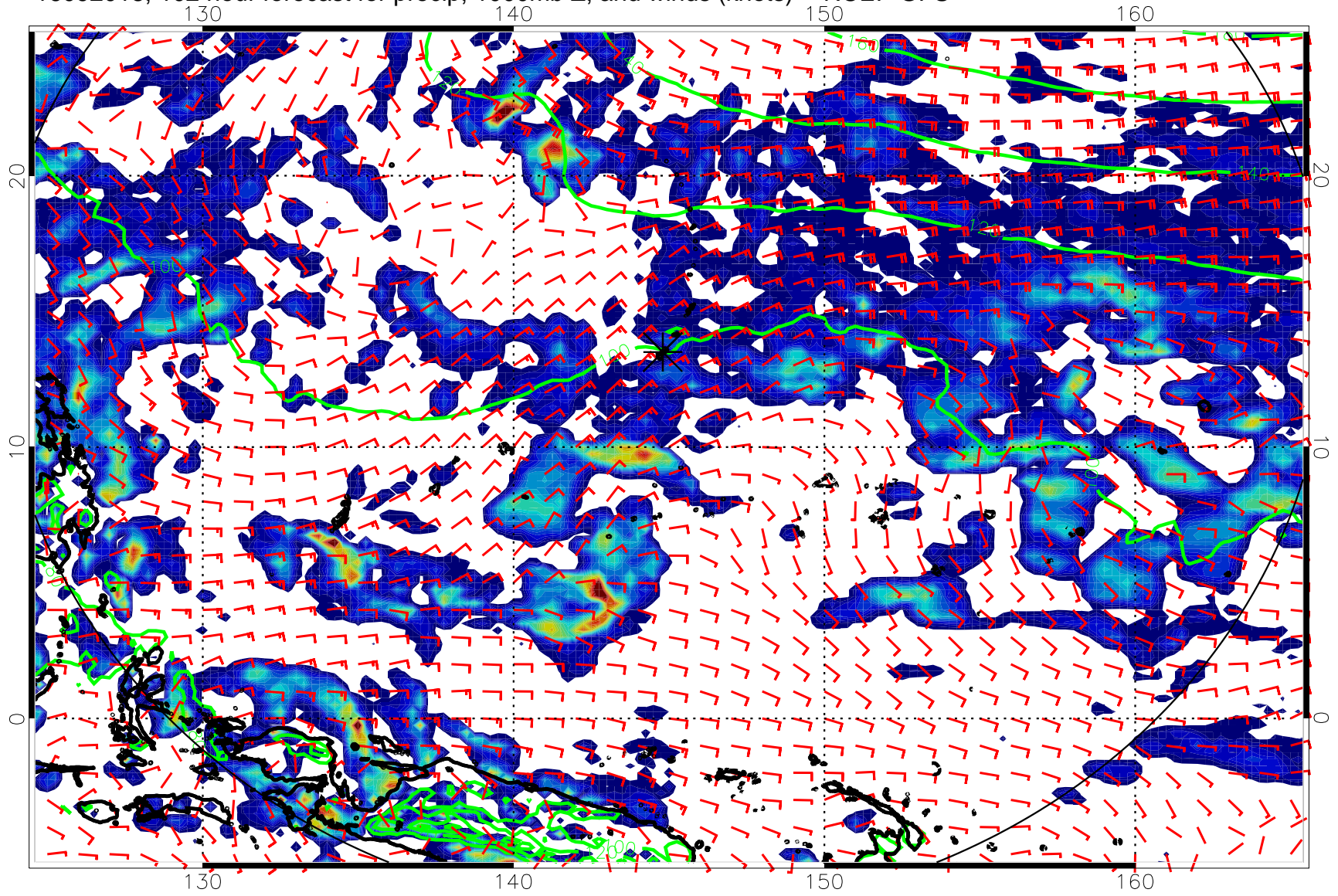
16092018, 102 hour forecast for precip, 1000mb Z, and winds (knots) -- NCEP GFS
