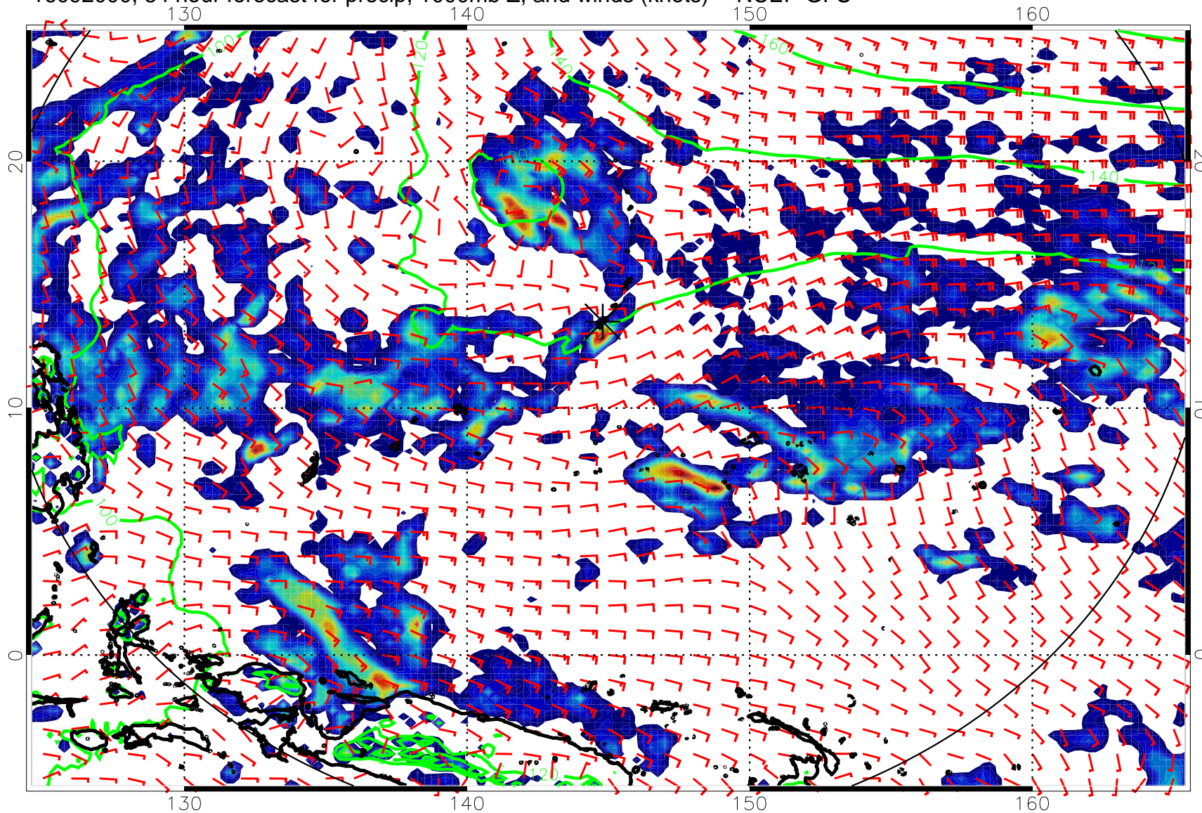
16092000, 84 hour forecast for precip, 1000mb Z, and winds (knots) -- NCEP GFS
