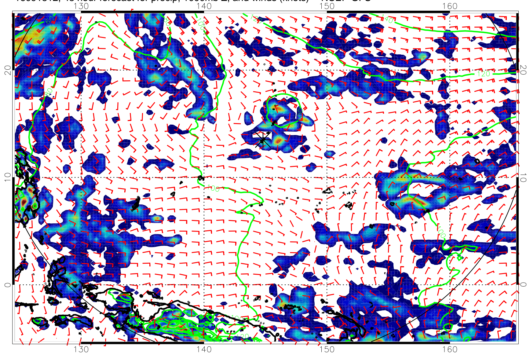
16091812, 48 hour forecast for precip, 1000mb Z, and winds (knots) -- NCEP GFS
