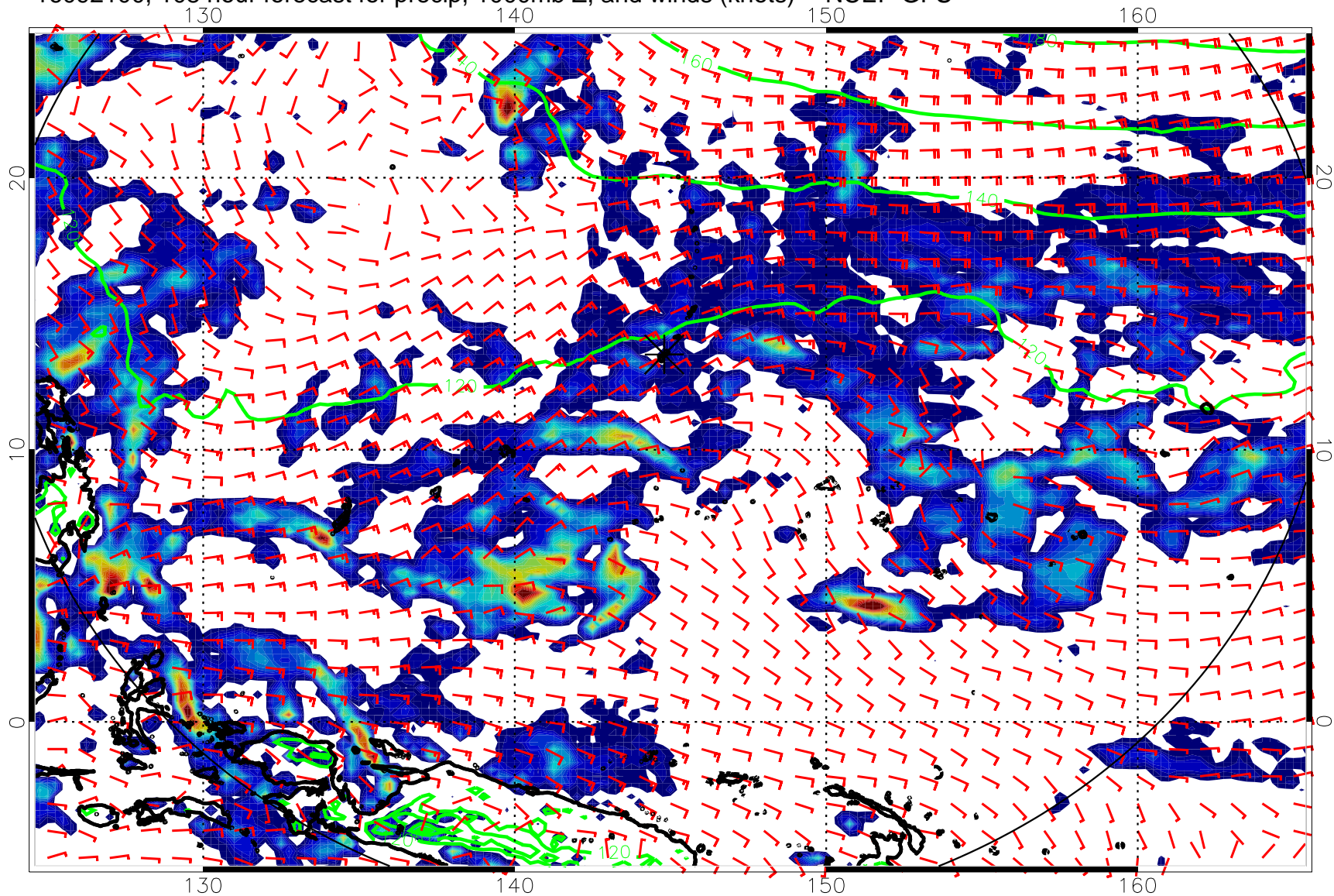
16092100, 108 hour forecast for precip, 1000mb Z, and winds (knots) -- NCEP GFS
