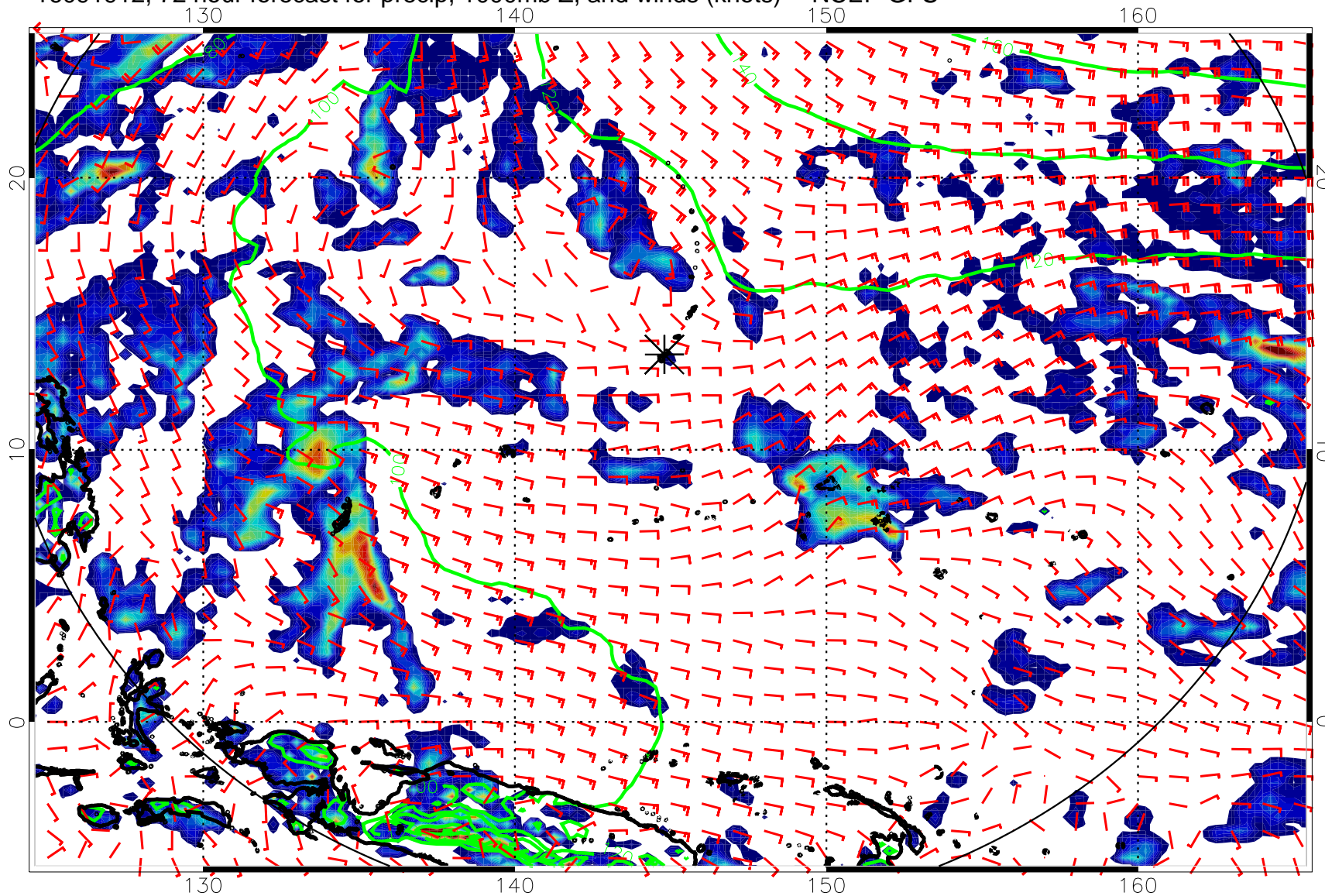
16091912, 72 hour forecast for precip, 1000mb Z, and winds (knots) -- NCEP GFS
