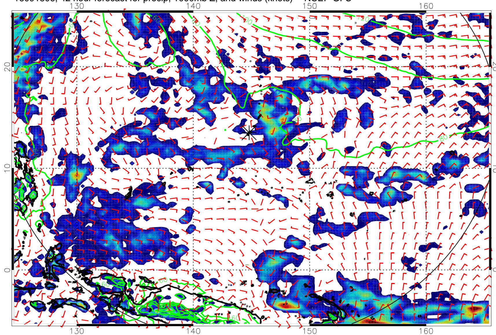
16091806, 42 hour forecast for precip, 1000mb Z, and winds (knots) -- NCEP GFS
