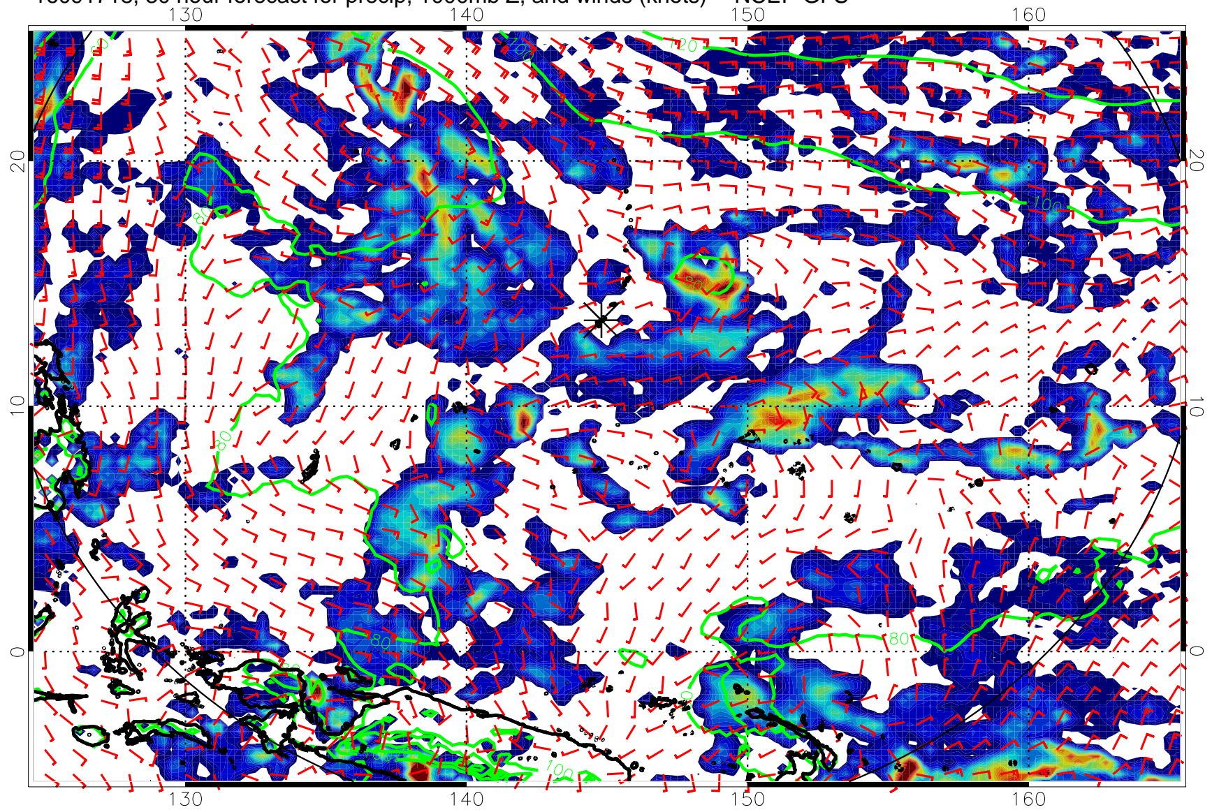
16091718, 30 hour forecast for precip, 1000mb Z, and winds (knots) -- NCEP GFS
