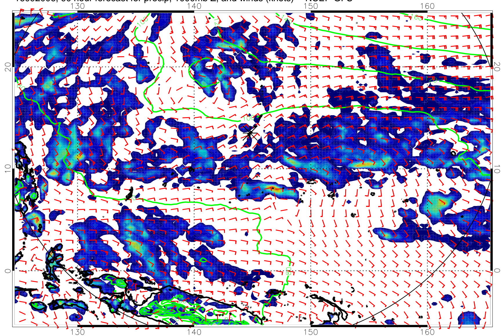
16092006, 90 hour forecast for precip, 1000mb Z, and winds (knots) -- NCEP GFS
