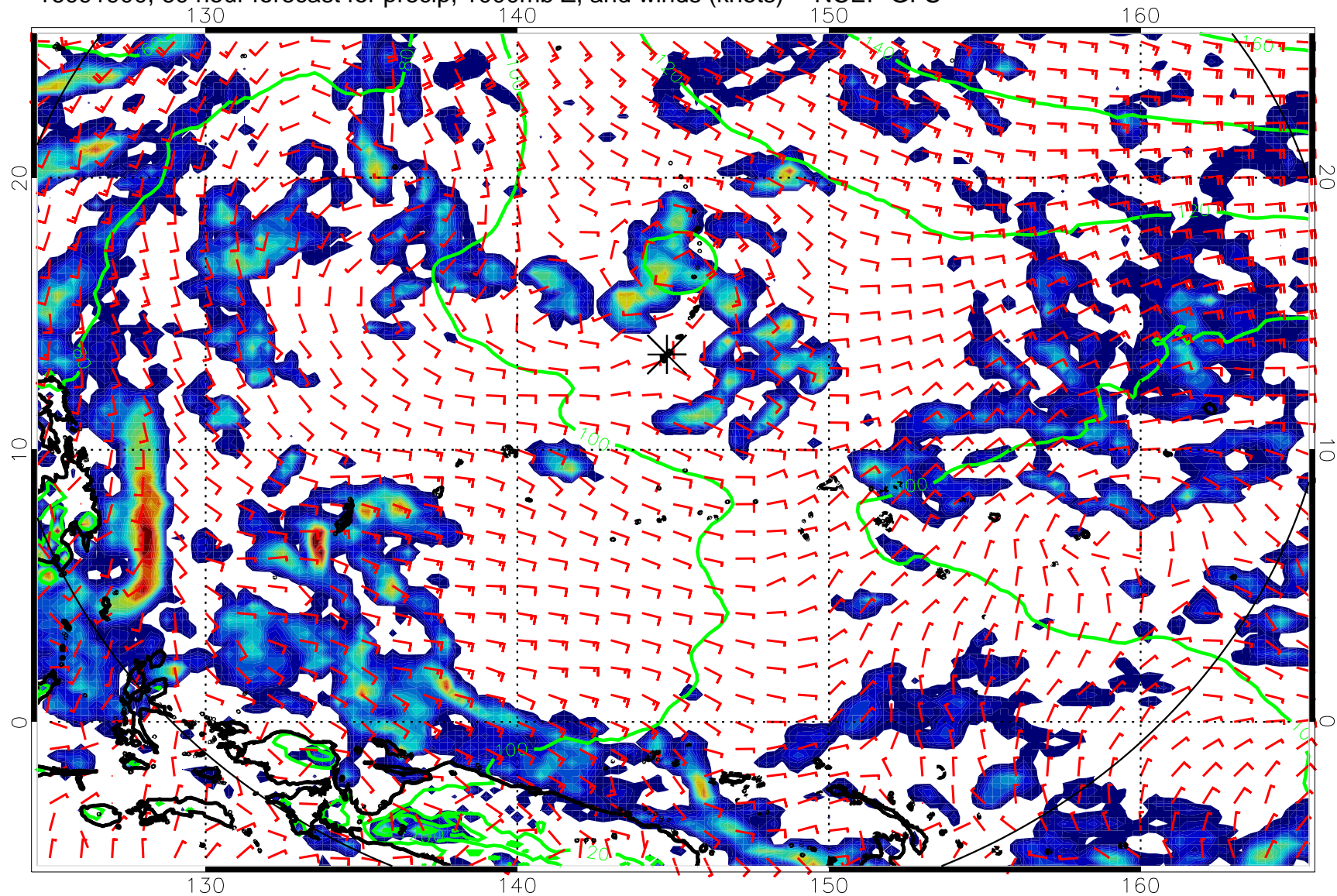
16091900, 60 hour forecast for precip, 1000mb Z, and winds (knots) -- NCEP GFS
