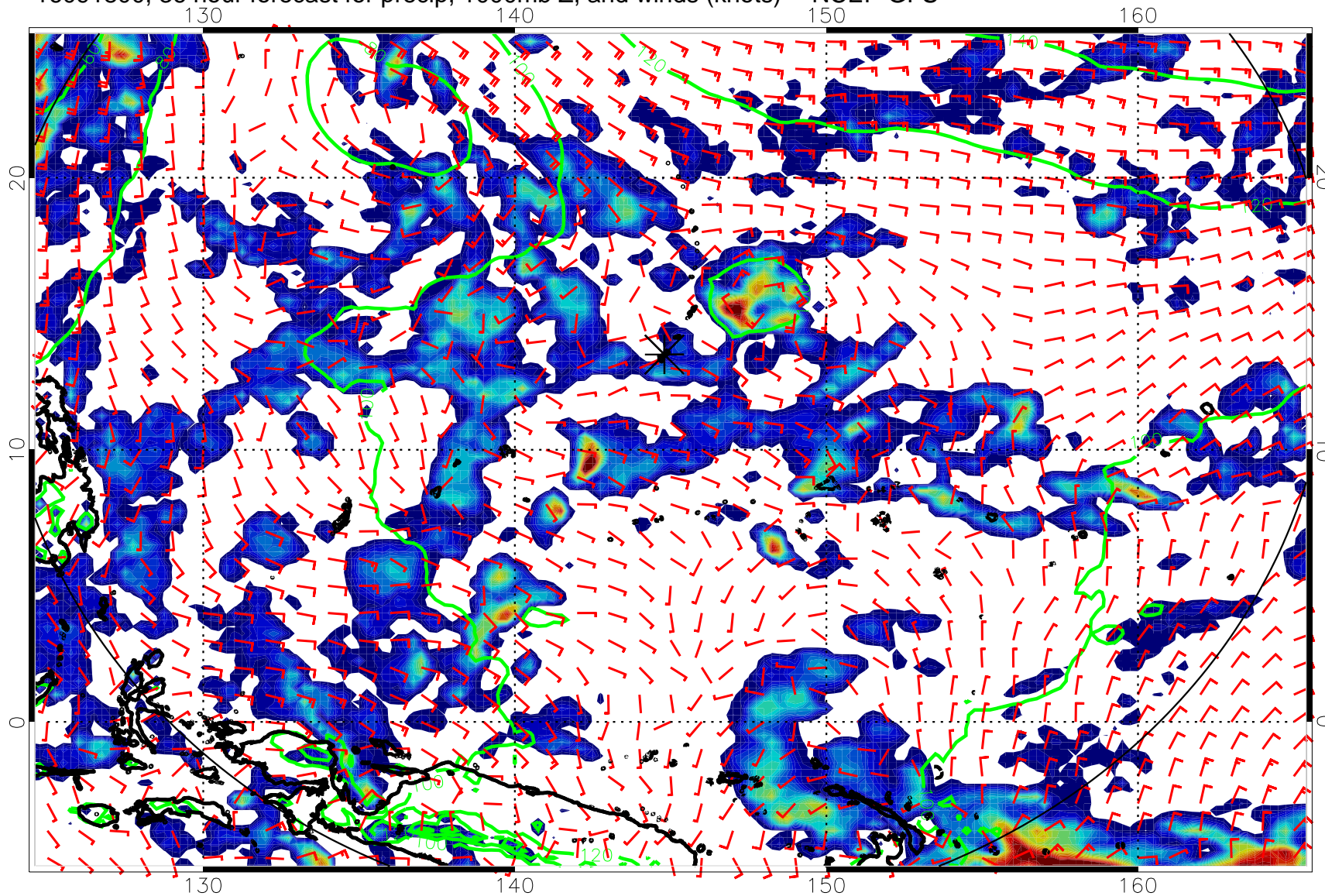
16091800, 36 hour forecast for precip, 1000mb Z, and winds (knots) -- NCEP GFS
