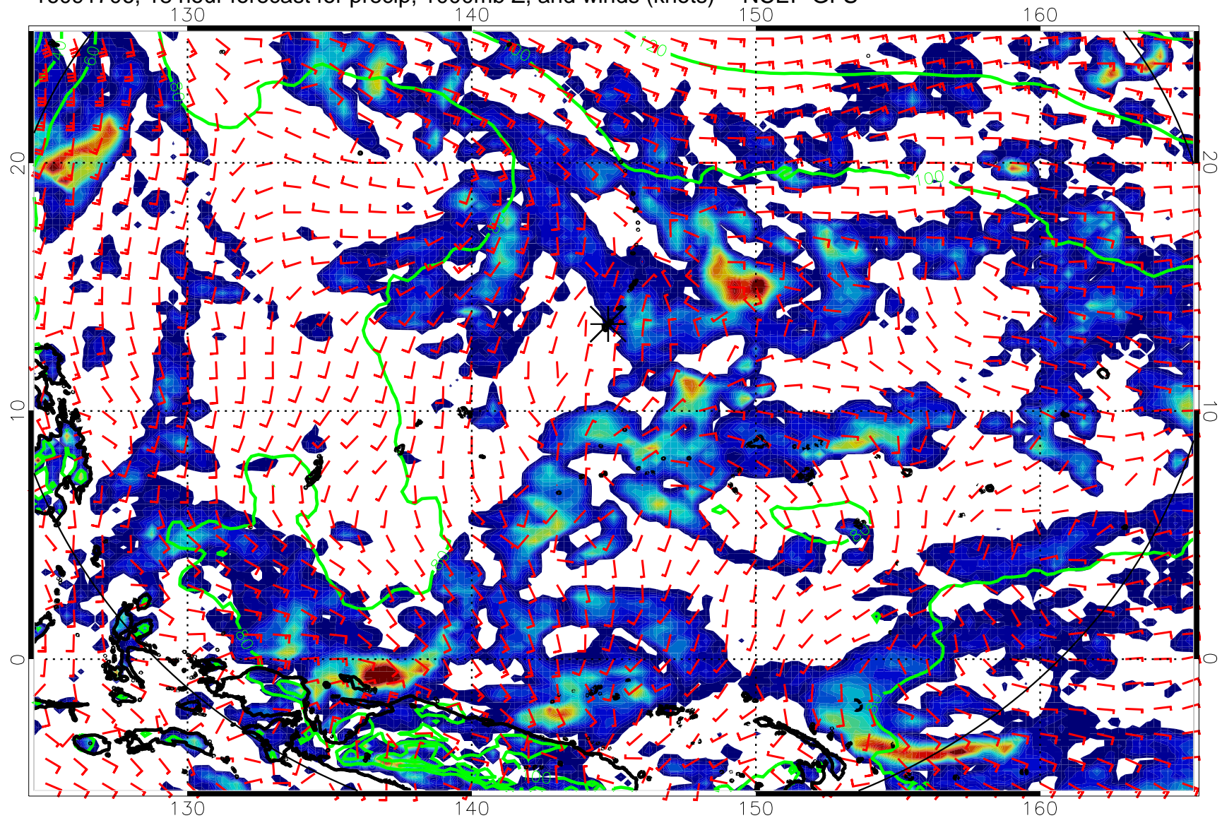
16091706, 18 hour forecast for precip, 1000mb Z, and winds (knots) -- NCEP GFS
