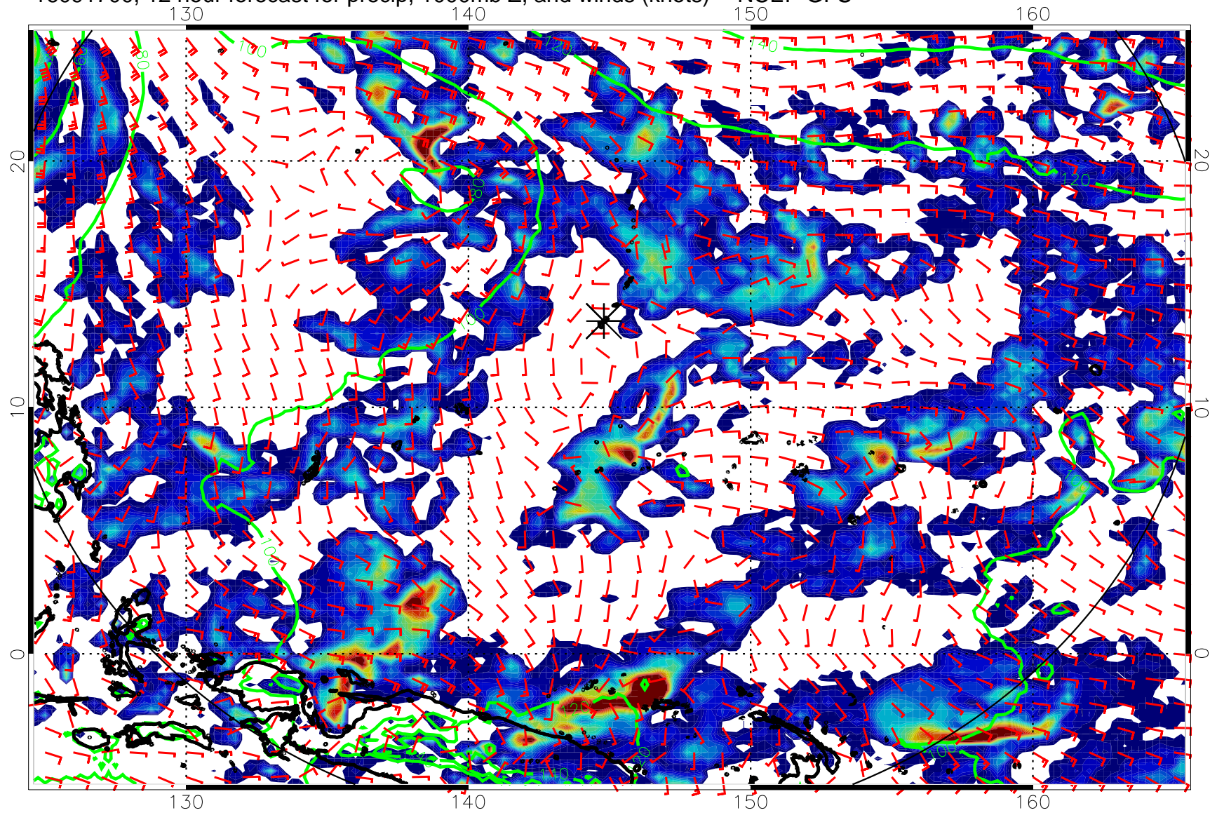
16091700, 12 hour forecast for precip, 1000mb Z, and winds (knots) -- NCEP GFS
