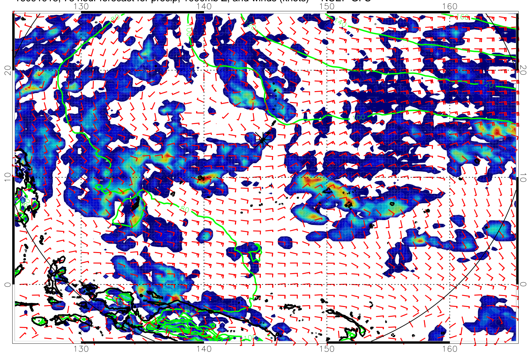
16091918, 78 hour forecast for precip, 1000mb Z, and winds (knots) -- NCEP GFS
