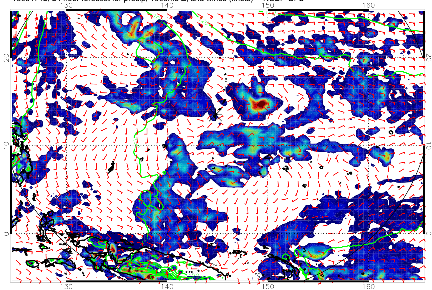
16091712, 24 hour forecast for precip, 1000mb Z, and winds (knots) -- NCEP GFS
