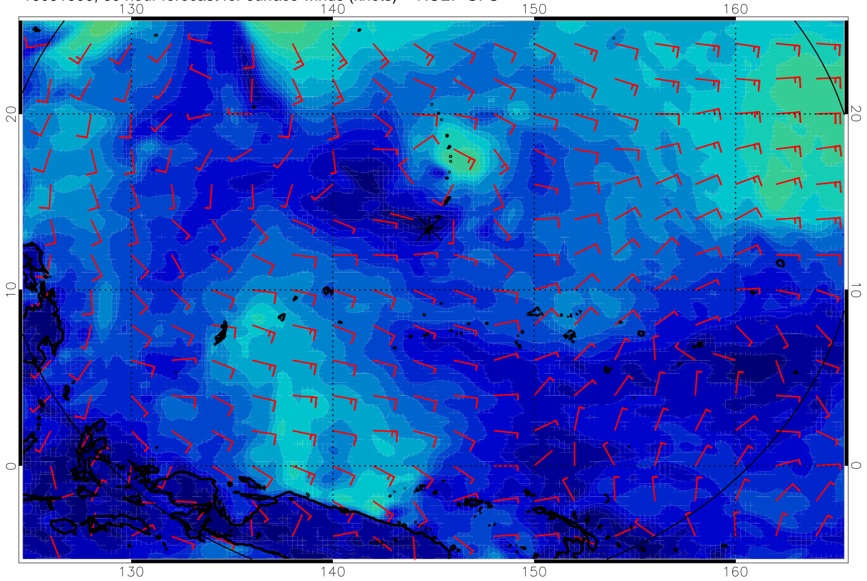
16091900, 60 hour forecast for surface winds (knots) -- NCEP GFS
