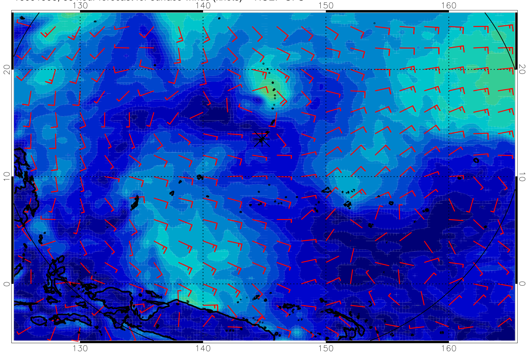
16091906, 66 hour forecast for surface winds (knots) -- NCEP GFS
