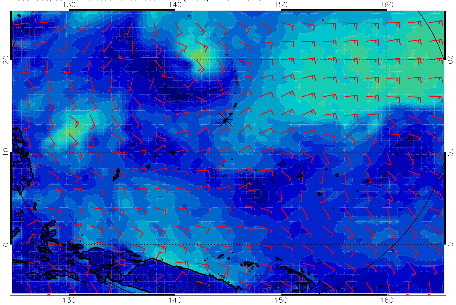
16092006, 90 hour forecast for surface winds (knots) -- NCEP GFS
