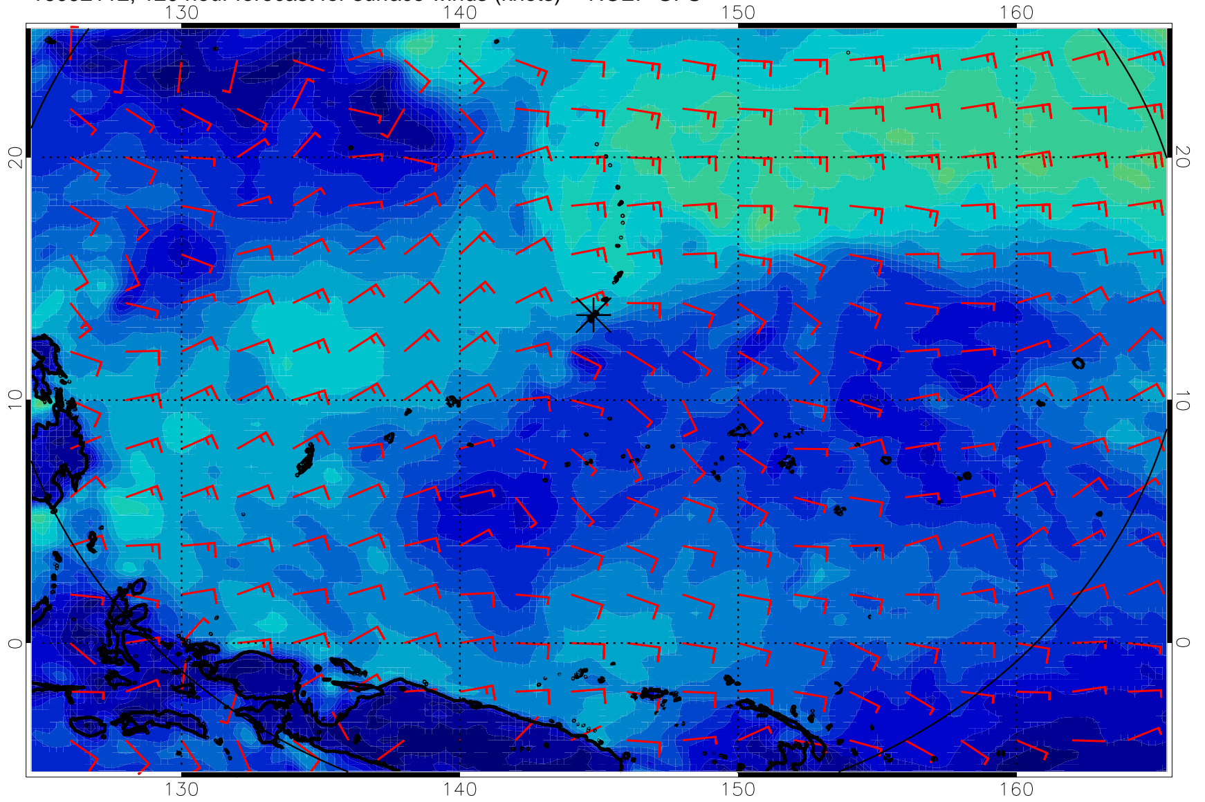
16092112, 120 hour forecast for surface winds (knots) -- NCEP GFS
