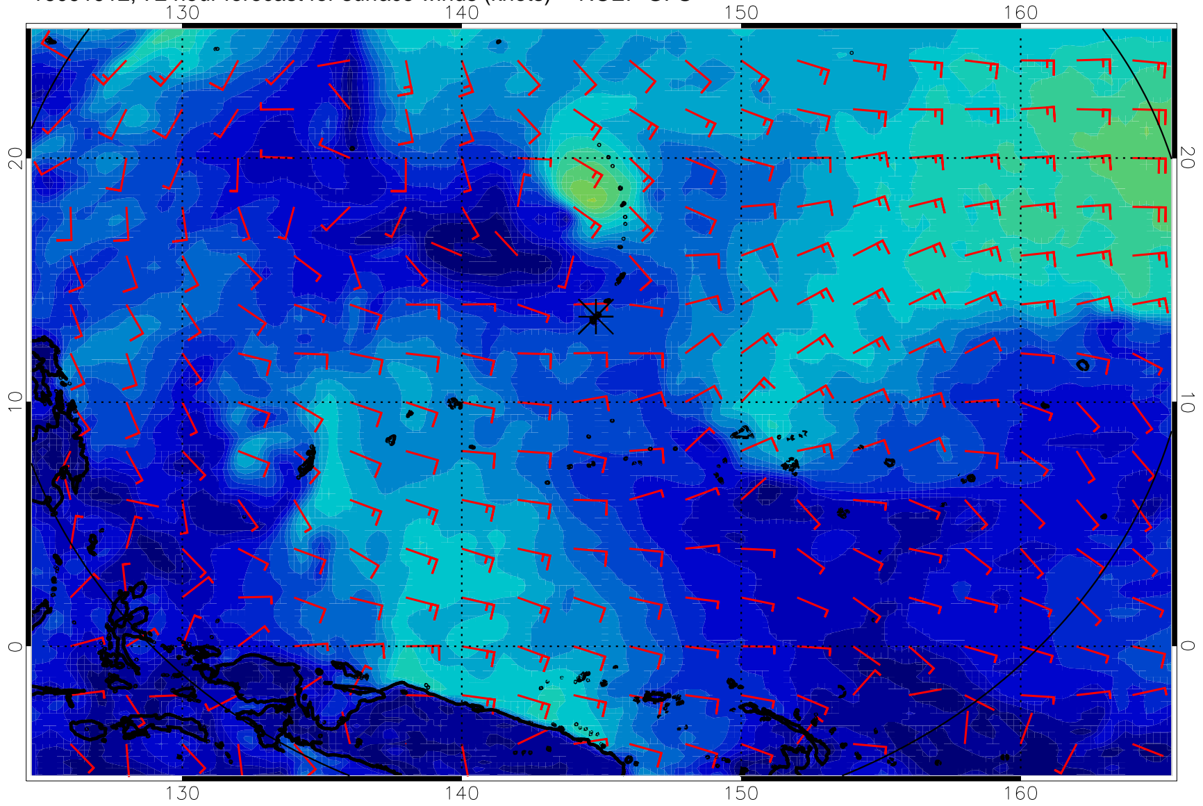
16091912, 72 hour forecast for surface winds (knots) -- NCEP GFS
