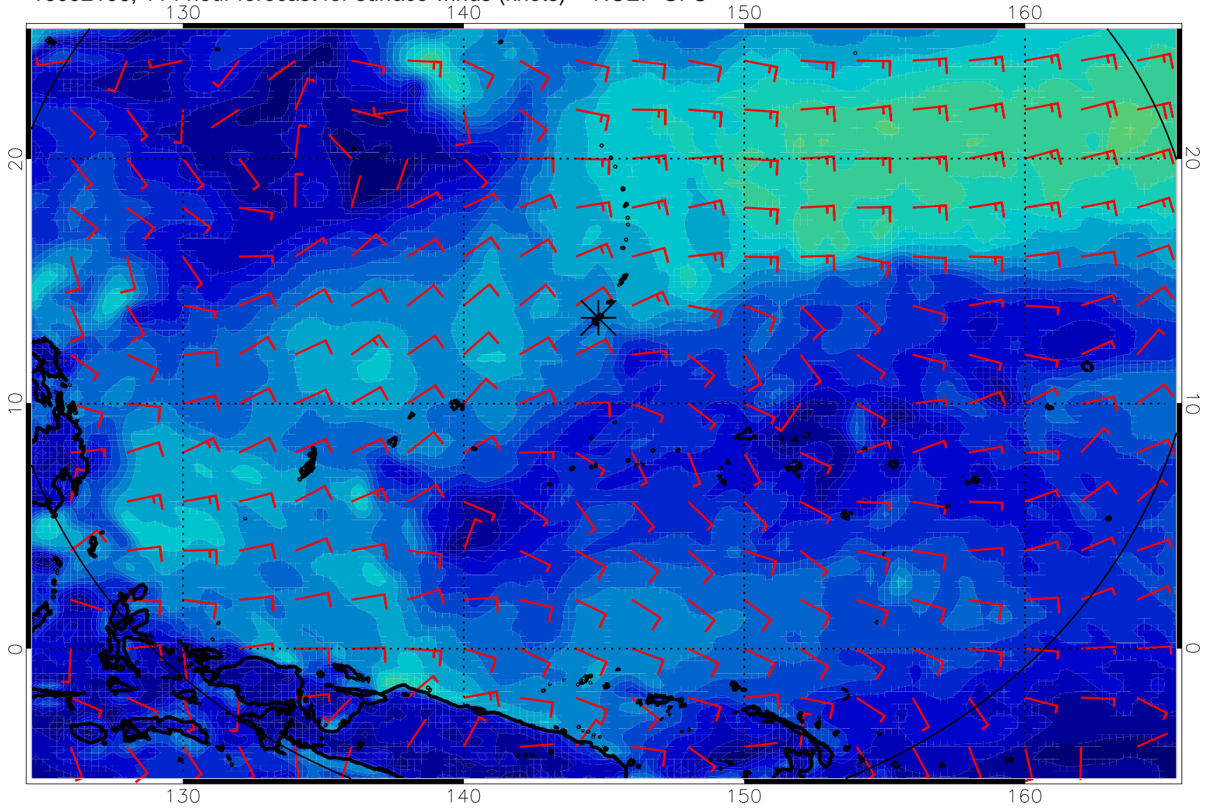
16092106, 114 hour forecast for surface winds (knots) -- NCEP GFS
