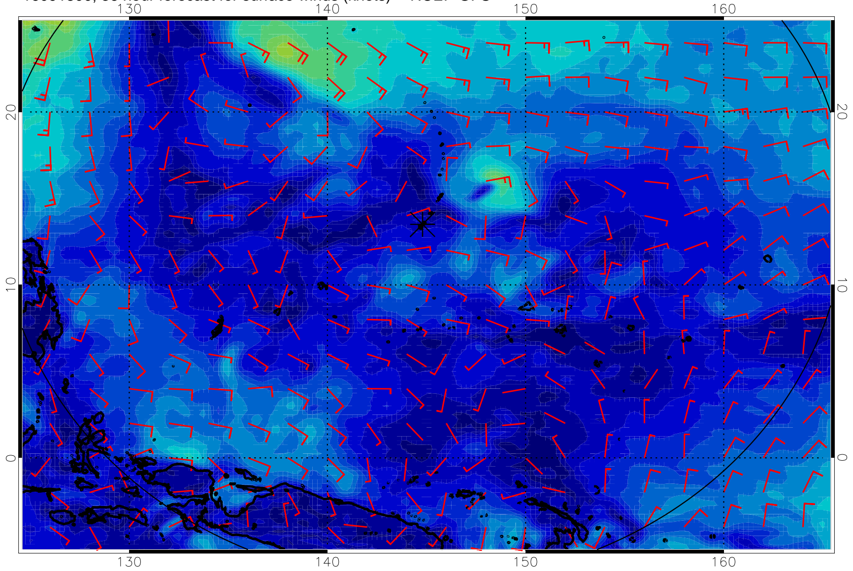
16091800, 36 hour forecast for surface winds (knots) -- NCEP GFS
