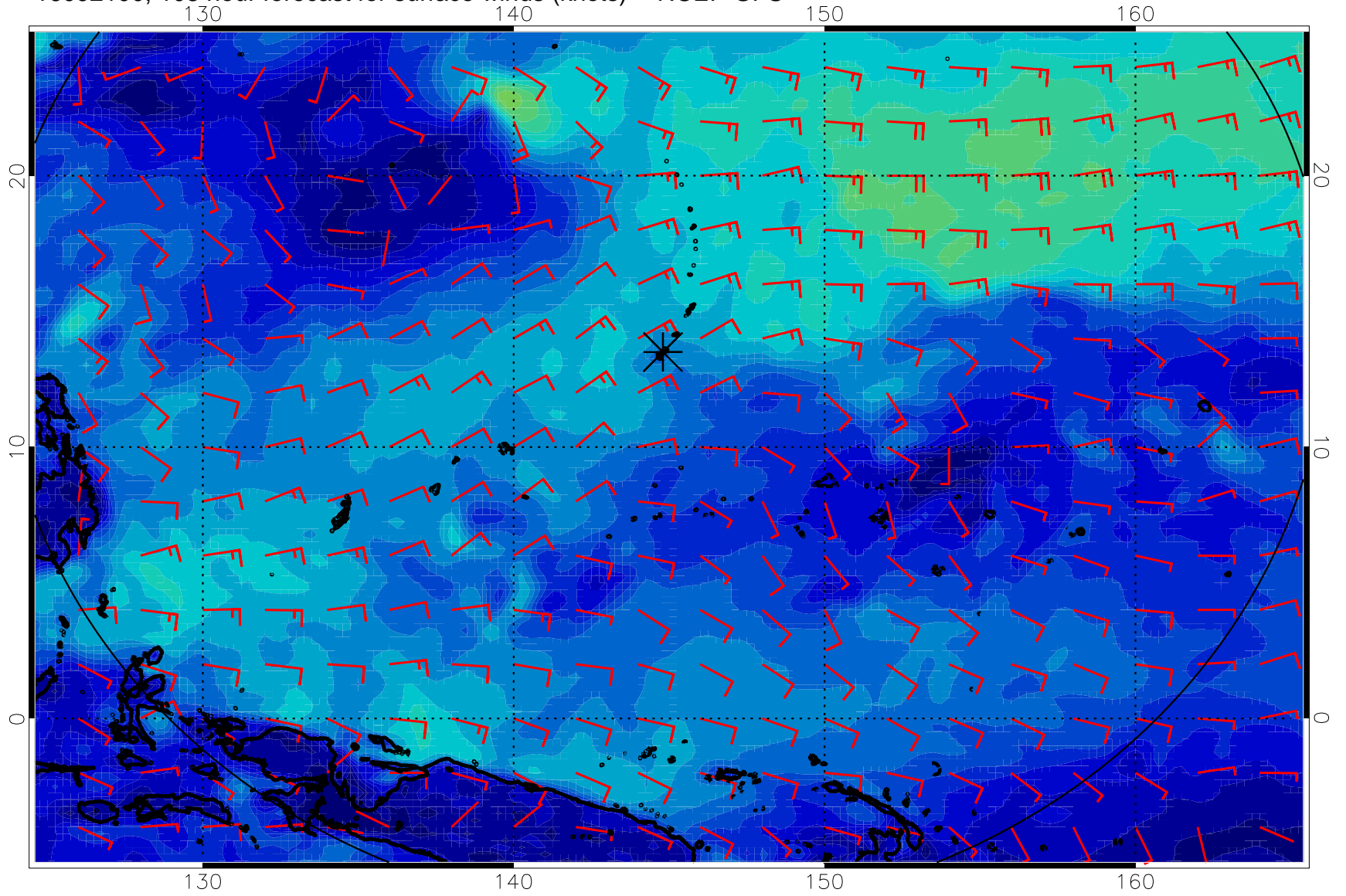
16092100, 108 hour forecast for surface winds (knots) -- NCEP GFS
