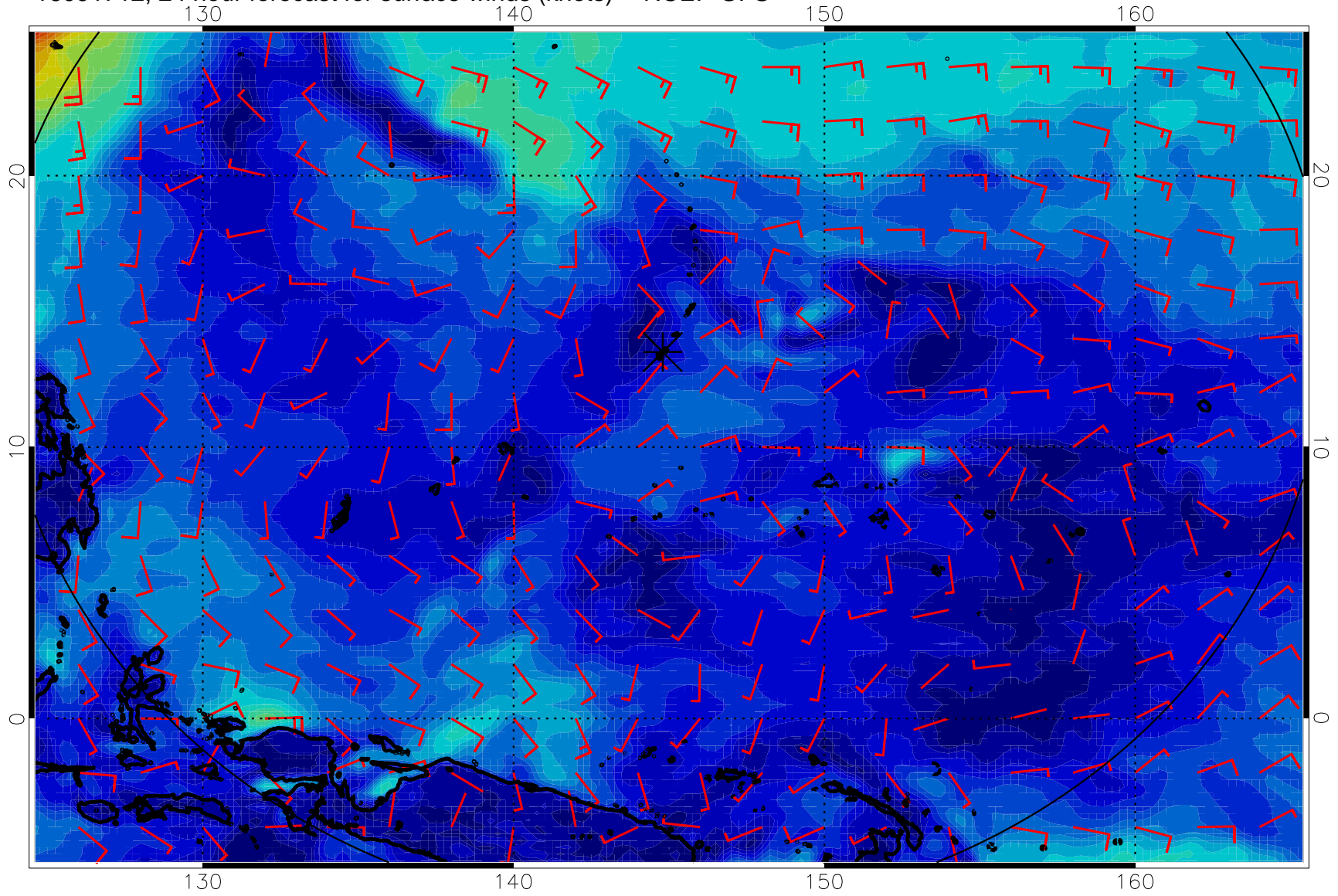
16091712, 24 hour forecast for surface winds (knots) -- NCEP GFS
