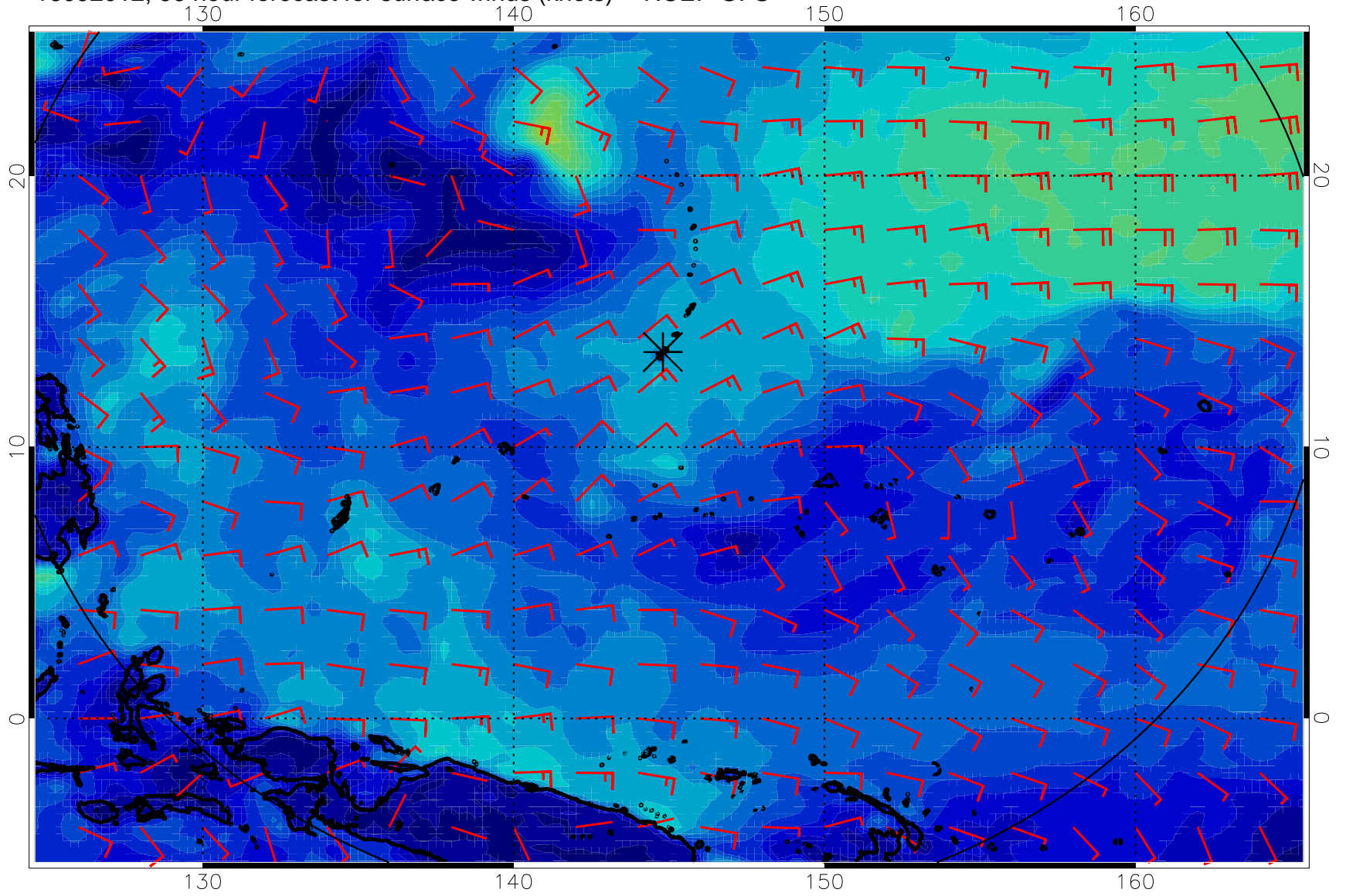
16092012, 96 hour forecast for surface winds (knots) -- NCEP GFS
