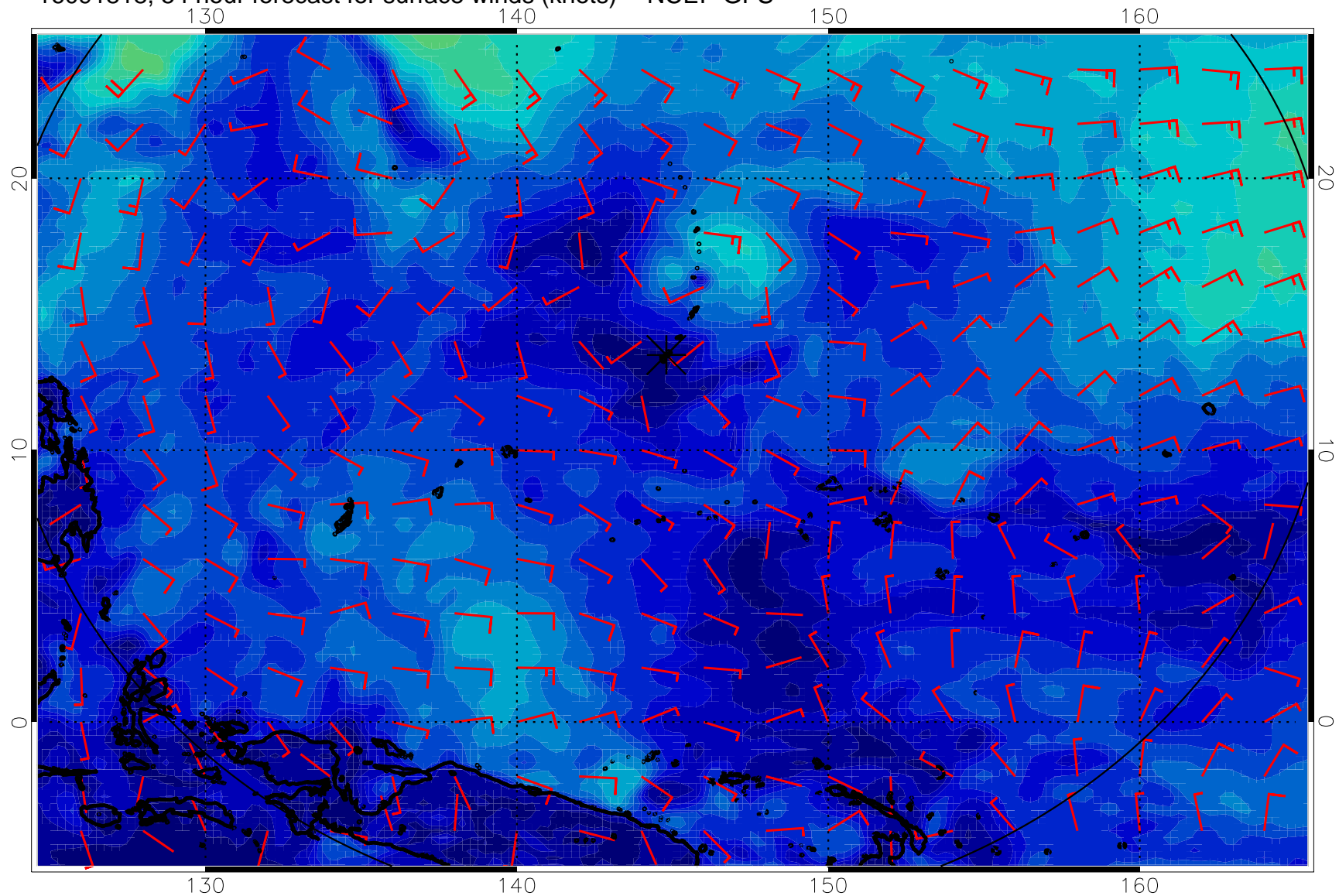
16091818, 54 hour forecast for surface winds (knots) -- NCEP GFS
