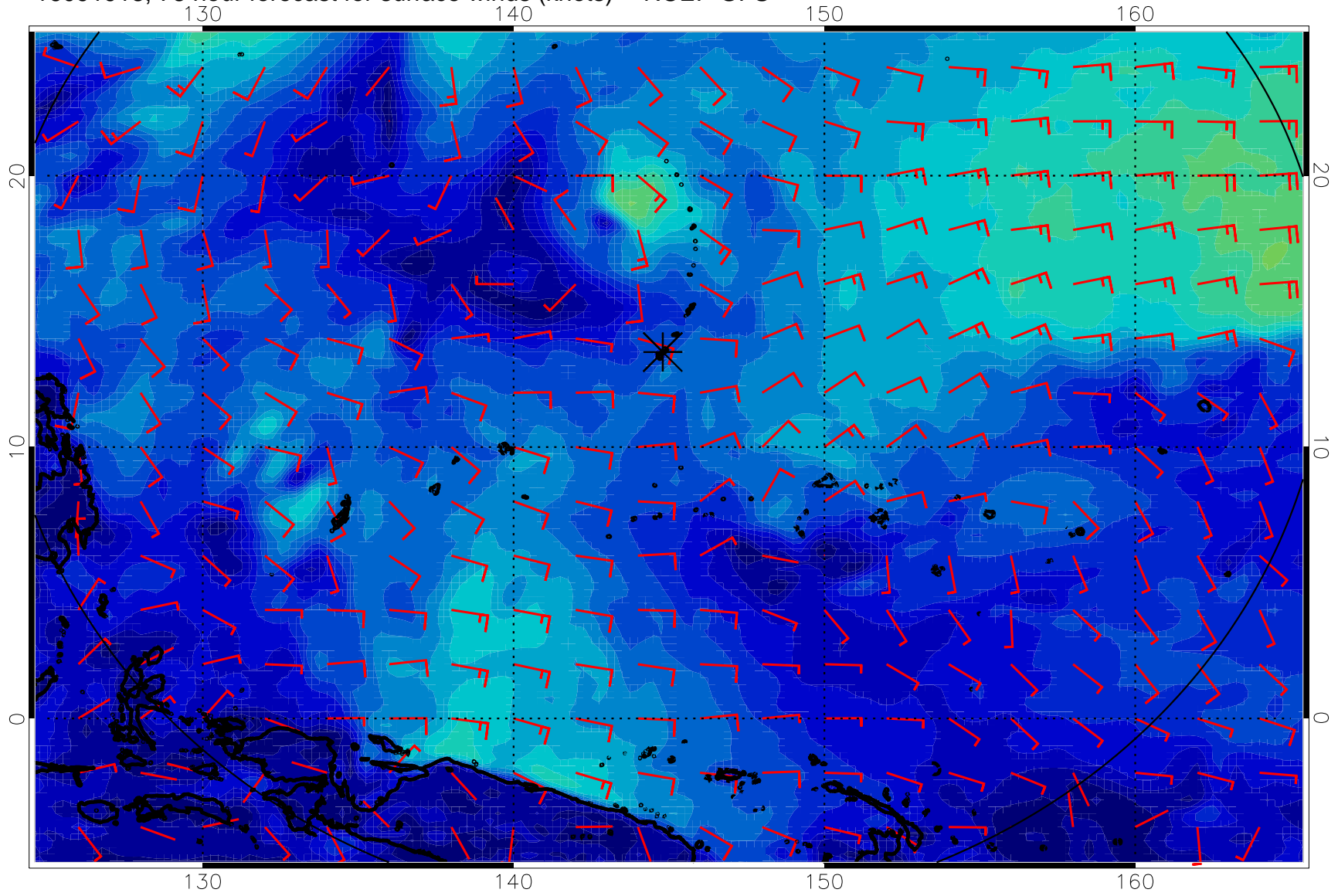
16091918, 78 hour forecast for surface winds (knots) -- NCEP GFS
