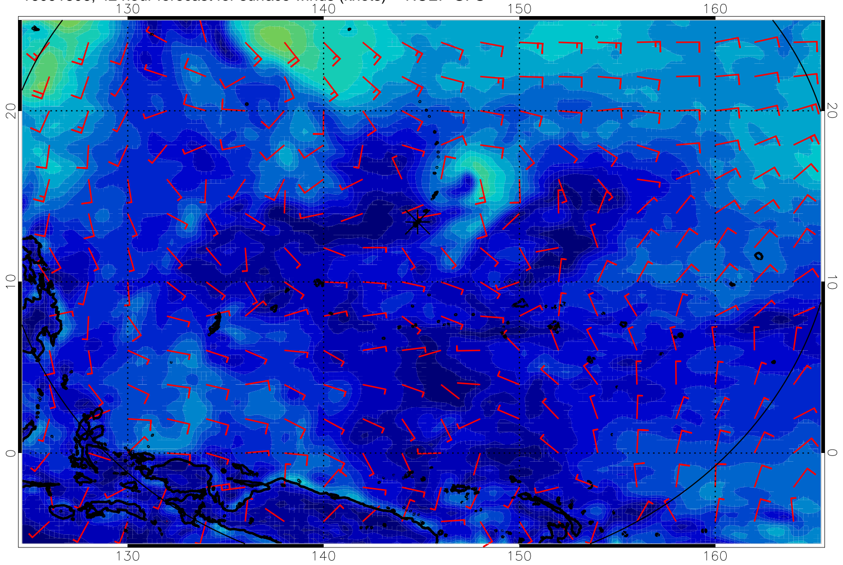
16091806, 42 hour forecast for surface winds (knots) -- NCEP GFS
