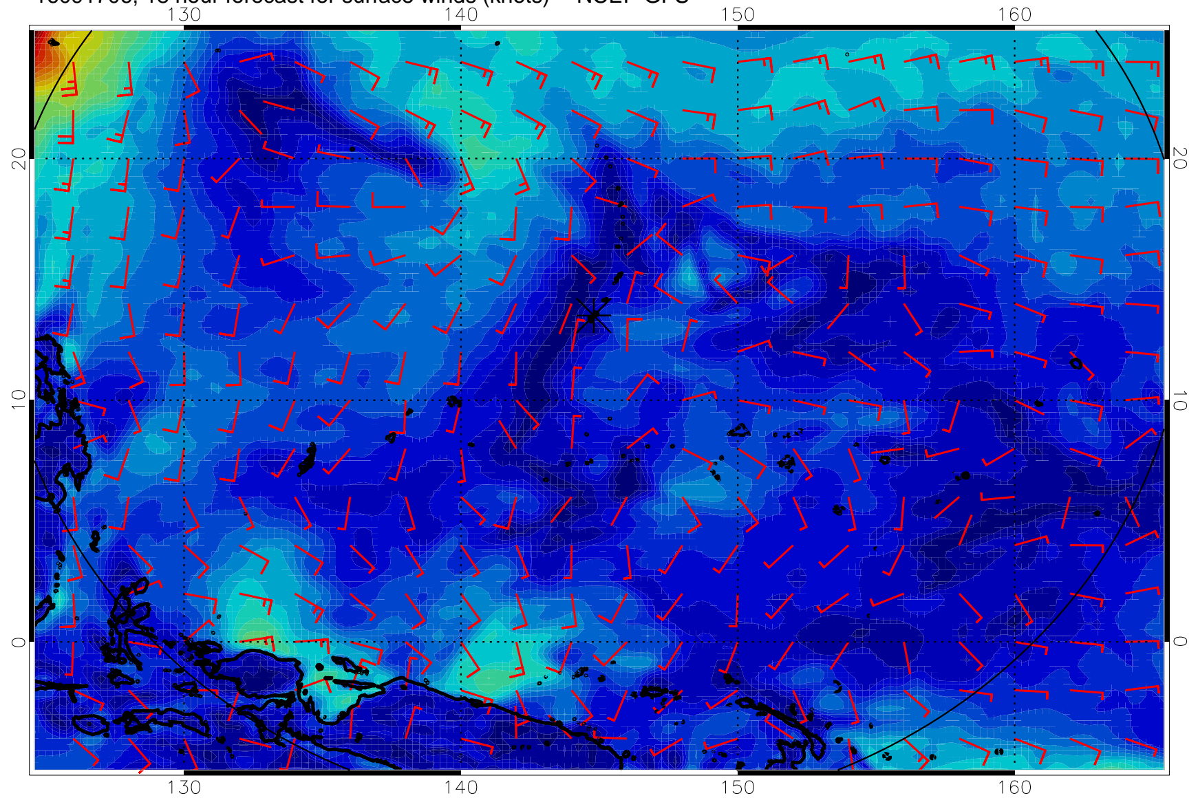
16091706, 18 hour forecast for surface winds (knots) -- NCEP GFS
