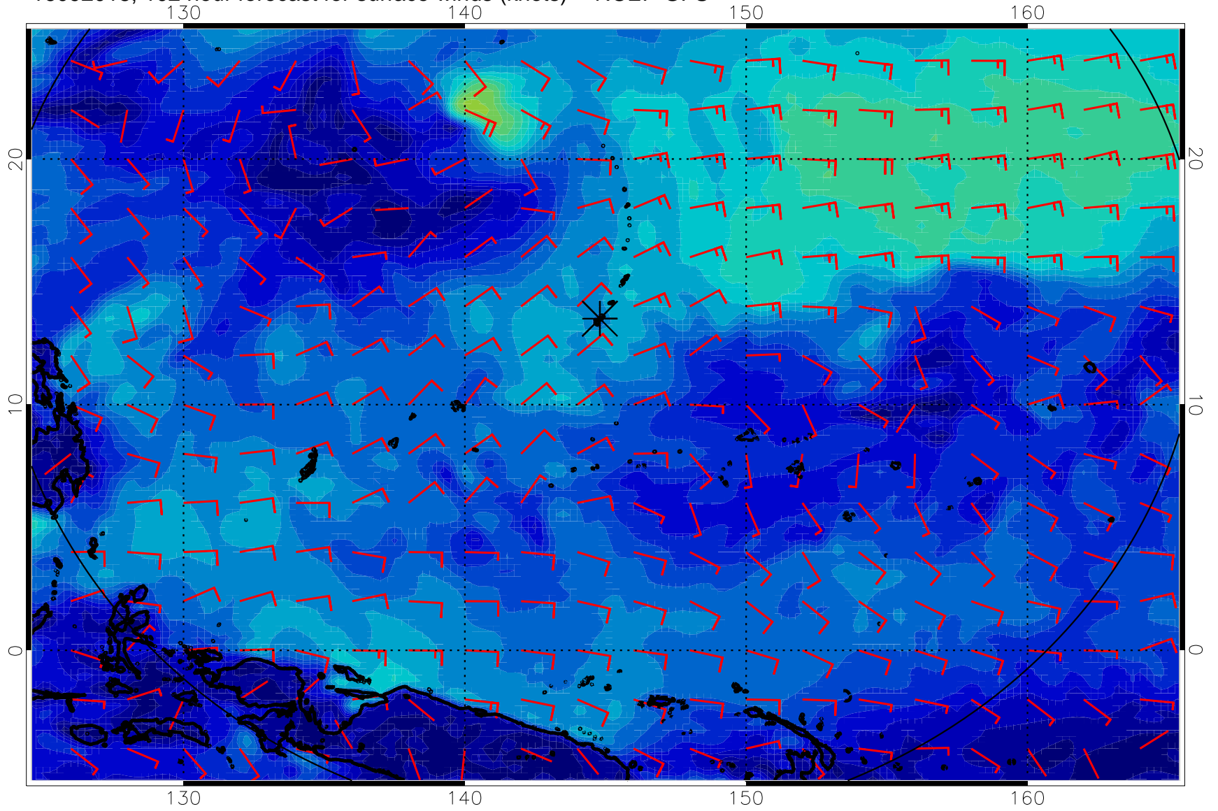
16092018, 102 hour forecast for surface winds (knots) -- NCEP GFS
