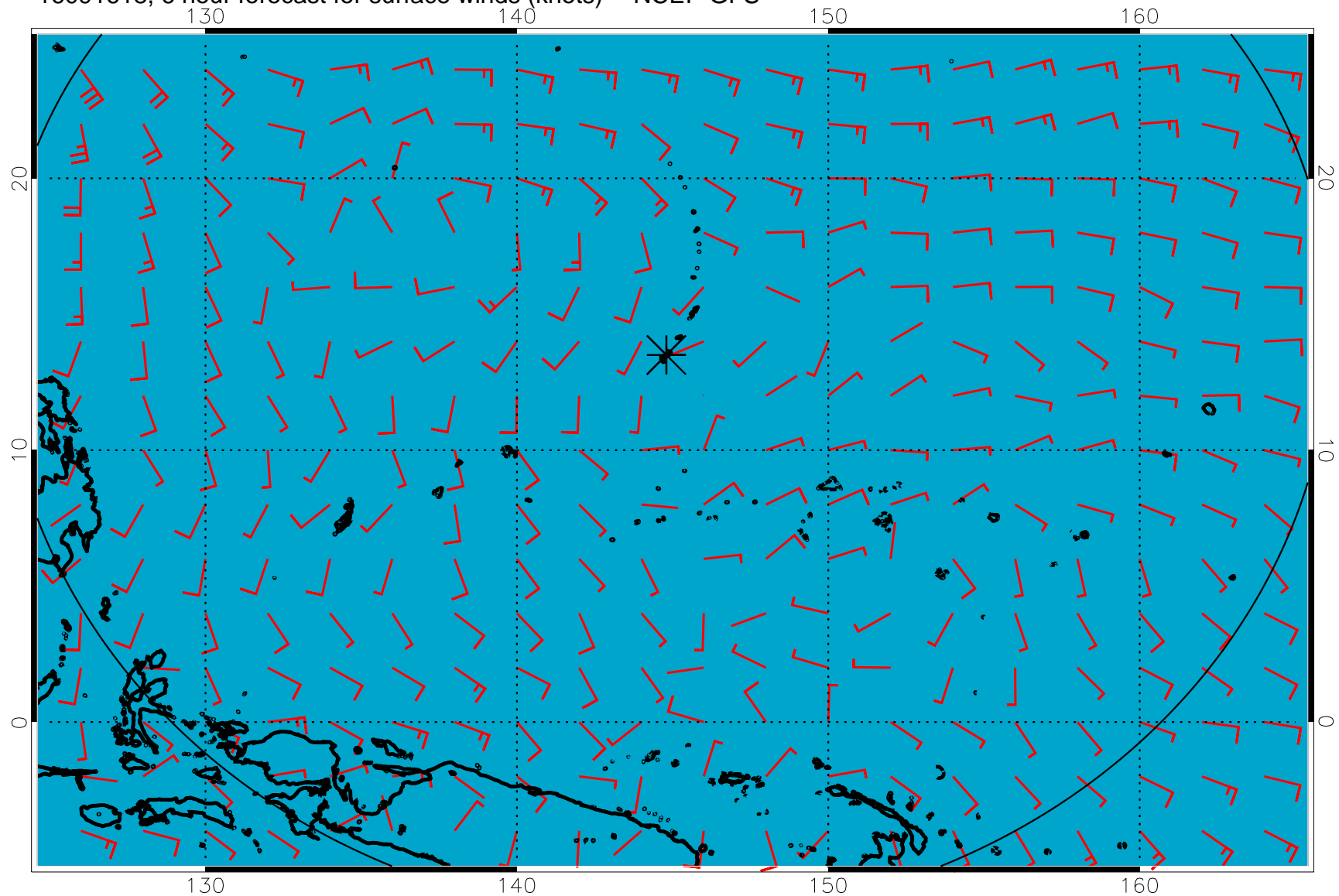
16091618, 6 hour forecast for surface winds (knots) -- NCEP GFS
