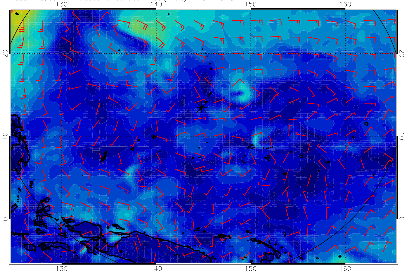
16091718, 30 hour forecast for surface winds (knots) -- NCEP GFS
