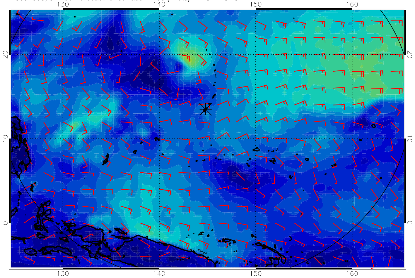
16092000, 84 hour forecast for surface winds (knots) -- NCEP GFS
