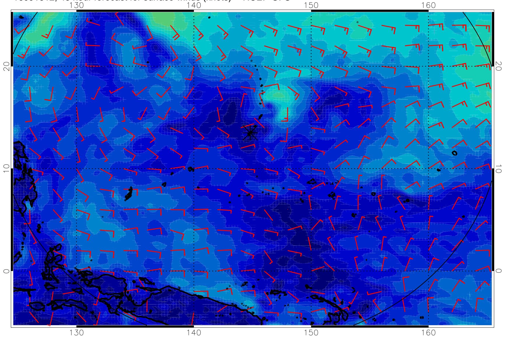
16091812, 48 hour forecast for surface winds (knots) -- NCEP GFS
