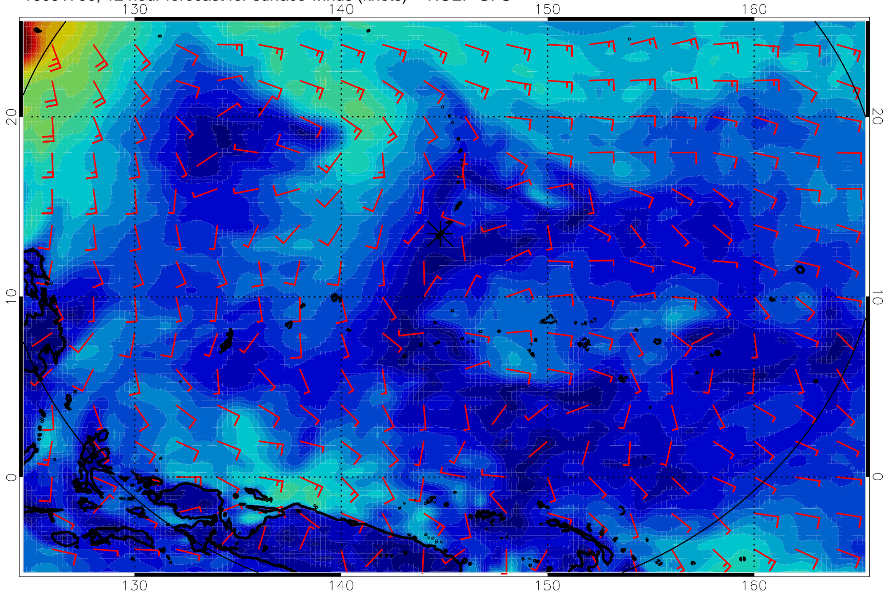
16091700, 12 hour forecast for surface winds (knots) -- NCEP GFS
