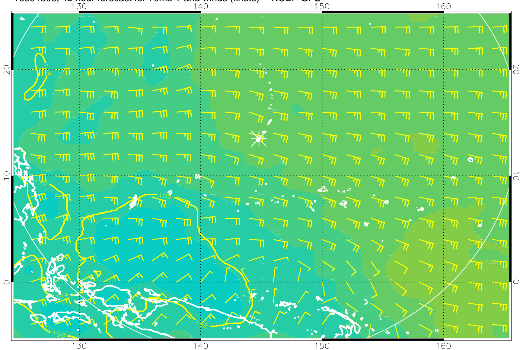
16091806, 42 hour forecast for 70mb T and winds (knots) -- NCEP GFS
