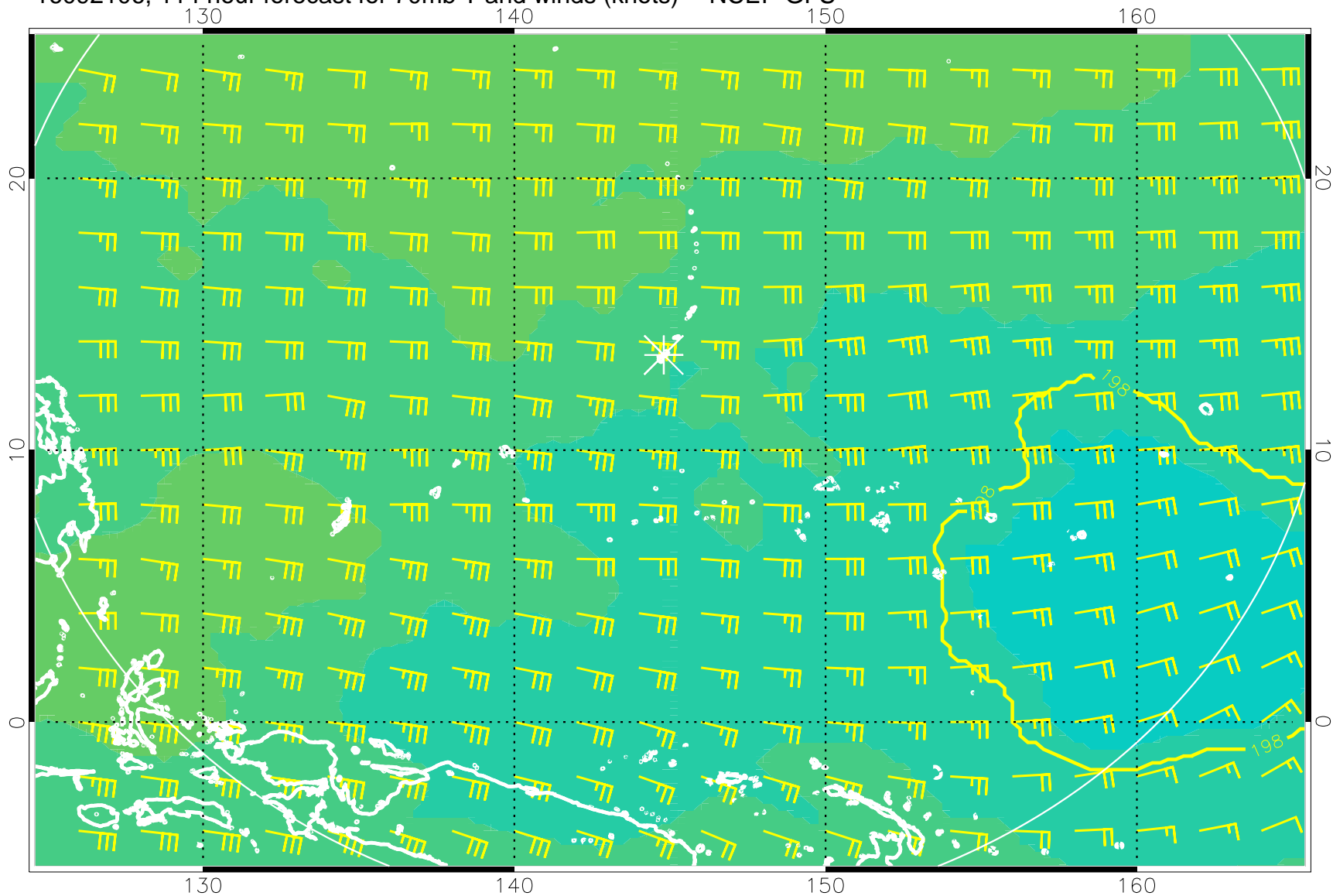
16092106, 114 hour forecast for 70mb T and winds (knots) -- NCEP GFS
