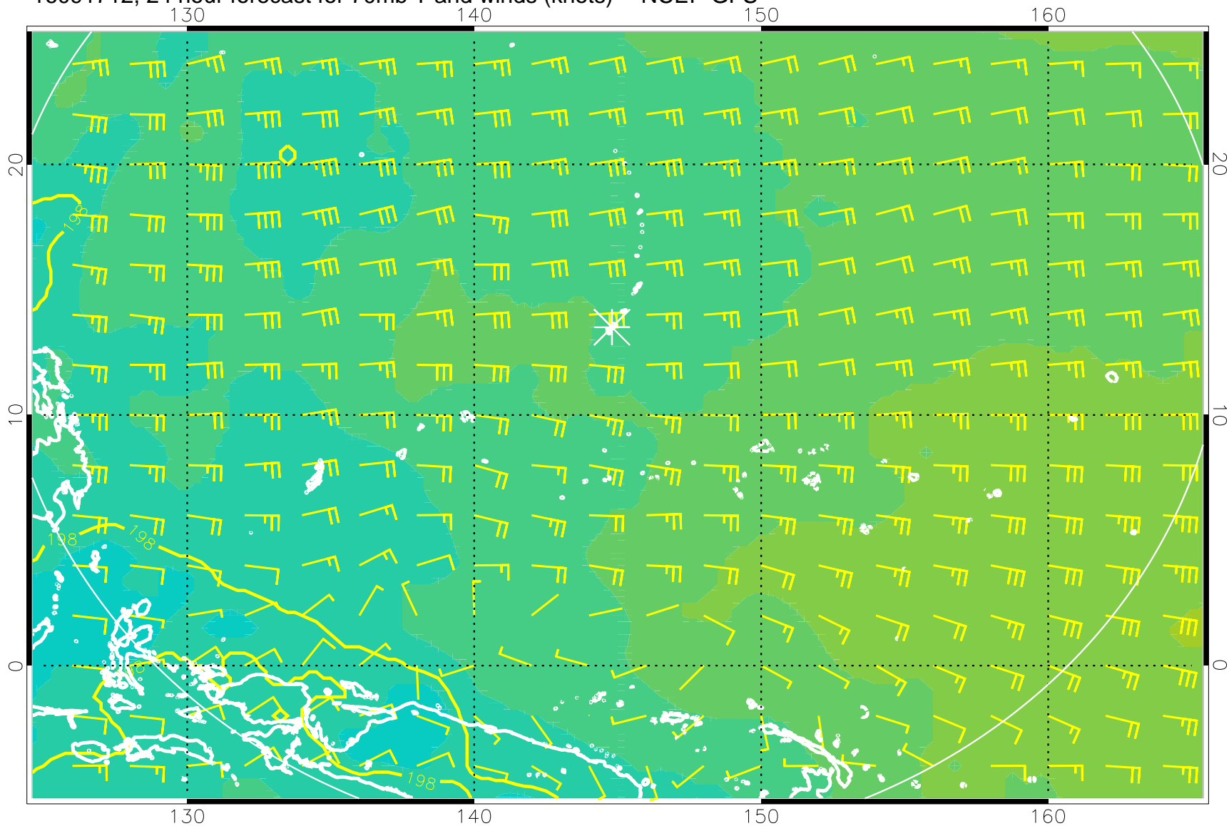
16091712, 24 hour forecast for 70mb T and winds (knots) -- NCEP GFS
