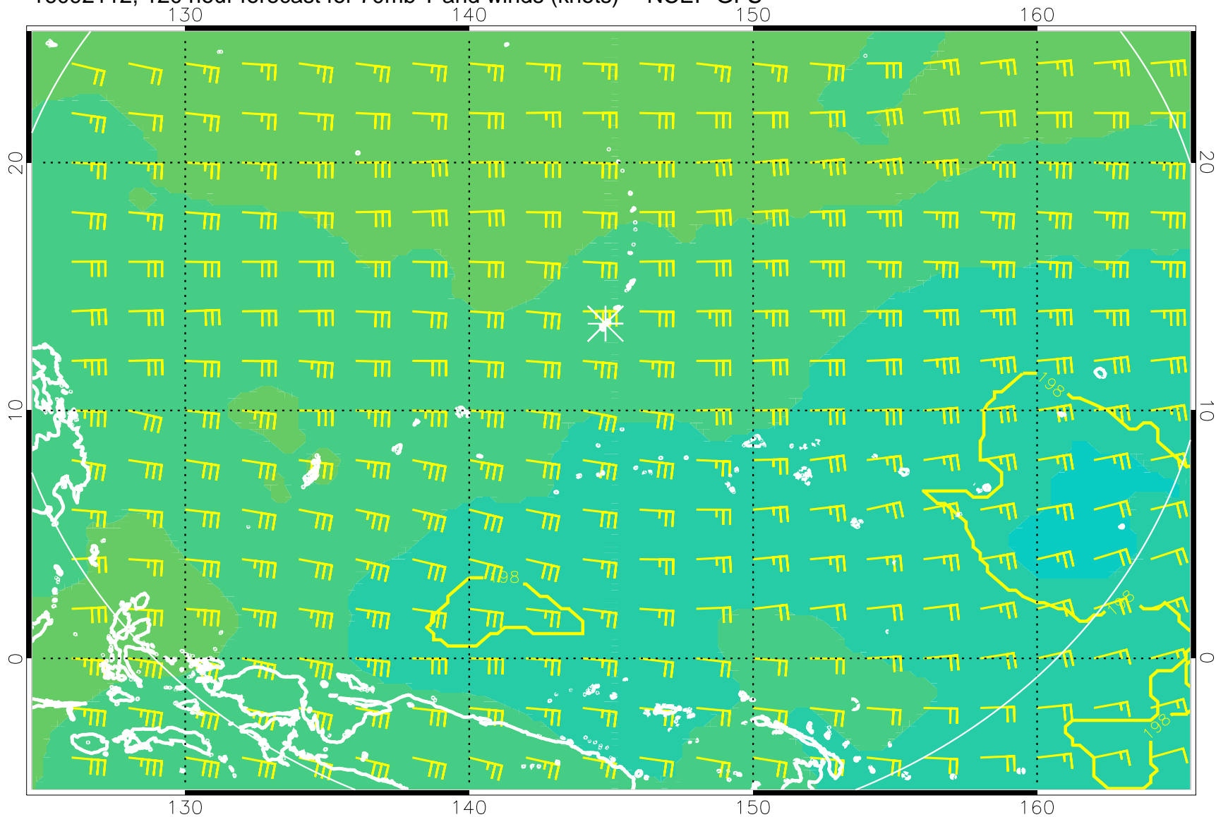
16092112, 120 hour forecast for 70mb T and winds (knots) -- NCEP GFS
