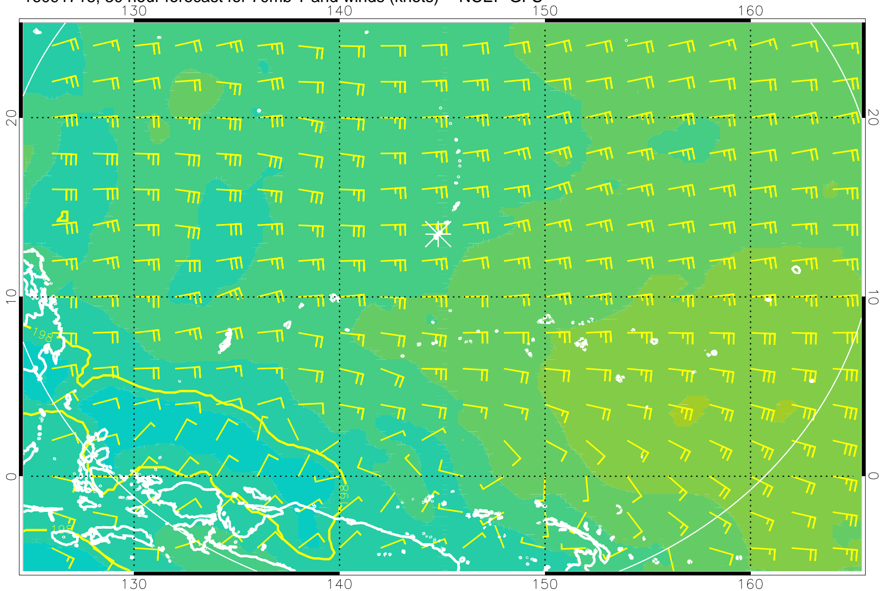
16091718, 30 hour forecast for 70mb T and winds (knots) -- NCEP GFS
