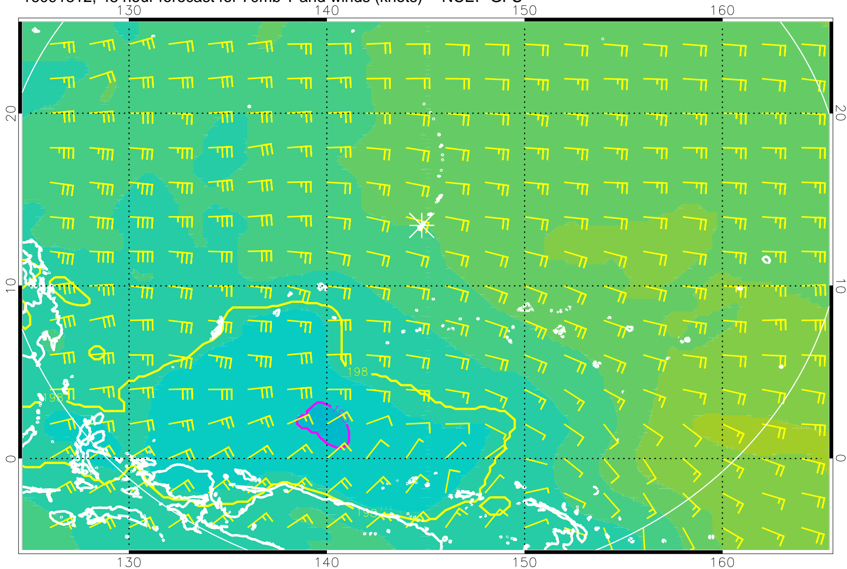
16091812, 48 hour forecast for 70mb T and winds (knots) -- NCEP GFS
