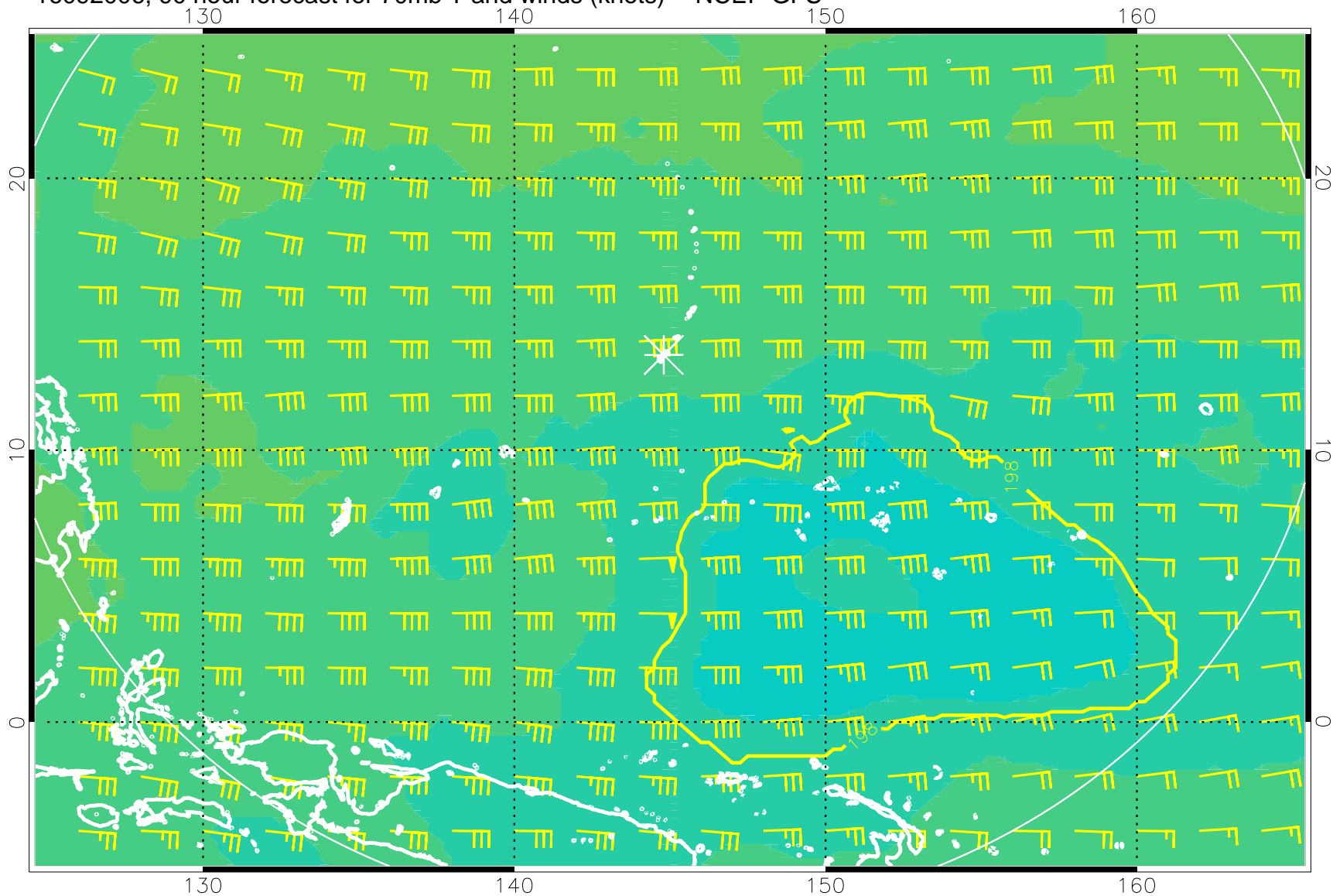
16092006, 90 hour forecast for 70mb T and winds (knots) -- NCEP GFS
