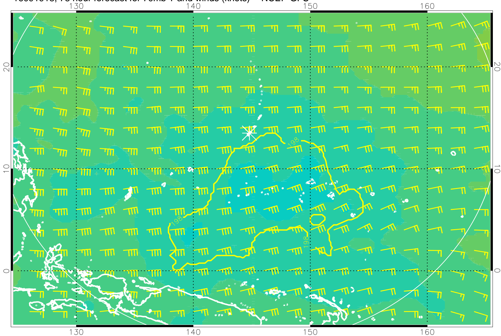
16091918, 78 hour forecast for 70mb T and winds (knots) -- NCEP GFS
