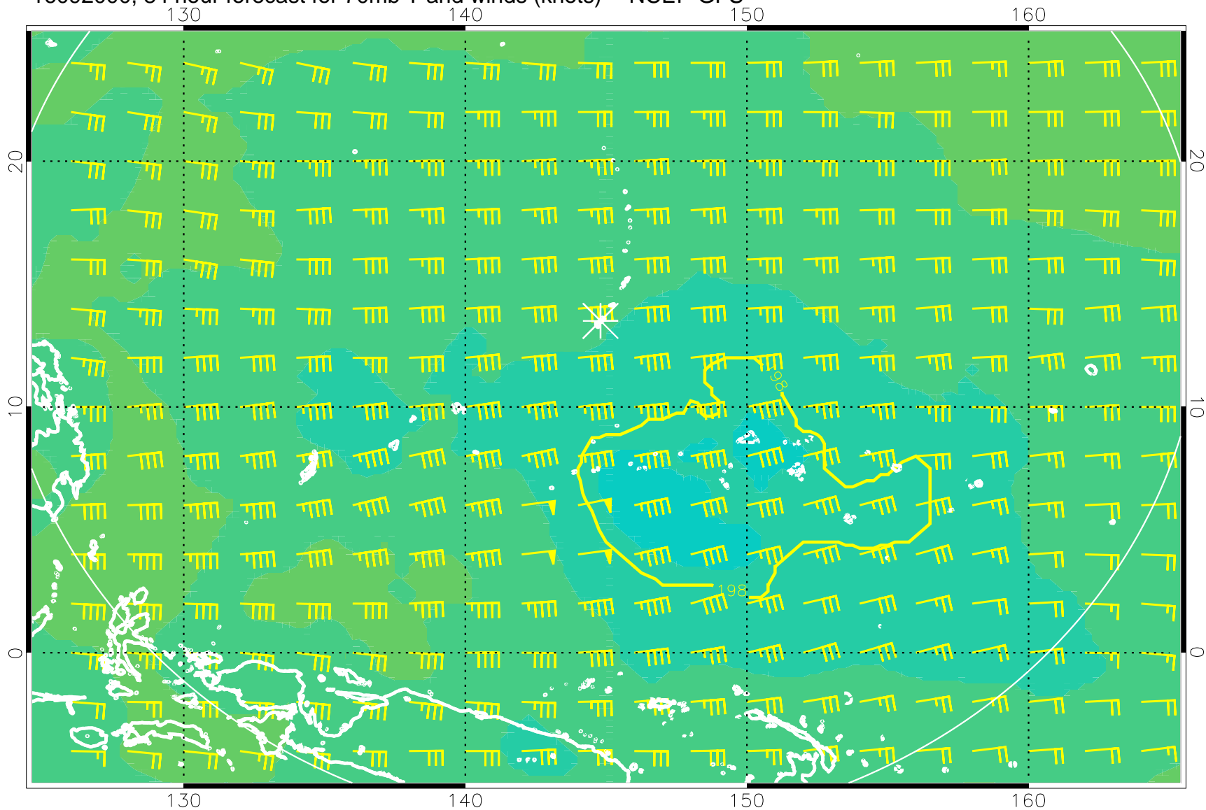
16092000, 84 hour forecast for 70mb T and winds (knots) -- NCEP GFS
