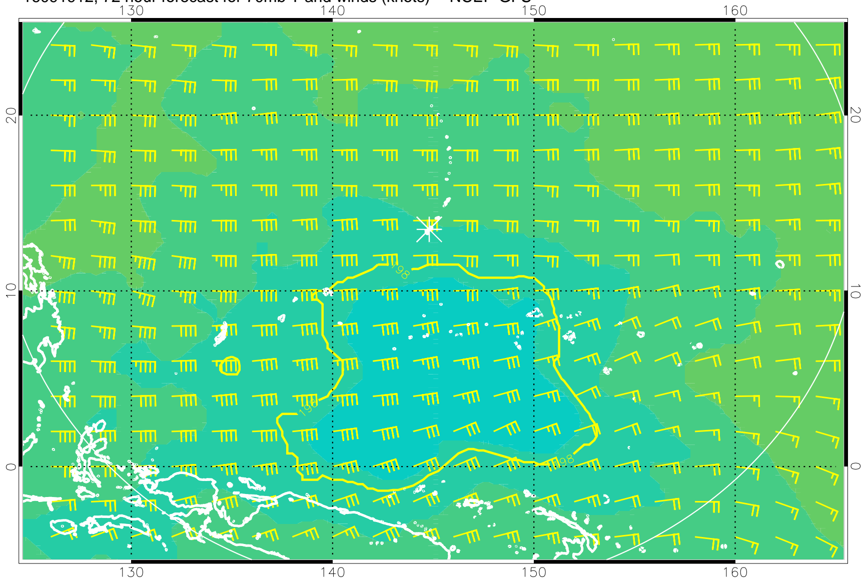
16091912, 72 hour forecast for 70mb T and winds (knots) -- NCEP GFS
