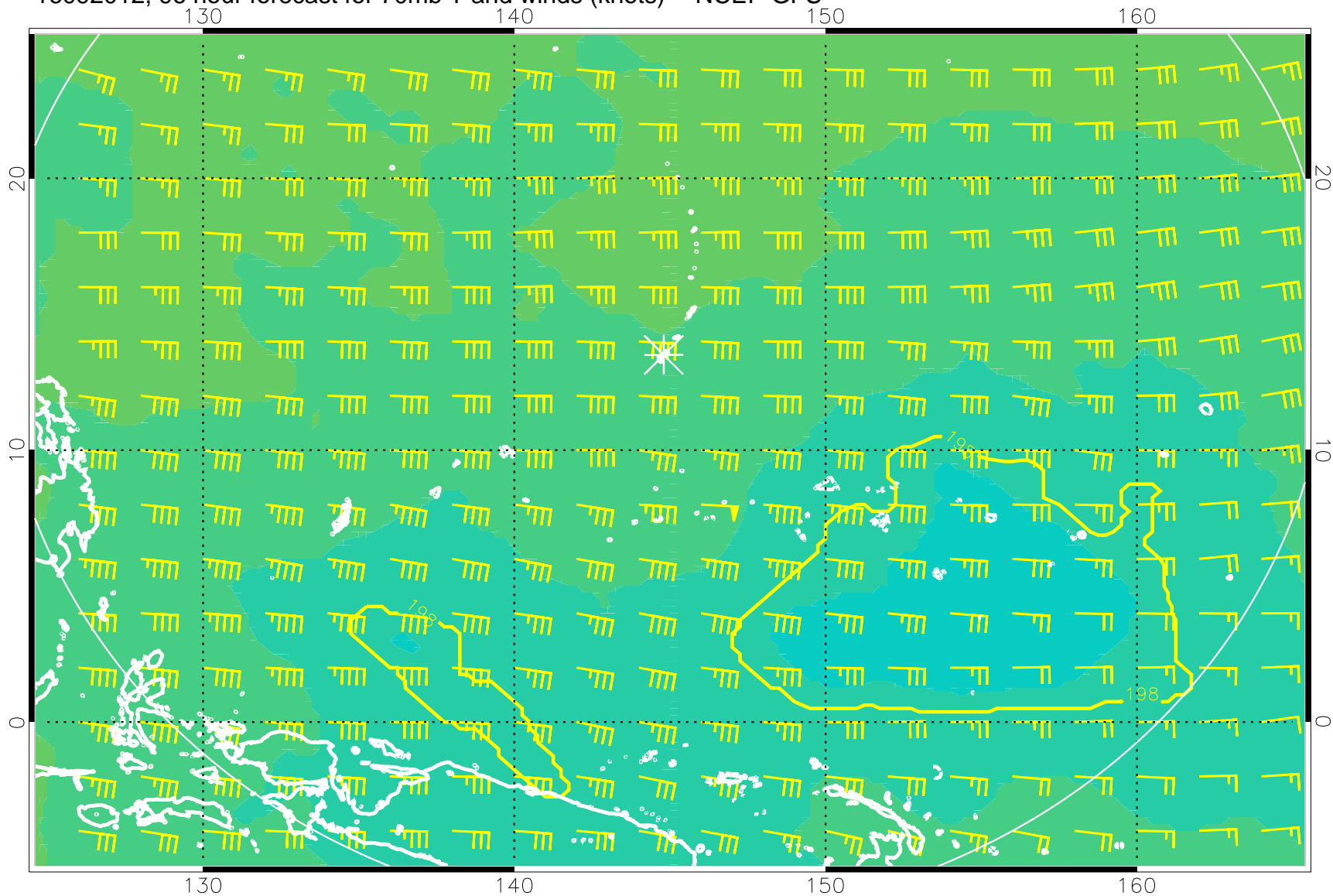
16092012, 96 hour forecast for 70mb T and winds (knots) -- NCEP GFS
