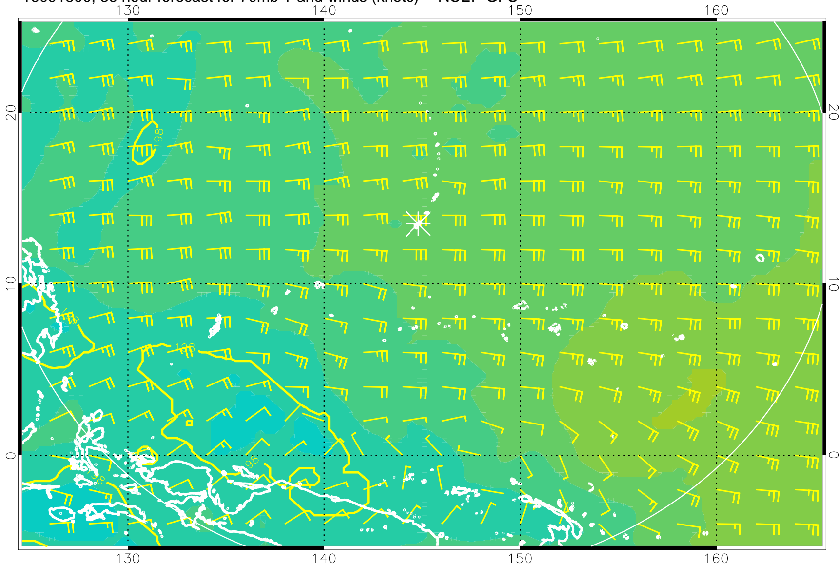
16091800, 36 hour forecast for 70mb T and winds (knots) -- NCEP GFS
