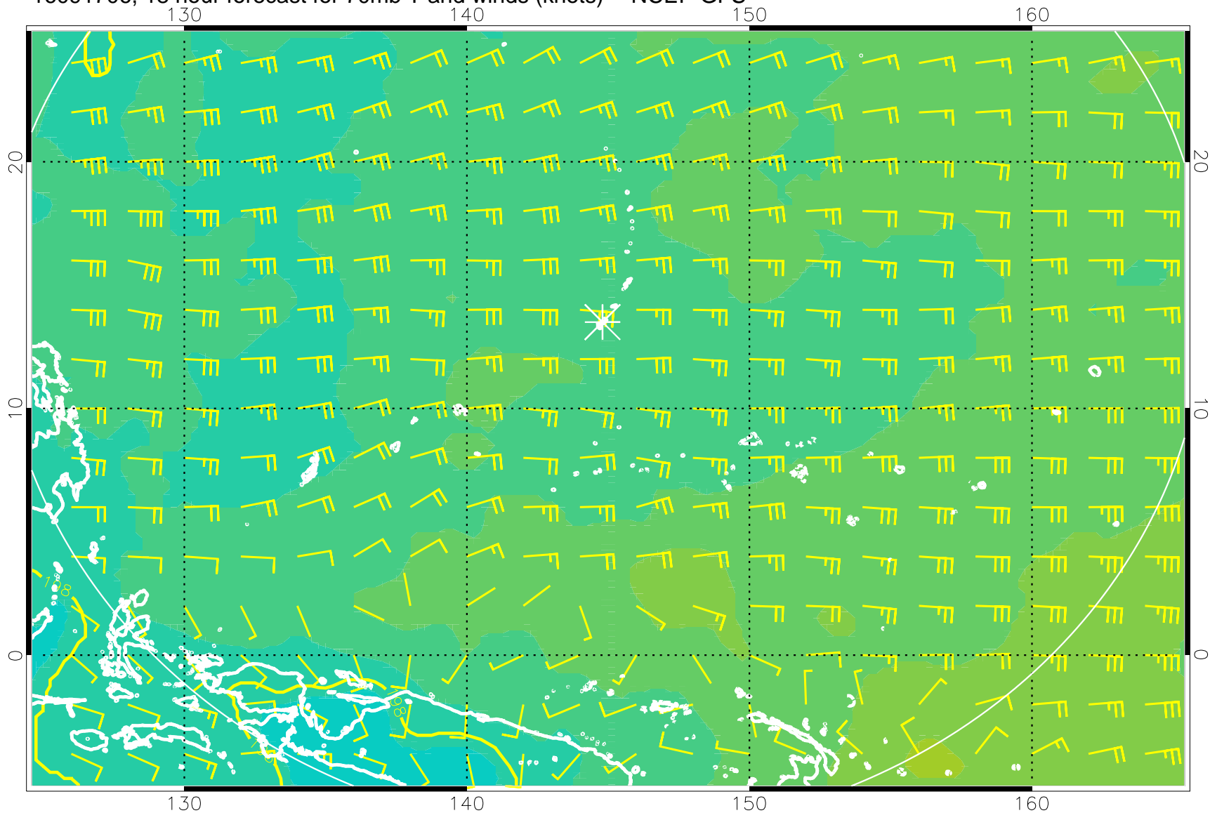
16091706, 18 hour forecast for 70mb T and winds (knots) -- NCEP GFS
