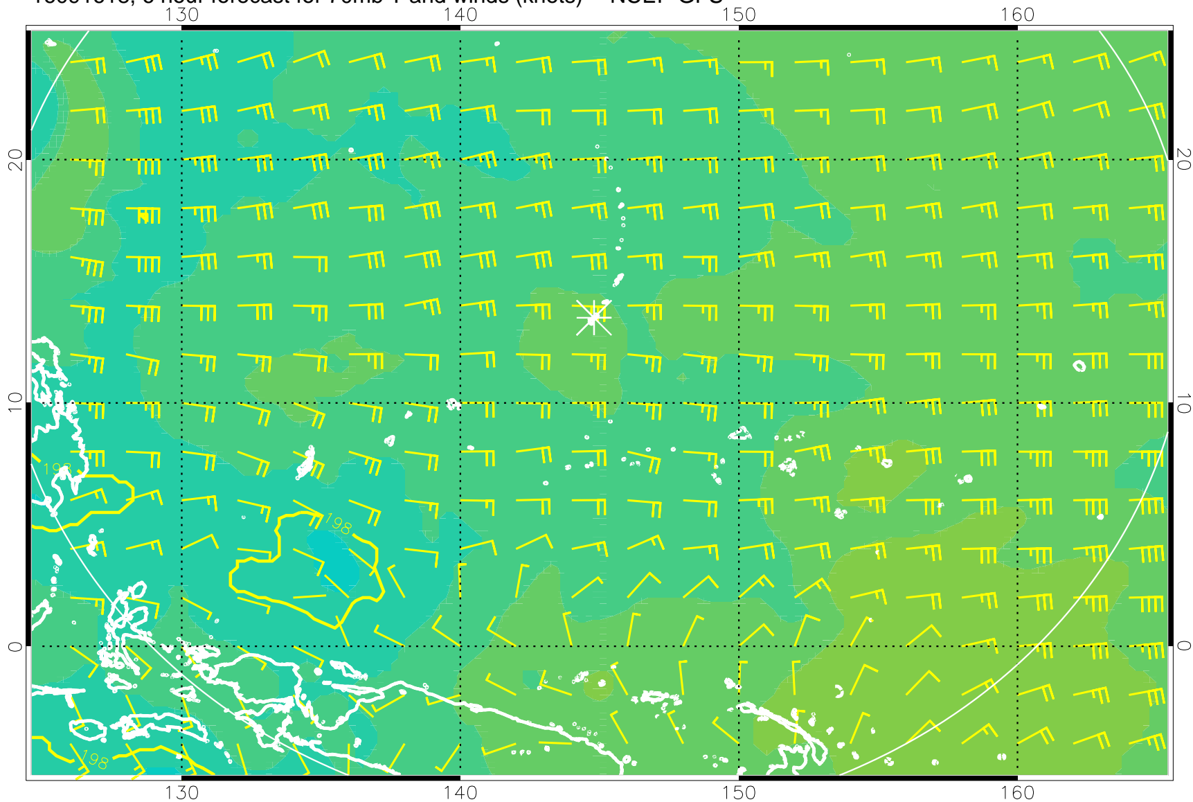
16091618, 6 hour forecast for 70mb T and winds (knots) -- NCEP GFS
