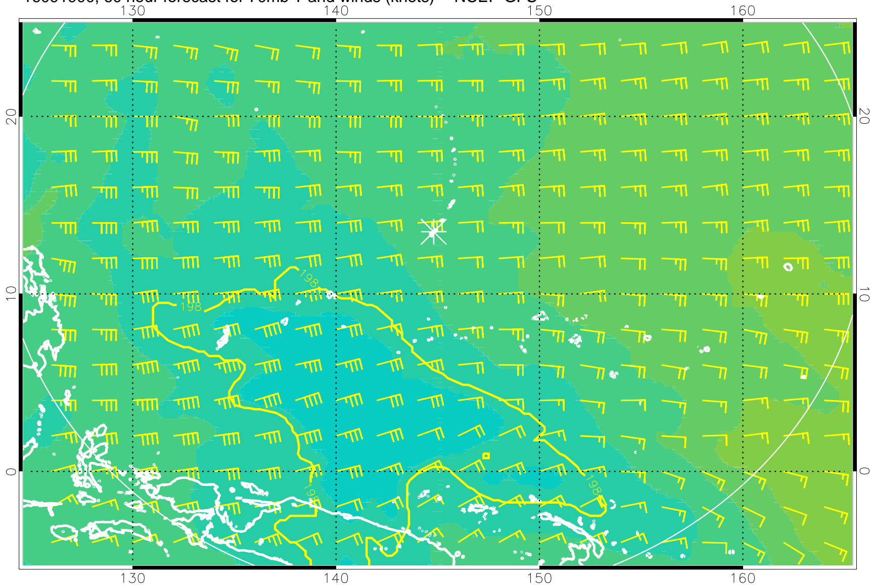
16091900, 60 hour forecast for 70mb T and winds (knots) -- NCEP GFS
