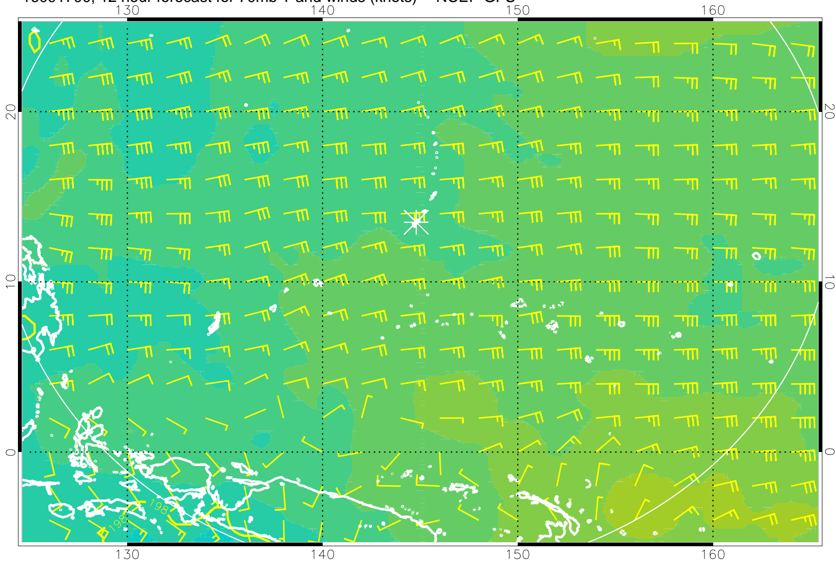
16091700, 12 hour forecast for 70mb T and winds (knots) -- NCEP GFS
