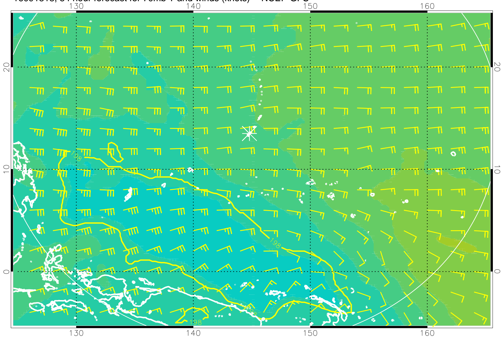
16091818, 54 hour forecast for 70mb T and winds (knots) -- NCEP GFS
