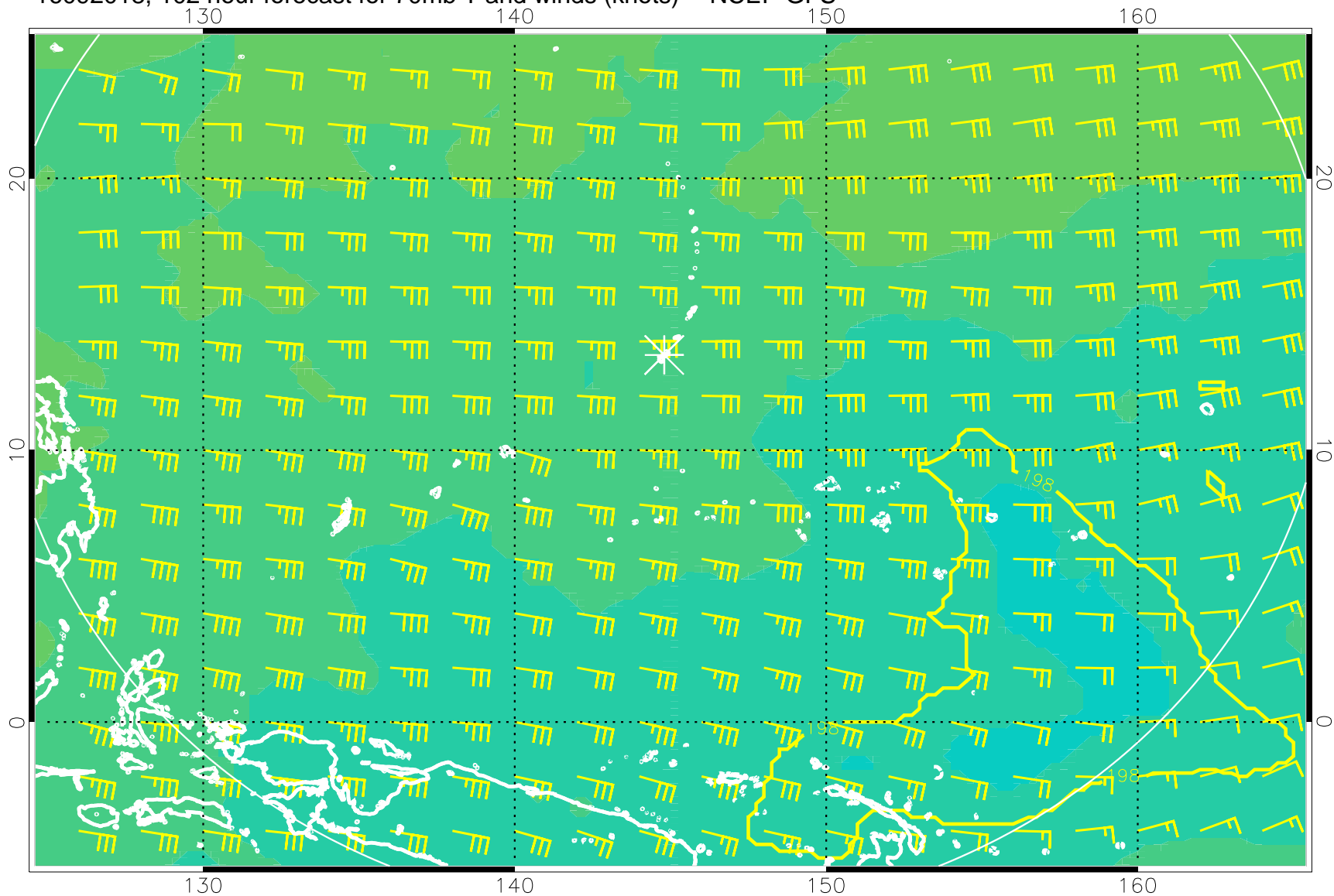
16092018, 102 hour forecast for 70mb T and winds (knots) -- NCEP GFS
