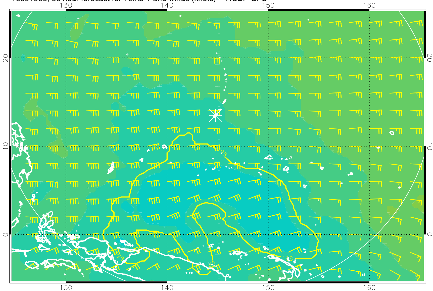
16091906, 66 hour forecast for 70mb T and winds (knots) -- NCEP GFS
