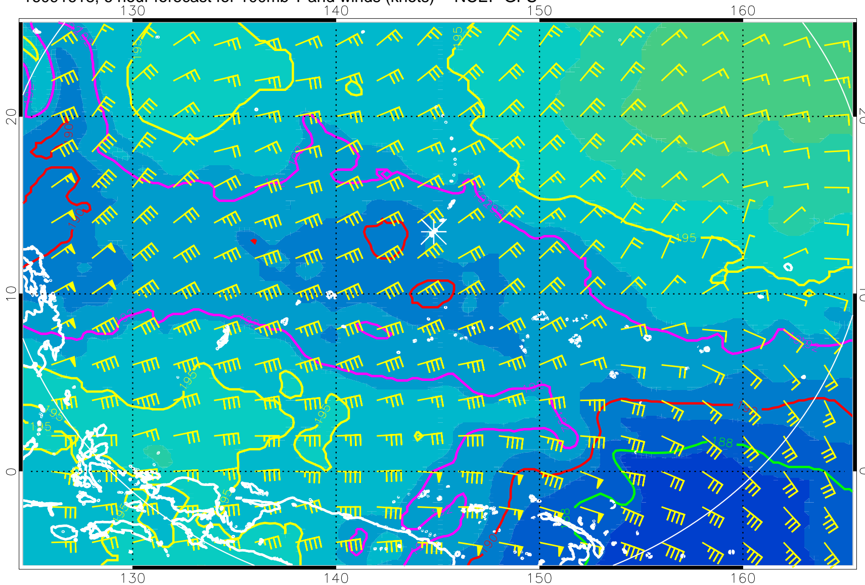
16091618, 6 hour forecast for 100mb T and winds (knots) -- NCEP GFS
