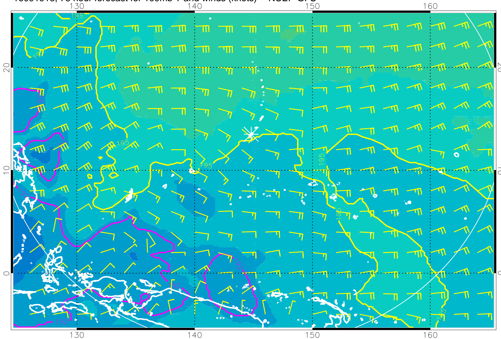
16091918, 78 hour forecast for 100mb T and winds (knots) -- NCEP GFS
