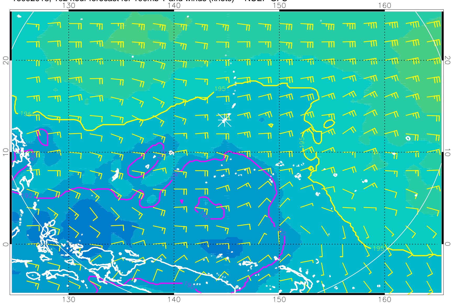
16092018, 102 hour forecast for 100mb T and winds (knots) -- NCEP GFS
