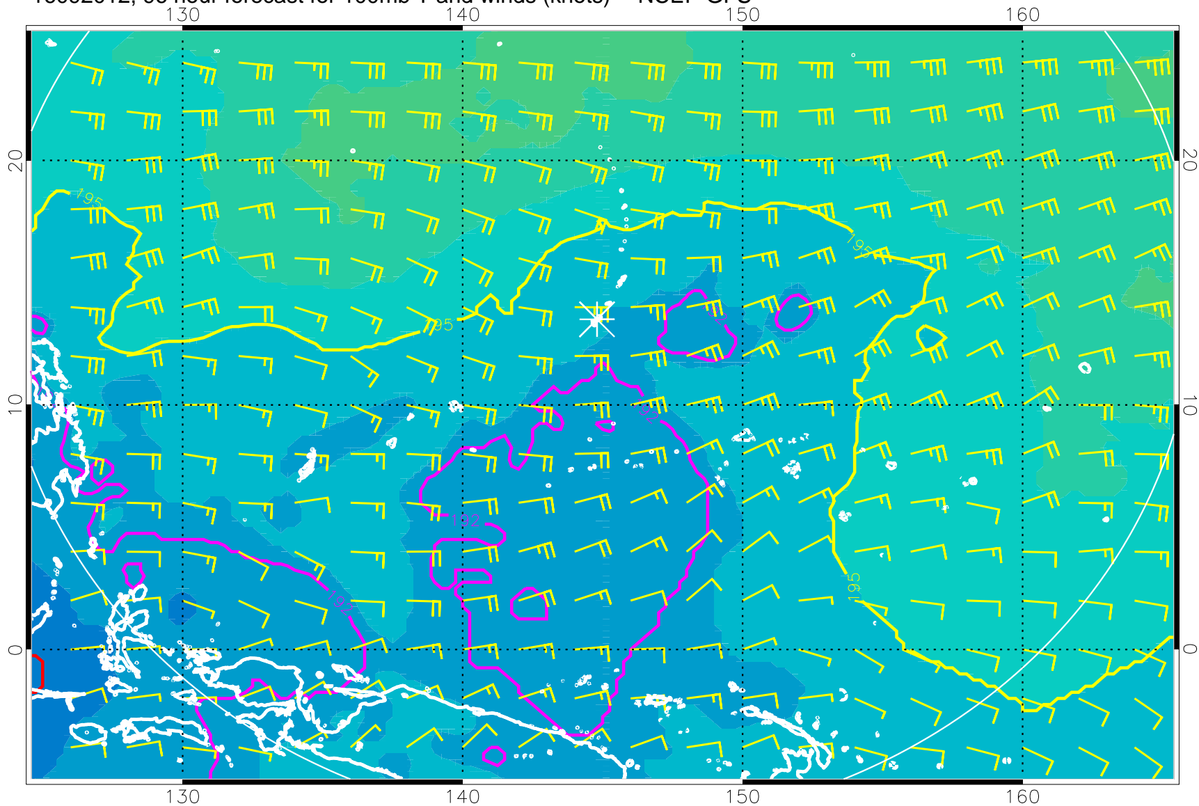
16092012, 96 hour forecast for 100mb T and winds (knots) -- NCEP GFS
