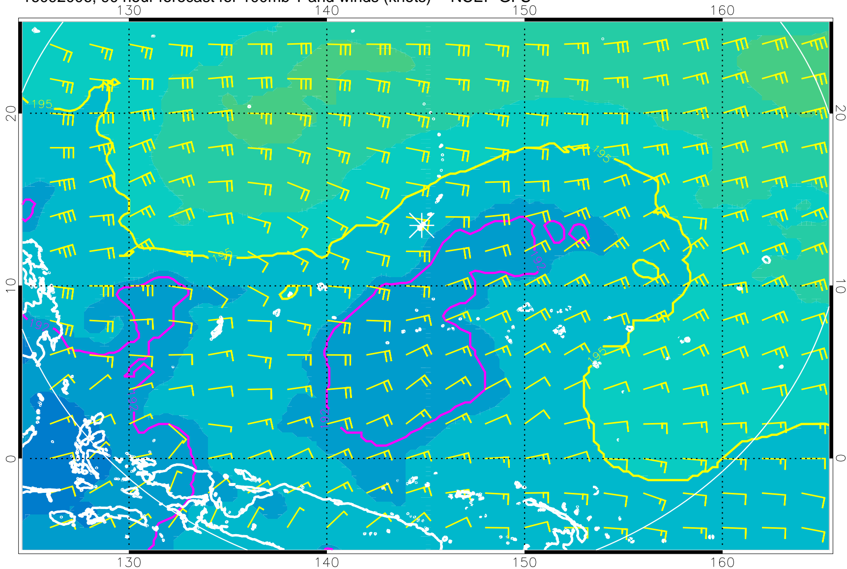
16092006, 90 hour forecast for 100mb T and winds (knots) -- NCEP GFS
