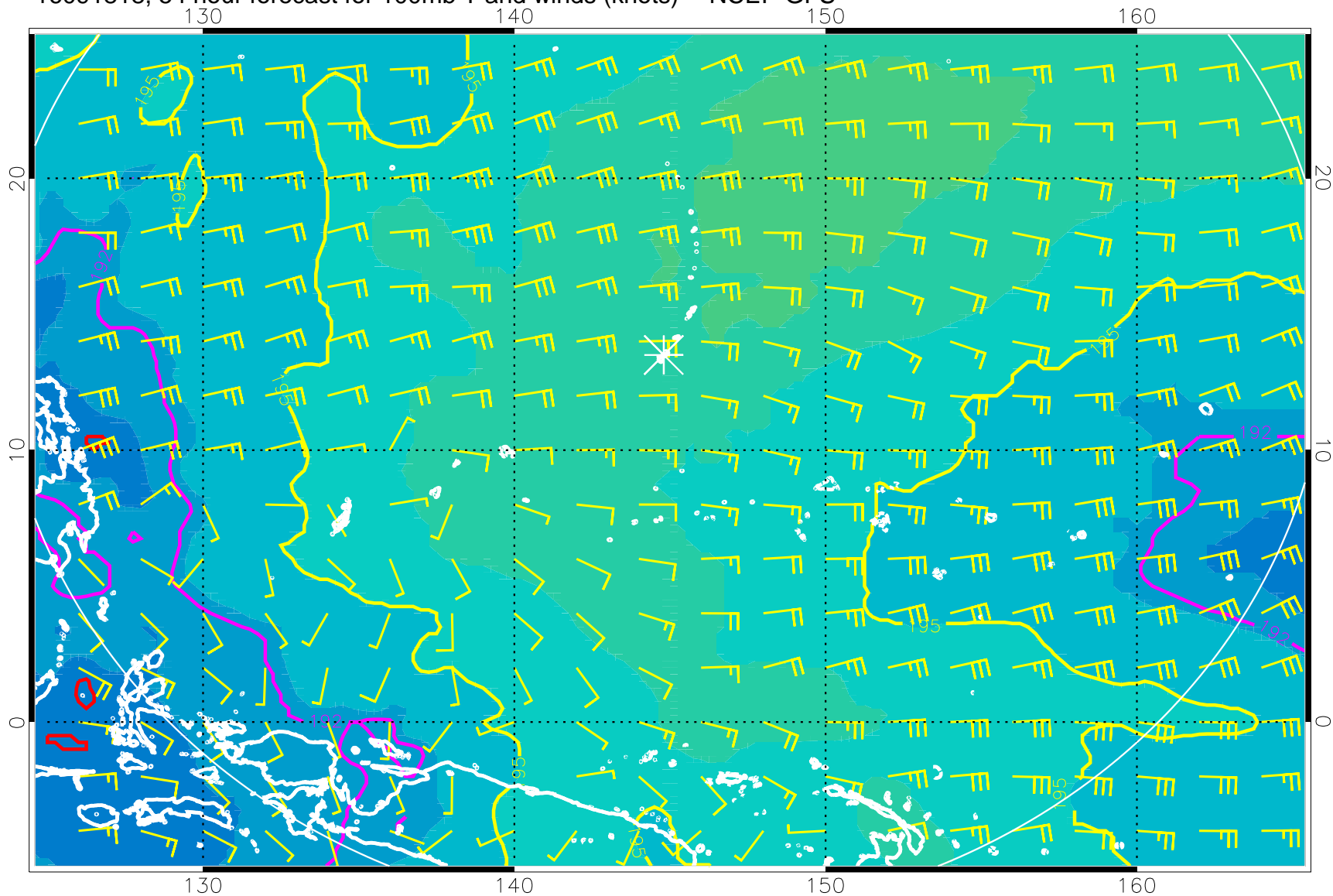
16091818, 54 hour forecast for 100mb T and winds (knots) -- NCEP GFS
