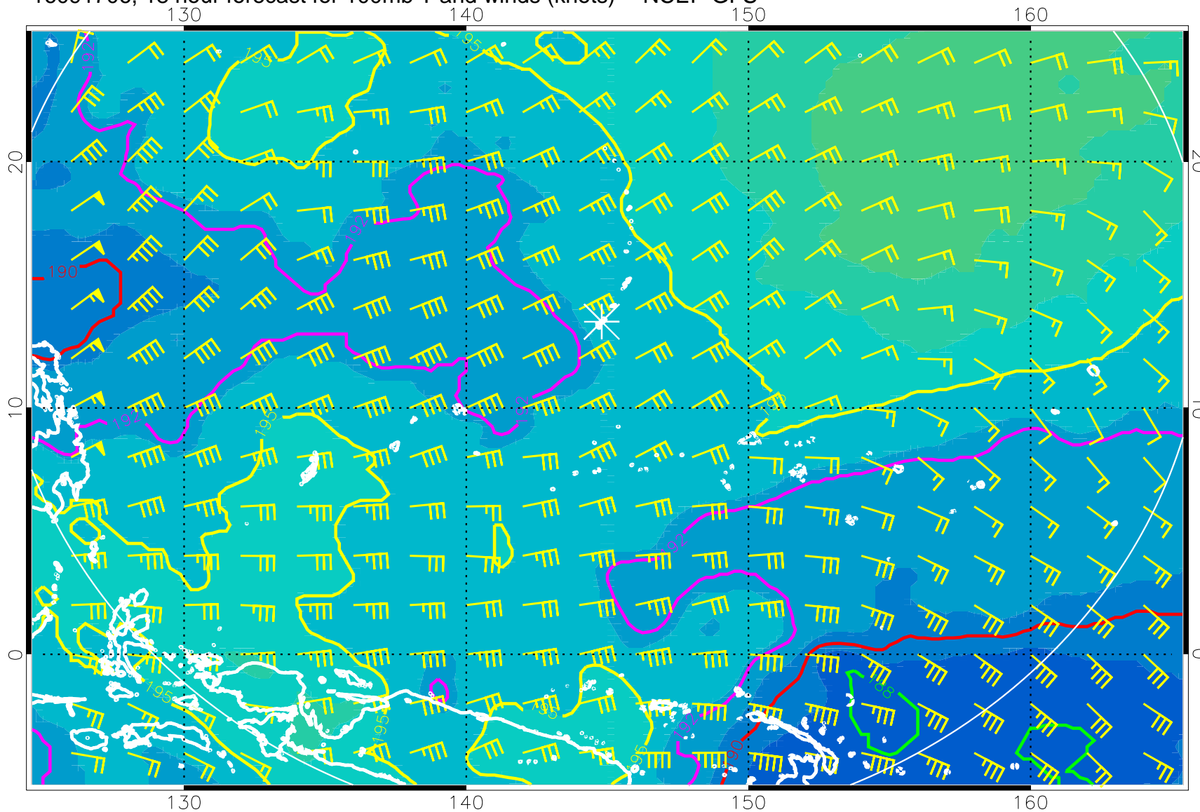
16091706, 18 hour forecast for 100mb T and winds (knots) -- NCEP GFS
