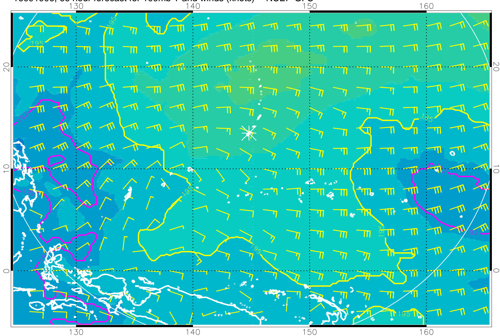
16091906, 66 hour forecast for 100mb T and winds (knots) -- NCEP GFS
