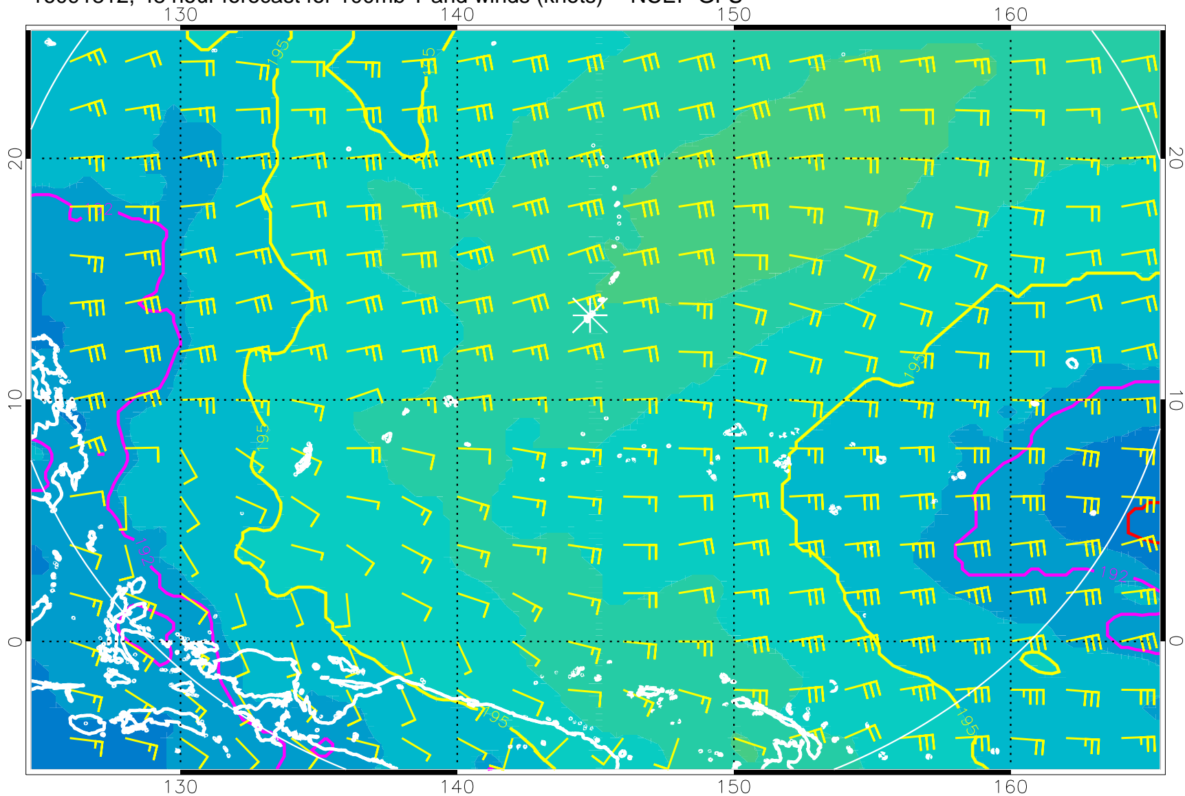
16091812, 48 hour forecast for 100mb T and winds (knots) -- NCEP GFS
