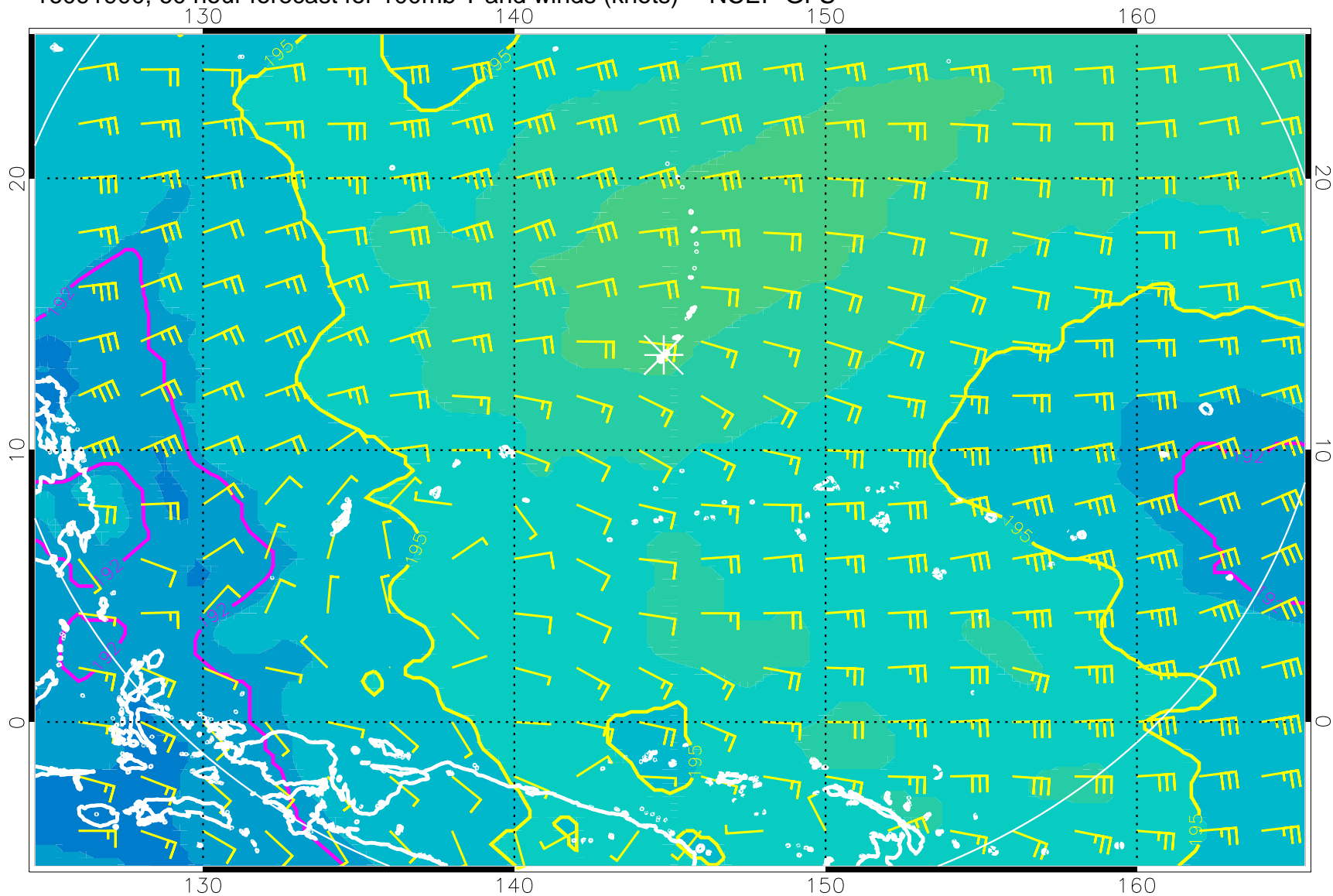
16091900, 60 hour forecast for 100mb T and winds (knots) -- NCEP GFS
