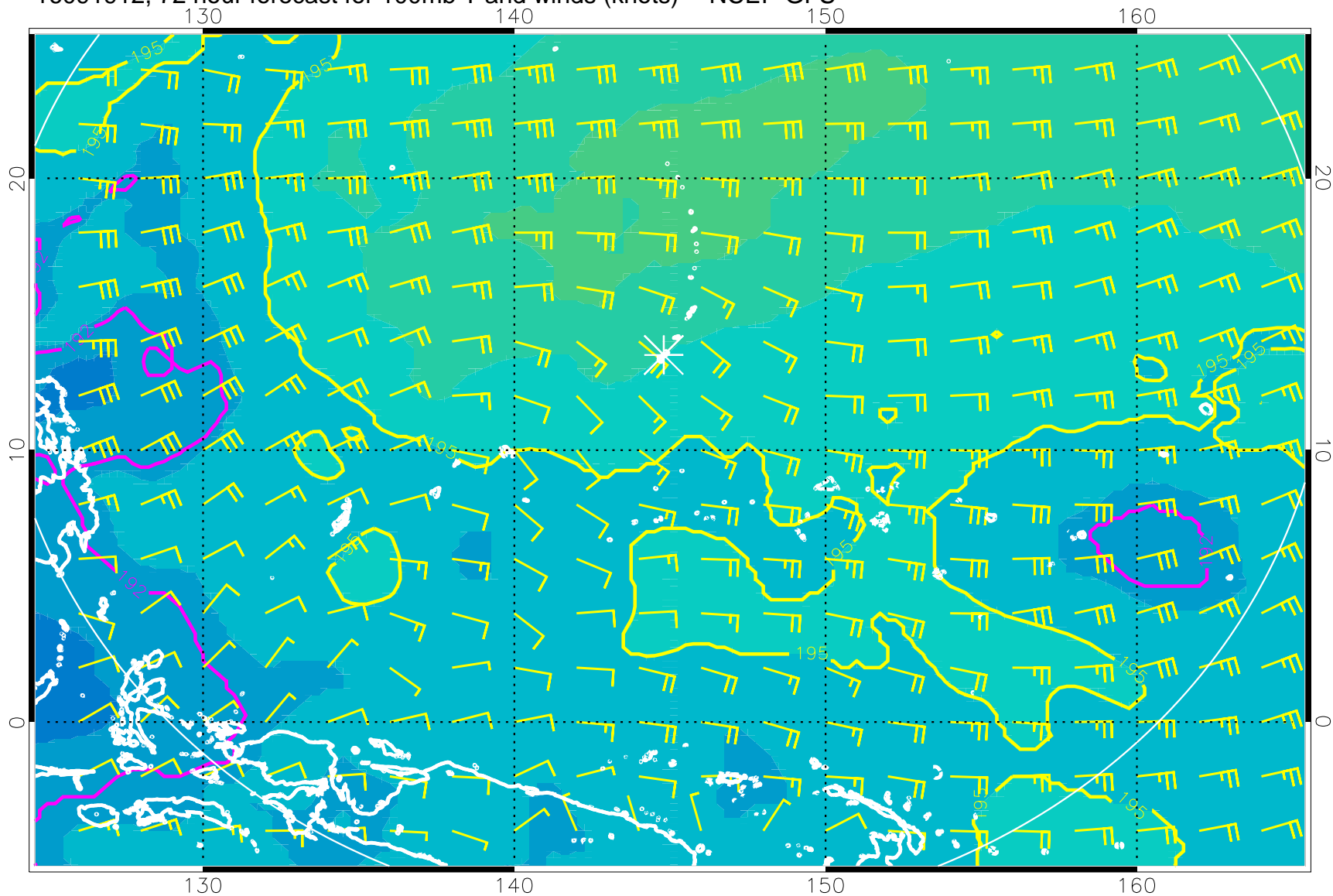
16091912, 72 hour forecast for 100mb T and winds (knots) -- NCEP GFS
