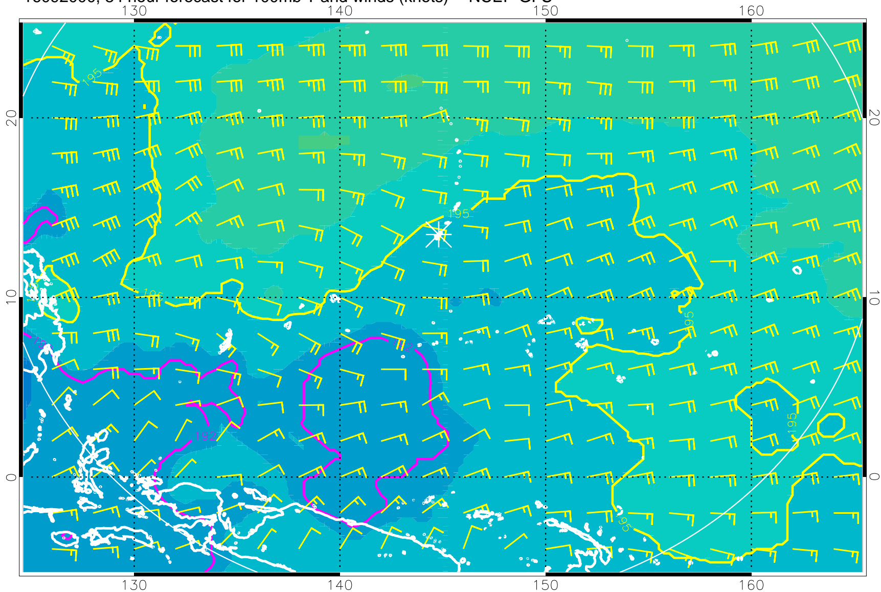
16092000, 84 hour forecast for 100mb T and winds (knots) -- NCEP GFS
