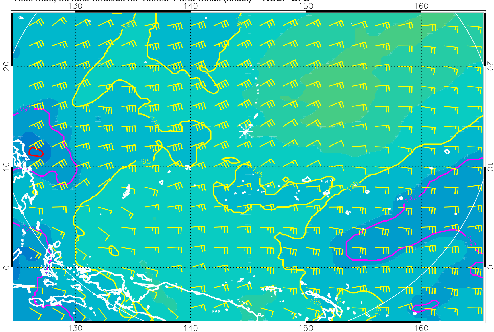
16091800, 36 hour forecast for 100mb T and winds (knots) -- NCEP GFS
