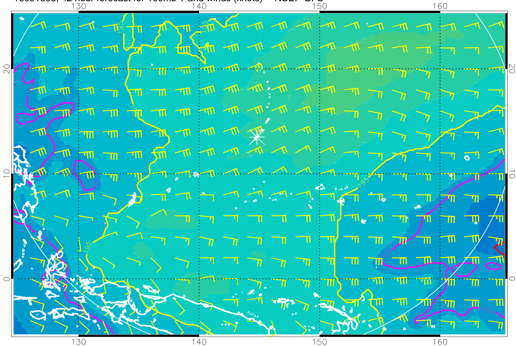
16091806, 42 hour forecast for 100mb T and winds (knots) -- NCEP GFS
