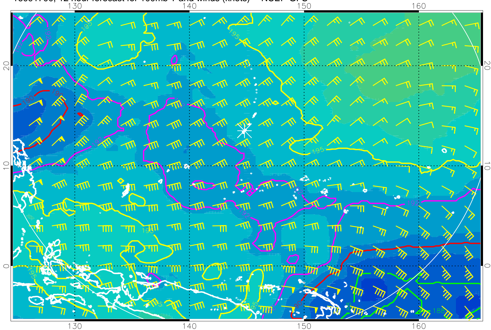
16091700, 12 hour forecast for 100mb T and winds (knots) -- NCEP GFS
