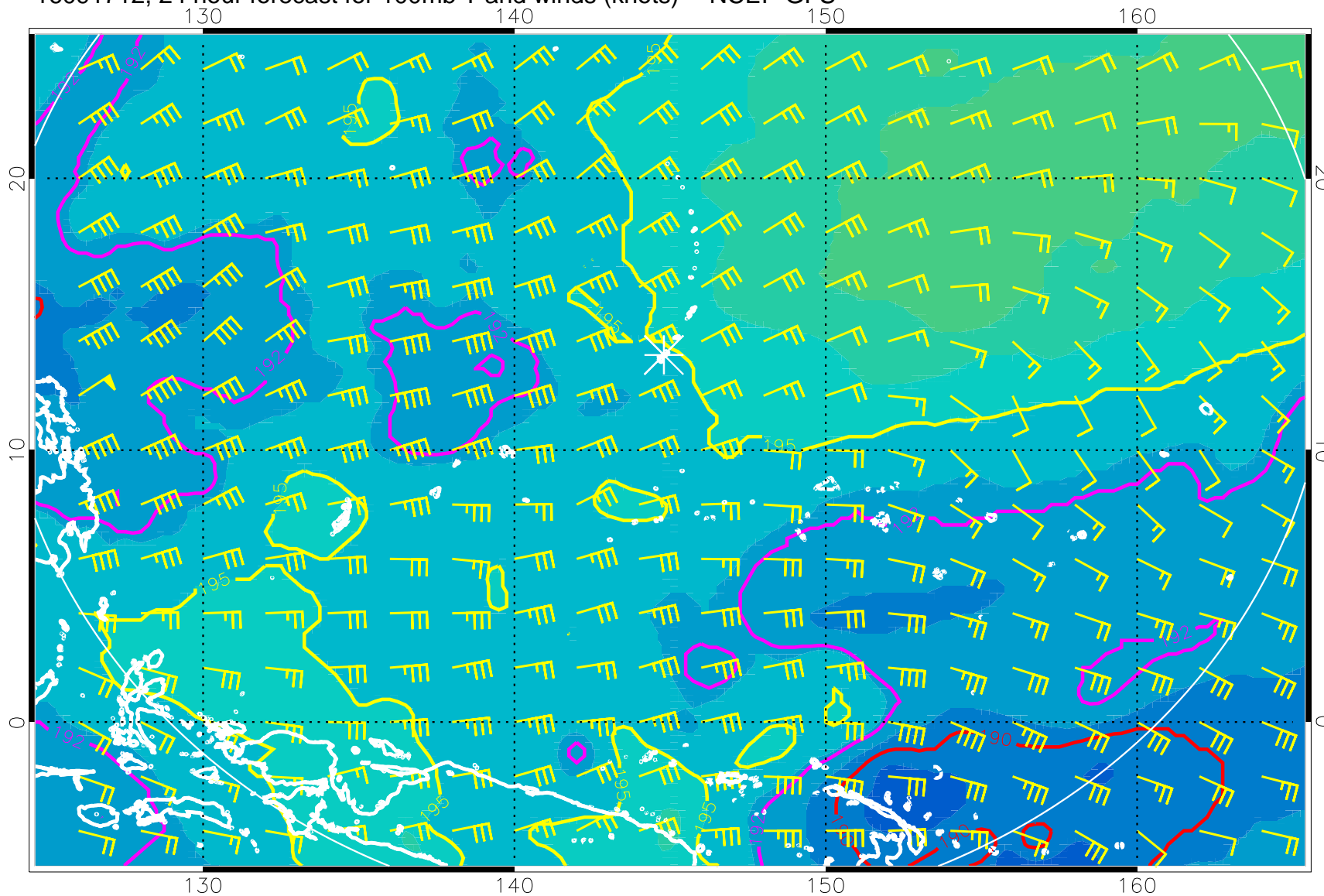
16091712, 24 hour forecast for 100mb T and winds (knots) -- NCEP GFS
