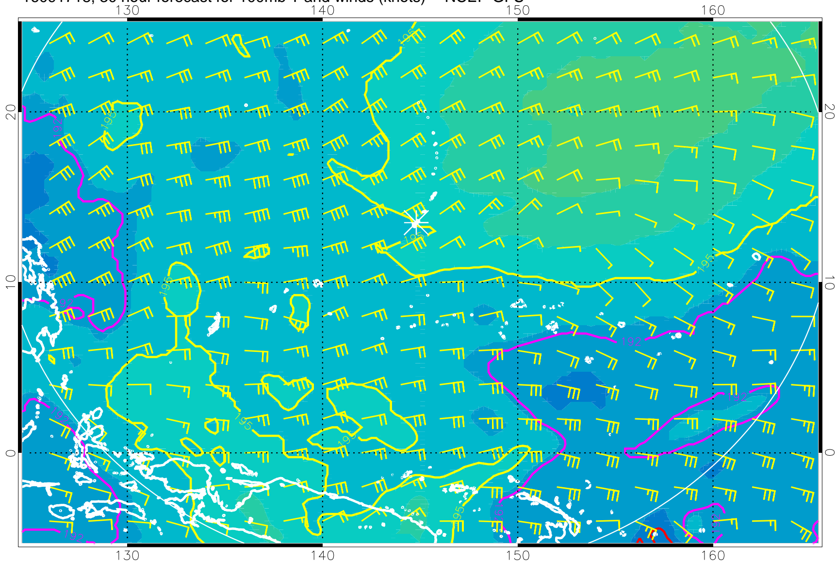
16091718, 30 hour forecast for 100mb T and winds (knots) -- NCEP GFS
