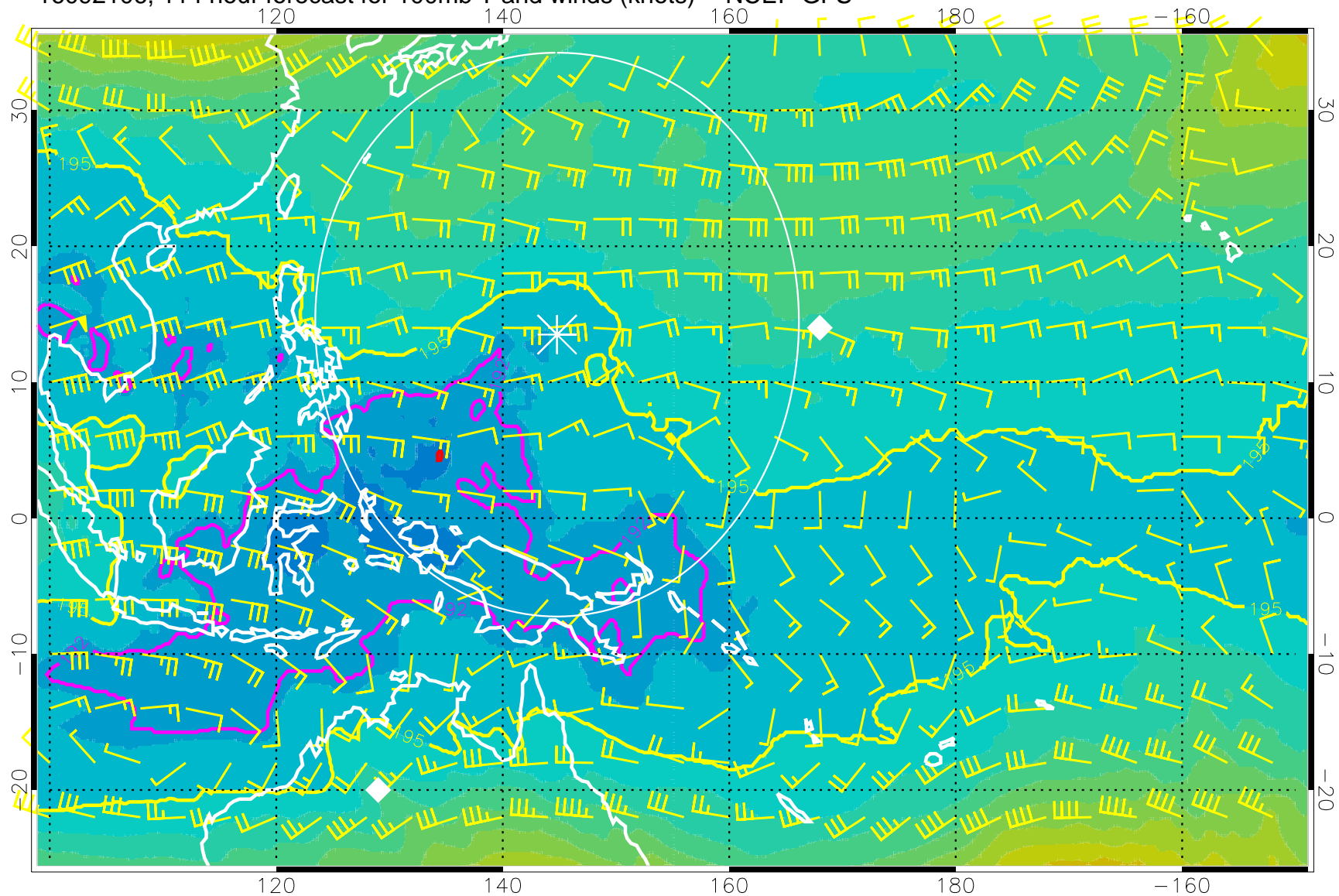
16092106, 114 hour forecast for 100mb T and winds (knots) -- NCEP GFS
