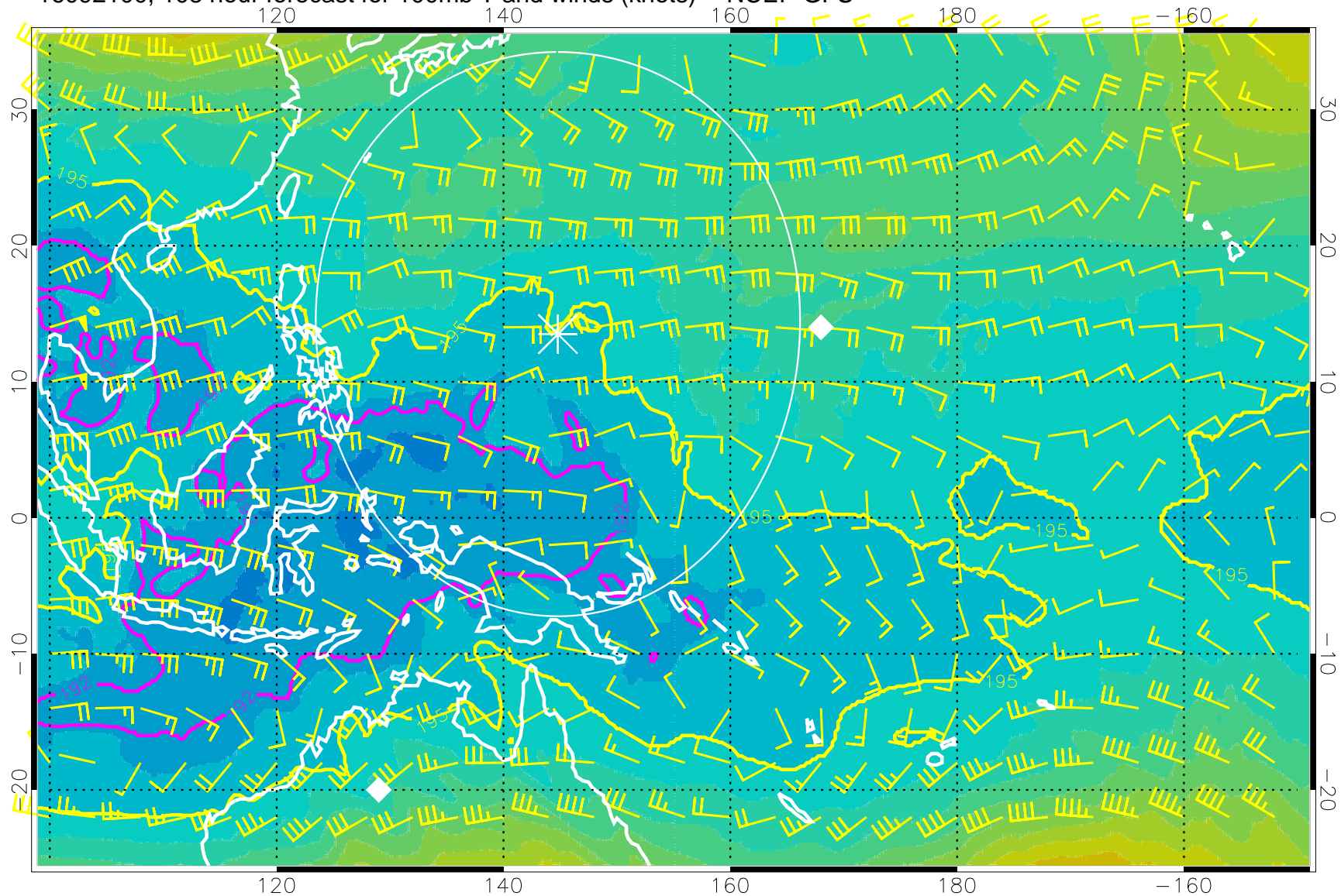
16092100, 108 hour forecast for 100mb T and winds (knots) -- NCEP GFS
