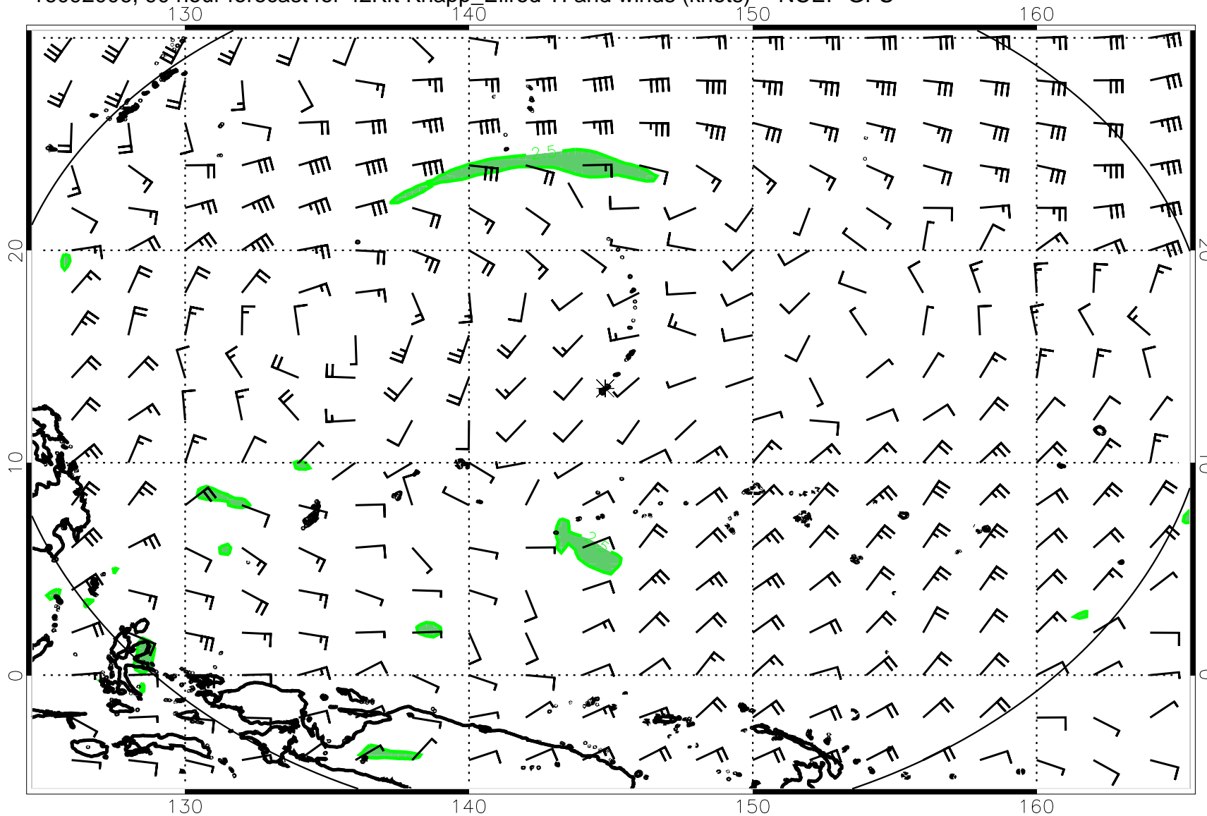
16092006, 90 hour forecast for 42Kft Knapp_Ellrod TI and winds (knots) -- NCEP GFS
