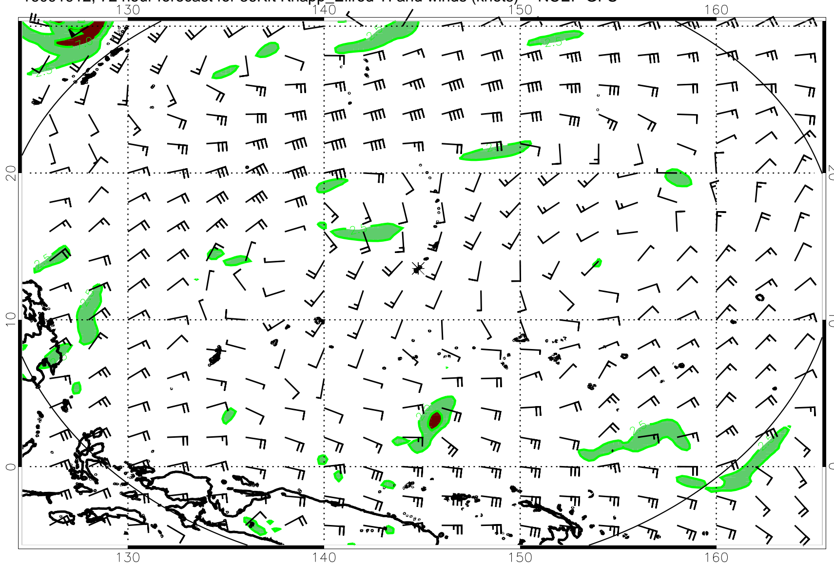
16091912, 72 hour forecast for 36Kft Knapp_Ellrod TI and winds (knots) -- NCEP GFS
