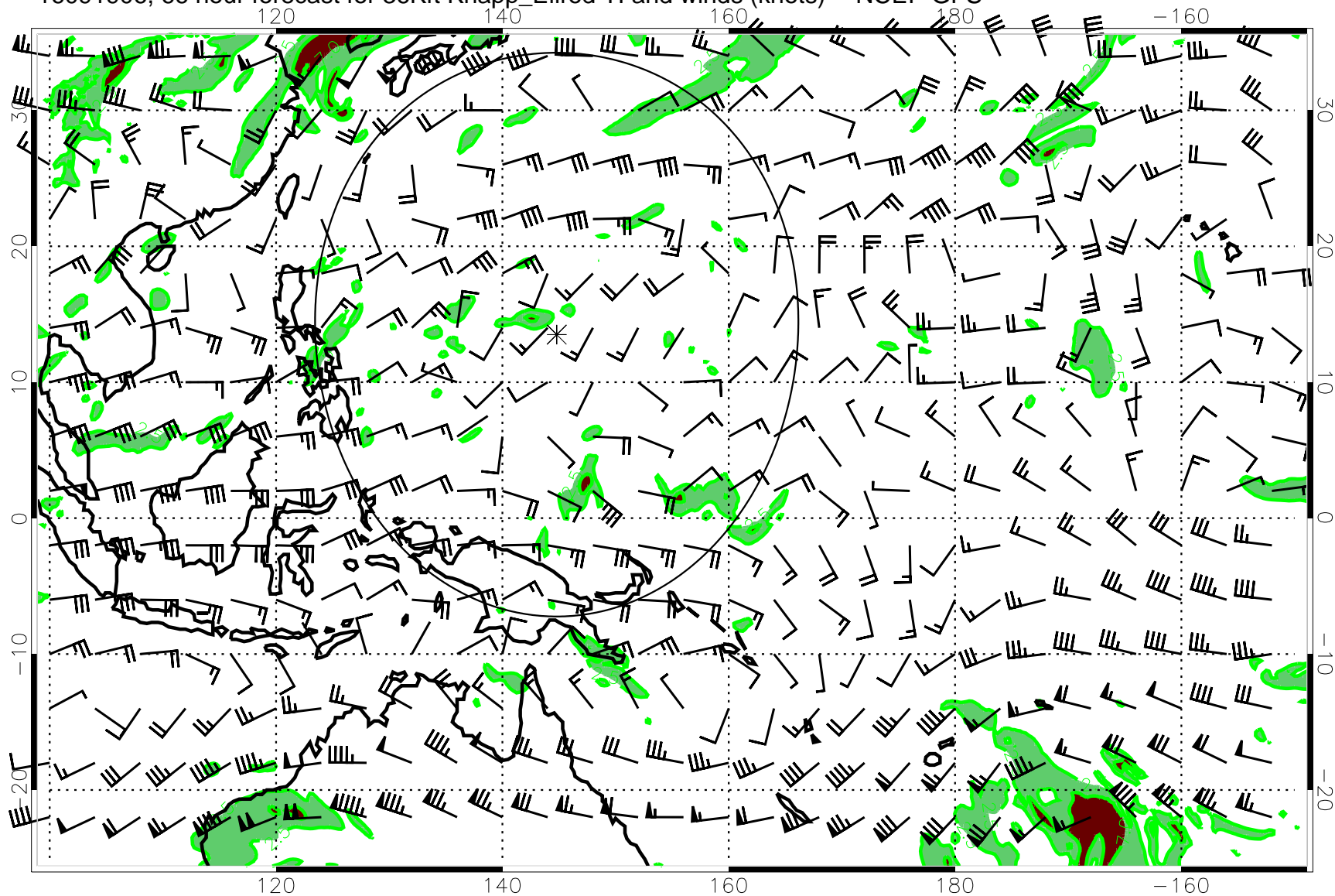
16091906, 66 hour forecast for 36Kft Knapp_Ellrod TI and winds (knots) -- NCEP GFS
