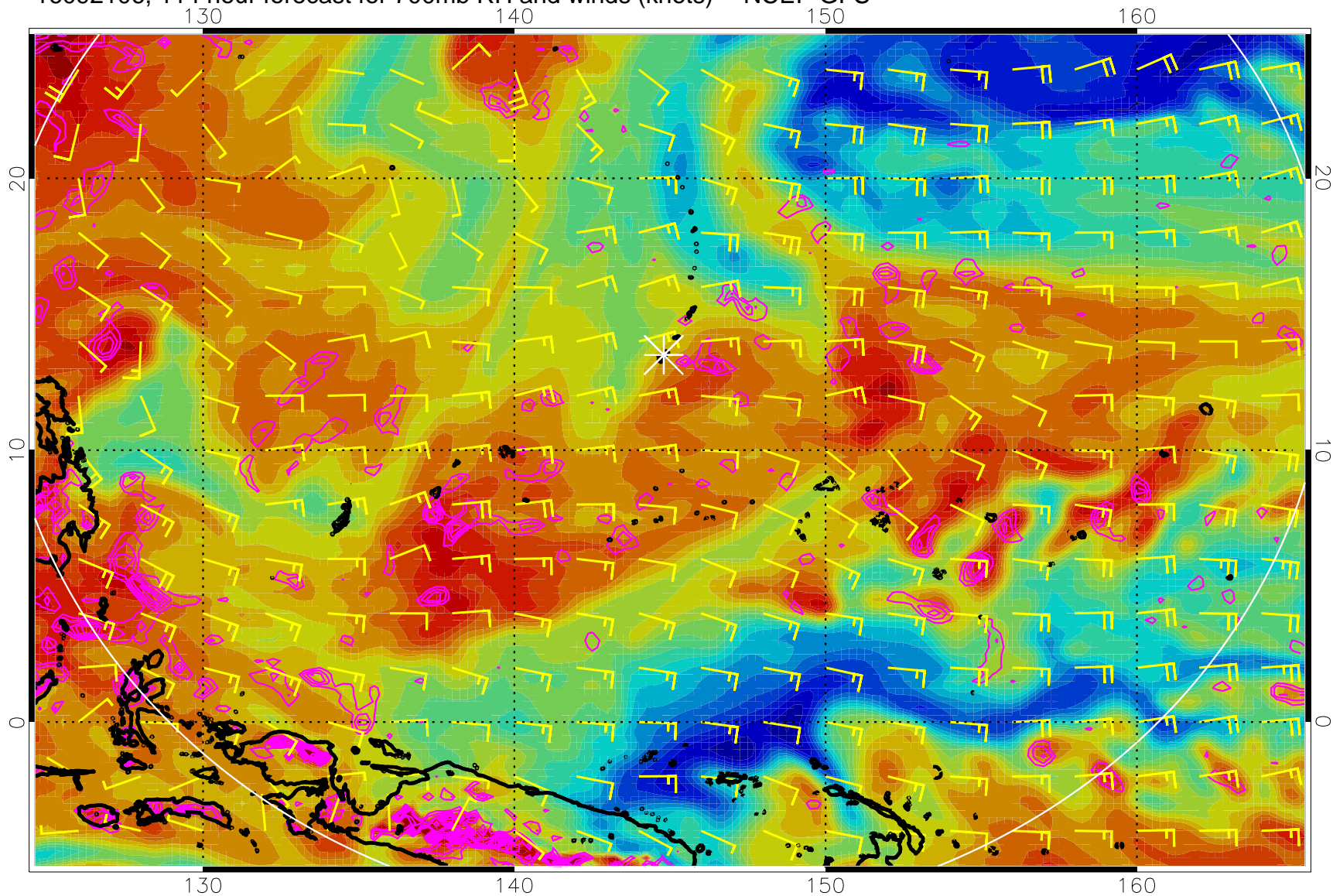
16092106, 114 hour forecast for 700mb RH and winds (knots) -- NCEP GFS
