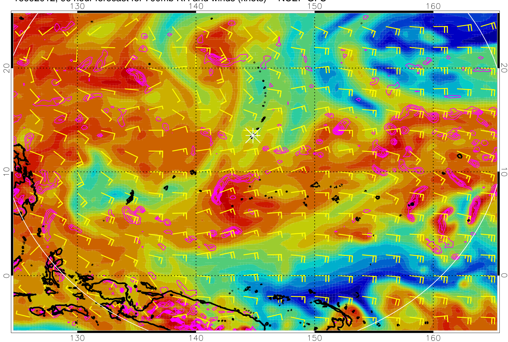
16092012, 96 hour forecast for 700mb RH and winds (knots) -- NCEP GFS
