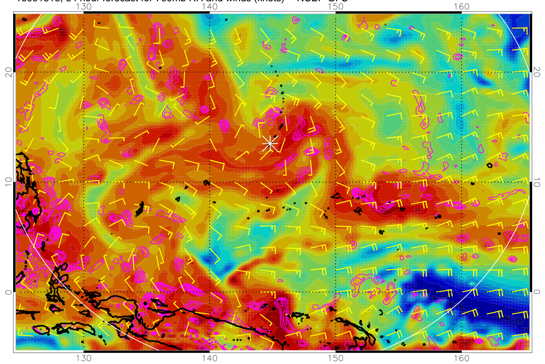
16091818, 54 hour forecast for 700mb RH and winds (knots) -- NCEP GFS
