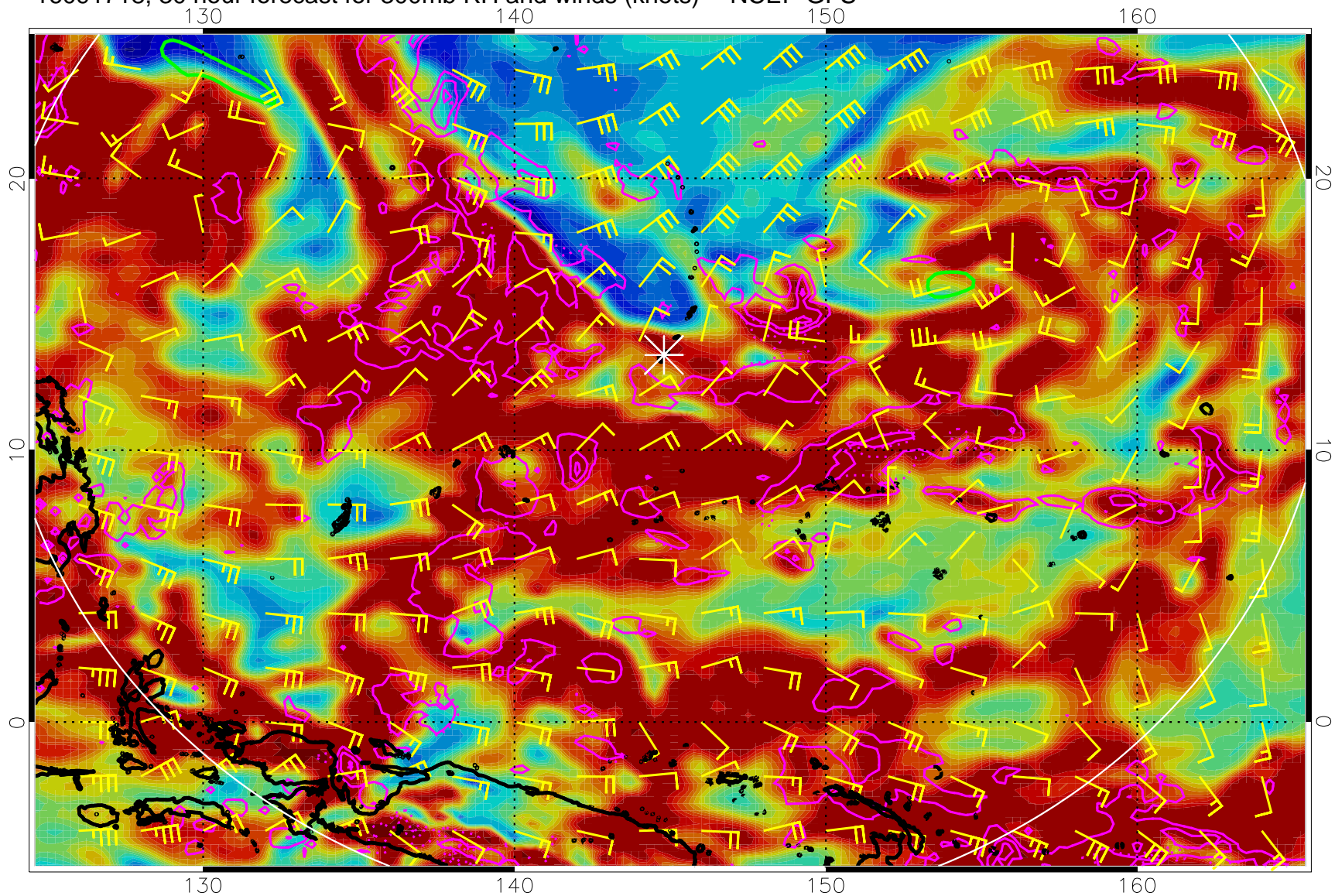
16091718, 30 hour forecast for 300mb RH and winds (knots) -- NCEP GFS
