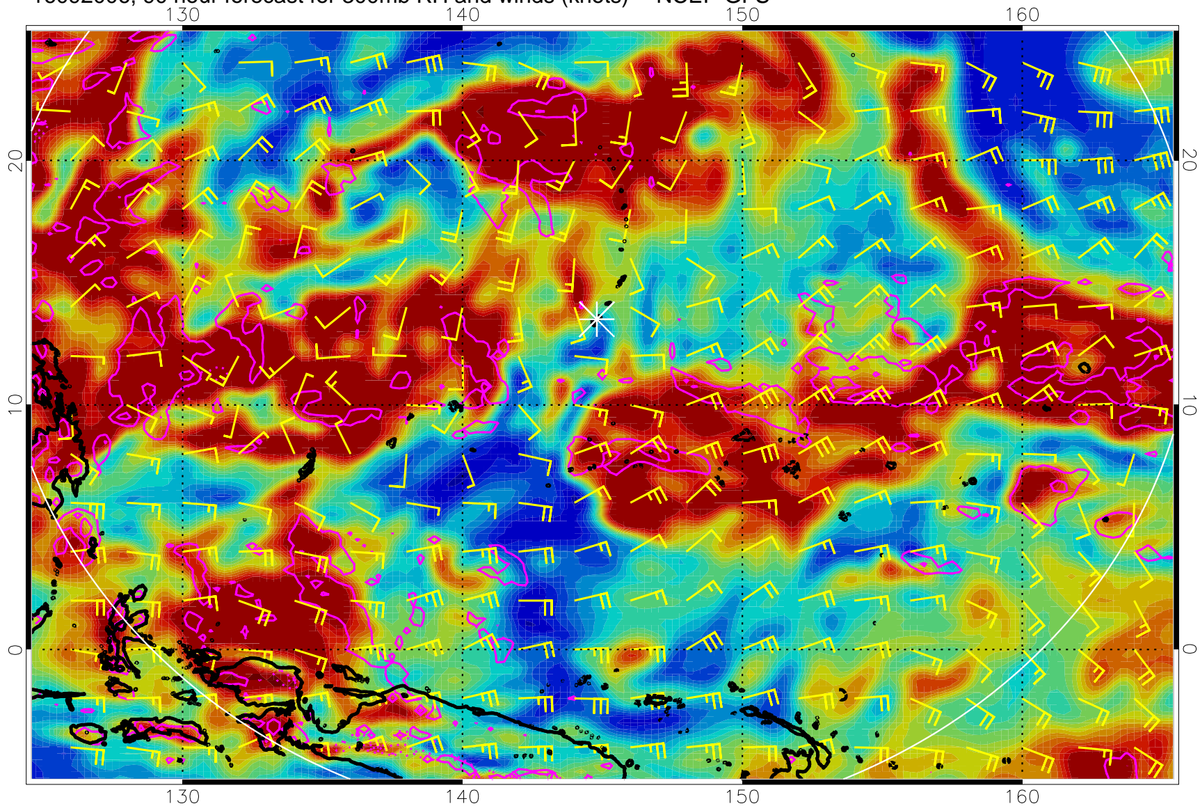
16092006, 90 hour forecast for 300mb RH and winds (knots) -- NCEP GFS
