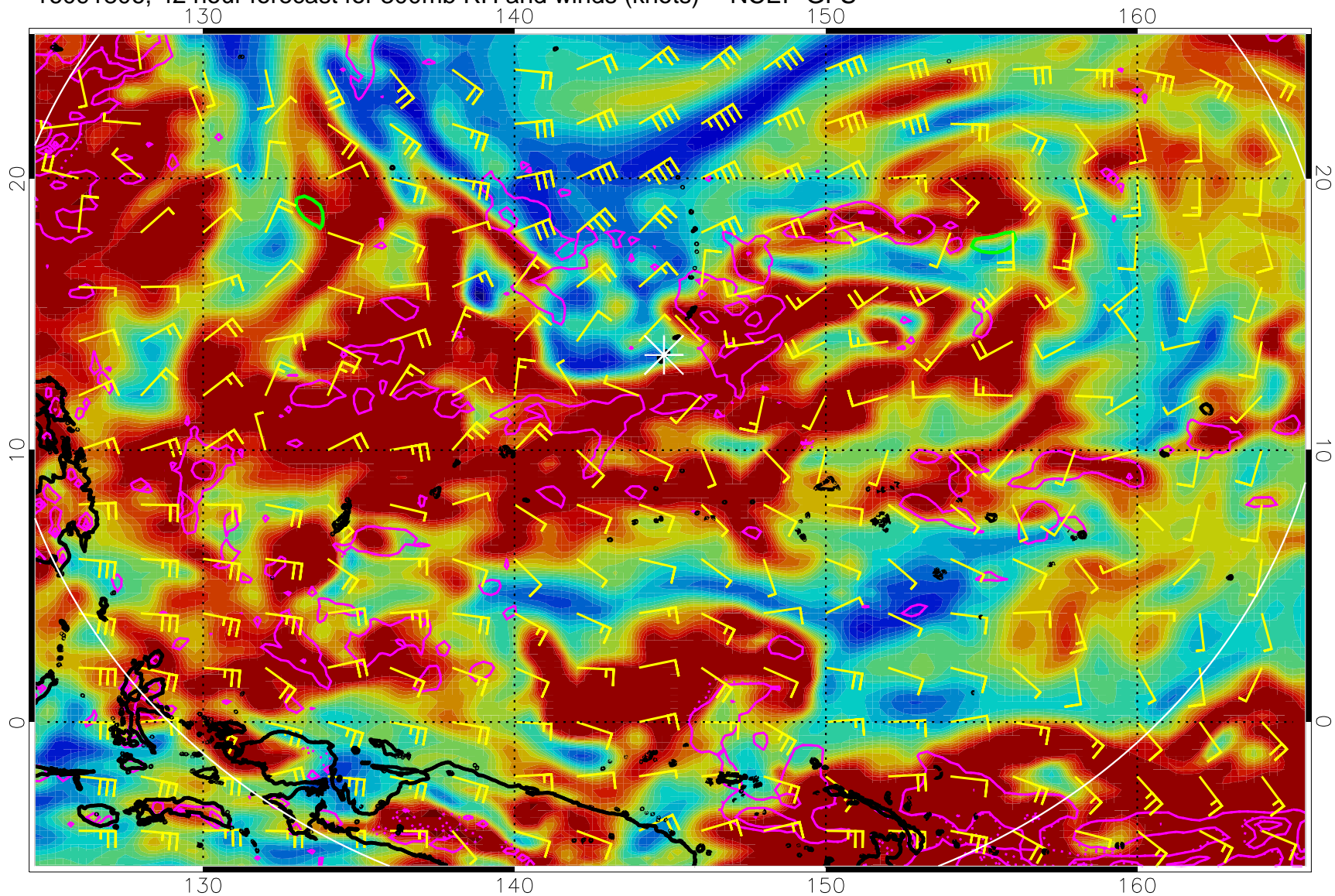
16091806, 42 hour forecast for 300mb RH and winds (knots) -- NCEP GFS
