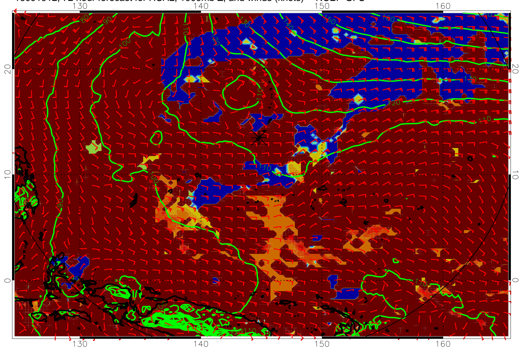
16091912, 72 hour forecast for HCAL, 1000mb Z, and winds (knots) -- NCEP GFS
