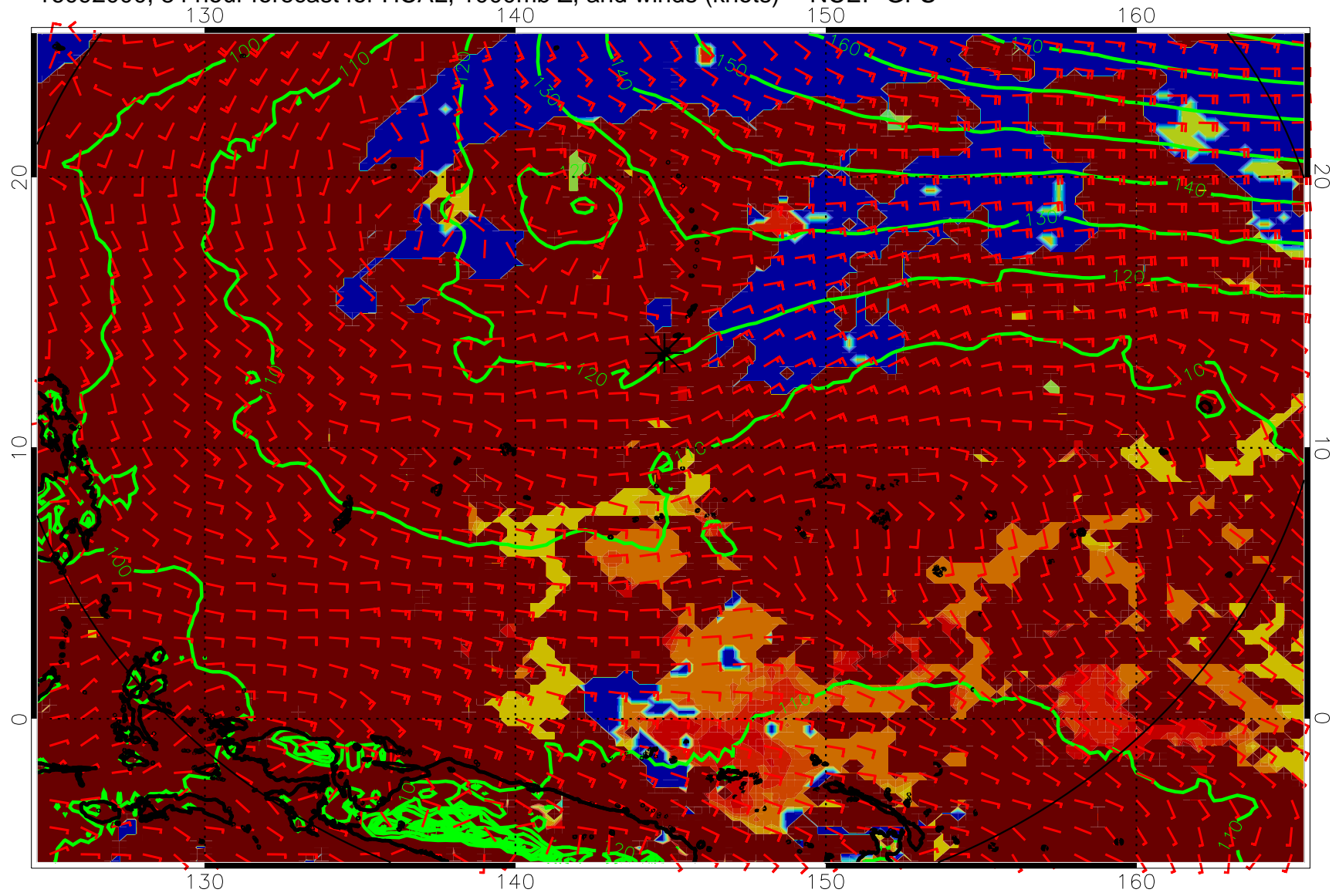
16092000, 84 hour forecast for HCAL, 1000mb Z, and winds (knots) -- NCEP GFS
