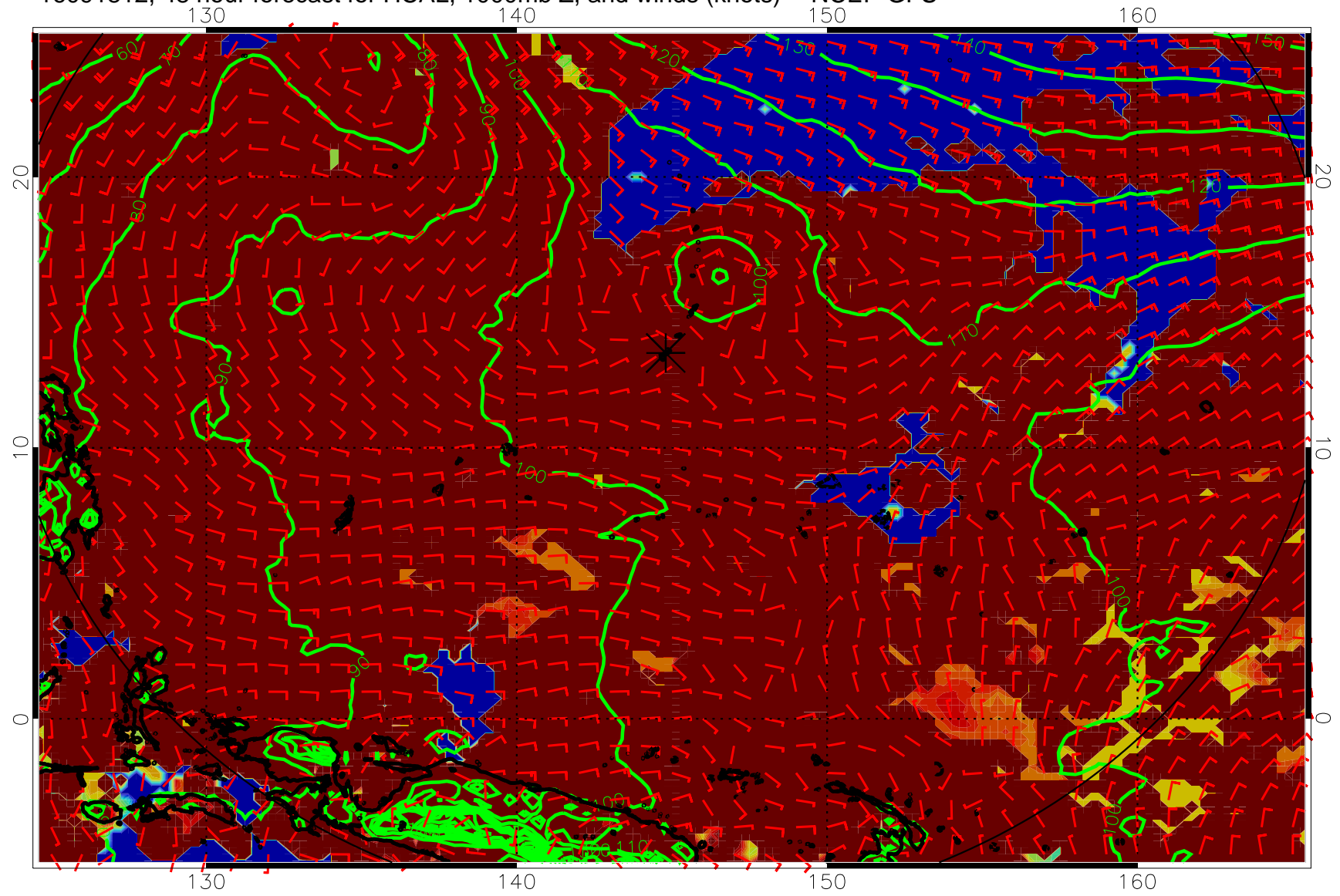
16091812, 48 hour forecast for HCAL, 1000mb Z, and winds (knots) -- NCEP GFS
