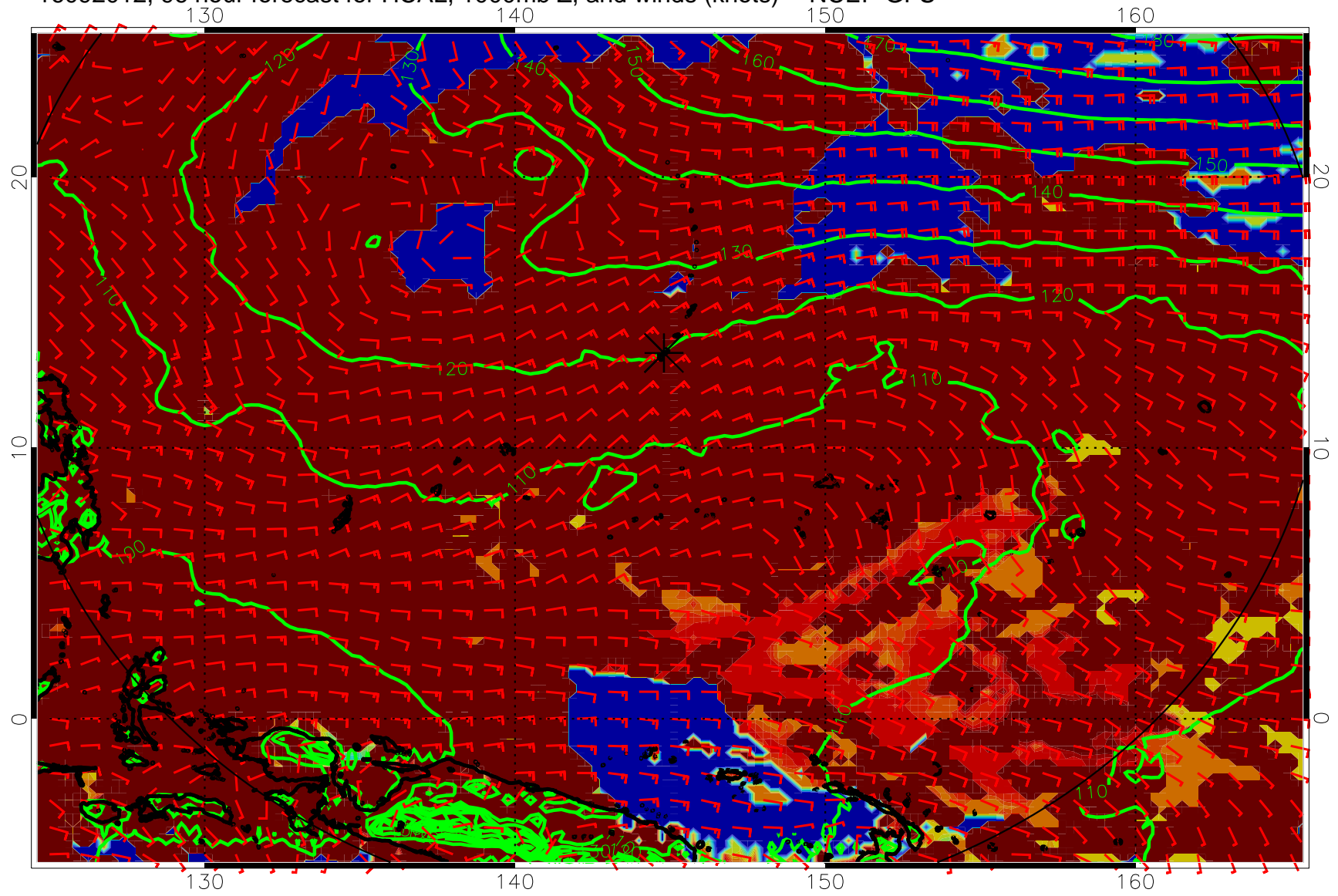
16092012, 96 hour forecast for HCAL, 1000mb Z, and winds (knots) -- NCEP GFS
