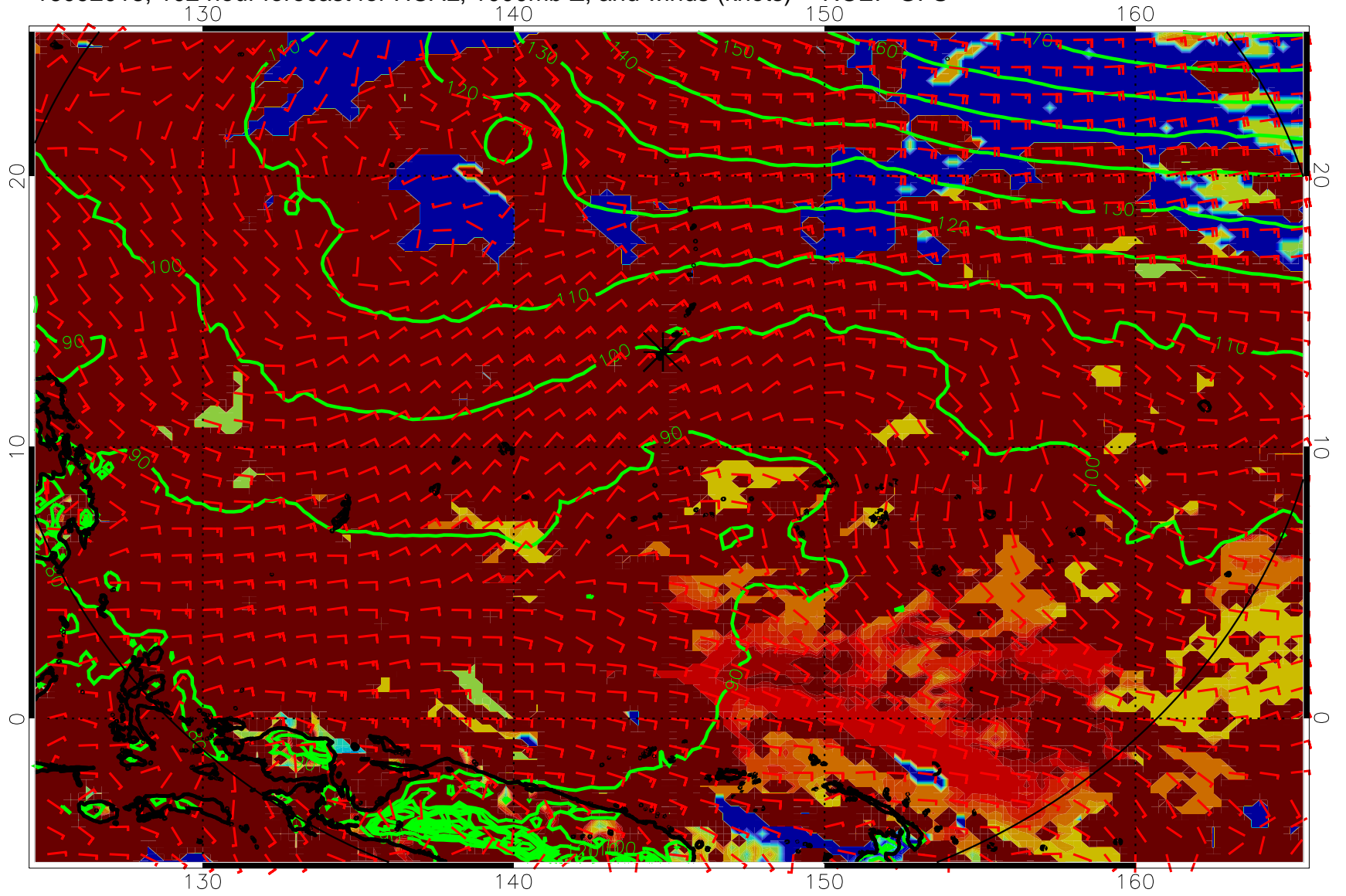
16092018, 102 hour forecast for HCAL, 1000mb Z, and winds (knots) -- NCEP GFS
