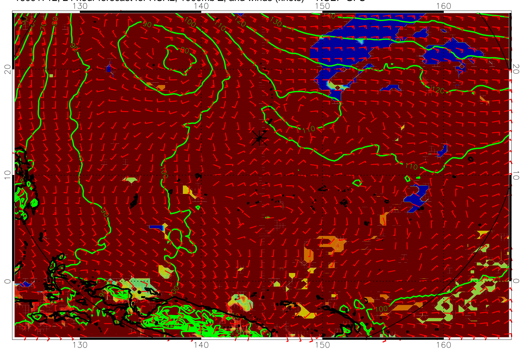
16091712, 24 hour forecast for HCAL, 1000mb Z, and winds (knots) -- NCEP GFS
