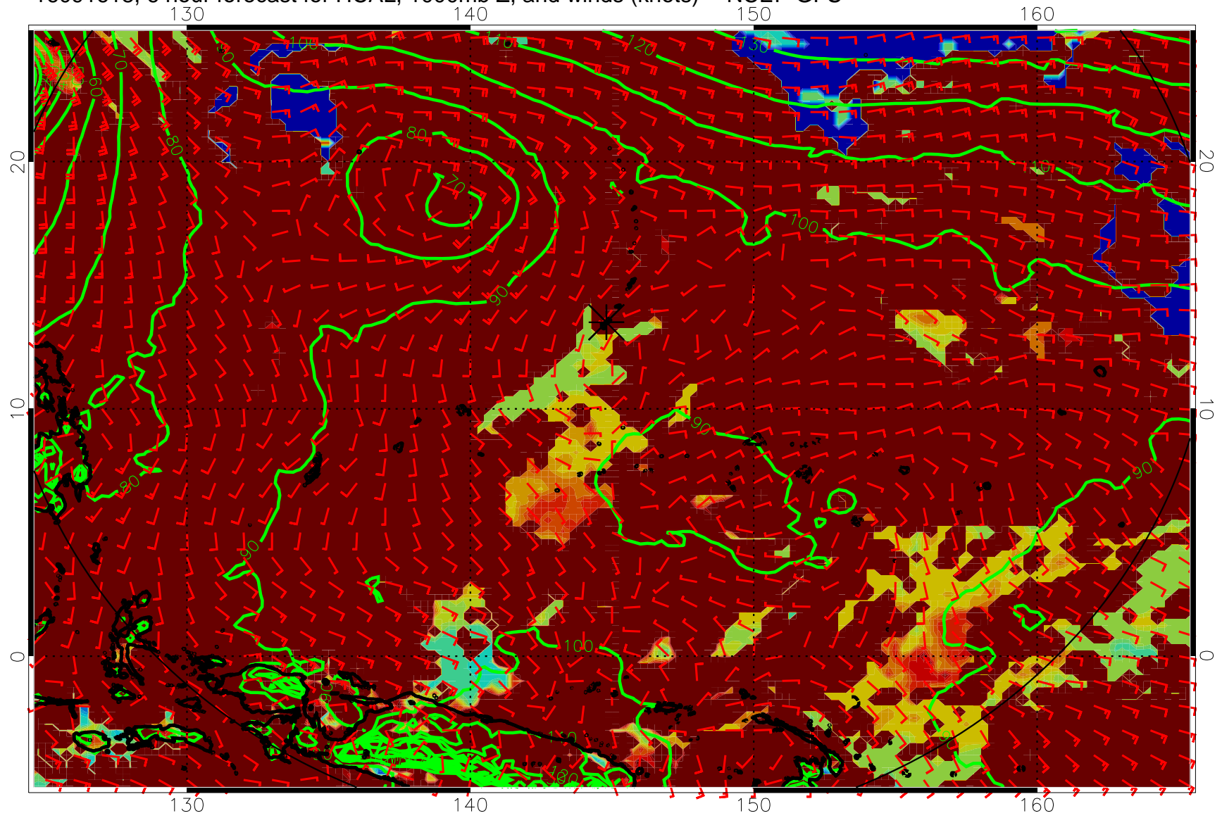
16091618, 6 hour forecast for HCAL, 1000mb Z, and winds (knots) -- NCEP GFS
