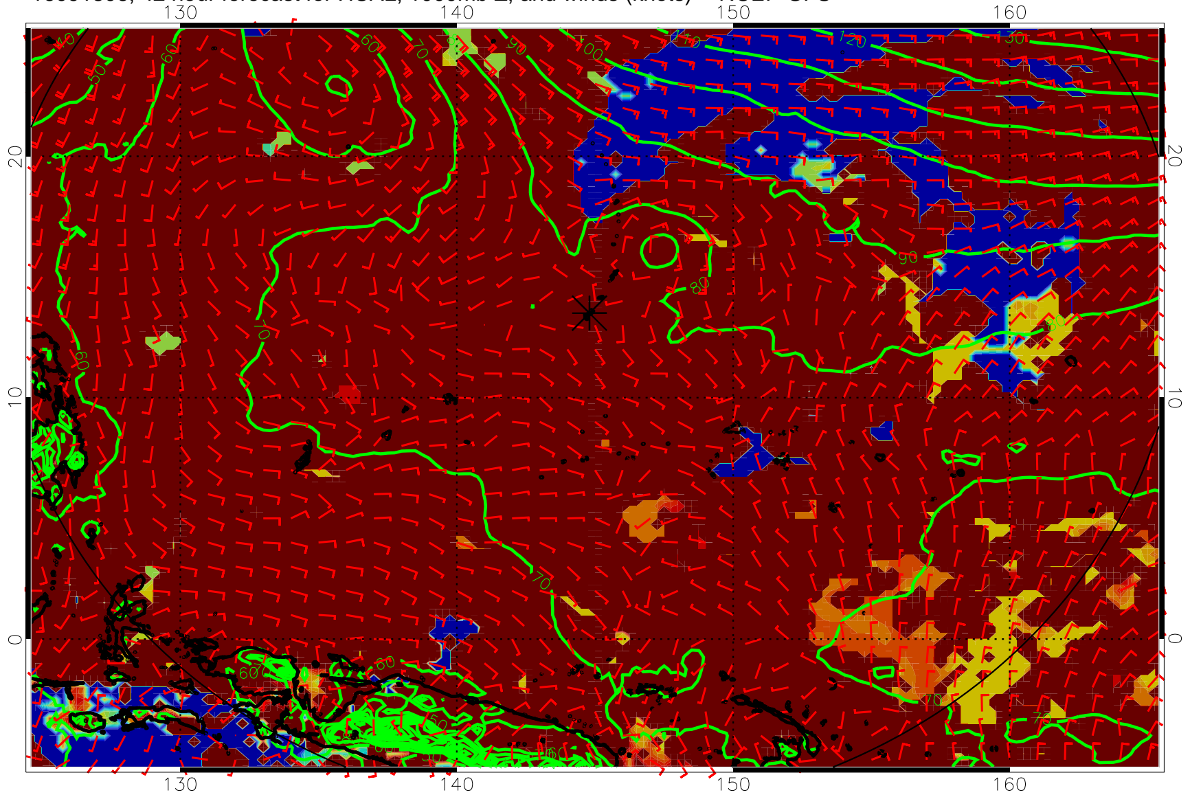
16091806, 42 hour forecast for HCAL, 1000mb Z, and winds (knots) -- NCEP GFS
