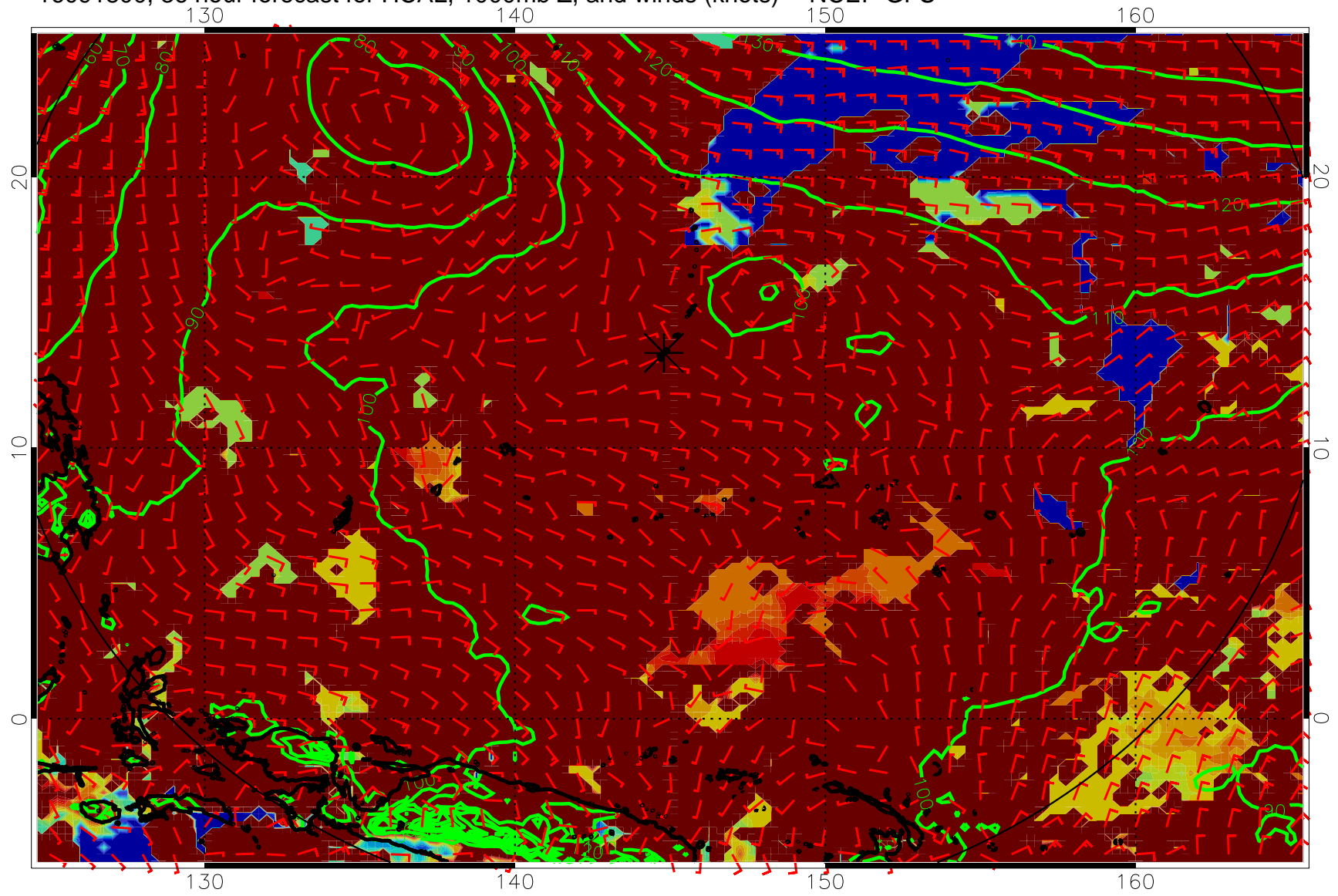
16091800, 36 hour forecast for HCAL, 1000mb Z, and winds (knots) -- NCEP GFS
