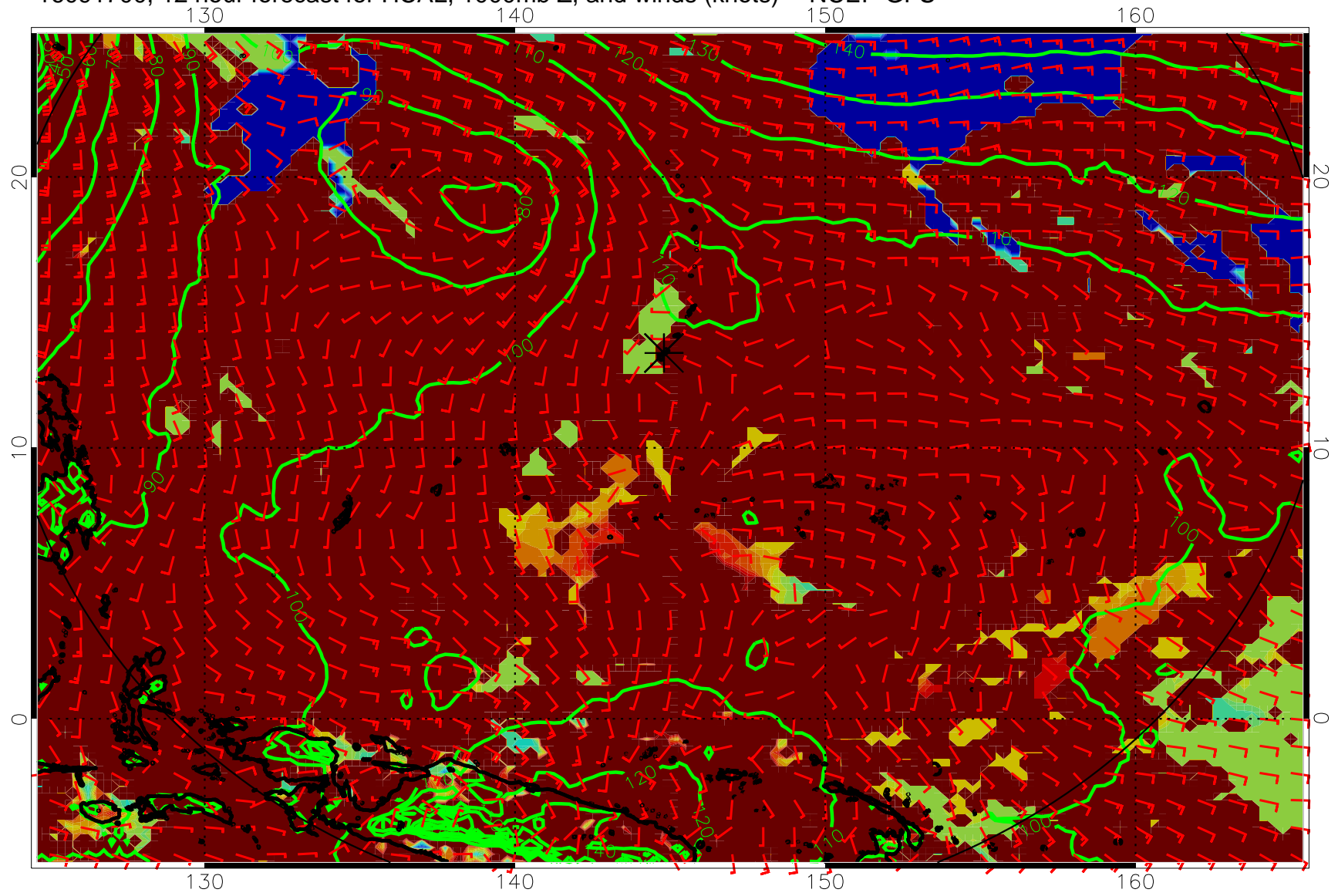
16091700, 12 hour forecast for HCAL, 1000mb Z, and winds (knots) -- NCEP GFS
