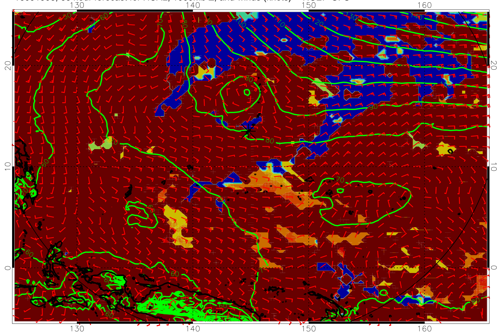
16091906, 66 hour forecast for HCAL, 1000mb Z, and winds (knots) -- NCEP GFS
