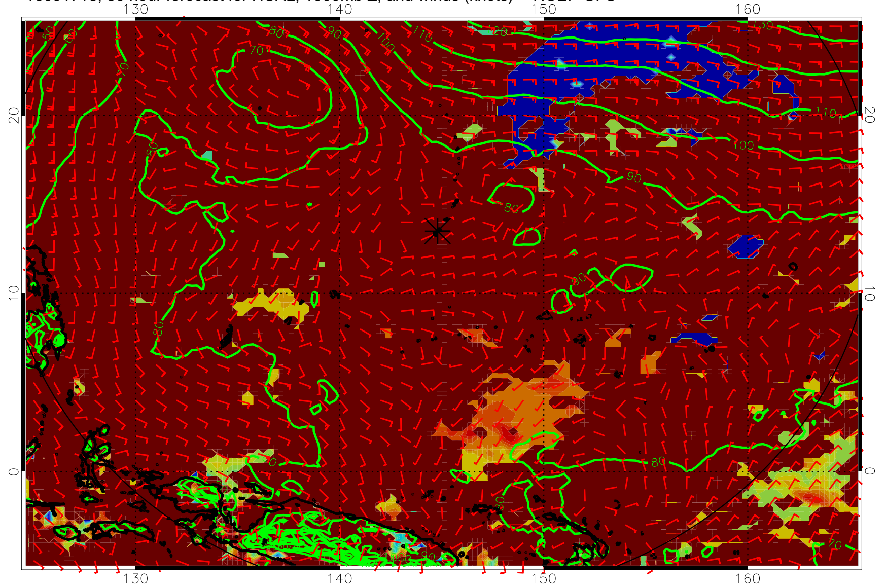
16091718, 30 hour forecast for HCAL, 1000mb Z, and winds (knots) -- NCEP GFS
