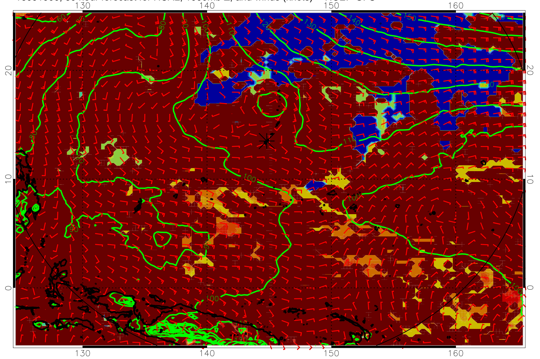
16091900, 60 hour forecast for HCAL, 1000mb Z, and winds (knots) -- NCEP GFS
