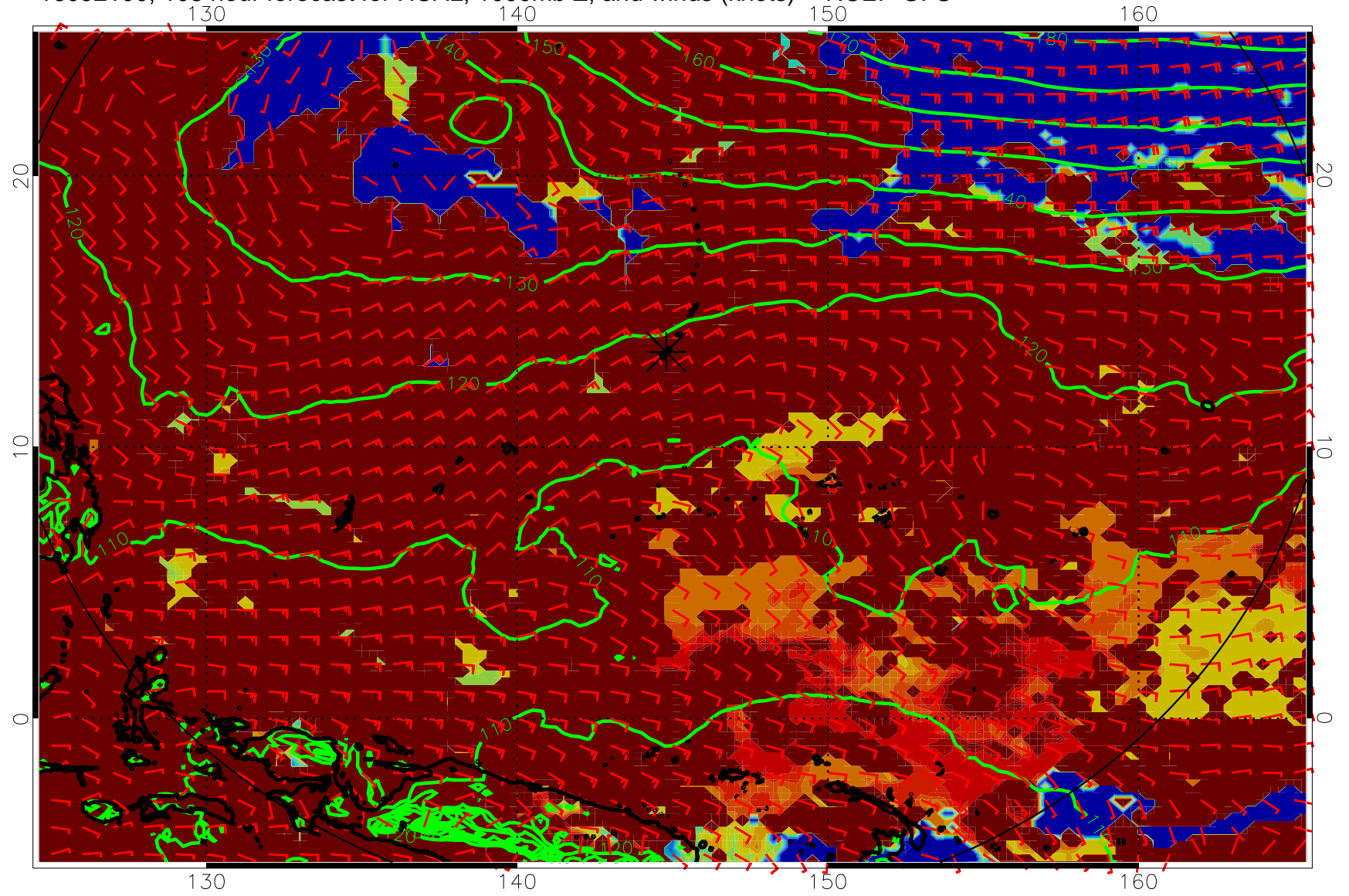
16092100, 108 hour forecast for HCAL, 1000mb Z, and winds (knots) -- NCEP GFS
