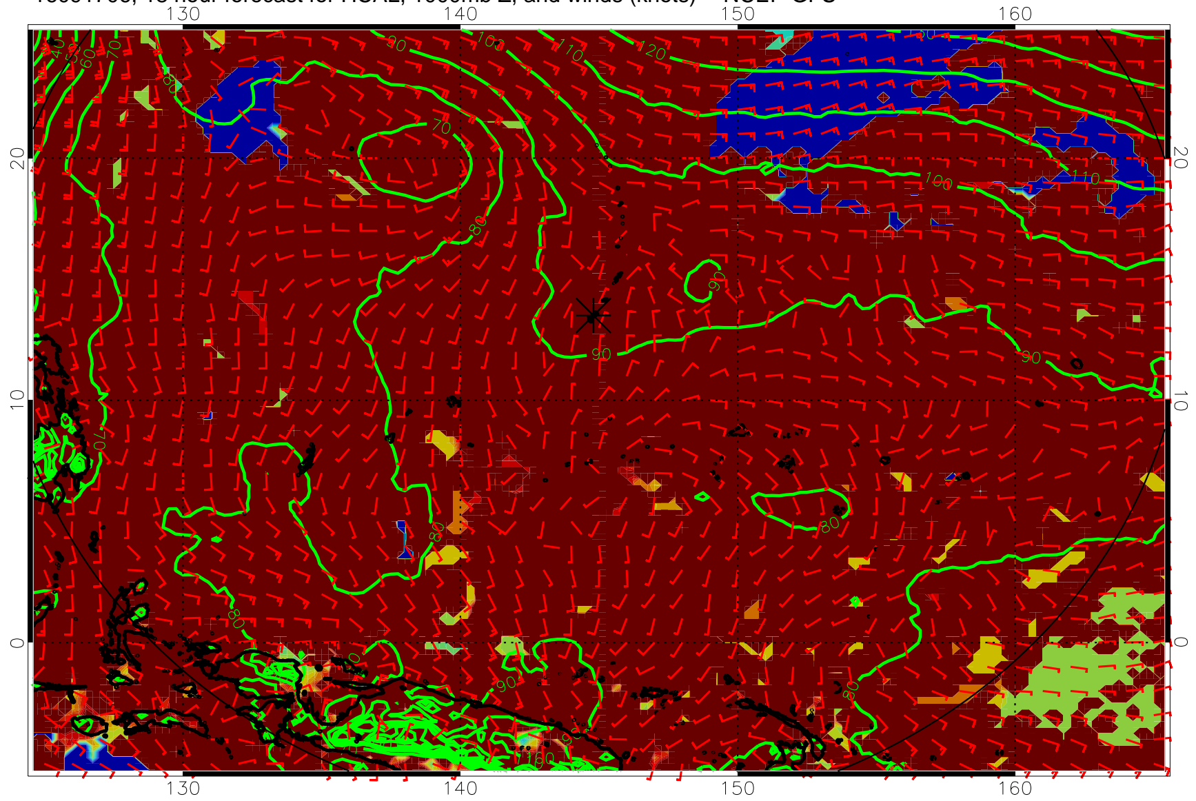
16091706, 18 hour forecast for HCAL, 1000mb Z, and winds (knots) -- NCEP GFS
