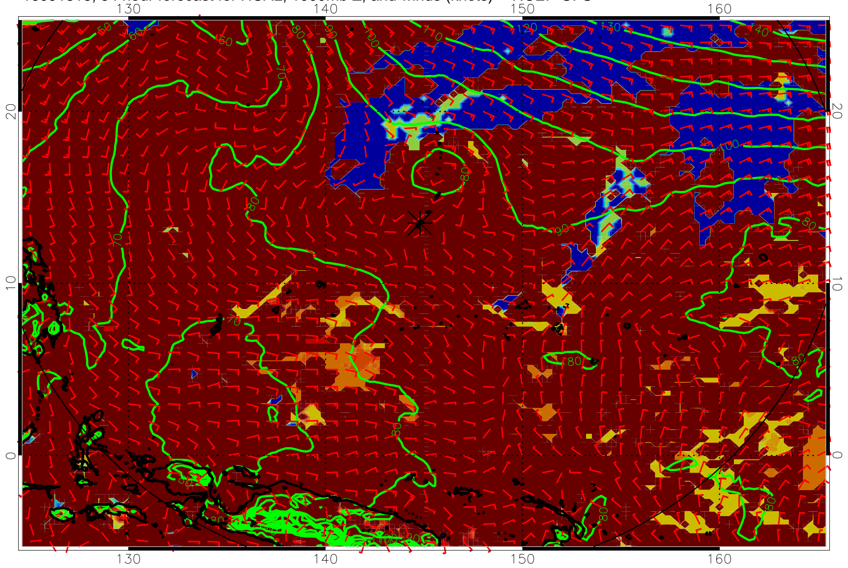
16091818, 54 hour forecast for HCAL, 1000mb Z, and winds (knots) -- NCEP GFS
