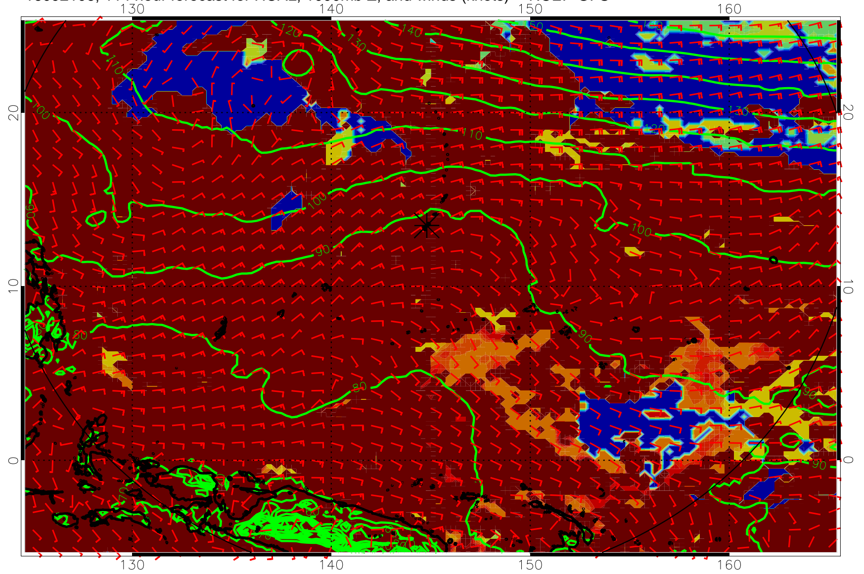
16092106, 114 hour forecast for HCAL, 1000mb Z, and winds (knots) -- NCEP GFS
