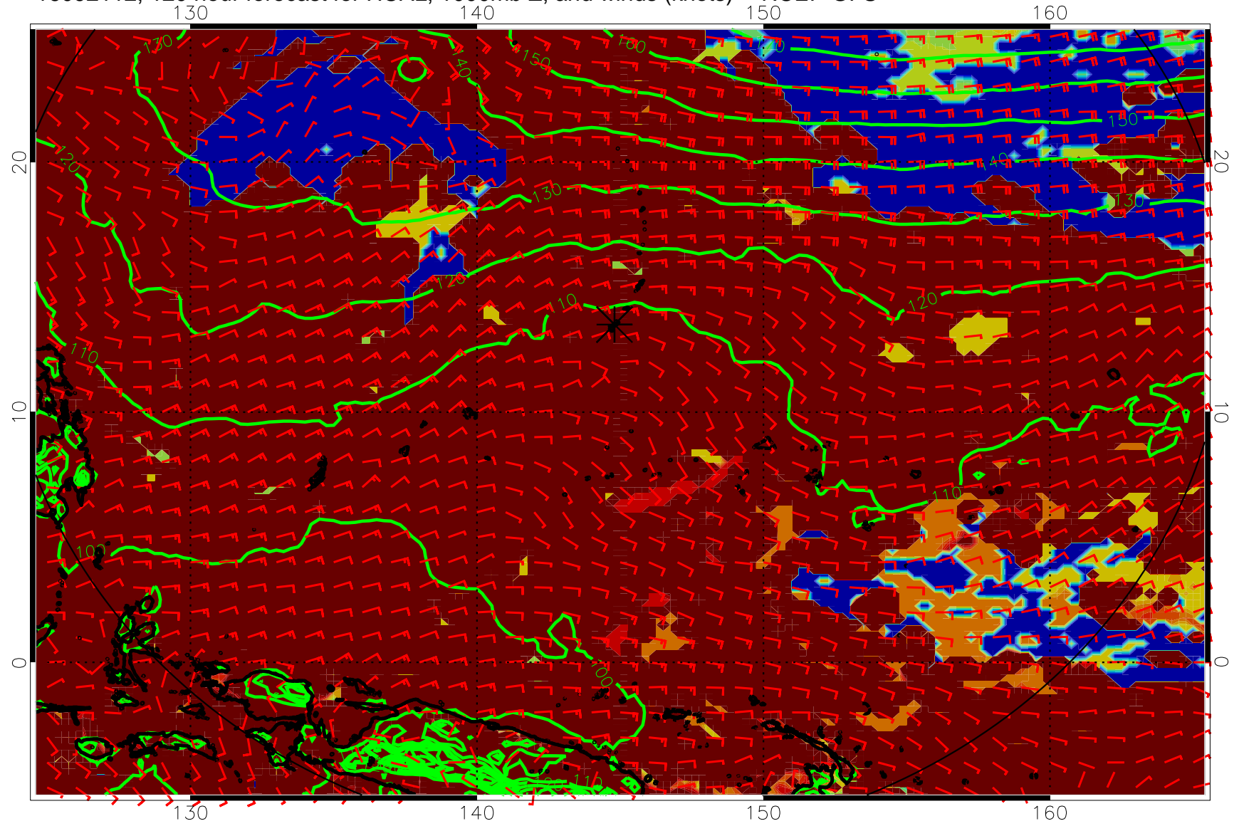
16092112, 120 hour forecast for HCAL, 1000mb Z, and winds (knots) -- NCEP GFS
