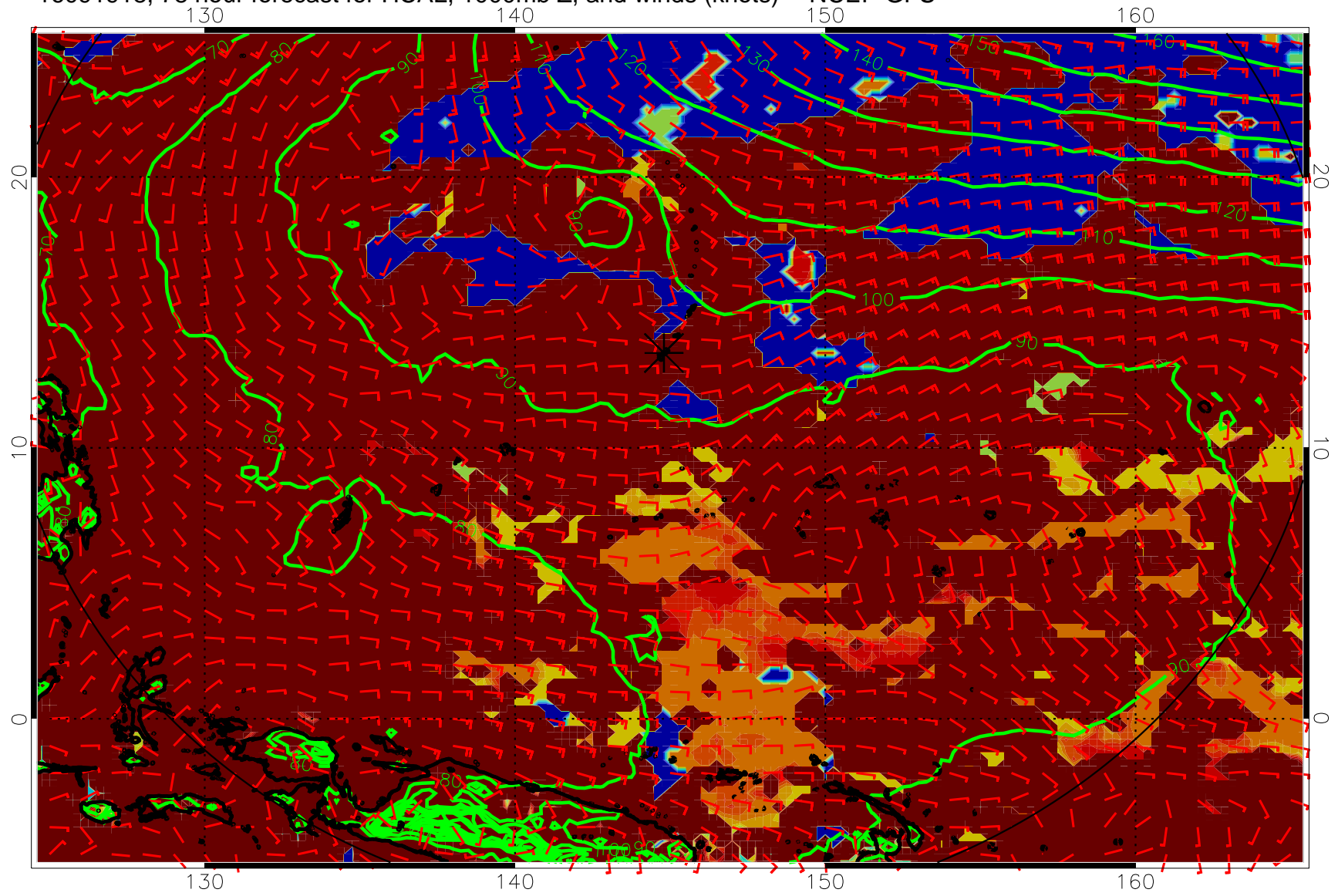
16091918, 78 hour forecast for HCAL, 1000mb Z, and winds (knots) -- NCEP GFS
