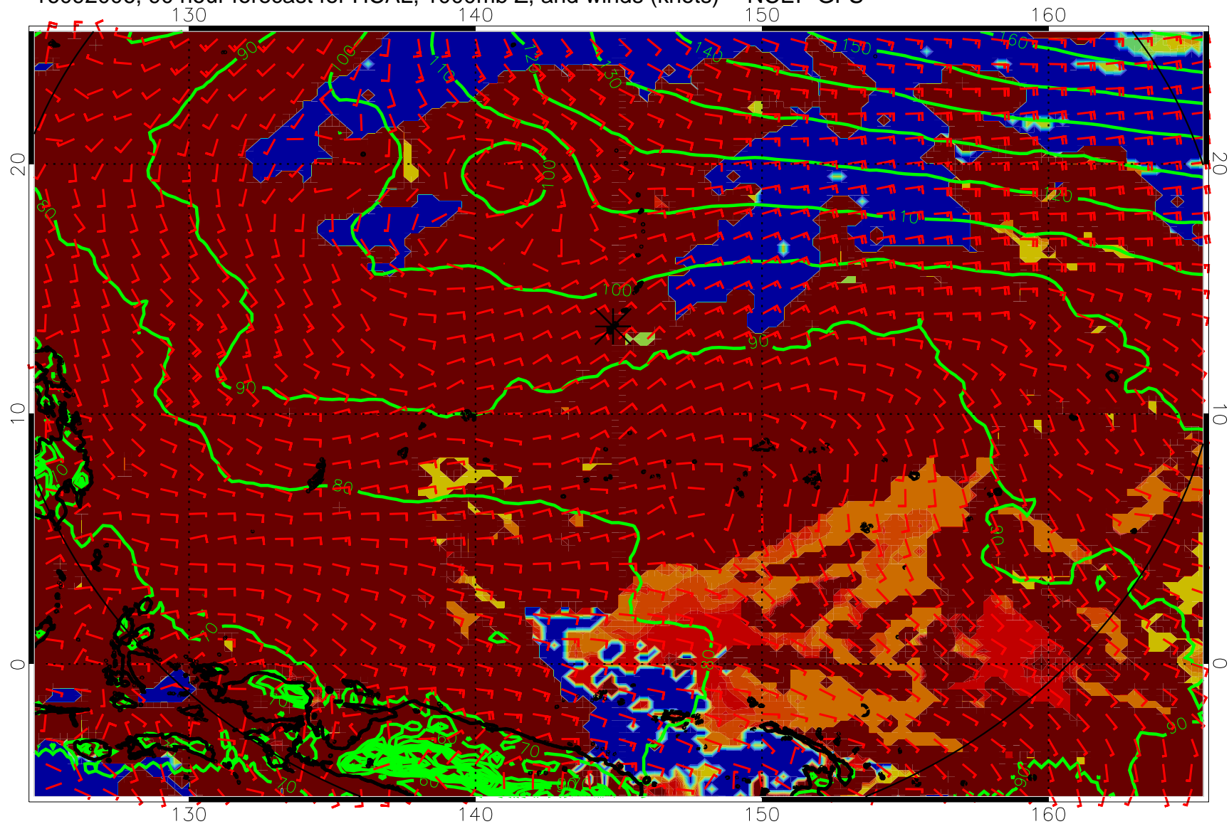
16092006, 90 hour forecast for HCAL, 1000mb Z, and winds (knots) -- NCEP GFS
