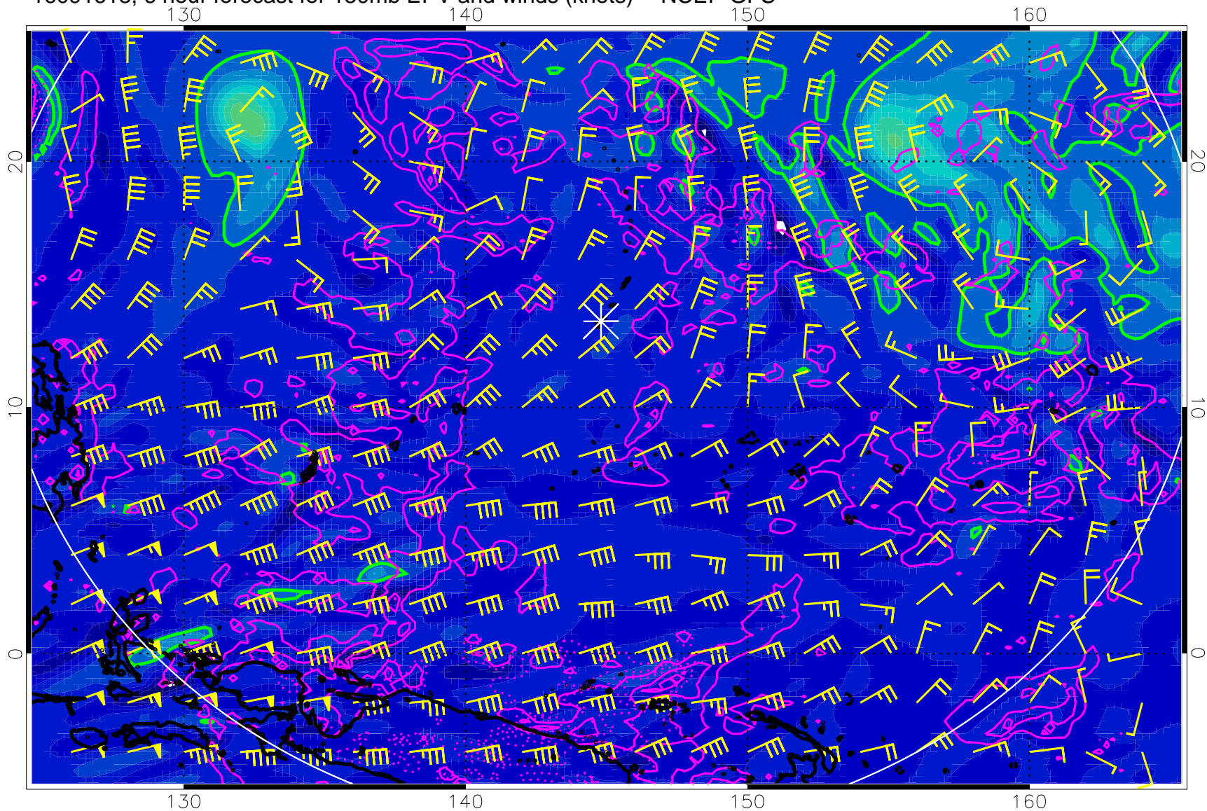
16091618, 6 hour forecast for 150mb EPV and winds (knots) -- NCEP GFS
