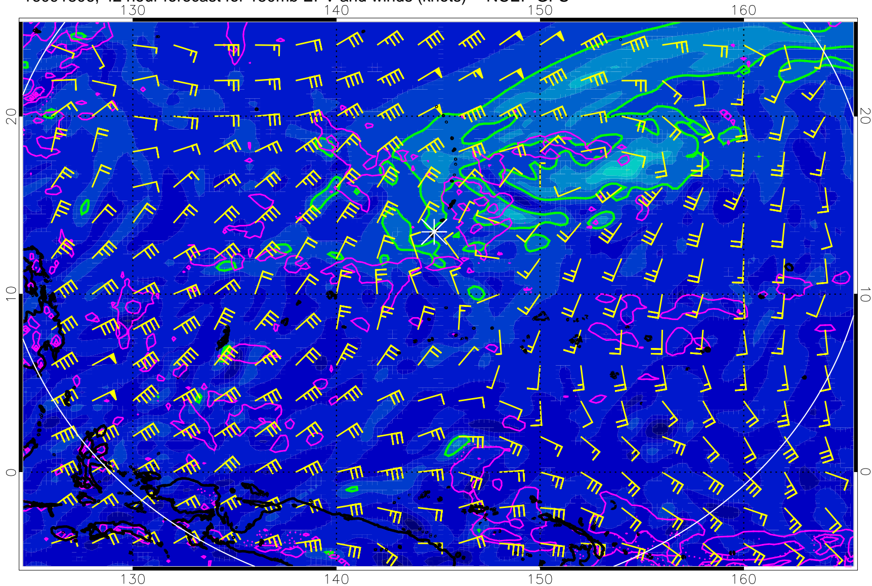
16091806, 42 hour forecast for 150mb EPV and winds (knots) -- NCEP GFS
