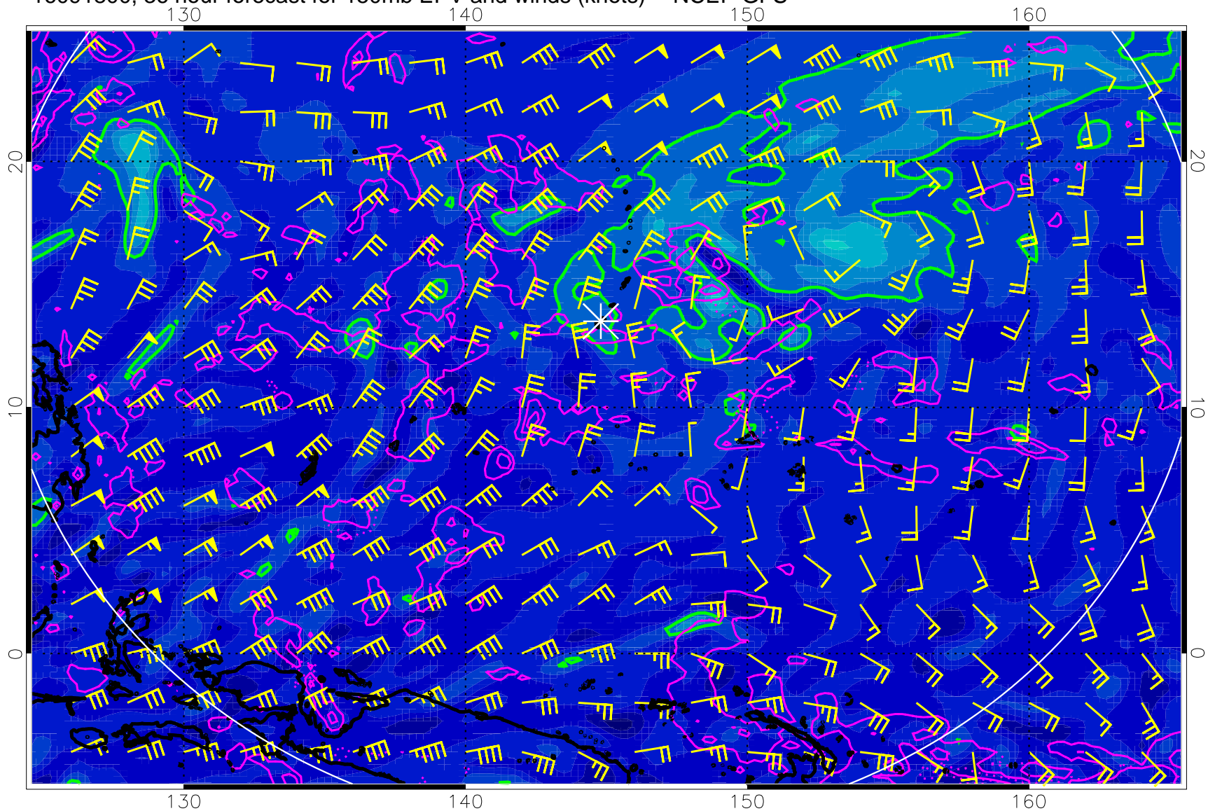
16091800, 36 hour forecast for 150mb EPV and winds (knots) -- NCEP GFS
