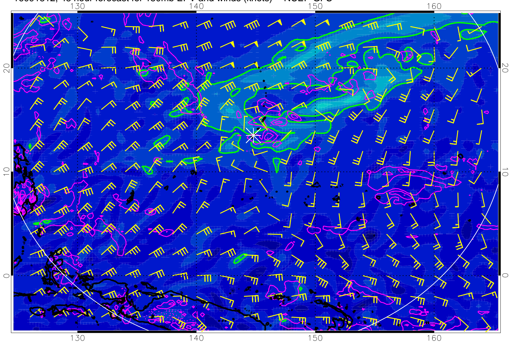
16091812, 48 hour forecast for 150mb EPV and winds (knots) -- NCEP GFS
