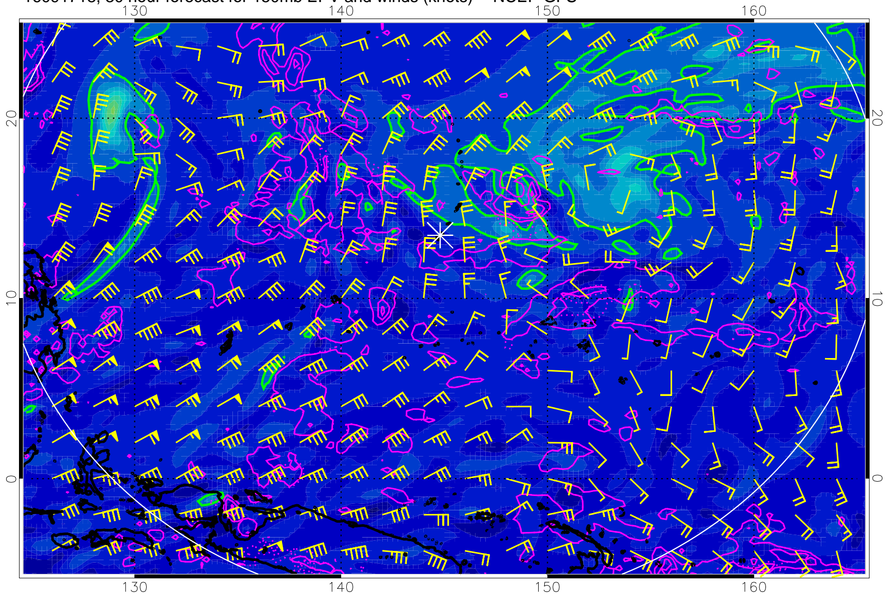
16091718, 30 hour forecast for 150mb EPV and winds (knots) -- NCEP GFS
