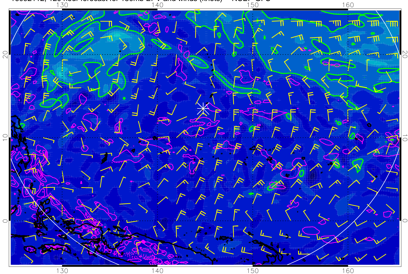
16092112, 120 hour forecast for 150mb EPV and winds (knots) -- NCEP GFS
