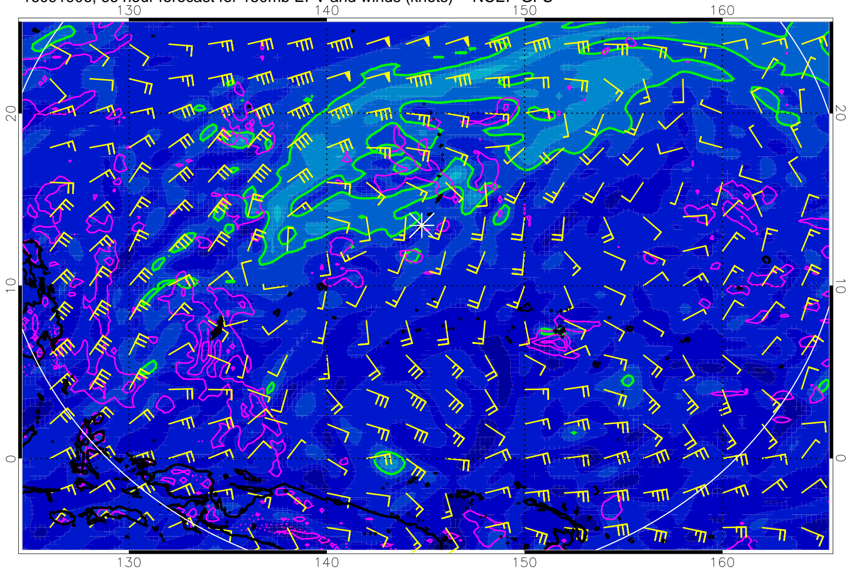
16091906, 66 hour forecast for 150mb EPV and winds (knots) -- NCEP GFS
