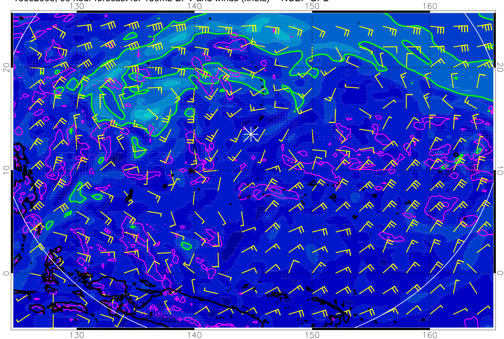
16092006, 90 hour forecast for 150mb EPV and winds (knots) -- NCEP GFS
