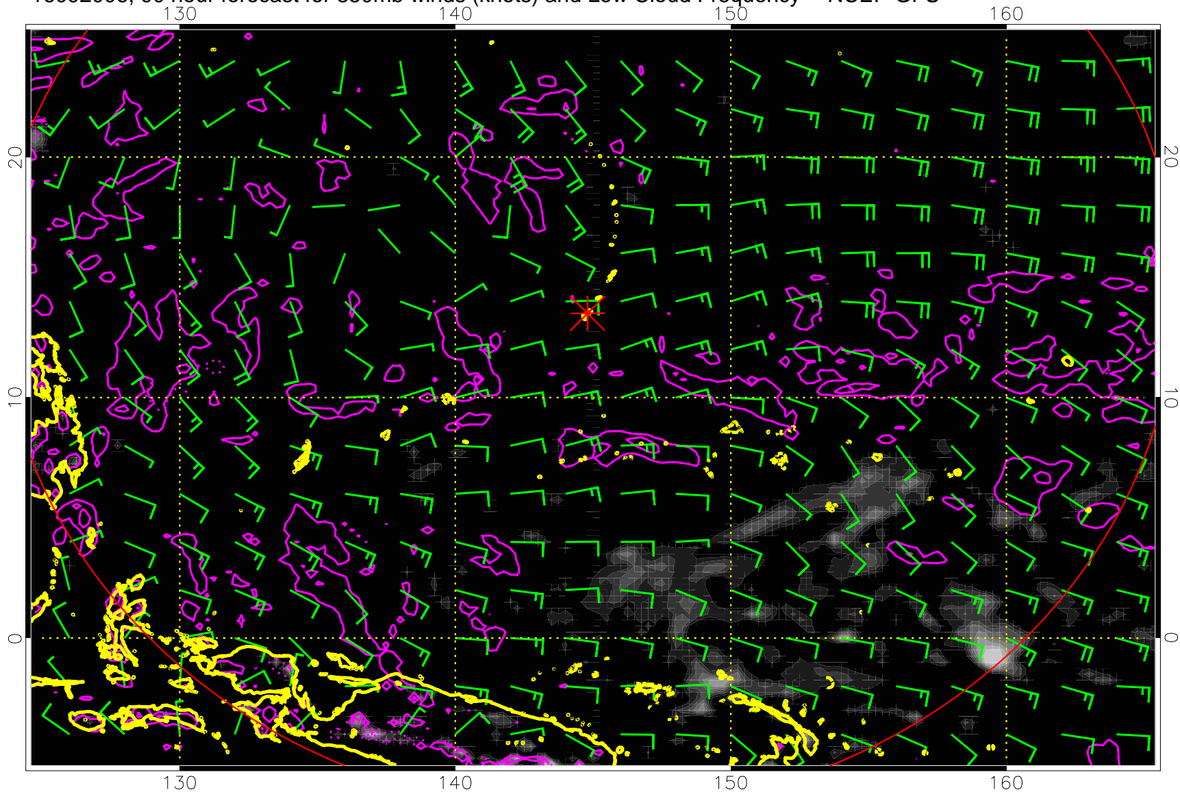
16092006, 90 hour forecast for 850mb winds (knots) and Low Cloud Frequency -- NCEP GFS
