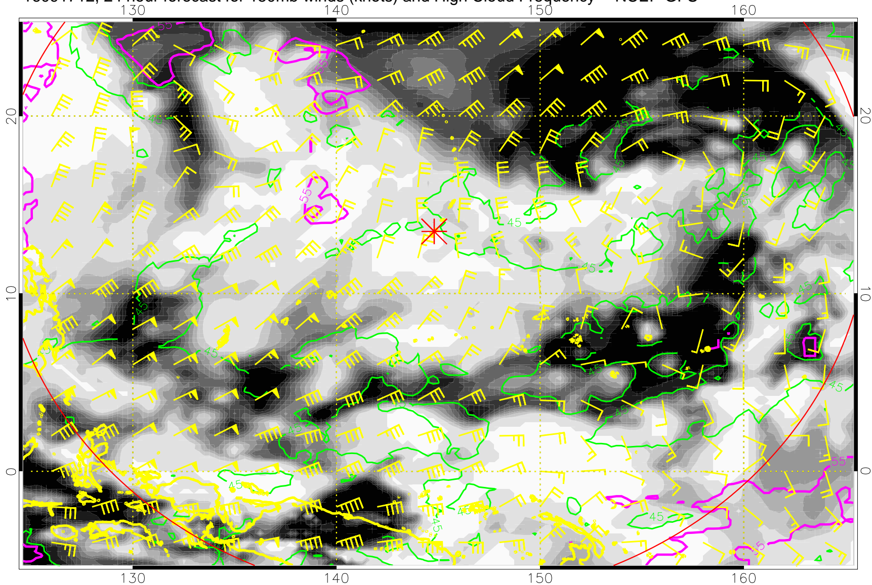
16091712, 24 hour forecast for 150mb winds (knots) and High Cloud Frequency -- NCEP GFS
