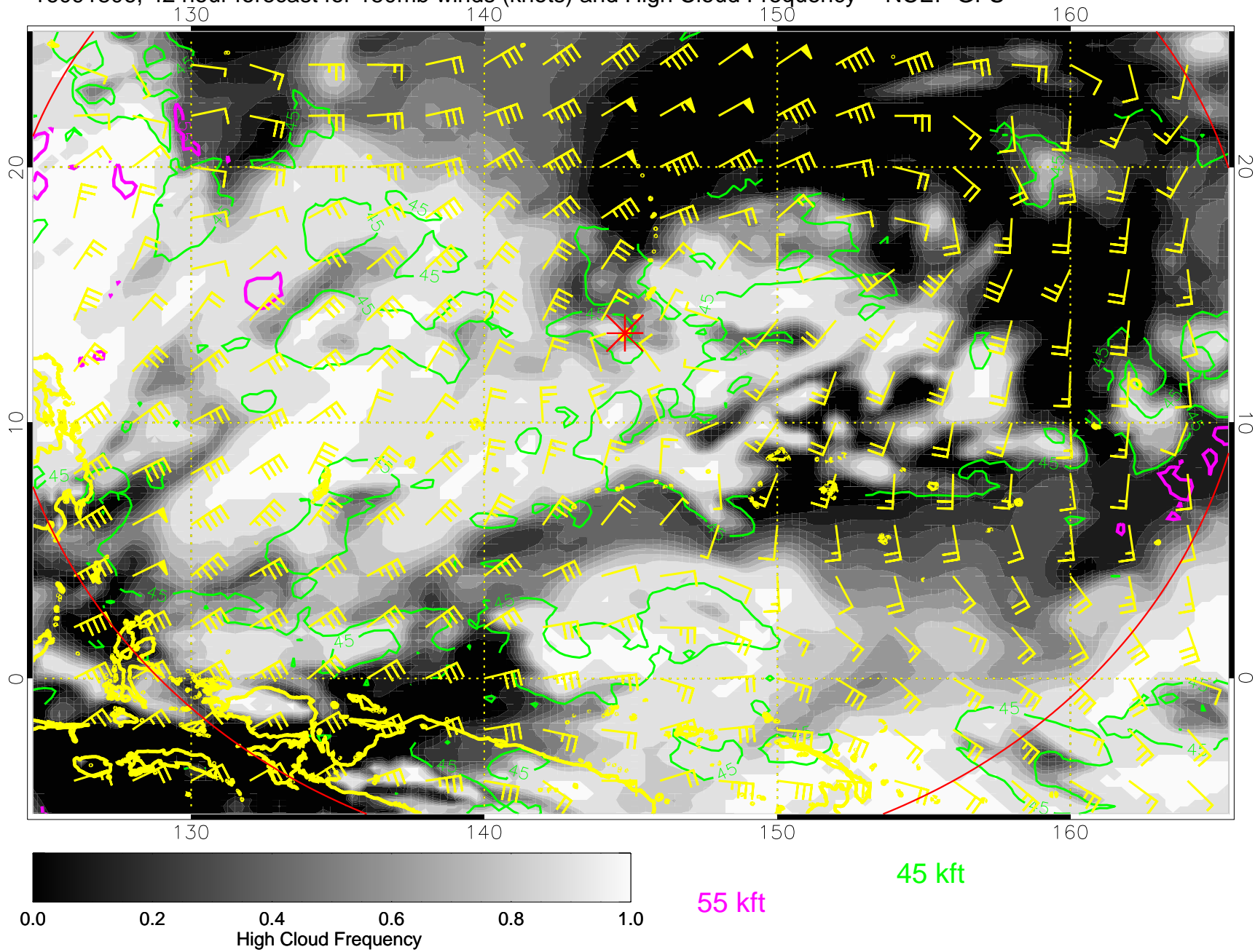
16091806, 42 hour forecast for 150mb winds (knots) and High Cloud Frequency -- NCEP GFS
