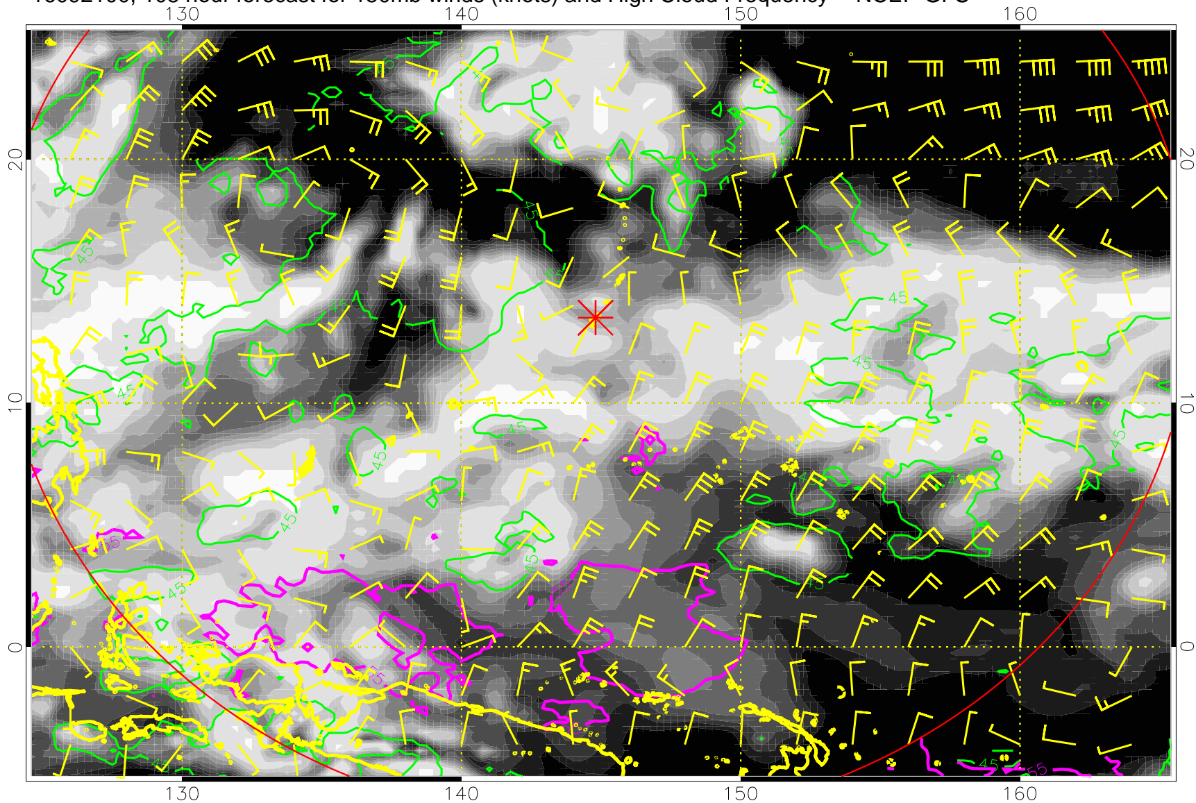
16092100, 108 hour forecast for 150mb winds (knots) and High Cloud Frequency -- NCEP GFS
