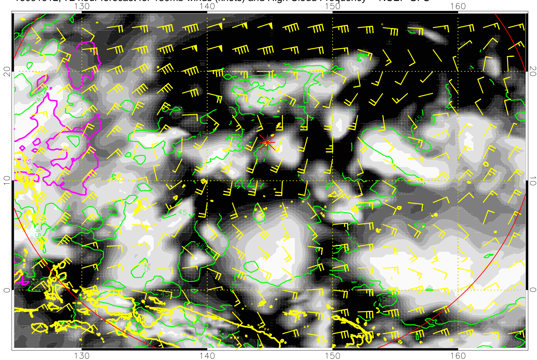
16091912, 72 hour forecast for 150mb winds (knots) and High Cloud Frequency -- NCEP GFS
