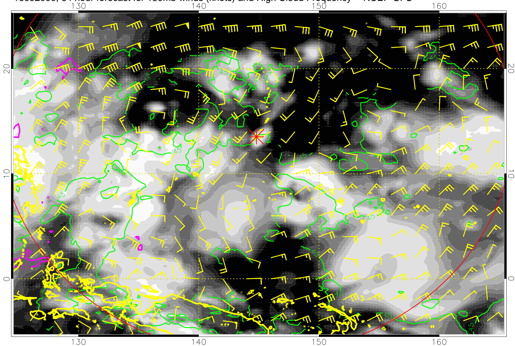
16092000, 84 hour forecast for 150mb winds (knots) and High Cloud Frequency -- NCEP GFS
