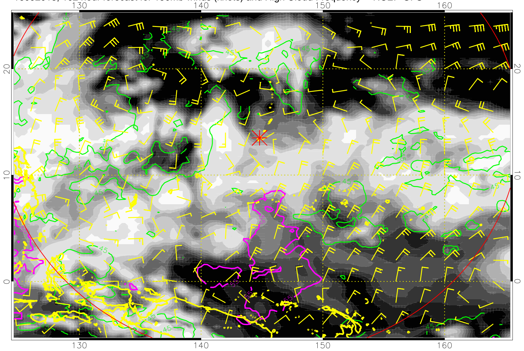
16092018, 102 hour forecast for 150mb winds (knots) and High Cloud Frequency -- NCEP GFS
