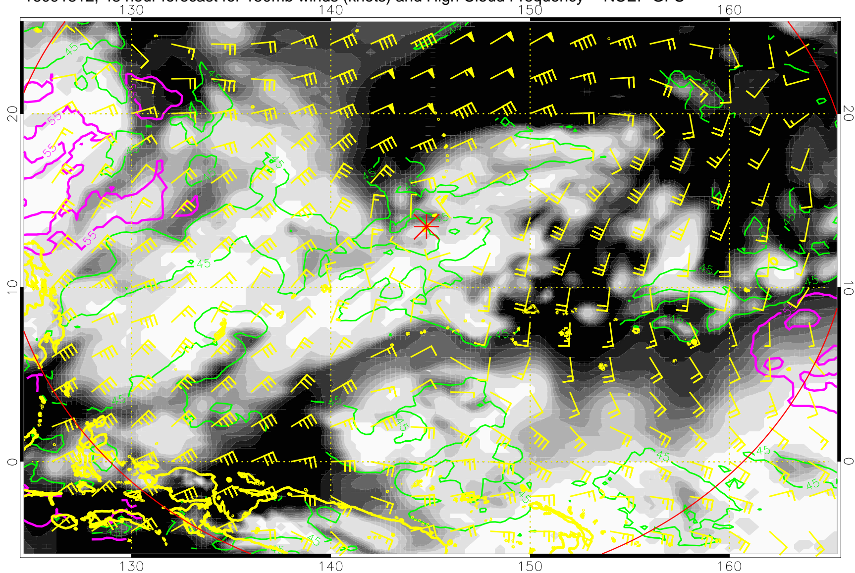
16091812, 48 hour forecast for 150mb winds (knots) and High Cloud Frequency -- NCEP GFS
