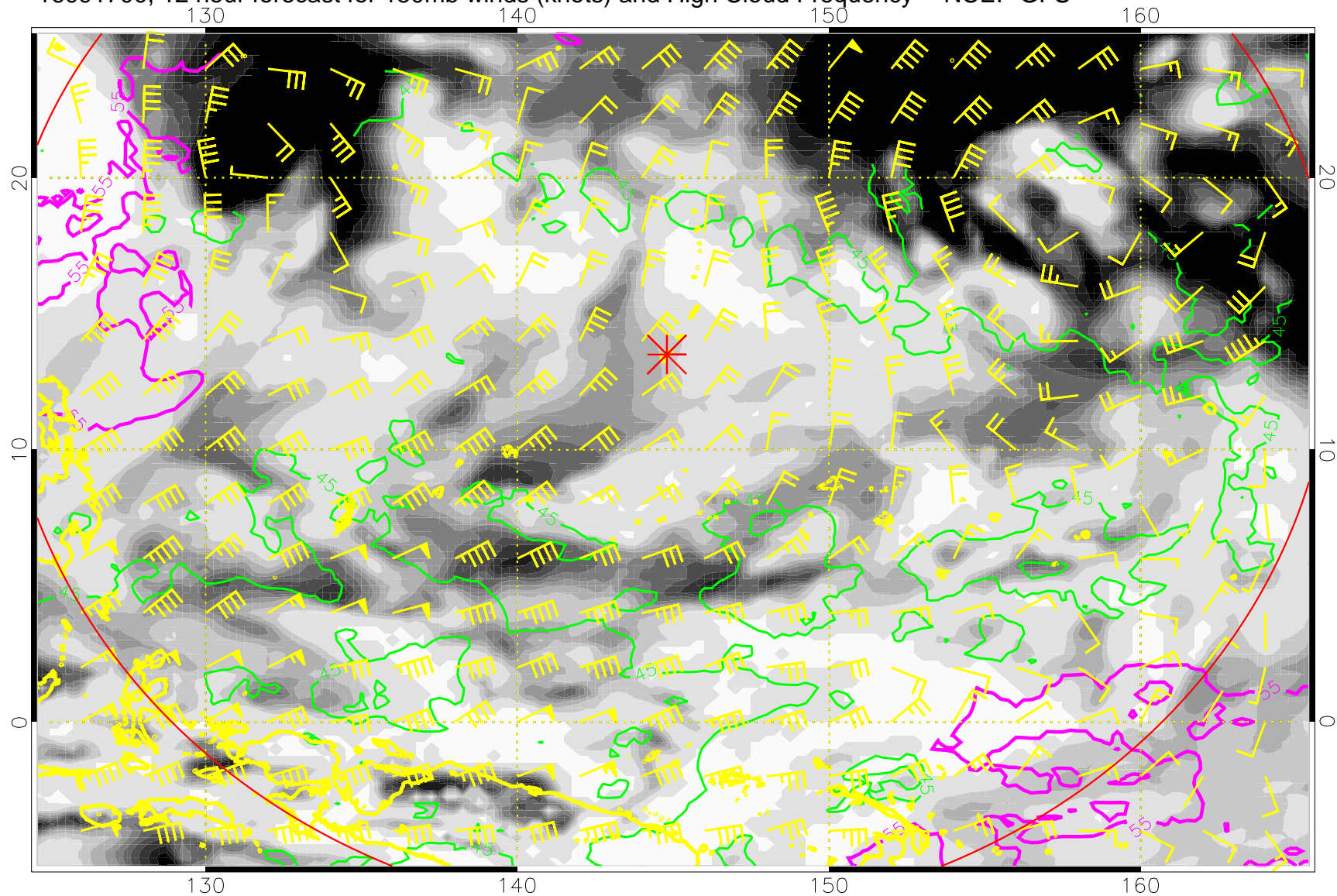
16091700, 12 hour forecast for 150mb winds (knots) and High Cloud Frequency -- NCEP GFS
