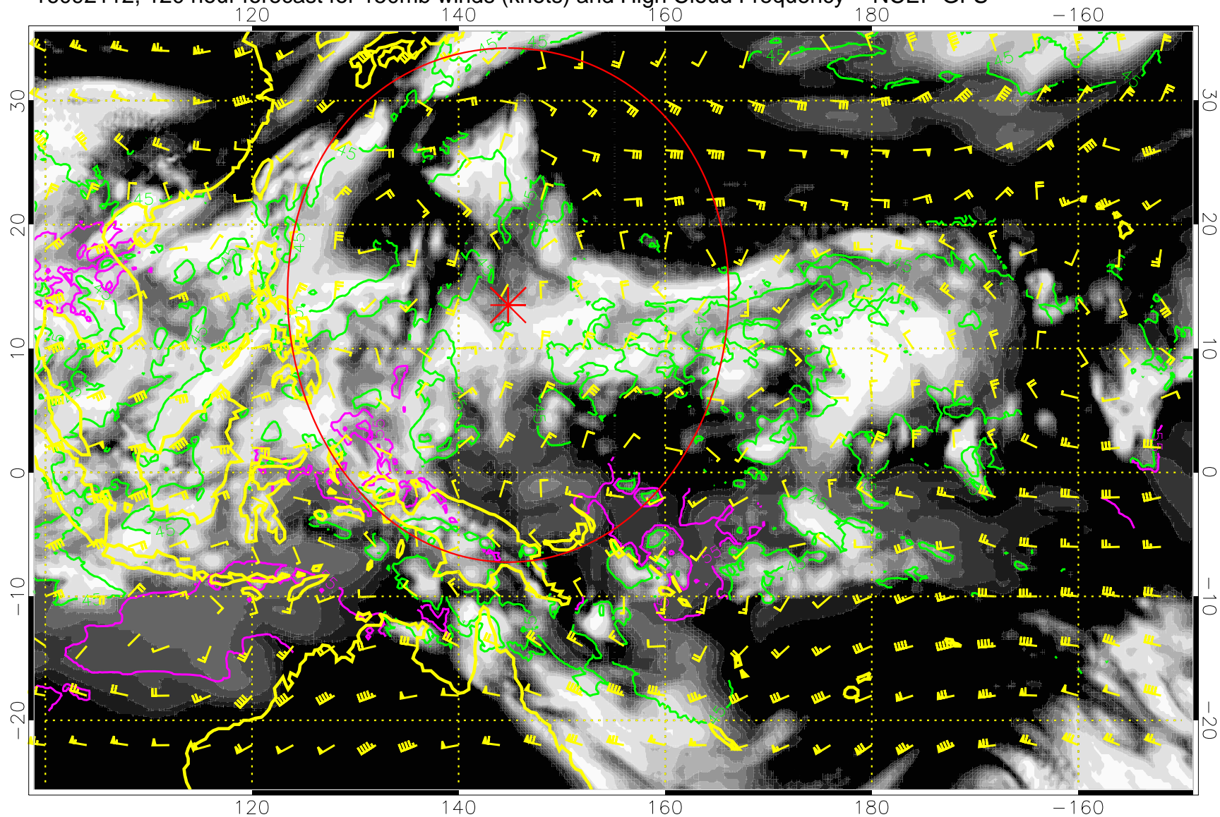
16092112, 120 hour forecast for 150mb winds (knots) and High Cloud Frequency -- NCEP GFS
