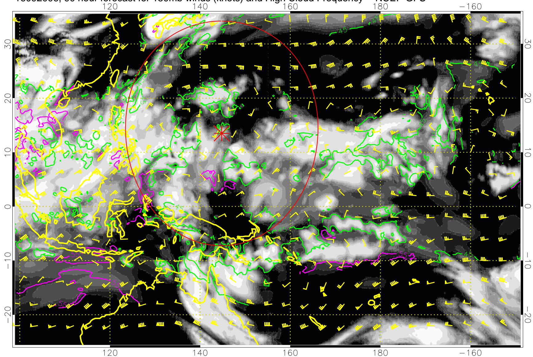
16092006, 90 hour forecast for 150mb winds (knots) and High Cloud Frequency -- NCEP GFS
