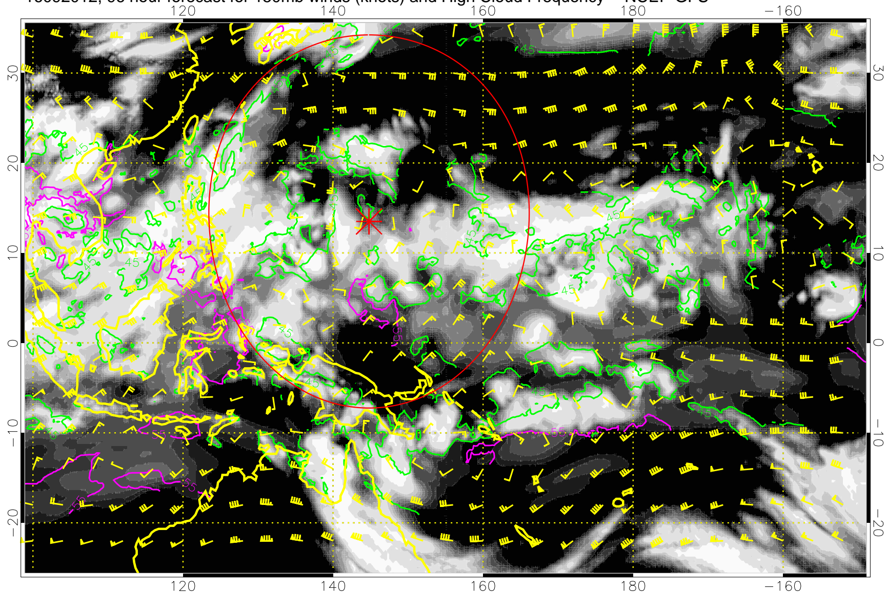
16092012, 96 hour forecast for 150mb winds (knots) and High Cloud Frequency -- NCEP GFS
