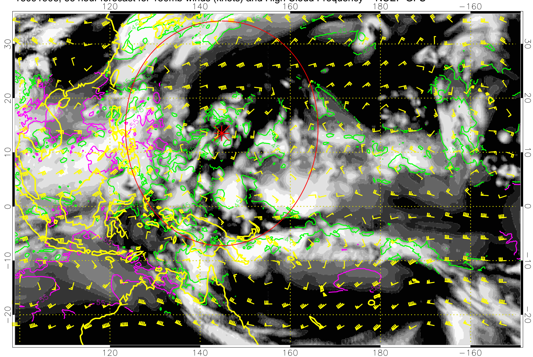
16091906, 66 hour forecast for 150mb winds (knots) and High Cloud Frequency -- NCEP GFS
