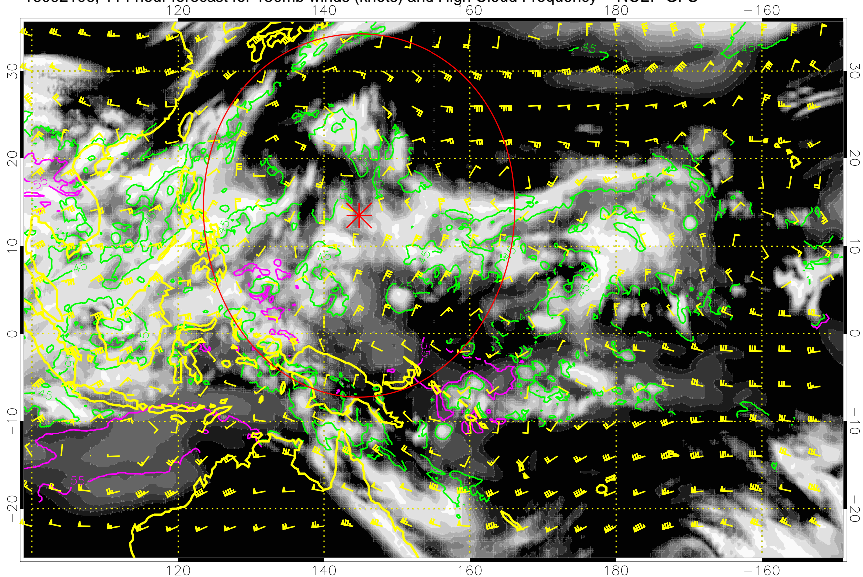
16092106, 114 hour forecast for 150mb winds (knots) and High Cloud Frequency -- NCEP GFS
