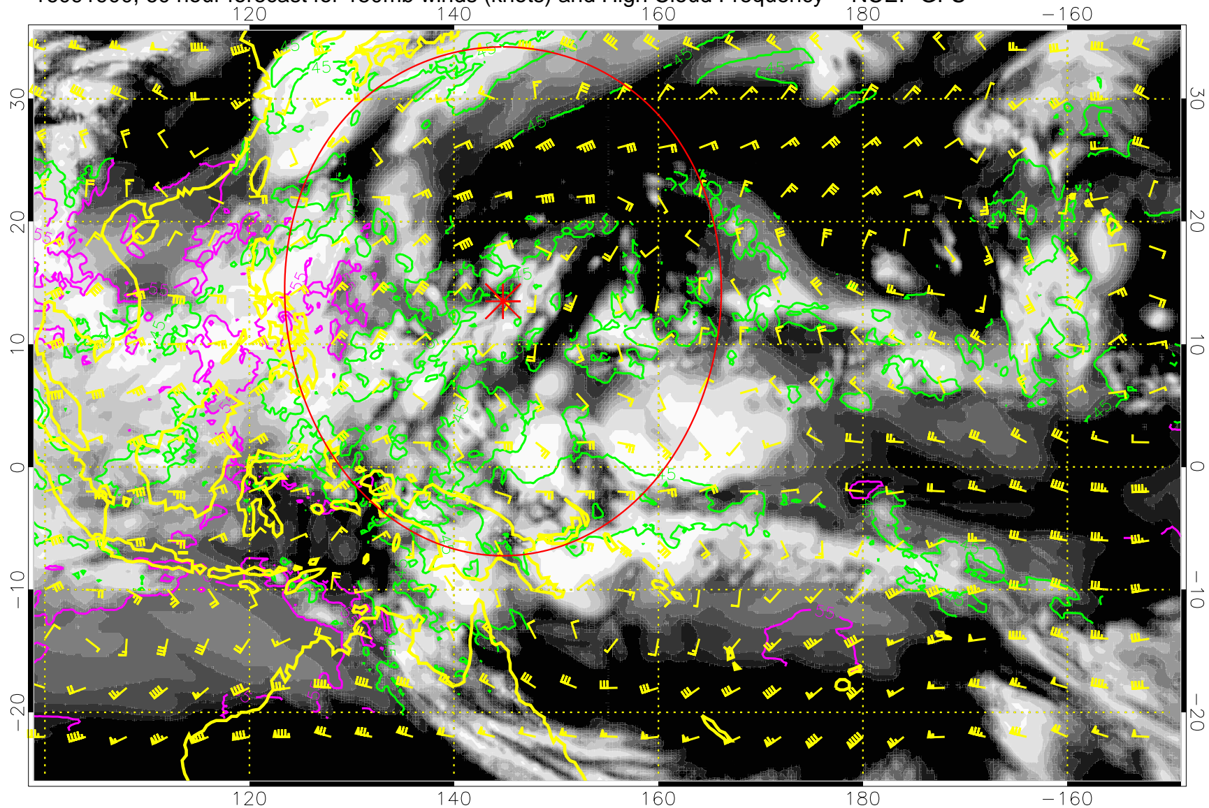
16091900, 60 hour forecast for 150mb winds (knots) and High Cloud Frequency -- NCEP GFS
