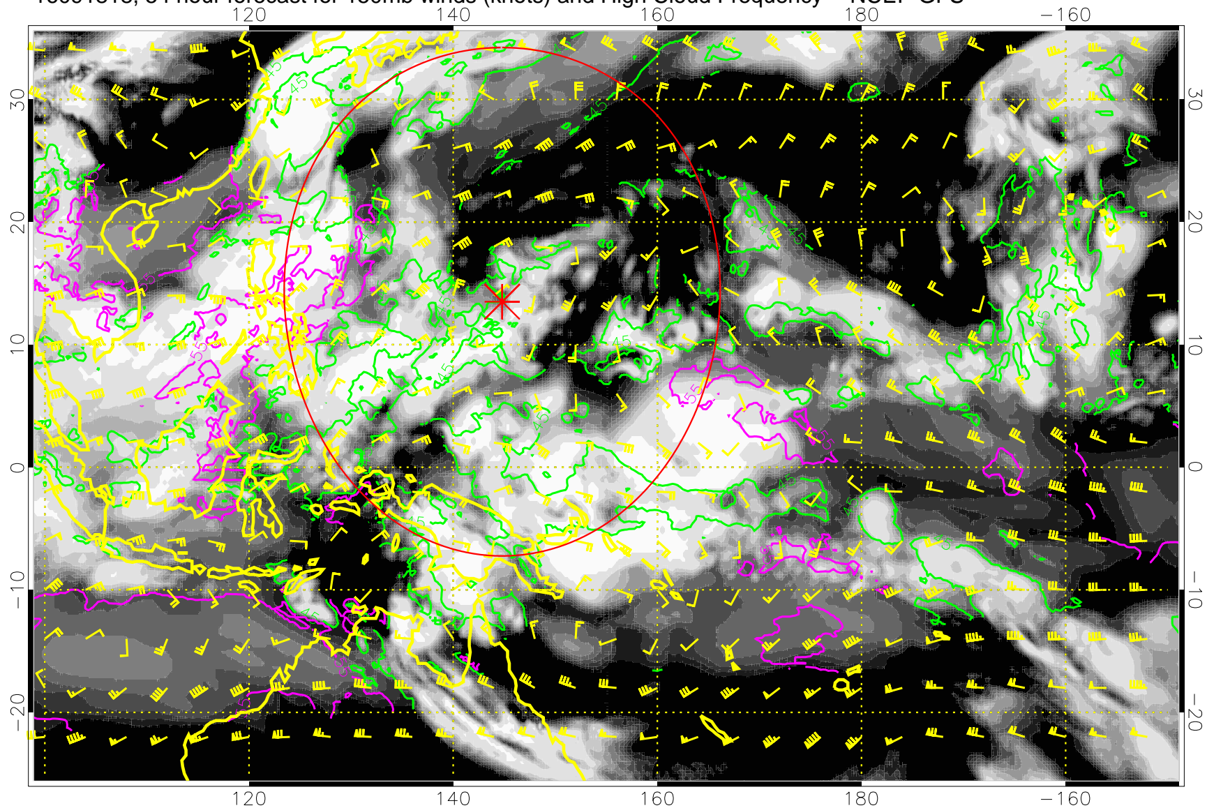
16091818, 54 hour forecast for 150mb winds (knots) and High Cloud Frequency -- NCEP GFS
