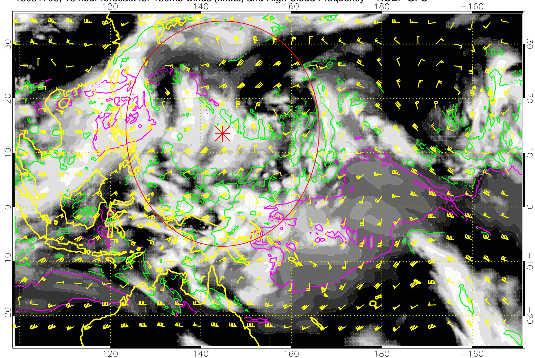
16091706, 18 hour forecast for 150mb winds (knots) and High Cloud Frequency -- NCEP GFS
