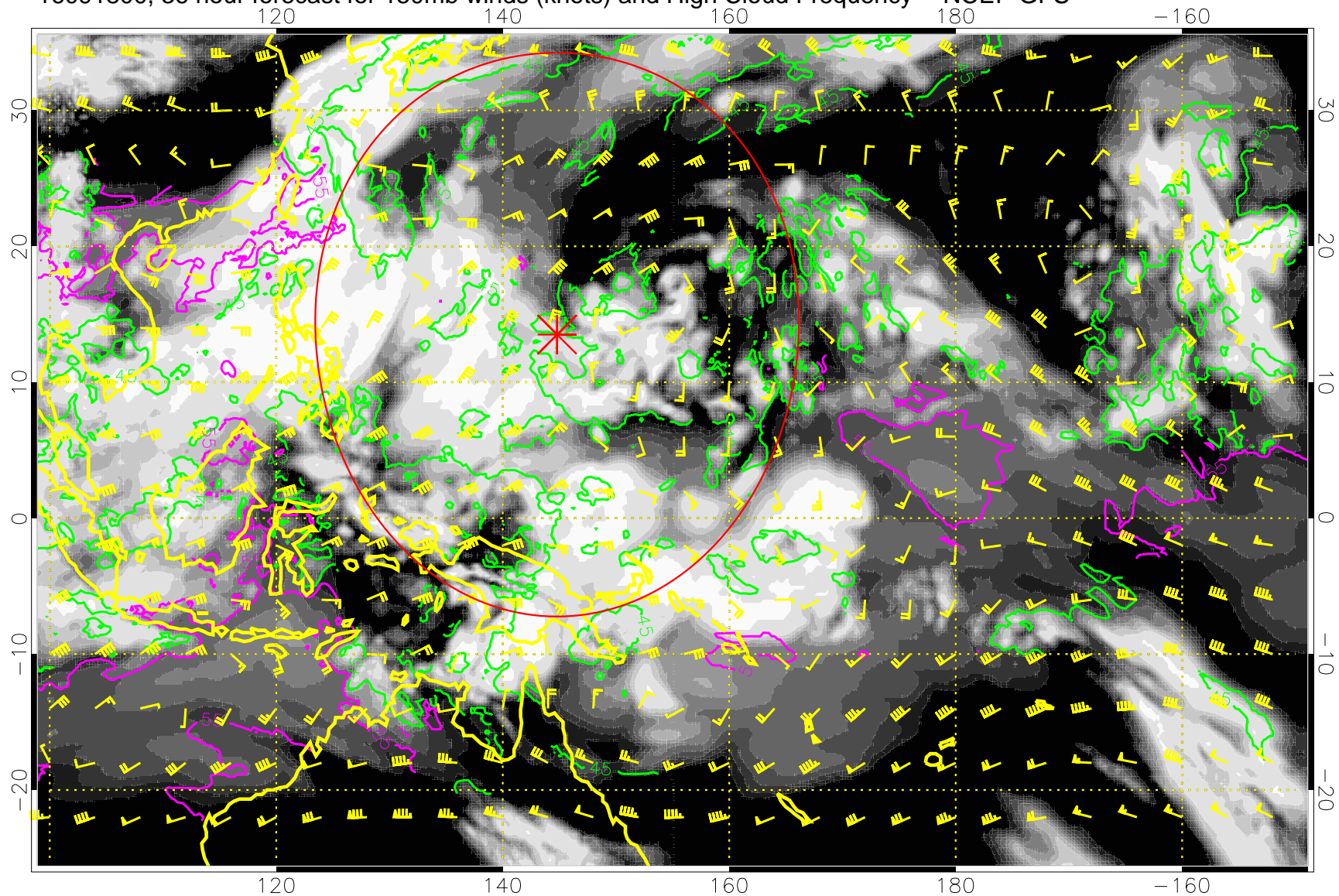
16091800, 36 hour forecast for 150mb winds (knots) and High Cloud Frequency -- NCEP GFS
