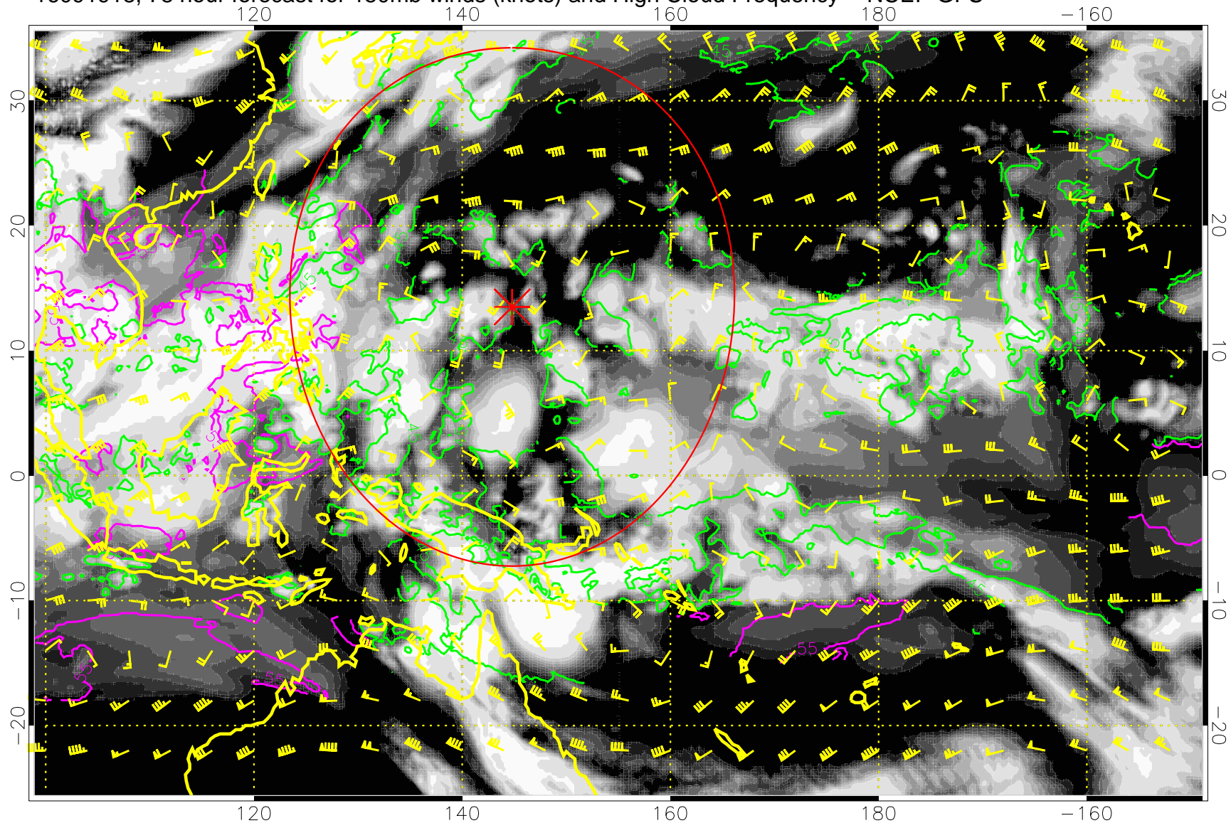
16091918, 78 hour forecast for 150mb winds (knots) and High Cloud Frequency -- NCEP GFS
