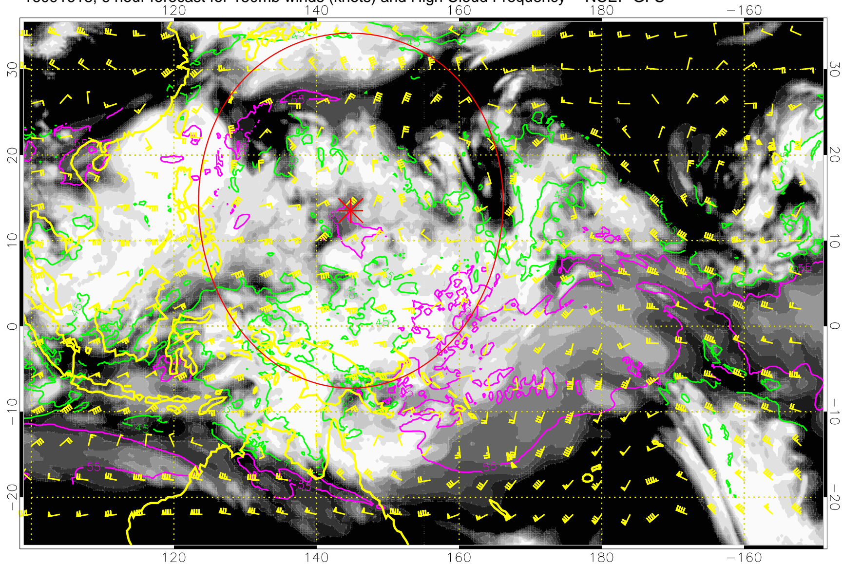
16091618, 6 hour forecast for 150mb winds (knots) and High Cloud Frequency -- NCEP GFS
