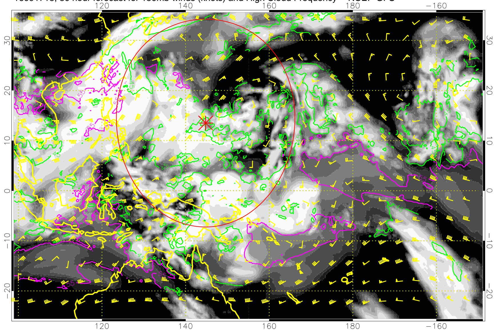
16091718, 30 hour forecast for 150mb winds (knots) and High Cloud Frequency -- NCEP GFS
