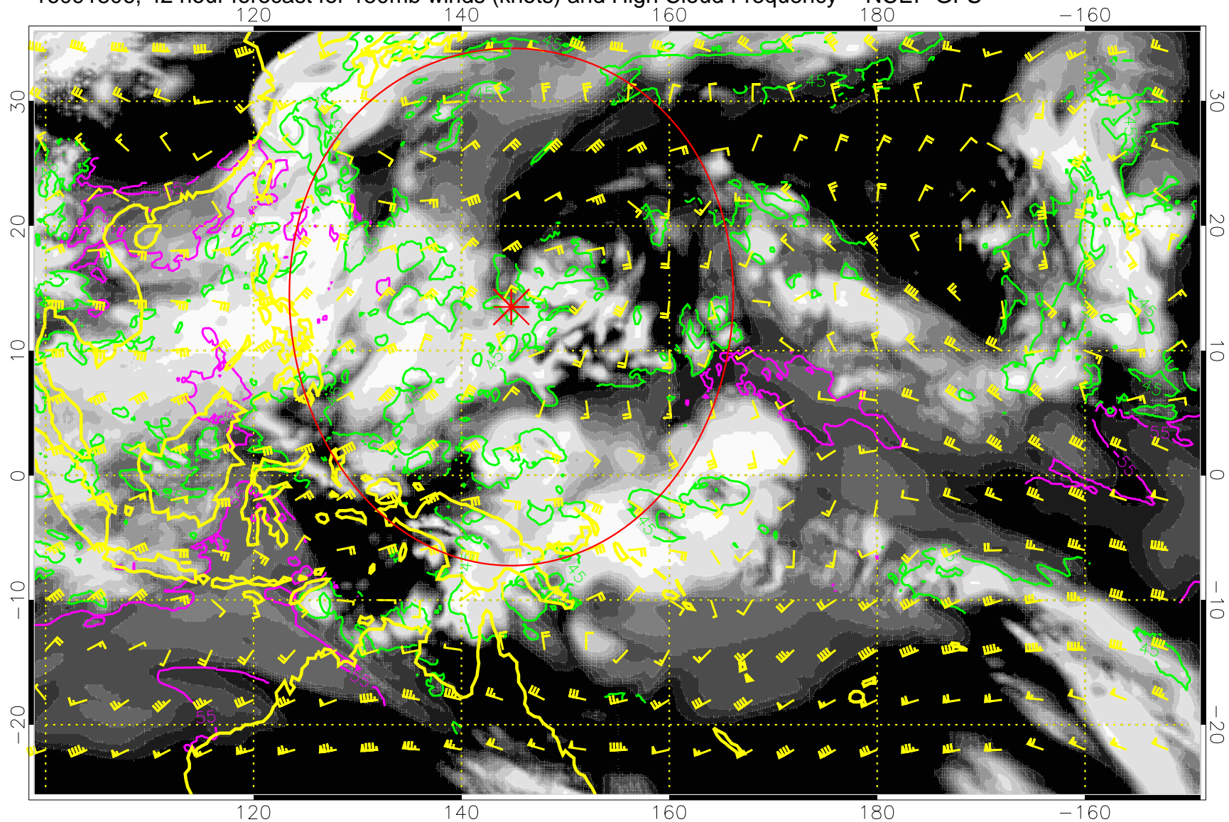
16091806, 42 hour forecast for 150mb winds (knots) and High Cloud Frequency -- NCEP GFS
