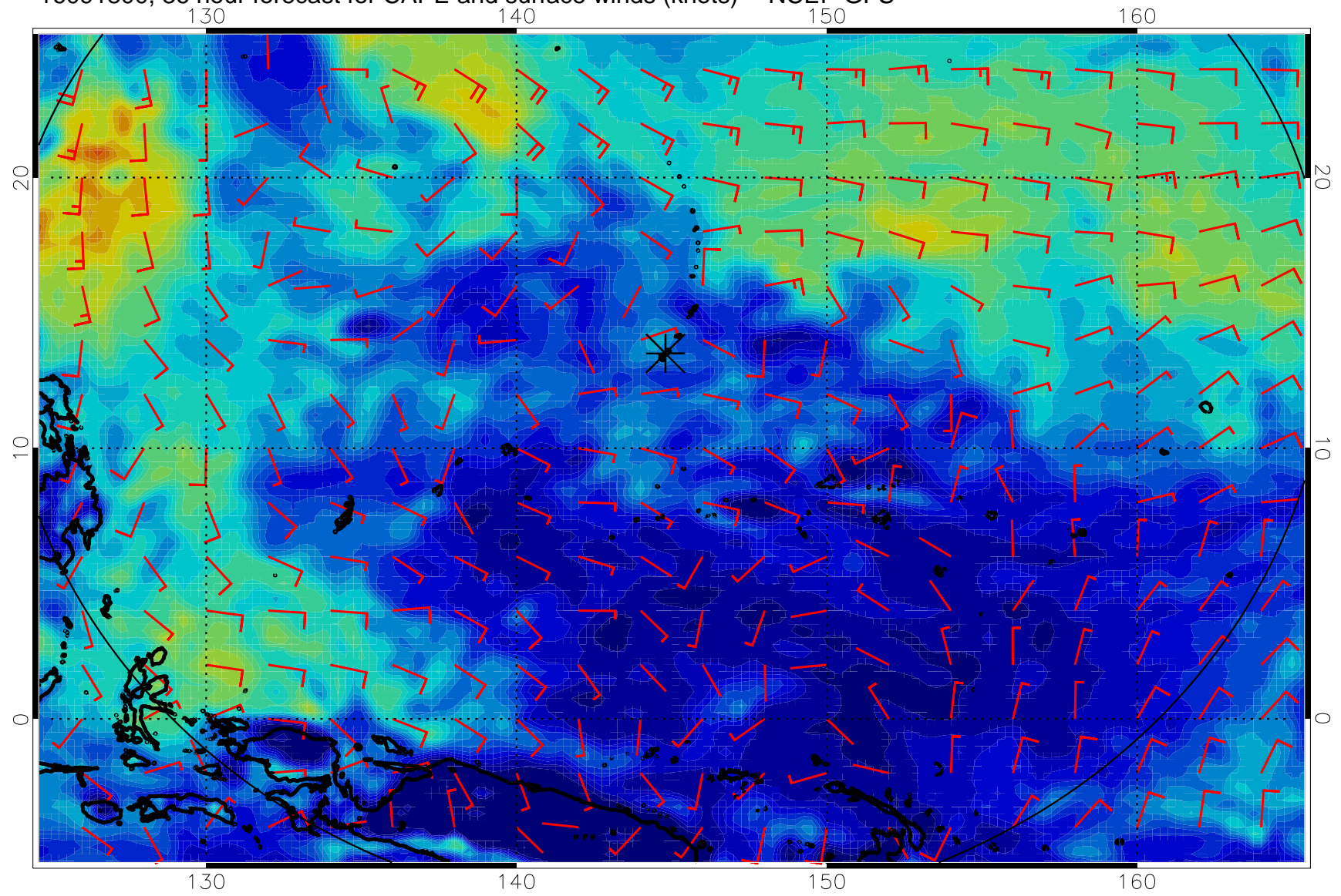
16091800, 36 hour forecast for CAPE and surface winds (knots) -- NCEP GFS
