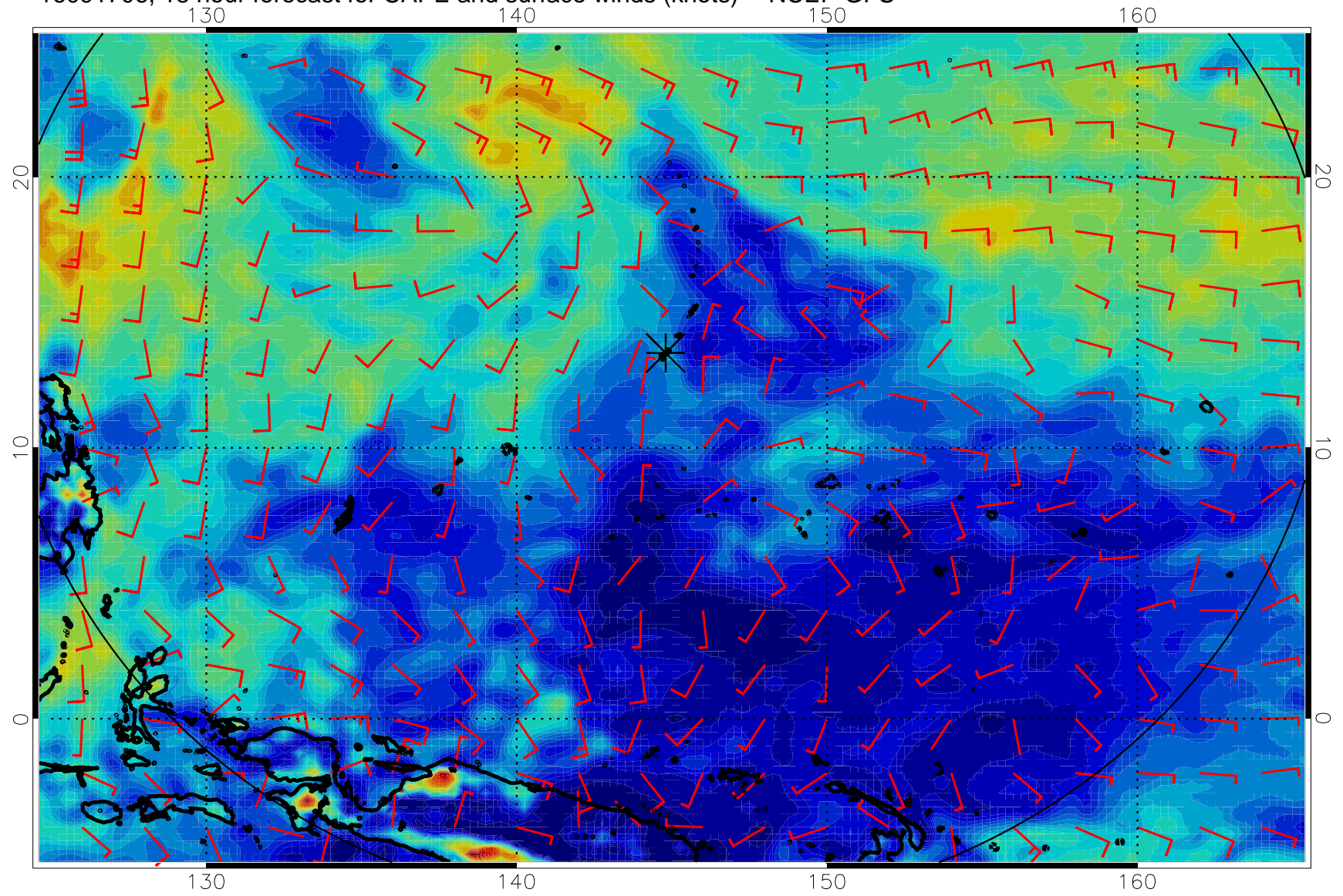
16091706, 18 hour forecast for CAPE and surface winds (knots) -- NCEP GFS
