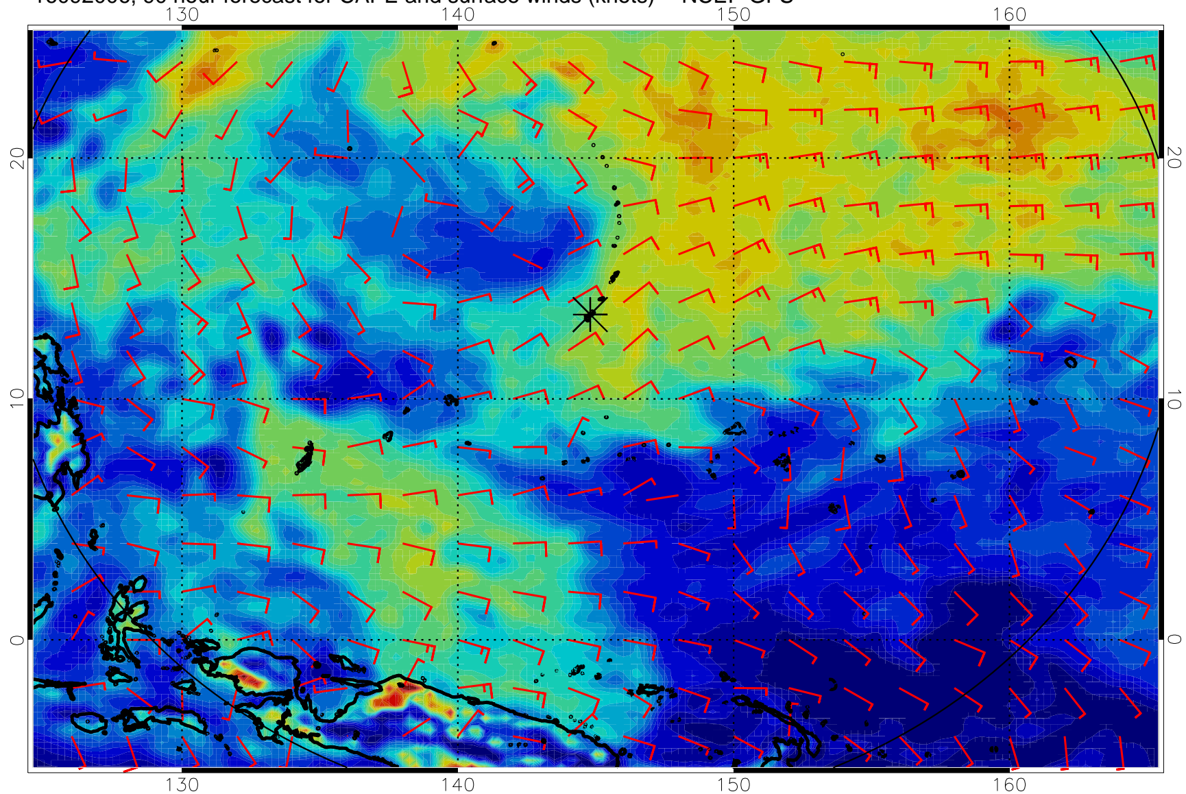
16092006, 90 hour forecast for CAPE and surface winds (knots) -- NCEP GFS
