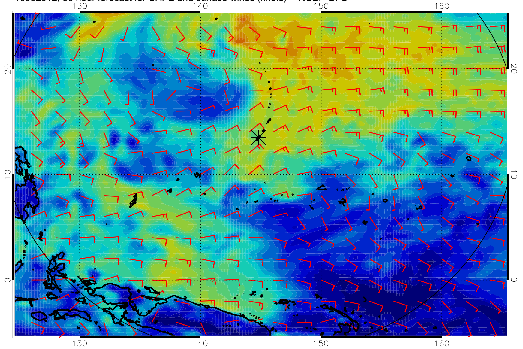
16092012, 96 hour forecast for CAPE and surface winds (knots) -- NCEP GFS
