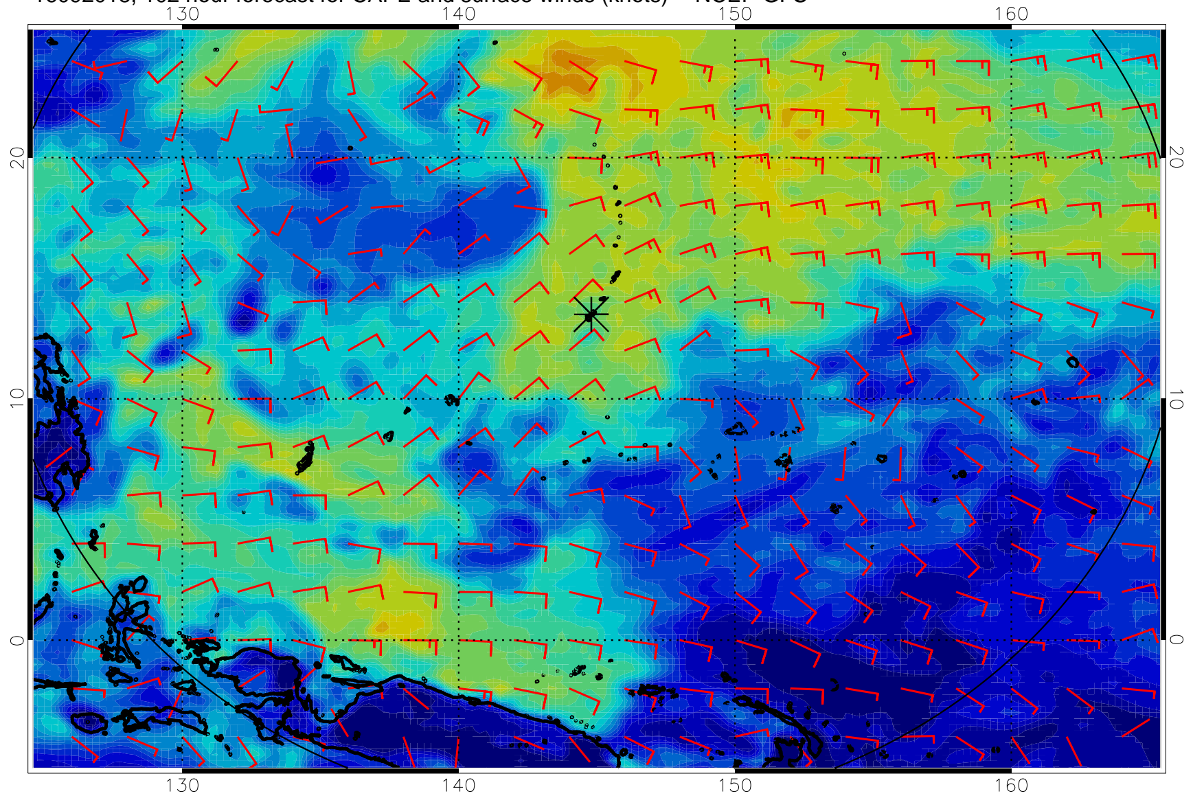
16092018, 102 hour forecast for CAPE and surface winds (knots) -- NCEP GFS
