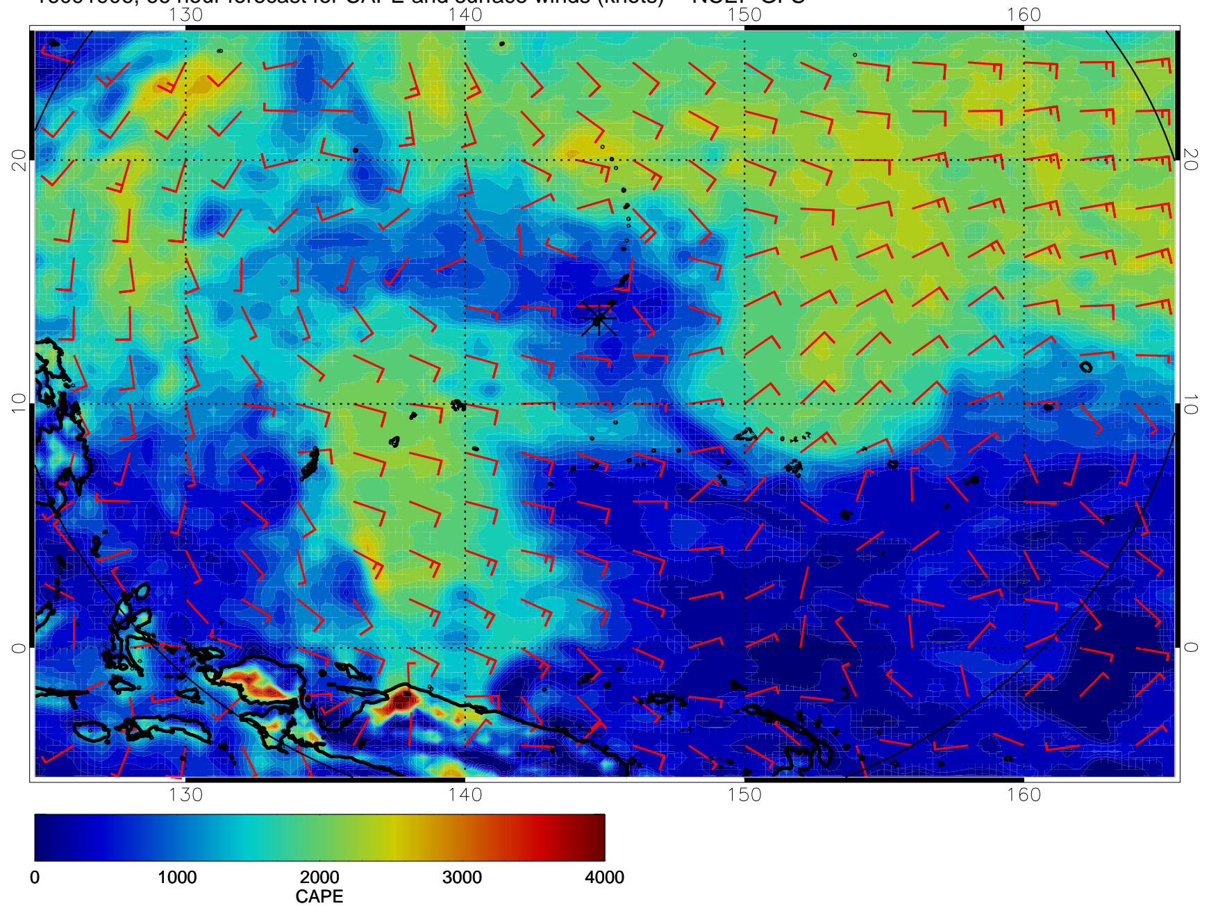
16091906, 66 hour forecast for CAPE and surface winds (knots) -- NCEP GFS
