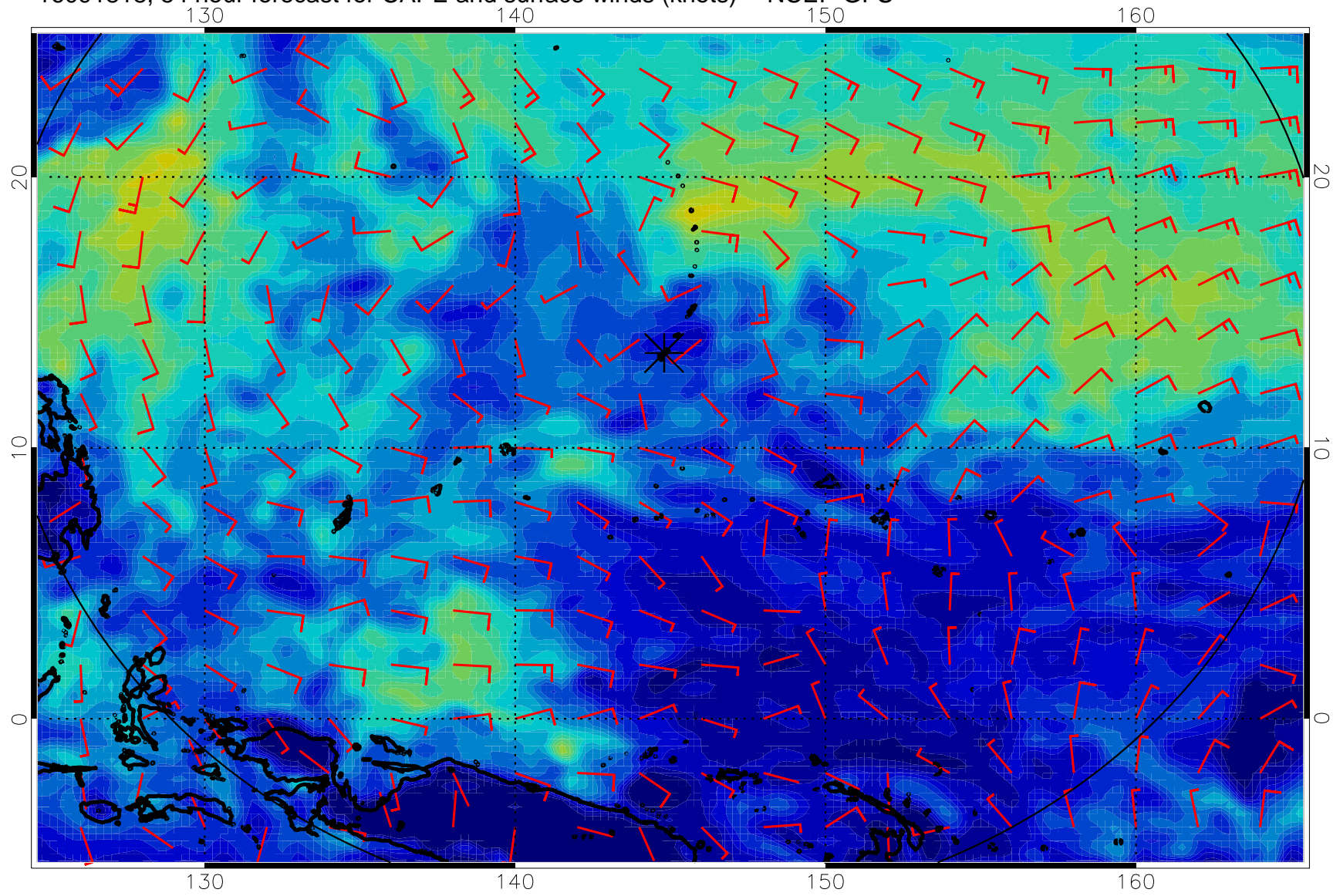
16091818, 54 hour forecast for CAPE and surface winds (knots) -- NCEP GFS
