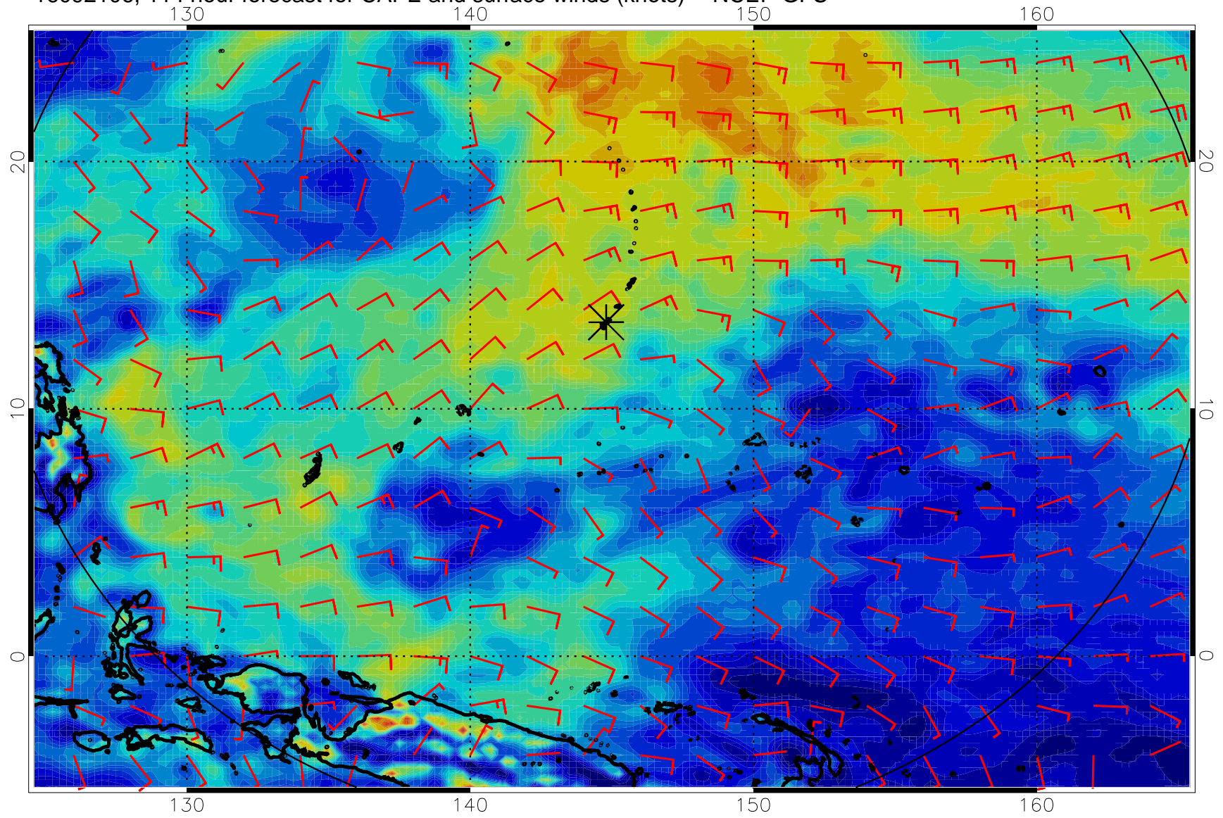
16092106, 114 hour forecast for CAPE and surface winds (knots) -- NCEP GFS
