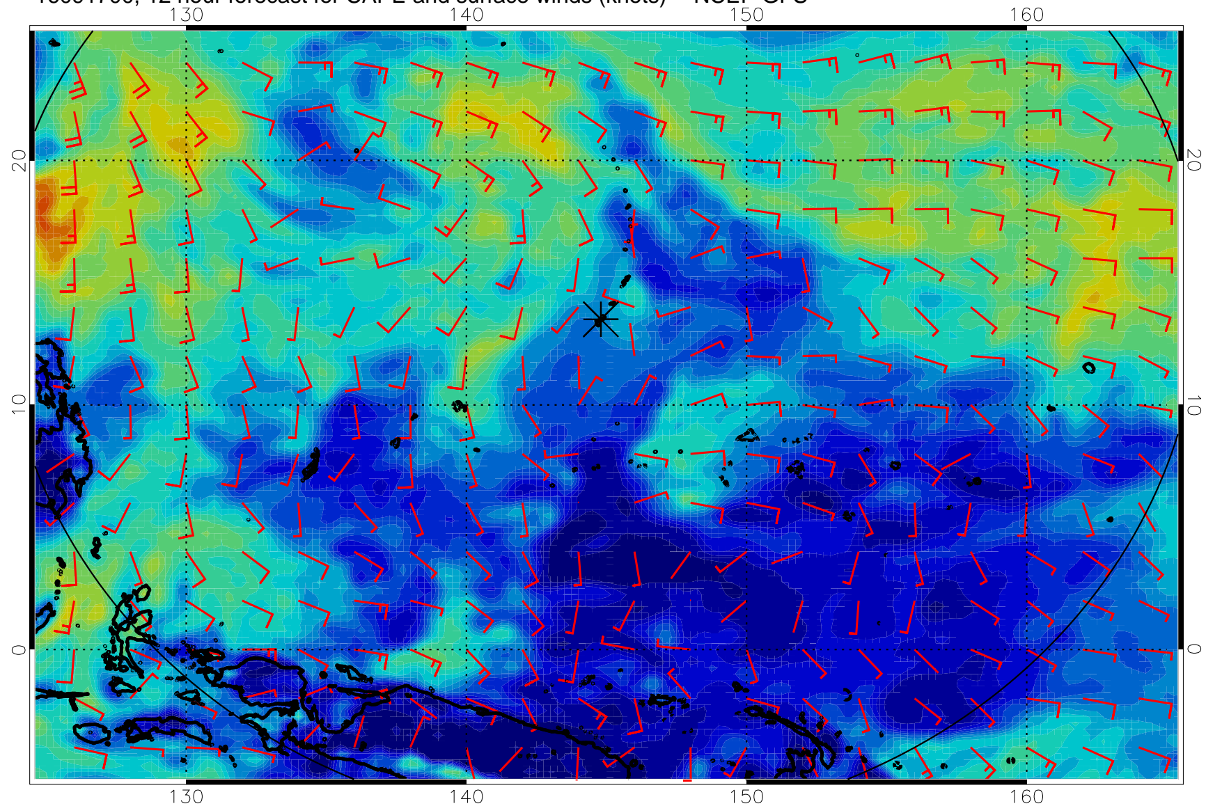
16091700, 12 hour forecast for CAPE and surface winds (knots) -- NCEP GFS
