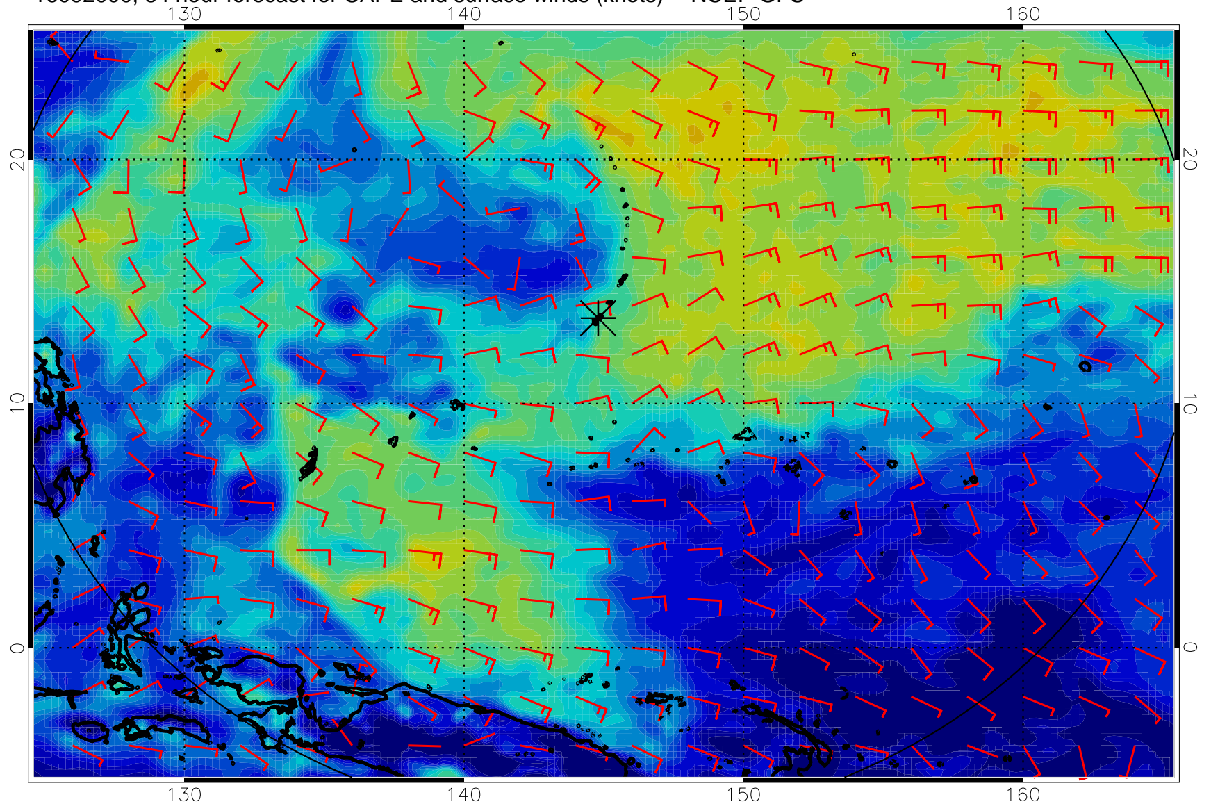
16092000, 84 hour forecast for CAPE and surface winds (knots) -- NCEP GFS
