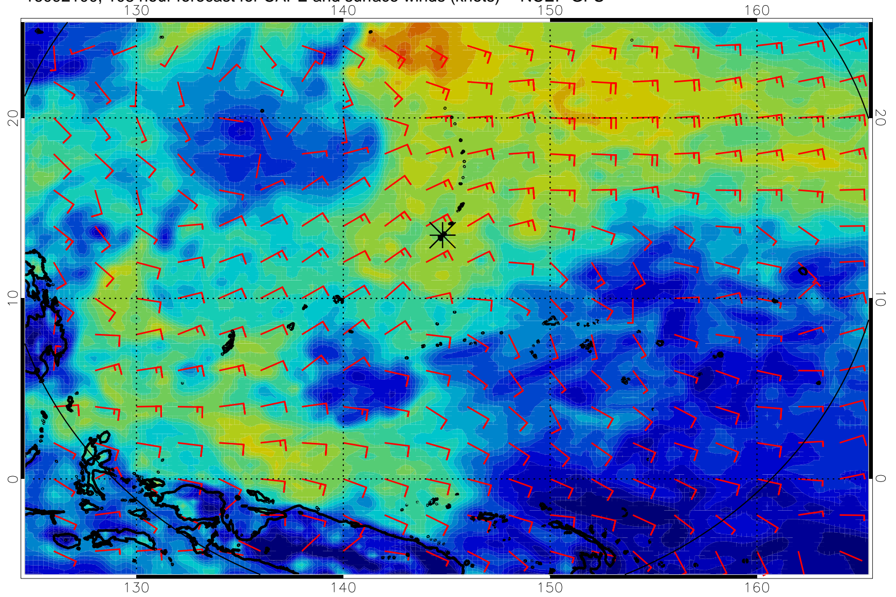
16092100, 108 hour forecast for CAPE and surface winds (knots) -- NCEP GFS
