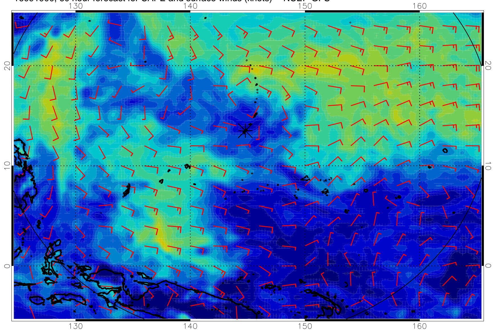
16091900, 60 hour forecast for CAPE and surface winds (knots) -- NCEP GFS
