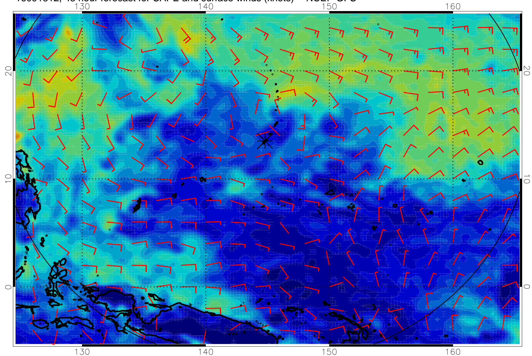
16091812, 48 hour forecast for CAPE and surface winds (knots) -- NCEP GFS
