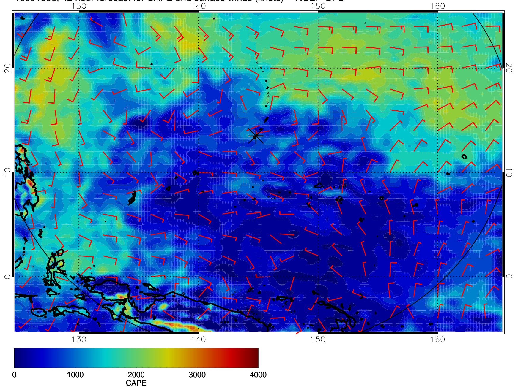
16091806, 42 hour forecast for CAPE and surface winds (knots) -- NCEP GFS
