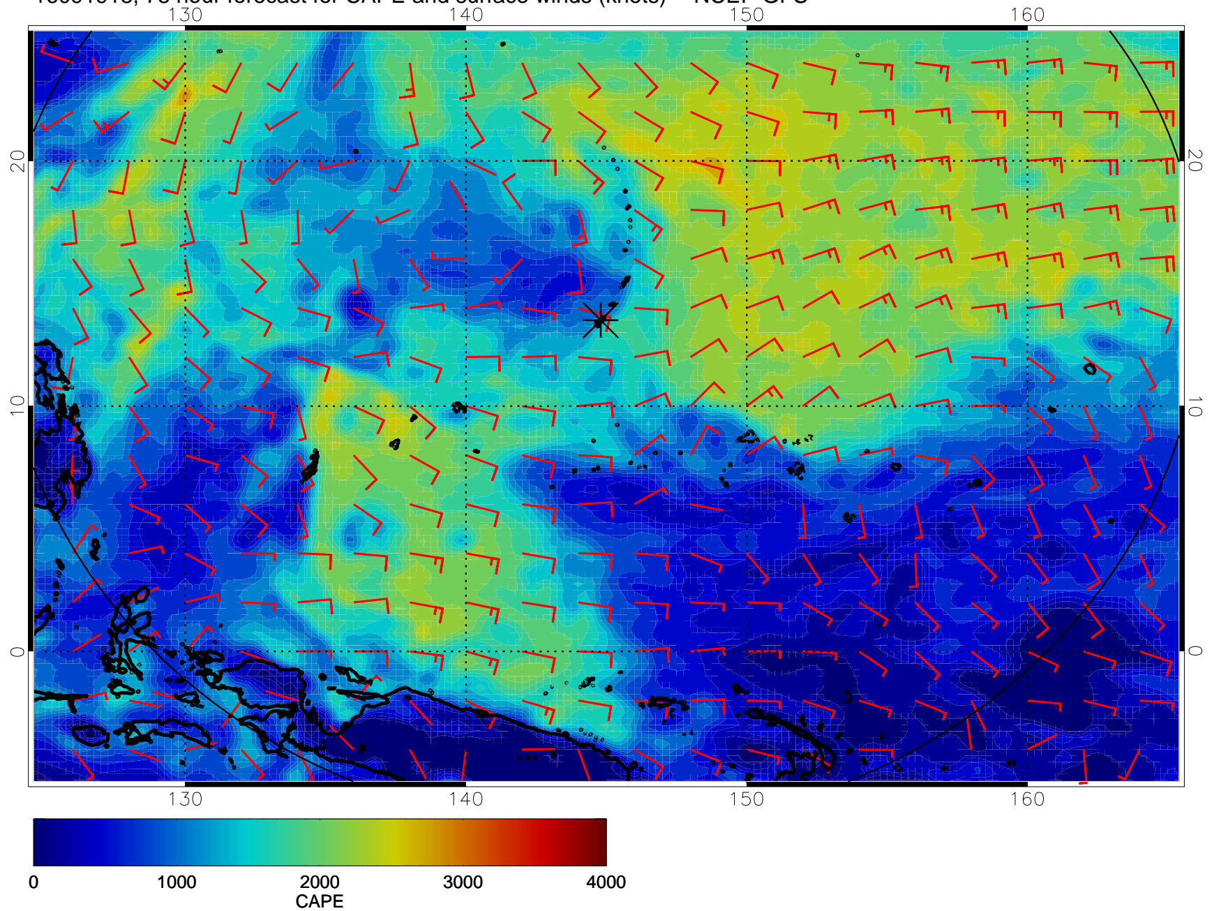
16091918, 78 hour forecast for CAPE and surface winds (knots) -- NCEP GFS
