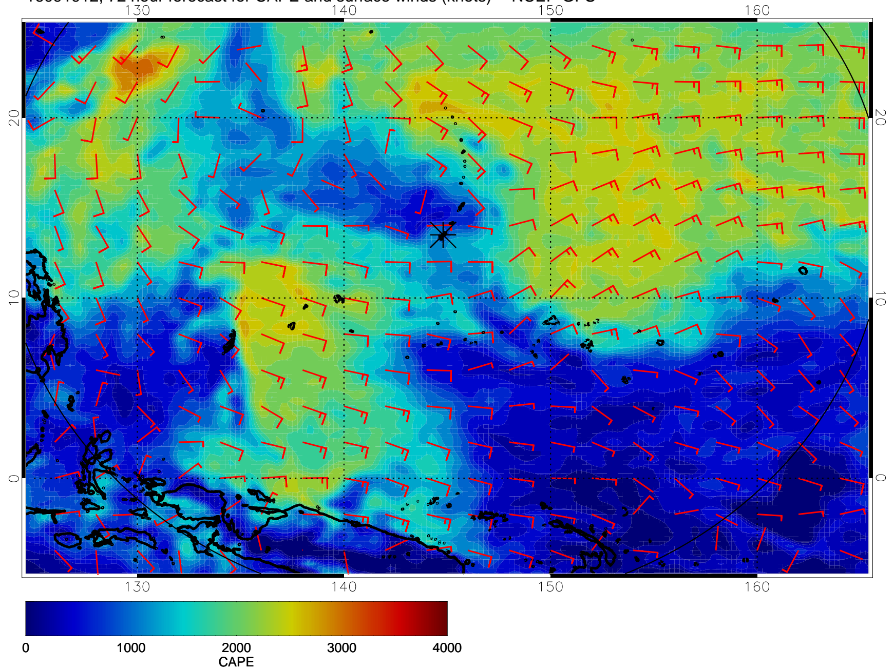
16091912, 72 hour forecast for CAPE and surface winds (knots) -- NCEP GFS
