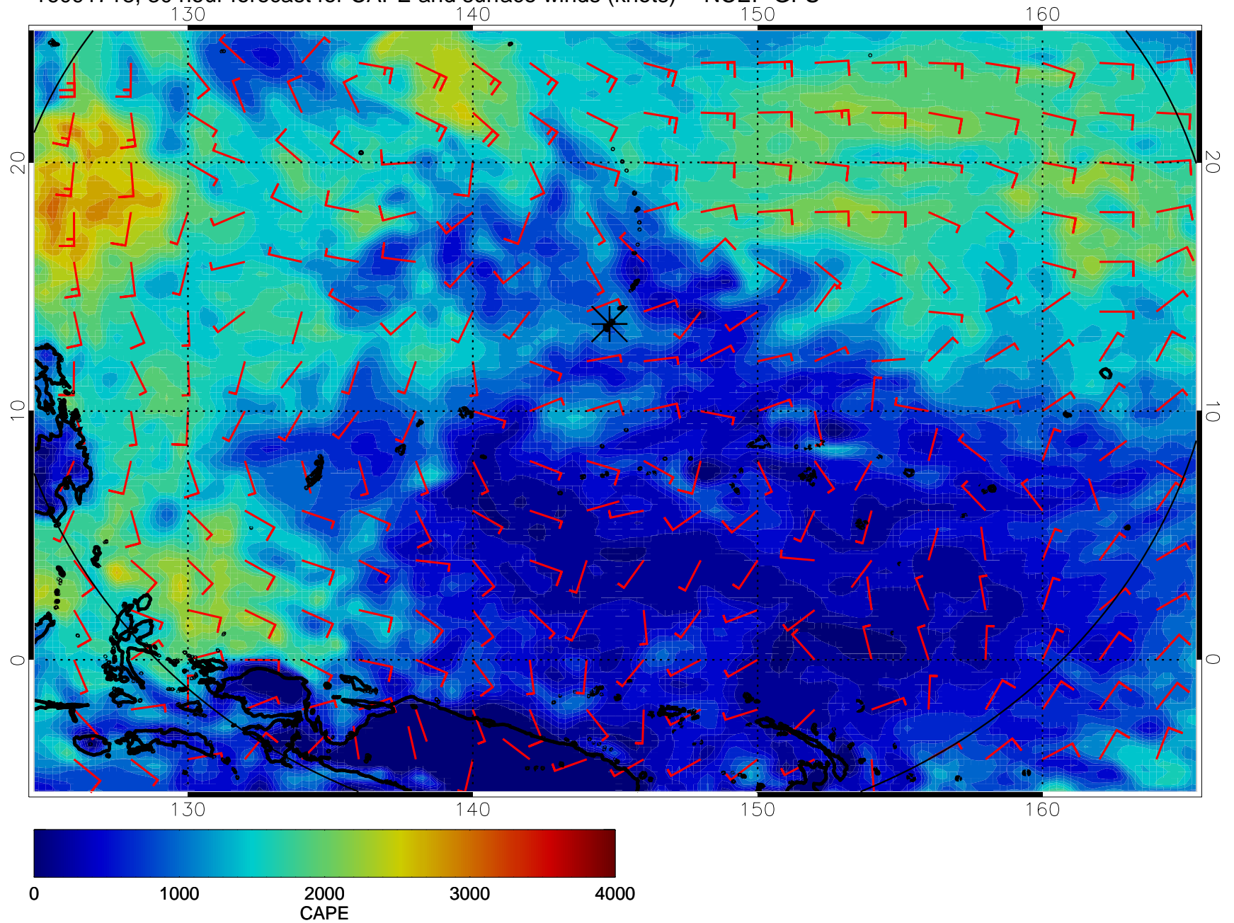
16091718, 30 hour forecast for CAPE and surface winds (knots) -- NCEP GFS
