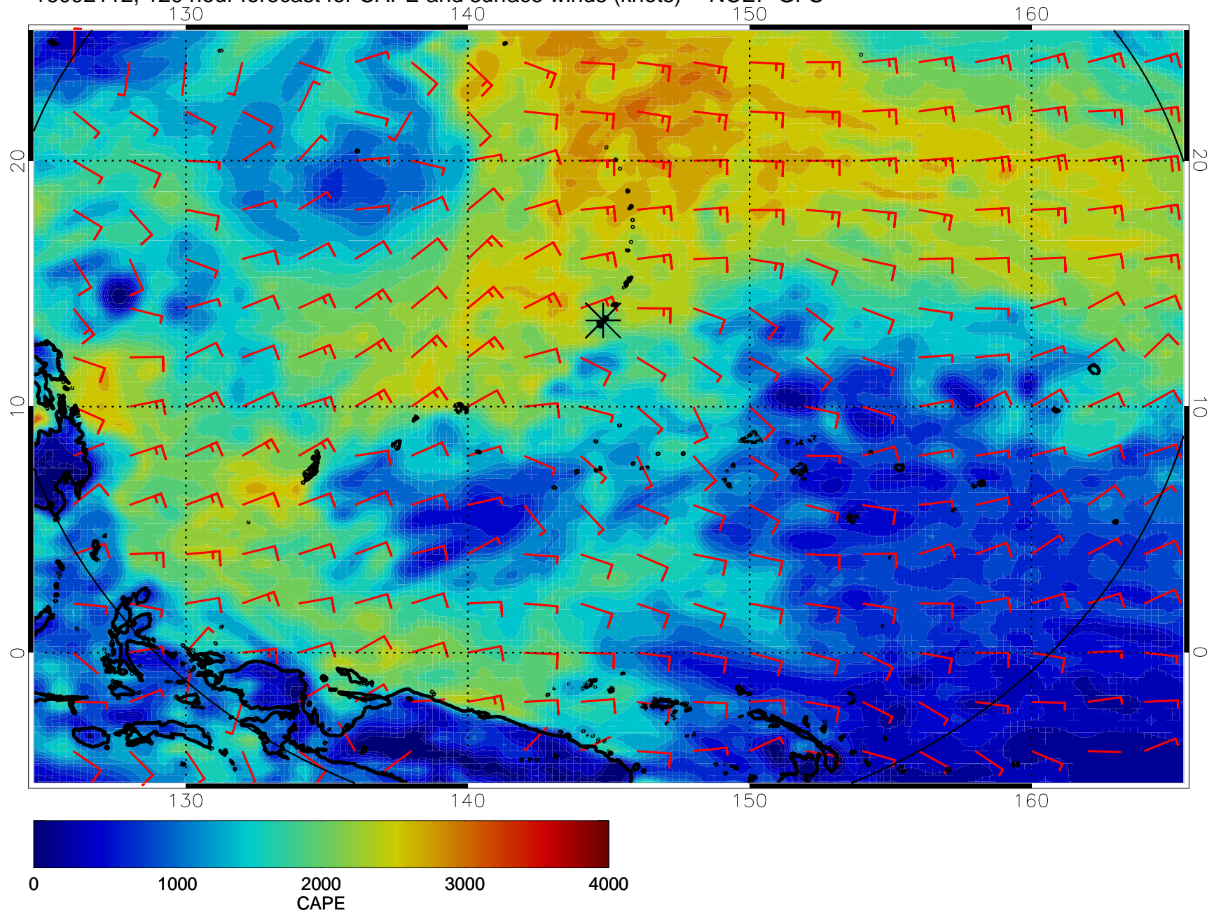
16092112, 120 hour forecast for CAPE and surface winds (knots) -- NCEP GFS
