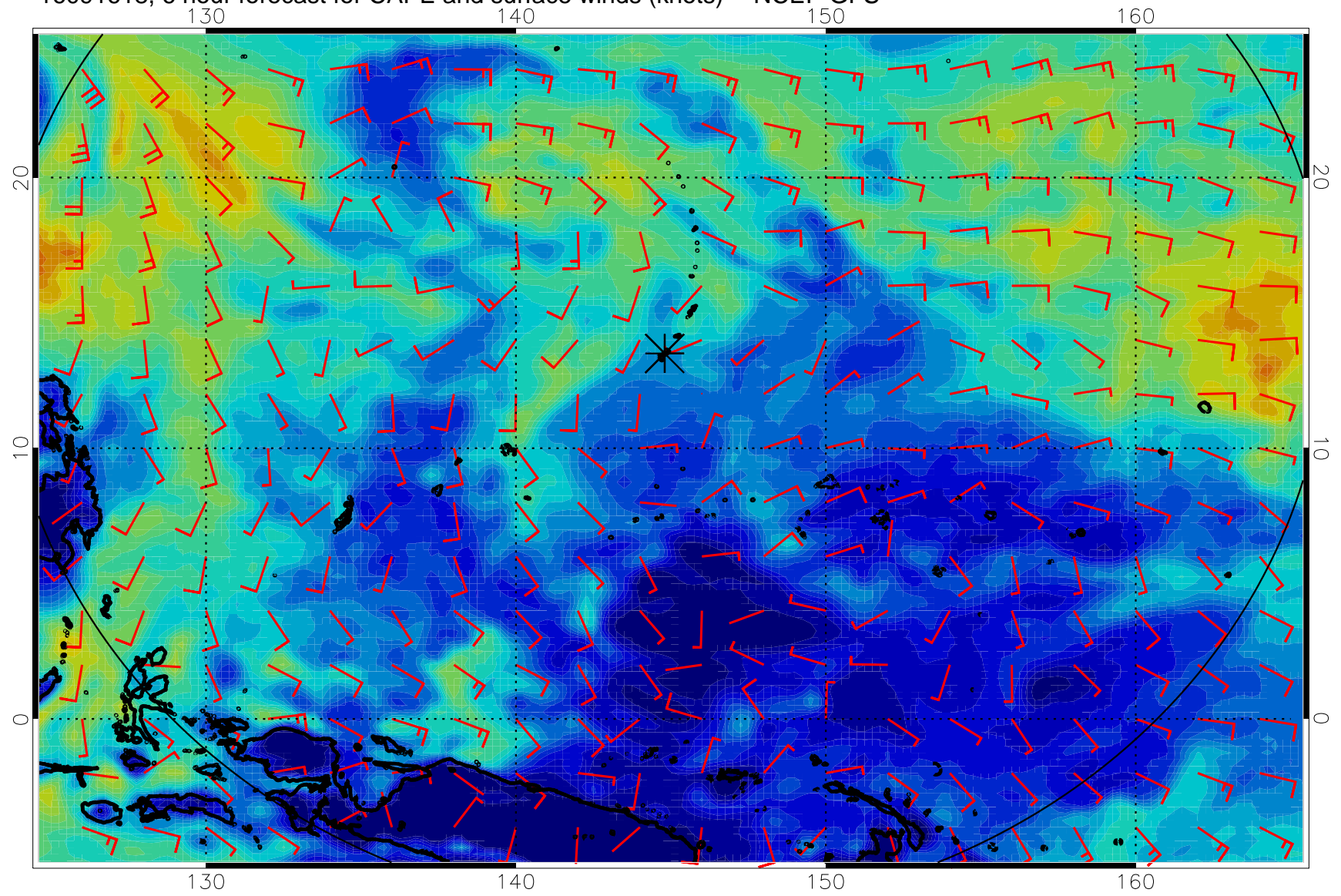
16091618, 6 hour forecast for CAPE and surface winds (knots) -- NCEP GFS
