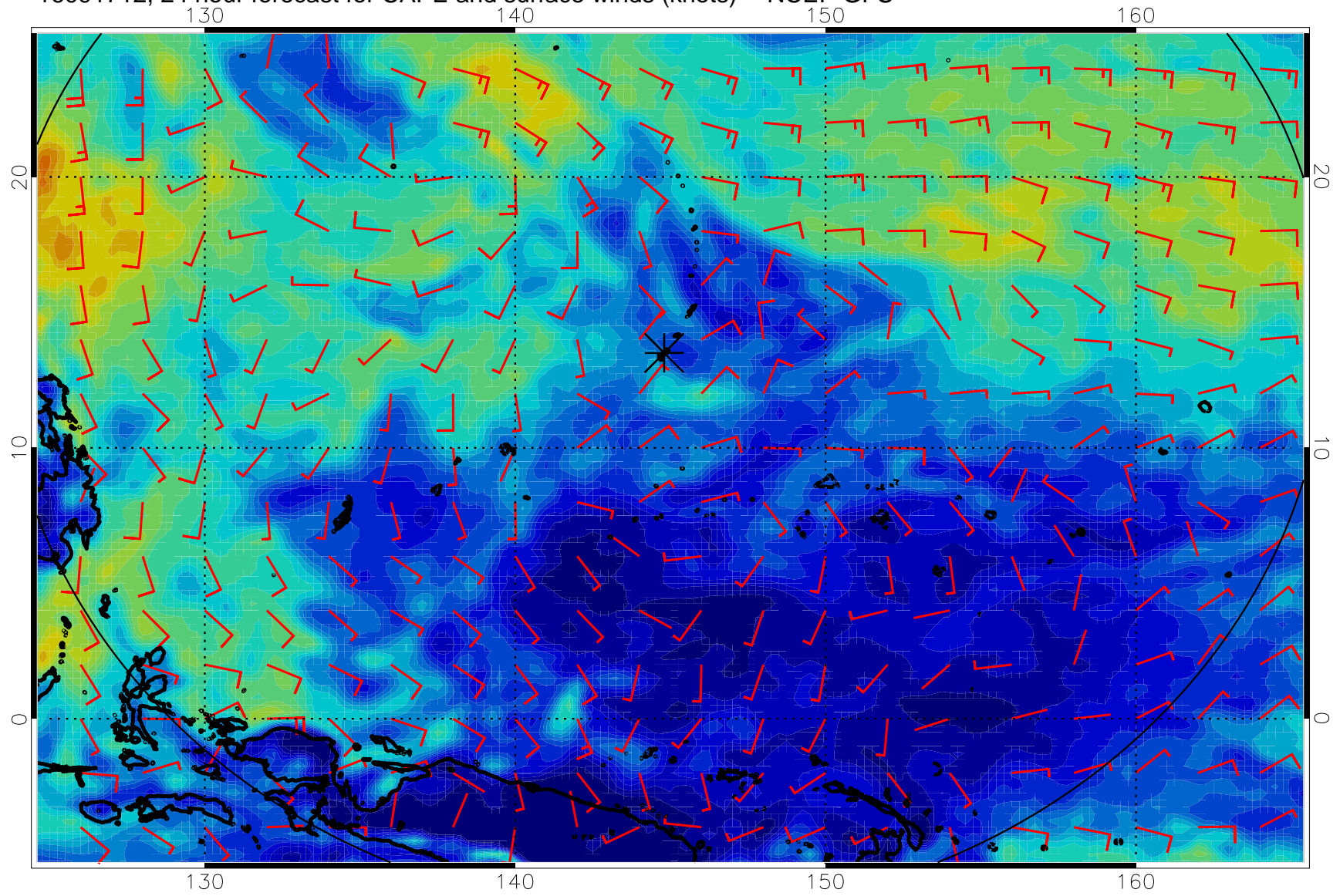
16091712, 24 hour forecast for CAPE and surface winds (knots) -- NCEP GFS
