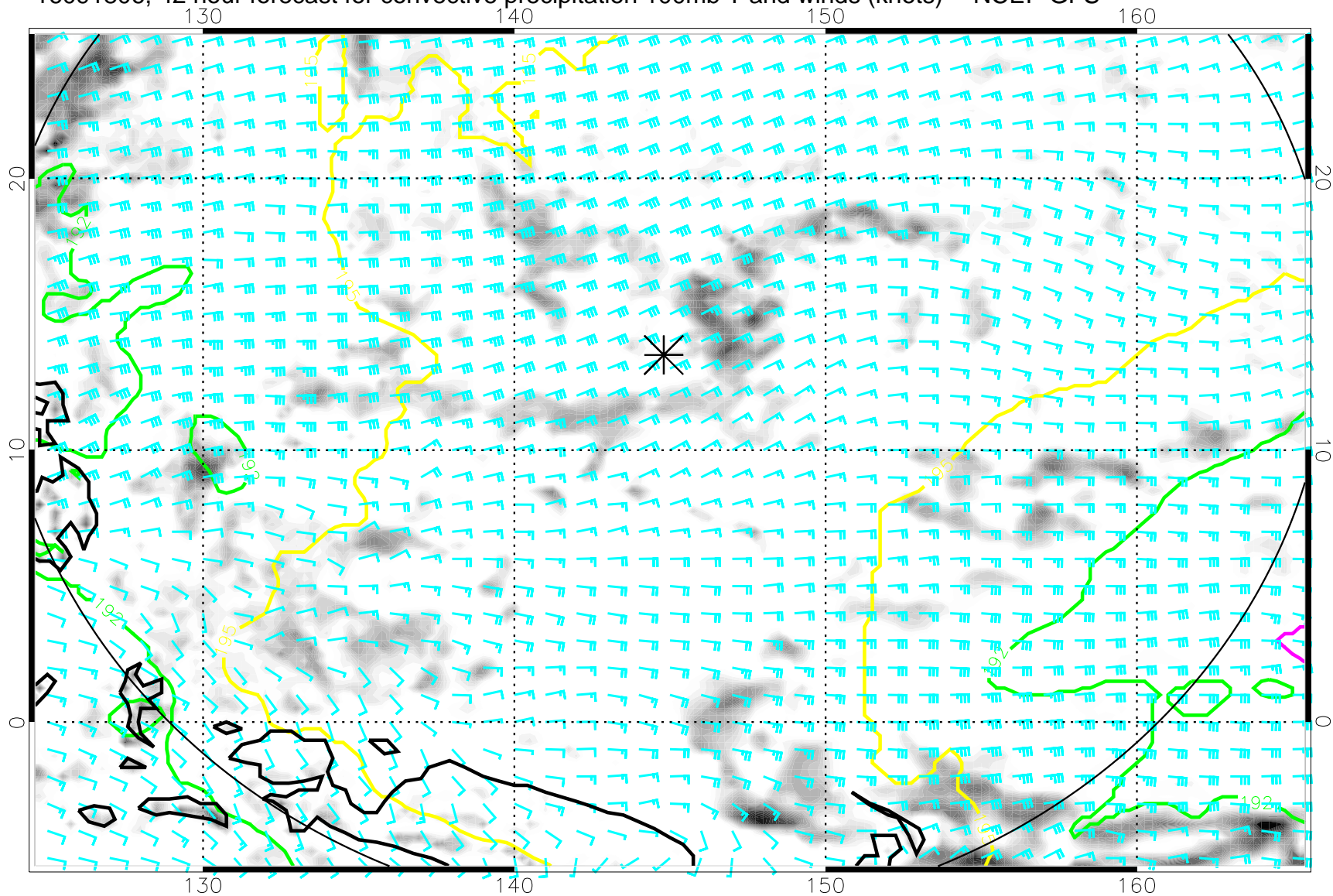
16091806, 42 hour forecast for convective precipitation 100mb T and winds (knots) -- NCEP GFS
