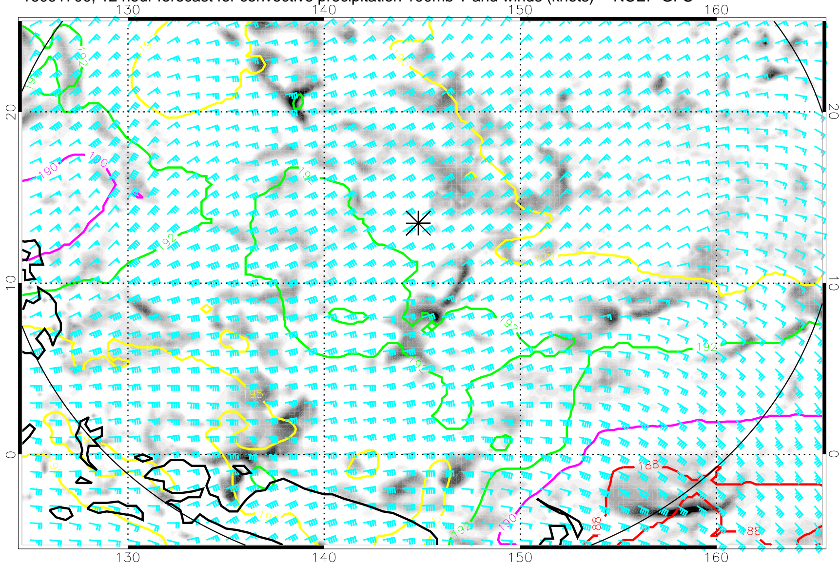
16091700, 12 hour forecast for convective precipitation 100mb T and winds (knots) -- NCEP GFS
