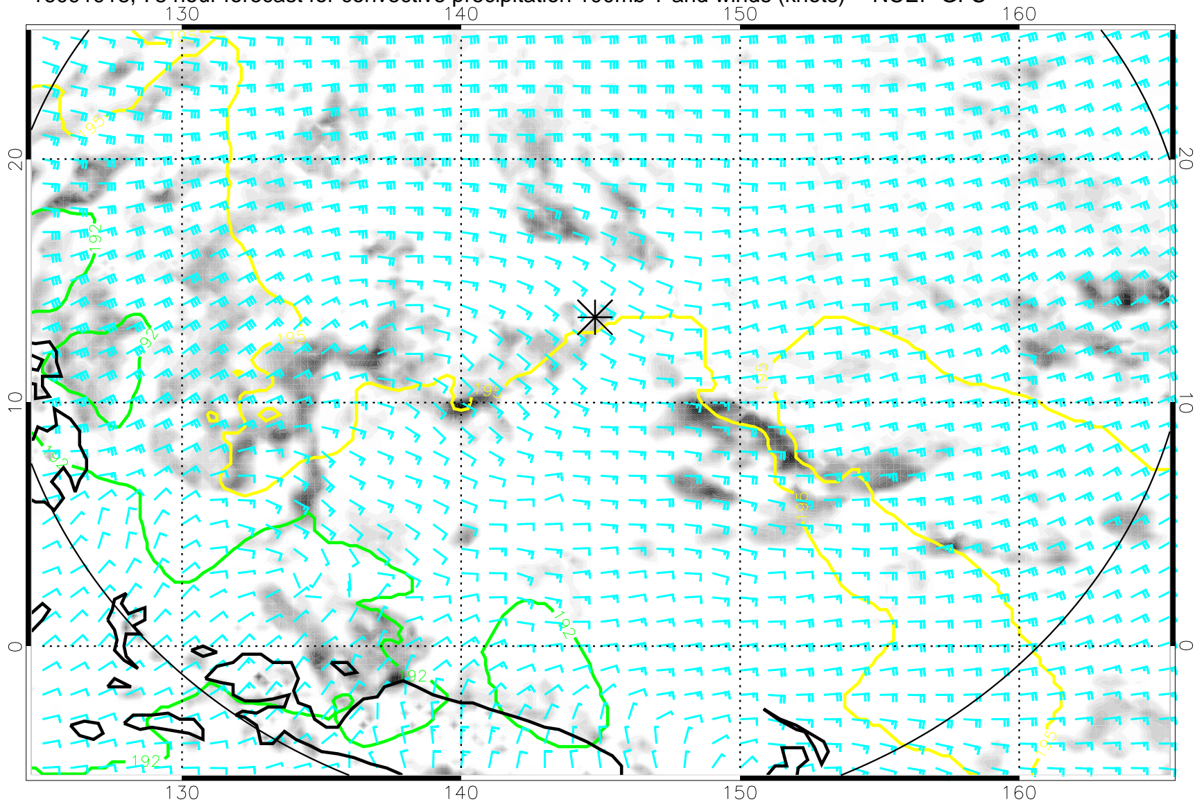
16091918, 78 hour forecast for convective precipitation 100mb T and winds (knots) -- NCEP GFS
