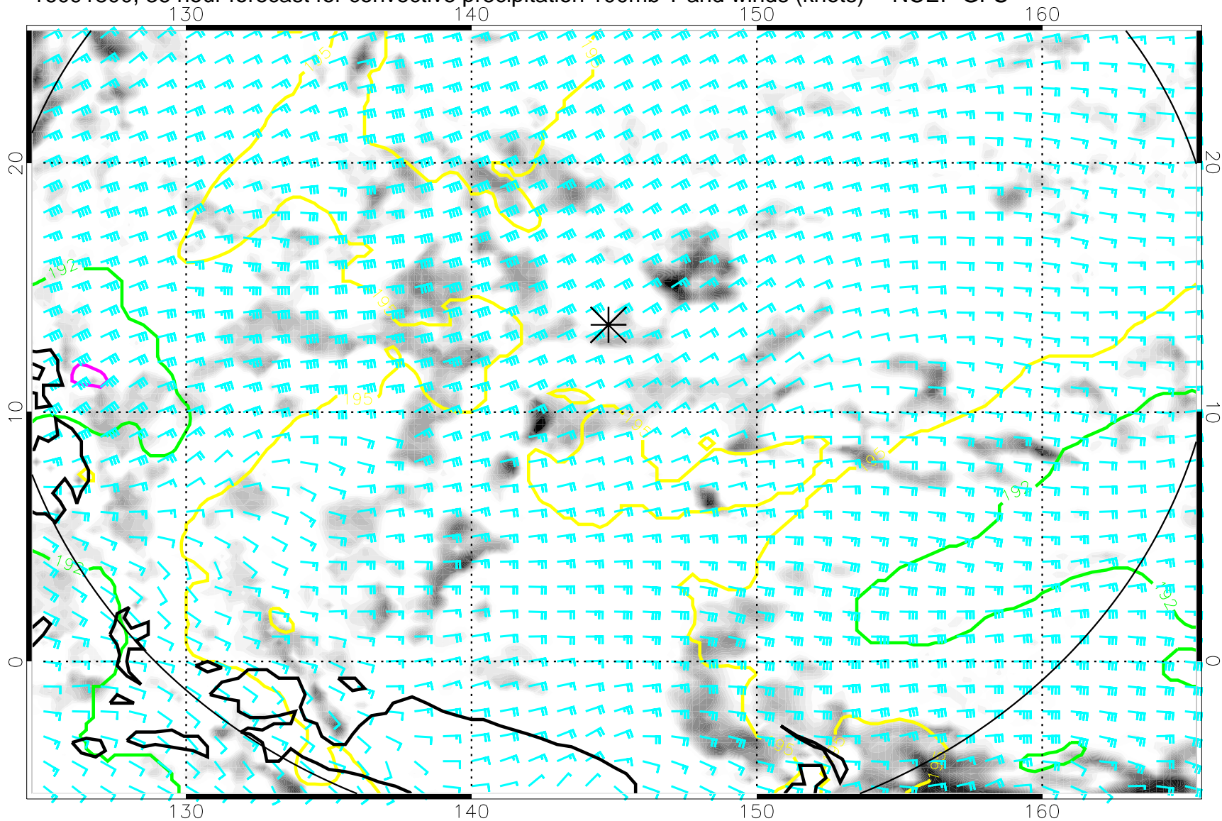
16091800, 36 hour forecast for convective precipitation 100mb T and winds (knots) -- NCEP GFS
