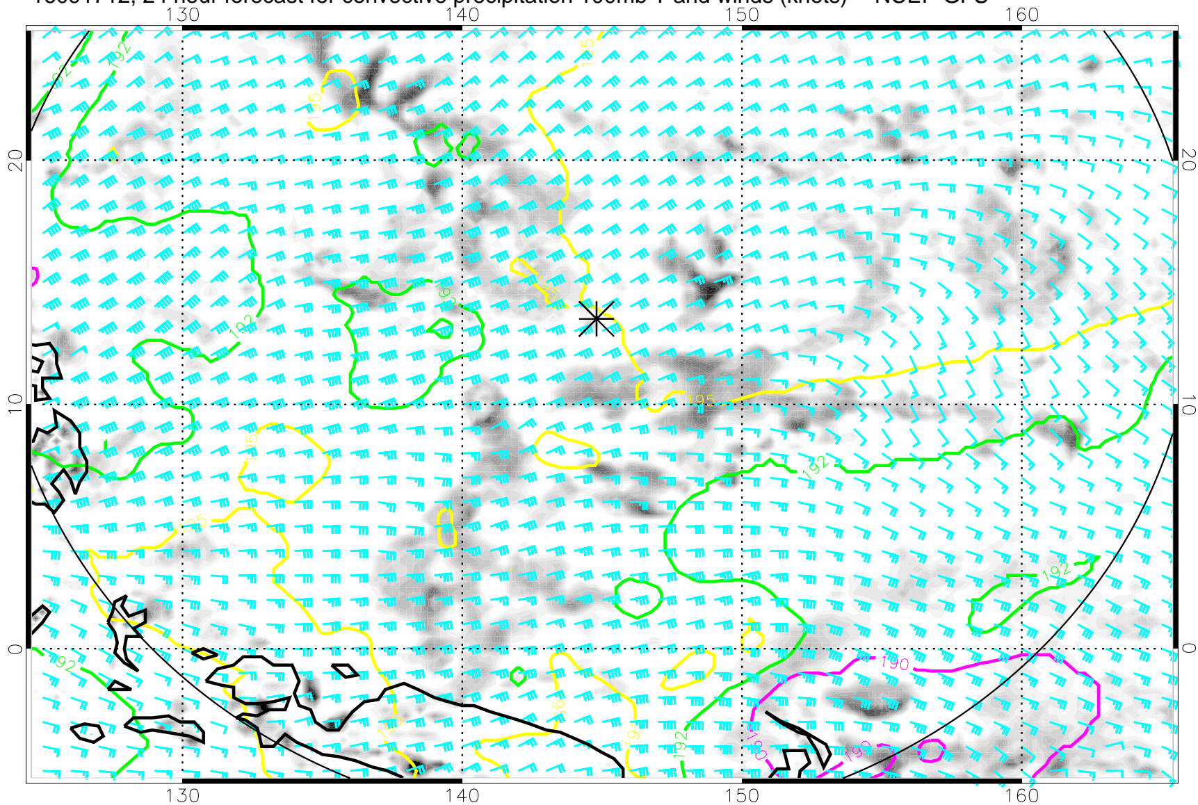
16091712, 24 hour forecast for convective precipitation 100mb T and winds (knots) -- NCEP GFS
