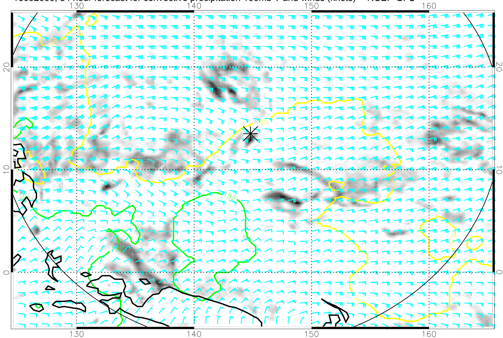
16092000, 84 hour forecast for convective precipitation 100mb T and winds (knots) -- NCEP GFS
