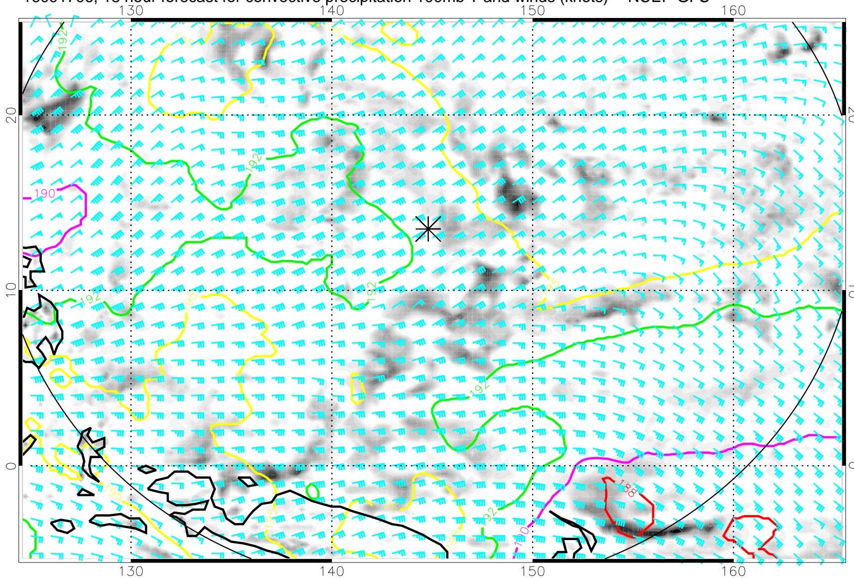
16091706, 18 hour forecast for convective precipitation 100mb T and winds (knots) -- NCEP GFS
