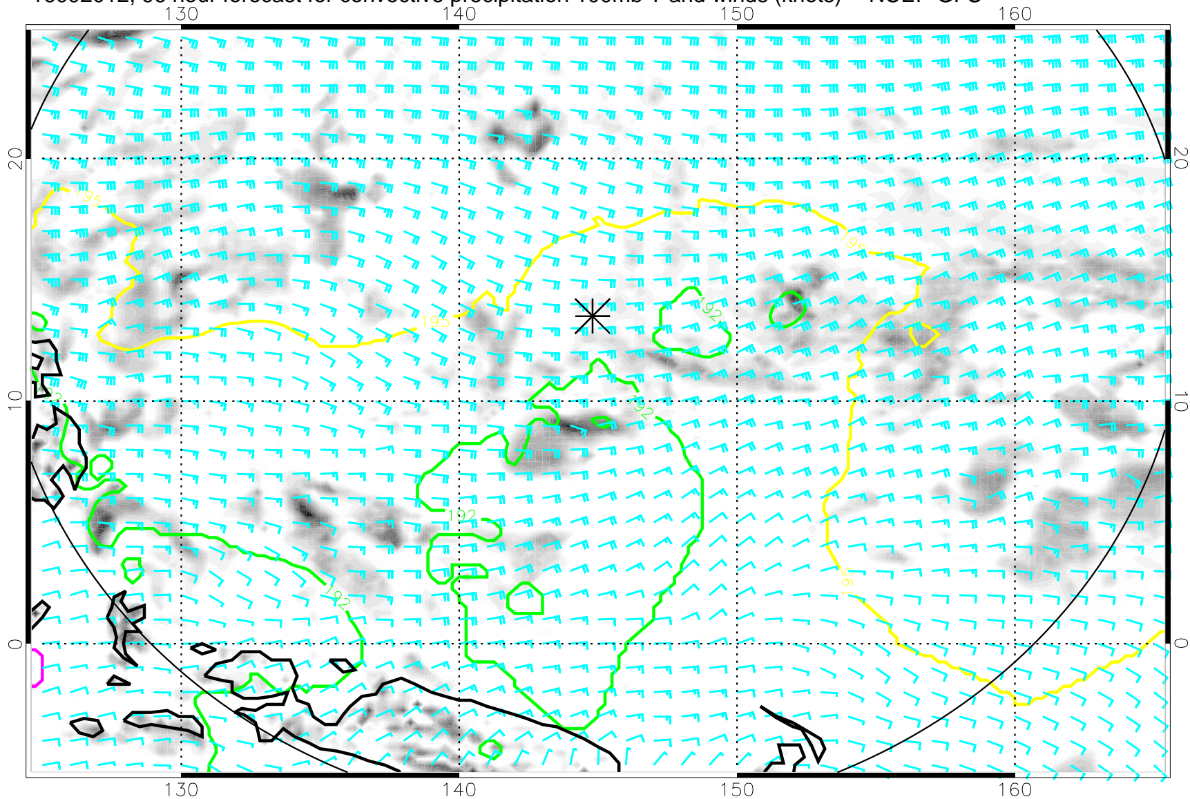
16092012, 96 hour forecast for convective precipitation 100mb T and winds (knots) -- NCEP GFS
