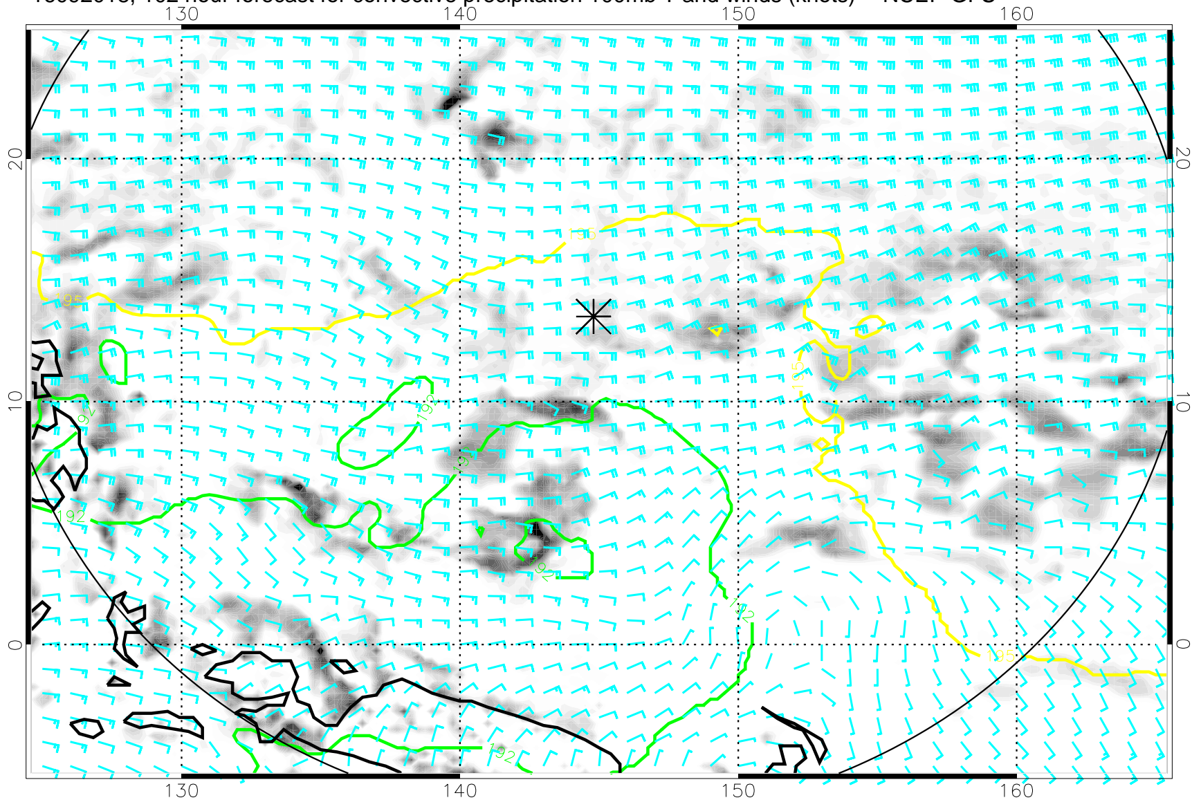
16092018, 102 hour forecast for convective precipitation 100mb T and winds (knots) -- NCEP GFS
