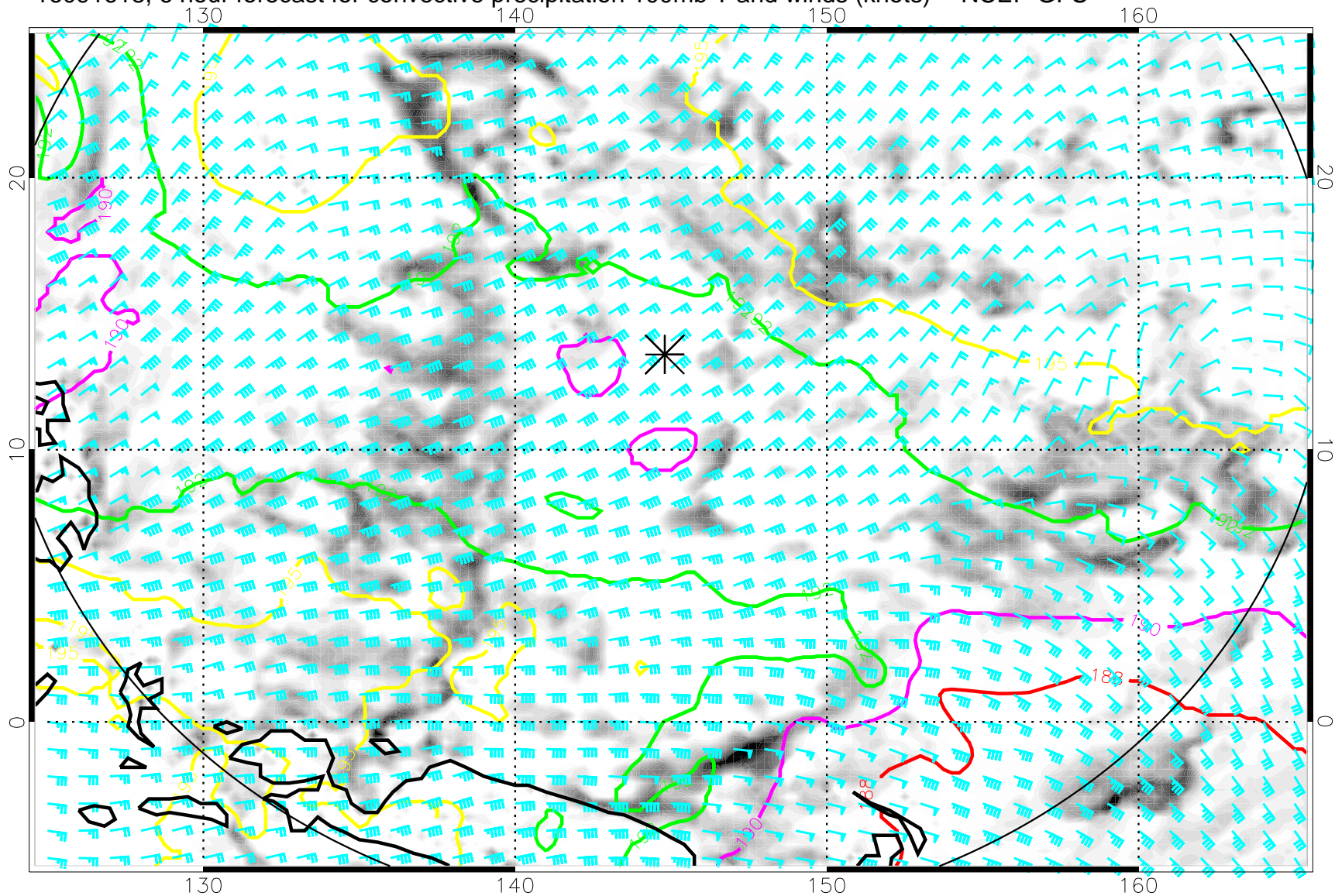
16091618, 6 hour forecast for convective precipitation 100mb T and winds (knots) -- NCEP GFS
