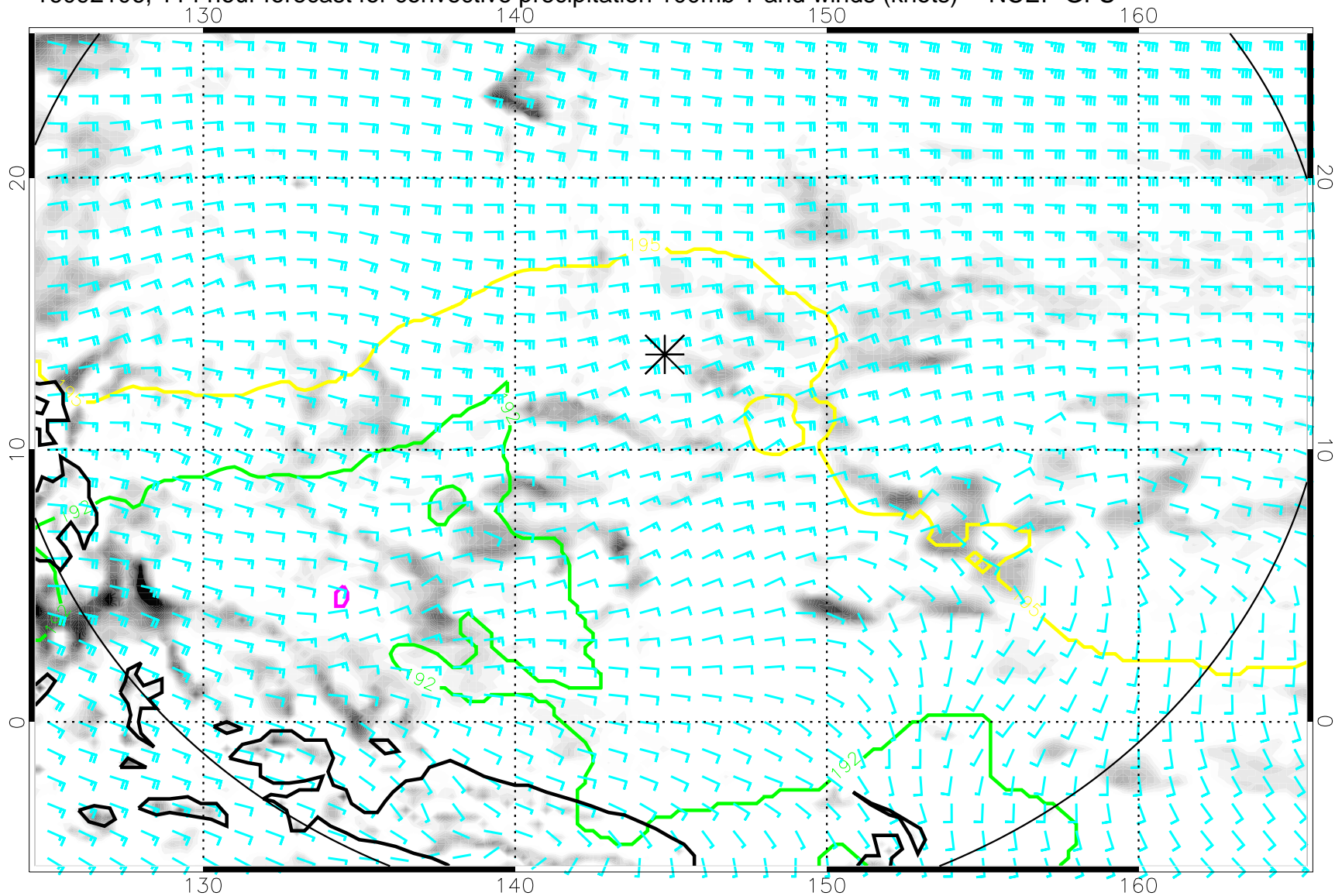
16092106, 114 hour forecast for convective precipitation 100mb T and winds (knots) -- NCEP GFS
