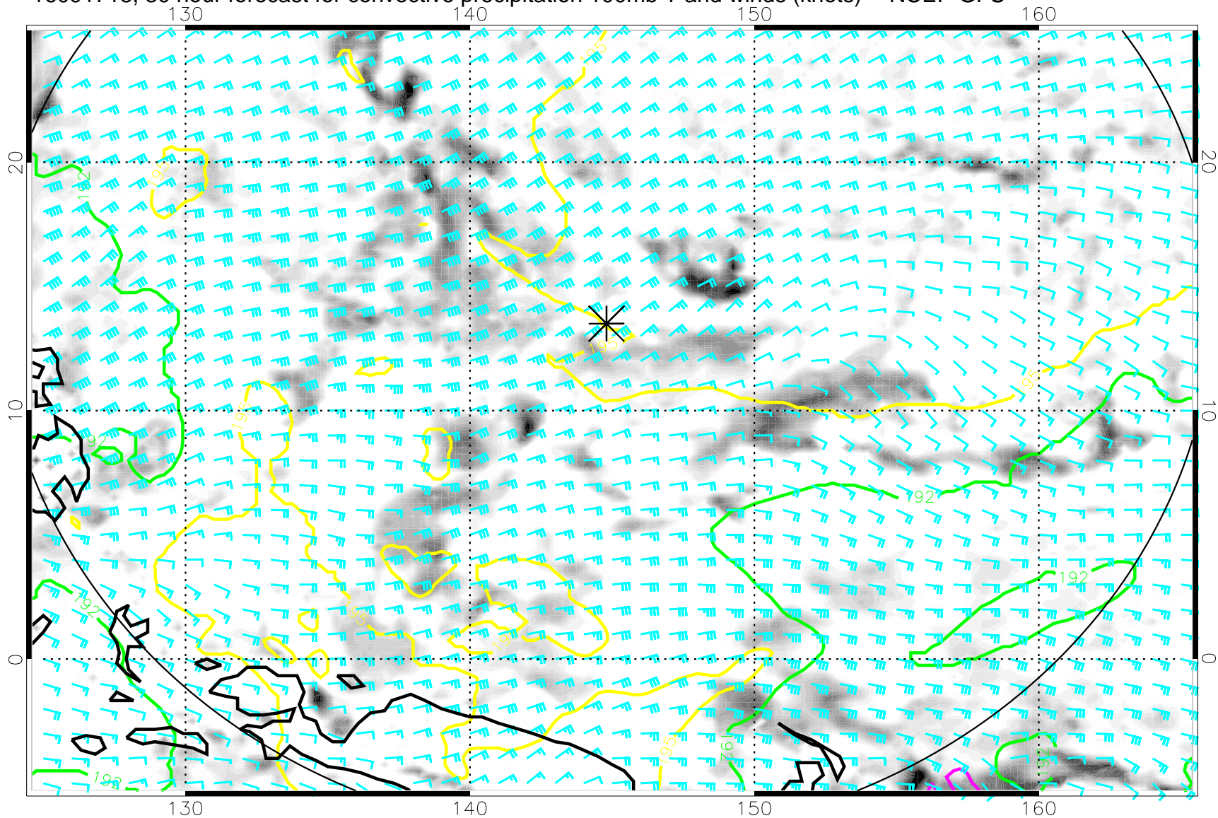
16091718, 30 hour forecast for convective precipitation 100mb T and winds (knots) -- NCEP GFS
