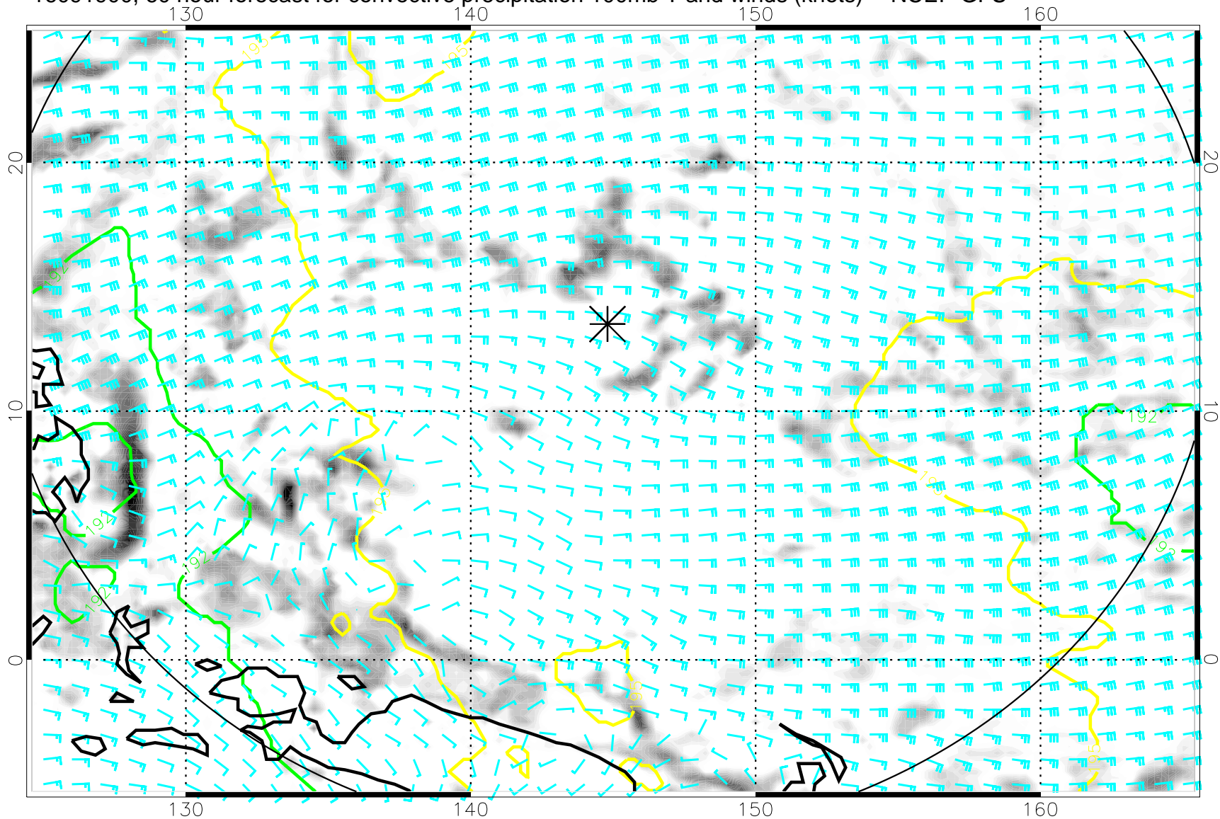
16091900, 60 hour forecast for convective precipitation 100mb T and winds (knots) -- NCEP GFS
