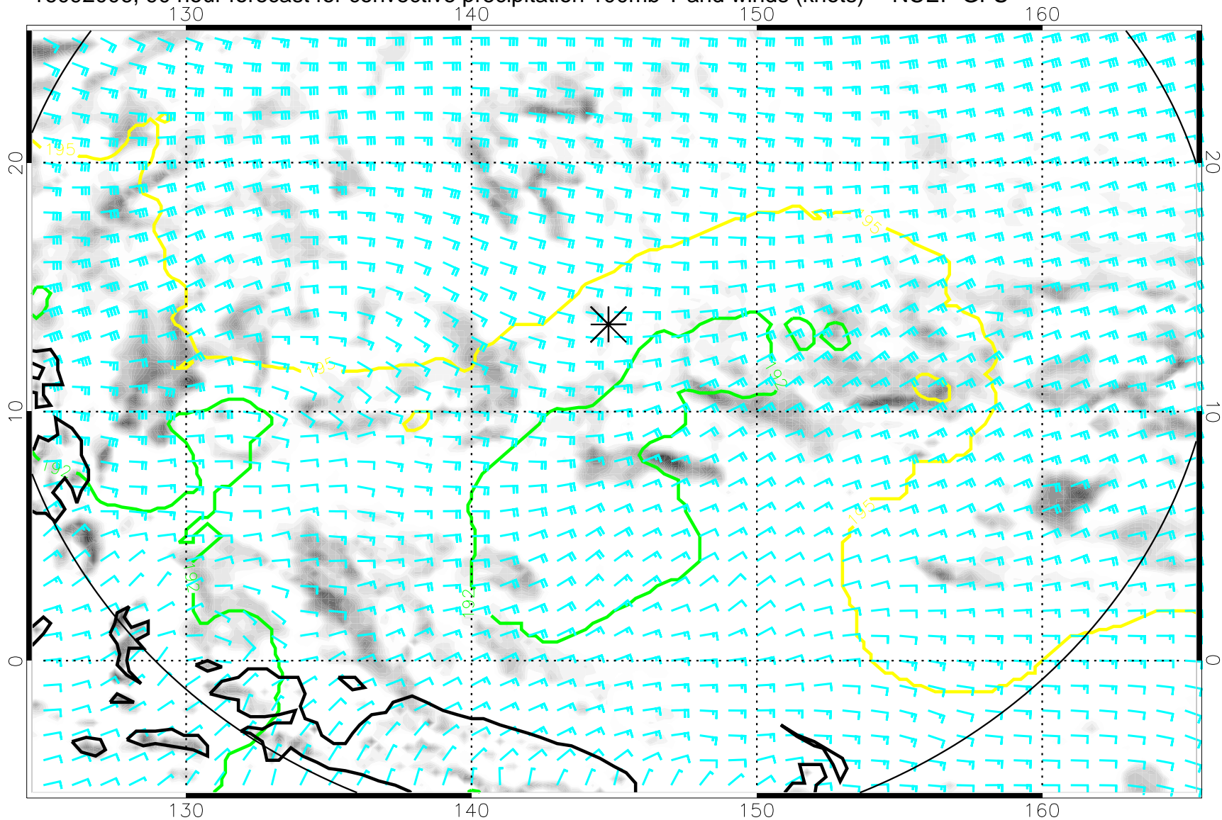
16092006, 90 hour forecast for convective precipitation 100mb T and winds (knots) -- NCEP GFS
