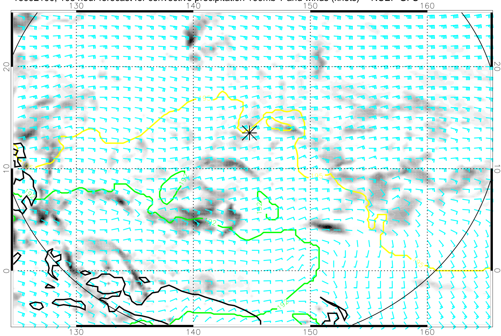
16092100, 108 hour forecast for convective precipitation 100mb T and winds (knots) -- NCEP GFS
