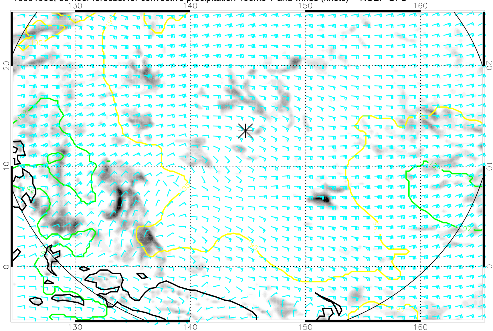
16091906, 66 hour forecast for convective precipitation 100mb T and winds (knots) -- NCEP GFS
