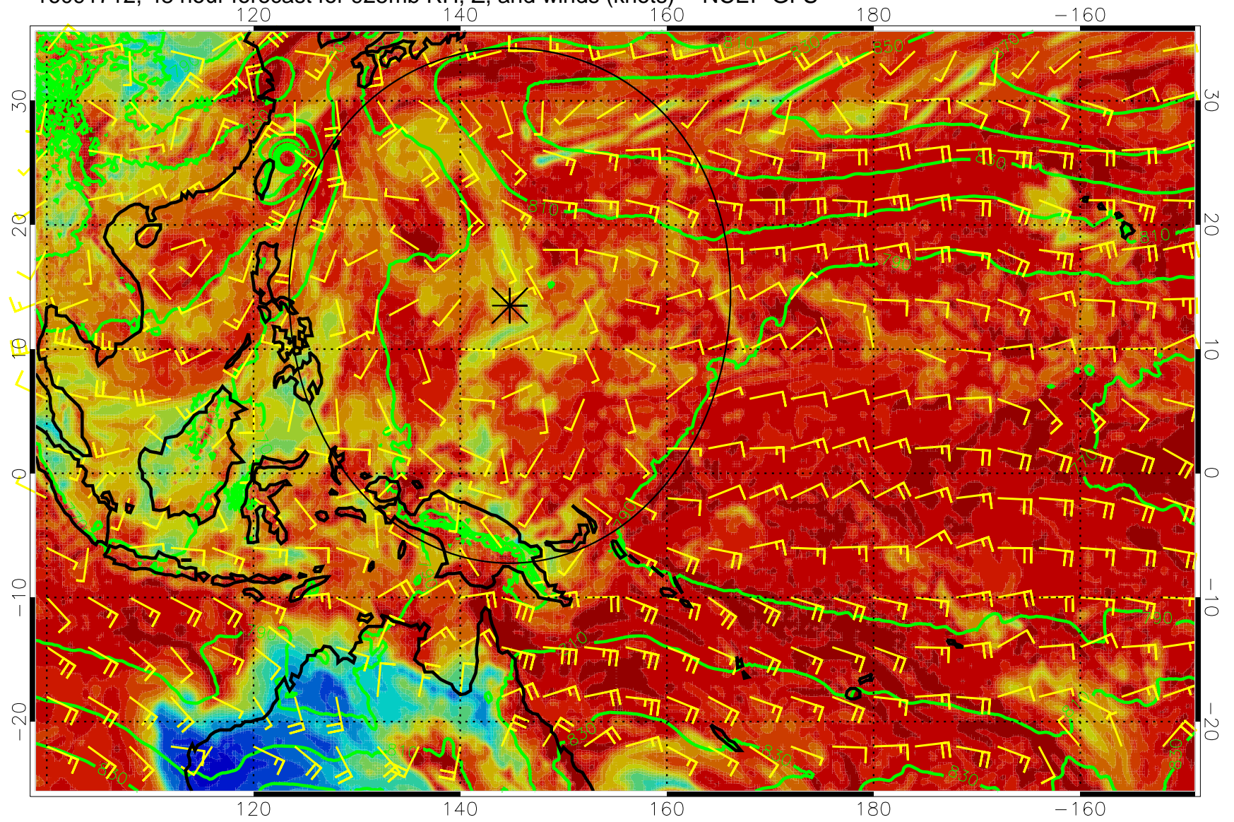
16091712, 48 hour forecast for 925mb RH, Z, and winds (knots) -- NCEP GFS
