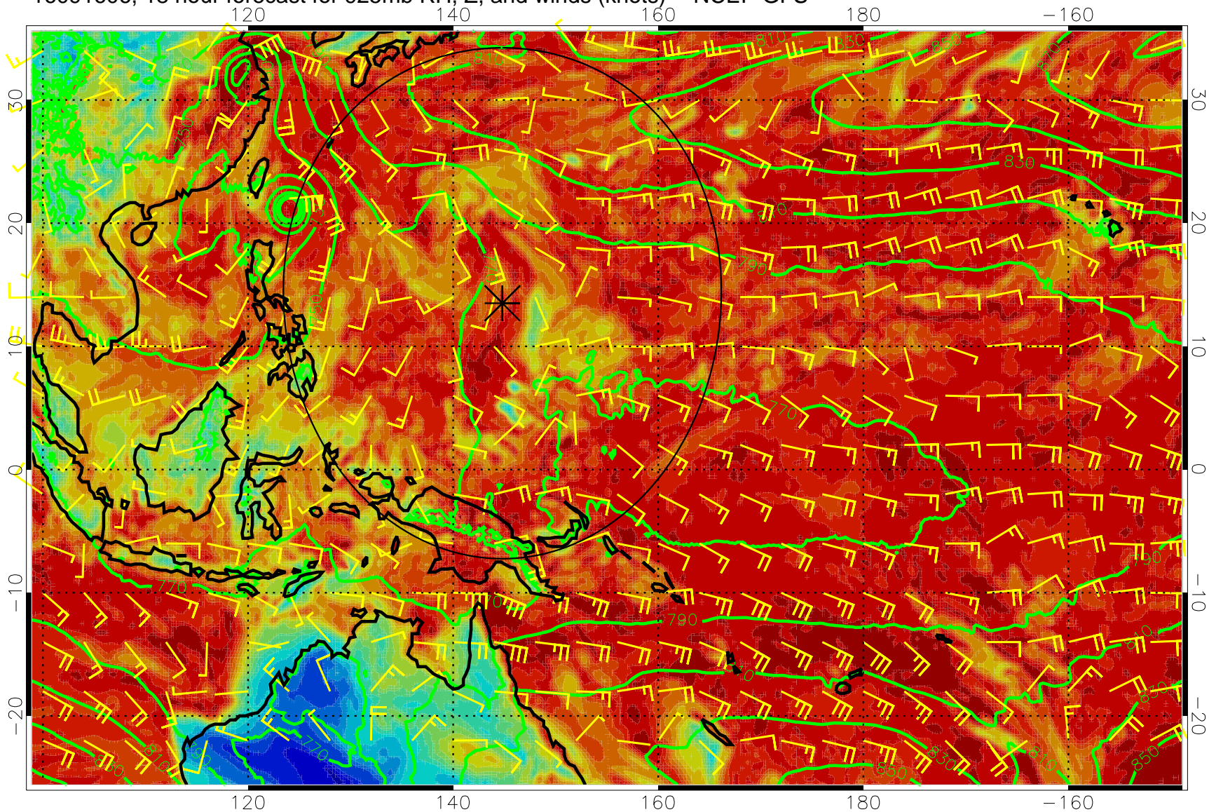
16091606, 18 hour forecast for 925mb RH, Z, and winds (knots) -- NCEP GFS
