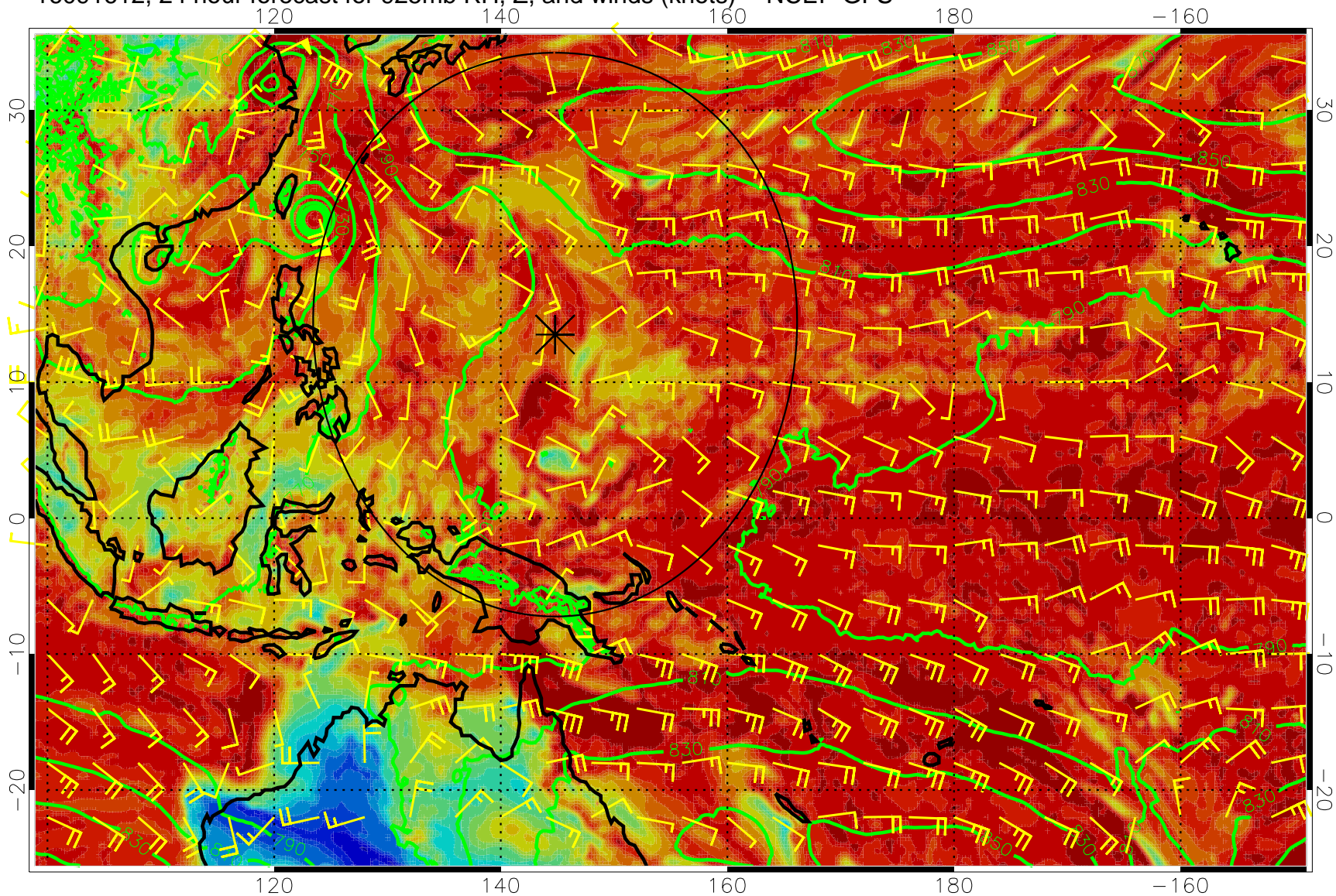
16091612, 24 hour forecast for 925mb RH, Z, and winds (knots) -- NCEP GFS
