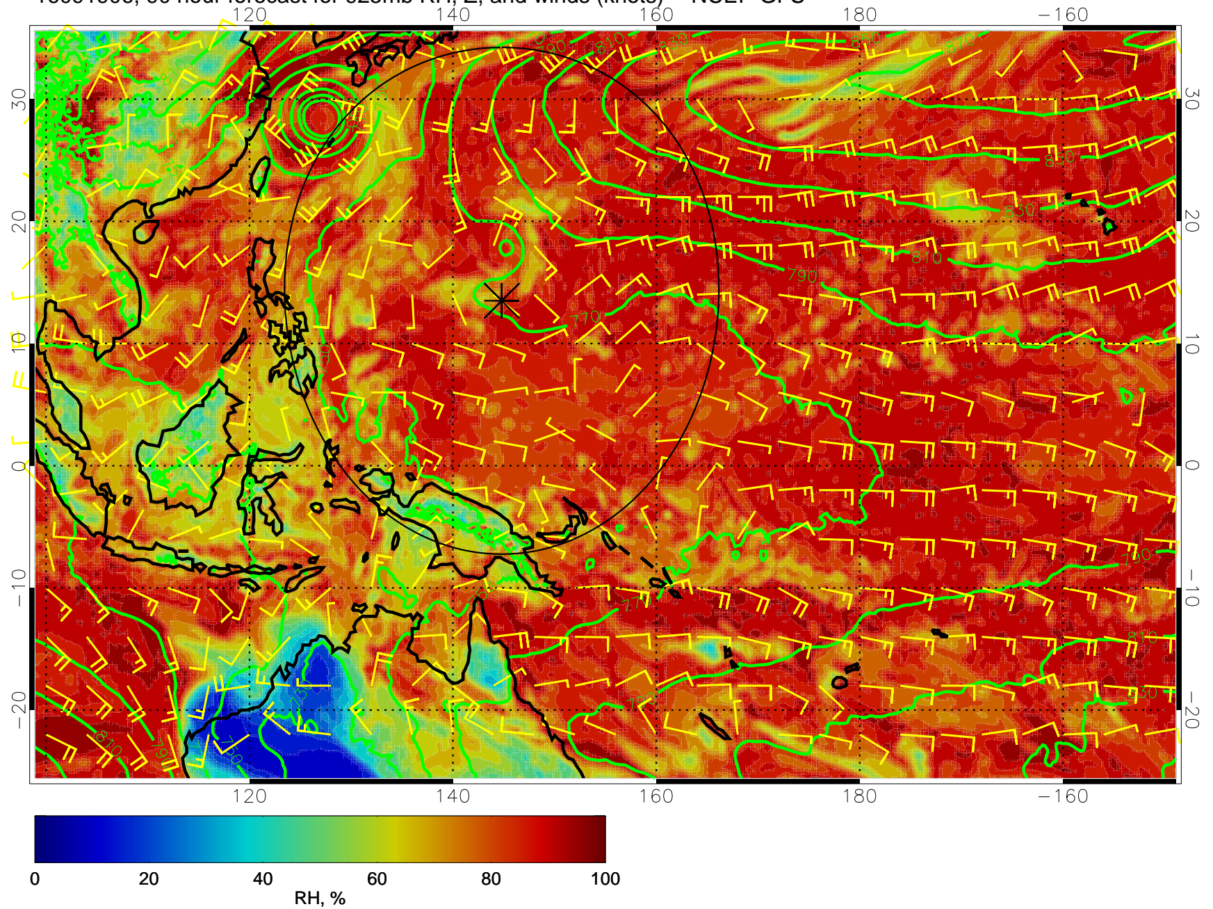
16091906, 90 hour forecast for 925mb RH, Z, and winds (knots) -- NCEP GFS
