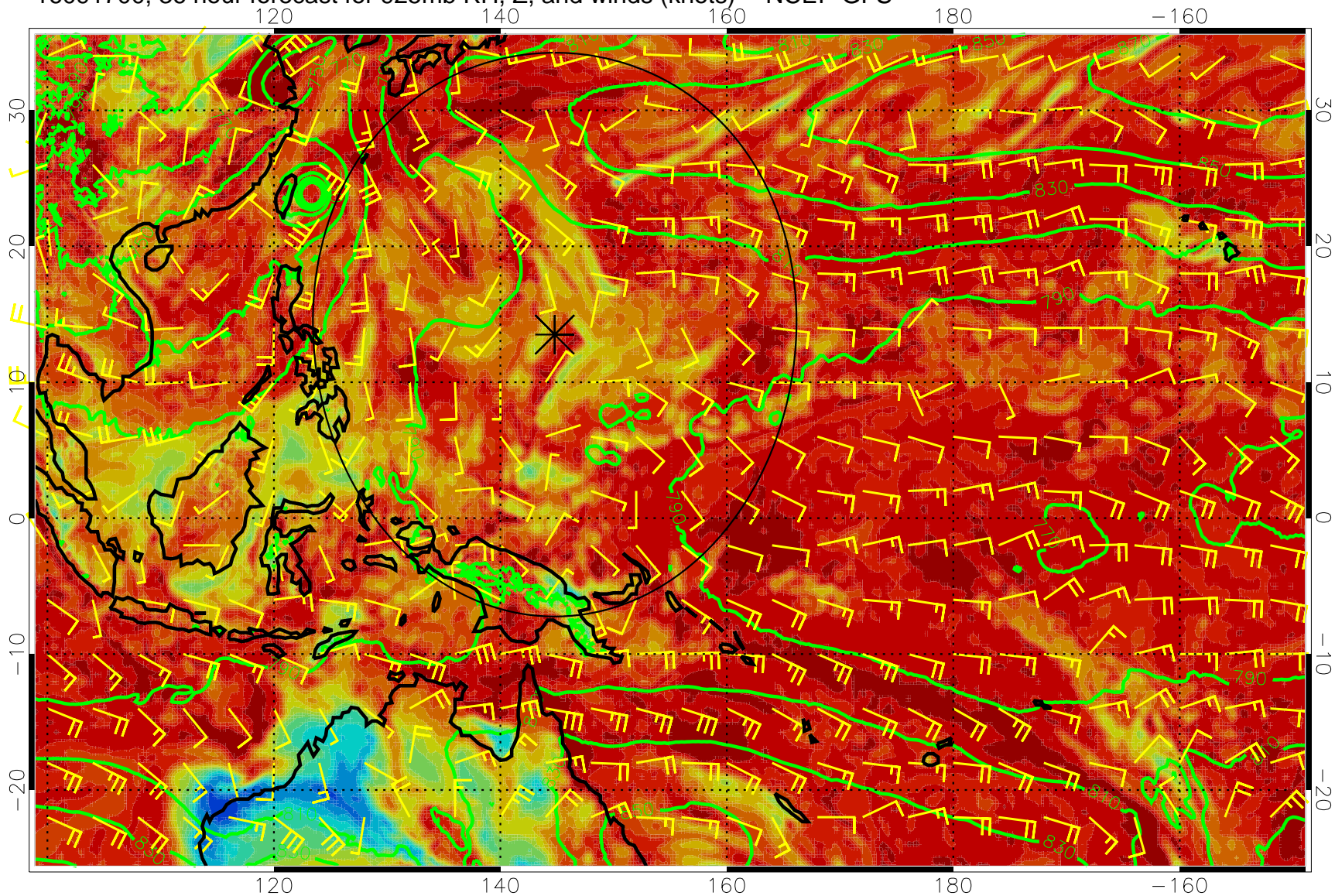
16091700, 36 hour forecast for 925mb RH, Z, and winds (knots) -- NCEP GFS
