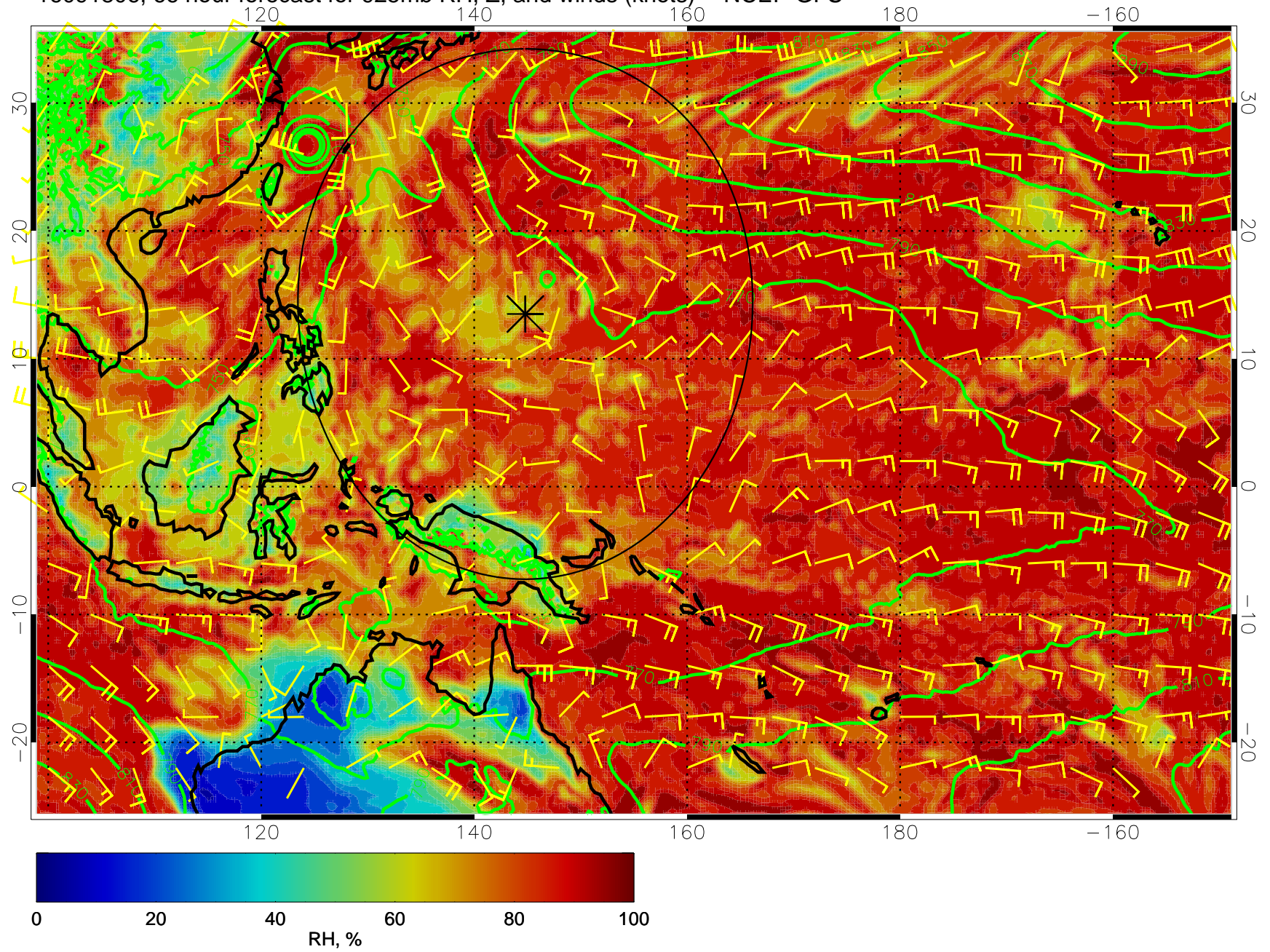
16091806, 66 hour forecast for 925mb RH, Z, and winds (knots) -- NCEP GFS
