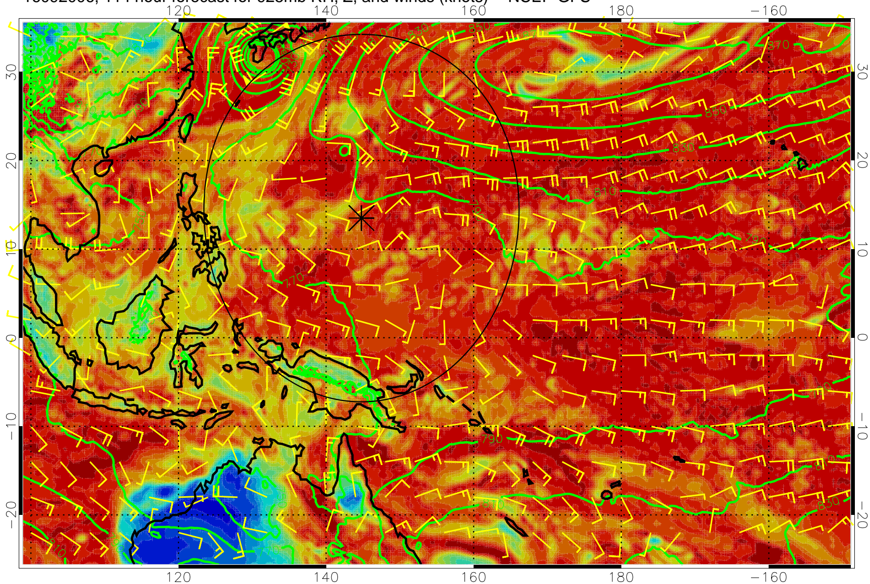
16092006, 114 hour forecast for 925mb RH, Z, and winds (knots) -- NCEP GFS
