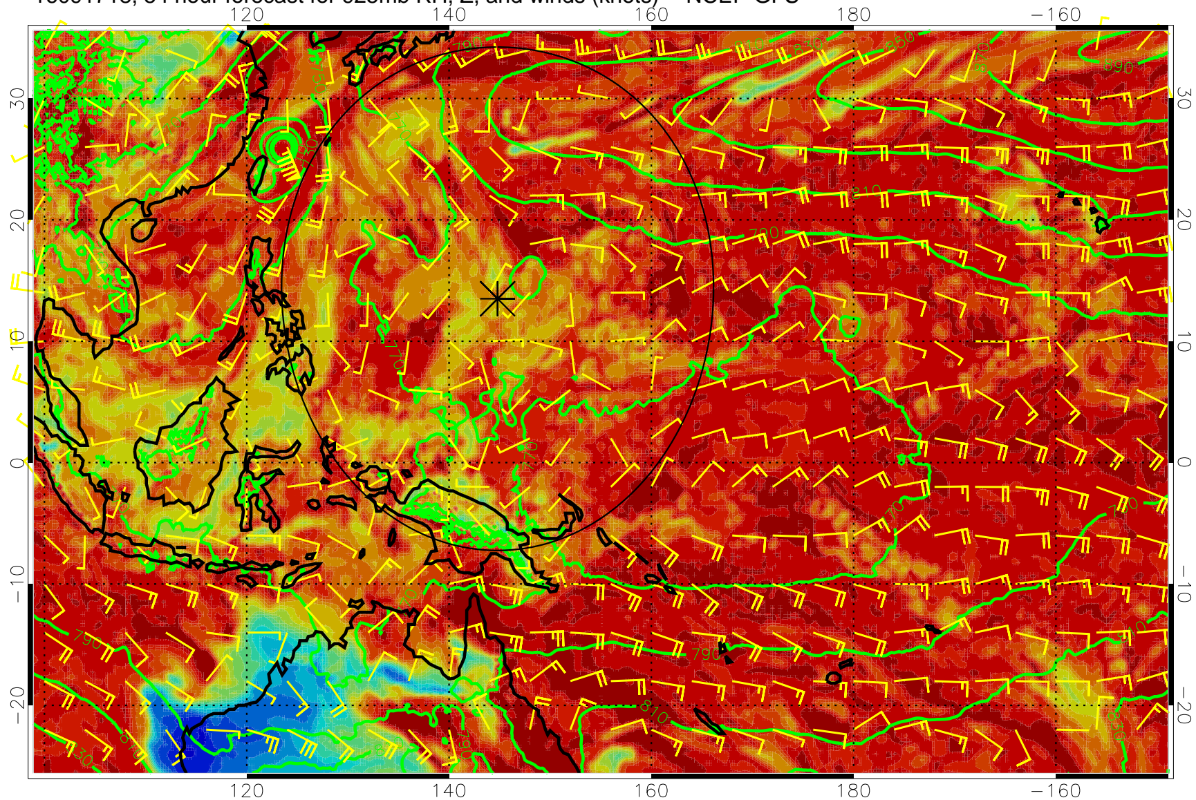
16091718, 54 hour forecast for 925mb RH, Z, and winds (knots) -- NCEP GFS
