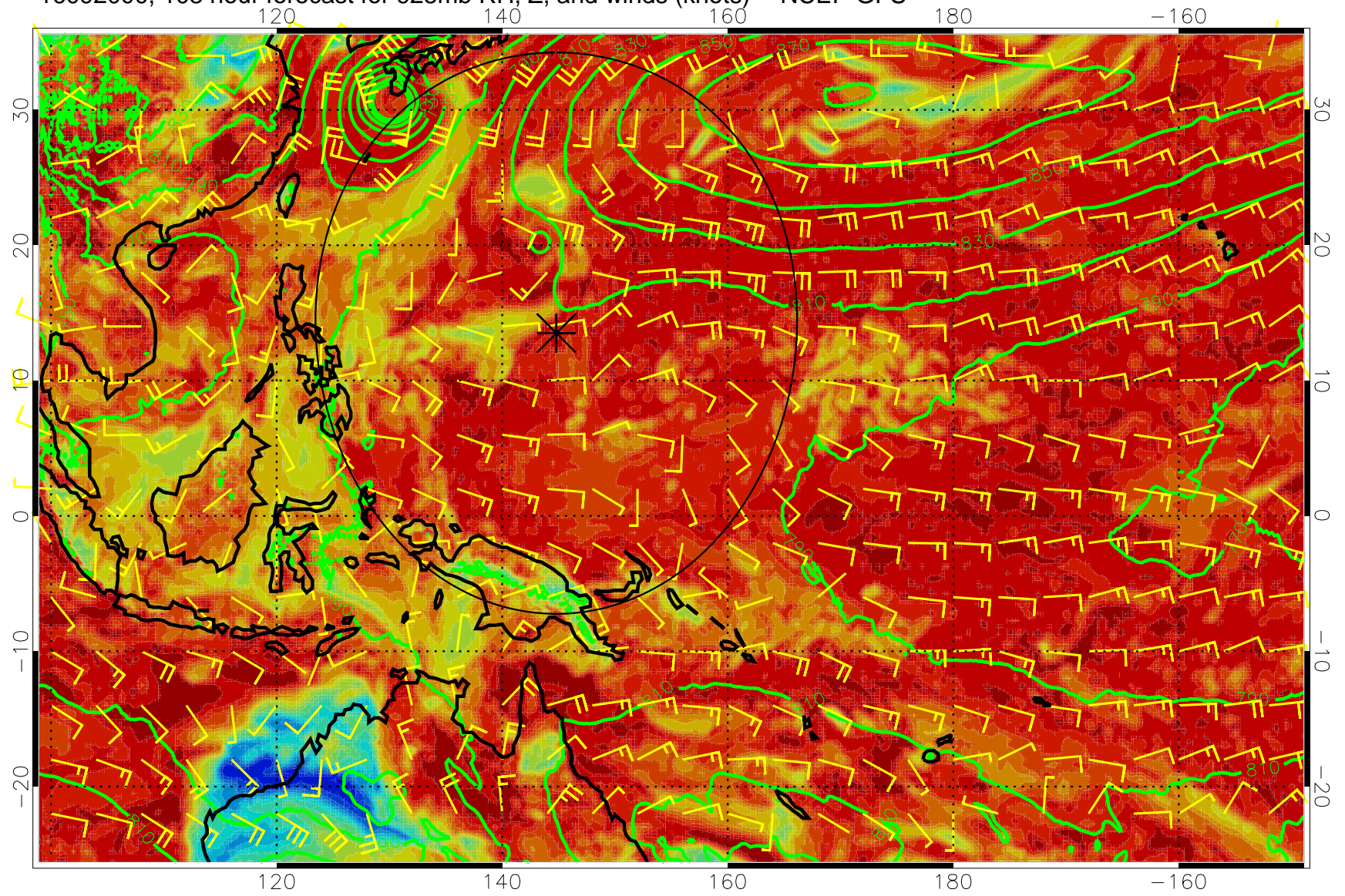
16092000, 108 hour forecast for 925mb RH, Z, and winds (knots) -- NCEP GFS
