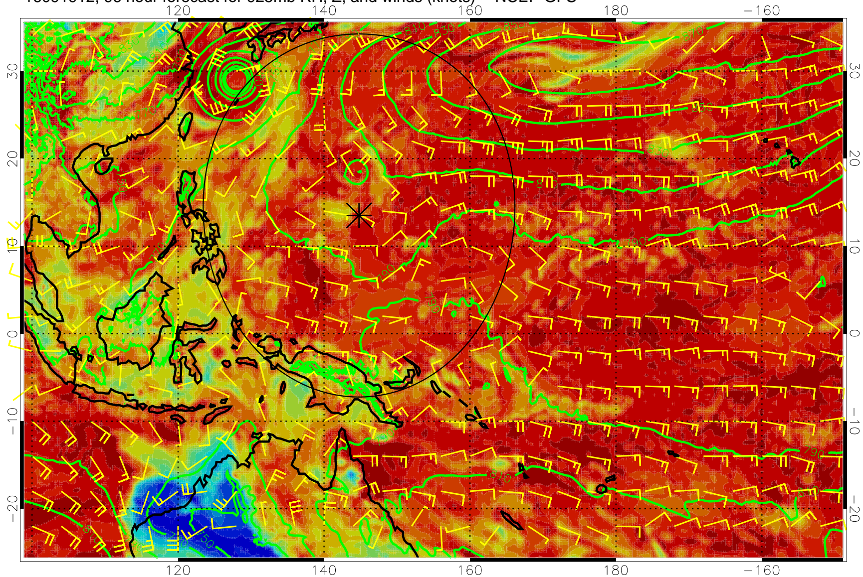
16091912, 96 hour forecast for 925mb RH, Z, and winds (knots) -- NCEP GFS
