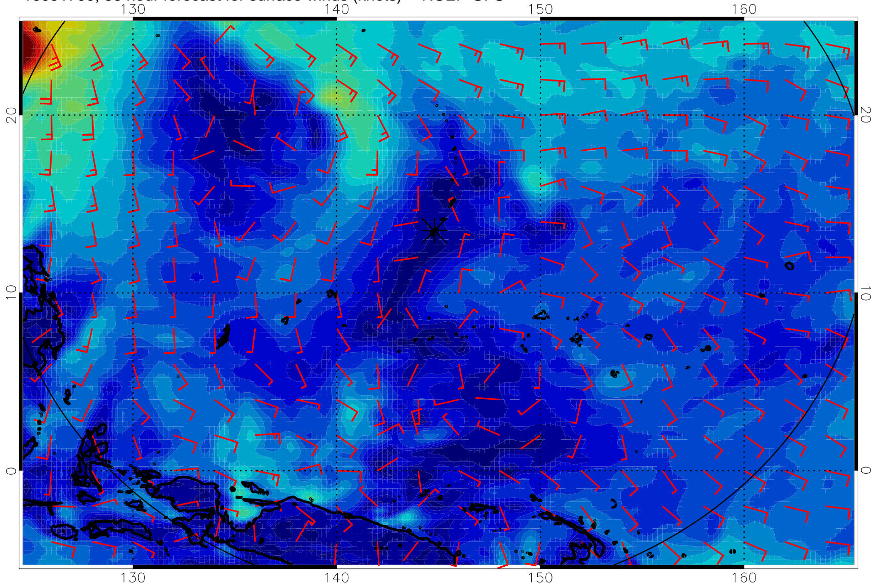
16091700, 36 hour forecast for surface winds (knots) -- NCEP GFS
