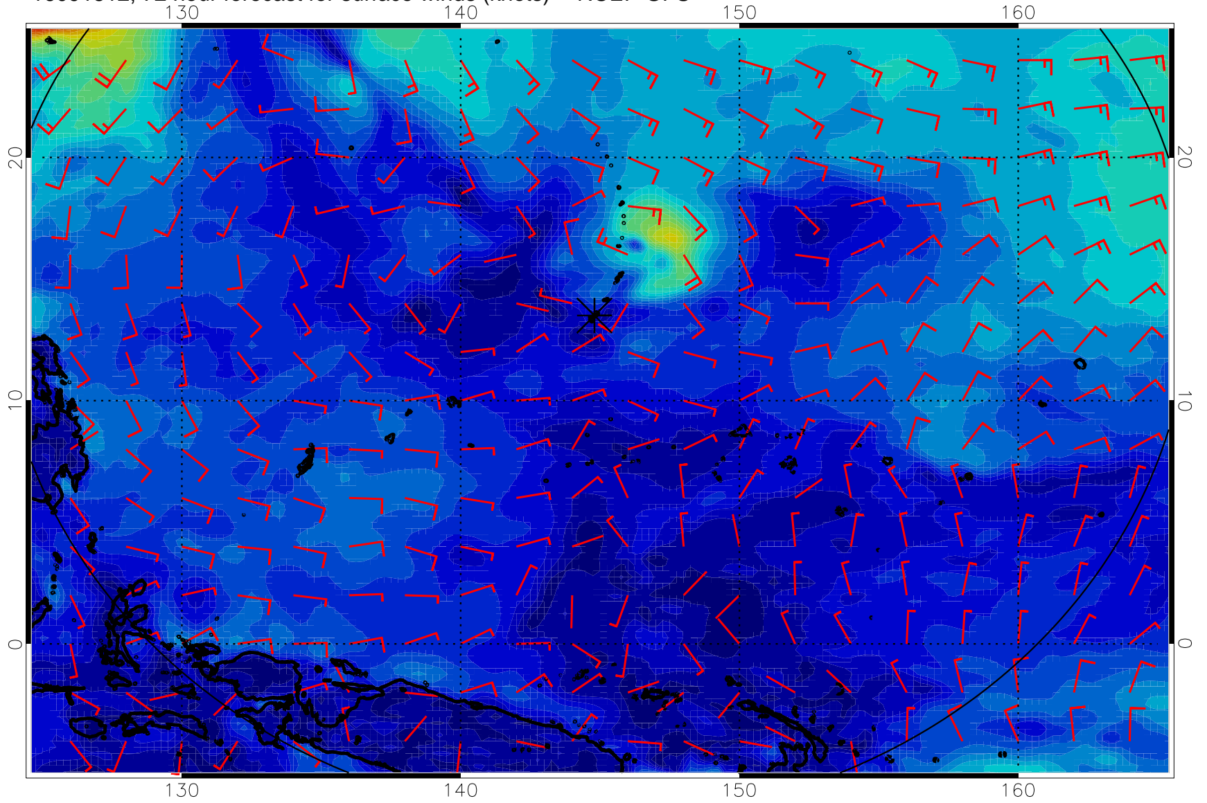
16091812, 72 hour forecast for surface winds (knots) -- NCEP GFS
