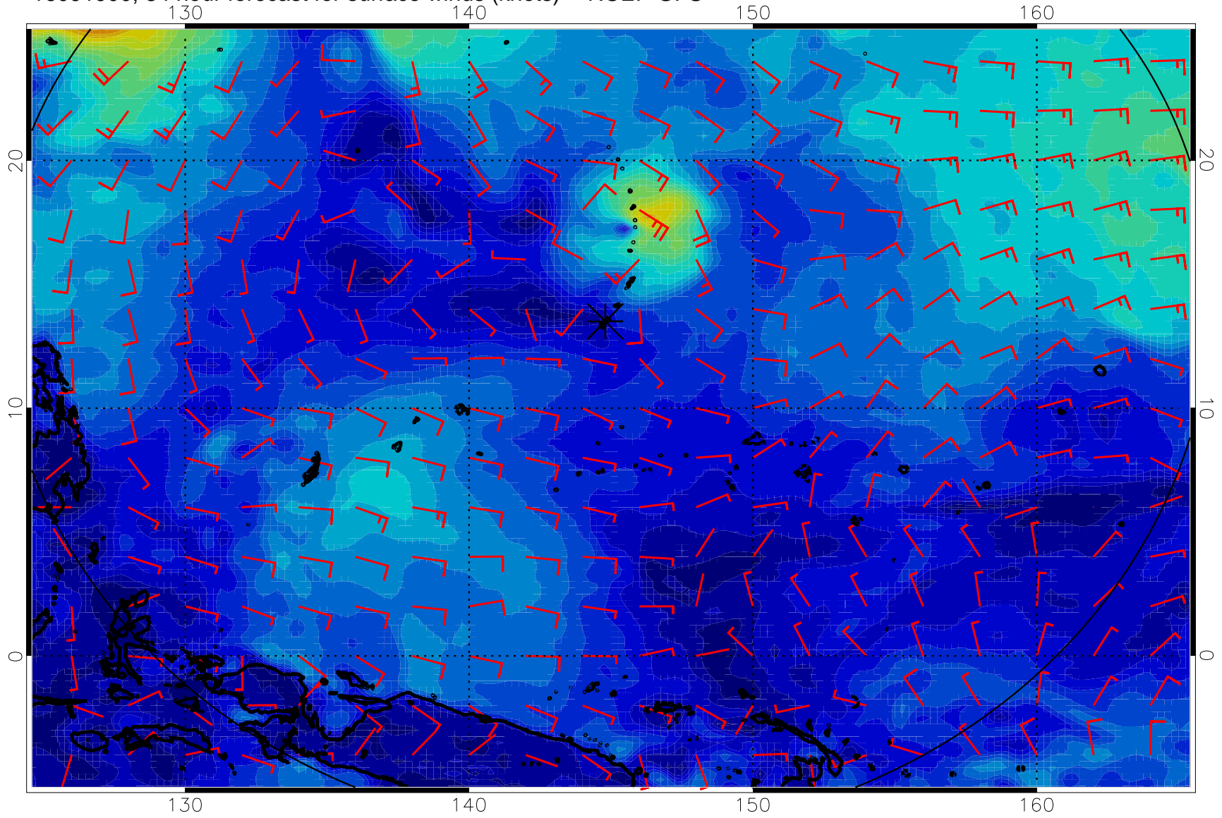
16091900, 84 hour forecast for surface winds (knots) -- NCEP GFS
