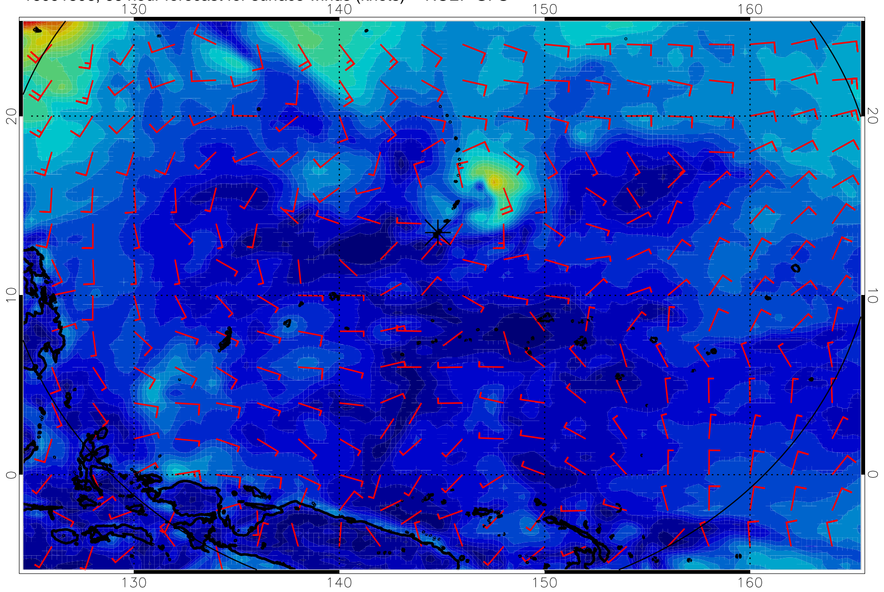
16091806, 66 hour forecast for surface winds (knots) -- NCEP GFS
