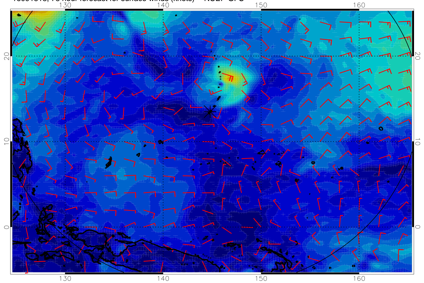
16091818, 78 hour forecast for surface winds (knots) -- NCEP GFS
