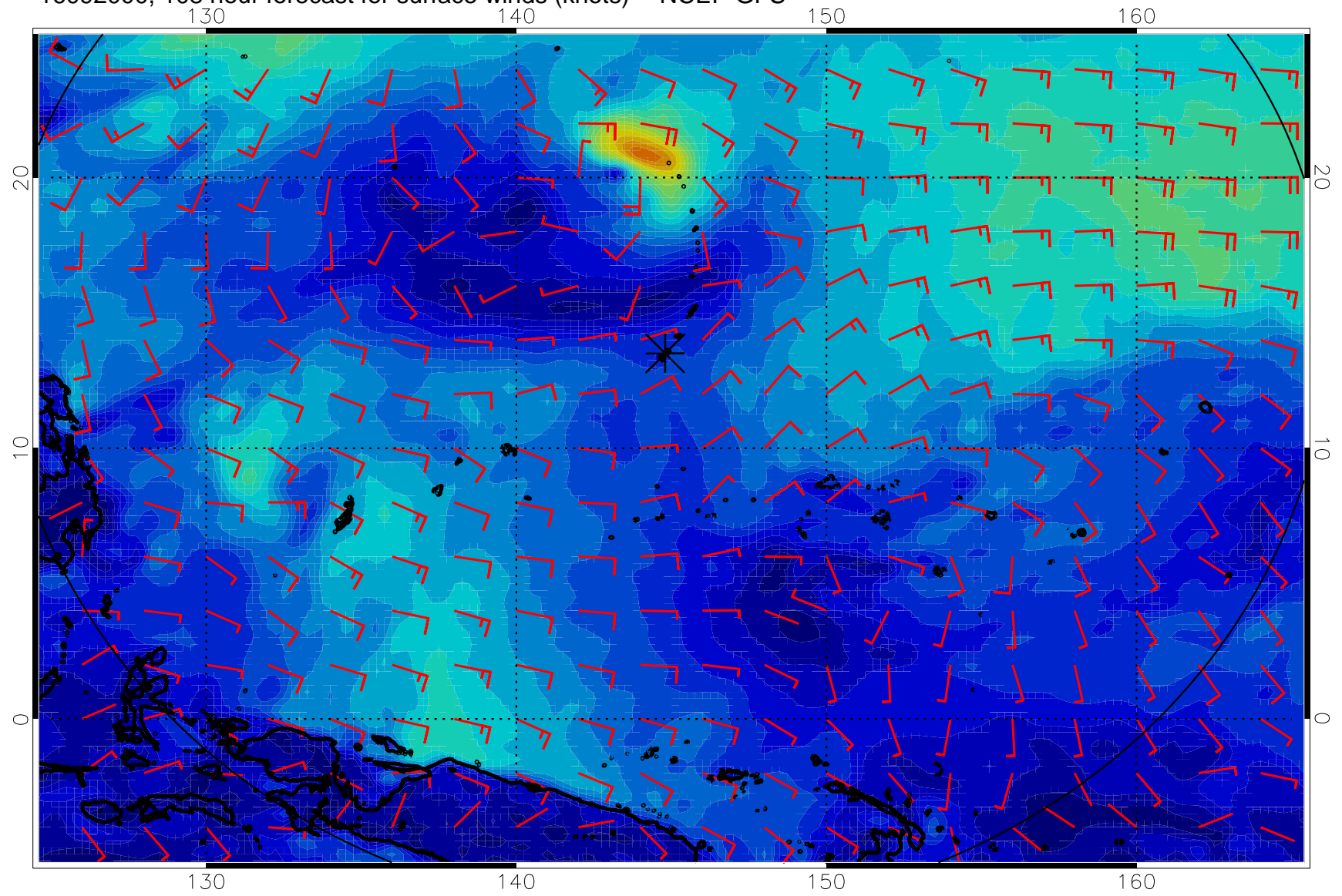
16092000, 108 hour forecast for surface winds (knots) -- NCEP GFS
