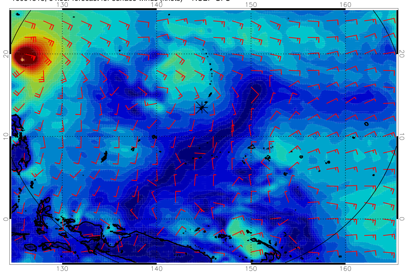
16091518, 6 hour forecast for surface winds (knots) -- NCEP GFS
