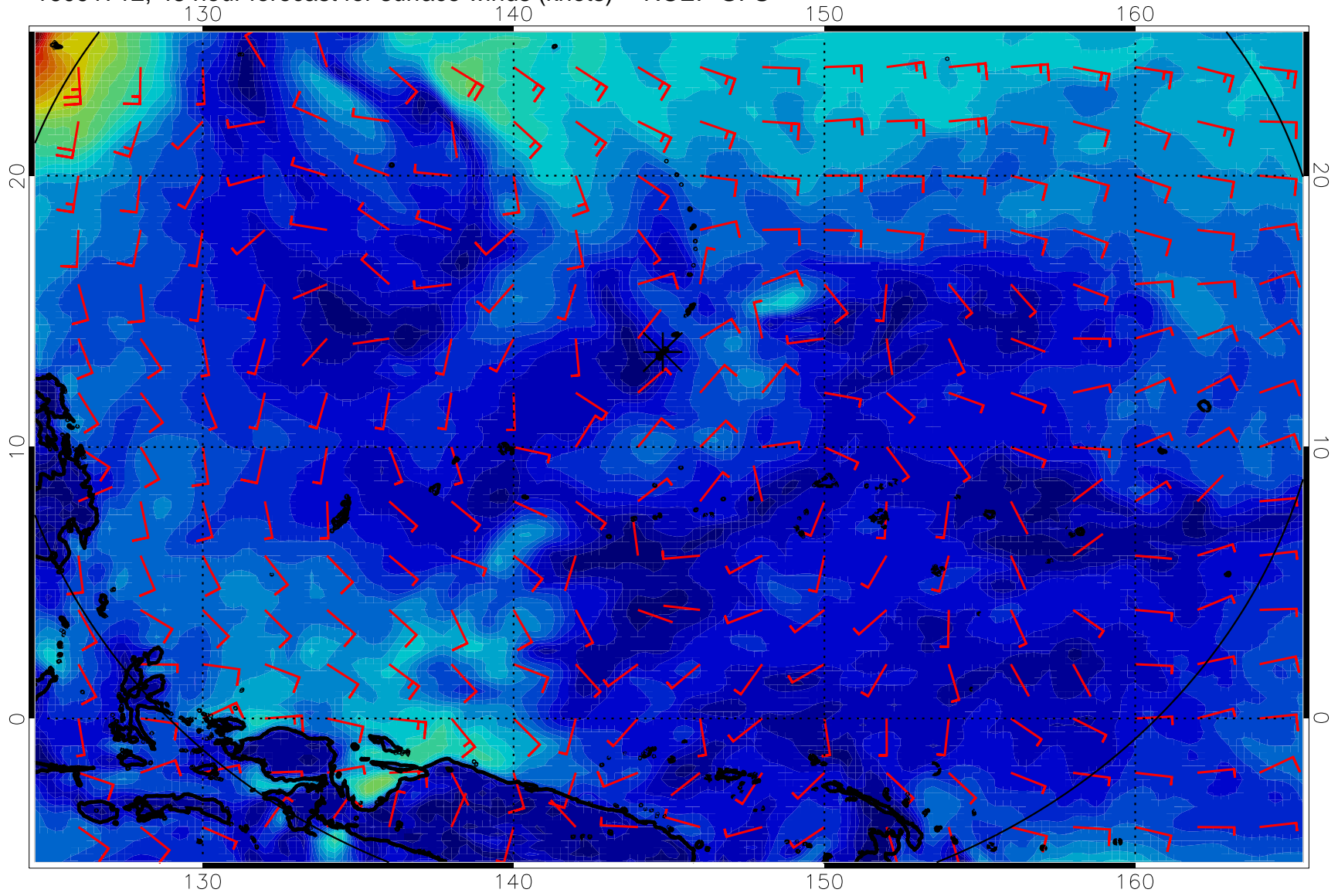
16091712, 48 hour forecast for surface winds (knots) -- NCEP GFS
