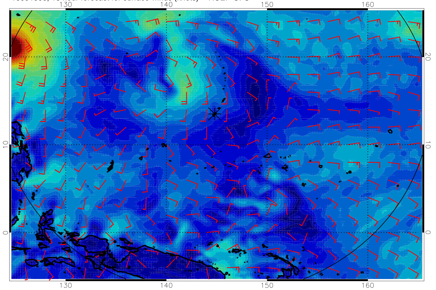
16091606, 18 hour forecast for surface winds (knots) -- NCEP GFS
