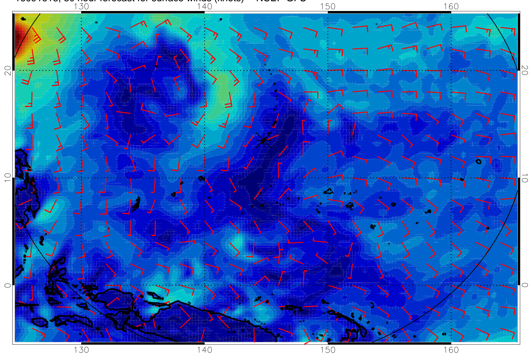
16091618, 30 hour forecast for surface winds (knots) -- NCEP GFS
