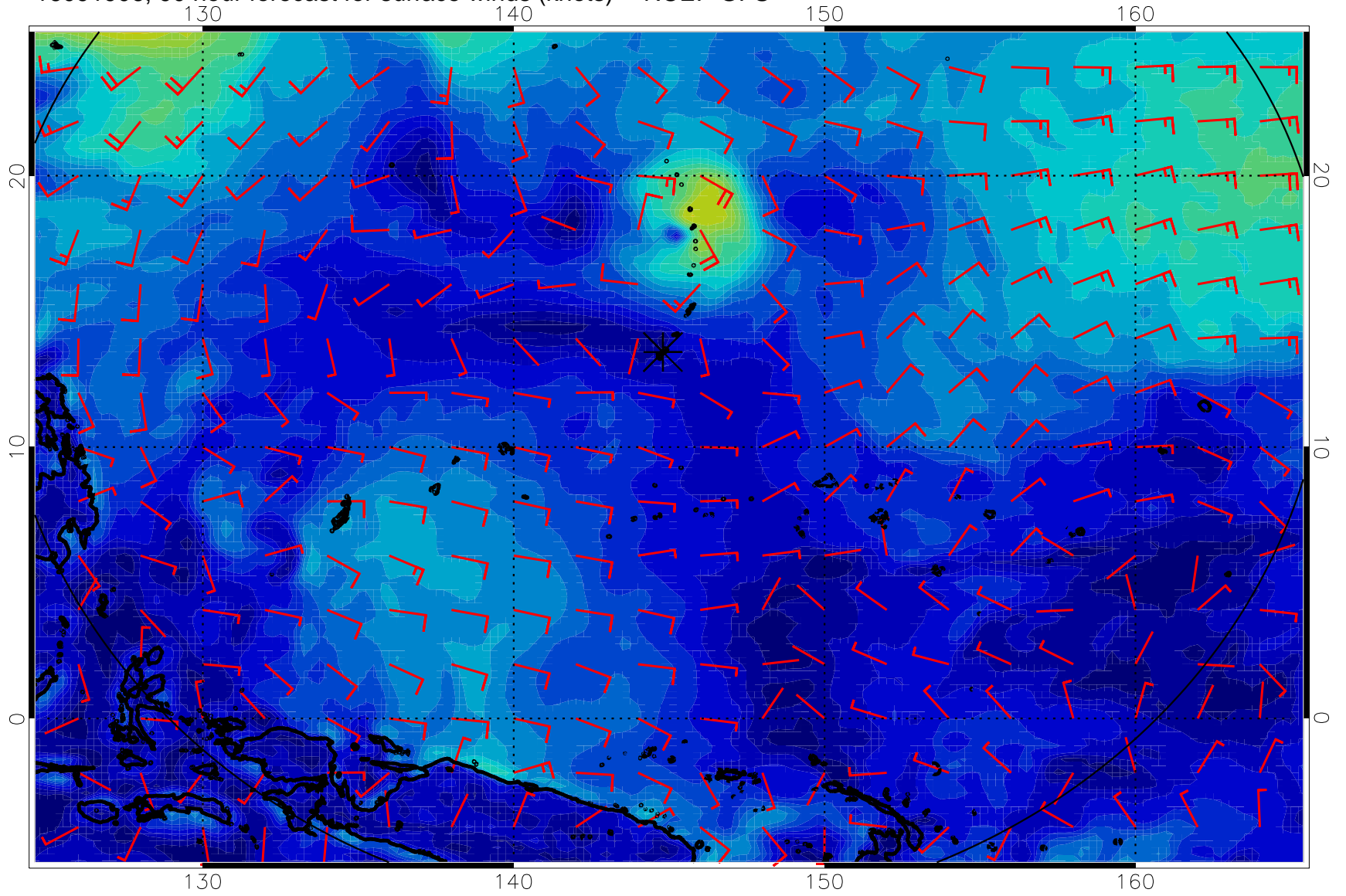
16091906, 90 hour forecast for surface winds (knots) -- NCEP GFS
