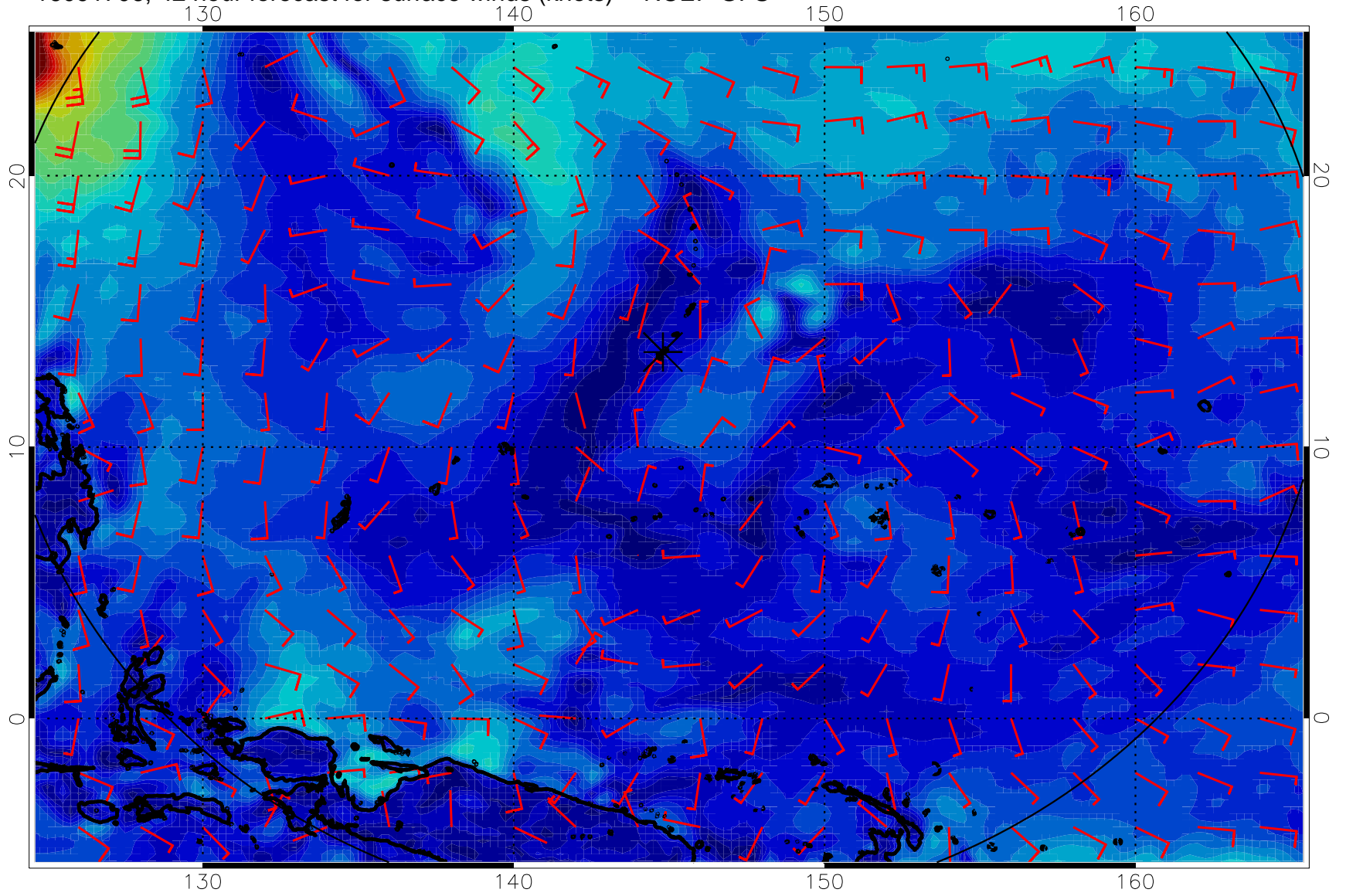
16091706, 42 hour forecast for surface winds (knots) -- NCEP GFS
