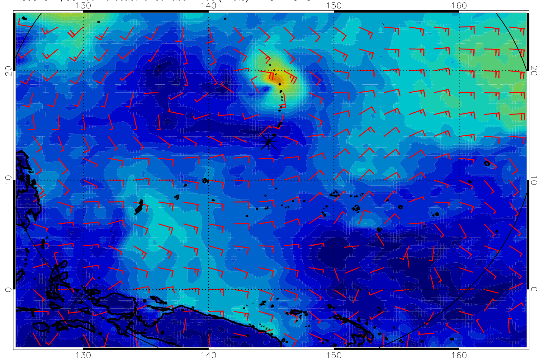
16091912, 96 hour forecast for surface winds (knots) -- NCEP GFS
