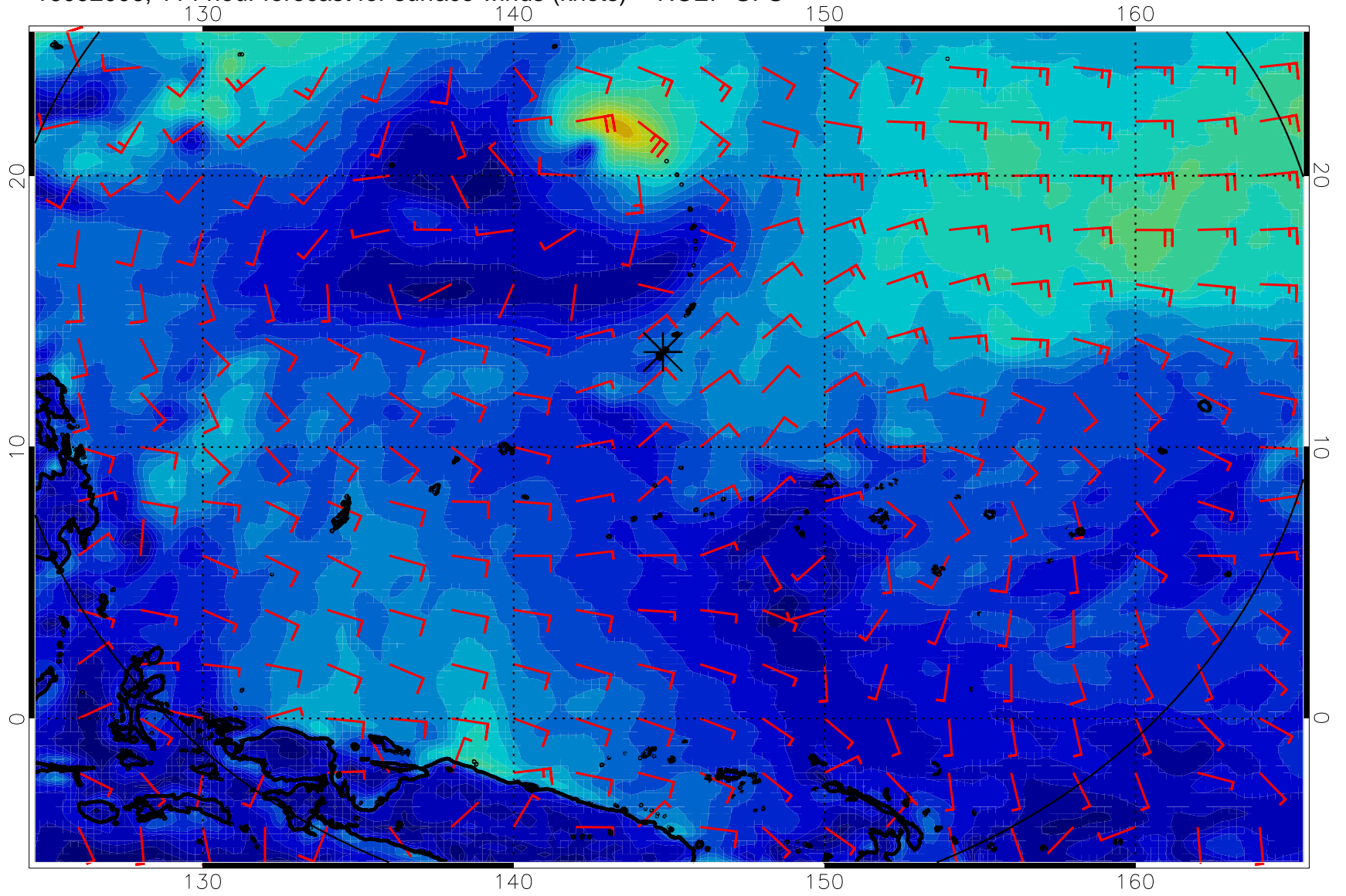
16092006, 114 hour forecast for surface winds (knots) -- NCEP GFS
