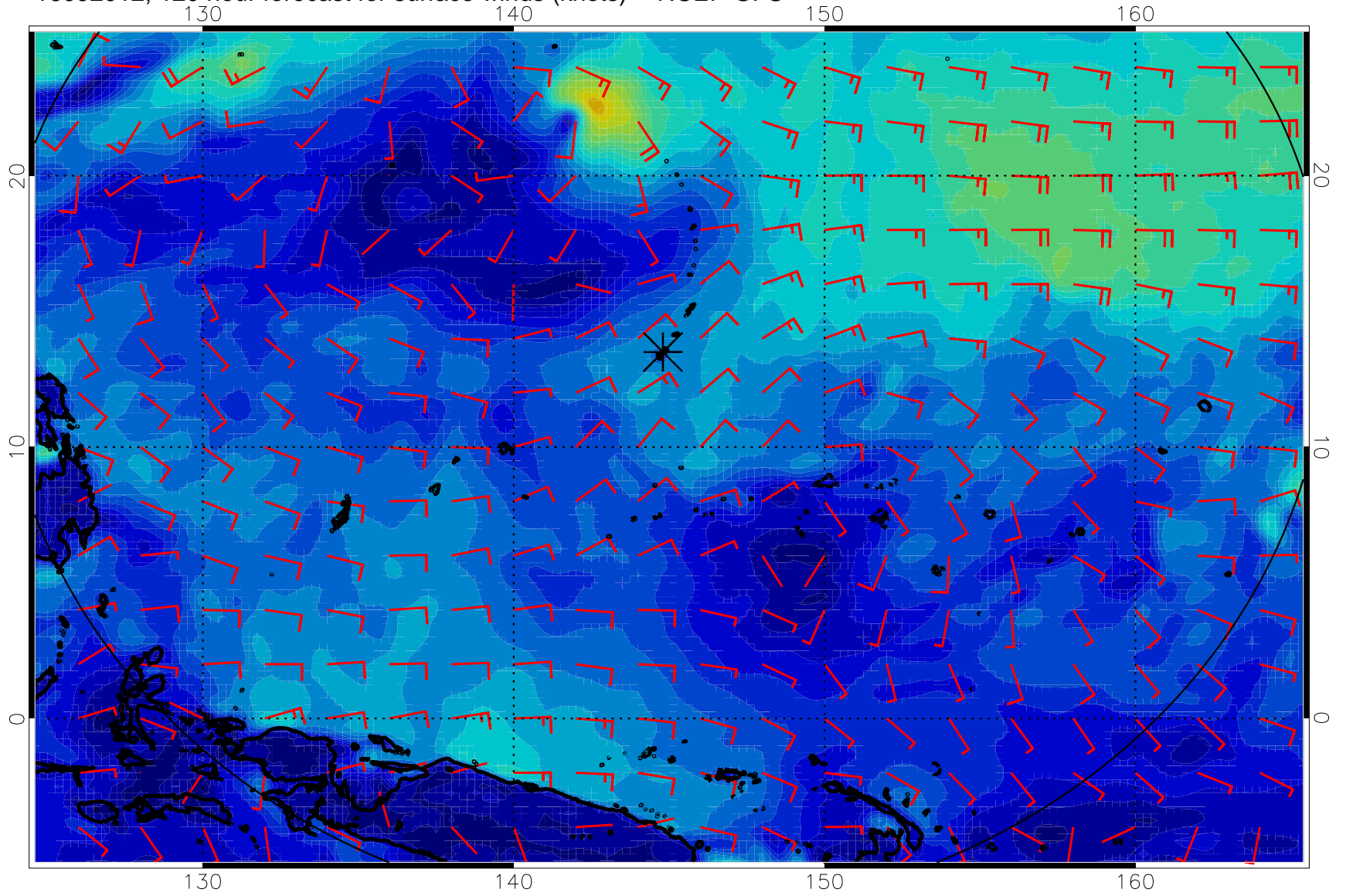
16092012, 120 hour forecast for surface winds (knots) -- NCEP GFS
