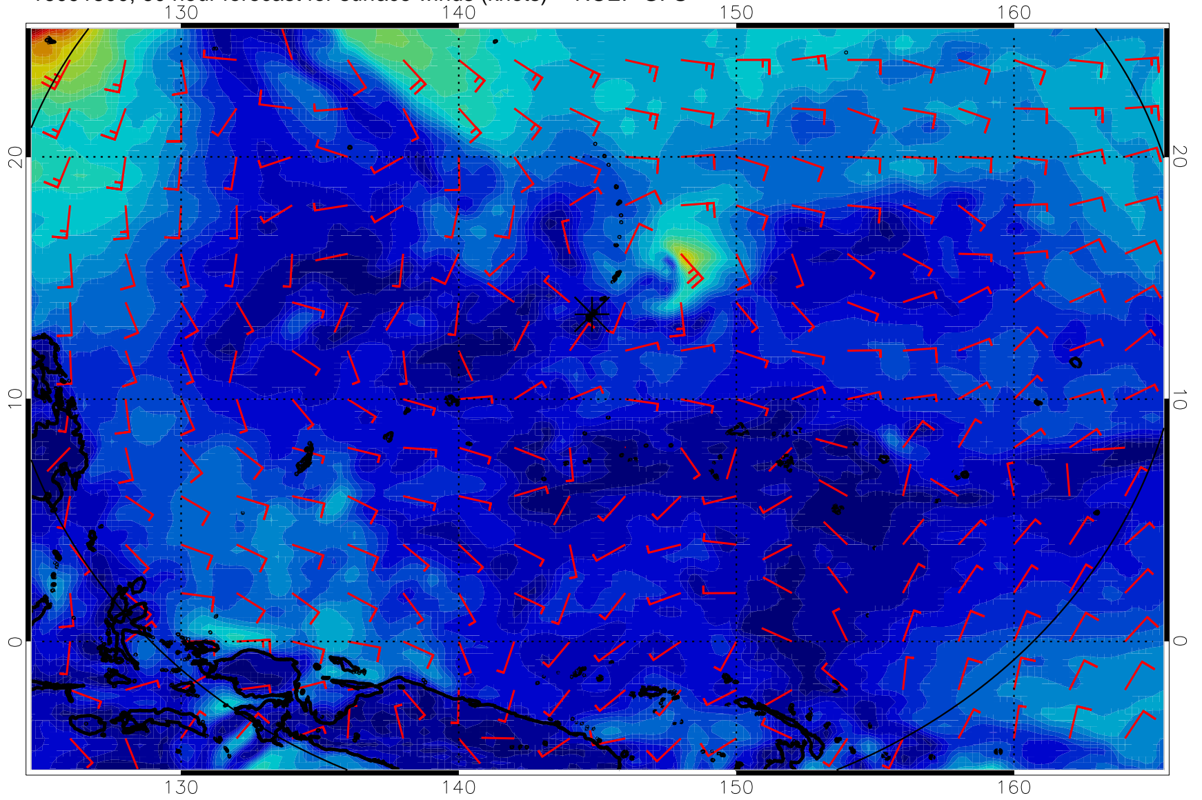
16091800, 60 hour forecast for surface winds (knots) -- NCEP GFS
