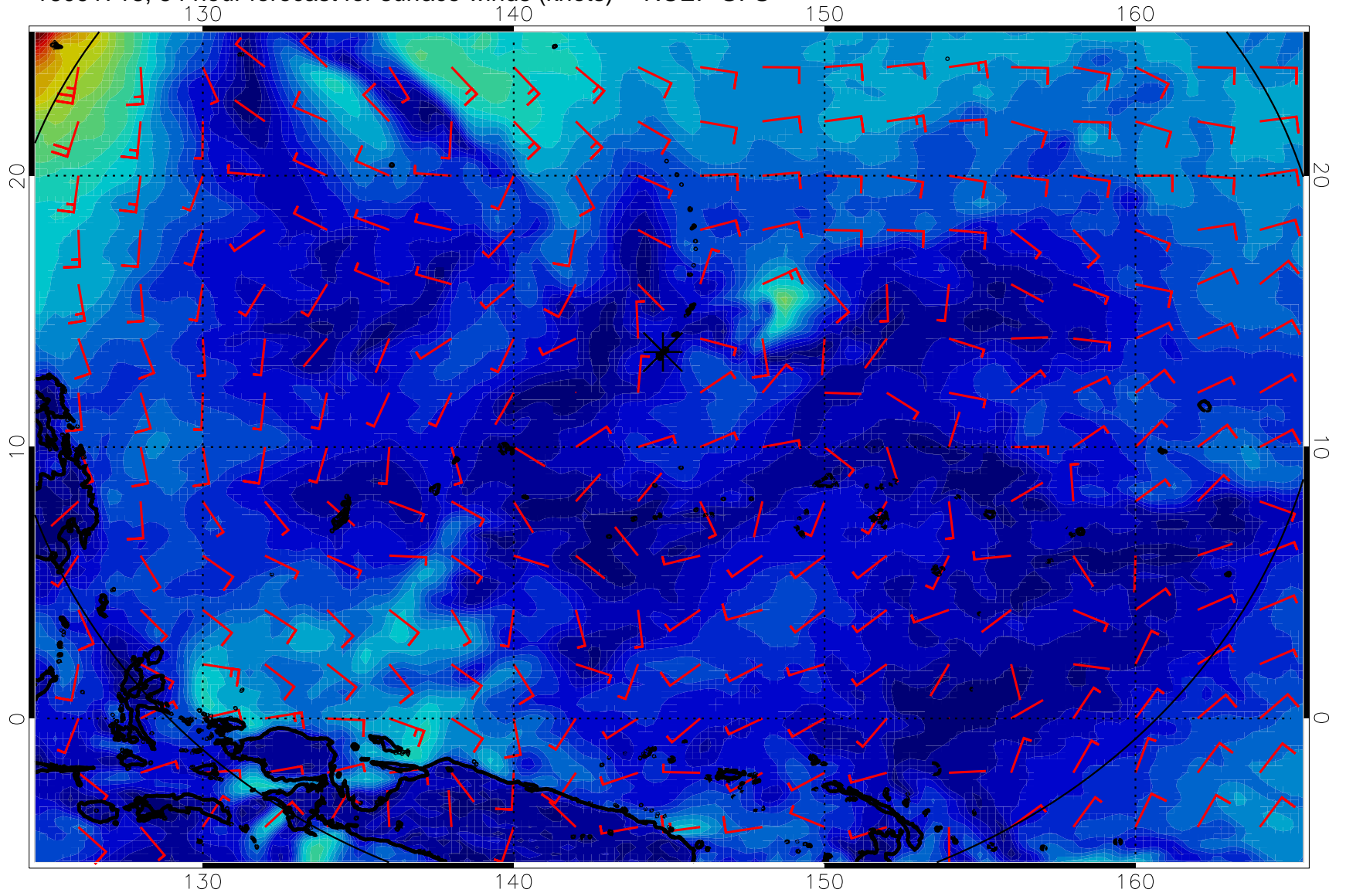
16091718, 54 hour forecast for surface winds (knots) -- NCEP GFS
