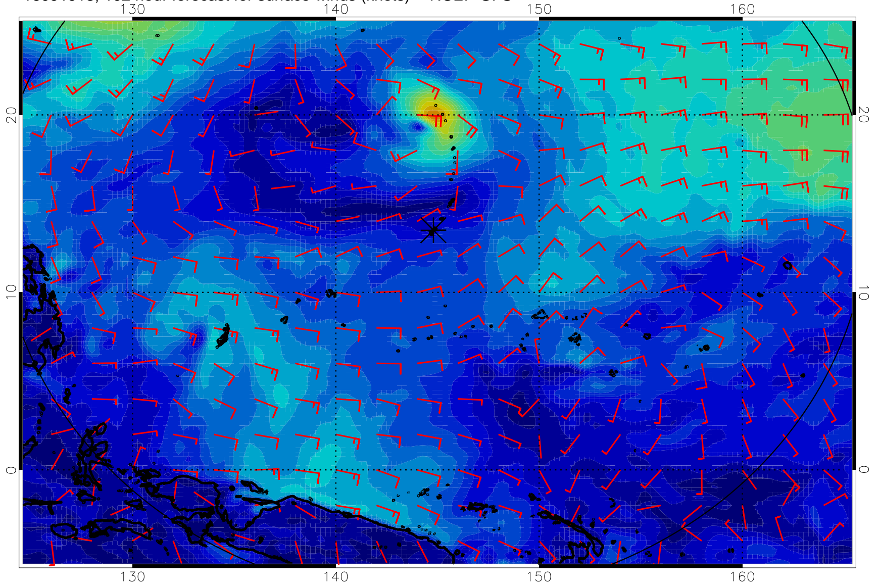
16091918, 102 hour forecast for surface winds (knots) -- NCEP GFS
