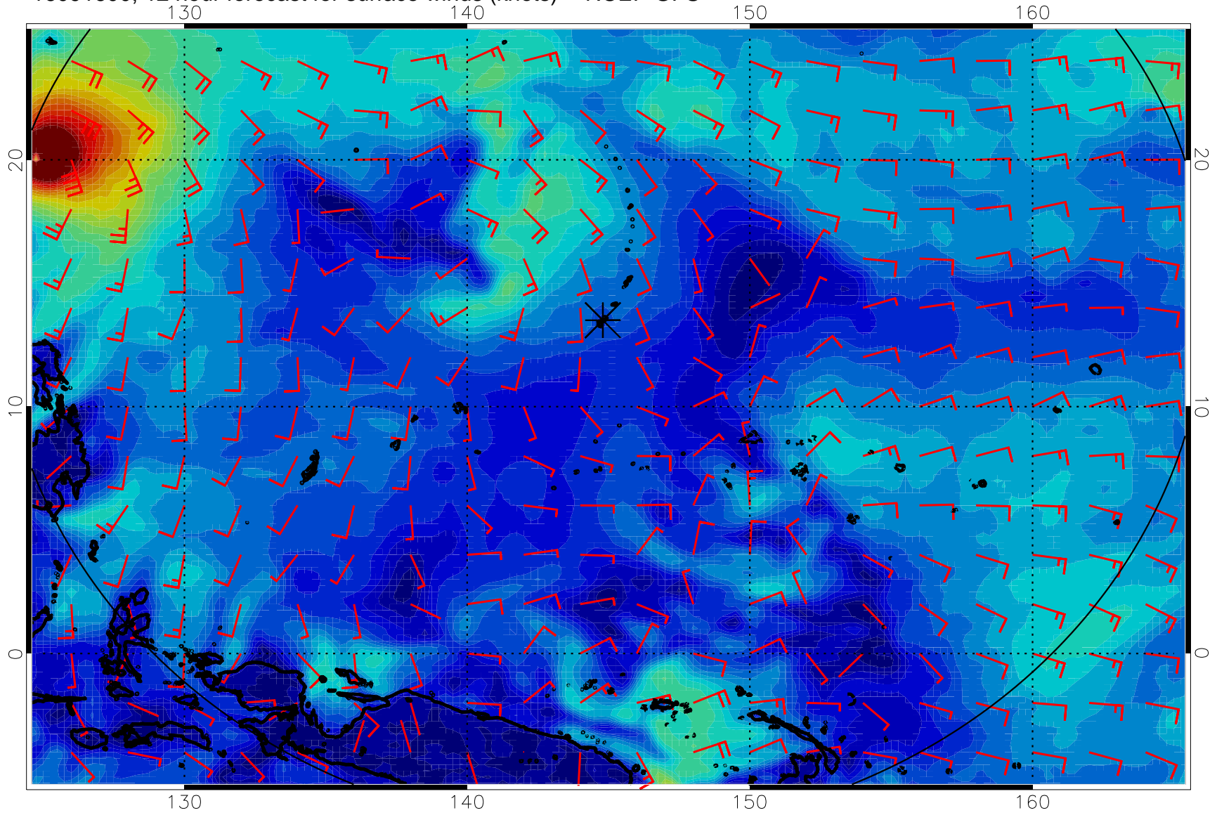
16091600, 12 hour forecast for surface winds (knots) -- NCEP GFS
