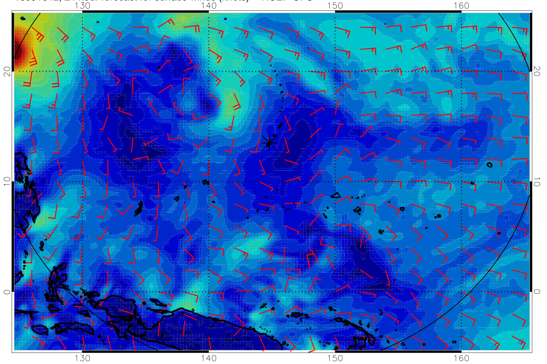
16091612, 24 hour forecast for surface winds (knots) -- NCEP GFS
