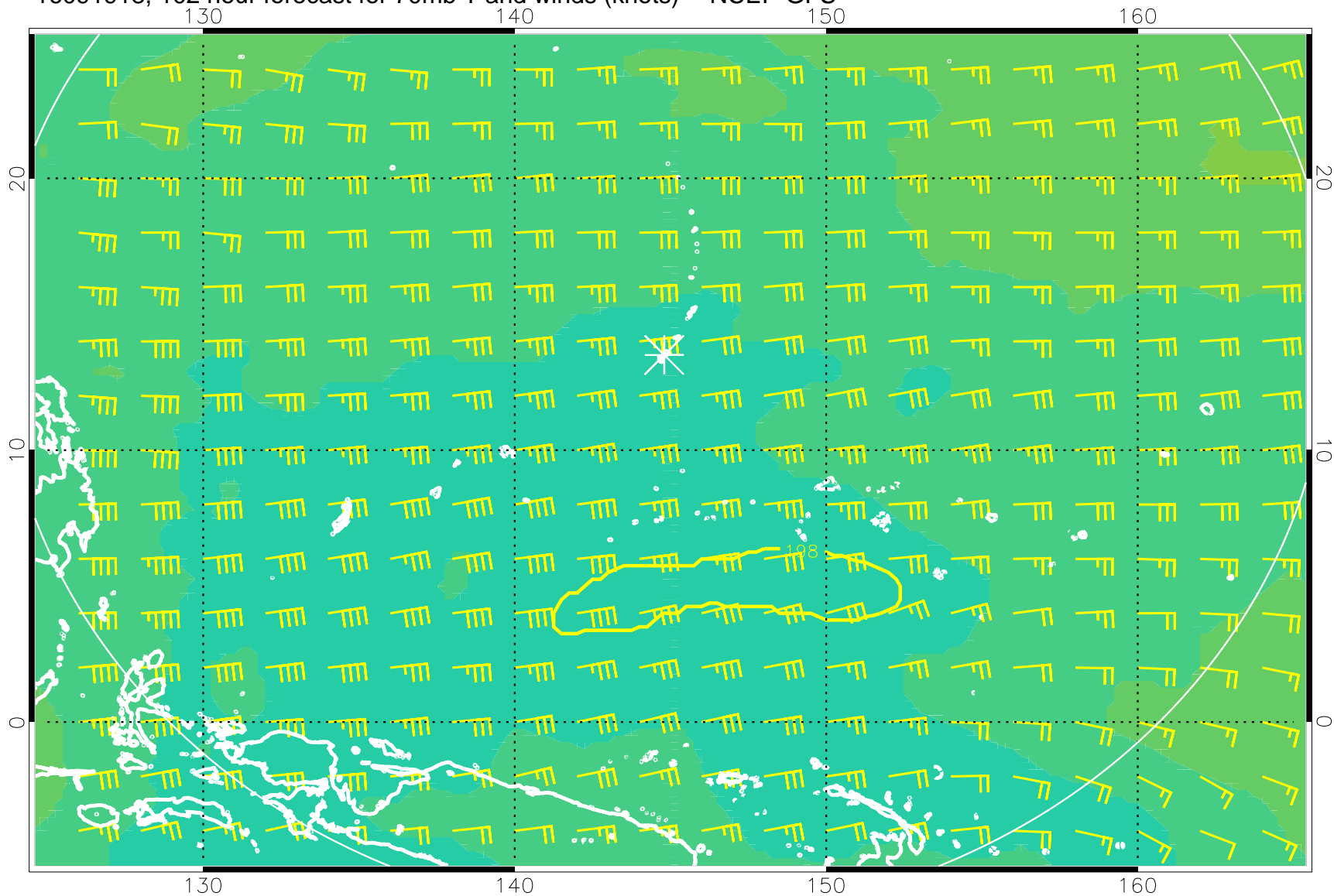
16091918, 102 hour forecast for 70mb T and winds (knots) -- NCEP GFS
