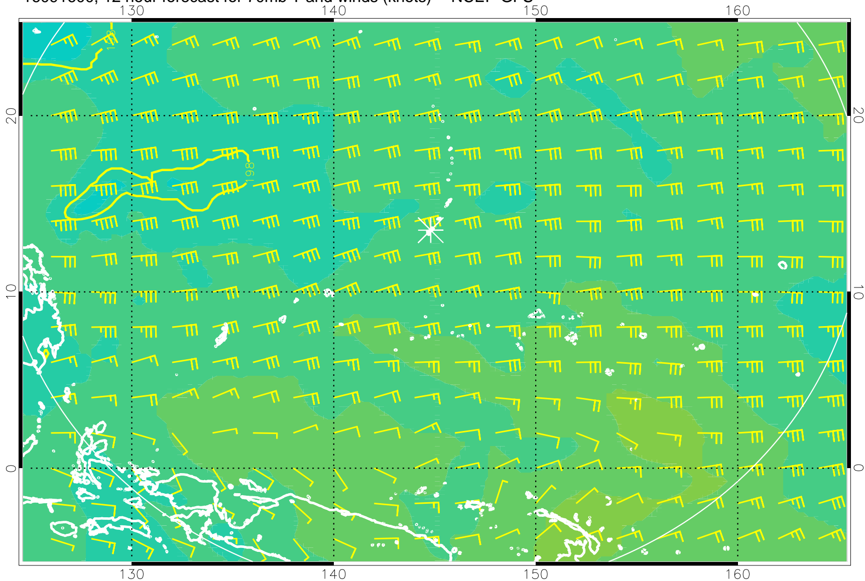
16091600, 12 hour forecast for 70mb T and winds (knots) -- NCEP GFS
