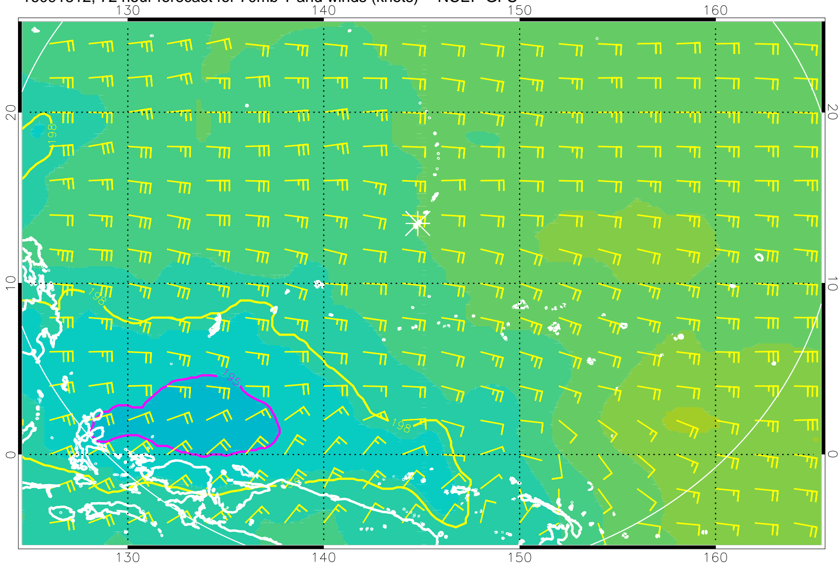
16091812, 72 hour forecast for 70mb T and winds (knots) -- NCEP GFS
