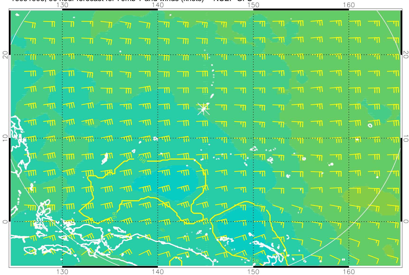
16091906, 90 hour forecast for 70mb T and winds (knots) -- NCEP GFS
