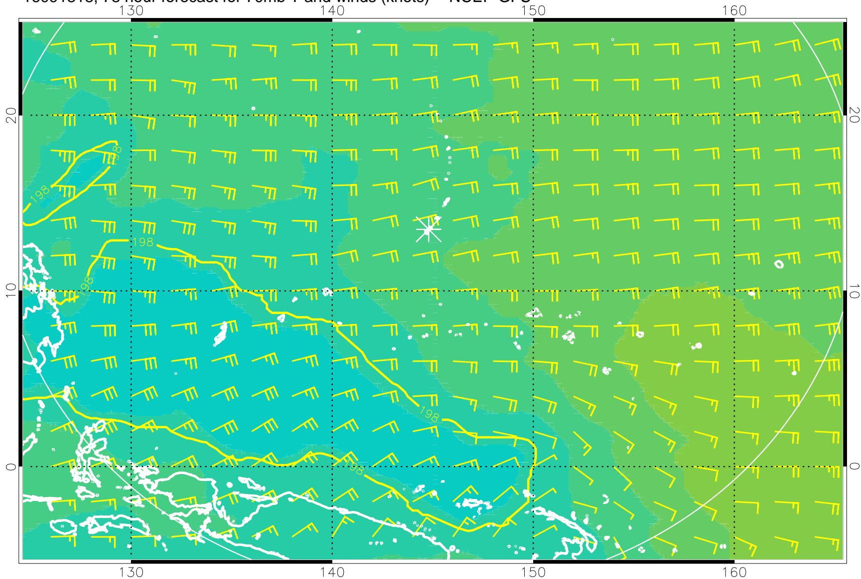
16091818, 78 hour forecast for 70mb T and winds (knots) -- NCEP GFS
