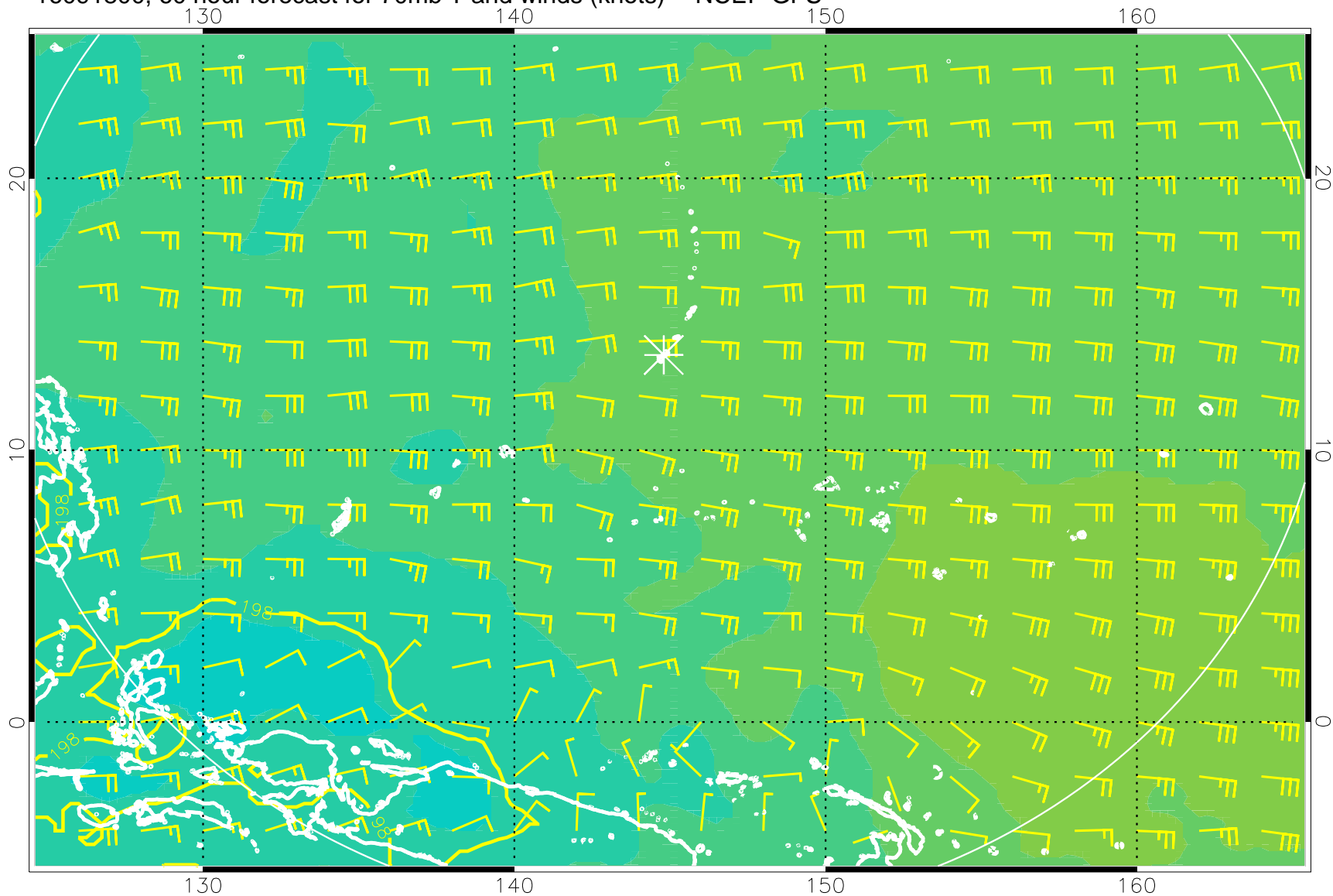
16091800, 60 hour forecast for 70mb T and winds (knots) -- NCEP GFS
