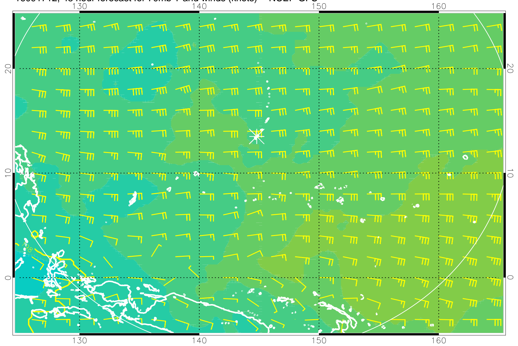
16091712, 48 hour forecast for 70mb T and winds (knots) -- NCEP GFS
