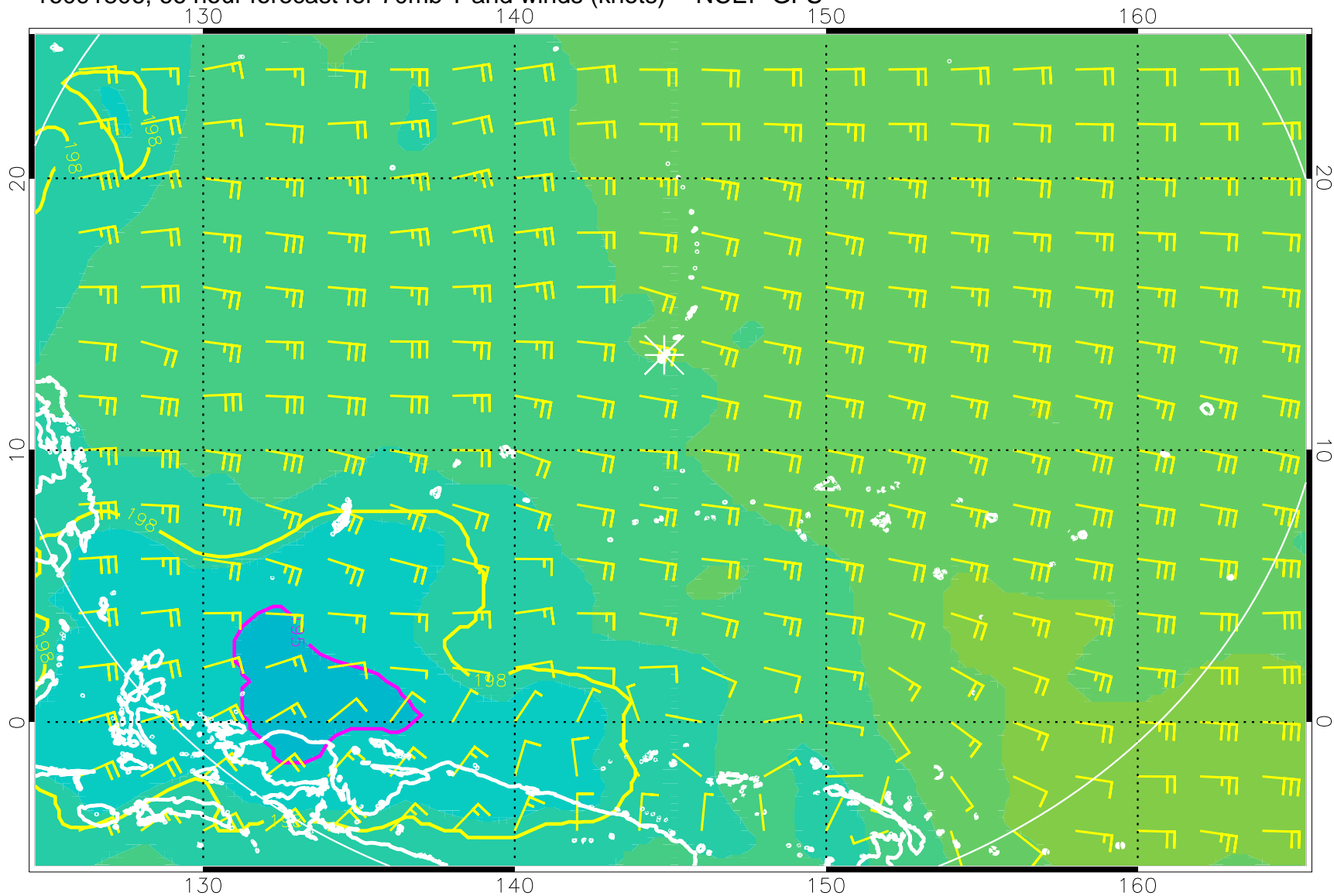
16091806, 66 hour forecast for 70mb T and winds (knots) -- NCEP GFS
