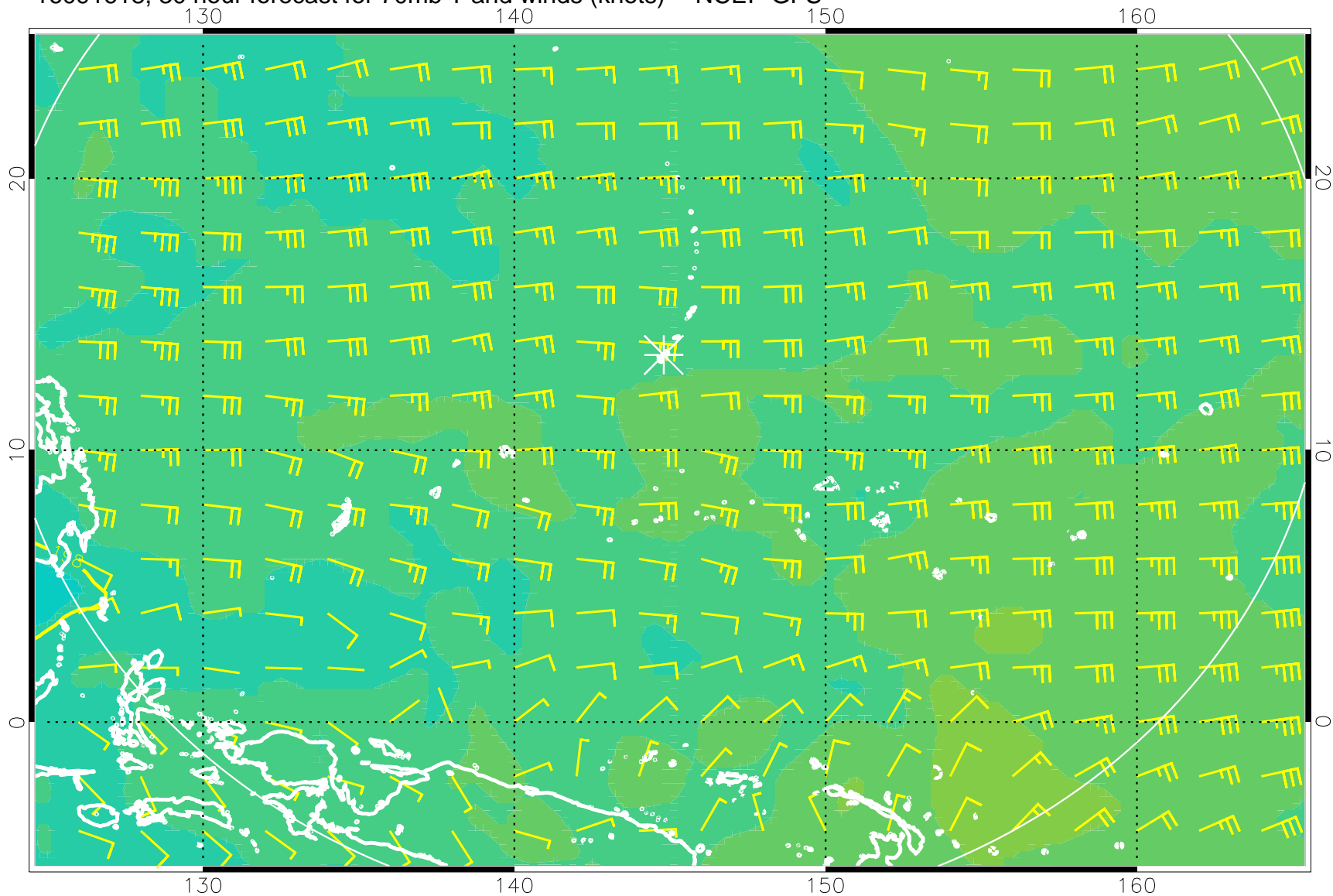
16091618, 30 hour forecast for 70mb T and winds (knots) -- NCEP GFS
