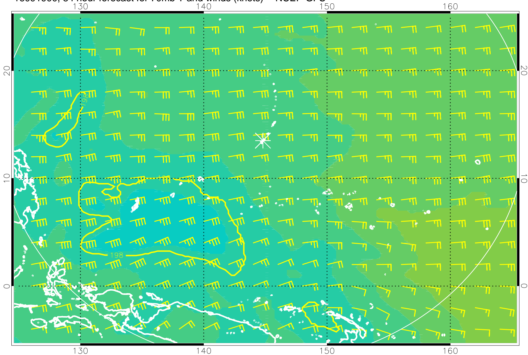
16091900, 84 hour forecast for 70mb T and winds (knots) -- NCEP GFS
