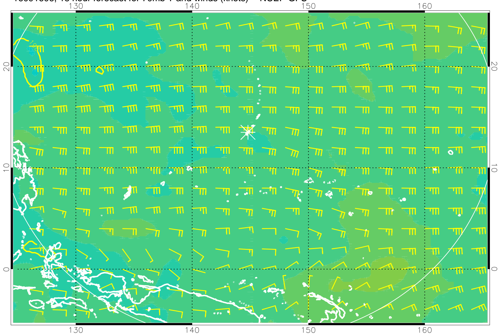
16091606, 18 hour forecast for 70mb T and winds (knots) -- NCEP GFS
