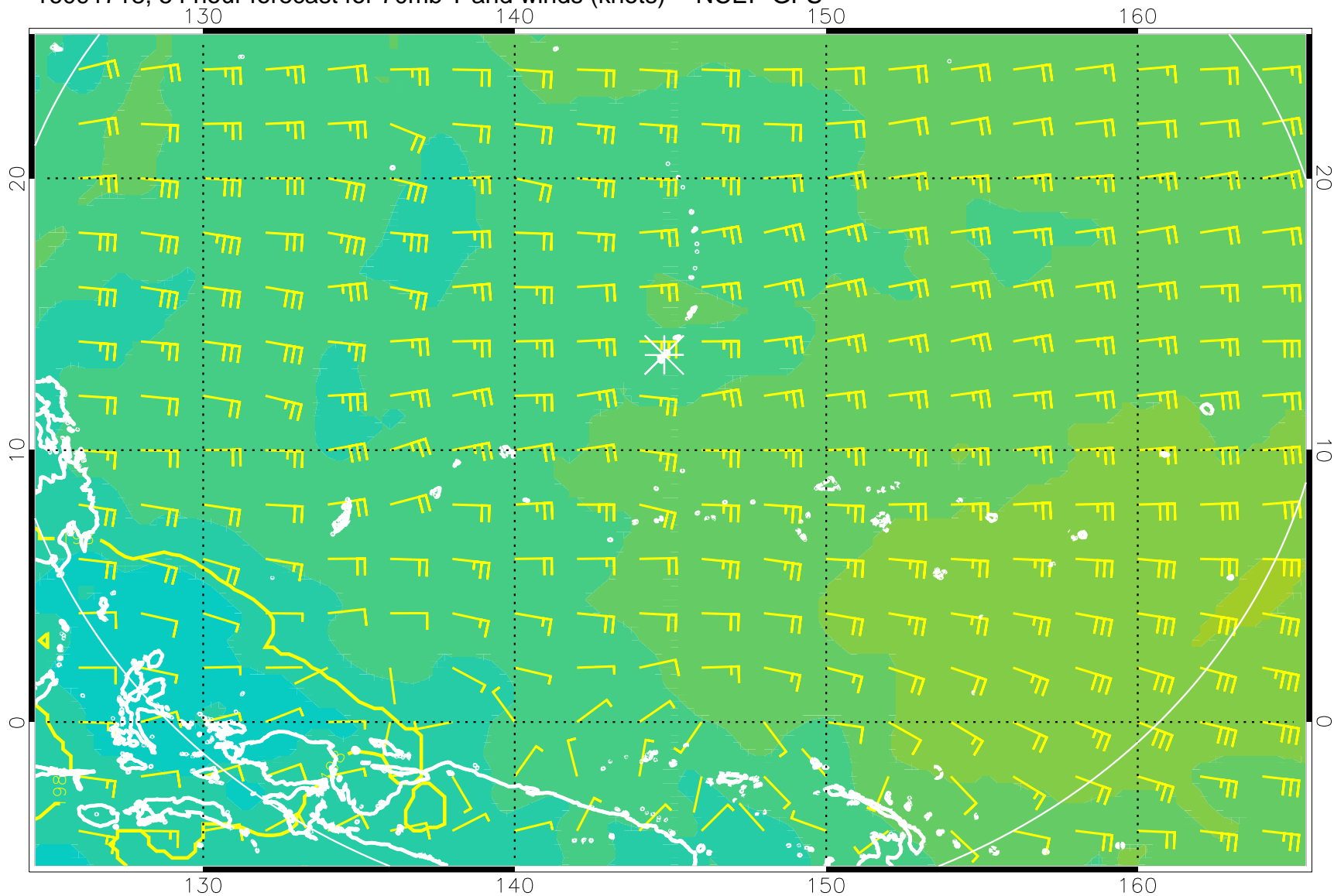
16091718, 54 hour forecast for 70mb T and winds (knots) -- NCEP GFS
