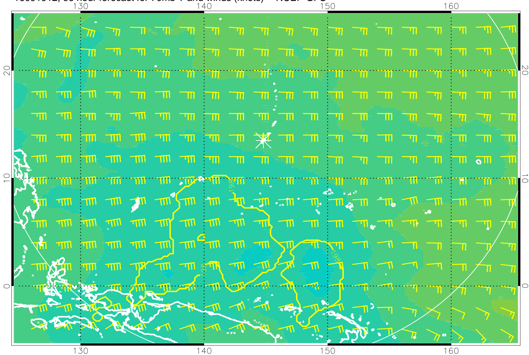
16091912, 96 hour forecast for 70mb T and winds (knots) -- NCEP GFS
