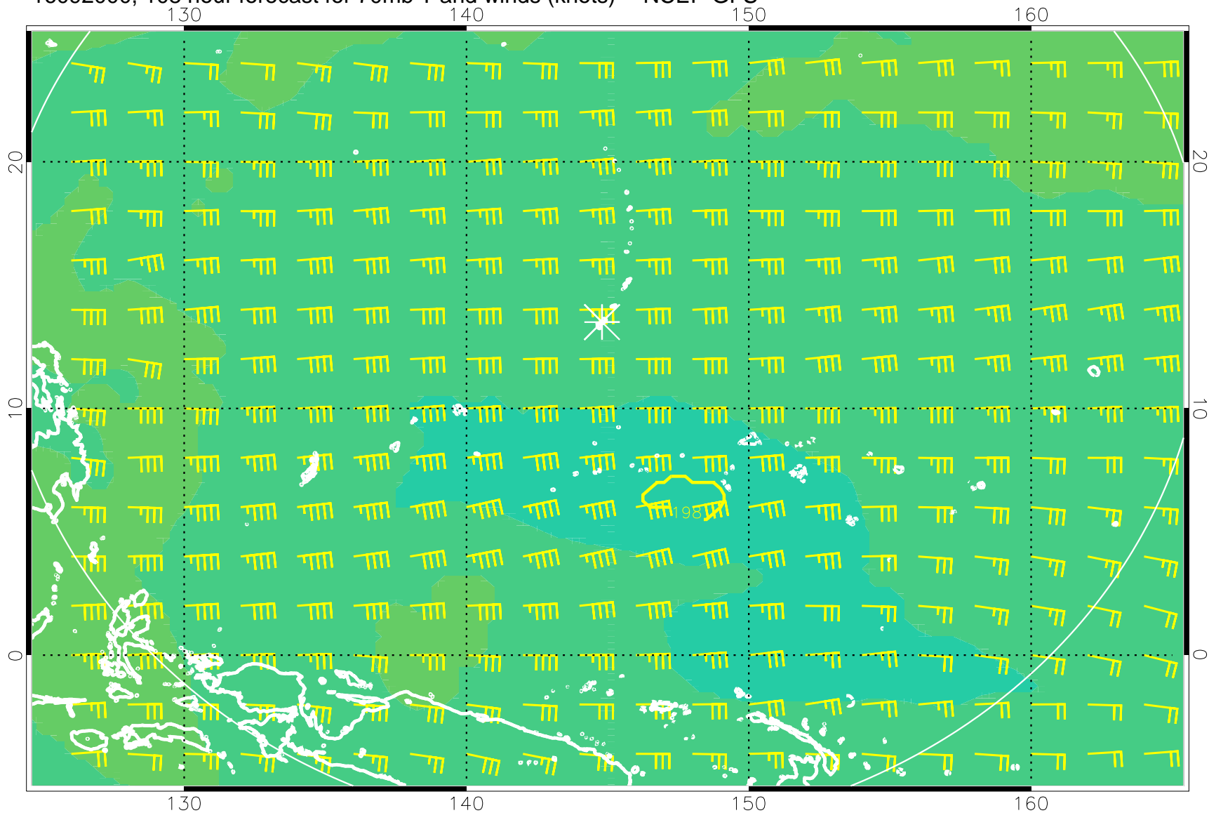
16092000, 108 hour forecast for 70mb T and winds (knots) -- NCEP GFS
