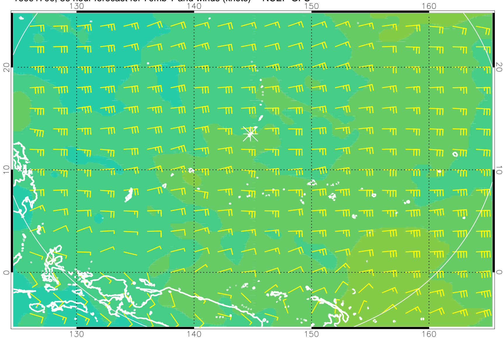
16091700, 36 hour forecast for 70mb T and winds (knots) -- NCEP GFS
