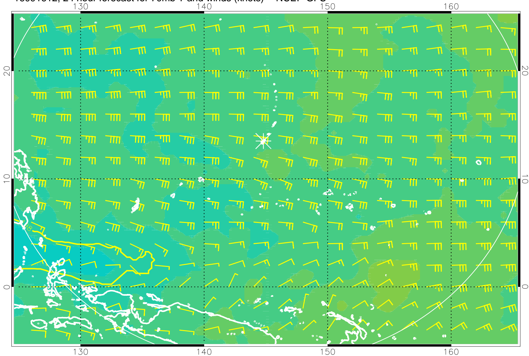
16091612, 24 hour forecast for 70mb T and winds (knots) -- NCEP GFS
