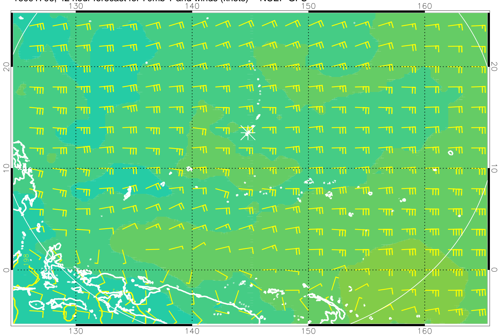
16091706, 42 hour forecast for 70mb T and winds (knots) -- NCEP GFS
