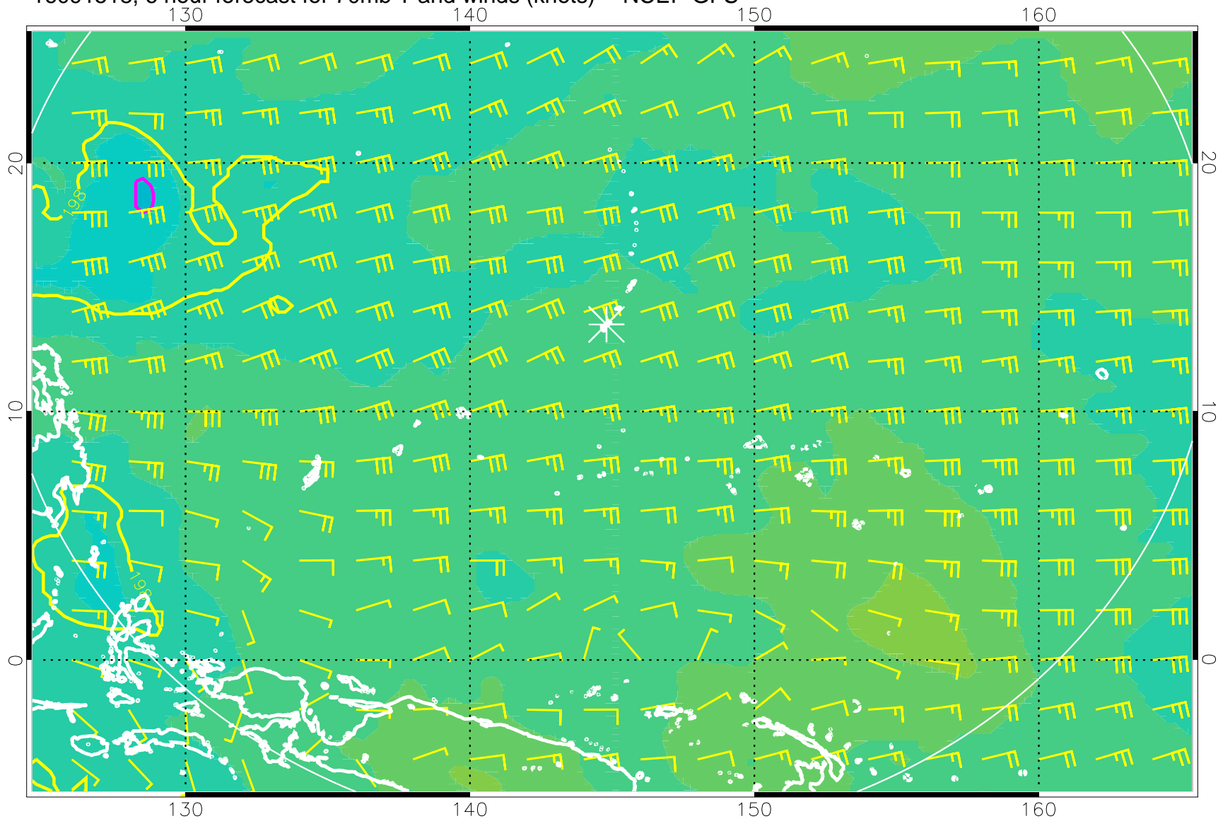
16091518, 6 hour forecast for 70mb T and winds (knots) -- NCEP GFS
