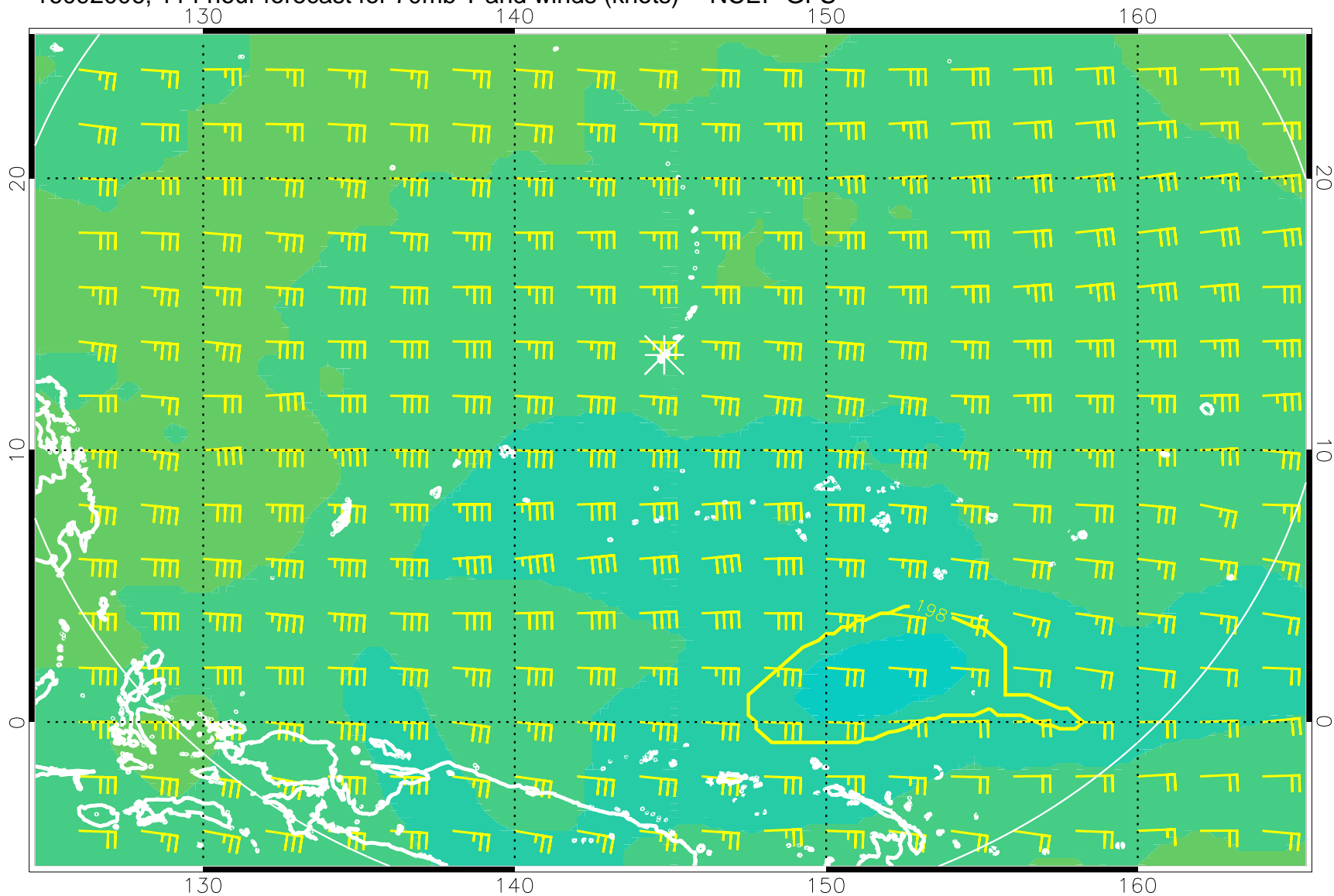
16092006, 114 hour forecast for 70mb T and winds (knots) -- NCEP GFS
