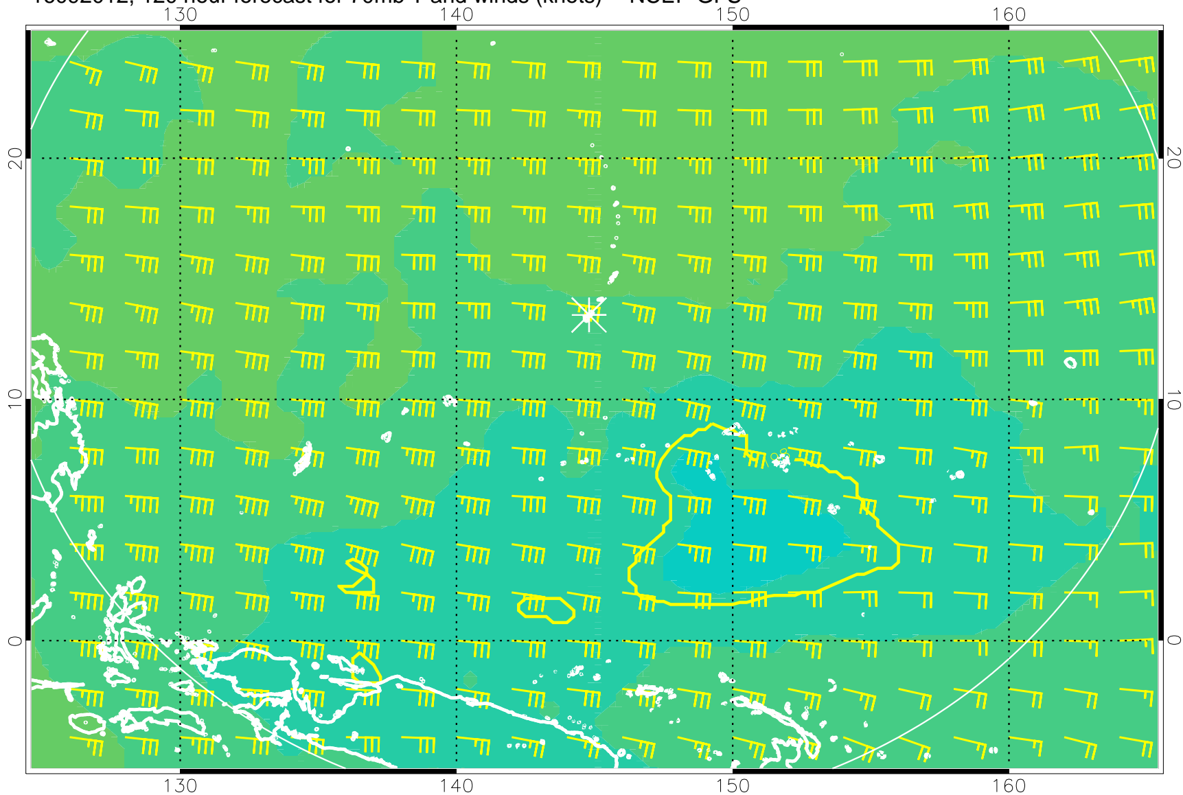
16092012, 120 hour forecast for 70mb T and winds (knots) -- NCEP GFS
