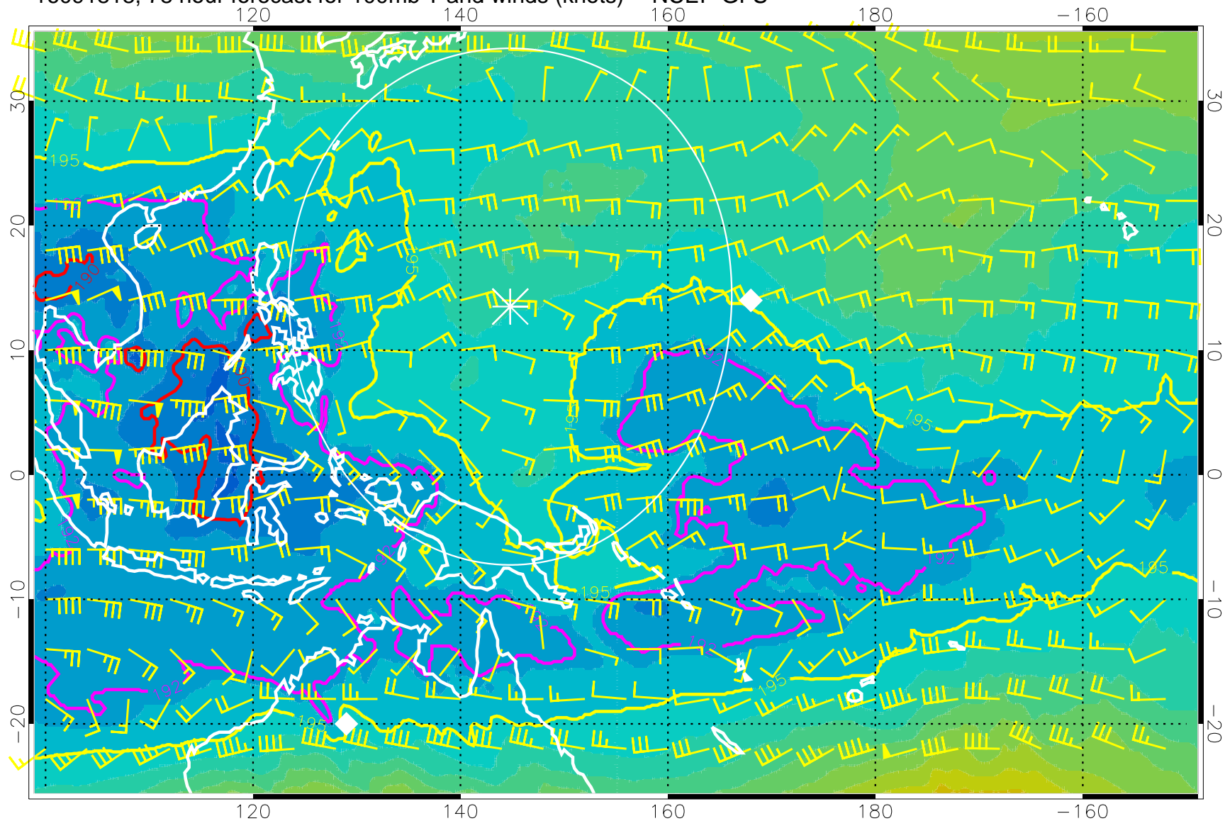
16091818, 78 hour forecast for 100mb T and winds (knots) -- NCEP GFS
