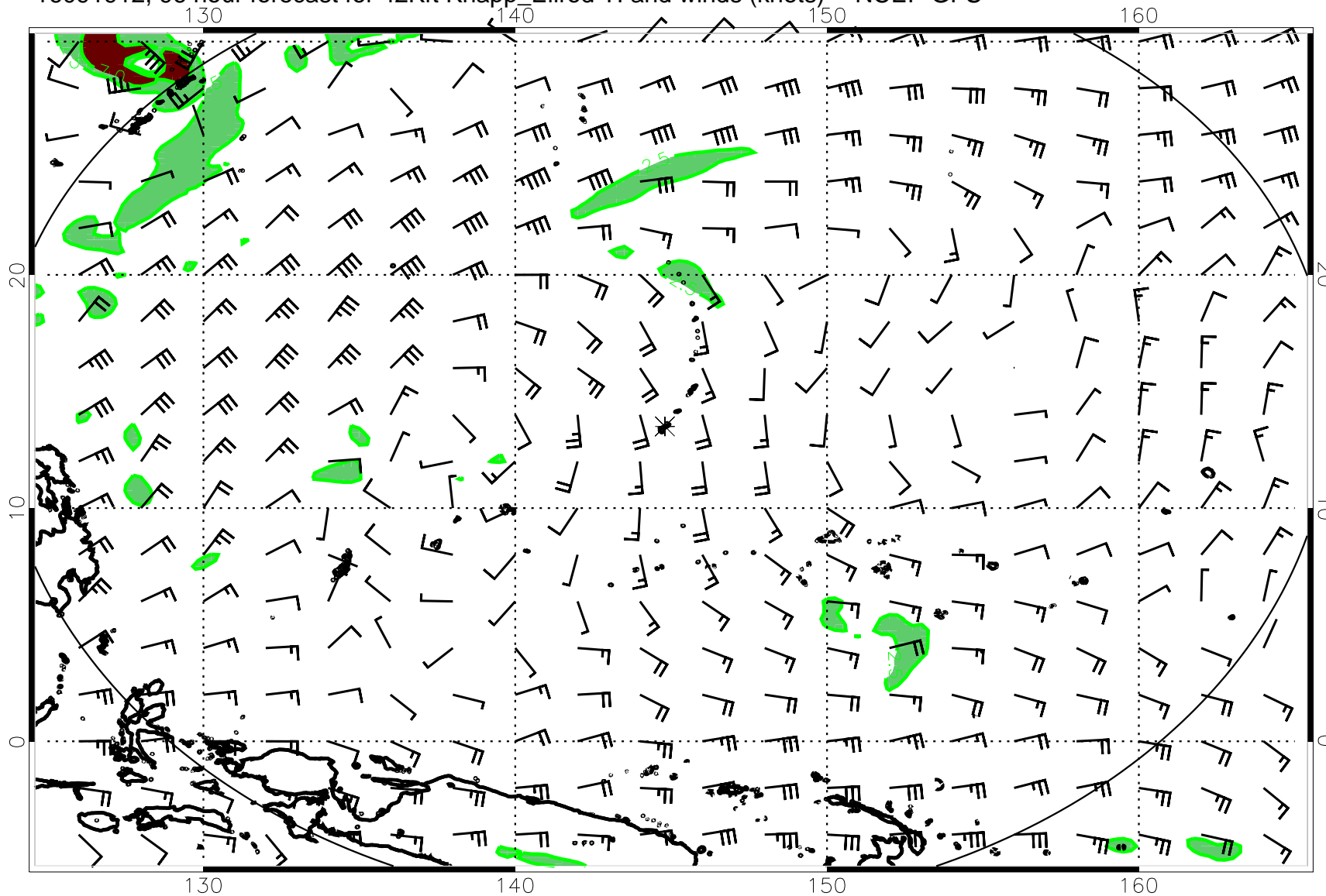
16091912, 96 hour forecast for 42Kft Knapp_Ellrod TI and winds (knots) -- NCEP GFS
