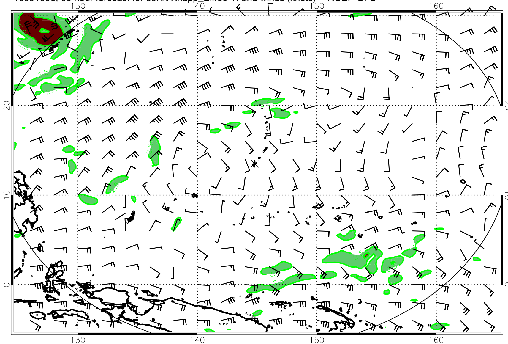
16091906, 90 hour forecast for 39Kft Knapp_Ellrod TI and winds (knots) -- NCEP GFS
