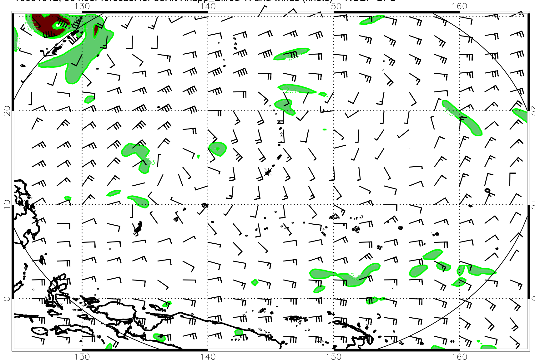
16091912, 96 hour forecast for 36Kft Knapp_Ellrod TI and winds (knots) -- NCEP GFS
