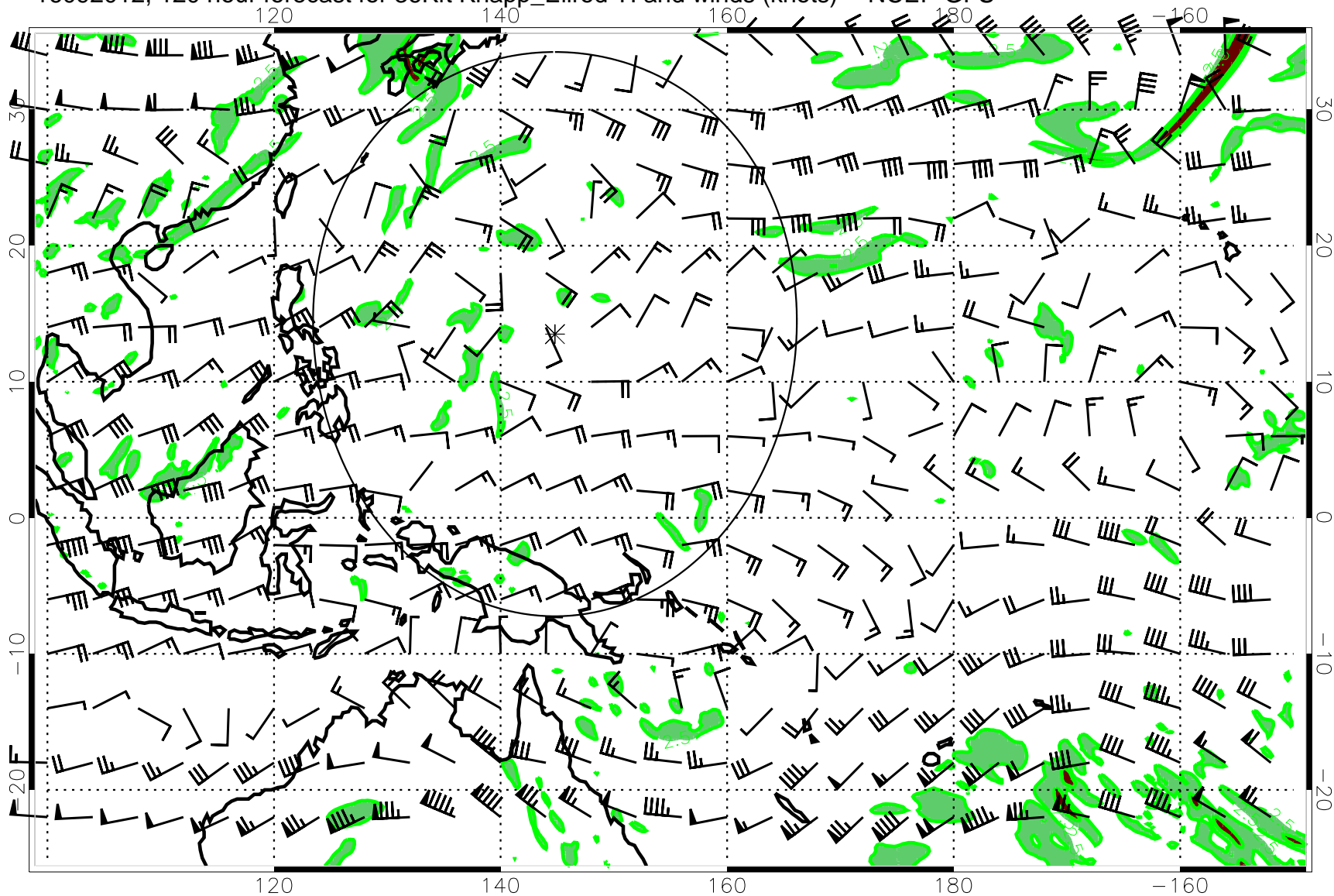
16092012, 120 hour forecast for 36Kft Knapp_Ellrod TI and winds (knots) -- NCEP GFS
