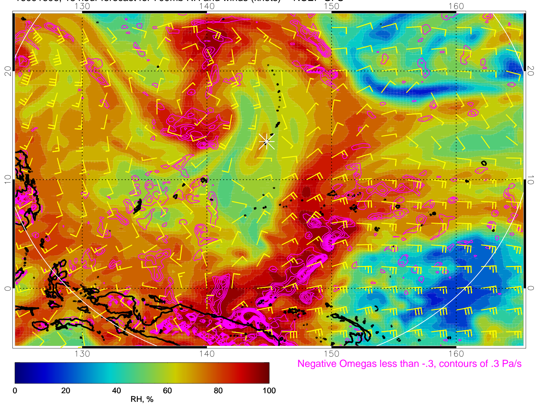
16091606, 18 hour forecast for 700mb RH and winds (knots) -- NCEP GFS
