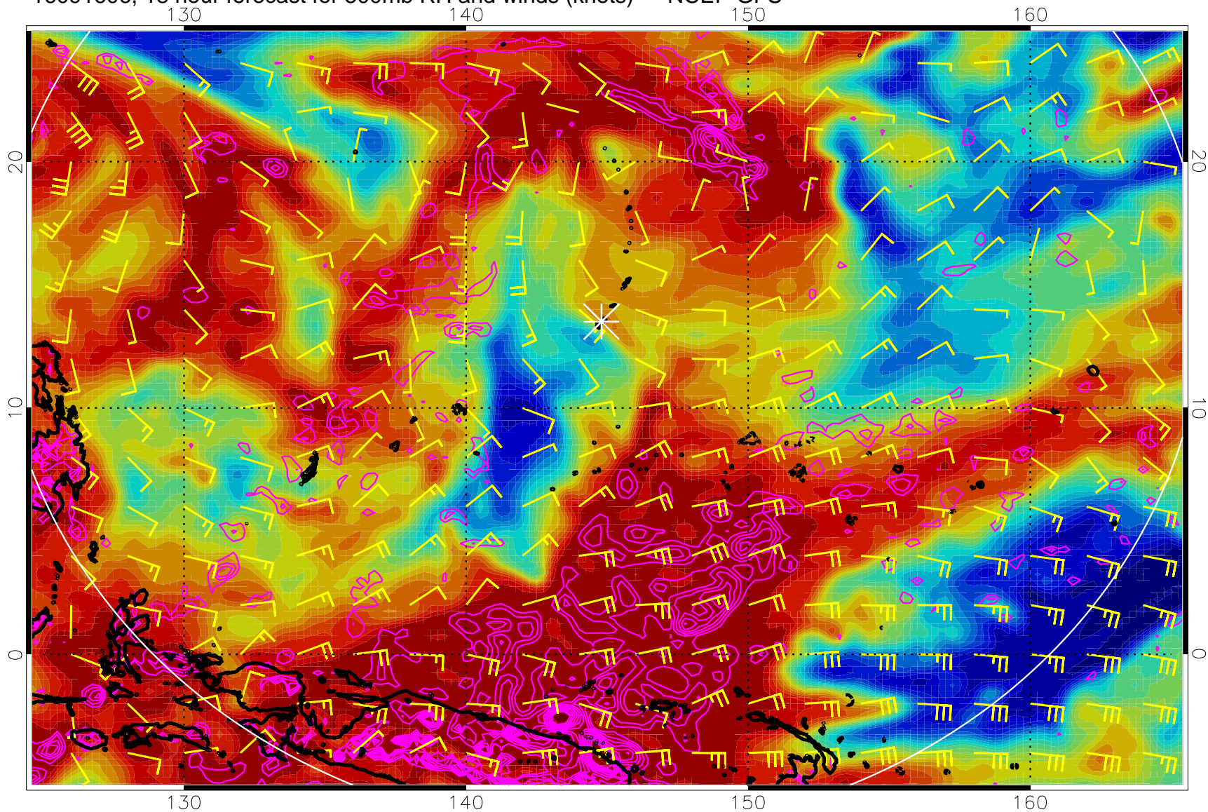
16091606, 18 hour forecast for 500mb RH and winds (knots) -- NCEP GFS
