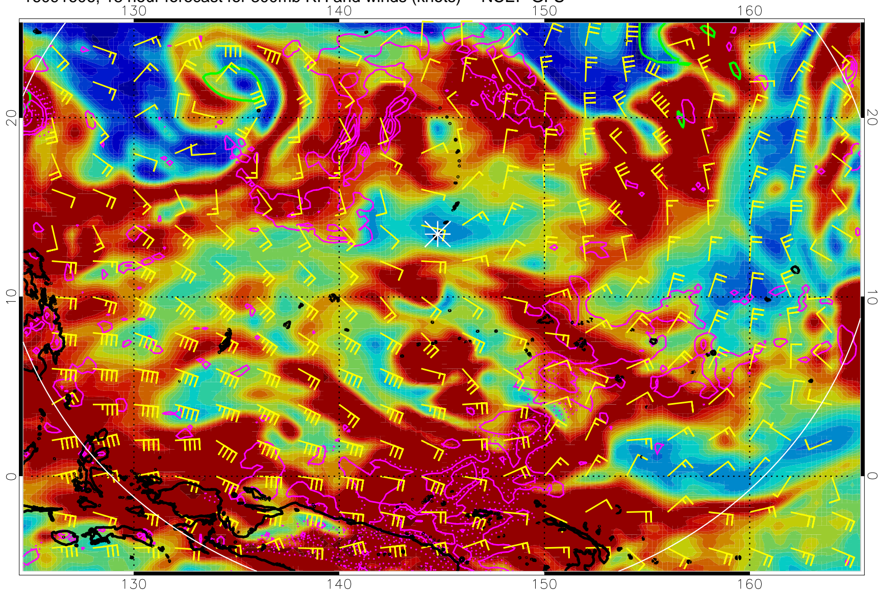
16091606, 18 hour forecast for 300mb RH and winds (knots) -- NCEP GFS
