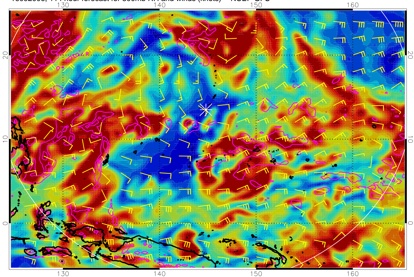
16092006, 114 hour forecast for 300mb RH and winds (knots) -- NCEP GFS
