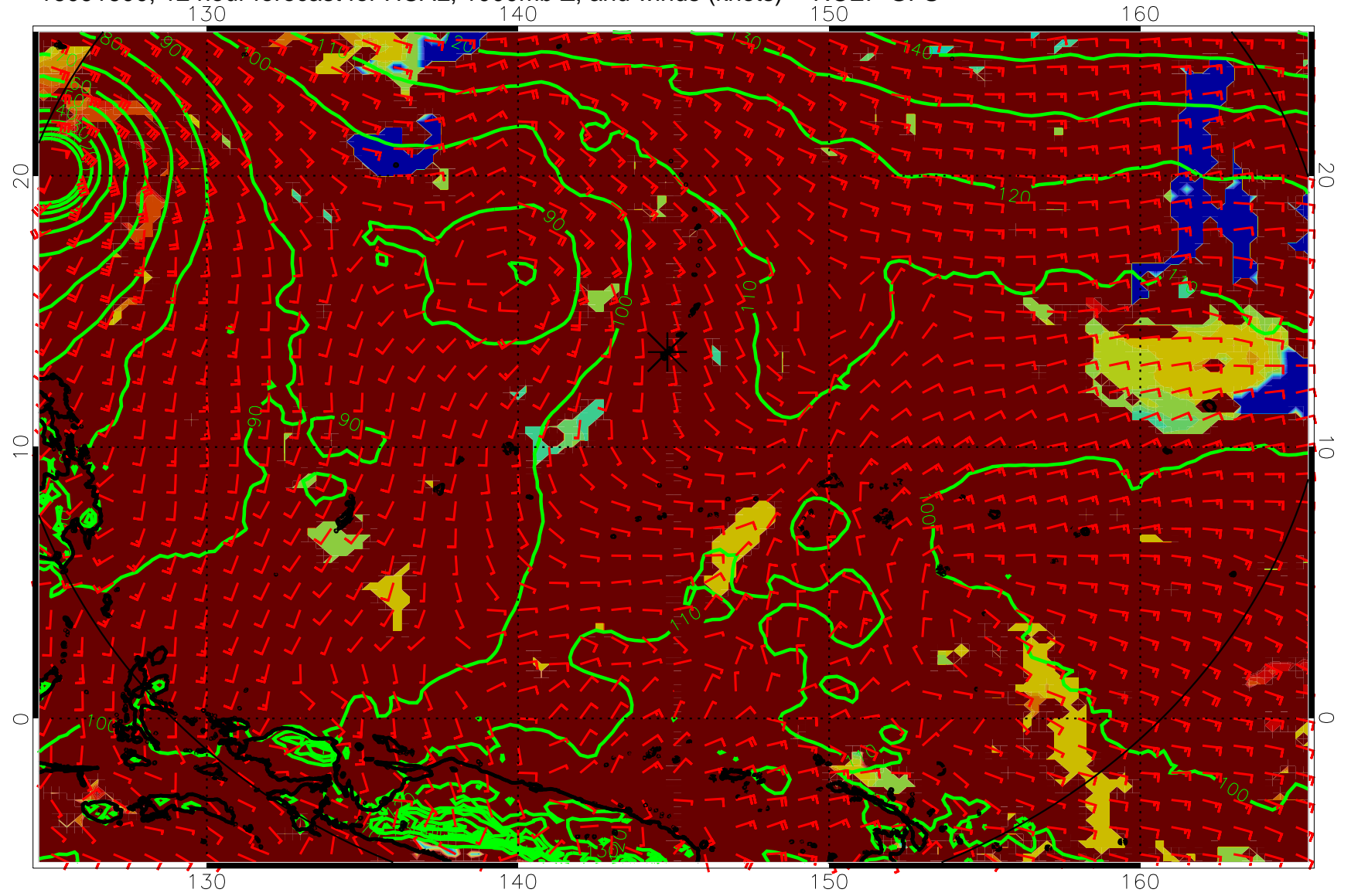
16091600, 12 hour forecast for HCAL, 1000mb Z, and winds (knots) -- NCEP GFS
