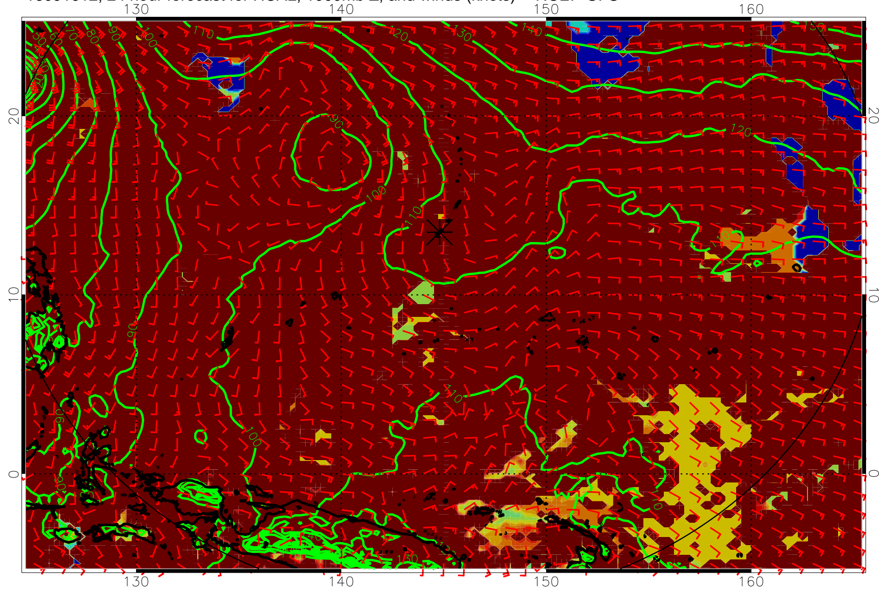
16091612, 24 hour forecast for HCAL, 1000mb Z, and winds (knots) -- NCEP GFS
