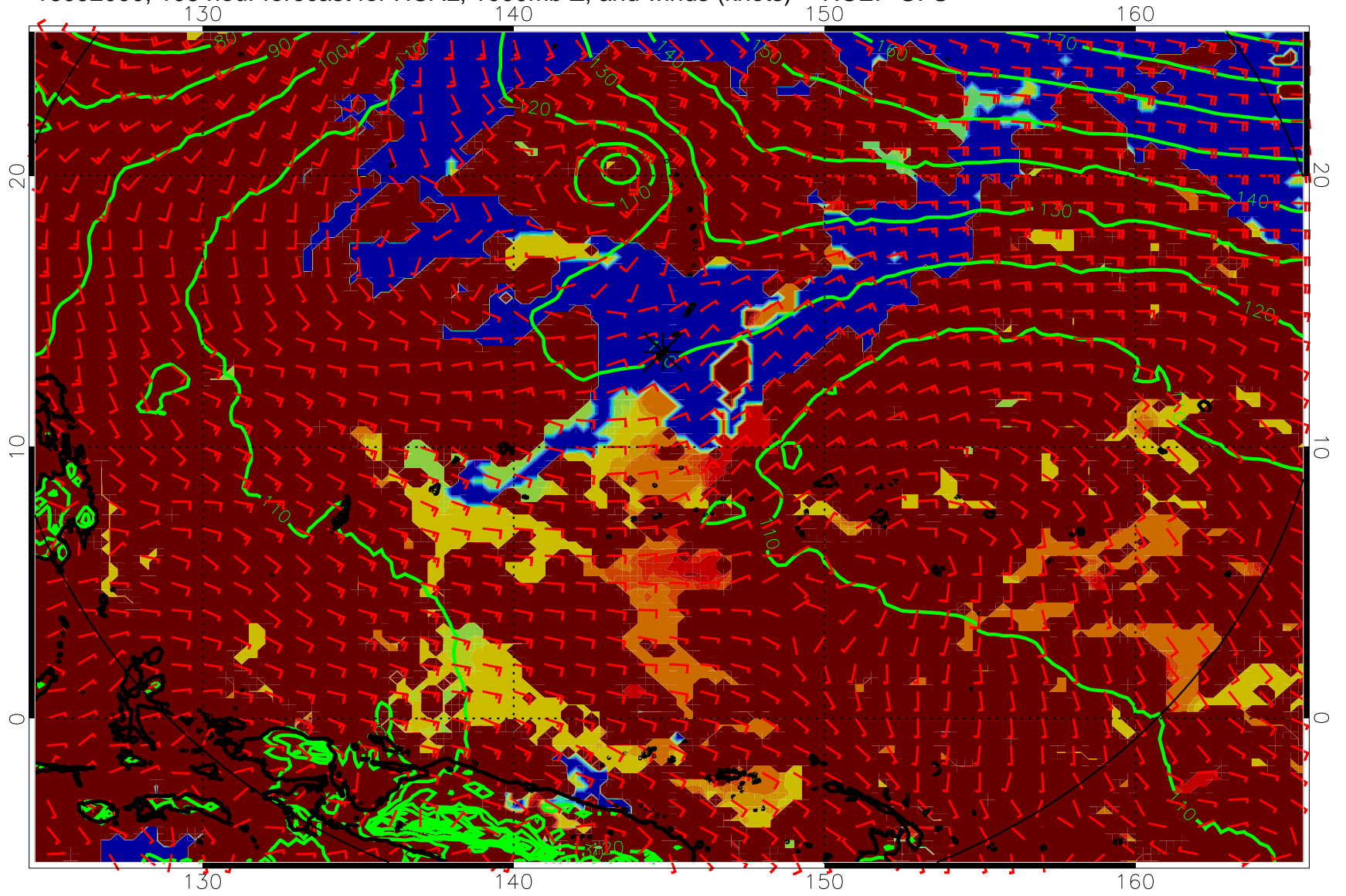
16092000, 108 hour forecast for HCAL, 1000mb Z, and winds (knots) -- NCEP GFS
