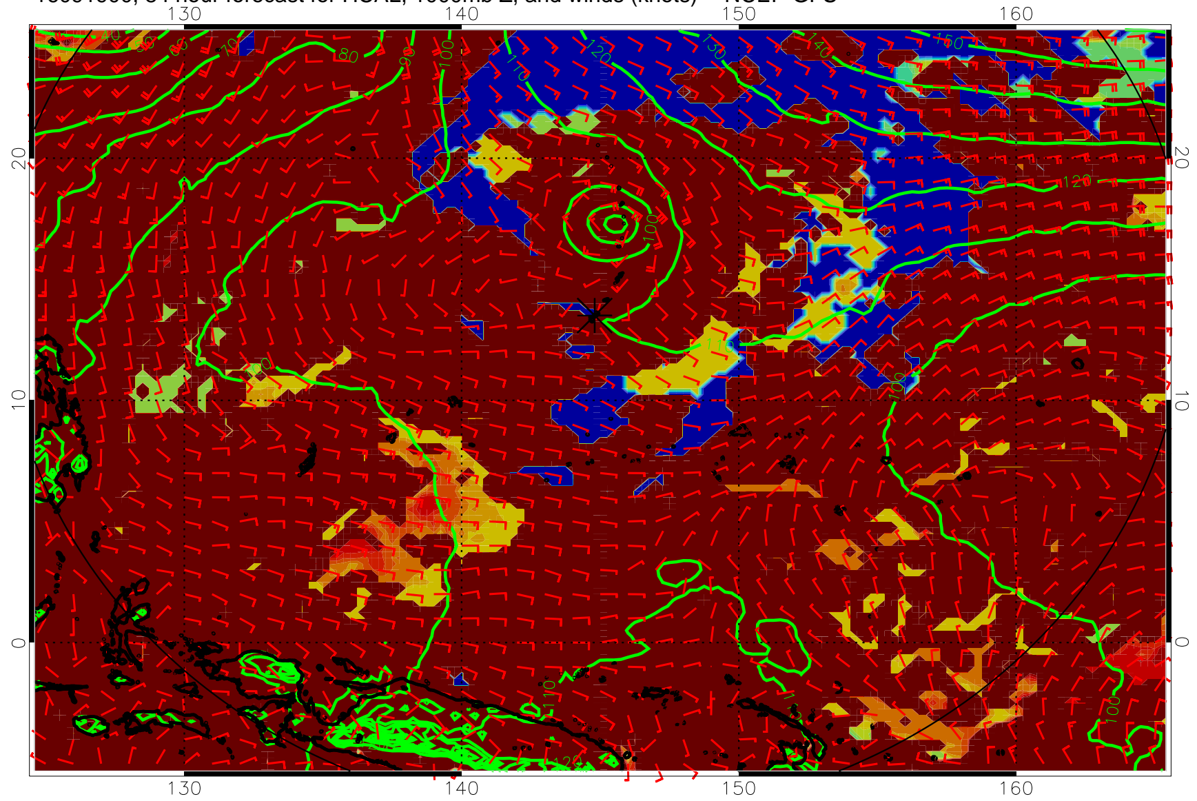
16091900, 84 hour forecast for HCAL, 1000mb Z, and winds (knots) -- NCEP GFS
