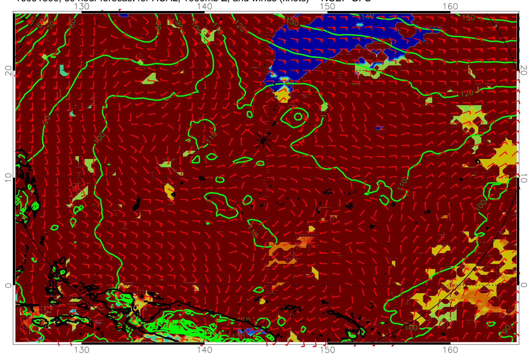
16091800, 60 hour forecast for HCAL, 1000mb Z, and winds (knots) -- NCEP GFS
