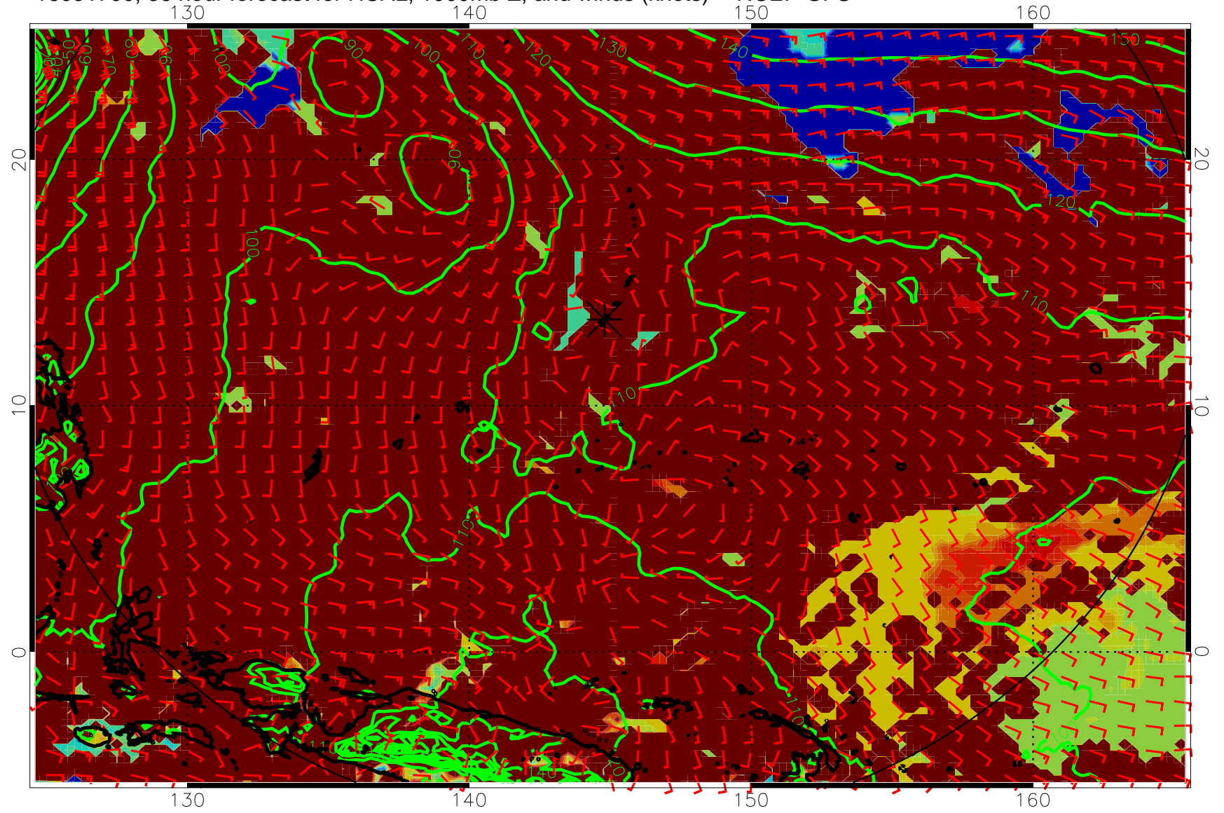
16091700, 36 hour forecast for HCAL, 1000mb Z, and winds (knots) -- NCEP GFS
