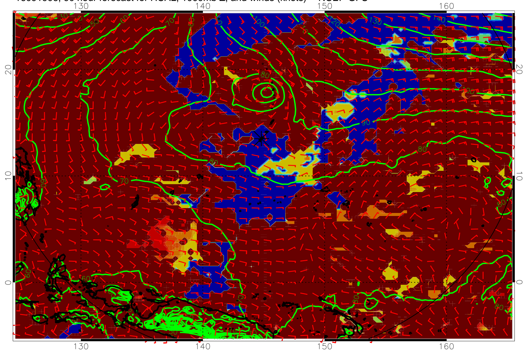
16091906, 90 hour forecast for HCAL, 1000mb Z, and winds (knots) -- NCEP GFS
