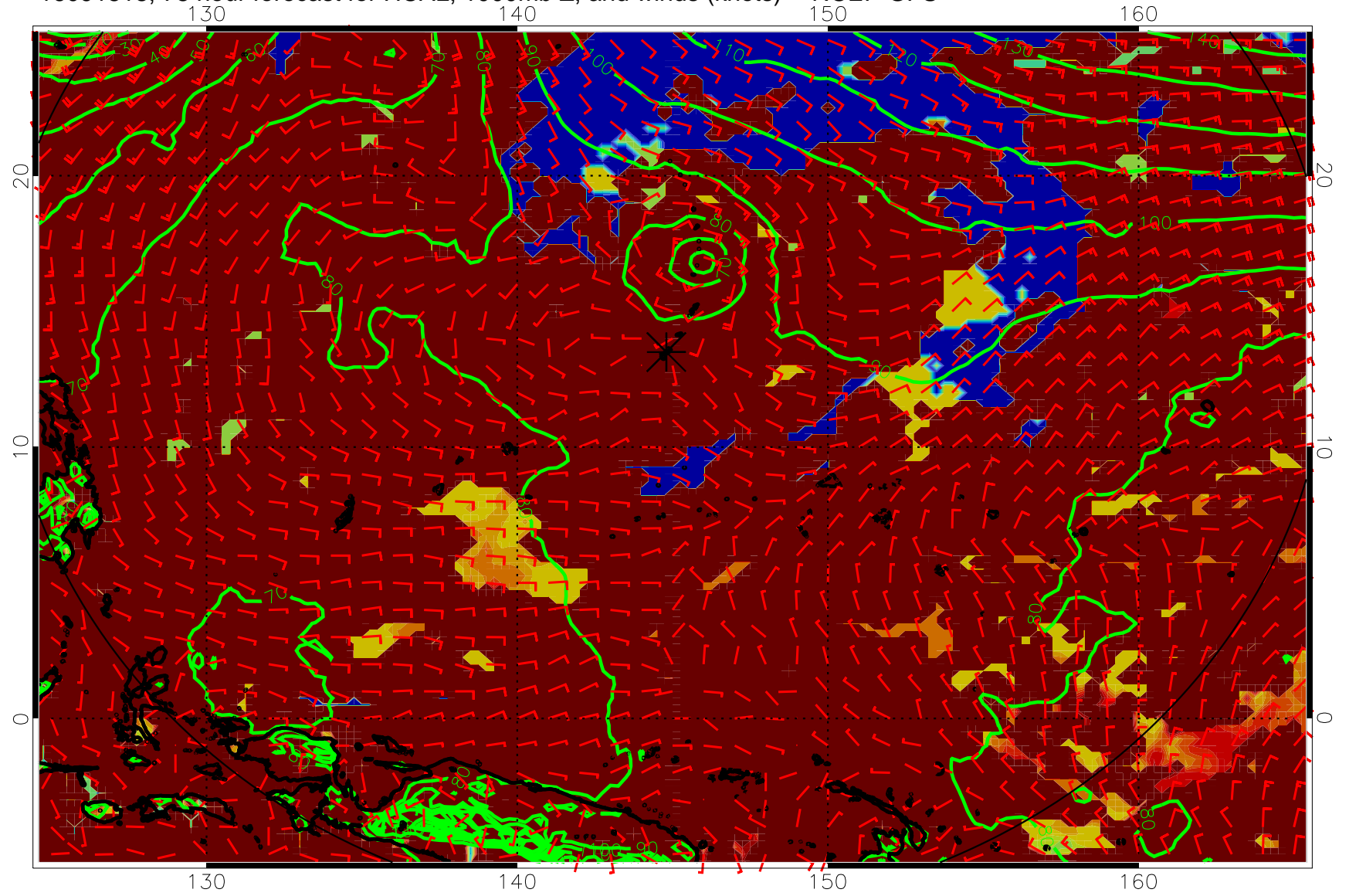
16091818, 78 hour forecast for HCAL, 1000mb Z, and winds (knots) -- NCEP GFS
