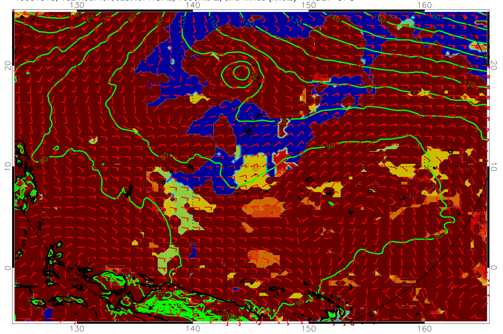
16091918, 102 hour forecast for HCAL, 1000mb Z, and winds (knots) -- NCEP GFS
