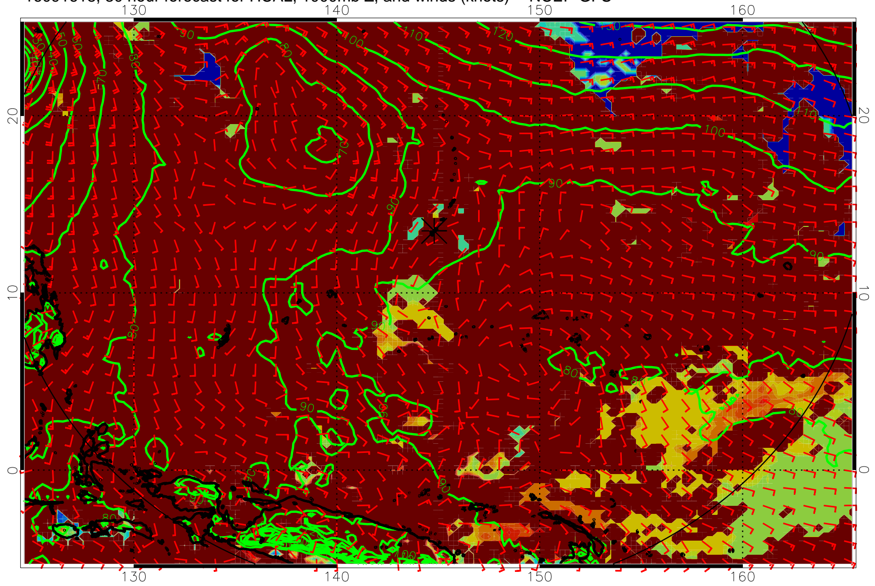
16091618, 30 hour forecast for HCAL, 1000mb Z, and winds (knots) -- NCEP GFS
