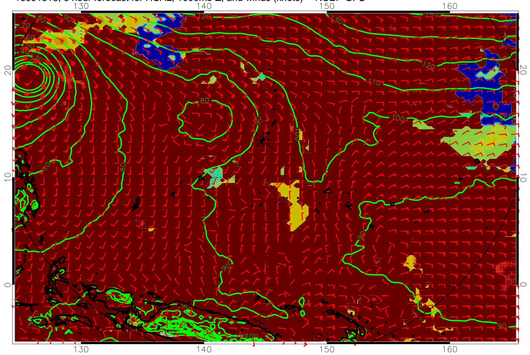
16091518, 6 hour forecast for HCAL, 1000mb Z, and winds (knots) -- NCEP GFS
