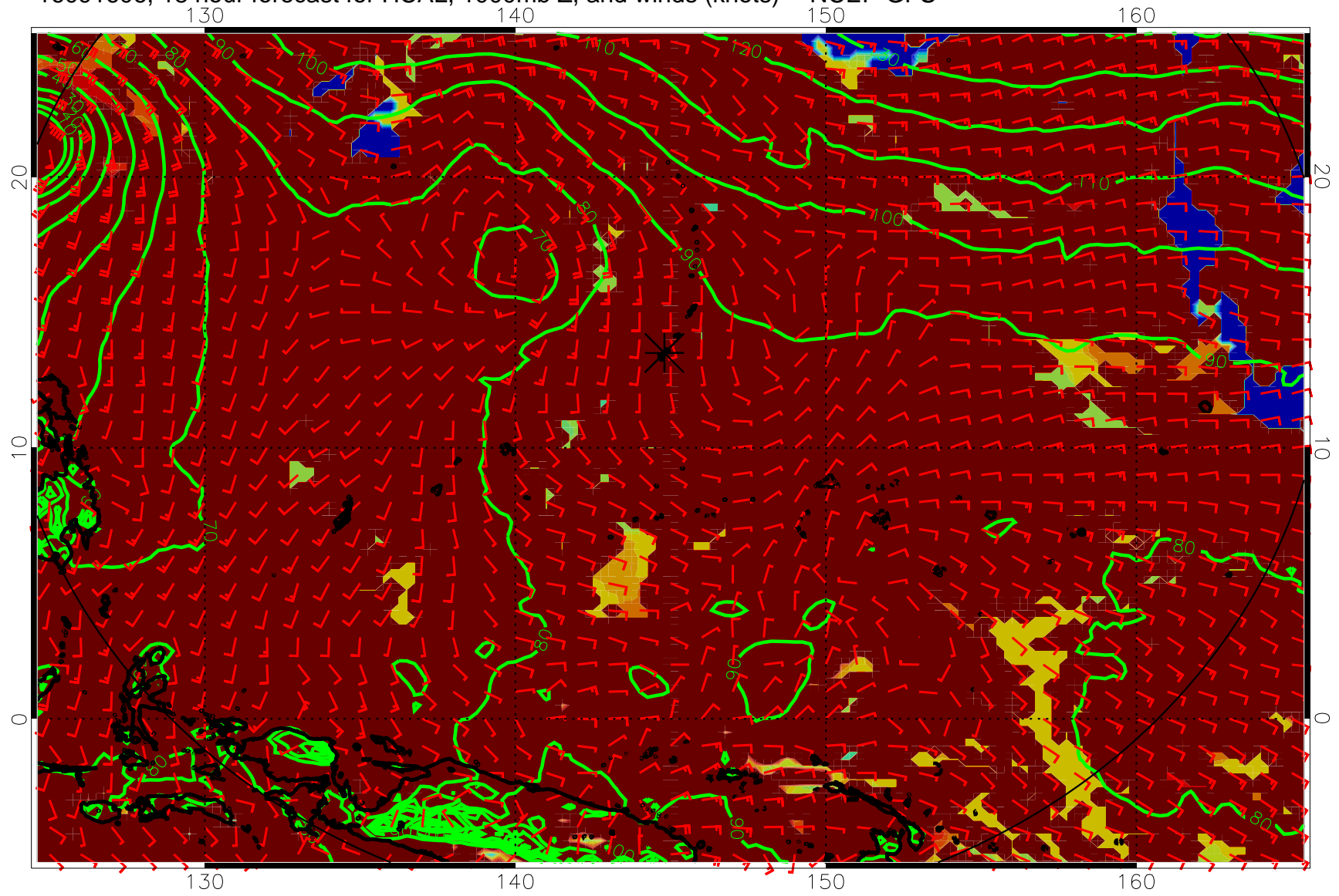
16091606, 18 hour forecast for HCAL, 1000mb Z, and winds (knots) -- NCEP GFS
