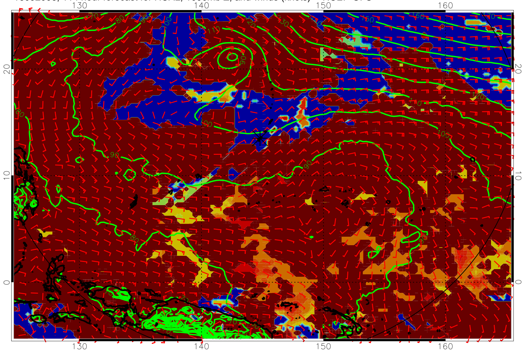
16092006, 114 hour forecast for HCAL, 1000mb Z, and winds (knots) -- NCEP GFS
