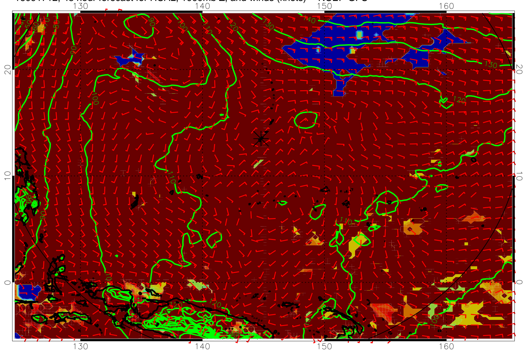
16091712, 48 hour forecast for HCAL, 1000mb Z, and winds (knots) -- NCEP GFS
