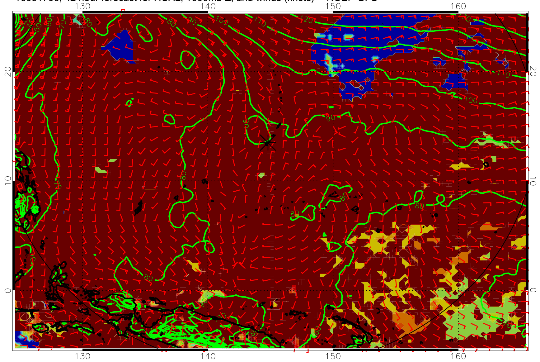
16091706, 42 hour forecast for HCAL, 1000mb Z, and winds (knots) -- NCEP GFS
