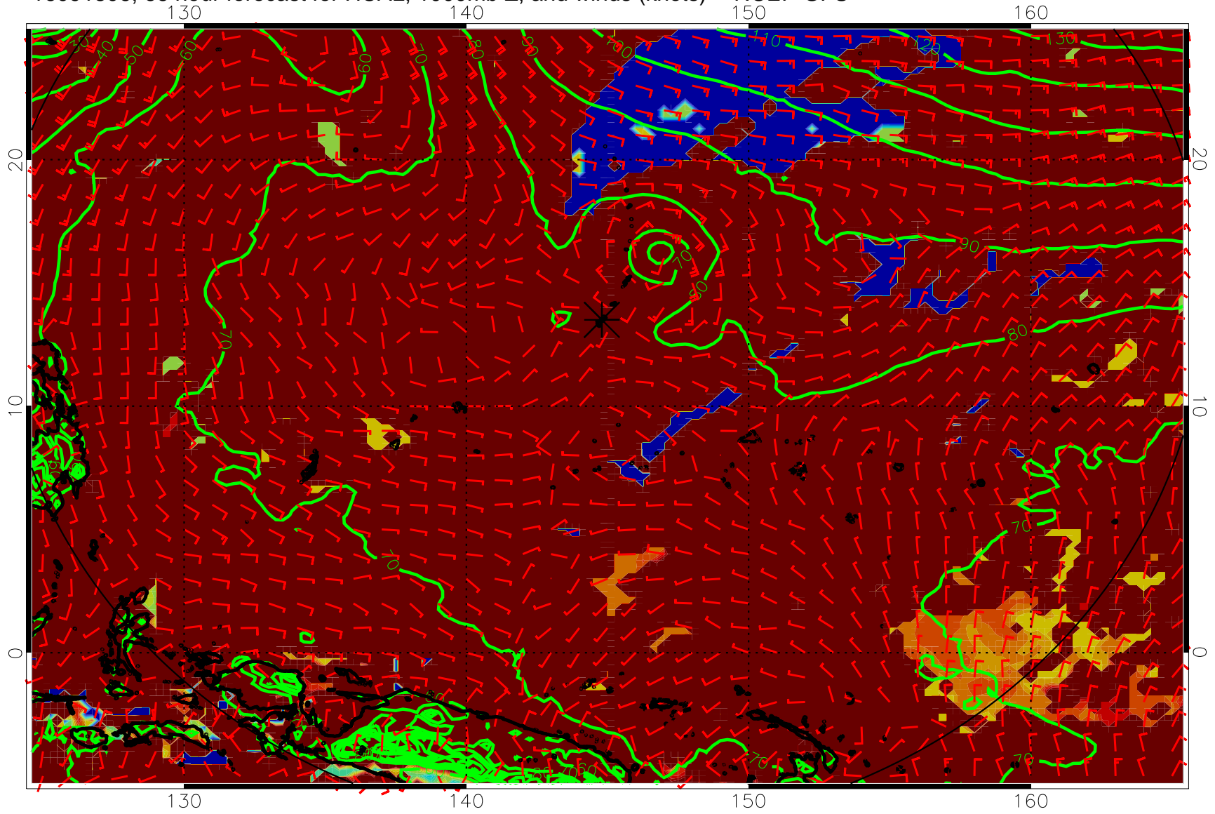
16091806, 66 hour forecast for HCAL, 1000mb Z, and winds (knots) -- NCEP GFS
