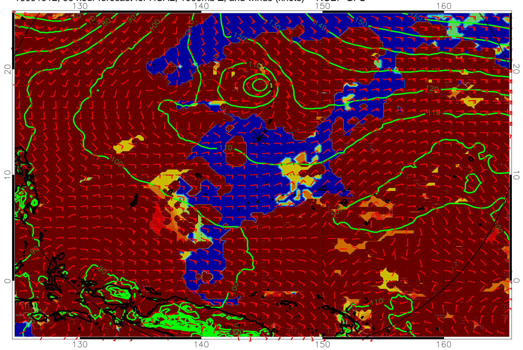
16091912, 96 hour forecast for HCAL, 1000mb Z, and winds (knots) -- NCEP GFS
