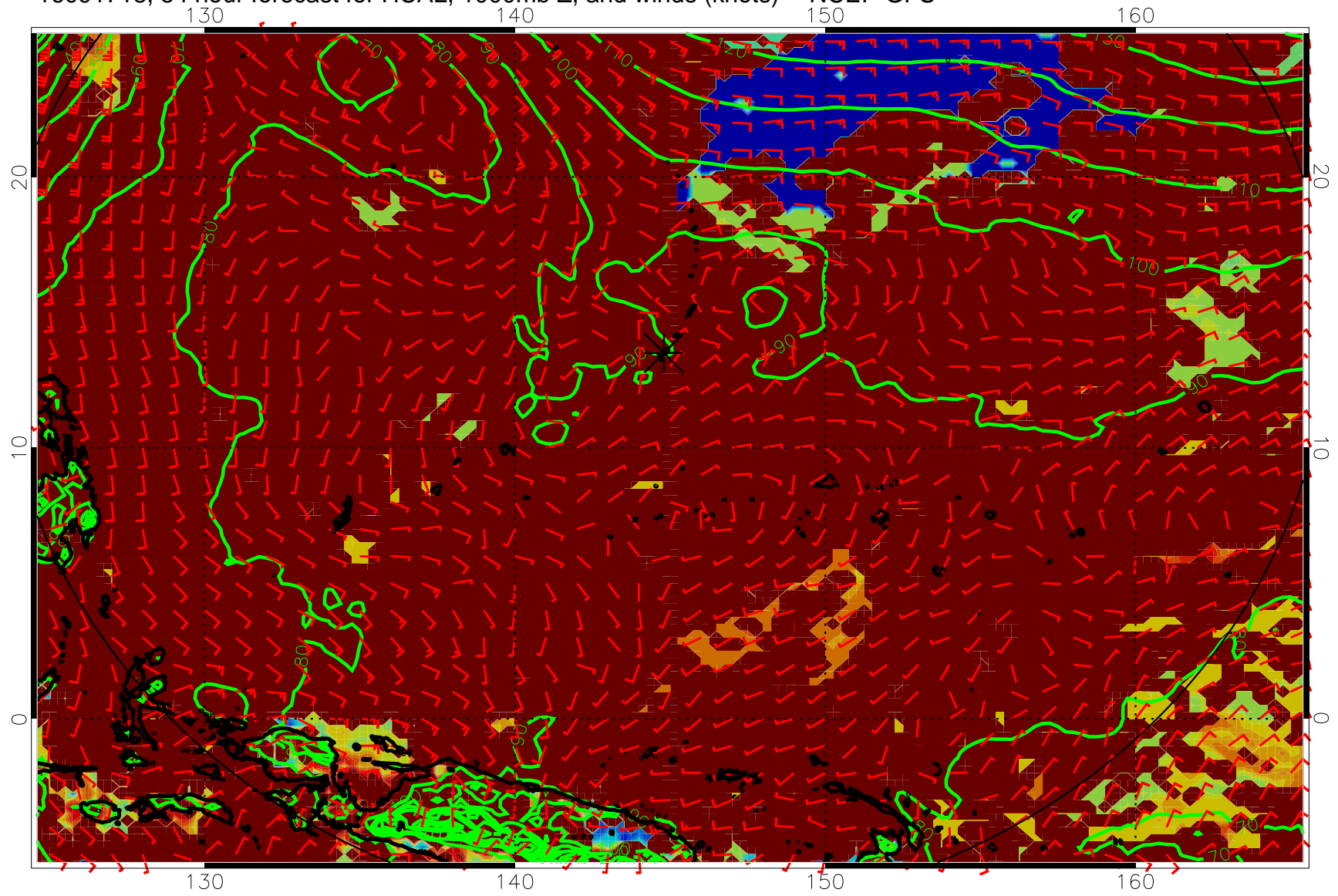
16091718, 54 hour forecast for HCAL, 1000mb Z, and winds (knots) -- NCEP GFS
