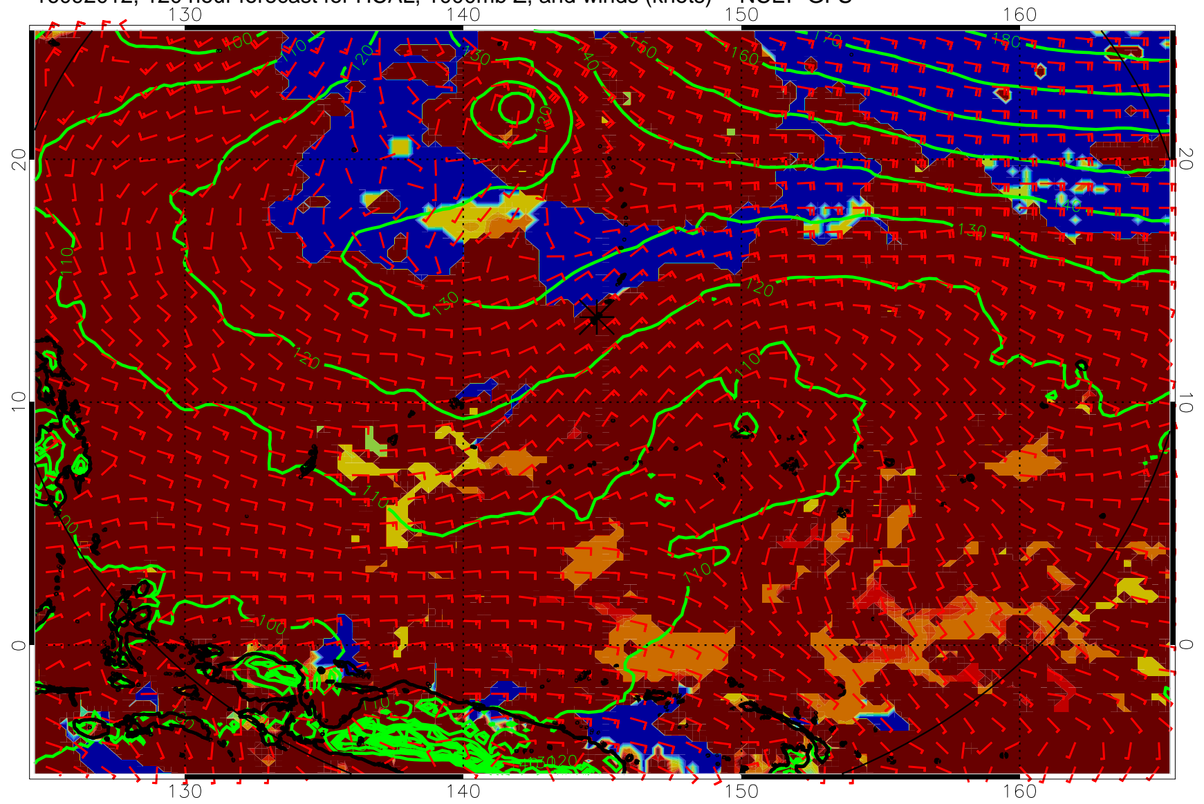
16092012, 120 hour forecast for HCAL, 1000mb Z, and winds (knots) -- NCEP GFS
