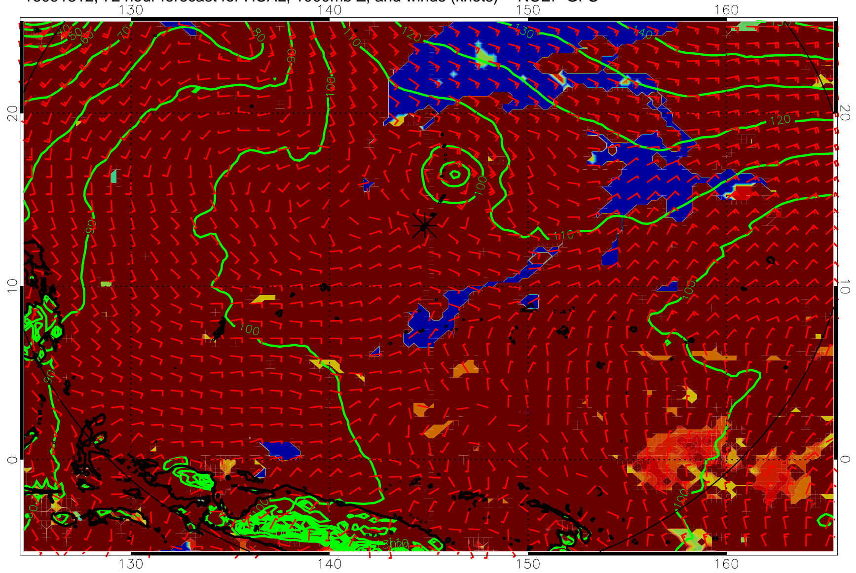
16091812, 72 hour forecast for HCAL, 1000mb Z, and winds (knots) -- NCEP GFS
