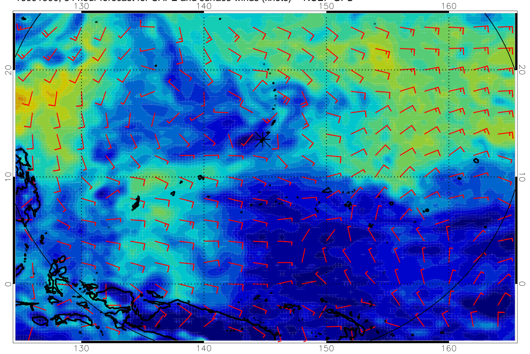
16091900, 84 hour forecast for CAPE and surface winds (knots) -- NCEP GFS
