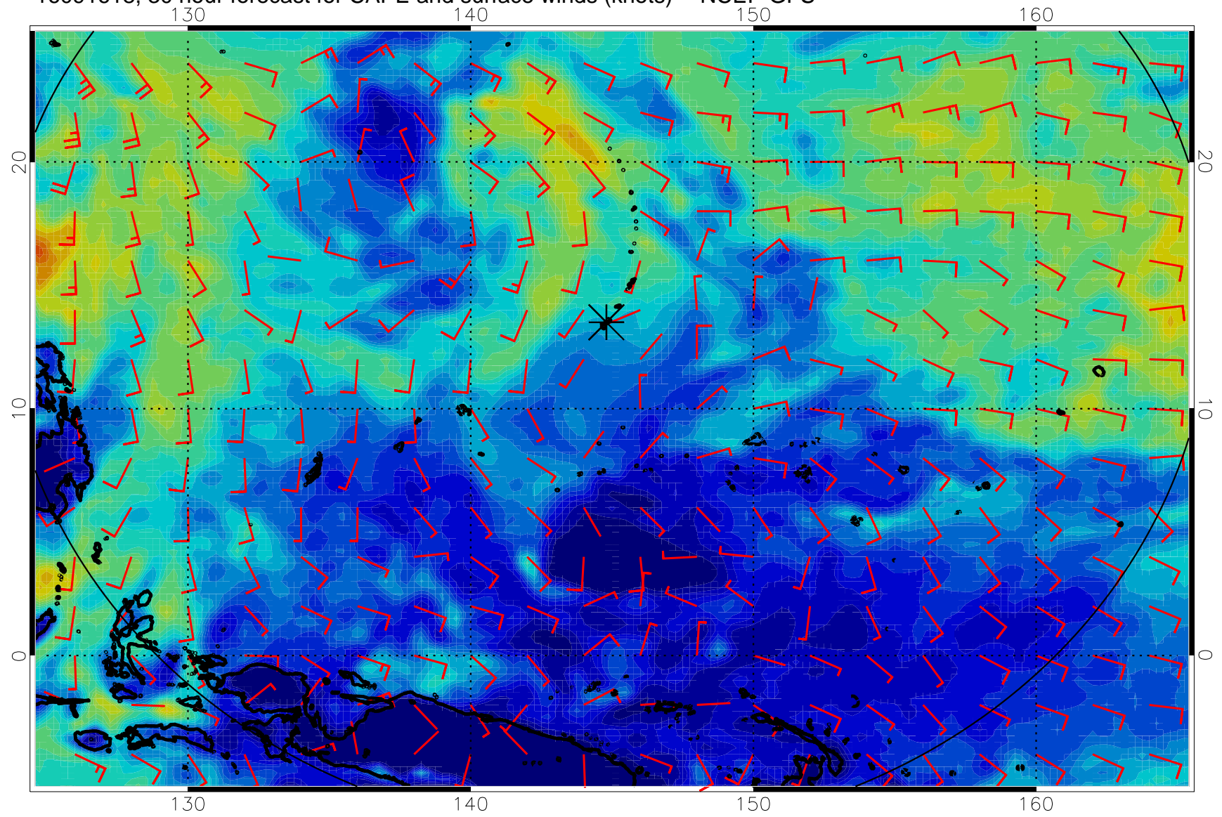
16091618, 30 hour forecast for CAPE and surface winds (knots) -- NCEP GFS
