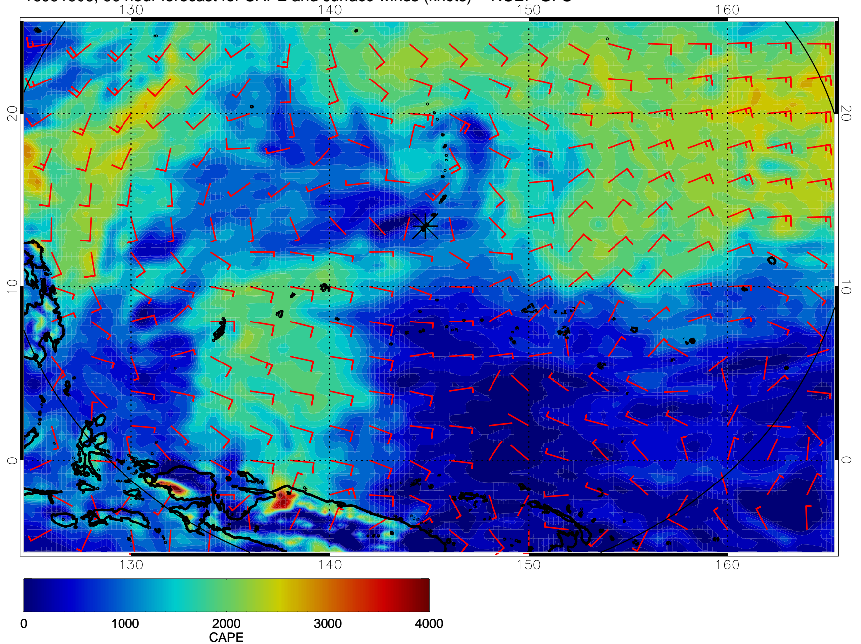
16091906, 90 hour forecast for CAPE and surface winds (knots) -- NCEP GFS
