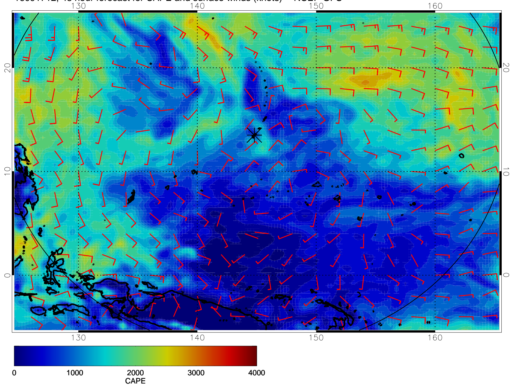
16091712, 48 hour forecast for CAPE and surface winds (knots) -- NCEP GFS
