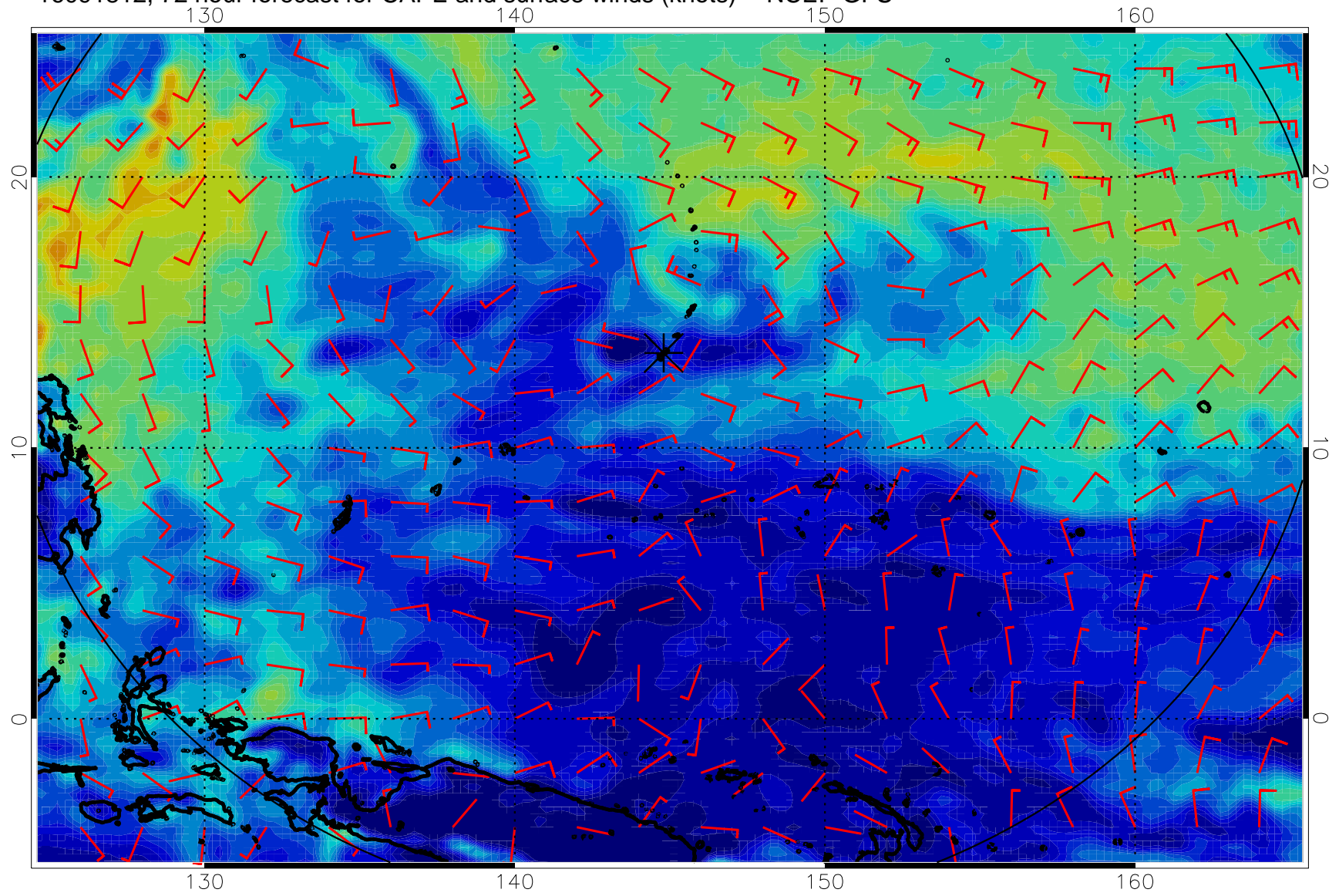
16091812, 72 hour forecast for CAPE and surface winds (knots) -- NCEP GFS
