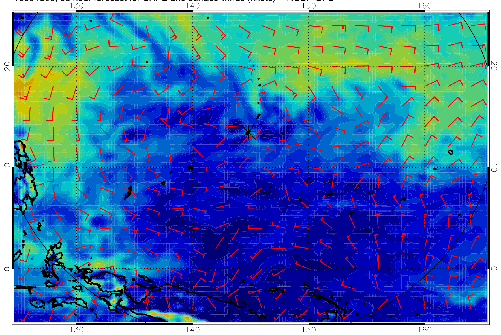
16091806, 66 hour forecast for CAPE and surface winds (knots) -- NCEP GFS
