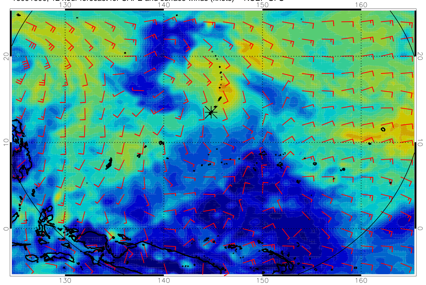
16091600, 12 hour forecast for CAPE and surface winds (knots) -- NCEP GFS
