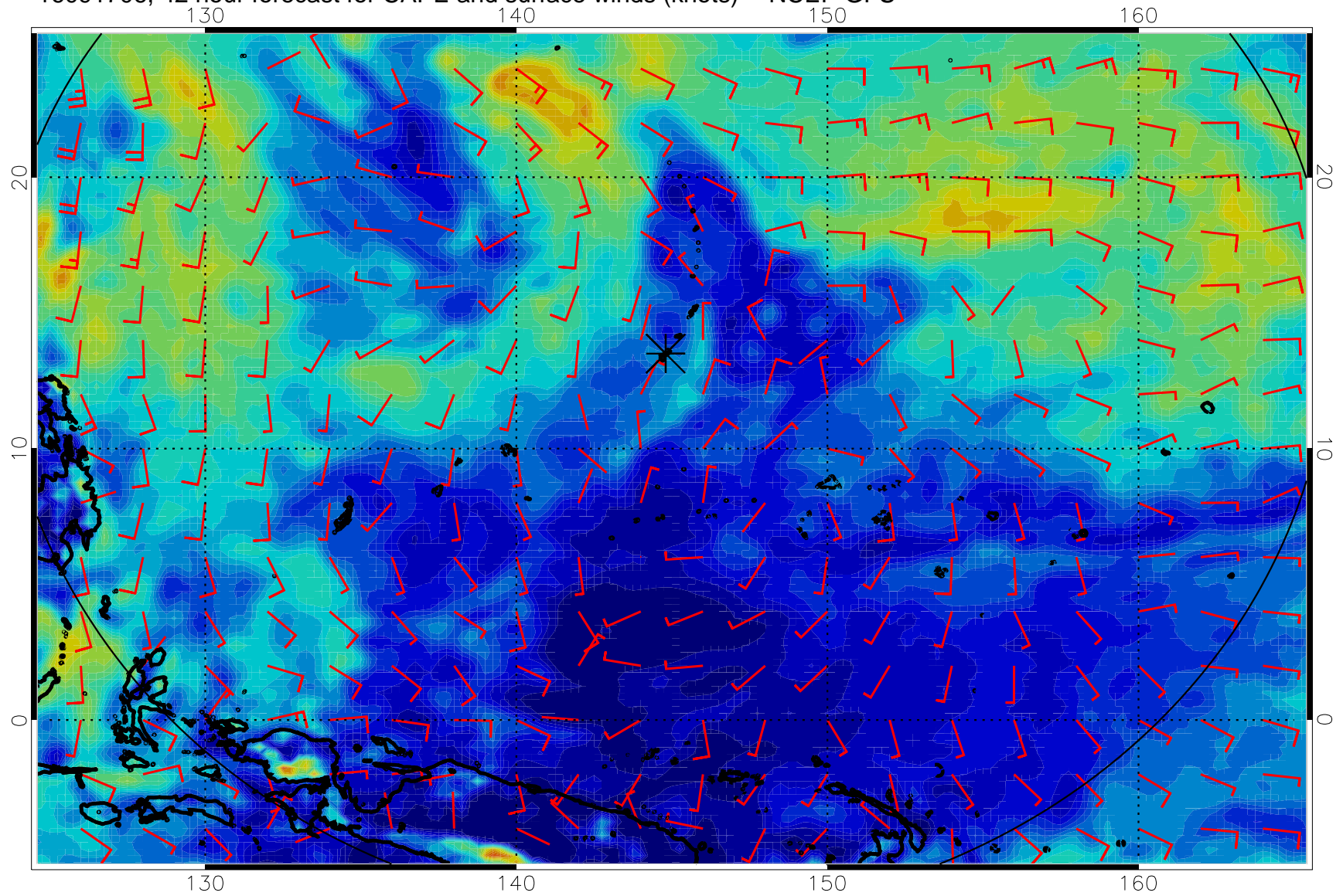
16091706, 42 hour forecast for CAPE and surface winds (knots) -- NCEP GFS
