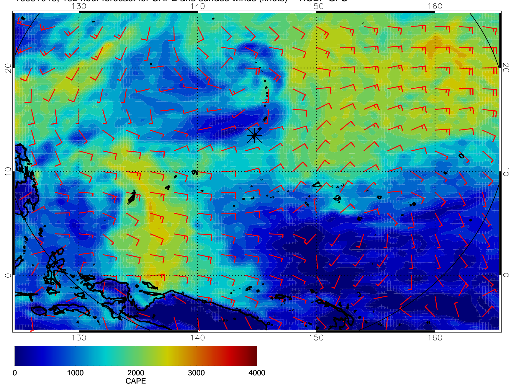
16091918, 102 hour forecast for CAPE and surface winds (knots) -- NCEP GFS
