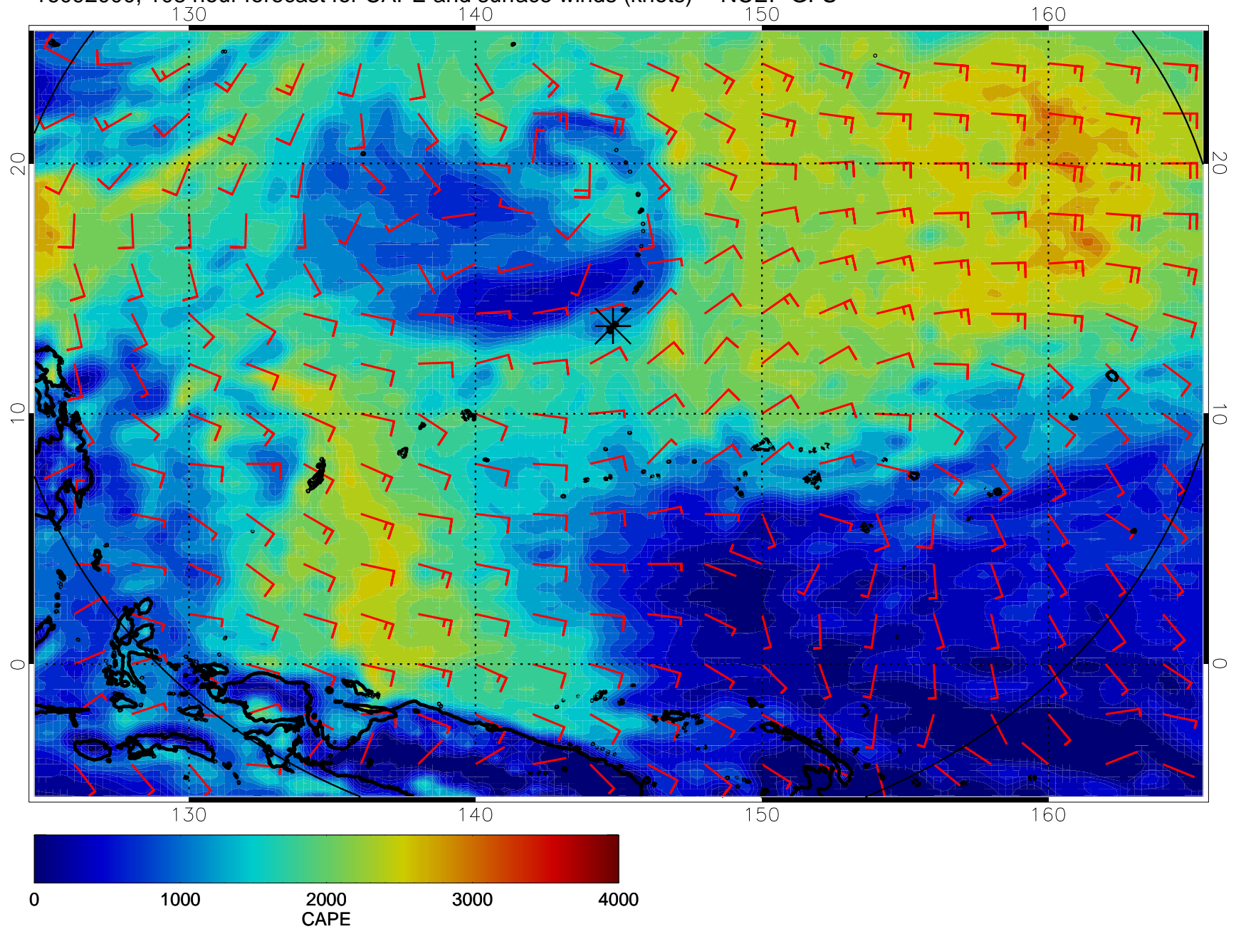
16092000, 108 hour forecast for CAPE and surface winds (knots) -- NCEP GFS
