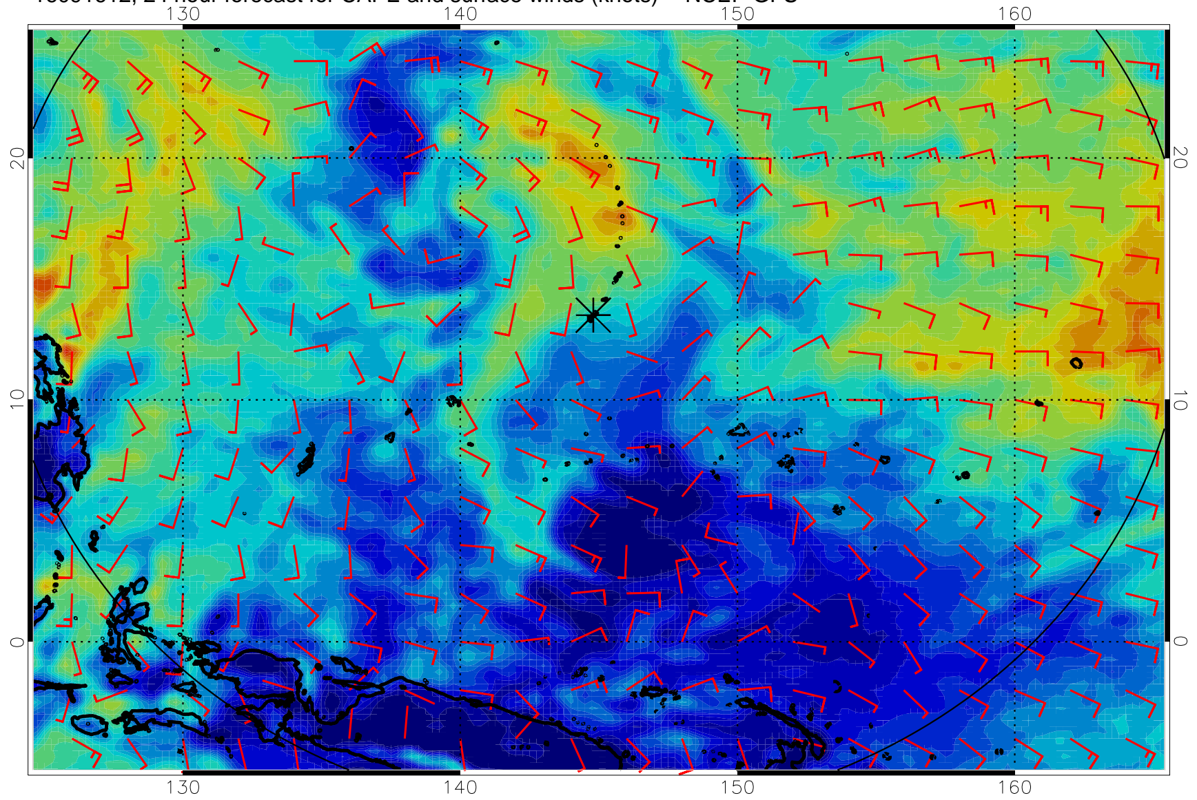
16091612, 24 hour forecast for CAPE and surface winds (knots) -- NCEP GFS
