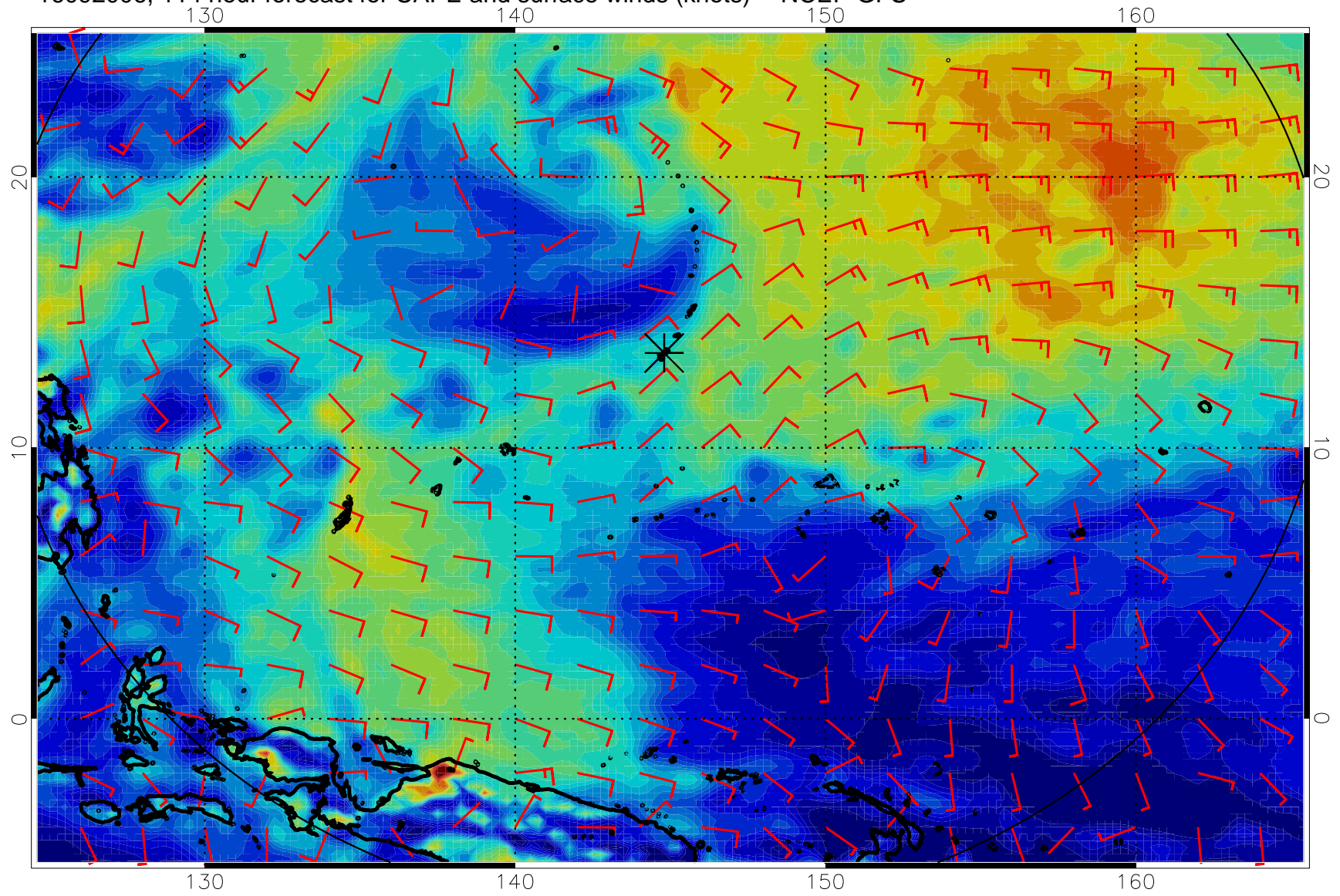
16092006, 114 hour forecast for CAPE and surface winds (knots) -- NCEP GFS
