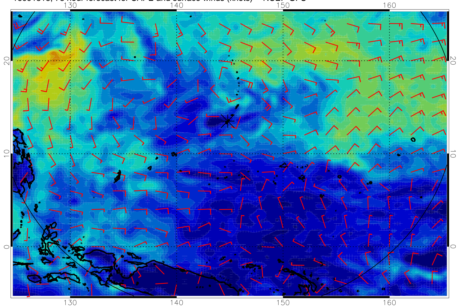
16091818, 78 hour forecast for CAPE and surface winds (knots) -- NCEP GFS
