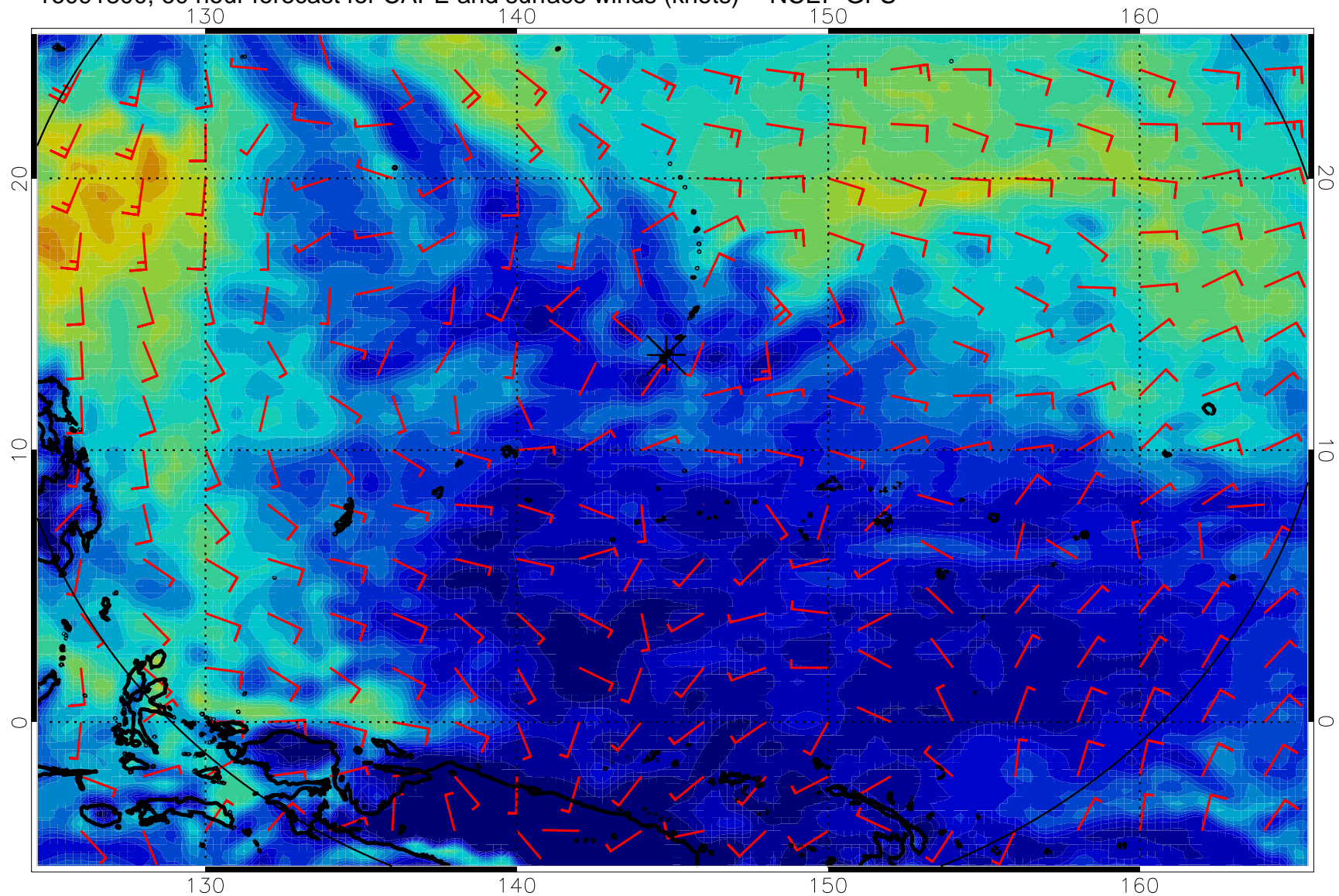
16091800, 60 hour forecast for CAPE and surface winds (knots) -- NCEP GFS
