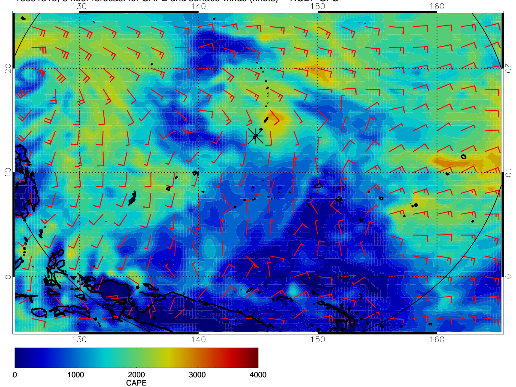
16091518, 6 hour forecast for CAPE and surface winds (knots) -- NCEP GFS
