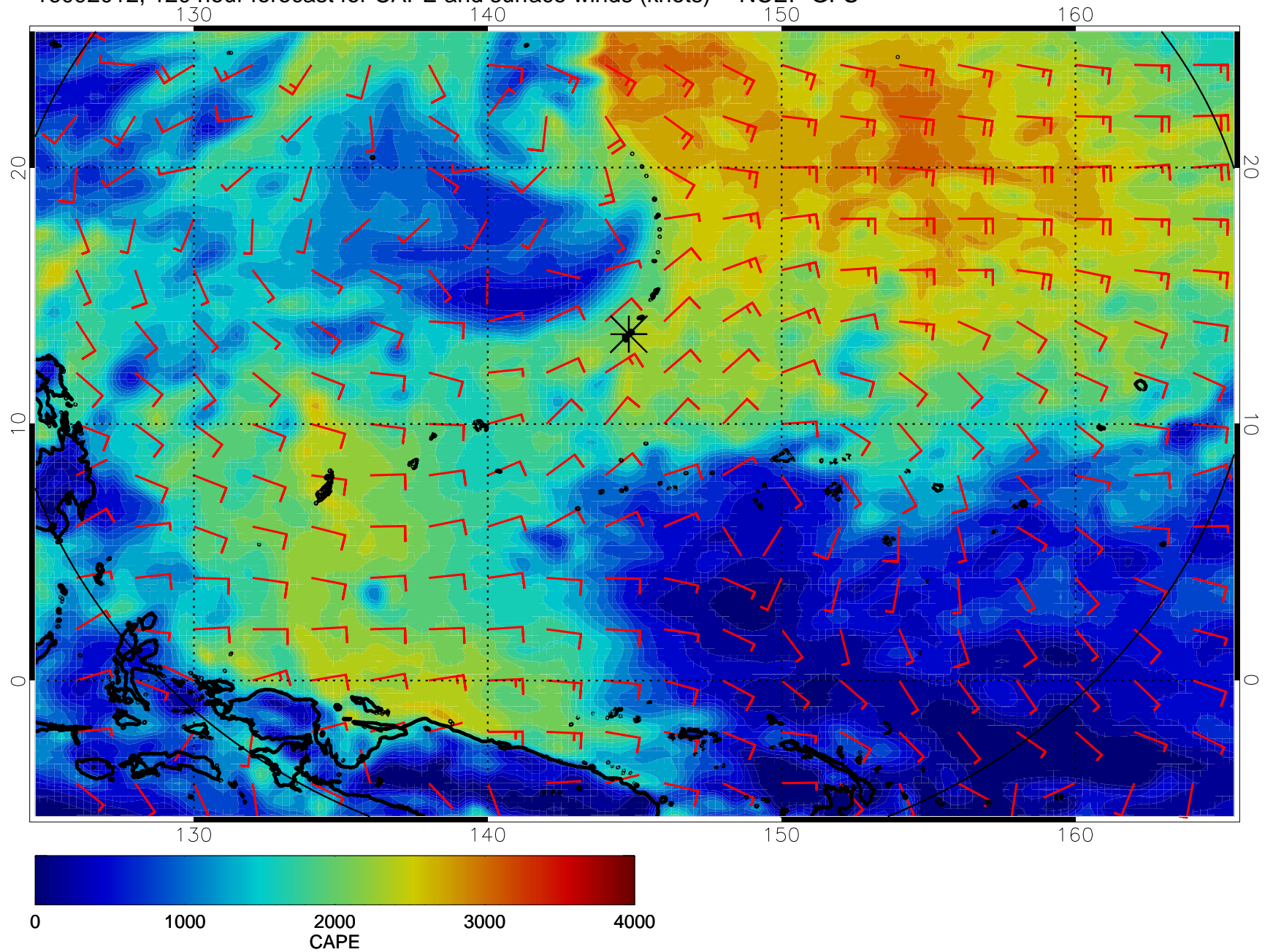
16092012, 120 hour forecast for CAPE and surface winds (knots) -- NCEP GFS
