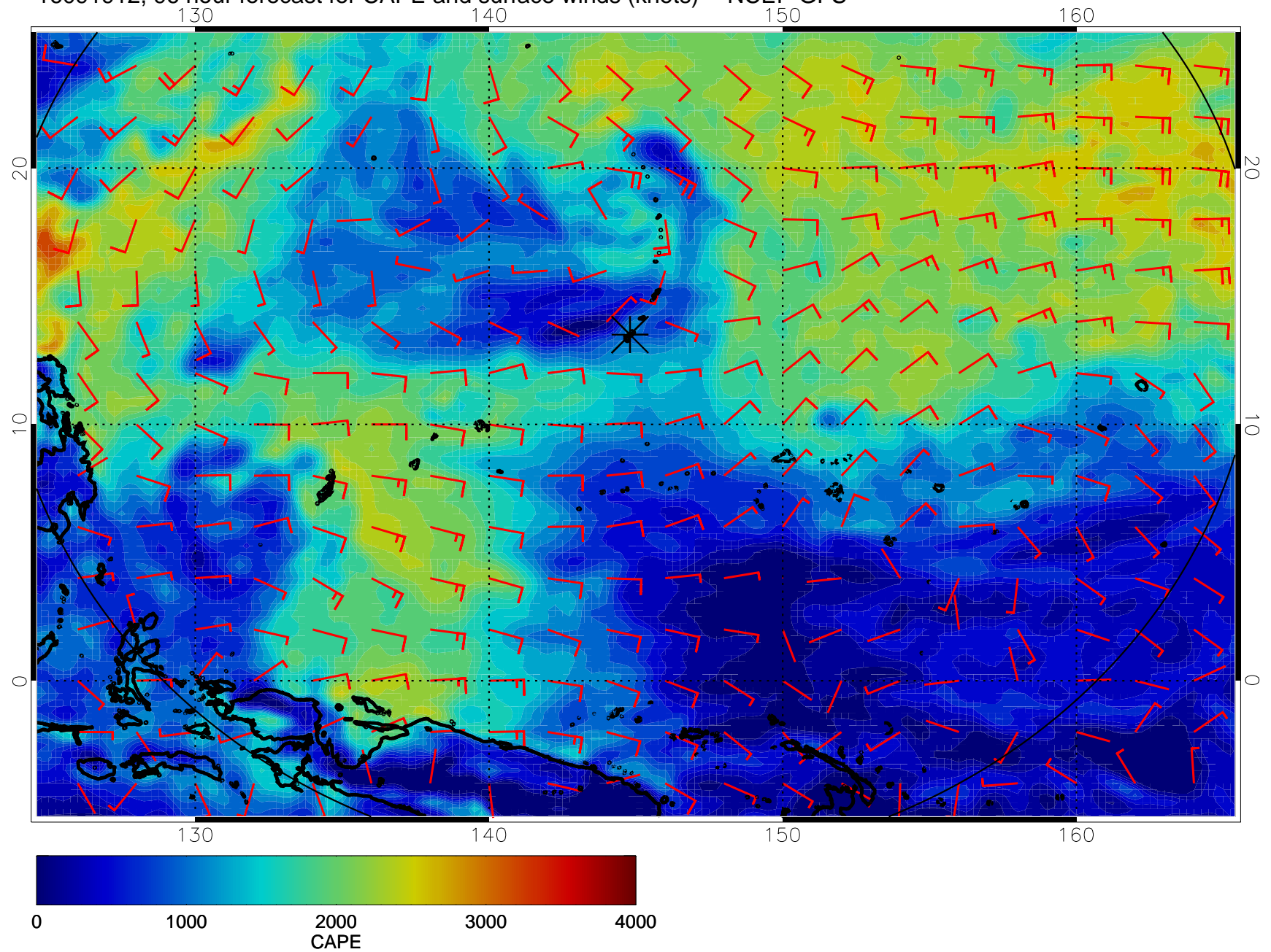
16091912, 96 hour forecast for CAPE and surface winds (knots) -- NCEP GFS
