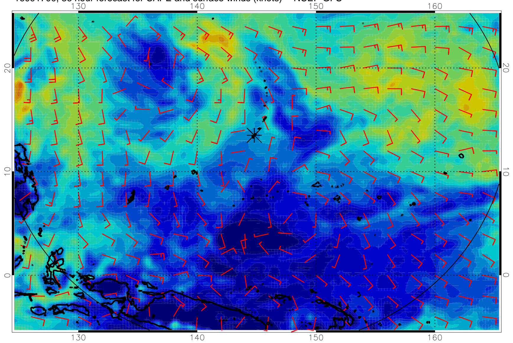
16091700, 36 hour forecast for CAPE and surface winds (knots) -- NCEP GFS
