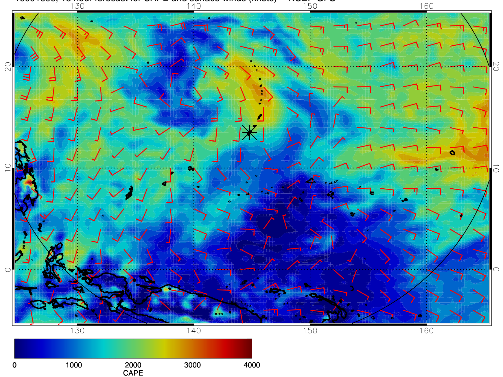
16091606, 18 hour forecast for CAPE and surface winds (knots) -- NCEP GFS
