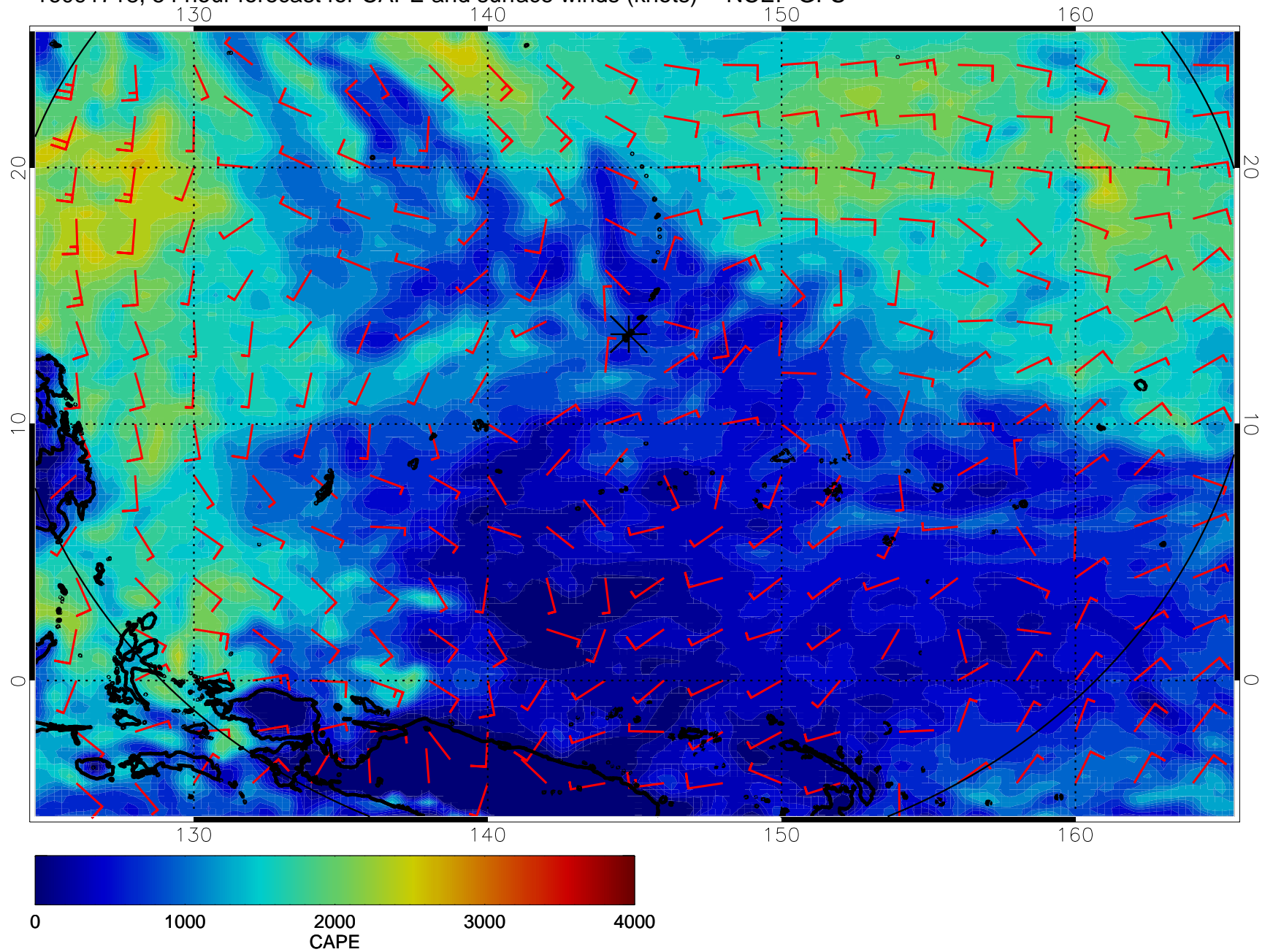
16091718, 54 hour forecast for CAPE and surface winds (knots) -- NCEP GFS
