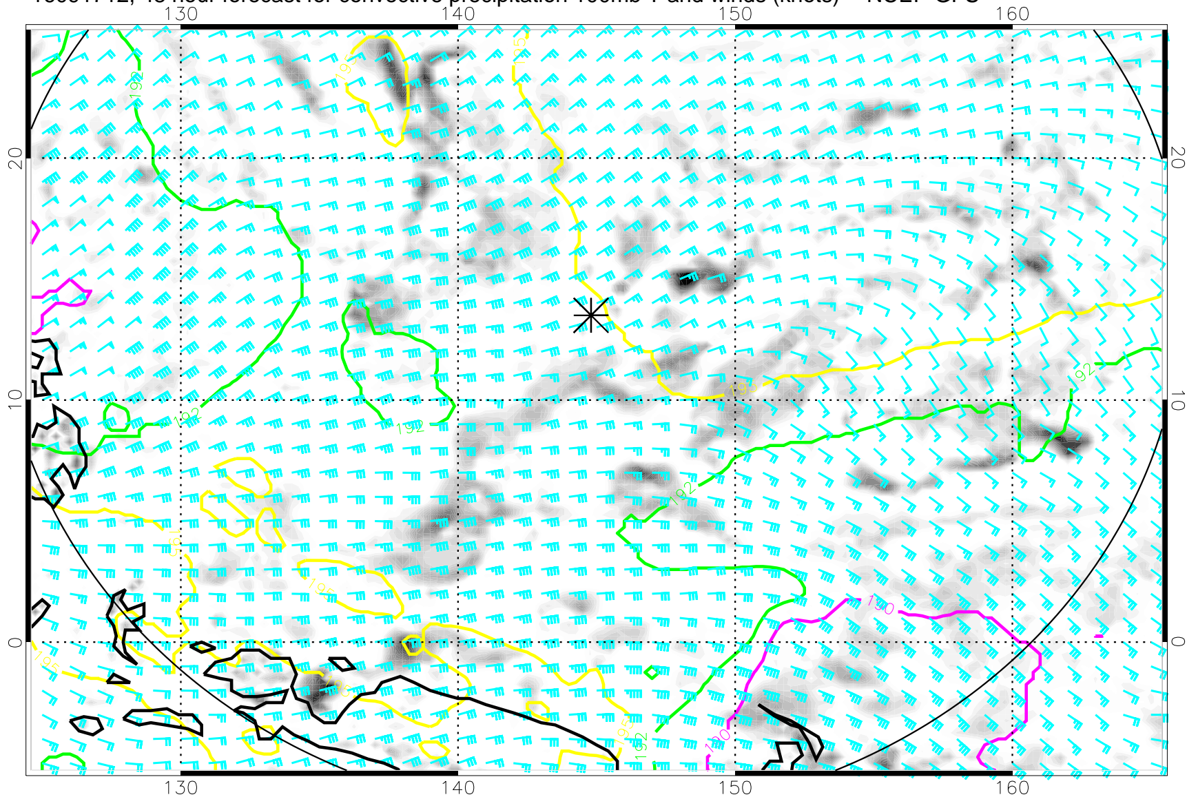
16091712, 48 hour forecast for convective precipitation 100mb T and winds (knots) -- NCEP GFS
