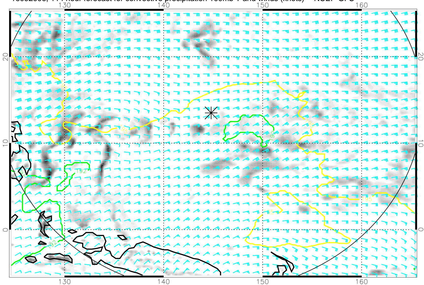
16092006, 114 hour forecast for convective precipitation 100mb T and winds (knots) -- NCEP GFS
