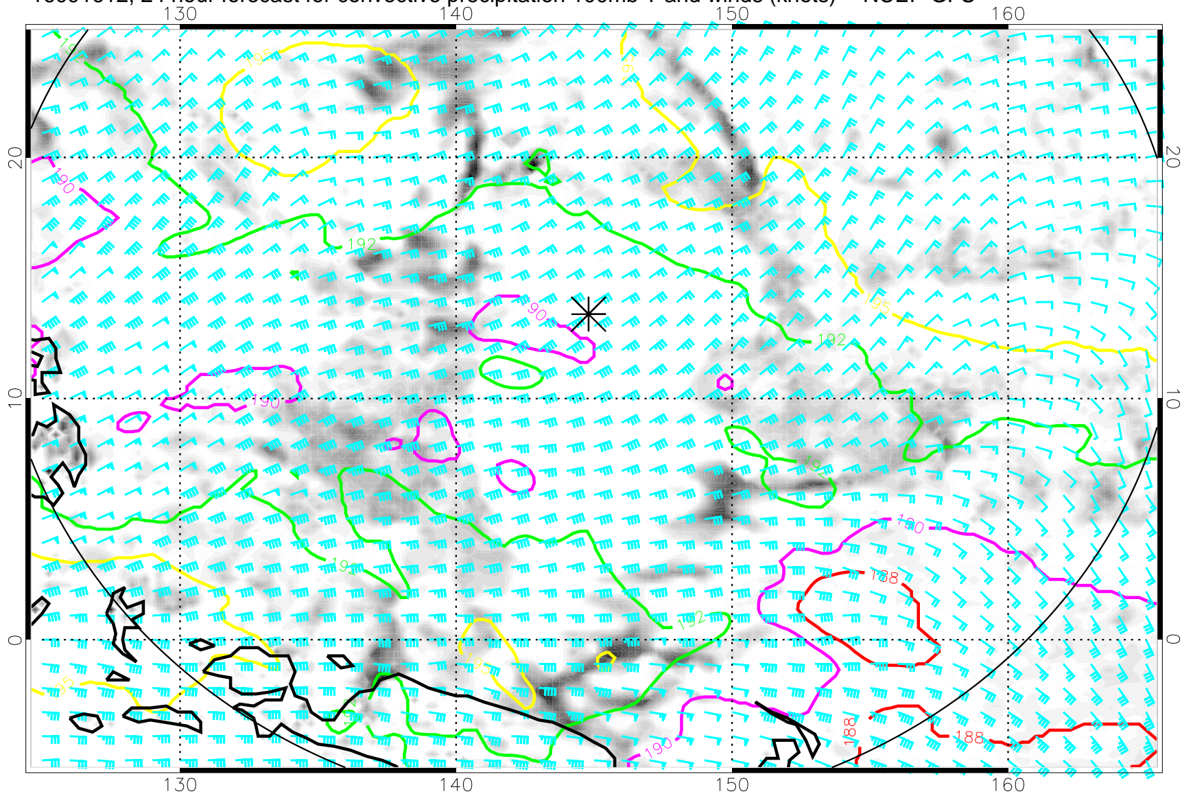
16091612, 24 hour forecast for convective precipitation 100mb T and winds (knots) -- NCEP GFS
