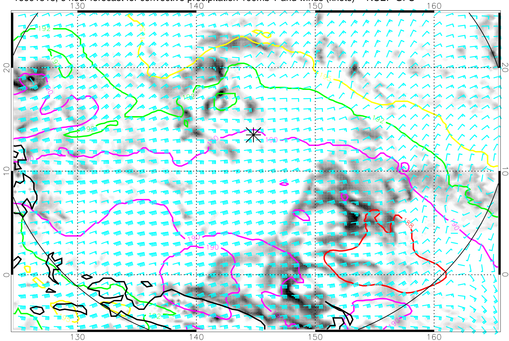
16091518, 6 hour forecast for convective precipitation 100mb T and winds (knots) -- NCEP GFS
