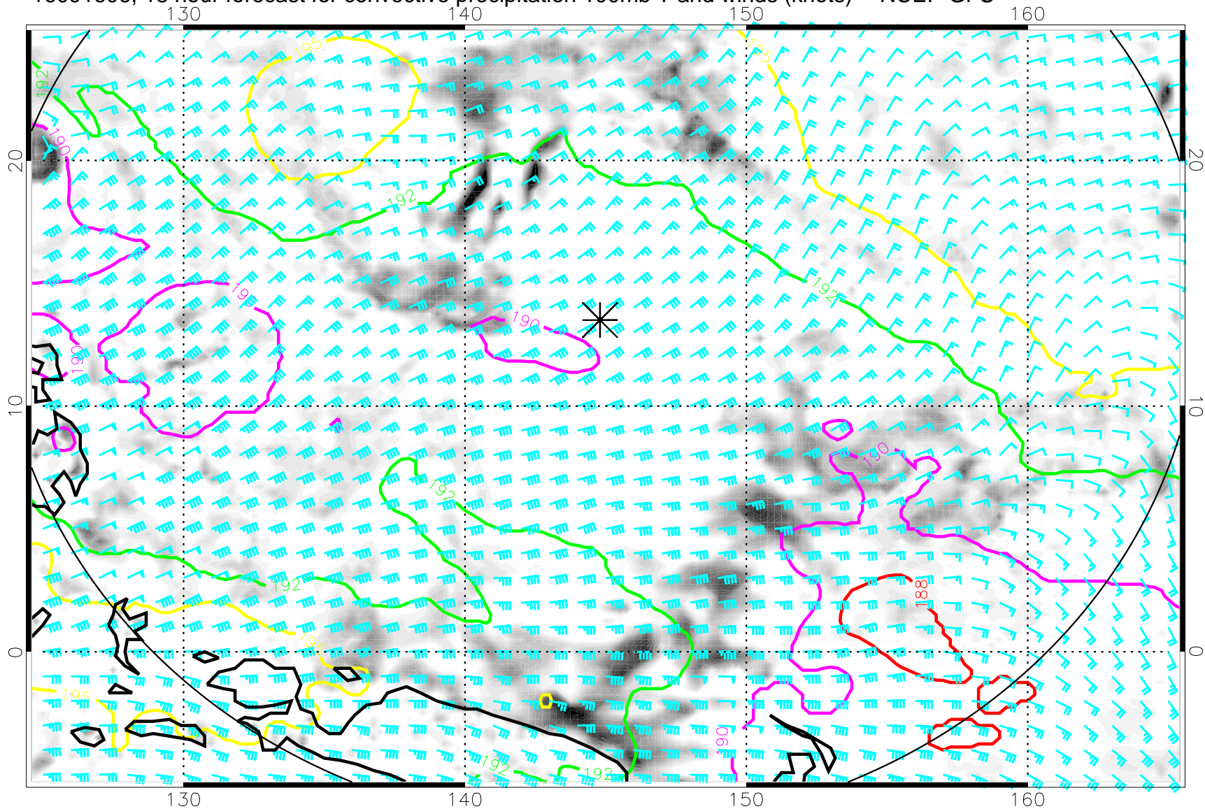
16091606, 18 hour forecast for convective precipitation 100mb T and winds (knots) -- NCEP GFS
