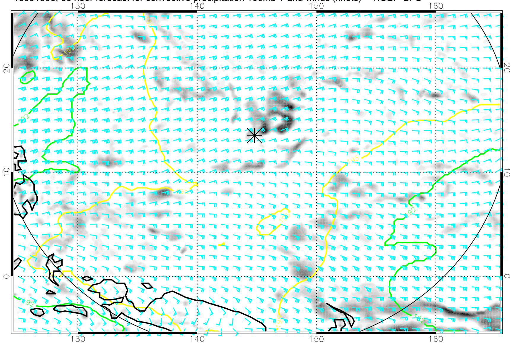
16091806, 66 hour forecast for convective precipitation 100mb T and winds (knots) -- NCEP GFS
