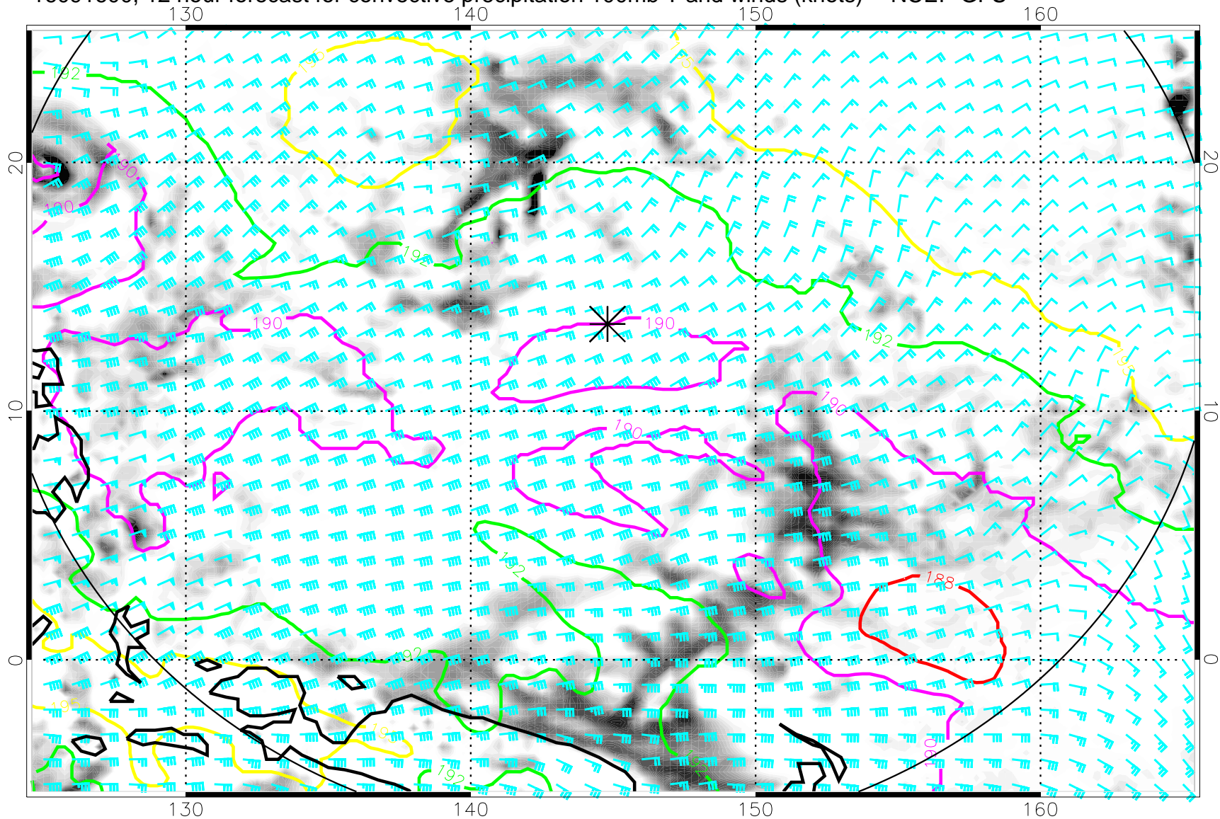
16091600, 12 hour forecast for convective precipitation 100mb T and winds (knots) -- NCEP GFS
