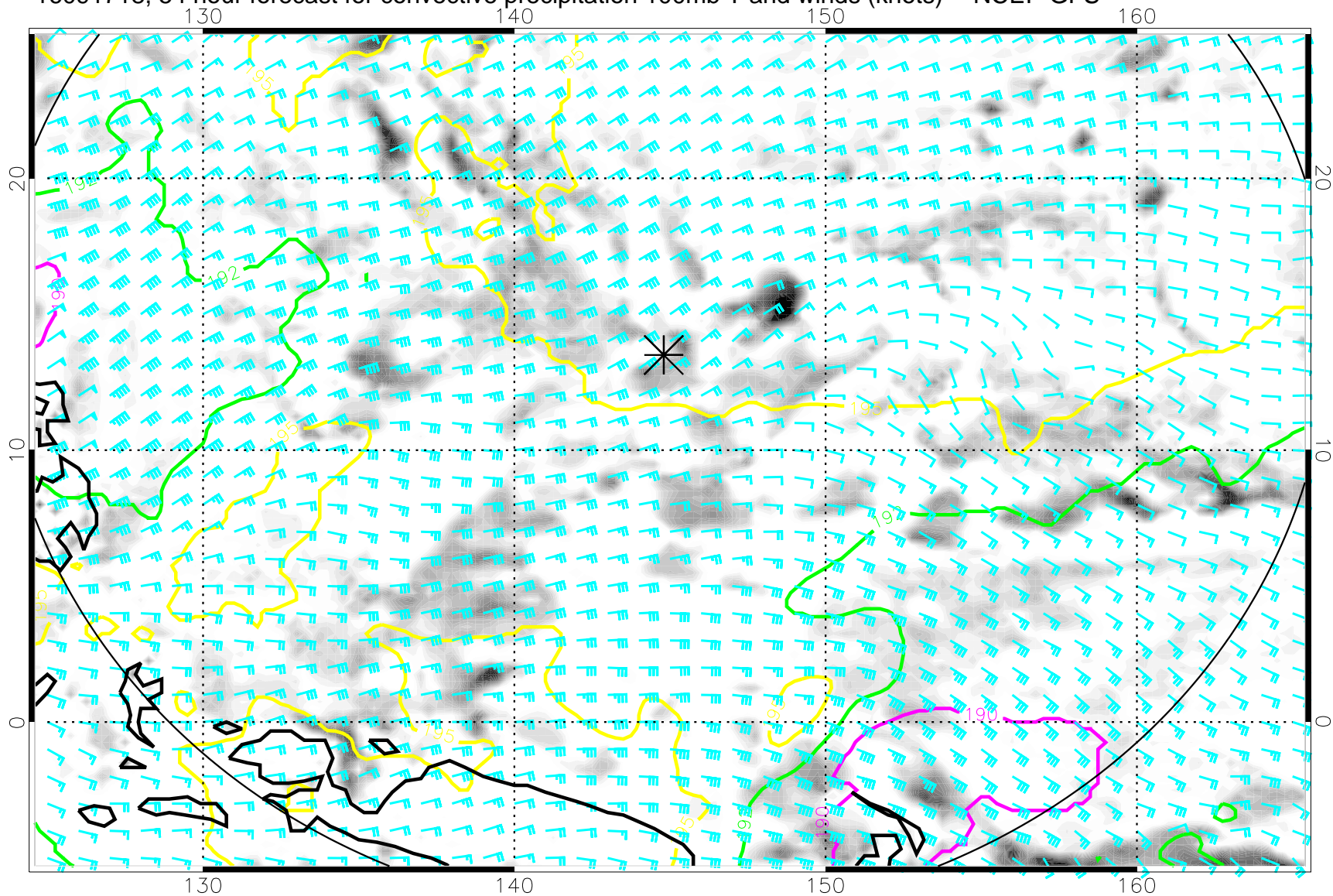
16091718, 54 hour forecast for convective precipitation 100mb T and winds (knots) -- NCEP GFS
