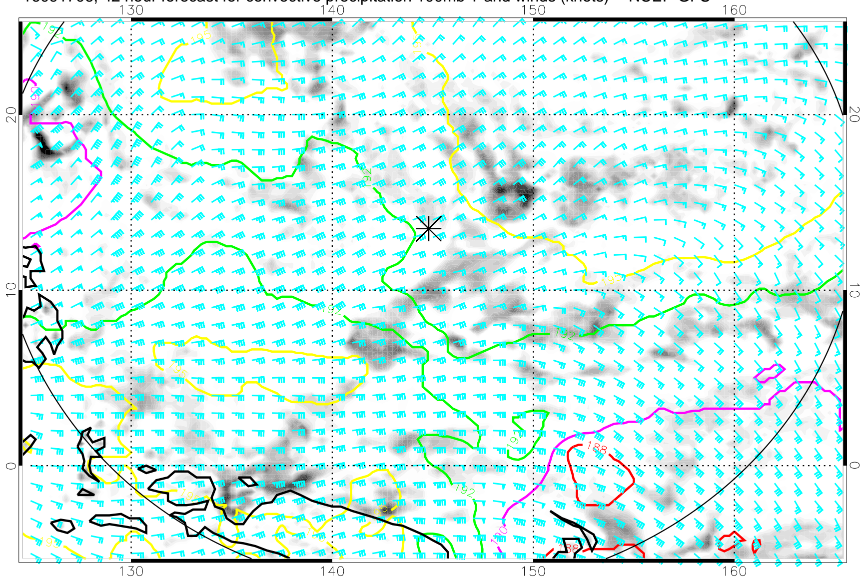
16091706, 42 hour forecast for convective precipitation 100mb T and winds (knots) -- NCEP GFS
