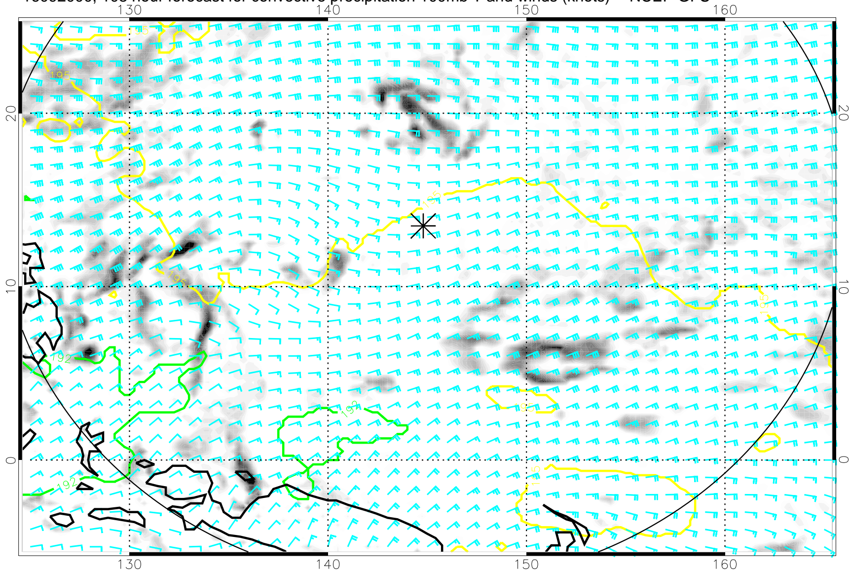
16092000, 108 hour forecast for convective precipitation 100mb T and winds (knots) -- NCEP GFS
