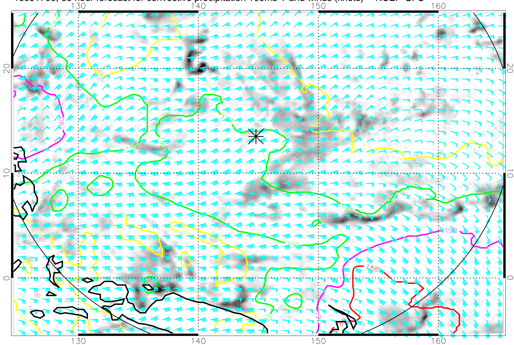
16091700, 36 hour forecast for convective precipitation 100mb T and winds (knots) -- NCEP GFS
