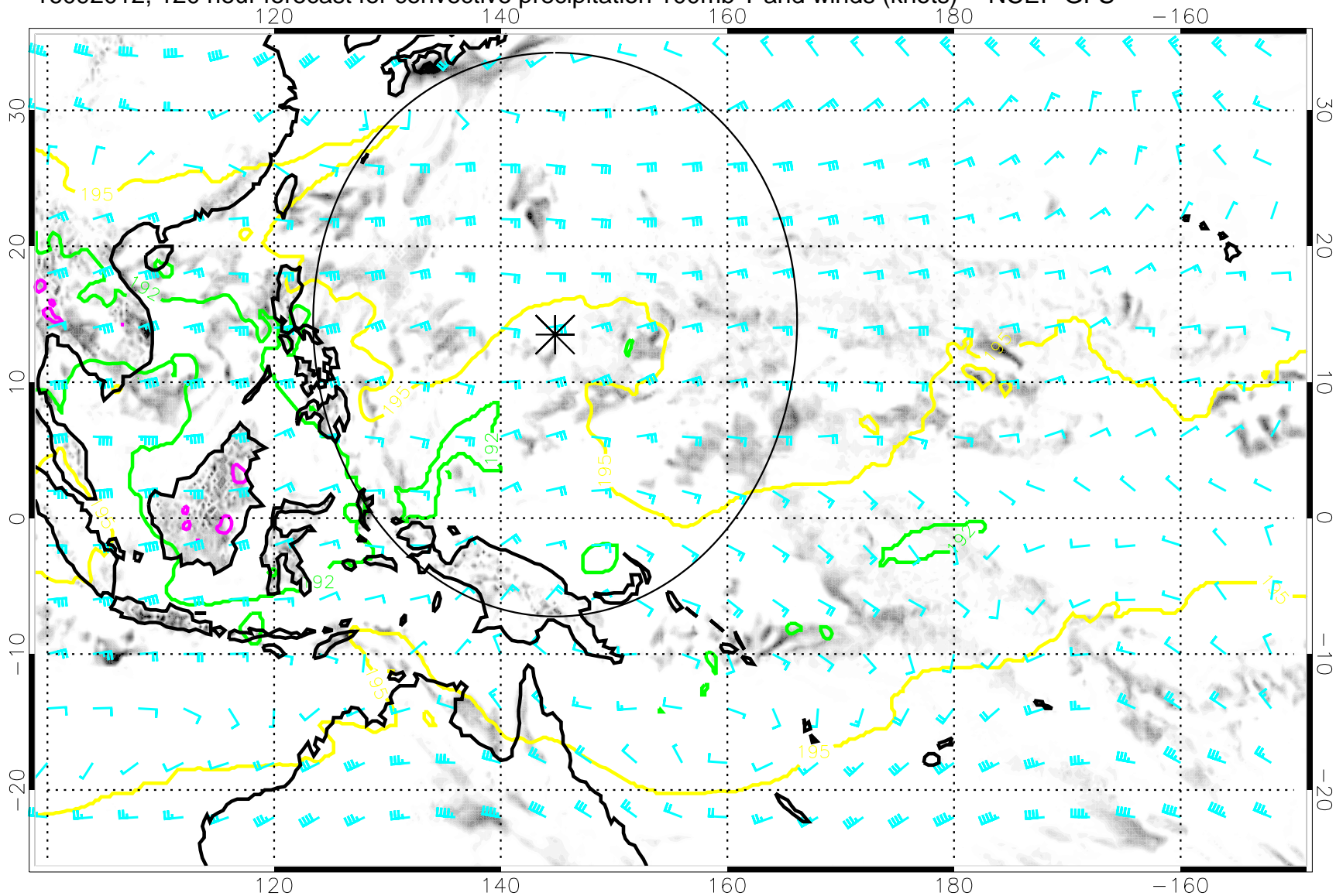
16092012, 120 hour forecast for convective precipitation 100mb T and winds (knots) -- NCEP GFS
