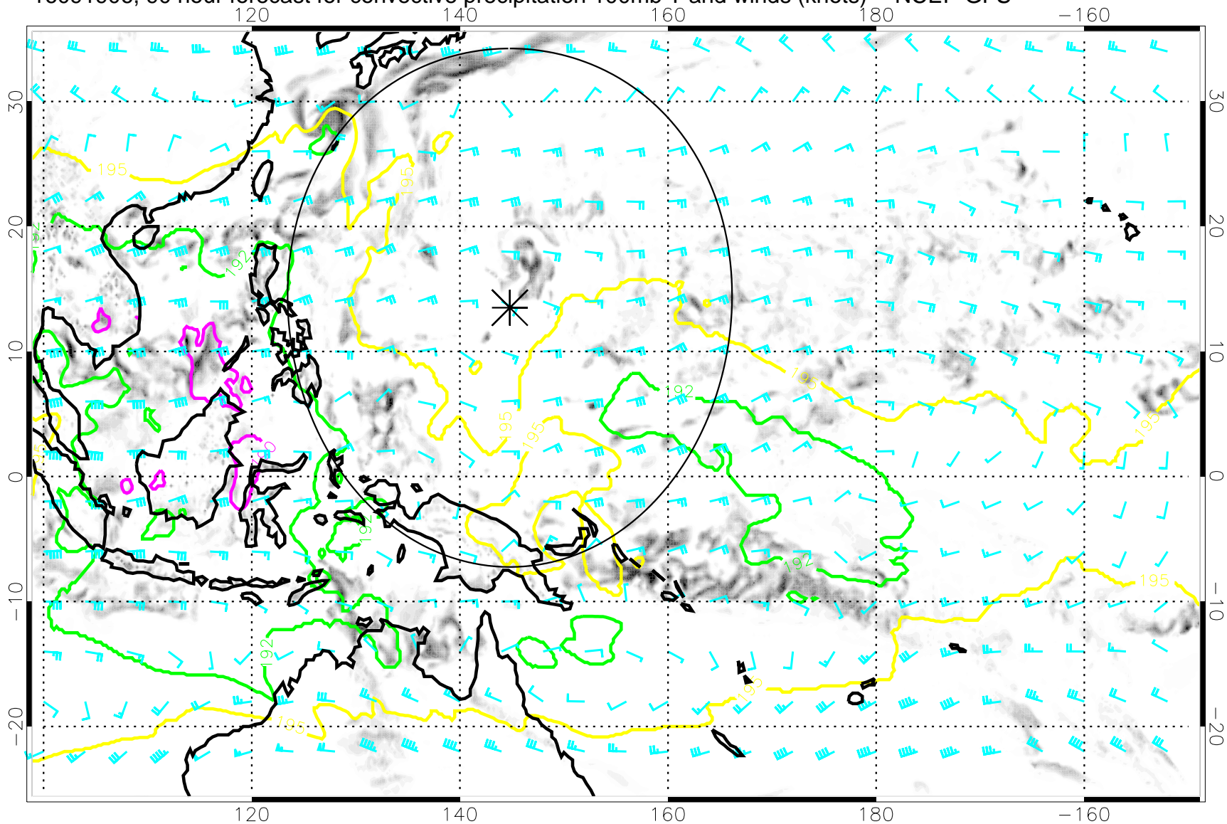
16091906, 90 hour forecast for convective precipitation 100mb T and winds (knots) -- NCEP GFS
