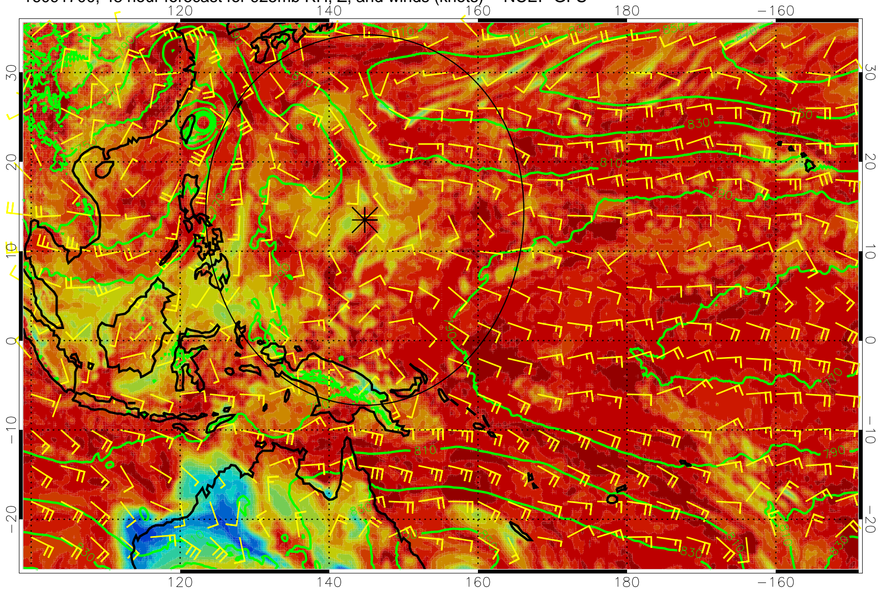
16091700, 48 hour forecast for 925mb RH, Z, and winds (knots) -- NCEP GFS
