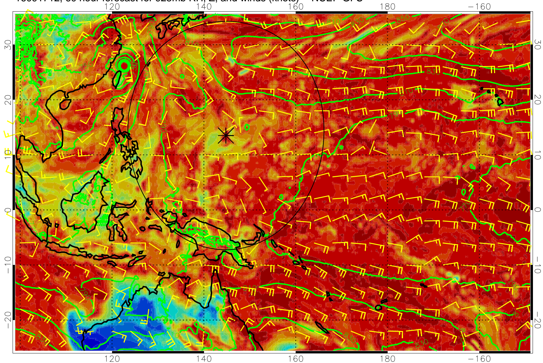
16091712, 60 hour forecast for 925mb RH, Z, and winds (knots) -- NCEP GFS
