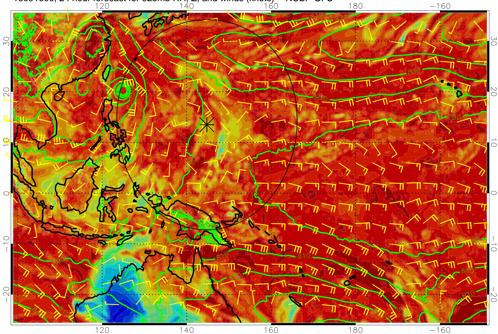
16091600, 24 hour forecast for 925mb RH, Z, and winds (knots) -- NCEP GFS
