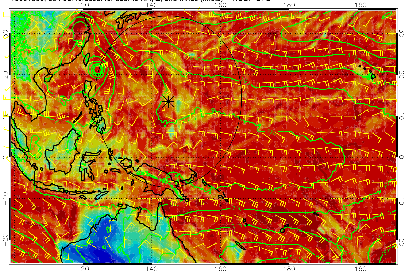
16091606, 30 hour forecast for 925mb RH, Z, and winds (knots) -- NCEP GFS
