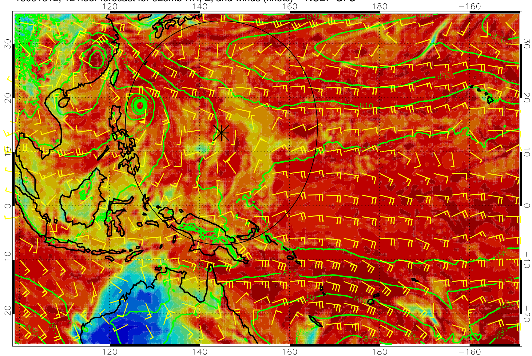
16091512, 12 hour forecast for 925mb RH, Z, and winds (knots) -- NCEP GFS
