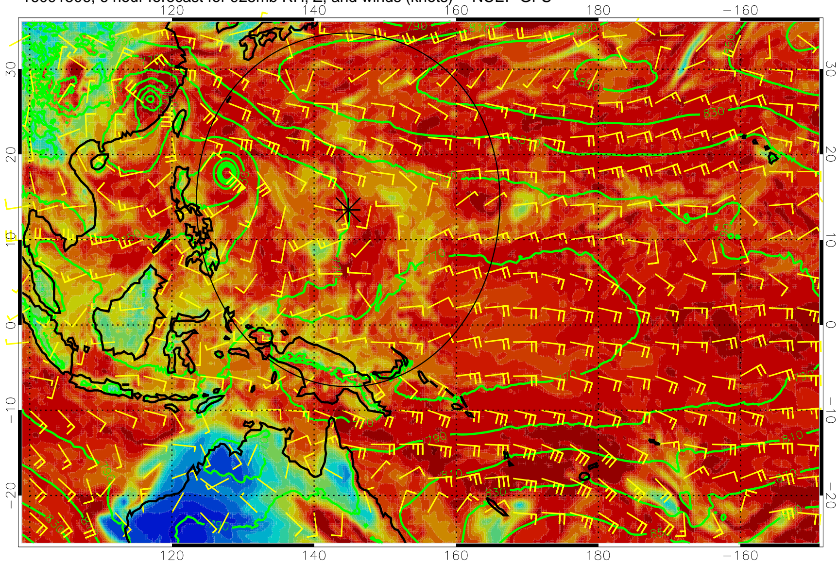
16091506, 6 hour forecast for 925mb RH, Z, and winds (knots) -- NCEP GFS
