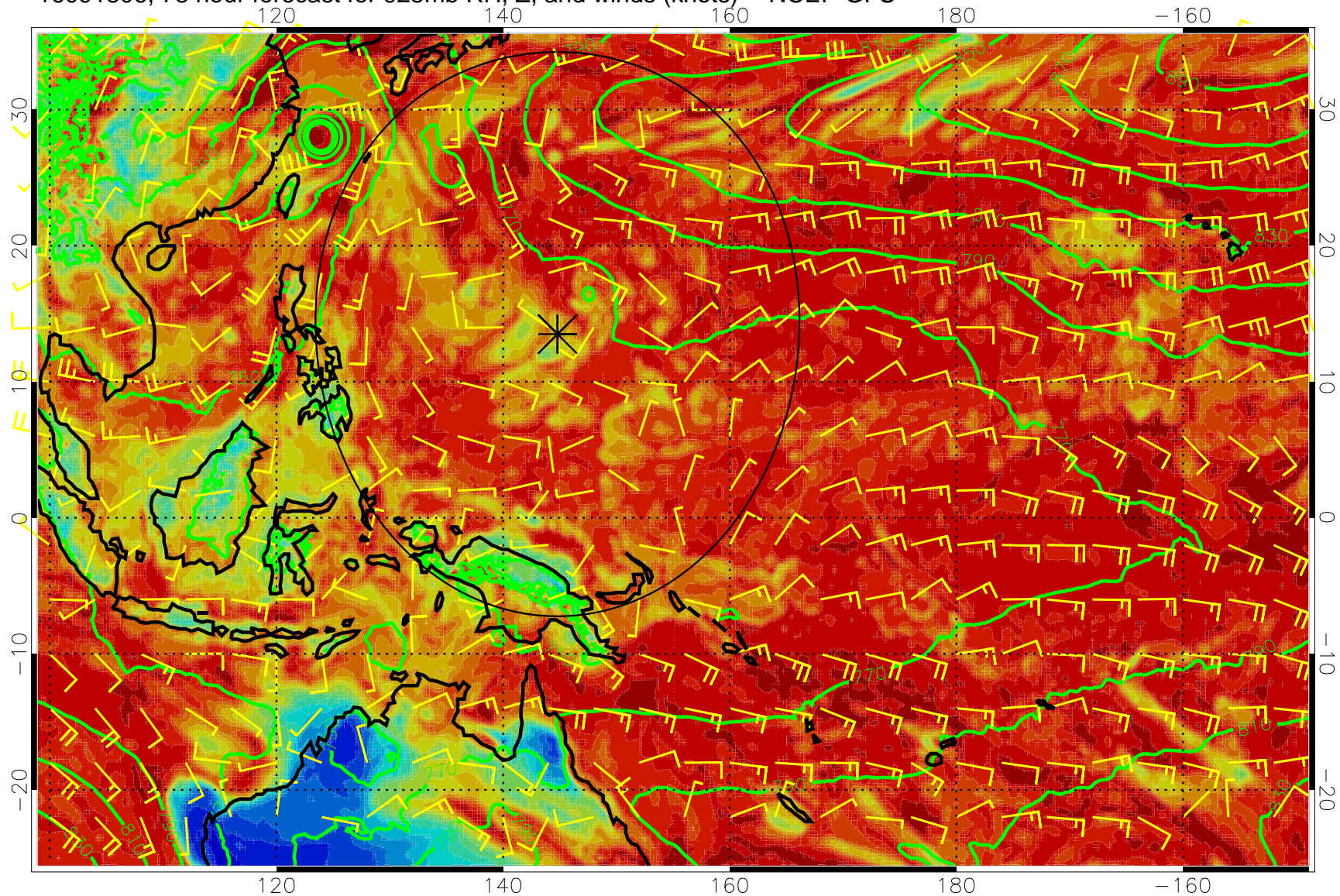
16091806, 78 hour forecast for 925mb RH, Z, and winds (knots) -- NCEP GFS
