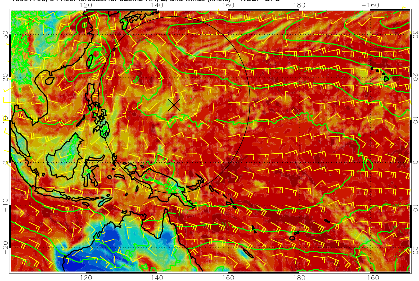
16091706, 54 hour forecast for 925mb RH, Z, and winds (knots) -- NCEP GFS
