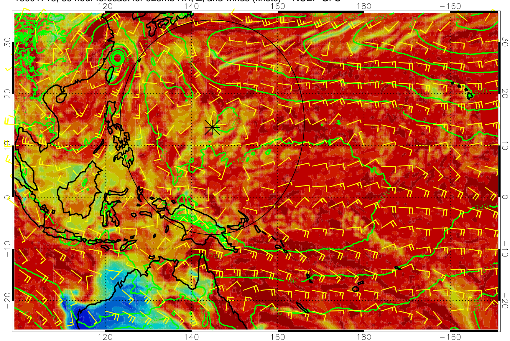
16091718, 66 hour forecast for 925mb RH, Z, and winds (knots) -- NCEP GFS
