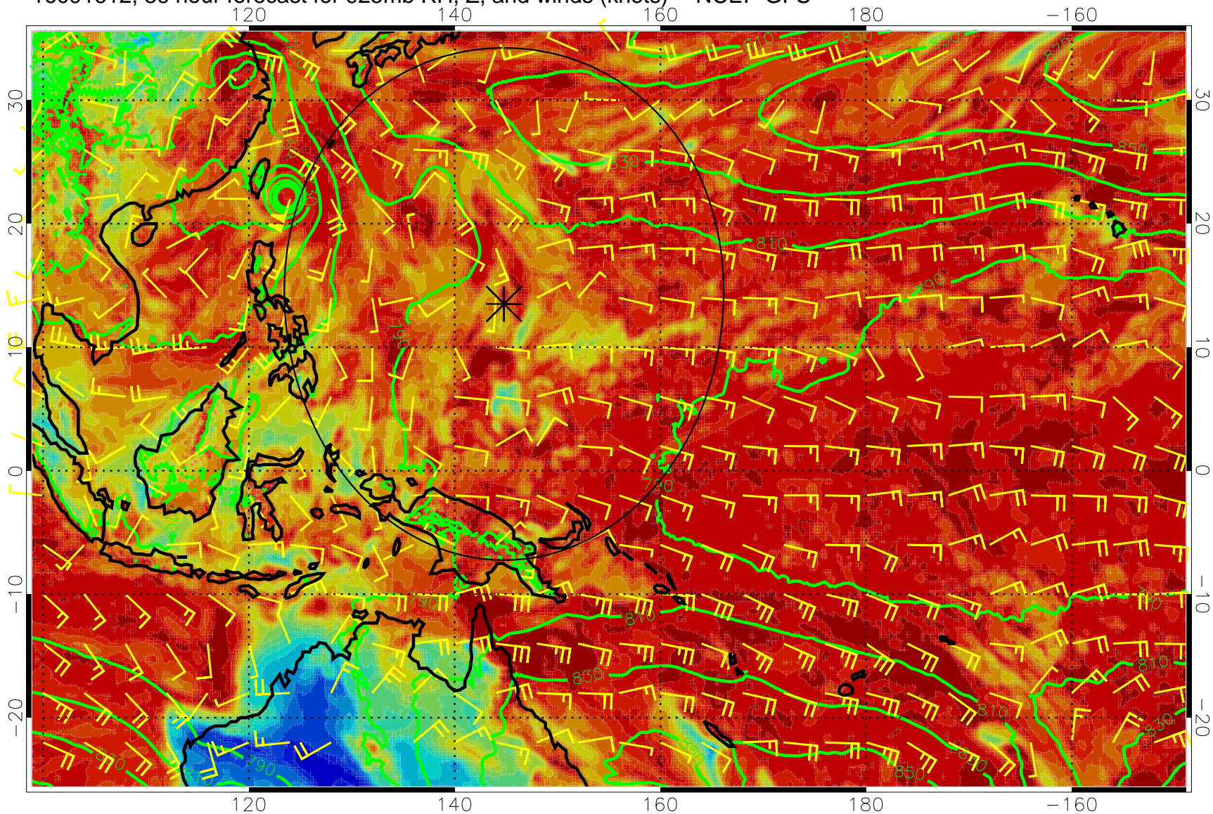
16091612, 36 hour forecast for 925mb RH, Z, and winds (knots) -- NCEP GFS
