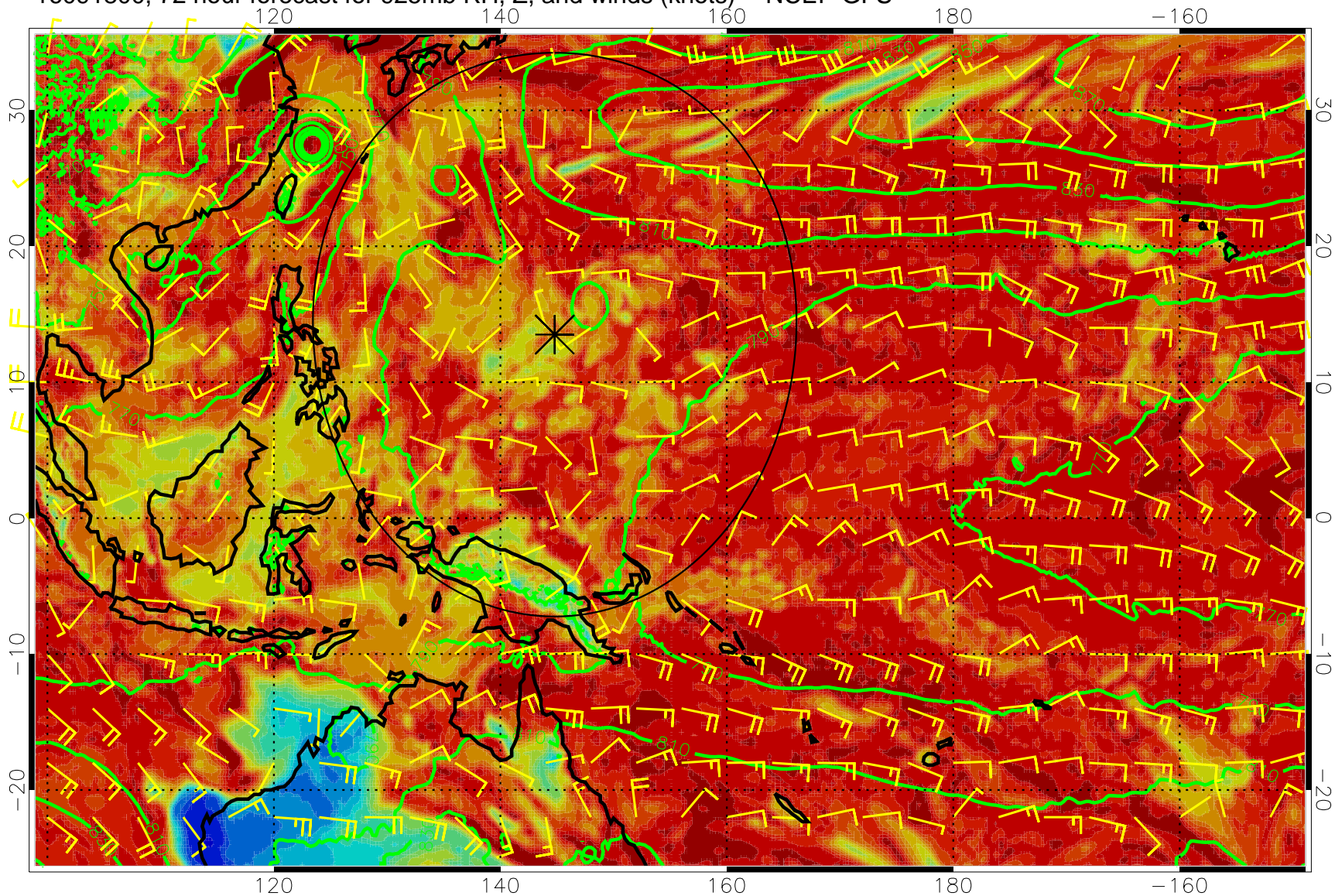
16091800, 72 hour forecast for 925mb RH, Z, and winds (knots) -- NCEP GFS
