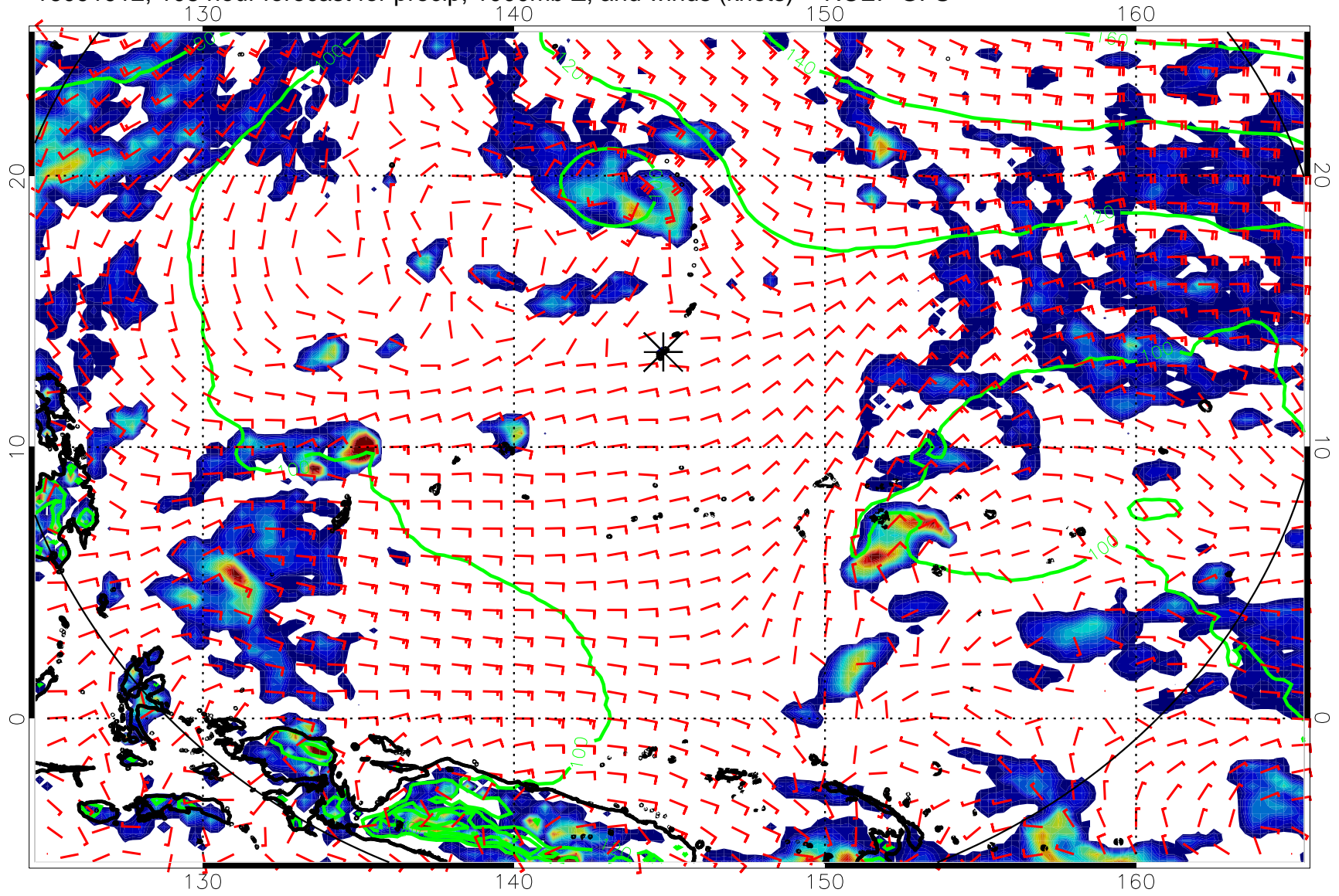
16091912, 108 hour forecast for precip, 1000mb Z, and winds (knots) -- NCEP GFS
