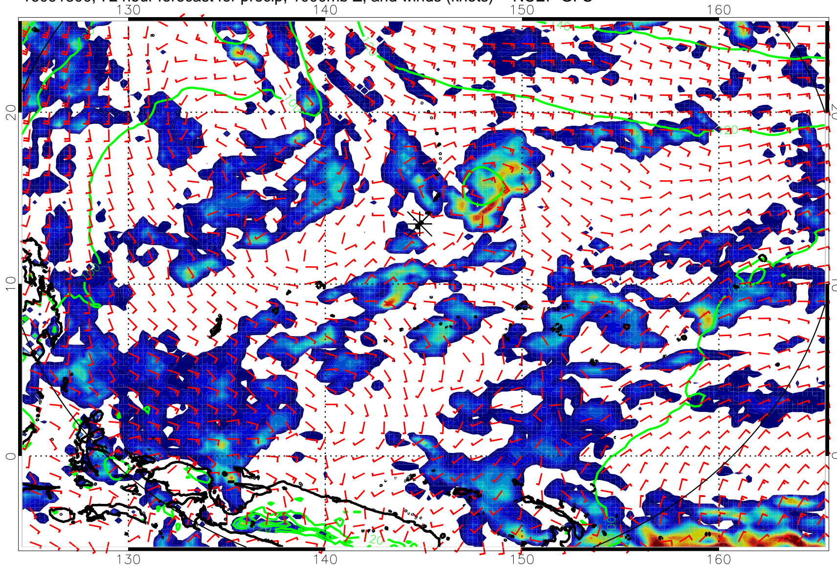
16091800, 72 hour forecast for precip, 1000mb Z, and winds (knots) -- NCEP GFS
