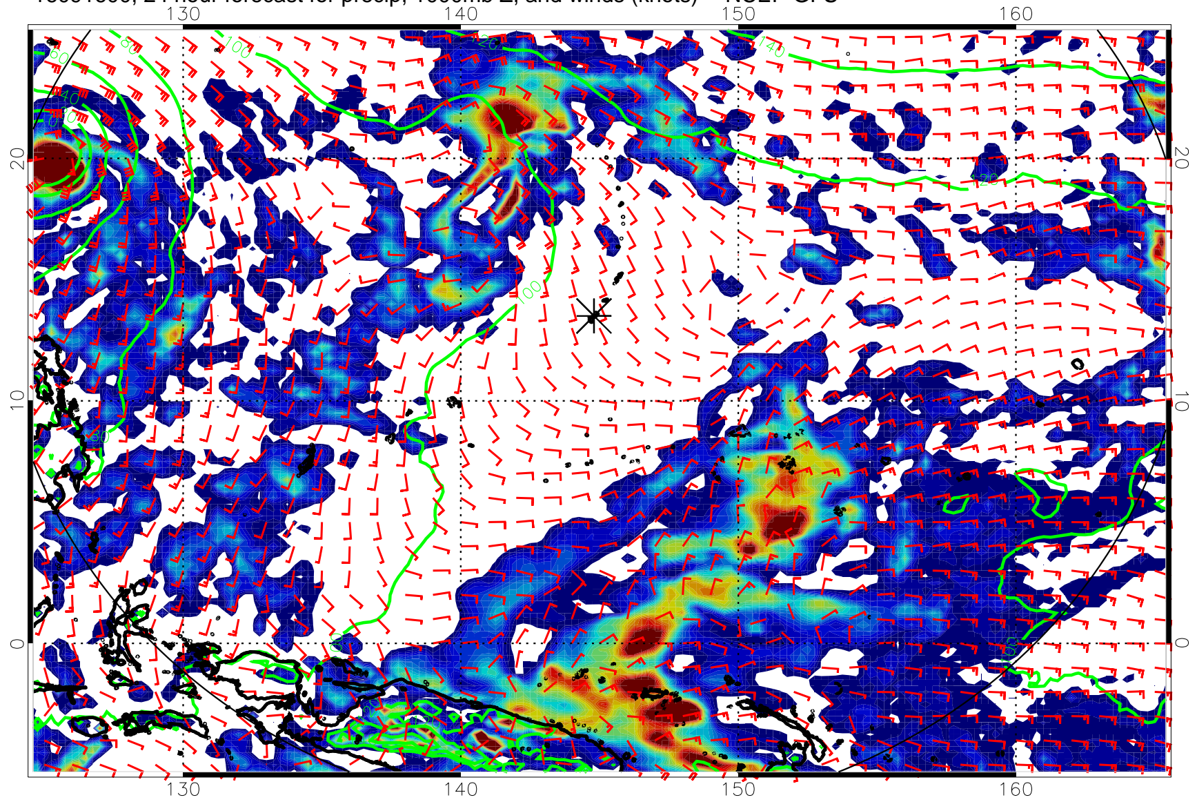
16091600, 24 hour forecast for precip, 1000mb Z, and winds (knots) -- NCEP GFS
