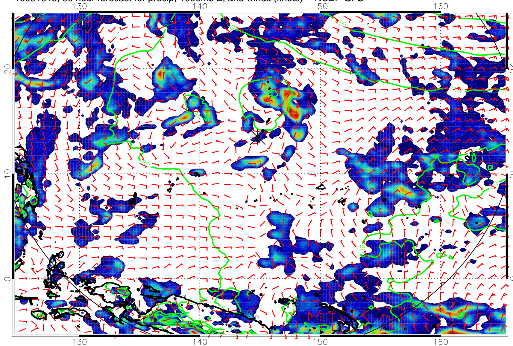
16091818, 90 hour forecast for precip, 1000mb Z, and winds (knots) -- NCEP GFS
