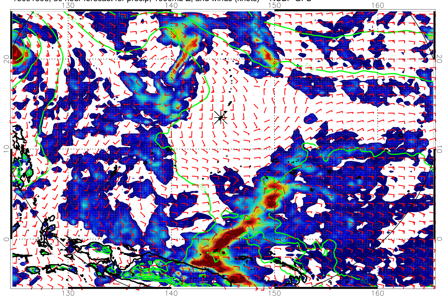
16091606, 30 hour forecast for precip, 1000mb Z, and winds (knots) -- NCEP GFS
