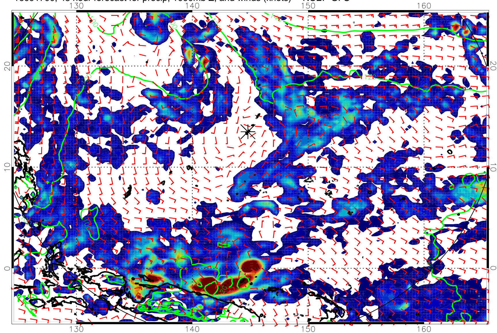
16091700, 48 hour forecast for precip, 1000mb Z, and winds (knots) -- NCEP GFS
