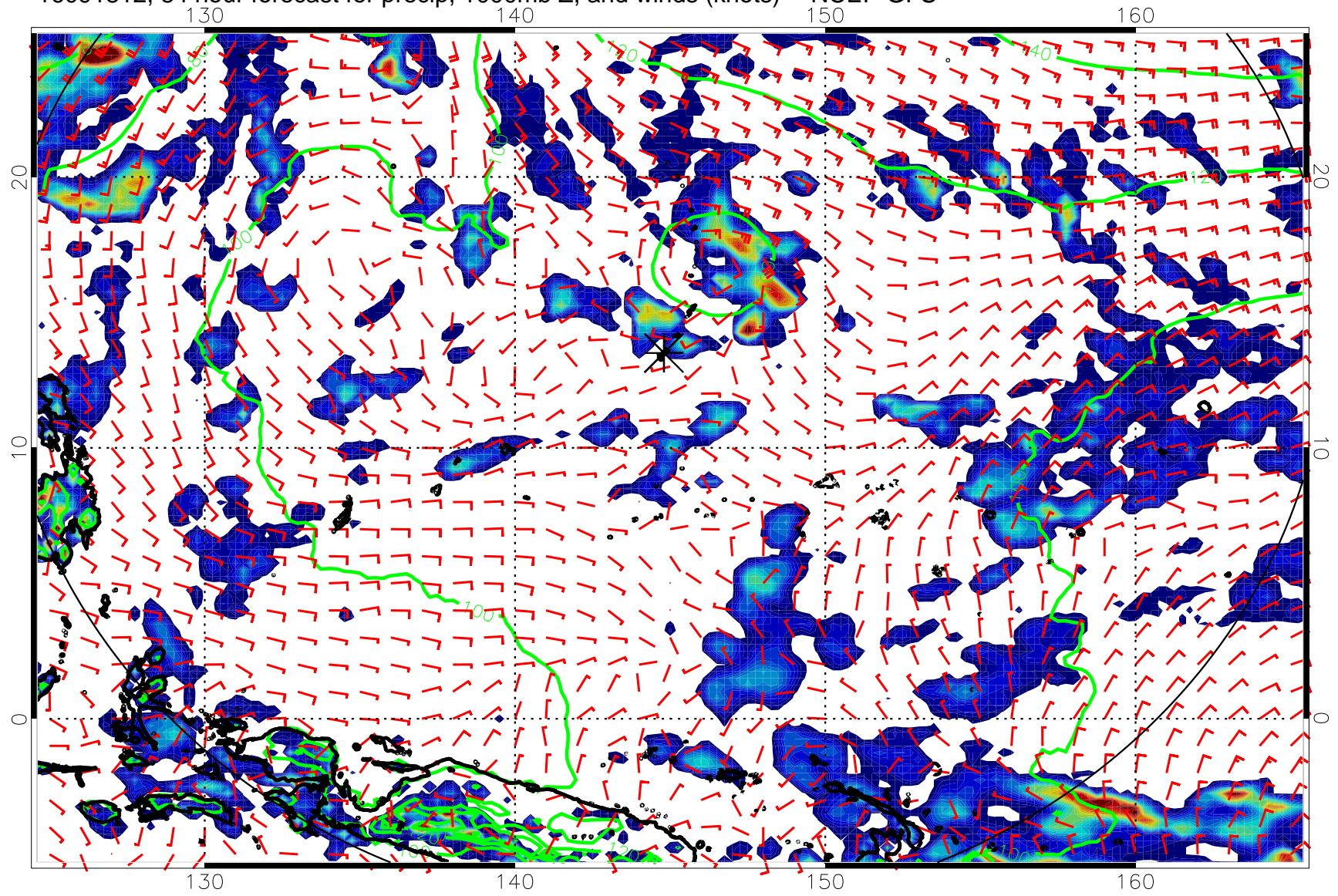
16091812, 84 hour forecast for precip, 1000mb Z, and winds (knots) -- NCEP GFS
