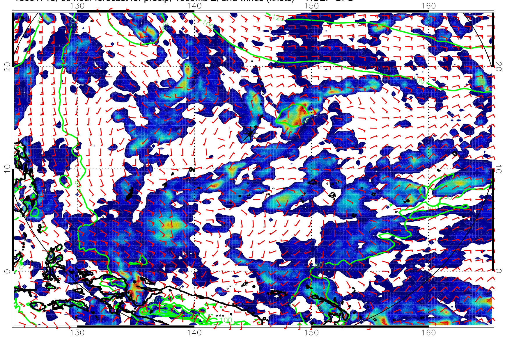
16091718, 66 hour forecast for precip, 1000mb Z, and winds (knots) -- NCEP GFS
