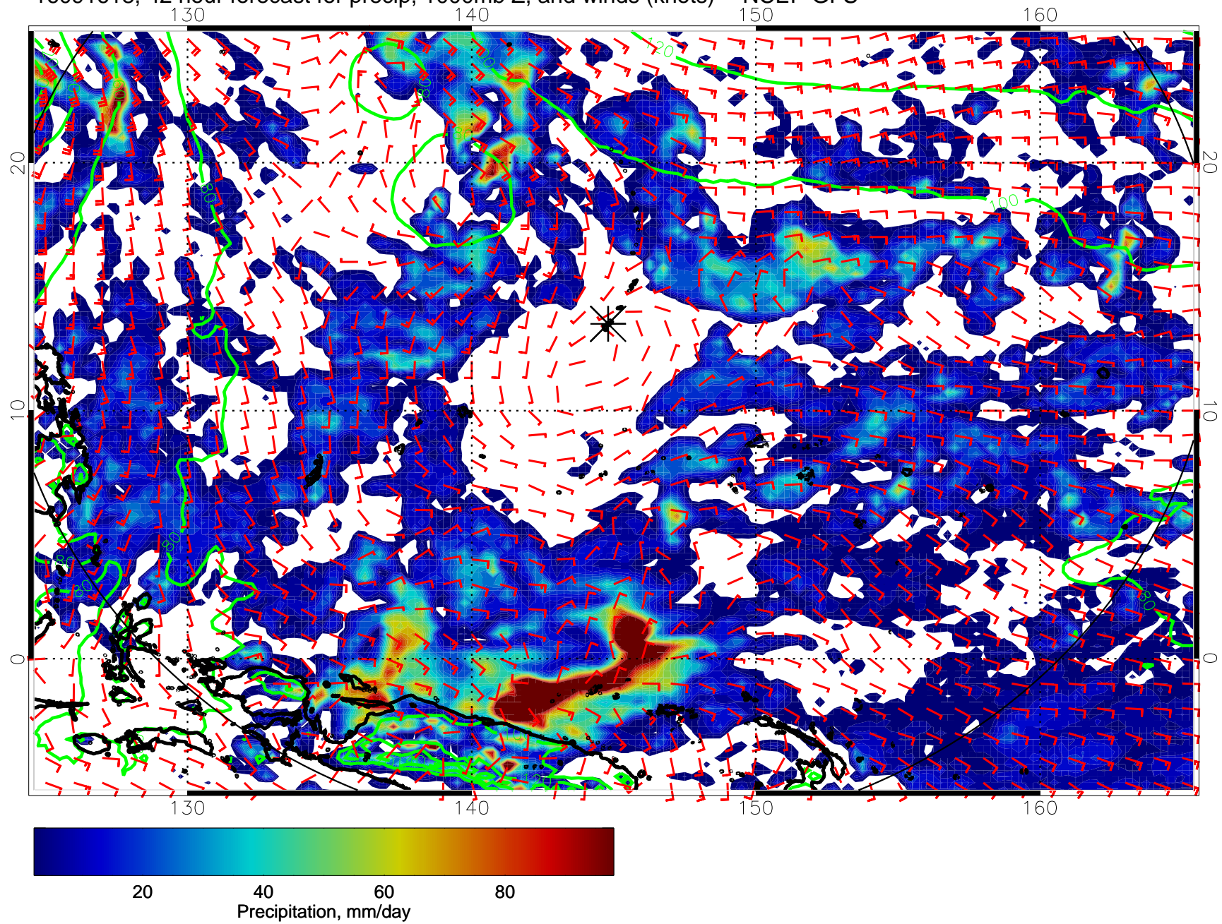
16091618, 42 hour forecast for precip, 1000mb Z, and winds (knots) -- NCEP GFS
