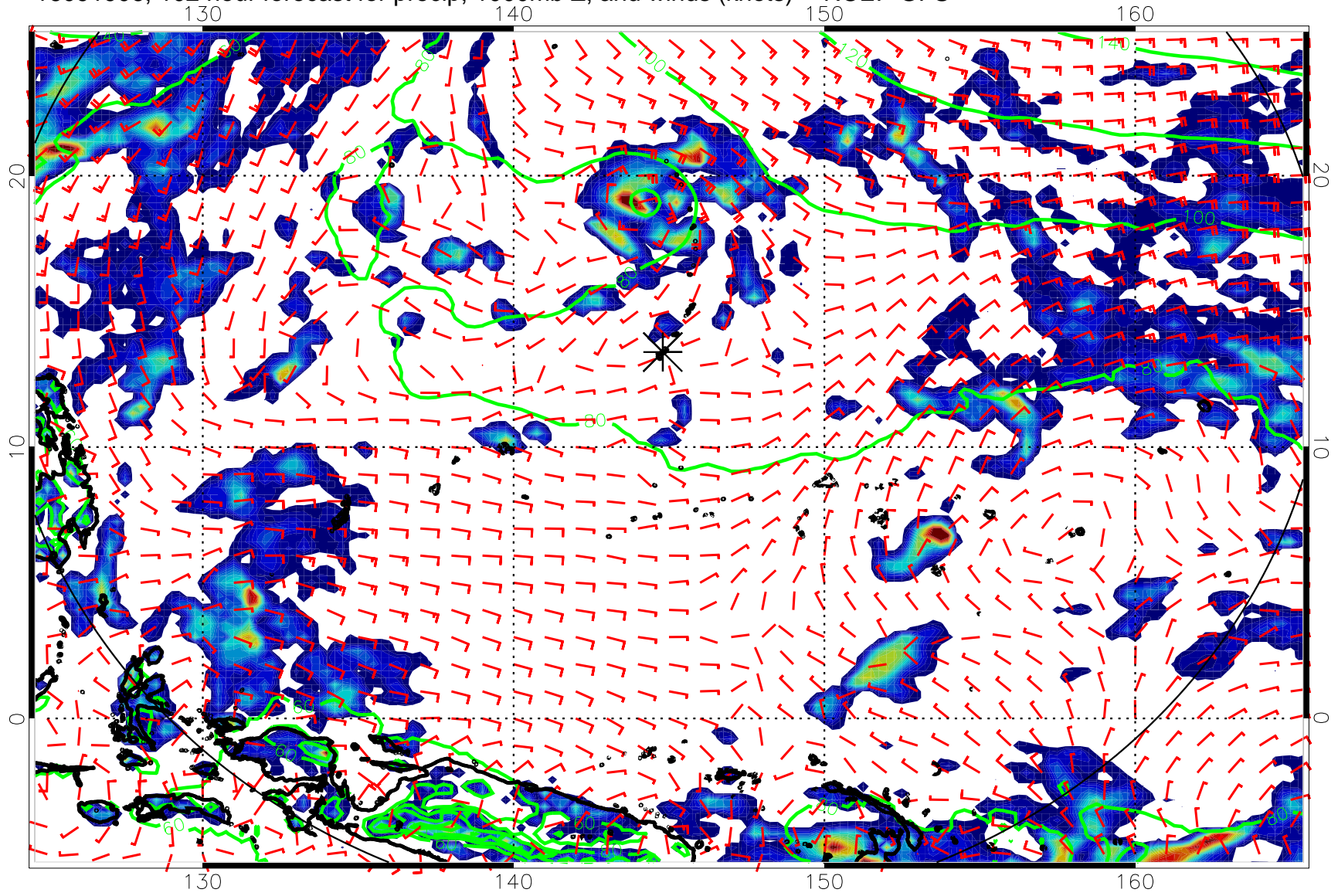
16091906, 102 hour forecast for precip, 1000mb Z, and winds (knots) -- NCEP GFS
