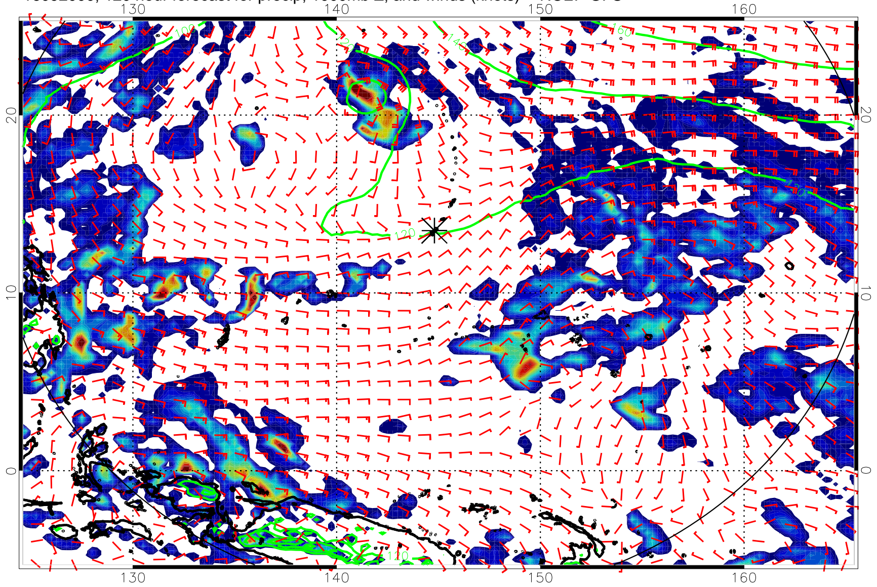
16092000, 120 hour forecast for precip, 1000mb Z, and winds (knots) -- NCEP GFS
