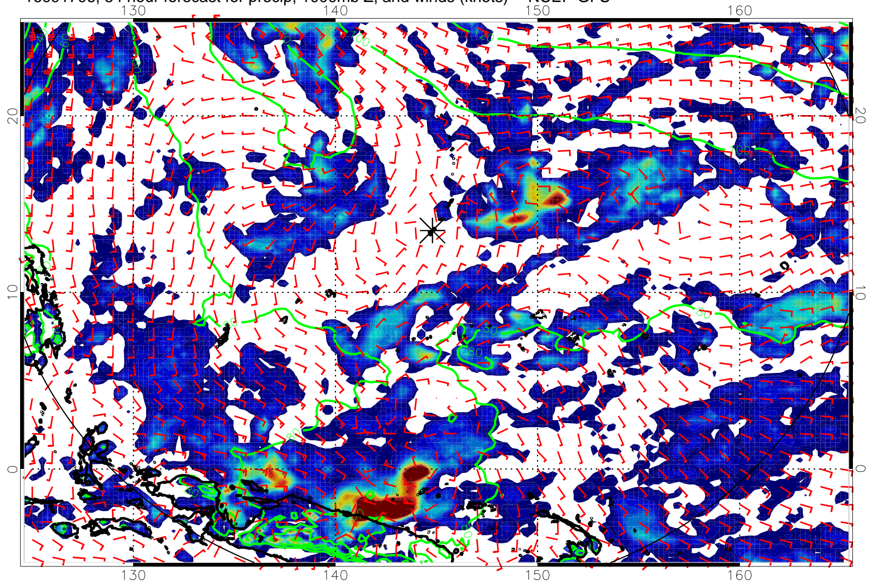
16091706, 54 hour forecast for precip, 1000mb Z, and winds (knots) -- NCEP GFS
