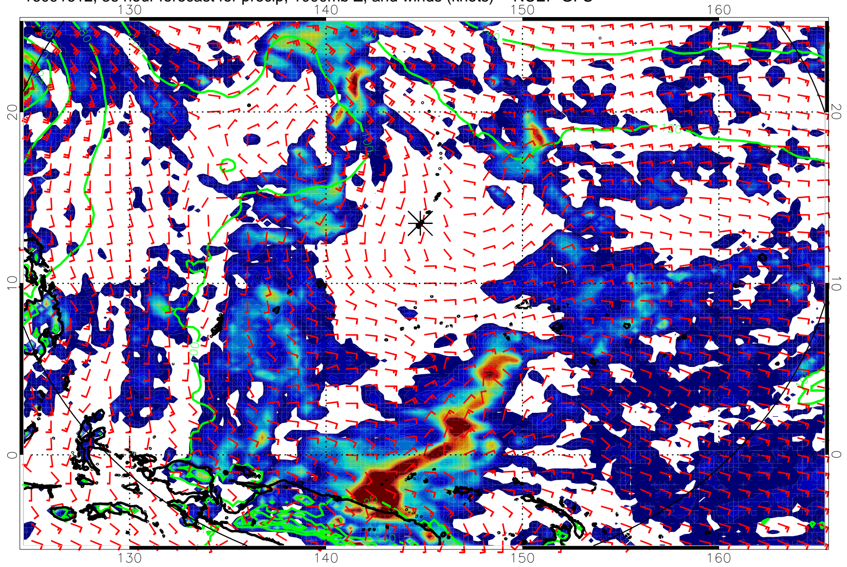
16091612, 36 hour forecast for precip, 1000mb Z, and winds (knots) -- NCEP GFS
