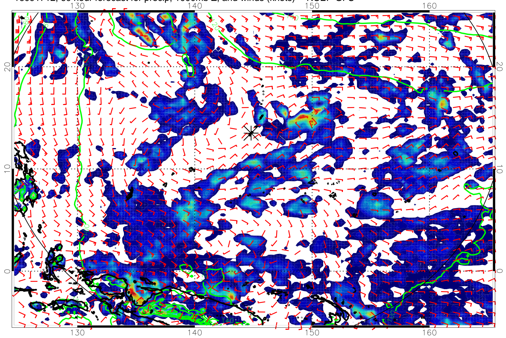
16091712, 60 hour forecast for precip, 1000mb Z, and winds (knots) -- NCEP GFS
