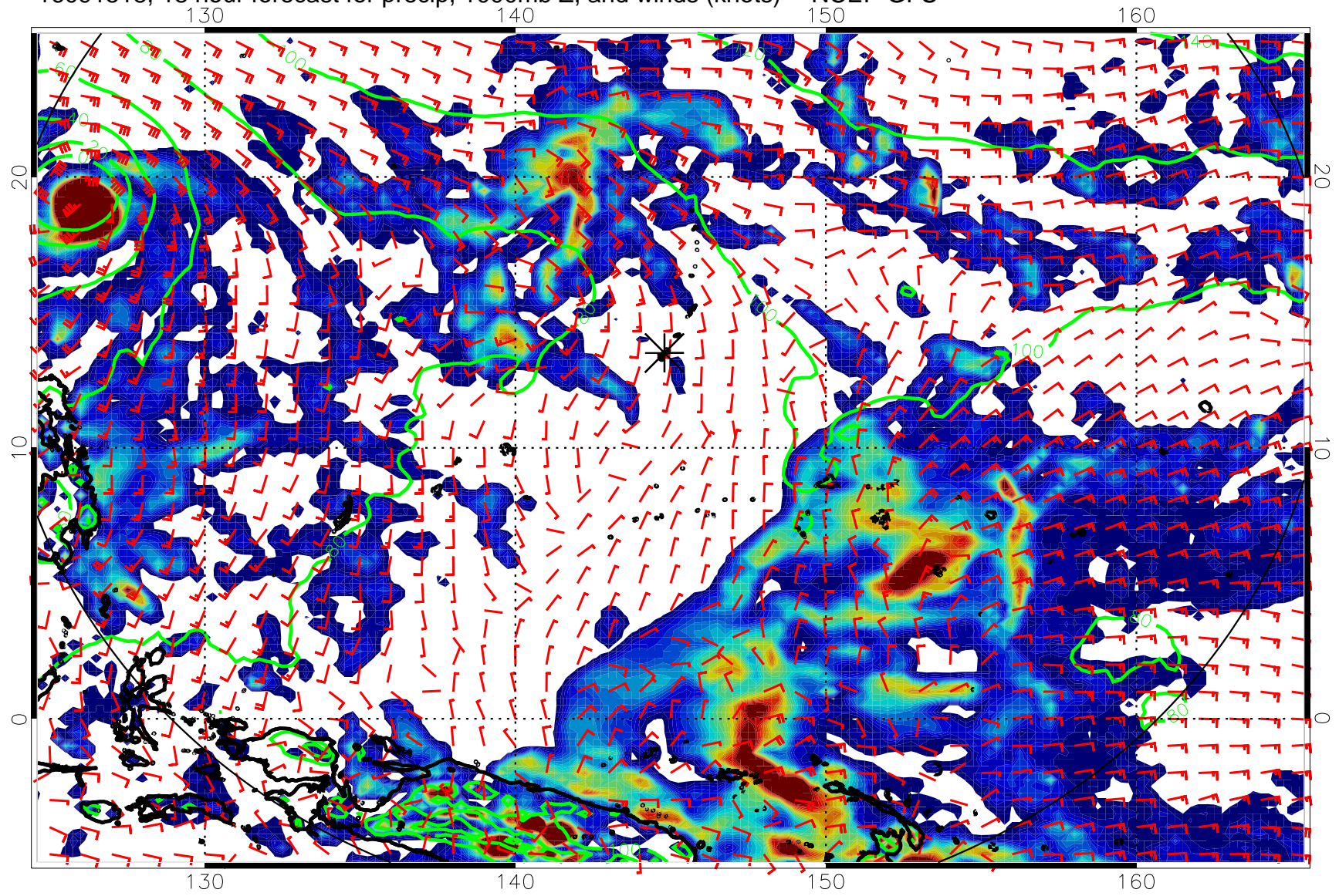
16091518, 18 hour forecast for precip, 1000mb Z, and winds (knots) -- NCEP GFS
