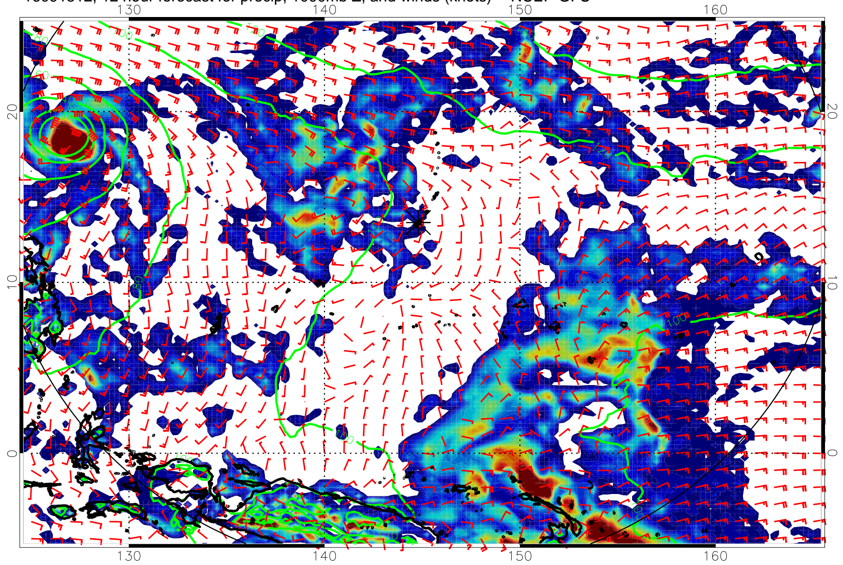
16091512, 12 hour forecast for precip, 1000mb Z, and winds (knots) -- NCEP GFS
