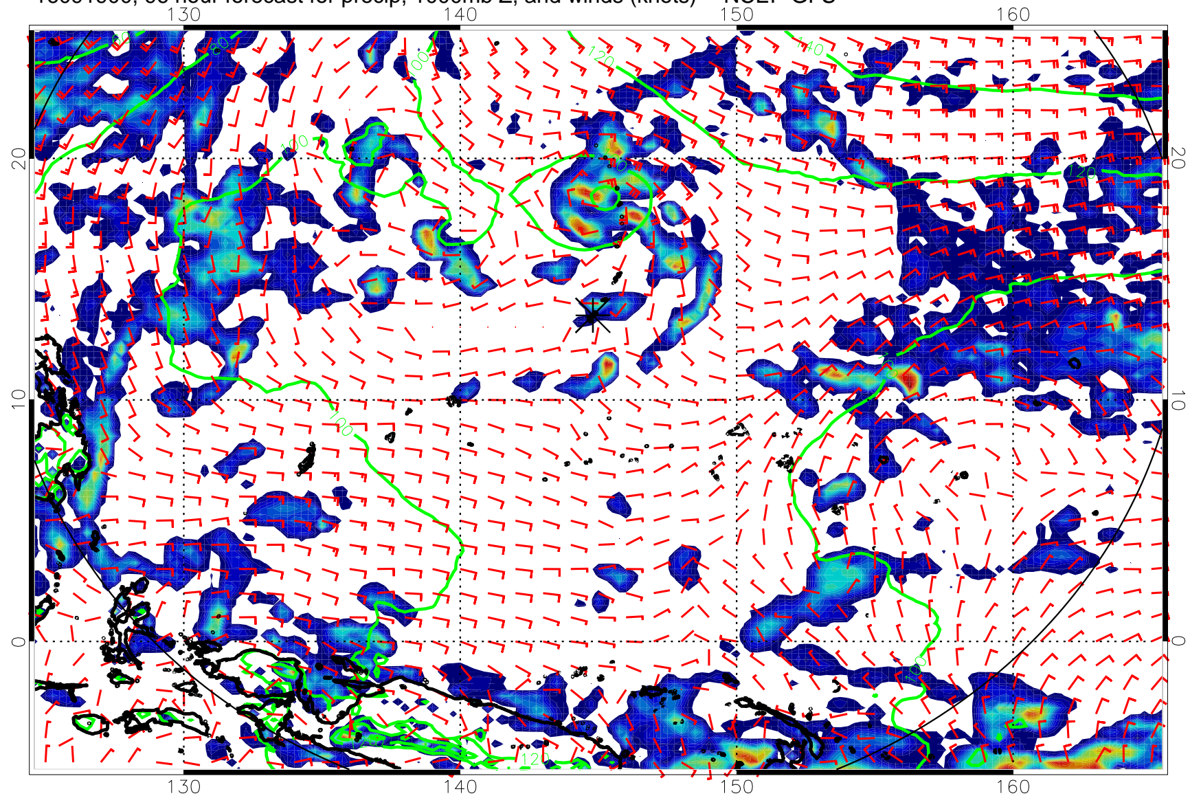
16091900, 96 hour forecast for precip, 1000mb Z, and winds (knots) -- NCEP GFS
