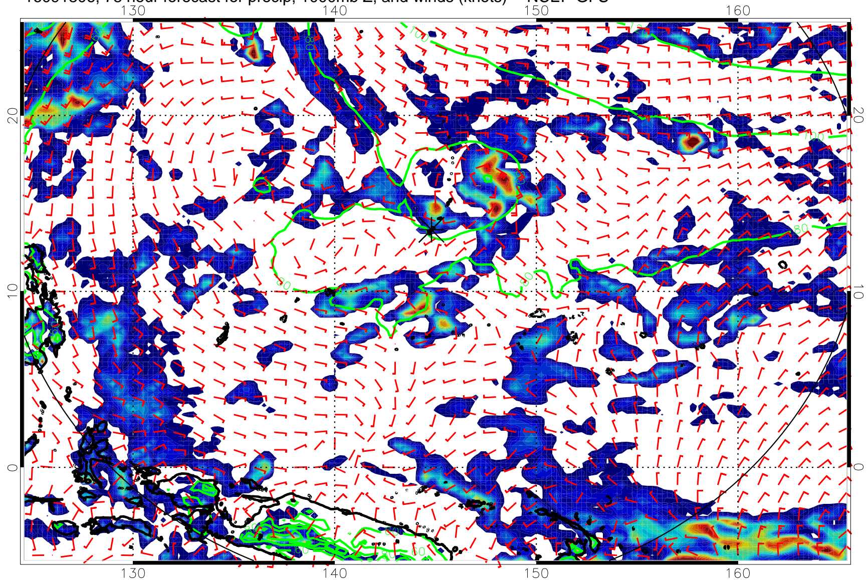
16091806, 78 hour forecast for precip, 1000mb Z, and winds (knots) -- NCEP GFS
