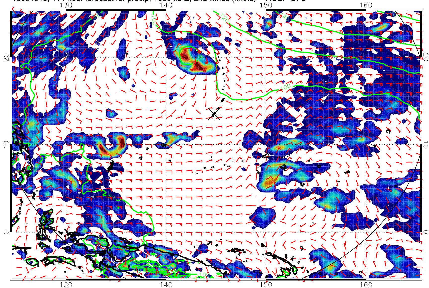
16091918, 114 hour forecast for precip, 1000mb Z, and winds (knots) -- NCEP GFS
