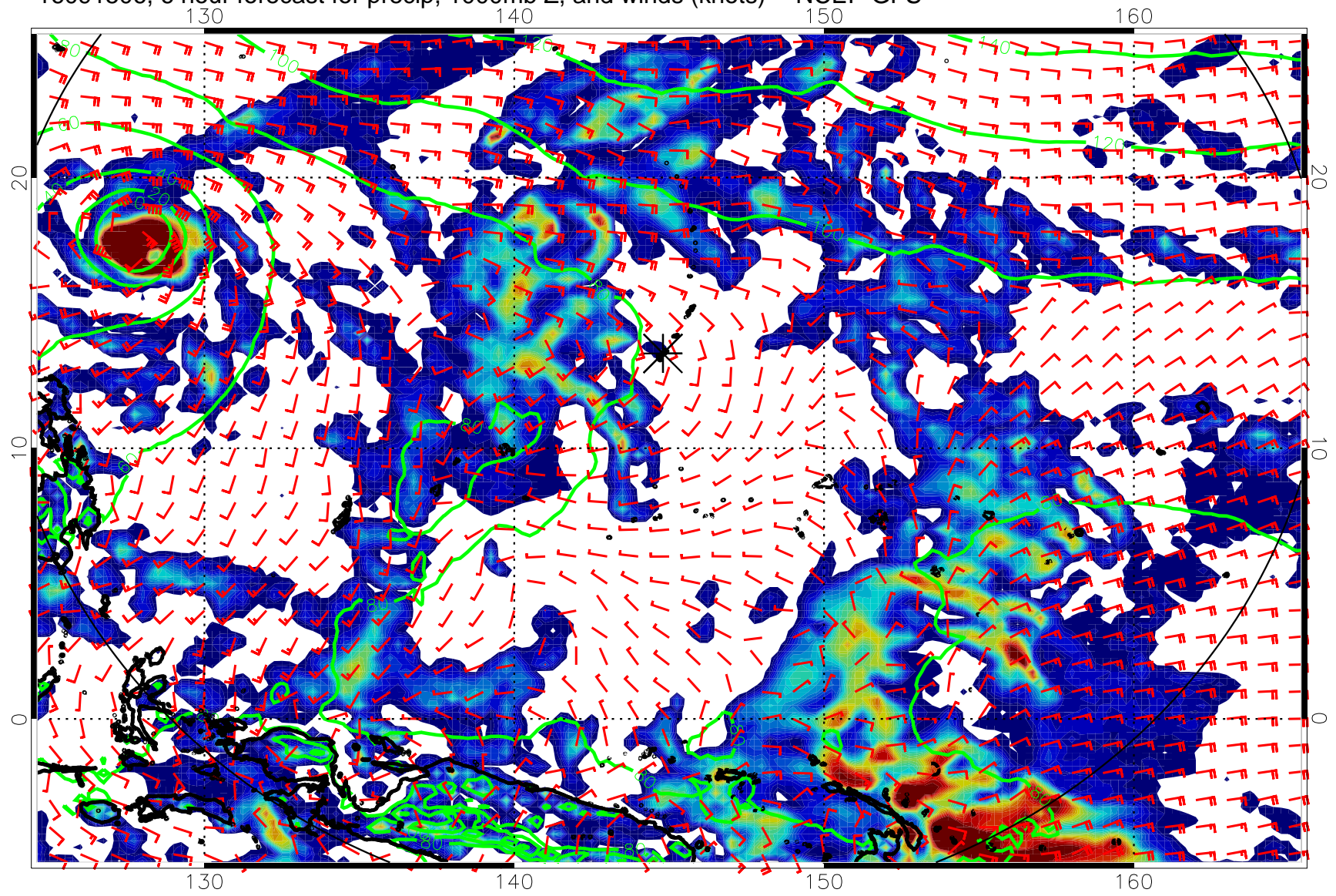
16091506, 6 hour forecast for precip, 1000mb Z, and winds (knots) -- NCEP GFS
