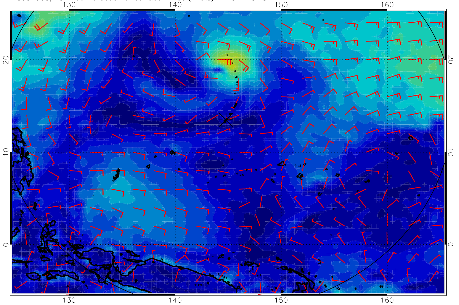
16091906, 102 hour forecast for surface winds (knots) -- NCEP GFS
