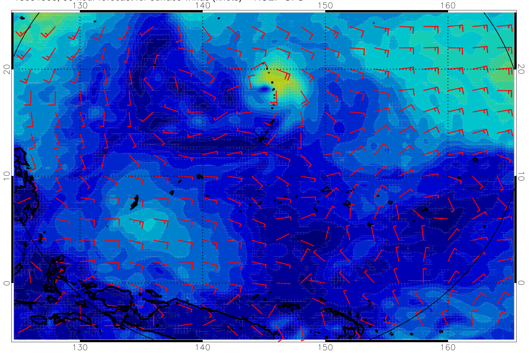
16091900, 96 hour forecast for surface winds (knots) -- NCEP GFS
