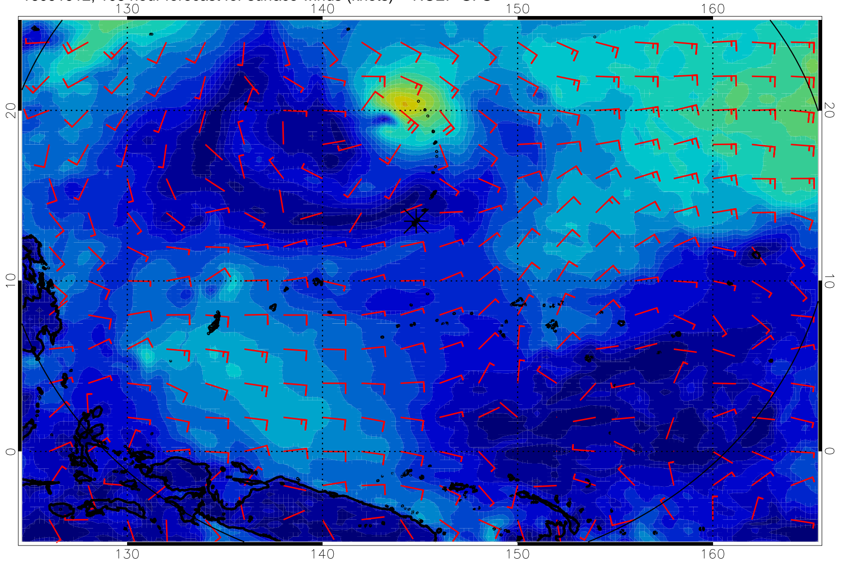
16091912, 108 hour forecast for surface winds (knots) -- NCEP GFS
