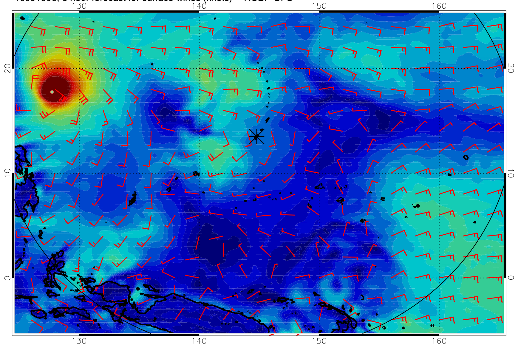
16091506, 6 hour forecast for surface winds (knots) -- NCEP GFS
