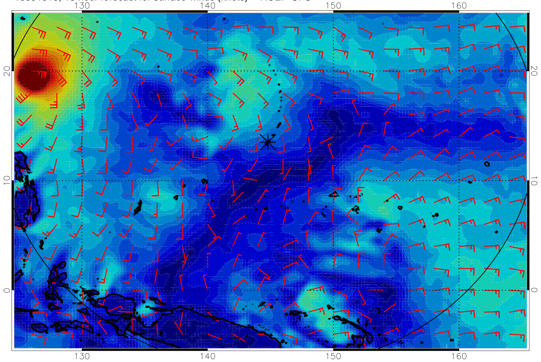
16091518, 18 hour forecast for surface winds (knots) -- NCEP GFS
