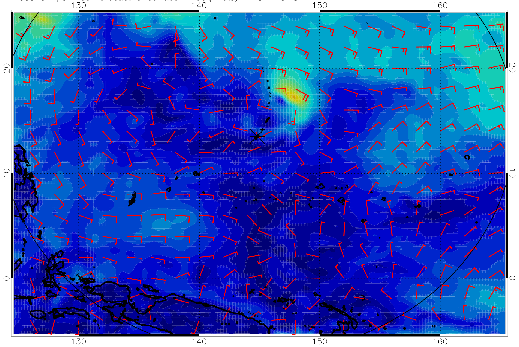
16091812, 84 hour forecast for surface winds (knots) -- NCEP GFS
