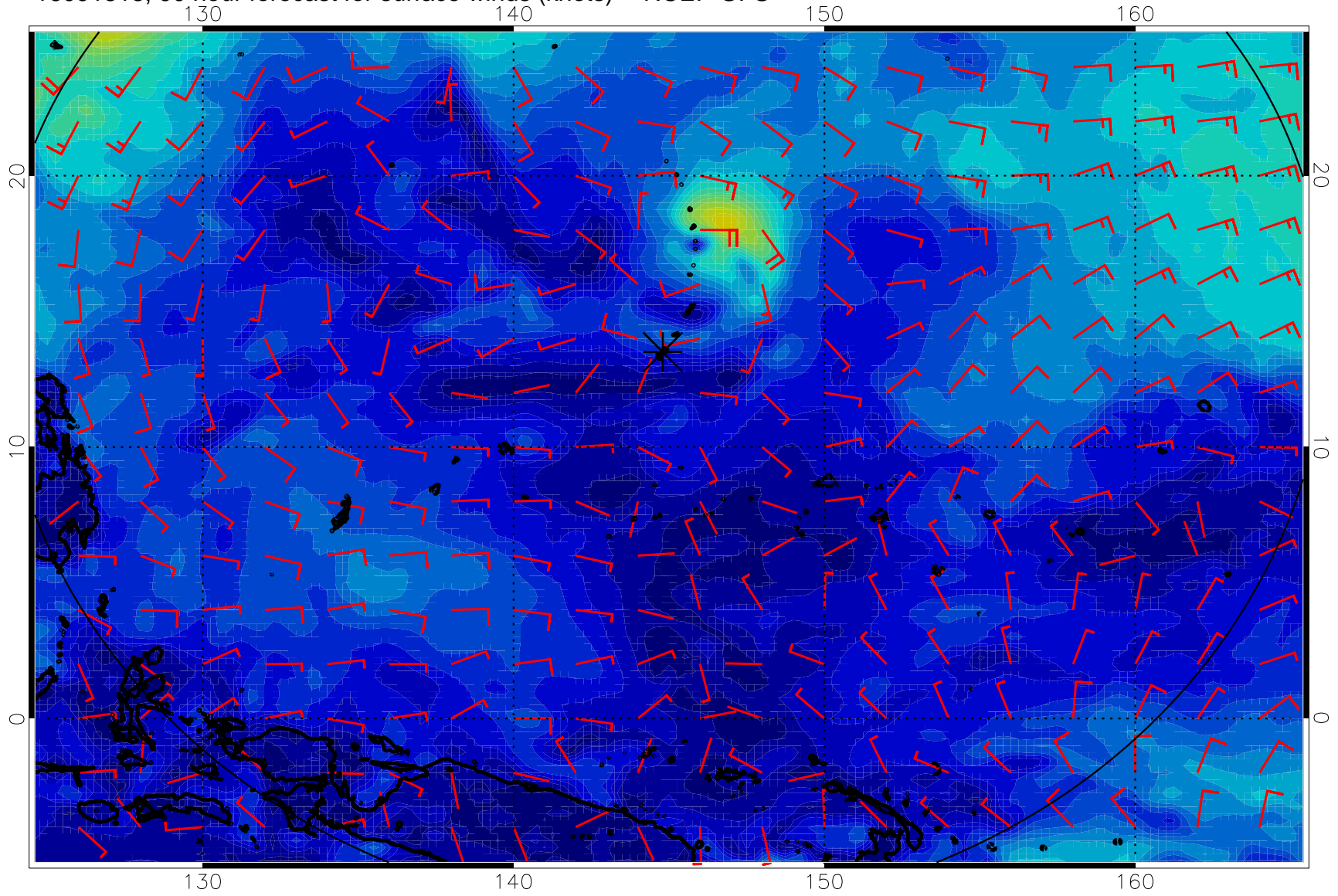
16091818, 90 hour forecast for surface winds (knots) -- NCEP GFS
