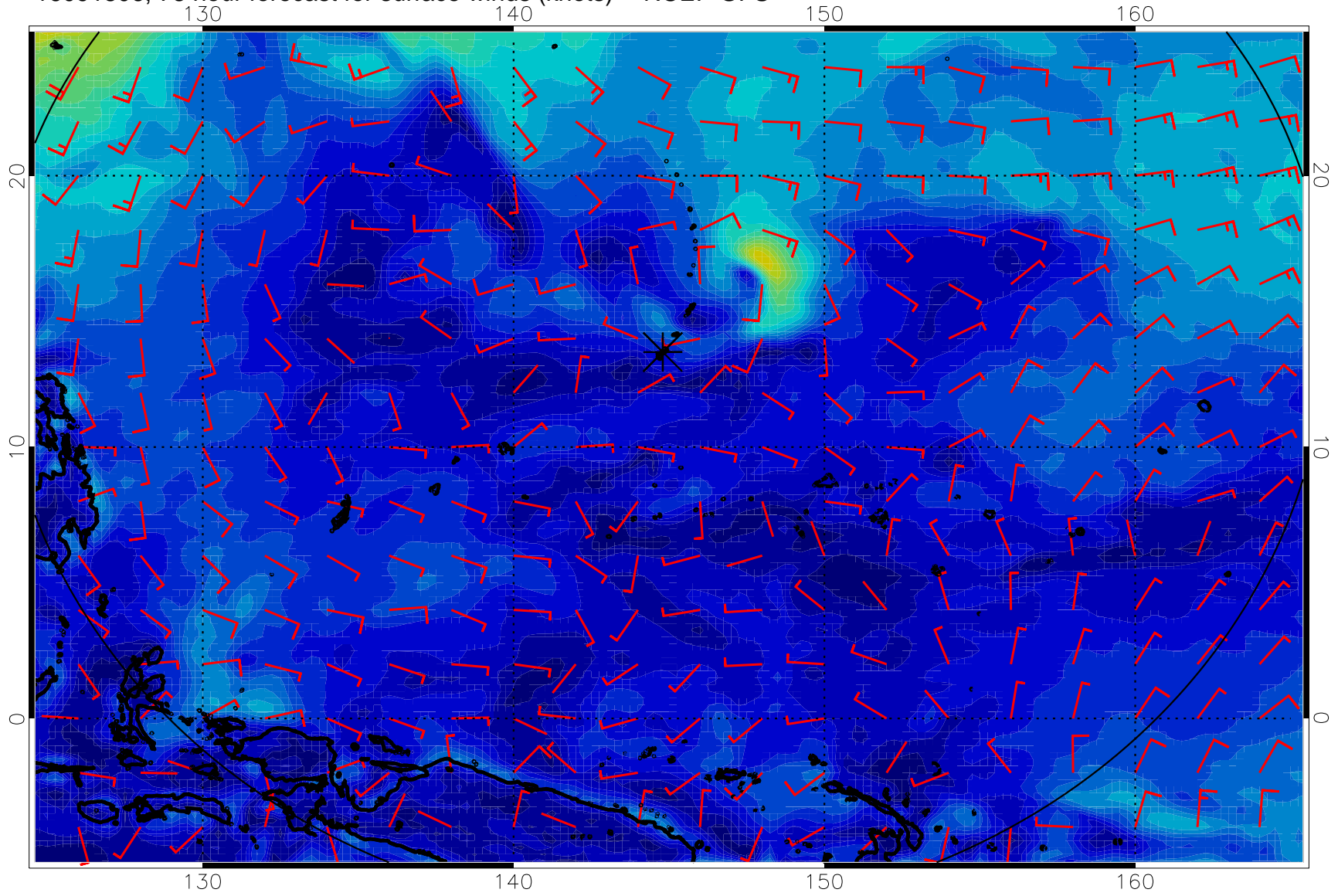
16091806, 78 hour forecast for surface winds (knots) -- NCEP GFS
