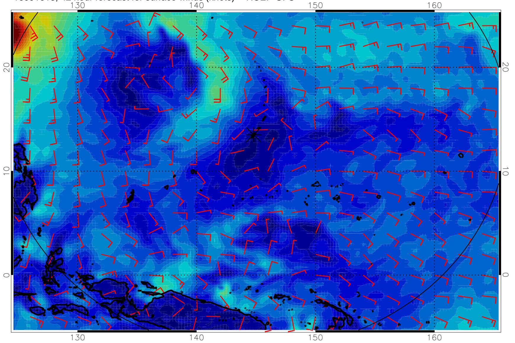
16091618, 42 hour forecast for surface winds (knots) -- NCEP GFS
