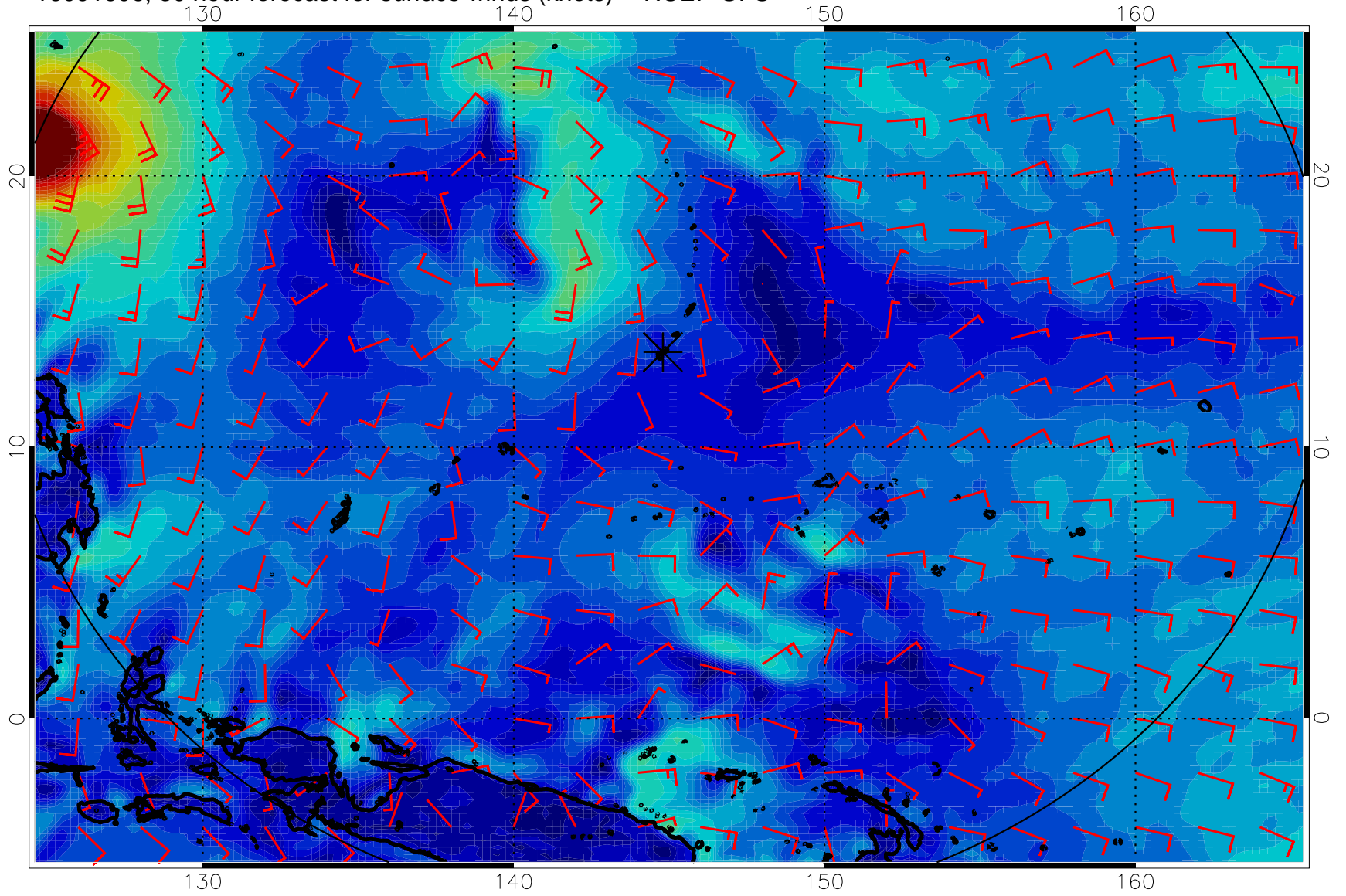
16091606, 30 hour forecast for surface winds (knots) -- NCEP GFS
