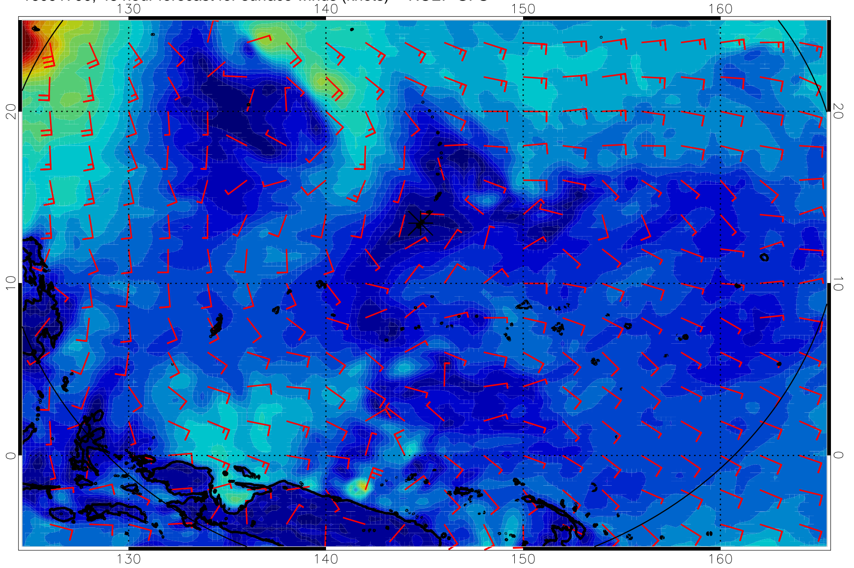
16091700, 48 hour forecast for surface winds (knots) -- NCEP GFS
