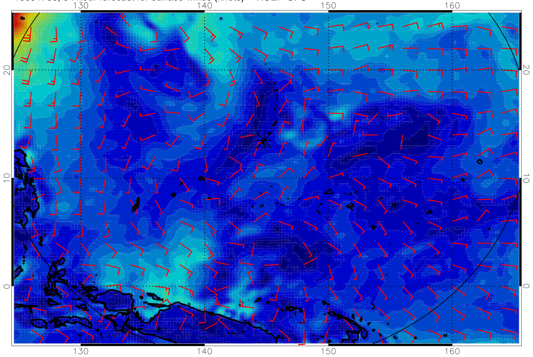
16091706, 54 hour forecast for surface winds (knots) -- NCEP GFS
