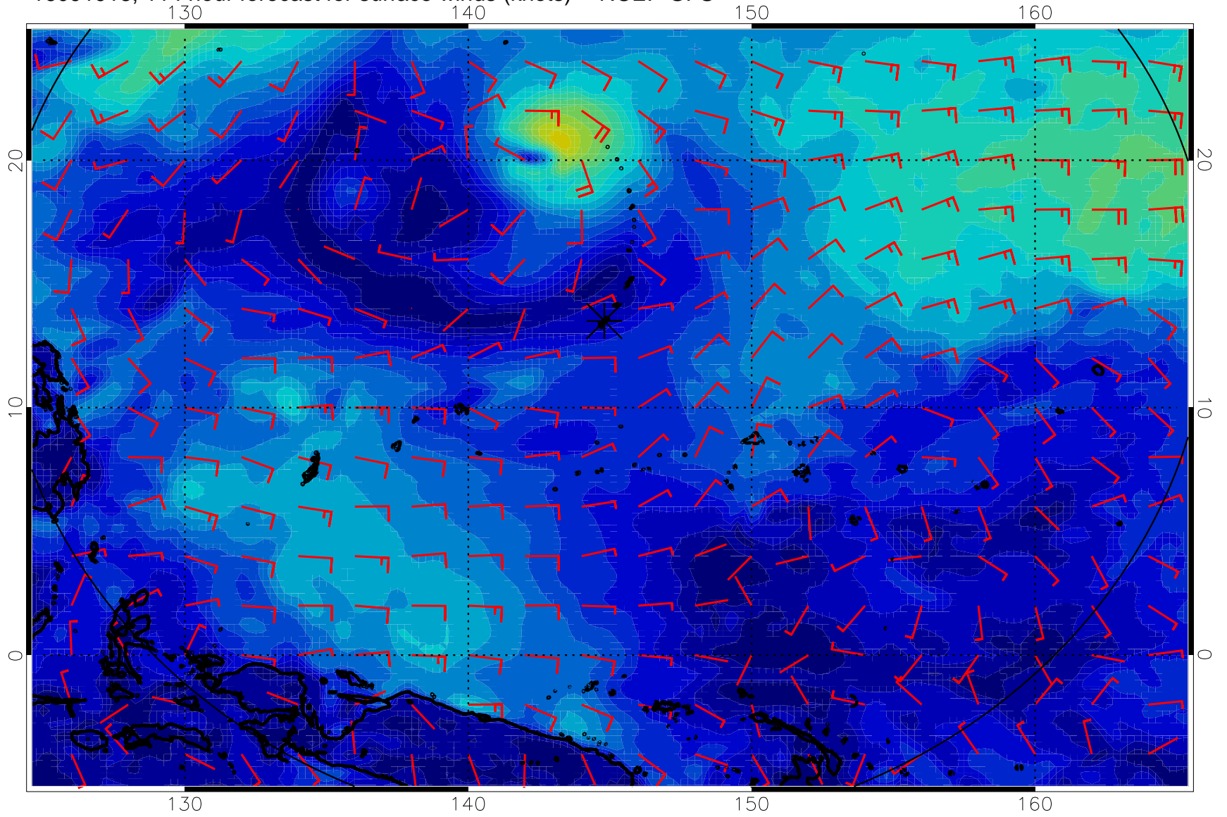
16091918, 114 hour forecast for surface winds (knots) -- NCEP GFS
