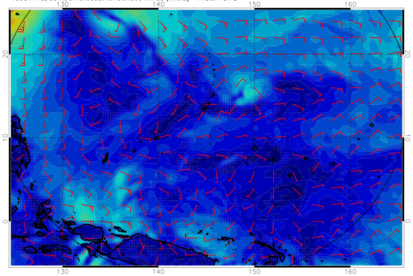
16091718, 66 hour forecast for surface winds (knots) -- NCEP GFS
