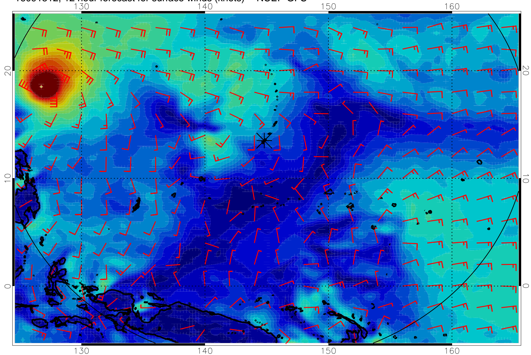
16091512, 12 hour forecast for surface winds (knots) -- NCEP GFS
