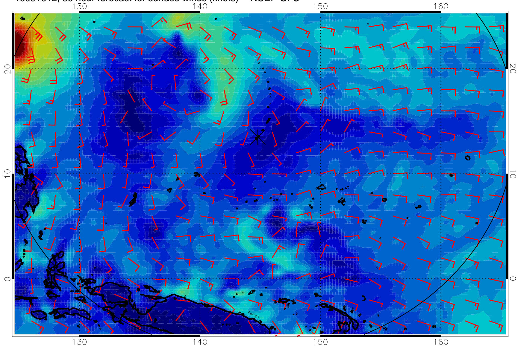
16091612, 36 hour forecast for surface winds (knots) -- NCEP GFS
