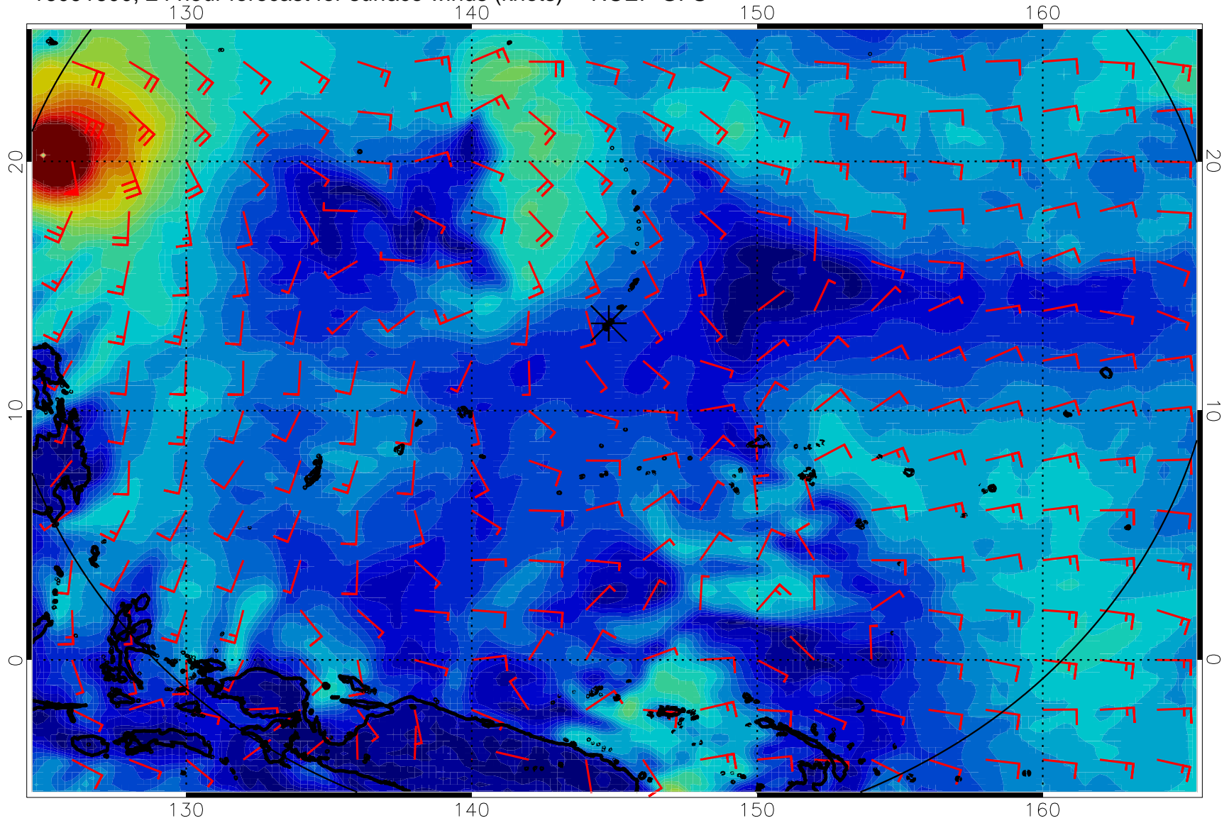
16091600, 24 hour forecast for surface winds (knots) -- NCEP GFS
