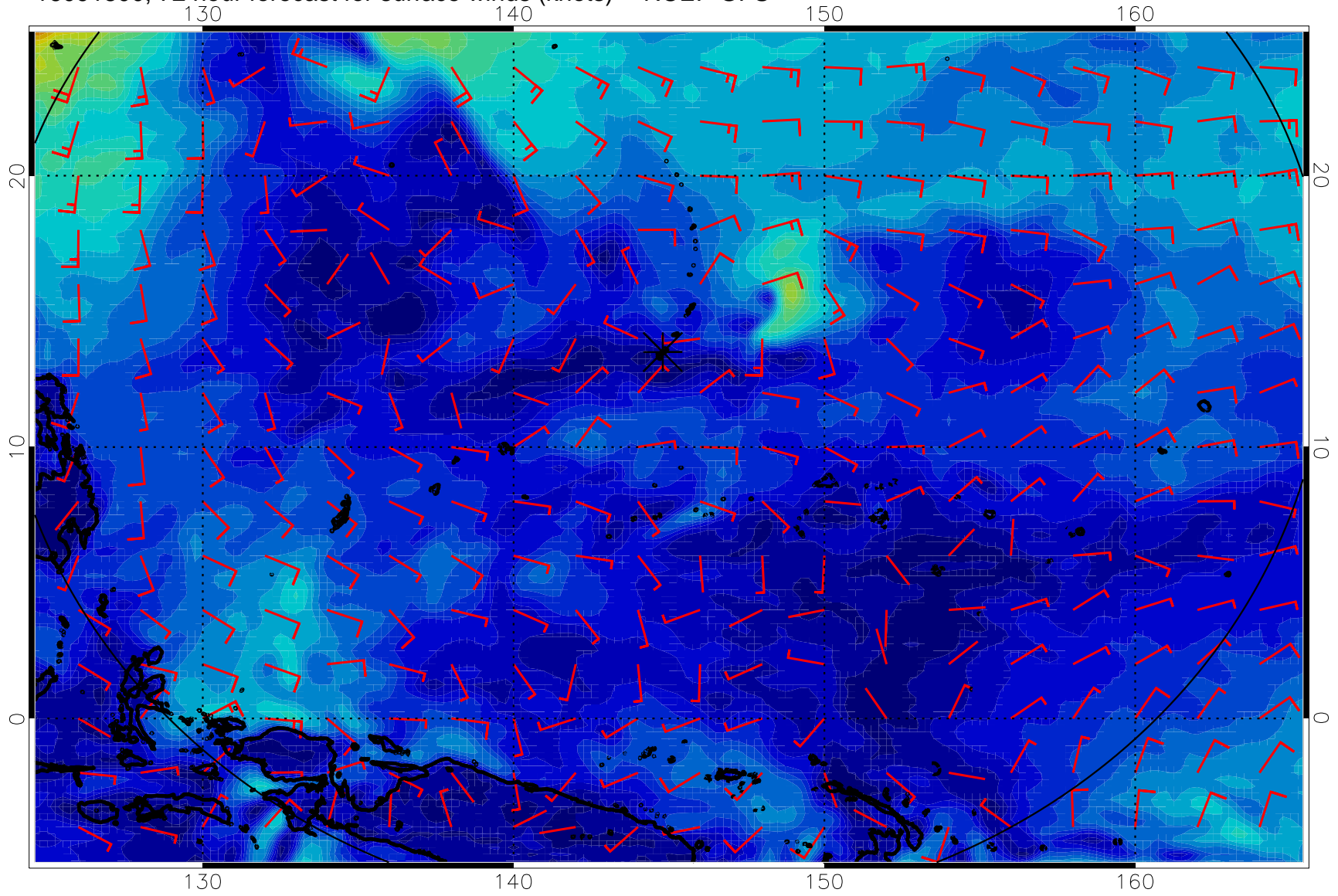
16091800, 72 hour forecast for surface winds (knots) -- NCEP GFS
