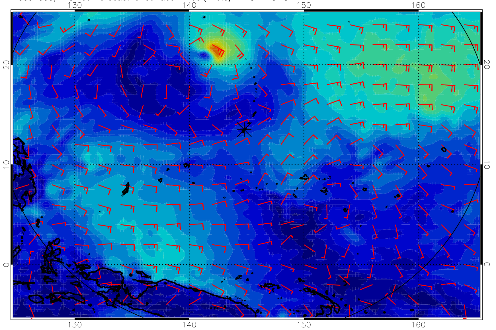
16092000, 120 hour forecast for surface winds (knots) -- NCEP GFS
