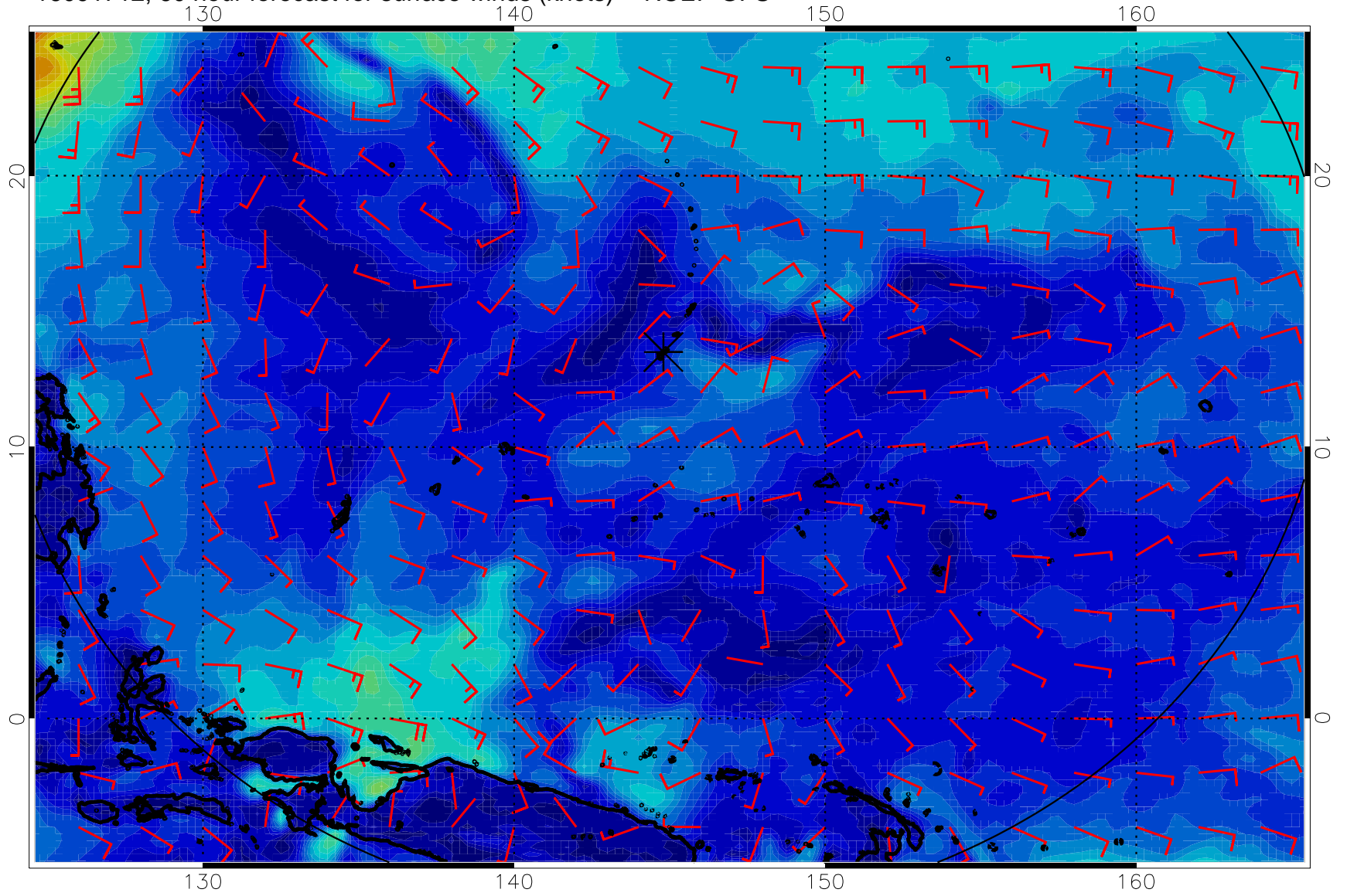
16091712, 60 hour forecast for surface winds (knots) -- NCEP GFS
