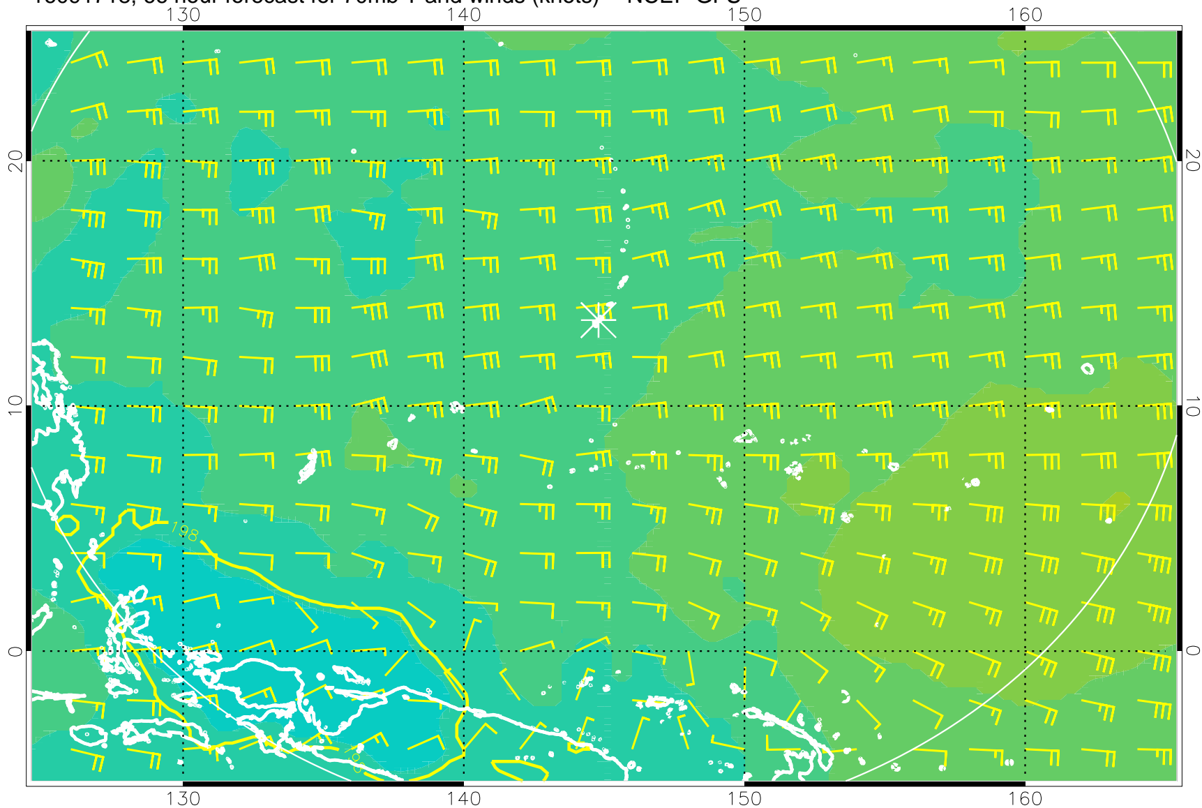
16091718, 66 hour forecast for 70mb T and winds (knots) -- NCEP GFS
