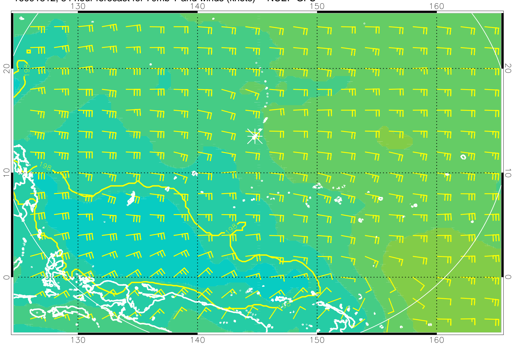
16091812, 84 hour forecast for 70mb T and winds (knots) -- NCEP GFS
