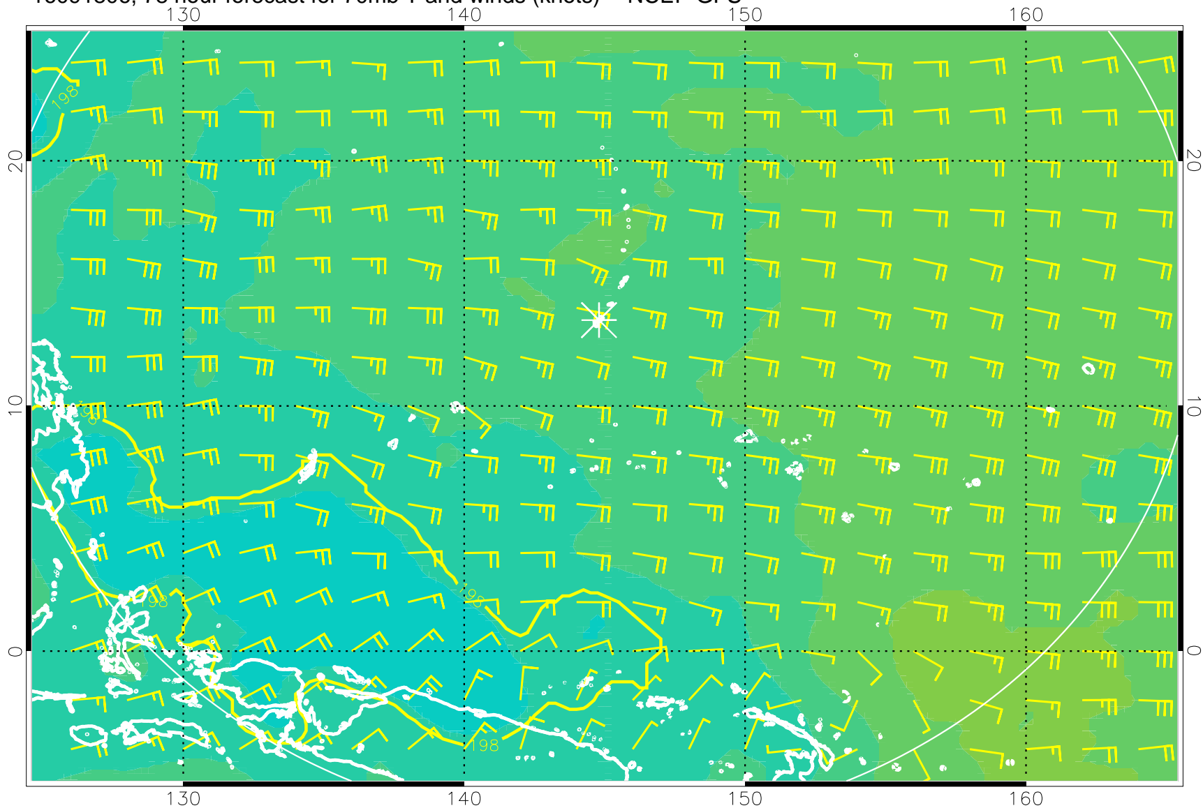
16091806, 78 hour forecast for 70mb T and winds (knots) -- NCEP GFS
