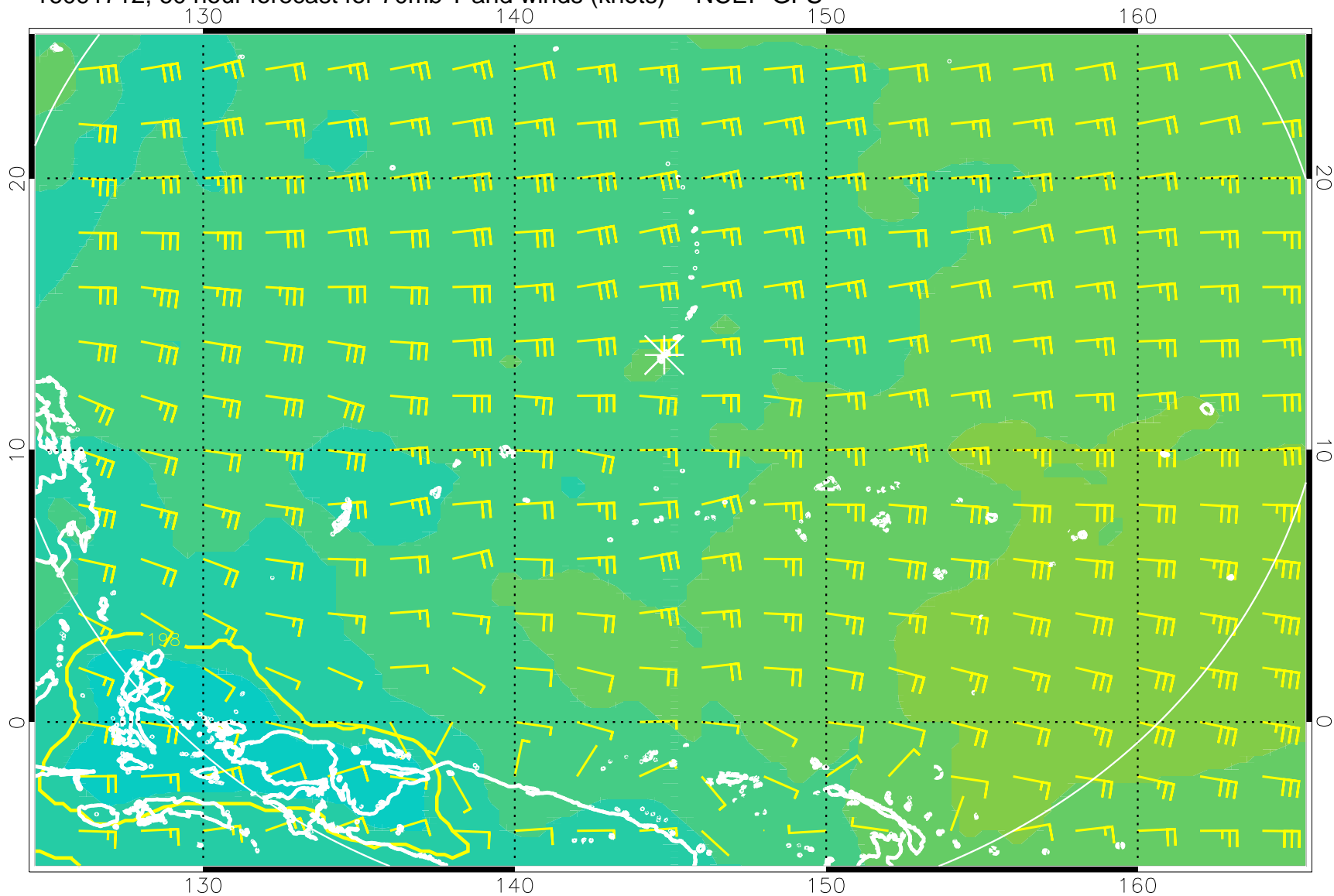
16091712, 60 hour forecast for 70mb T and winds (knots) -- NCEP GFS
