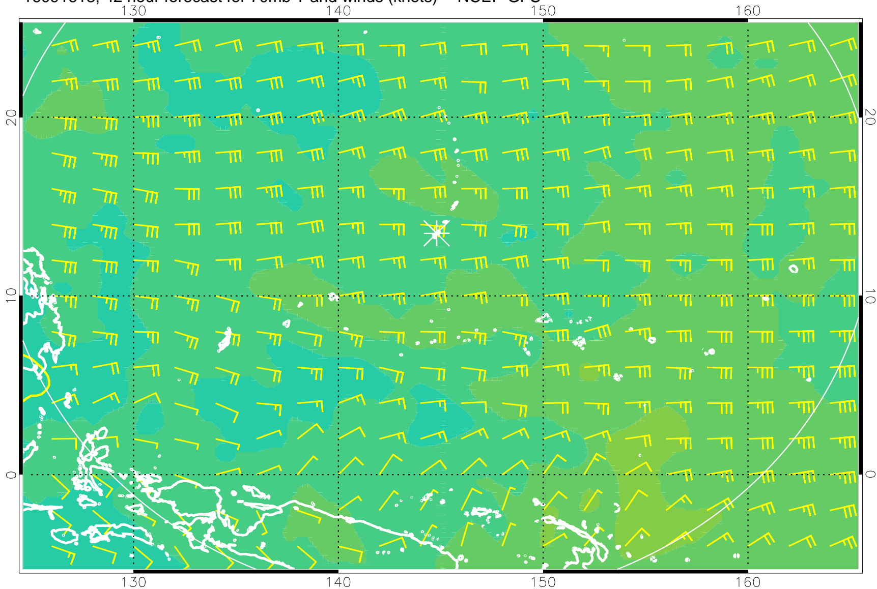
16091618, 42 hour forecast for 70mb T and winds (knots) -- NCEP GFS
