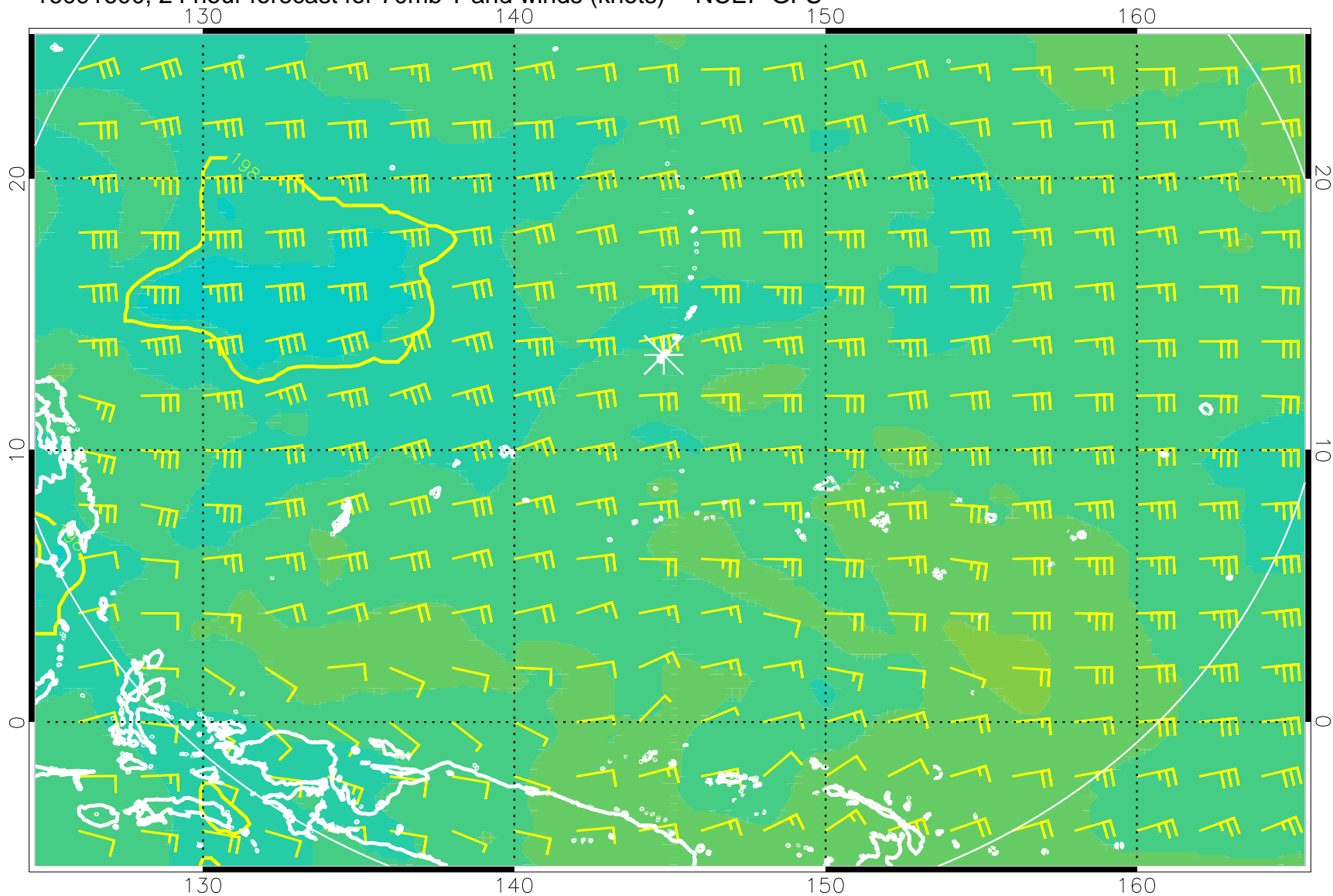
16091600, 24 hour forecast for 70mb T and winds (knots) -- NCEP GFS
