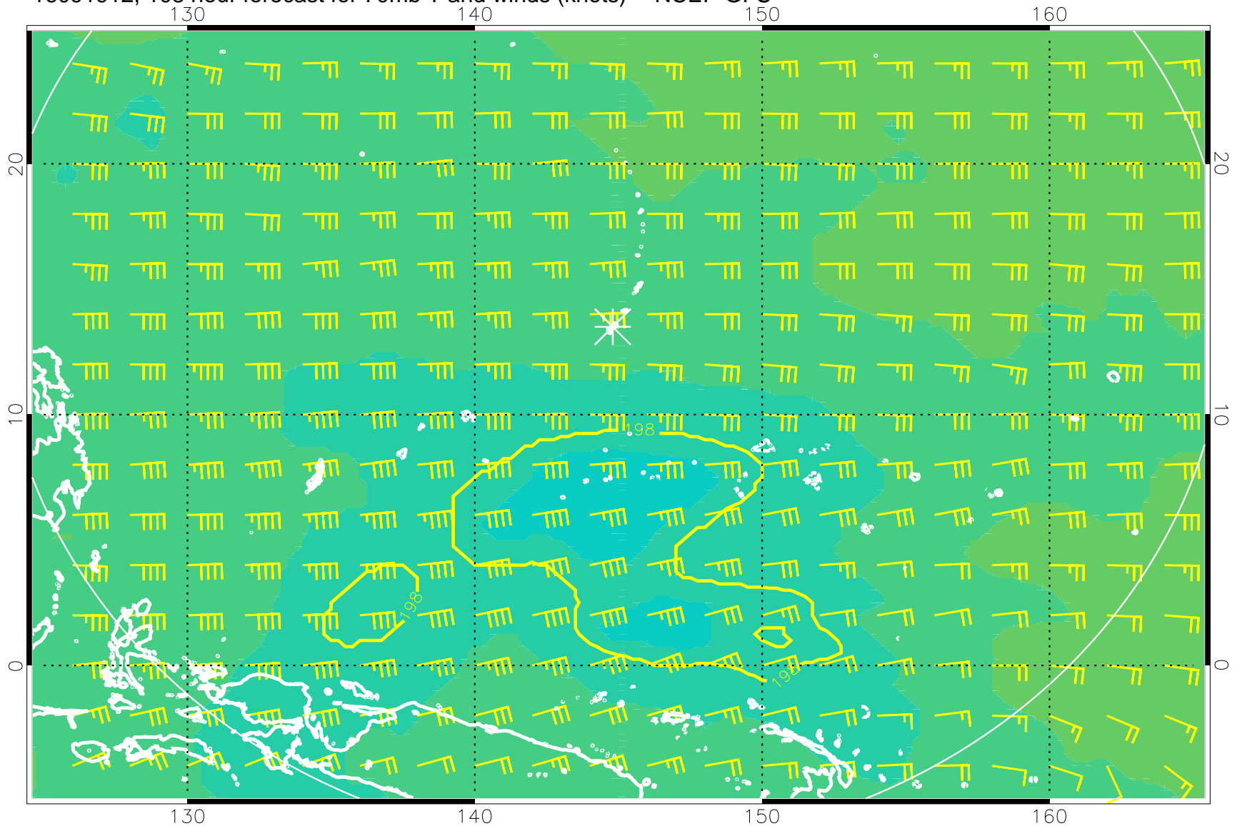
16091912, 108 hour forecast for 70mb T and winds (knots) -- NCEP GFS
