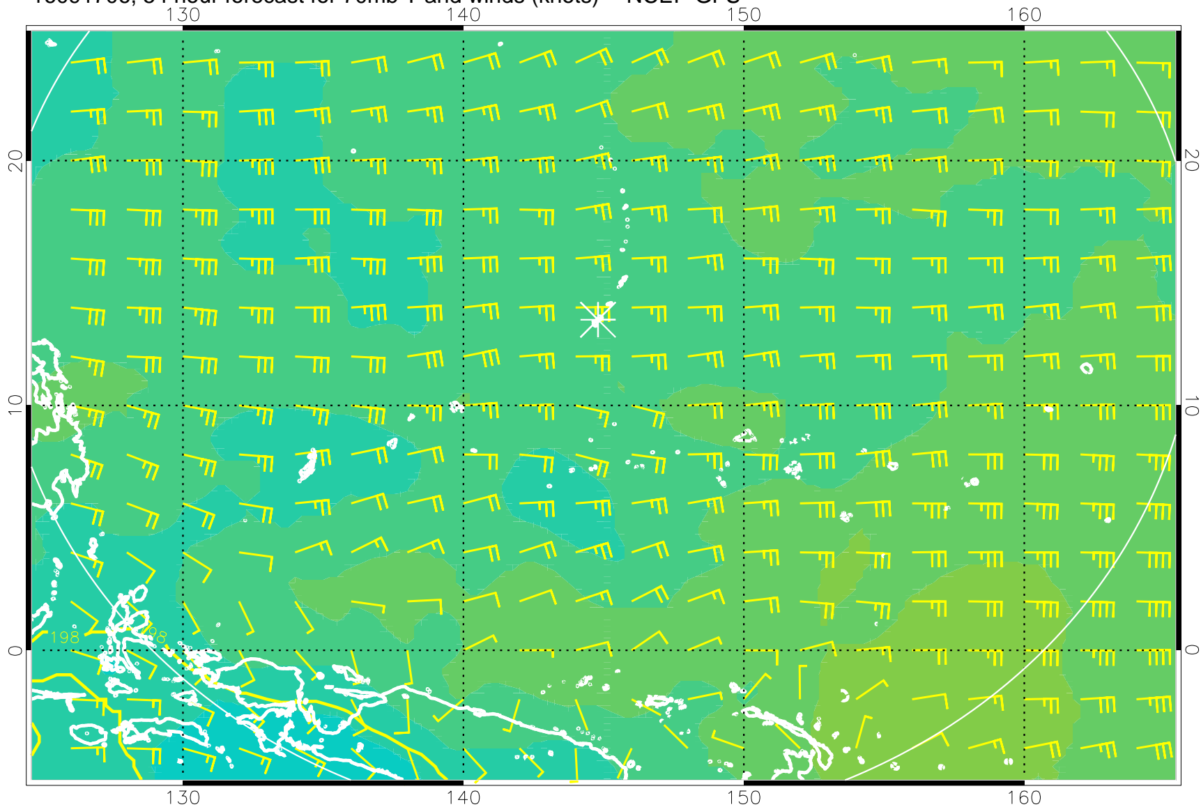
16091706, 54 hour forecast for 70mb T and winds (knots) -- NCEP GFS
