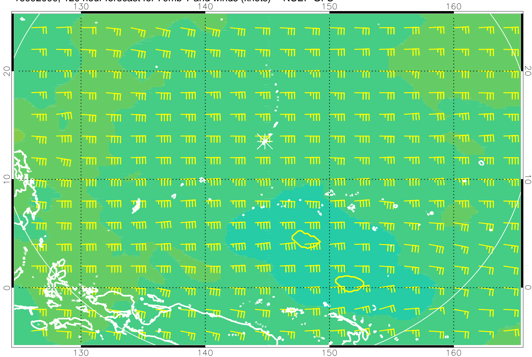
16092000, 120 hour forecast for 70mb T and winds (knots) -- NCEP GFS
