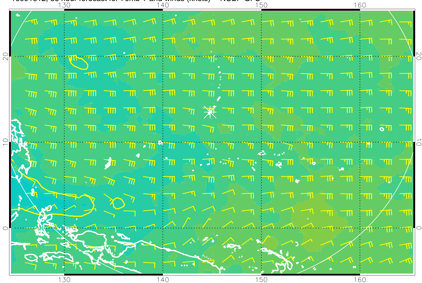
16091612, 36 hour forecast for 70mb T and winds (knots) -- NCEP GFS
