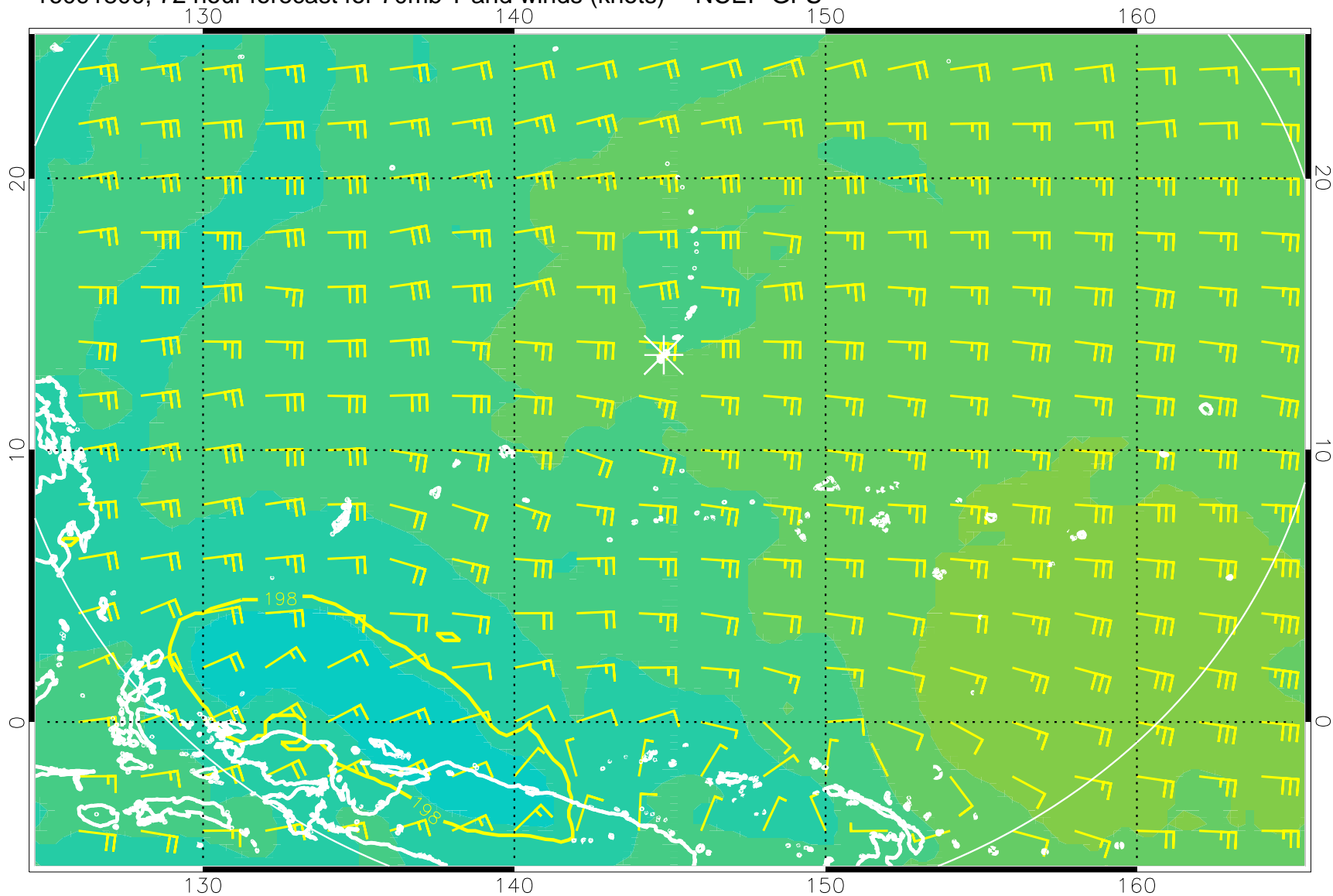
16091800, 72 hour forecast for 70mb T and winds (knots) -- NCEP GFS
