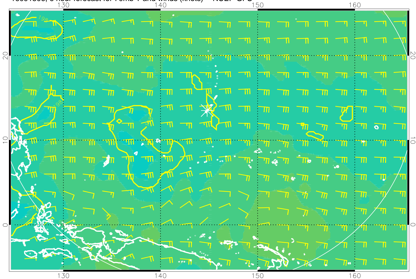
16091506, 6 hour forecast for 70mb T and winds (knots) -- NCEP GFS
