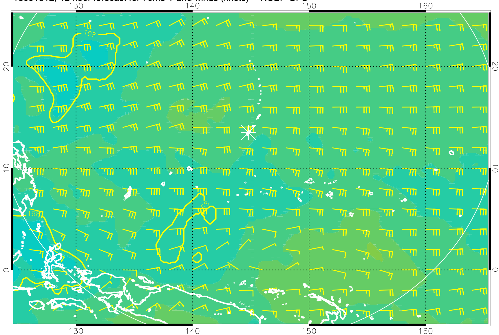
16091512, 12 hour forecast for 70mb T and winds (knots) -- NCEP GFS
