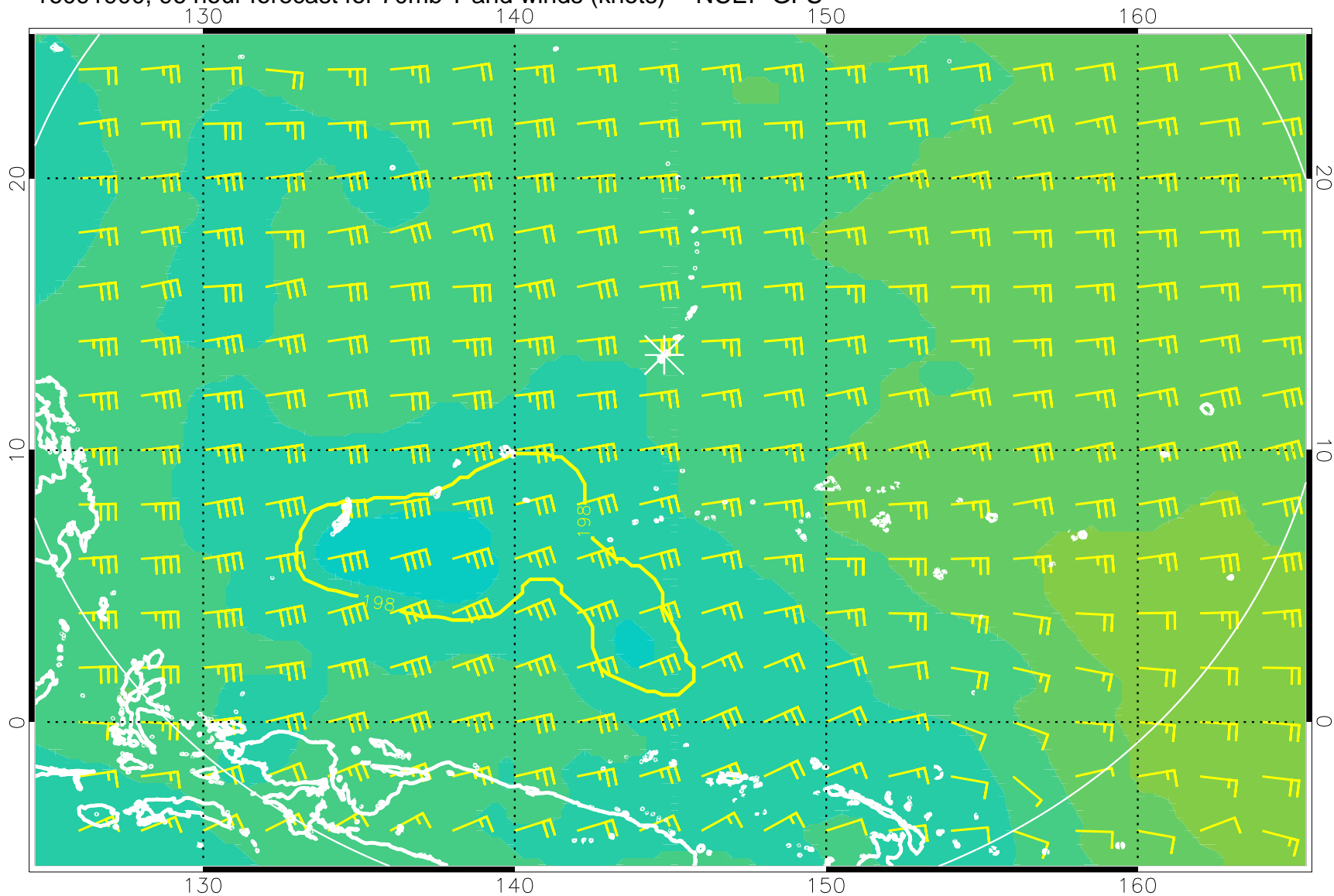
16091900, 96 hour forecast for 70mb T and winds (knots) -- NCEP GFS
