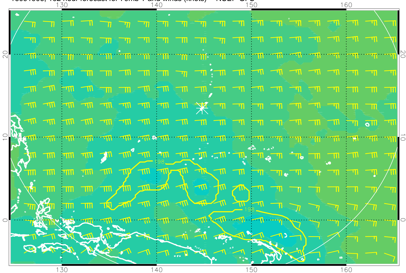
16091906, 102 hour forecast for 70mb T and winds (knots) -- NCEP GFS
