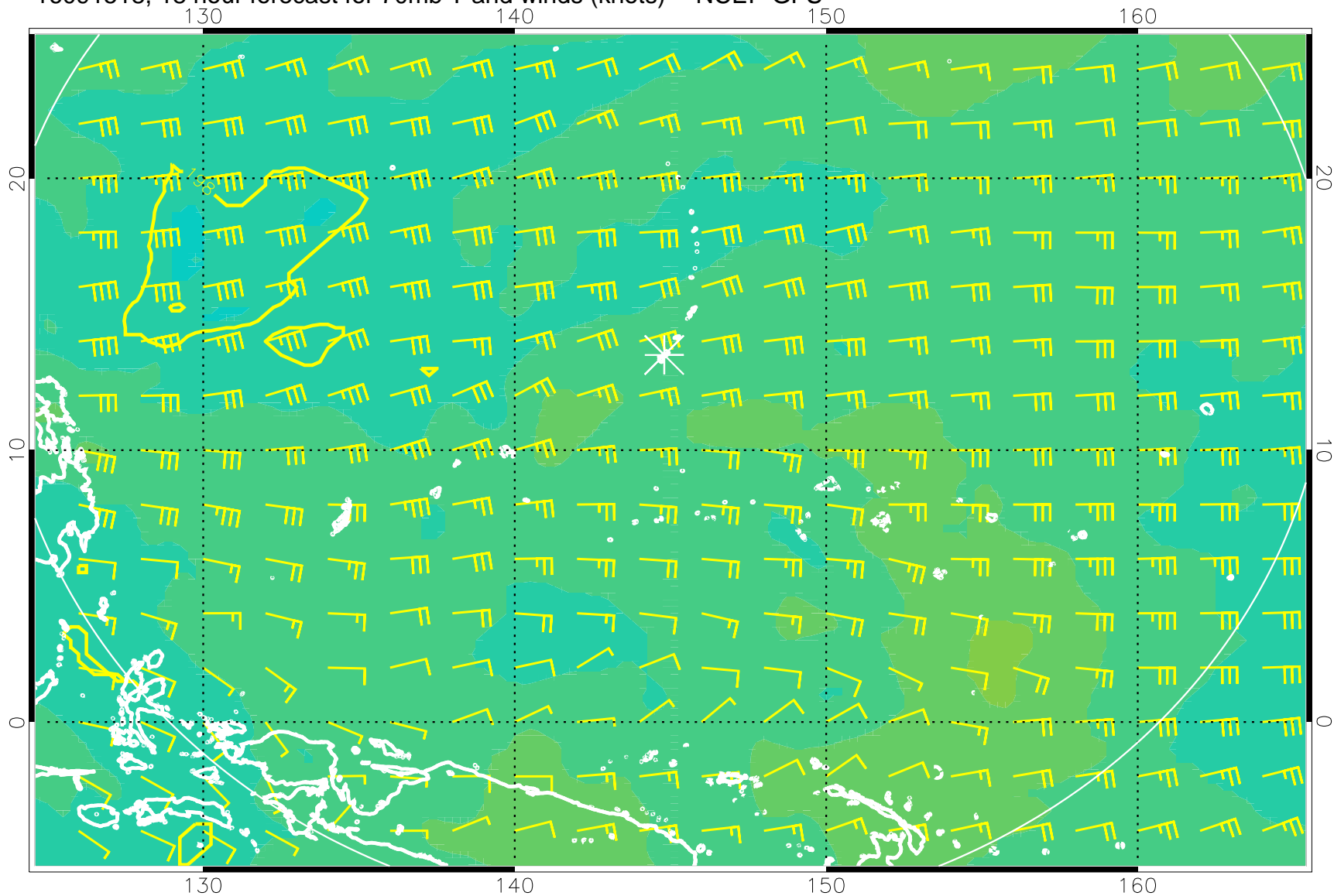
16091518, 18 hour forecast for 70mb T and winds (knots) -- NCEP GFS
