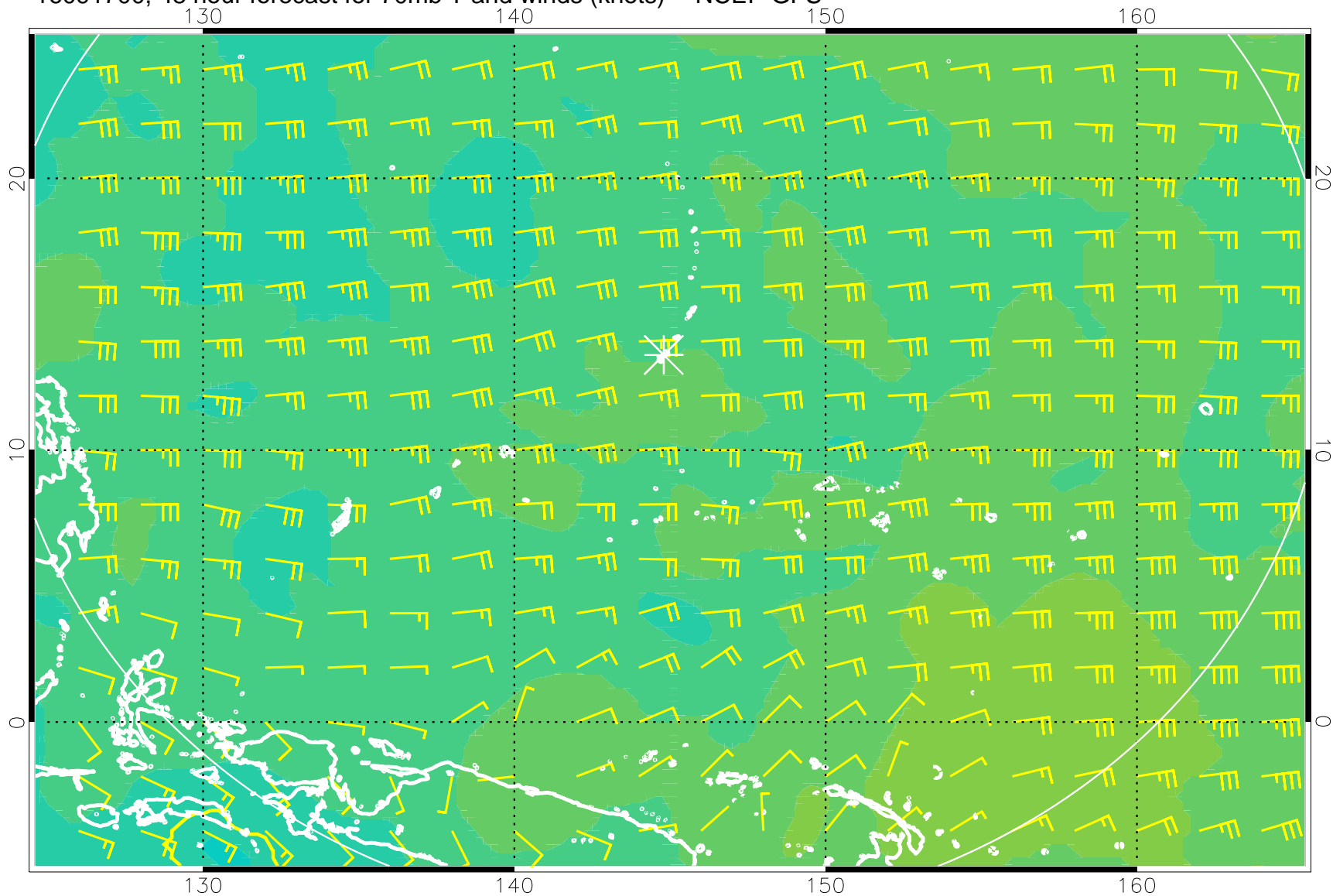
16091700, 48 hour forecast for 70mb T and winds (knots) -- NCEP GFS
