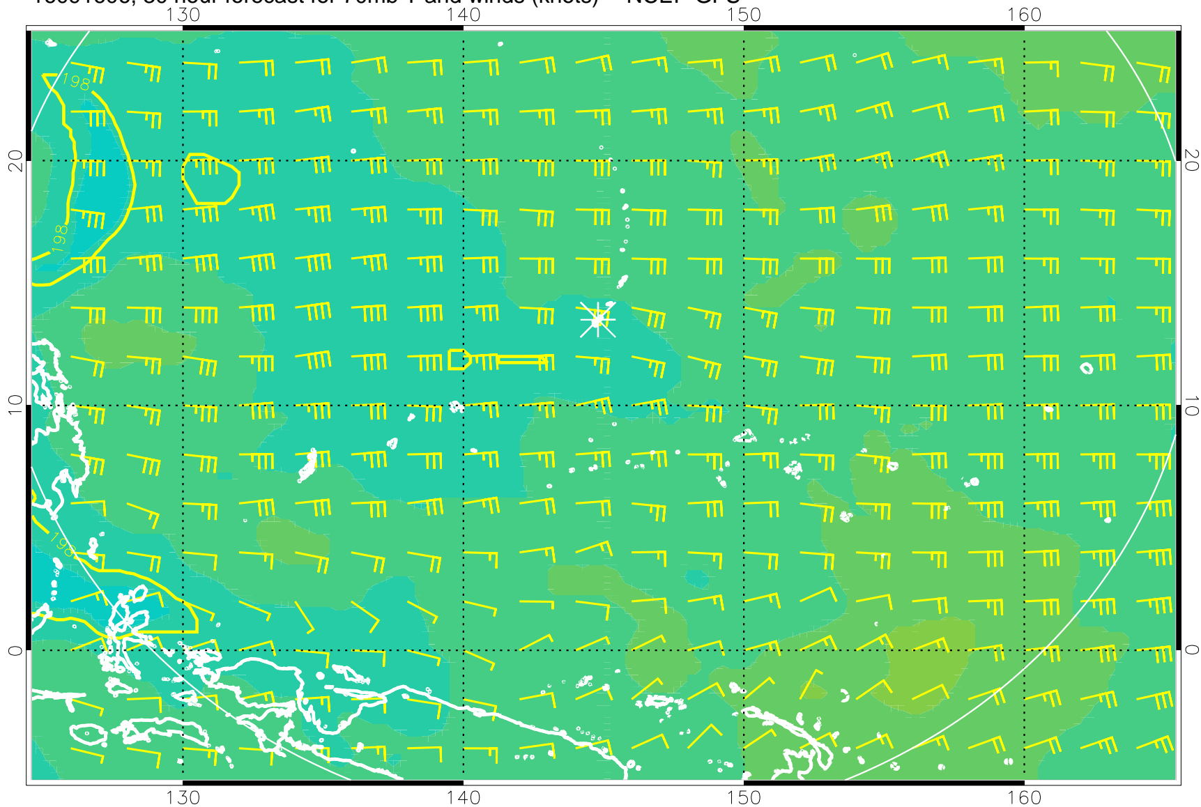
16091606, 30 hour forecast for 70mb T and winds (knots) -- NCEP GFS
