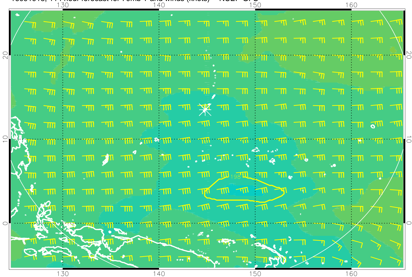
16091918, 114 hour forecast for 70mb T and winds (knots) -- NCEP GFS
