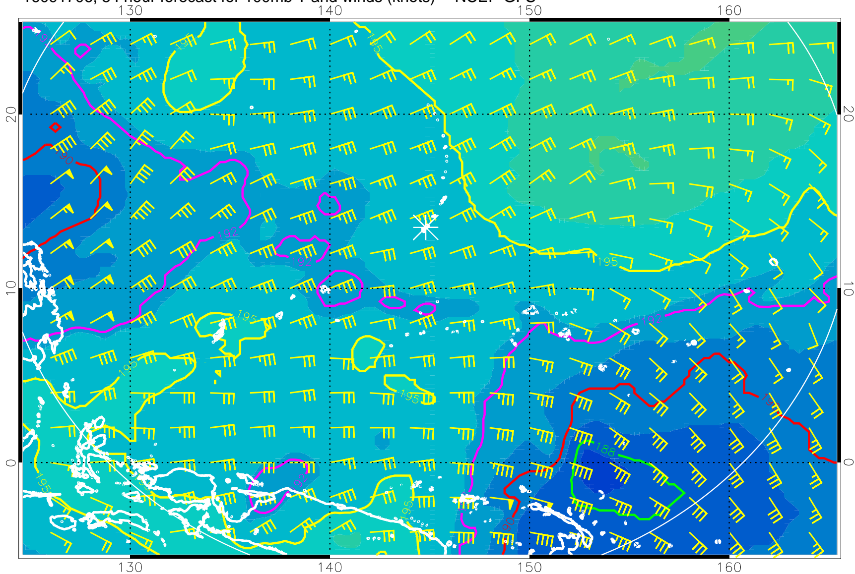
16091706, 54 hour forecast for 100mb T and winds (knots) -- NCEP GFS
