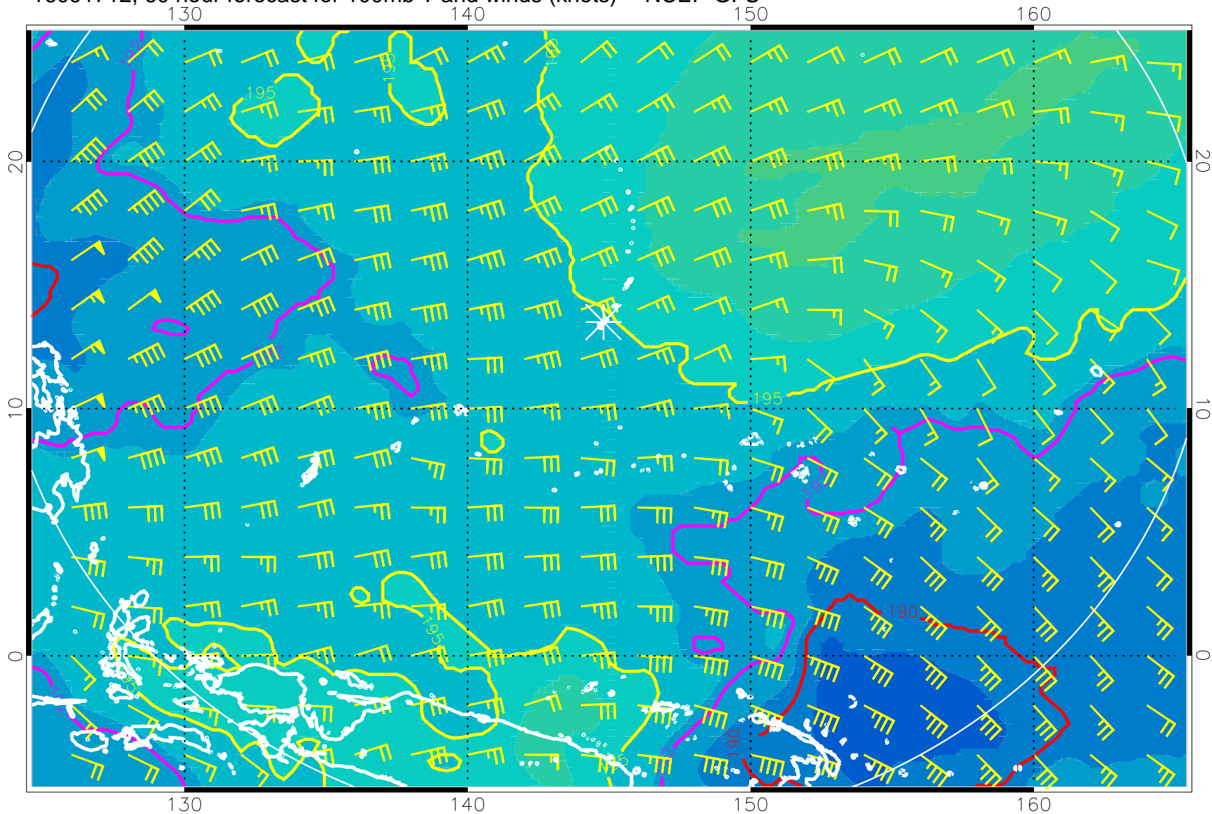
16091712, 60 hour forecast for 100mb T and winds (knots) -- NCEP GFS
