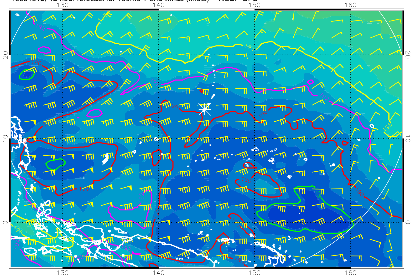
16091512, 12 hour forecast for 100mb T and winds (knots) -- NCEP GFS
