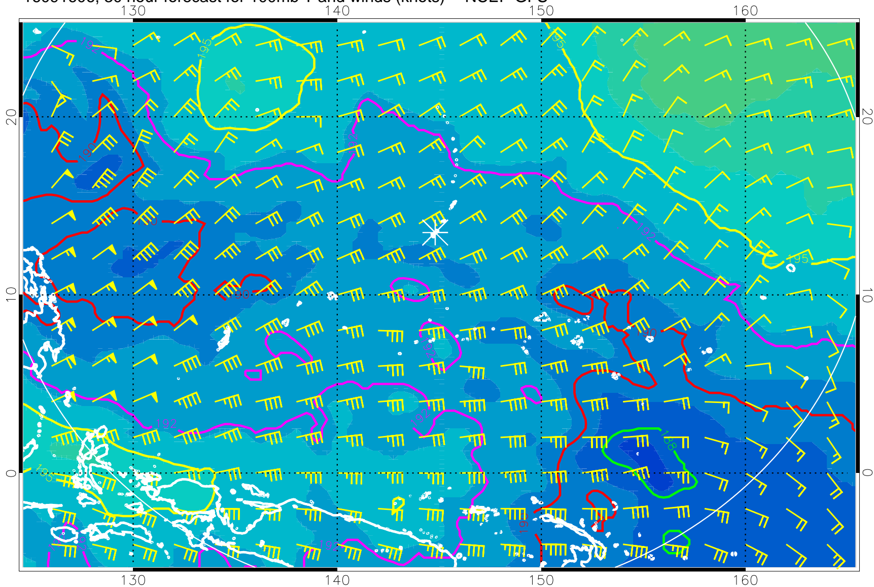
16091606, 30 hour forecast for 100mb T and winds (knots) -- NCEP GFS
