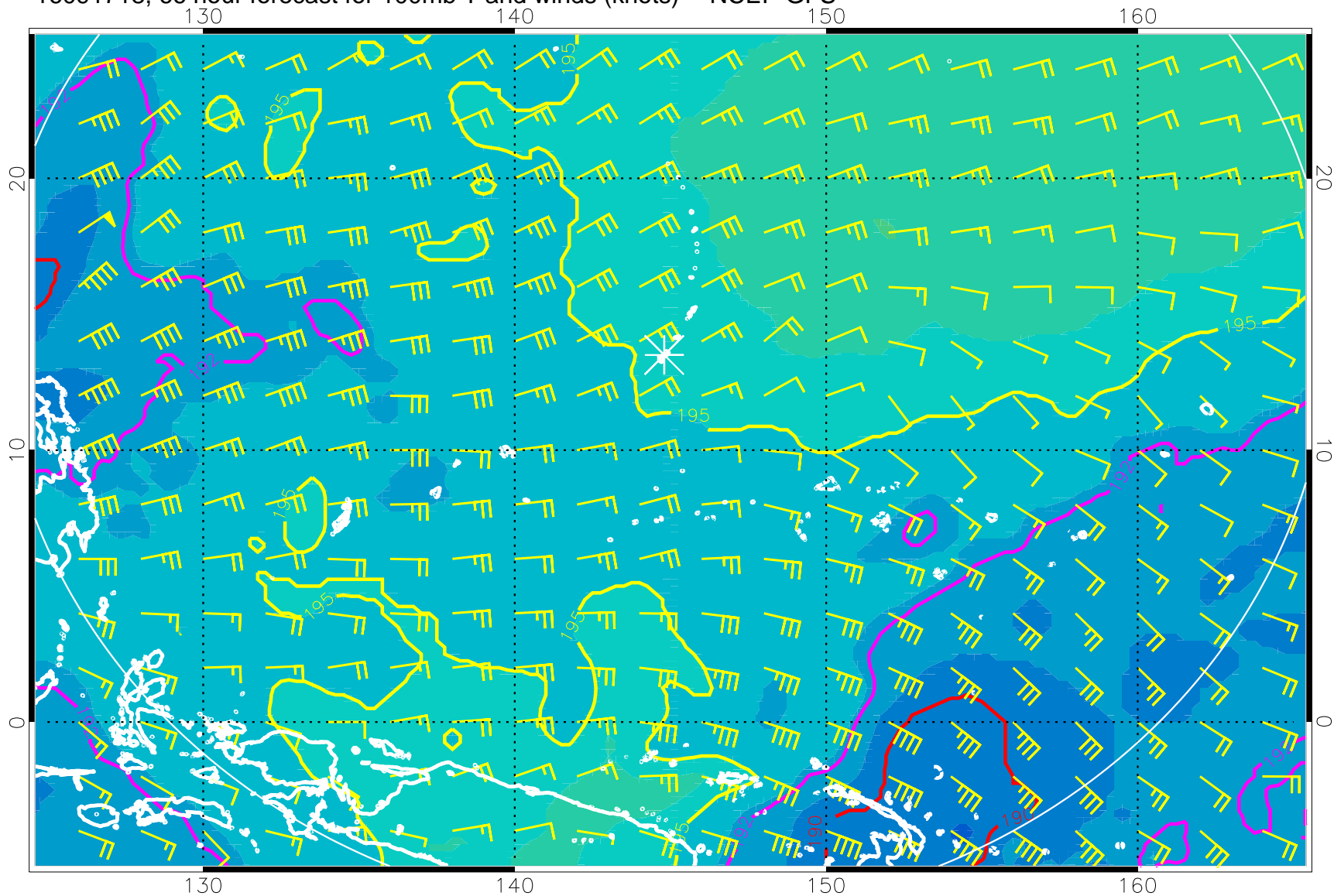
16091718, 66 hour forecast for 100mb T and winds (knots) -- NCEP GFS
