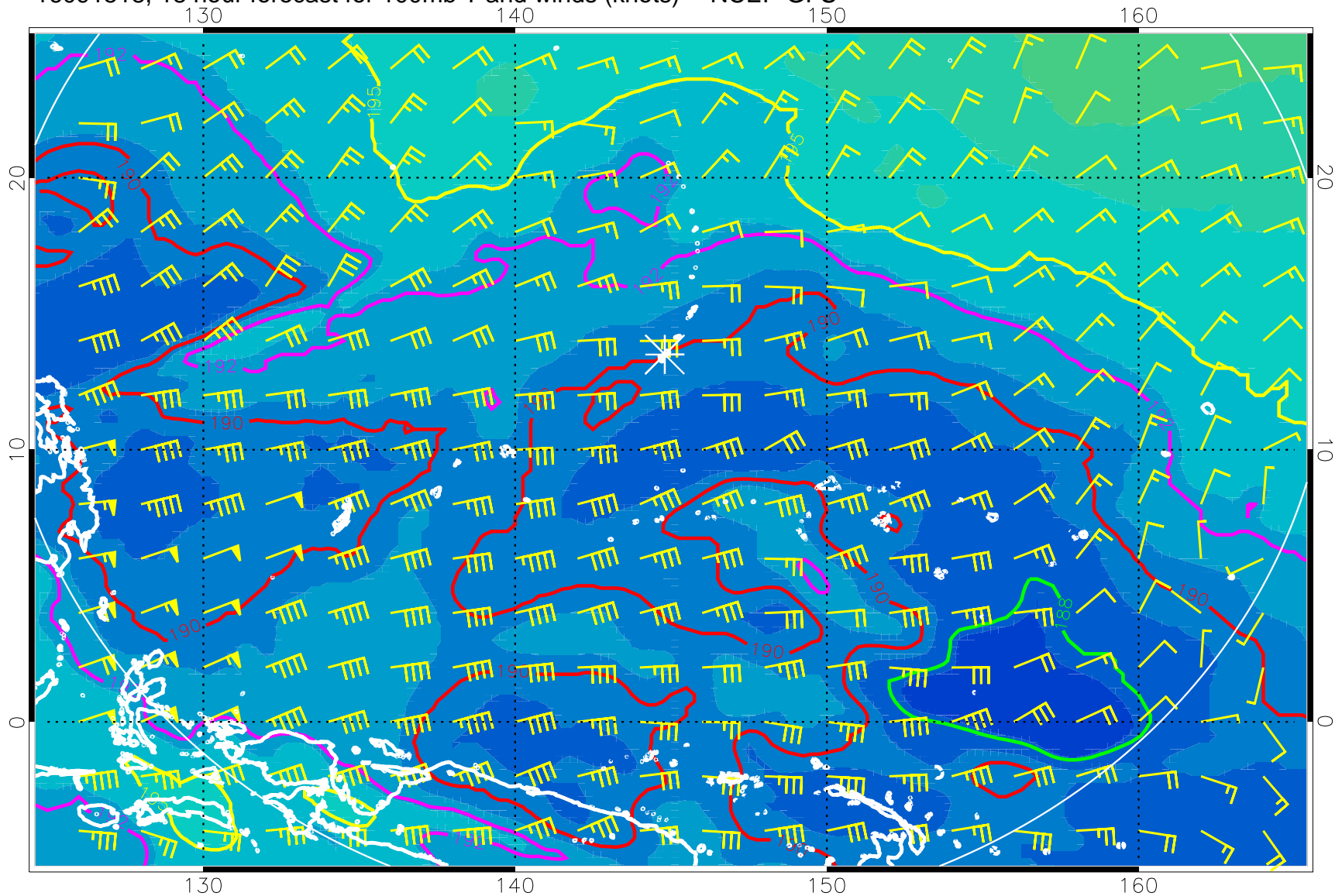
16091518, 18 hour forecast for 100mb T and winds (knots) -- NCEP GFS
