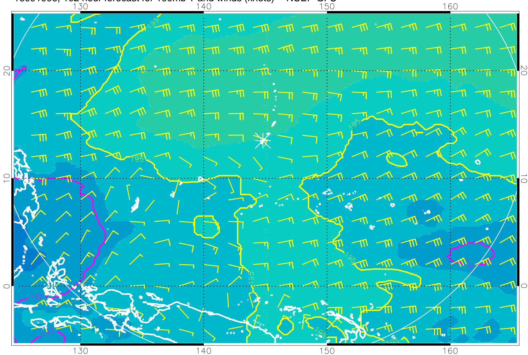
16091906, 102 hour forecast for 100mb T and winds (knots) -- NCEP GFS
