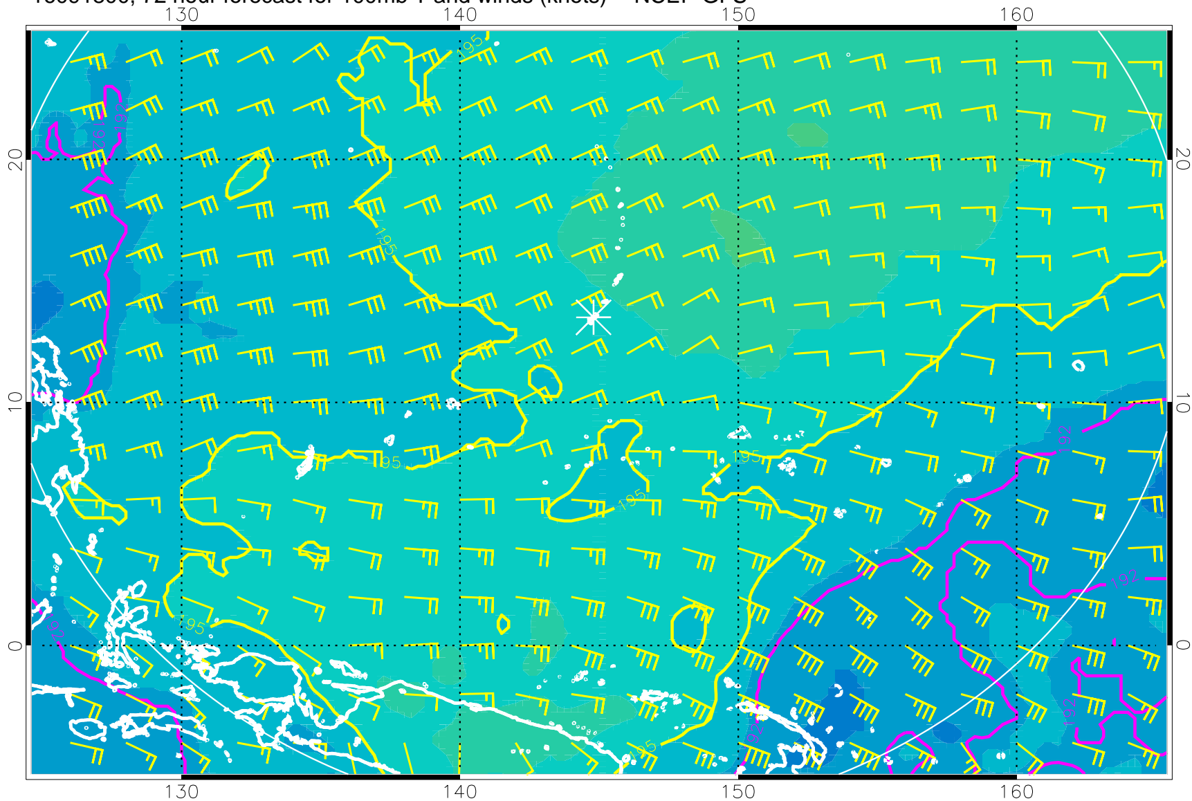
16091800, 72 hour forecast for 100mb T and winds (knots) -- NCEP GFS
