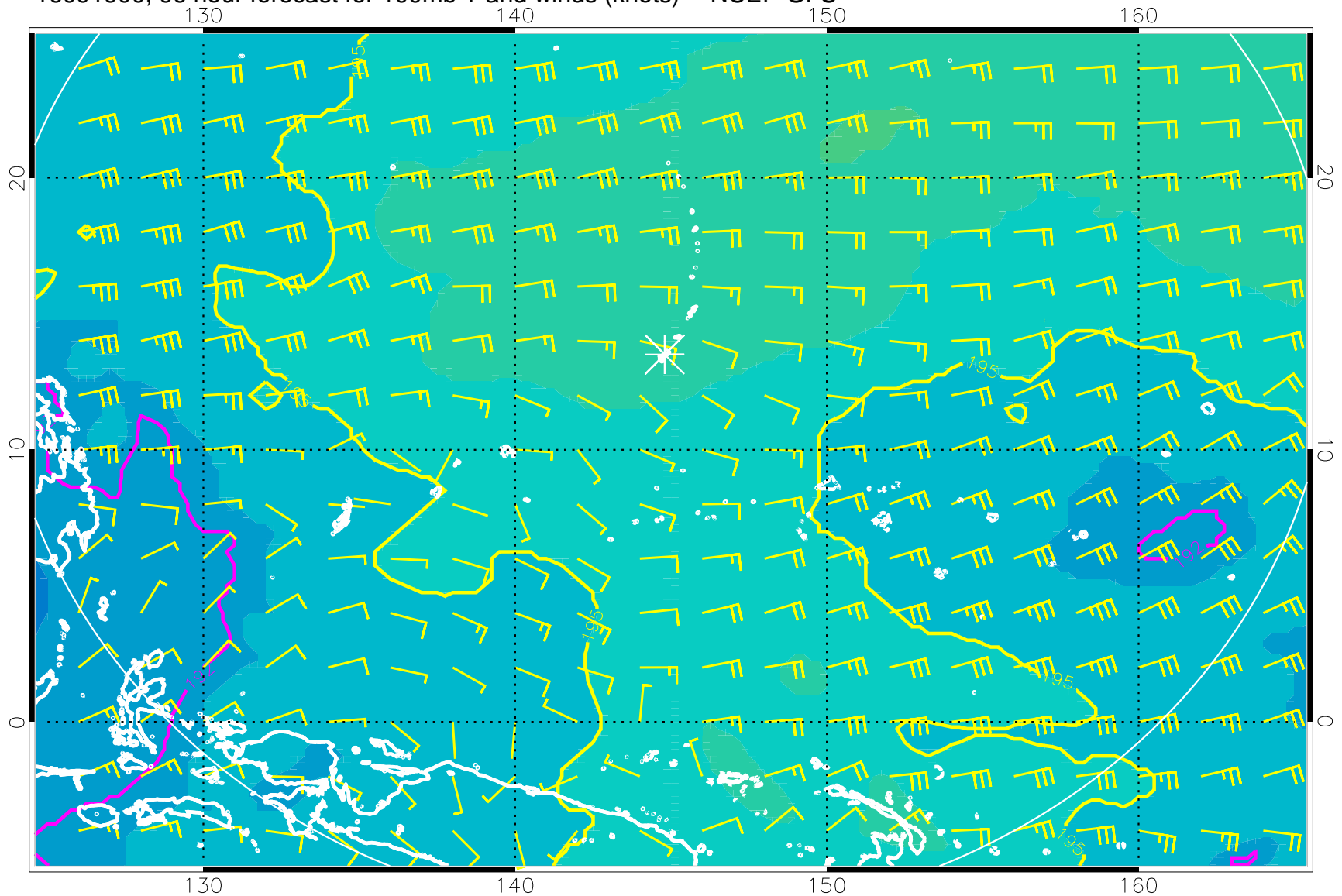
16091900, 96 hour forecast for 100mb T and winds (knots) -- NCEP GFS
