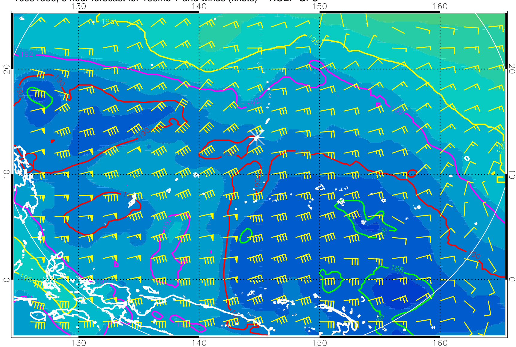
16091506, 6 hour forecast for 100mb T and winds (knots) -- NCEP GFS
