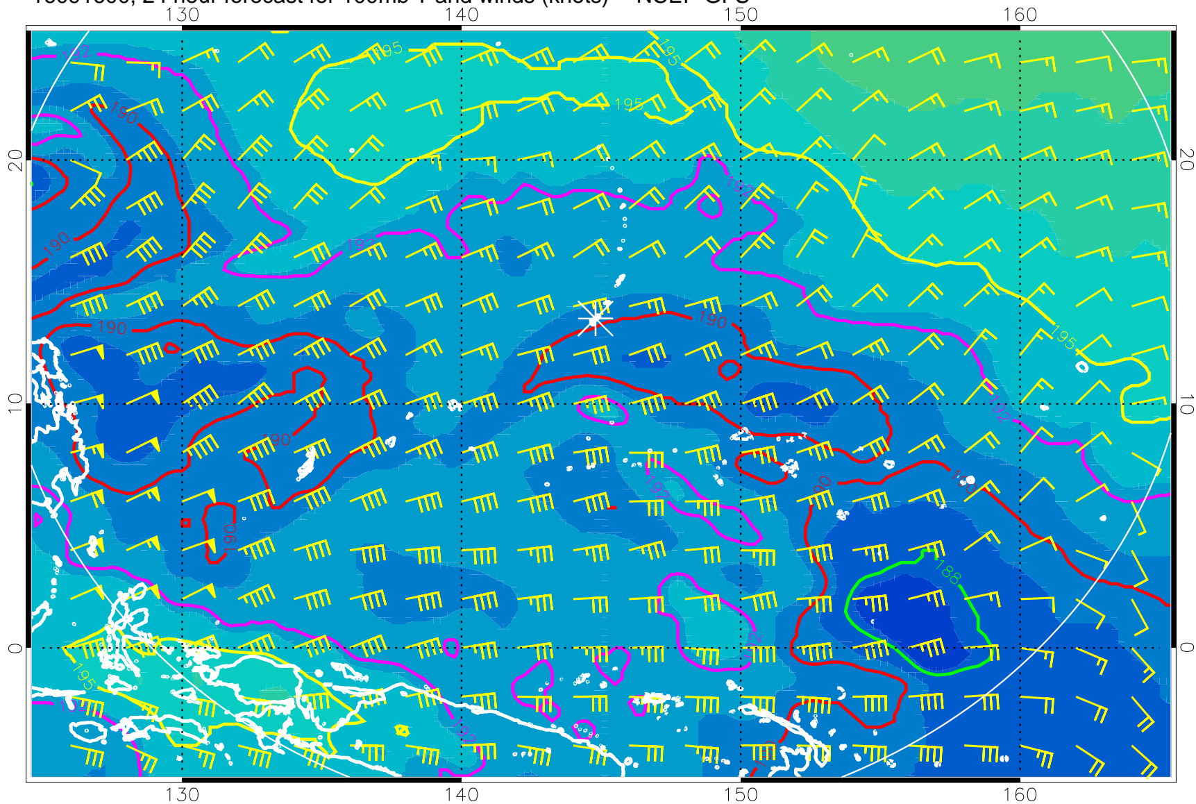
16091600, 24 hour forecast for 100mb T and winds (knots) -- NCEP GFS
