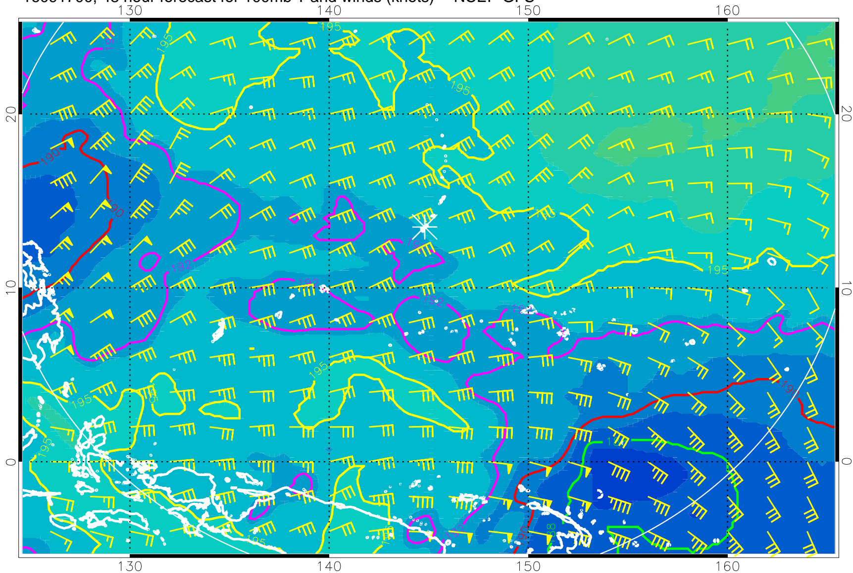
16091700, 48 hour forecast for 100mb T and winds (knots) -- NCEP GFS
