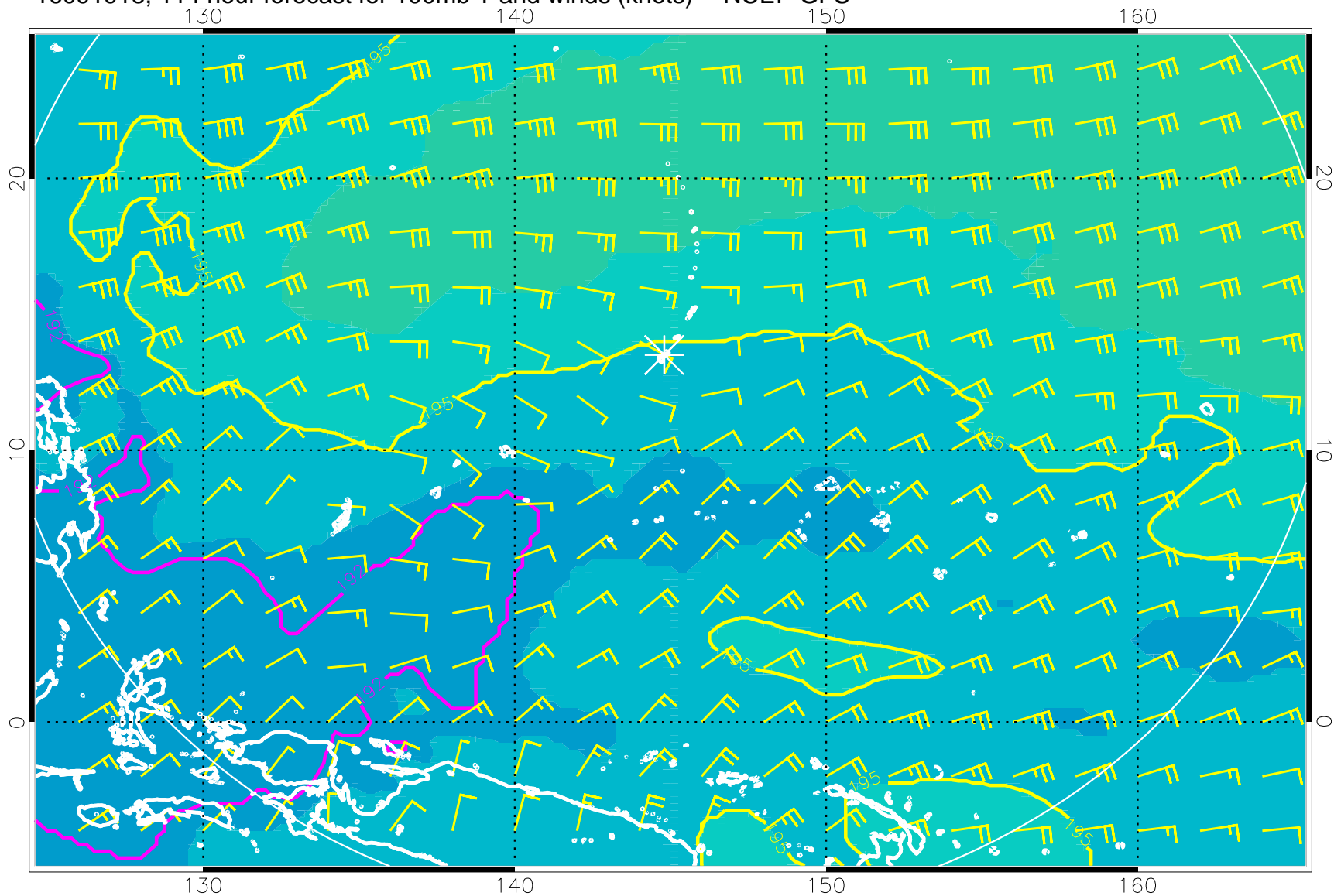
16091918, 114 hour forecast for 100mb T and winds (knots) -- NCEP GFS
