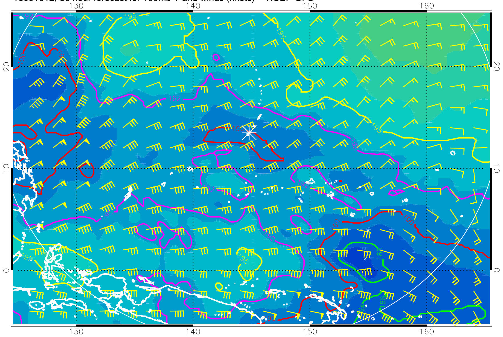
16091612, 36 hour forecast for 100mb T and winds (knots) -- NCEP GFS
