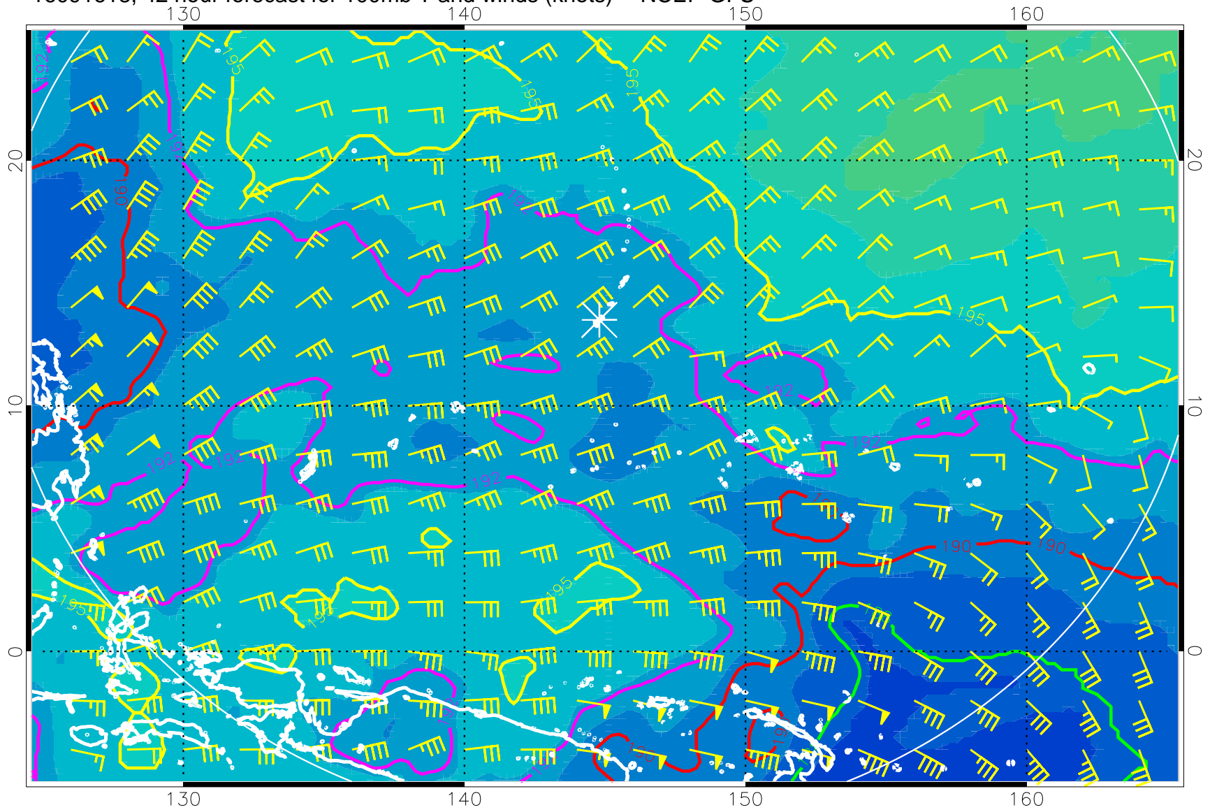
16091618, 42 hour forecast for 100mb T and winds (knots) -- NCEP GFS
