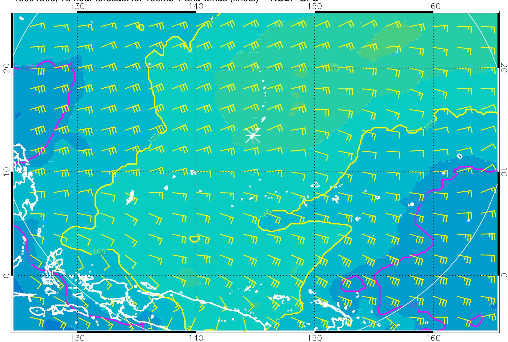
16091806, 78 hour forecast for 100mb T and winds (knots) -- NCEP GFS
