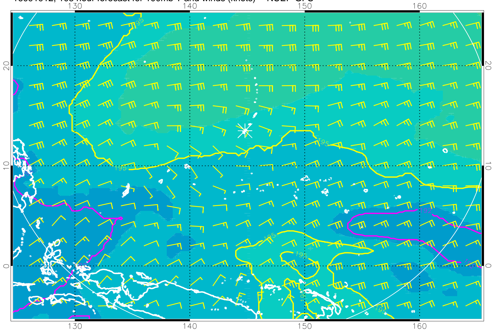
16091912, 108 hour forecast for 100mb T and winds (knots) -- NCEP GFS
