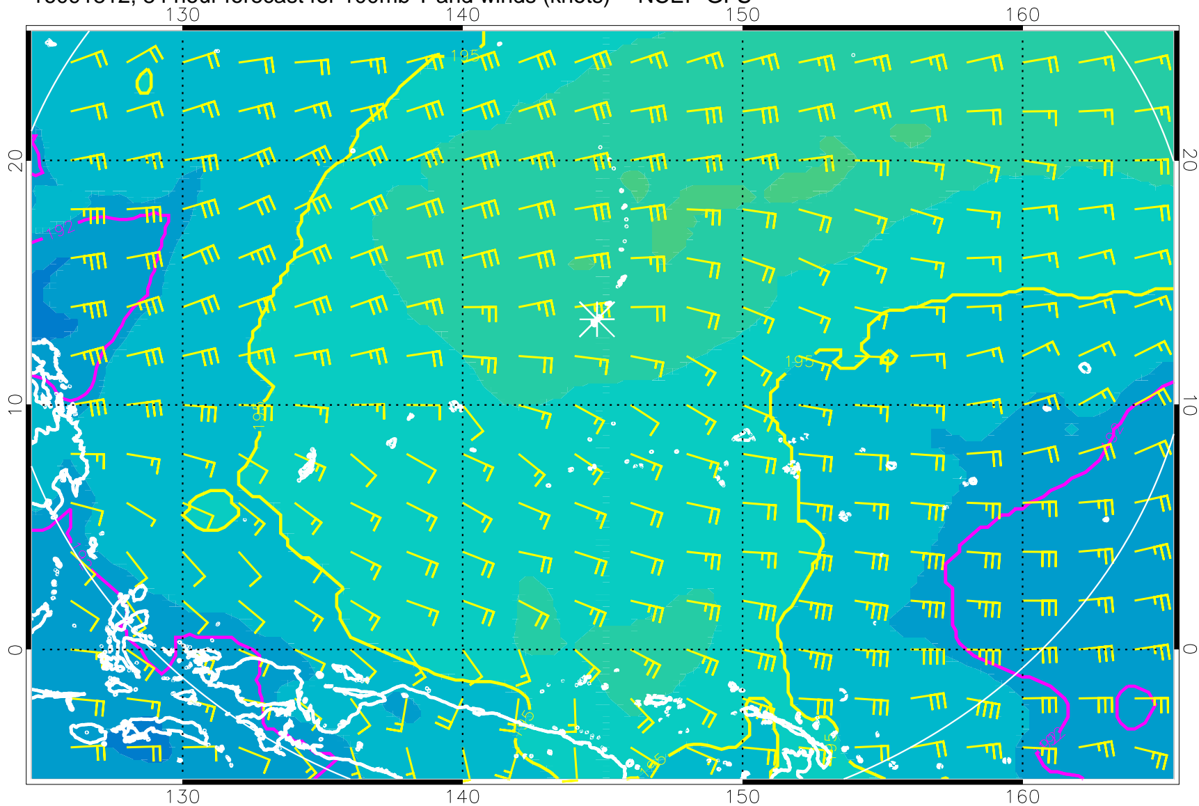
16091812, 84 hour forecast for 100mb T and winds (knots) -- NCEP GFS
