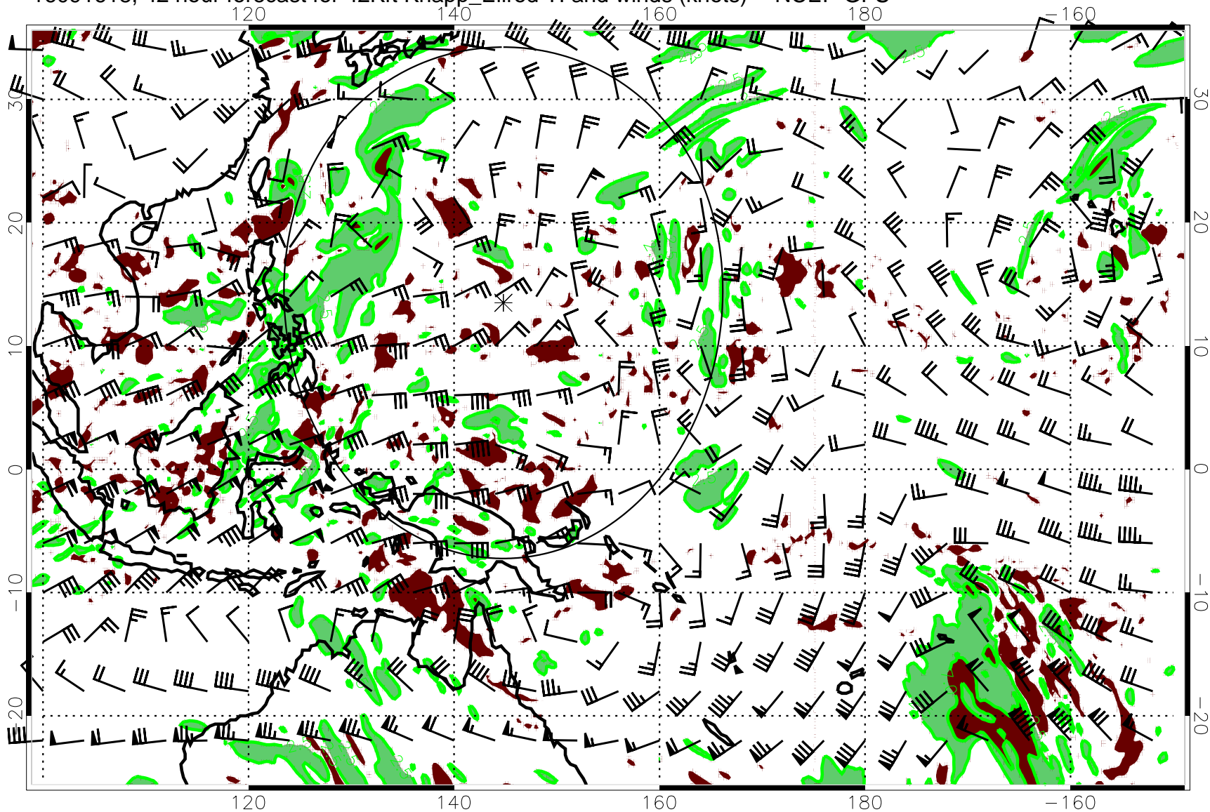
16091618, 42 hour forecast for 42Kft Knapp_Ellrod TI and winds (knots) -- NCEP GFS
