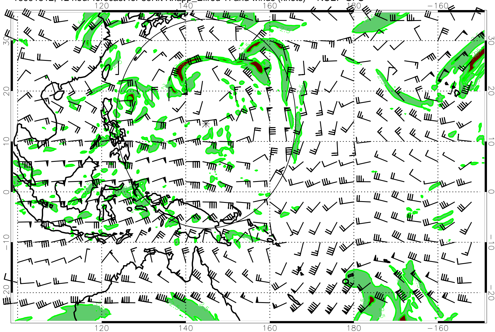
16091512, 12 hour forecast for 39Kft Knapp_Ellrod TI and winds (knots) -- NCEP GFS
