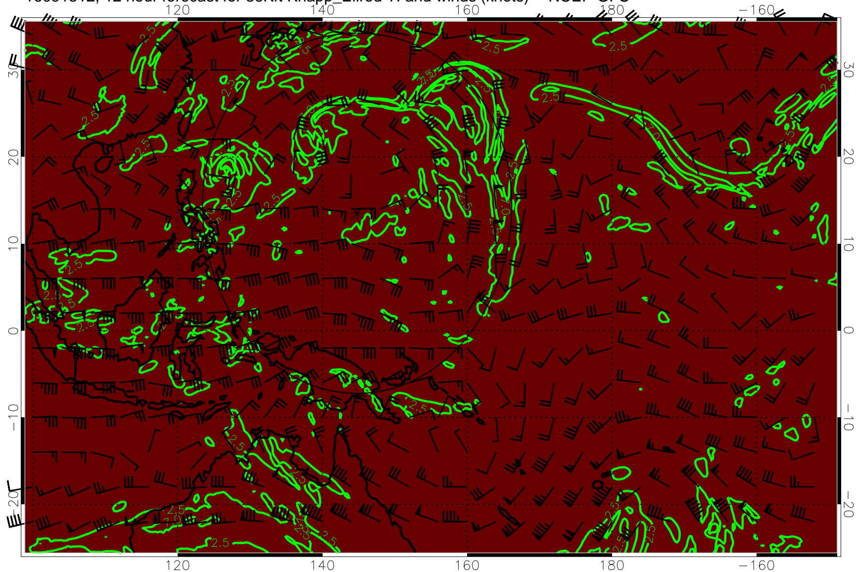
16091512, 12 hour forecast for 36Kft Knapp_Ellrod TI and winds (knots) -- NCEP GFS
