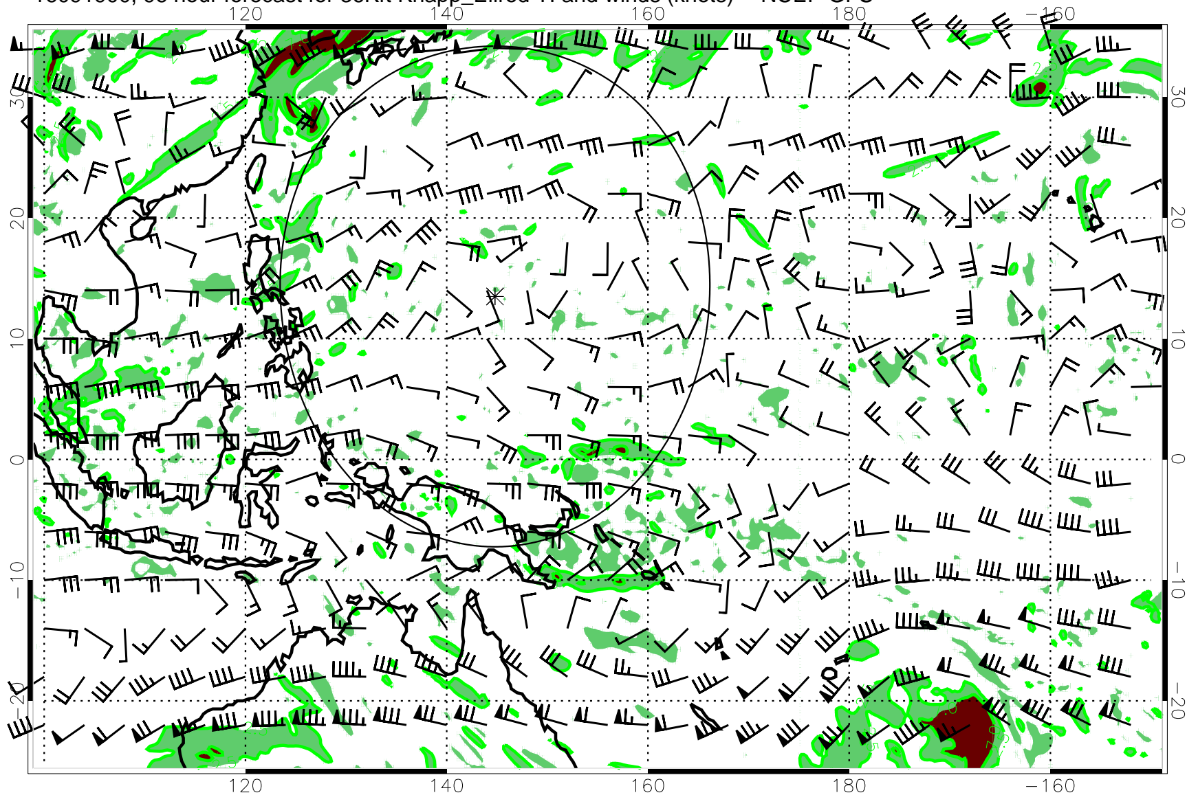
16091900, 96 hour forecast for 36Kft Knapp_Ellrod TI and winds (knots) -- NCEP GFS
